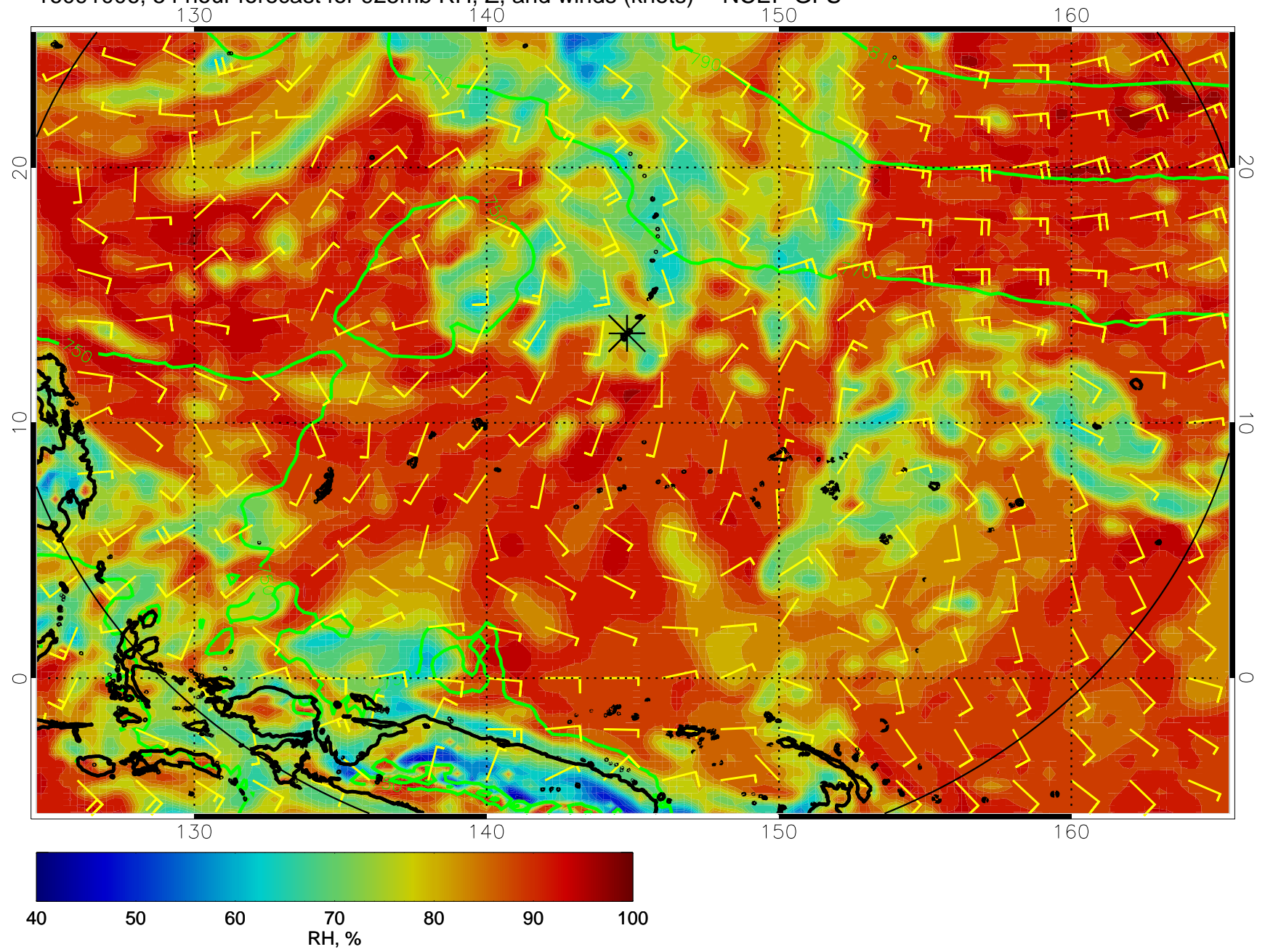
16091006, 54 hour forecast for 925mb RH, Z, and winds (knots) -- NCEP GFS
