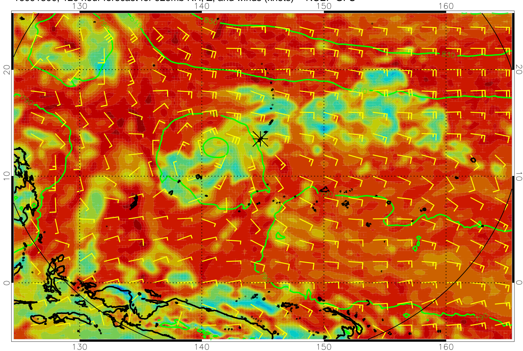
16091300, 120 hour forecast for 925mb RH, Z, and winds (knots) -- NCEP GFS
