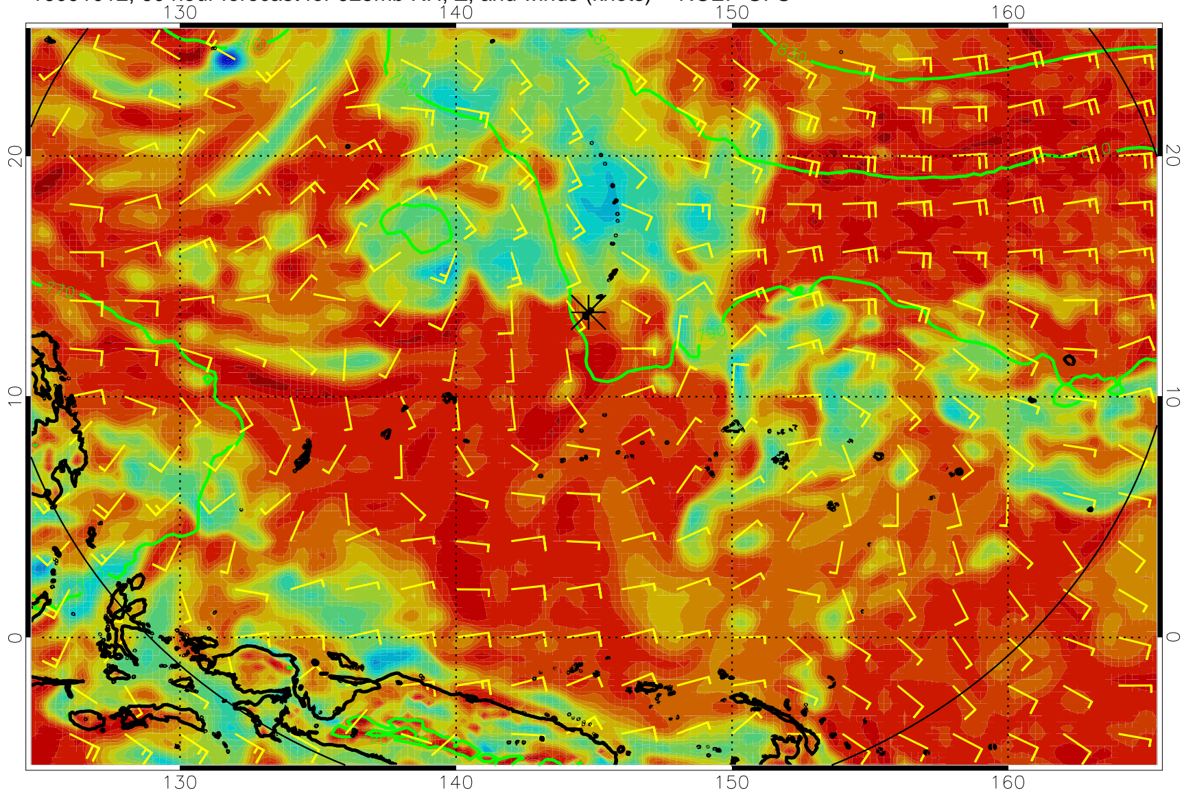
16091012, 60 hour forecast for 925mb RH, Z, and winds (knots) -- NCEP GFS
