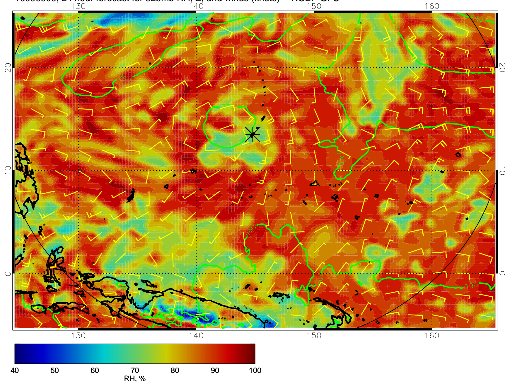
16090900, 24 hour forecast for 925mb RH, Z, and winds (knots) -- NCEP GFS
