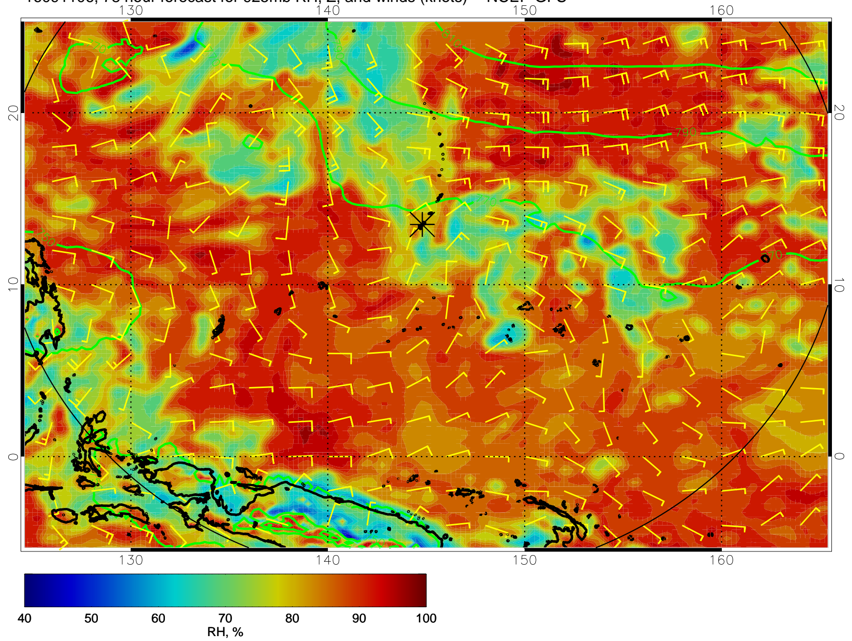
16091106, 78 hour forecast for 925mb RH, Z, and winds (knots) -- NCEP GFS
