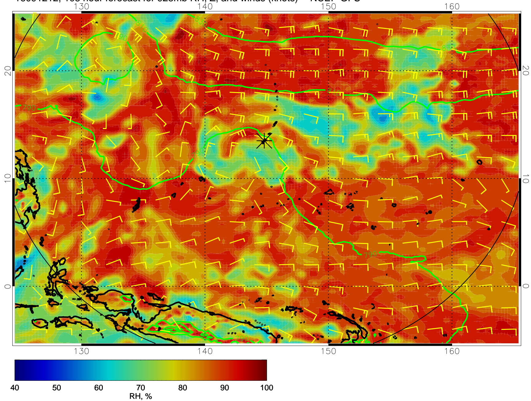
16091212, 108 hour forecast for 925mb RH, Z, and winds (knots) -- NCEP GFS
