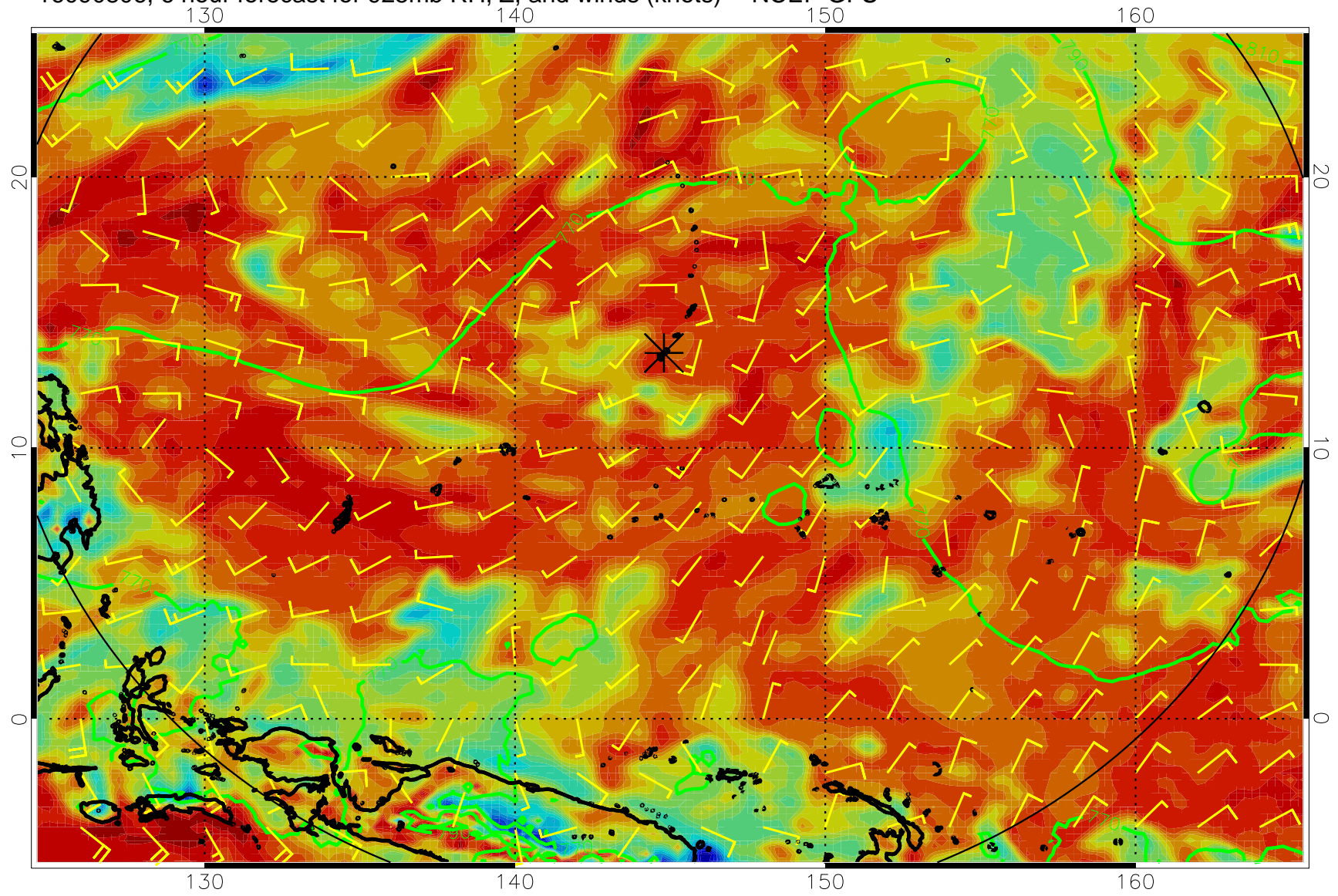
16090806, 6 hour forecast for 925mb RH, Z, and winds (knots) -- NCEP GFS
