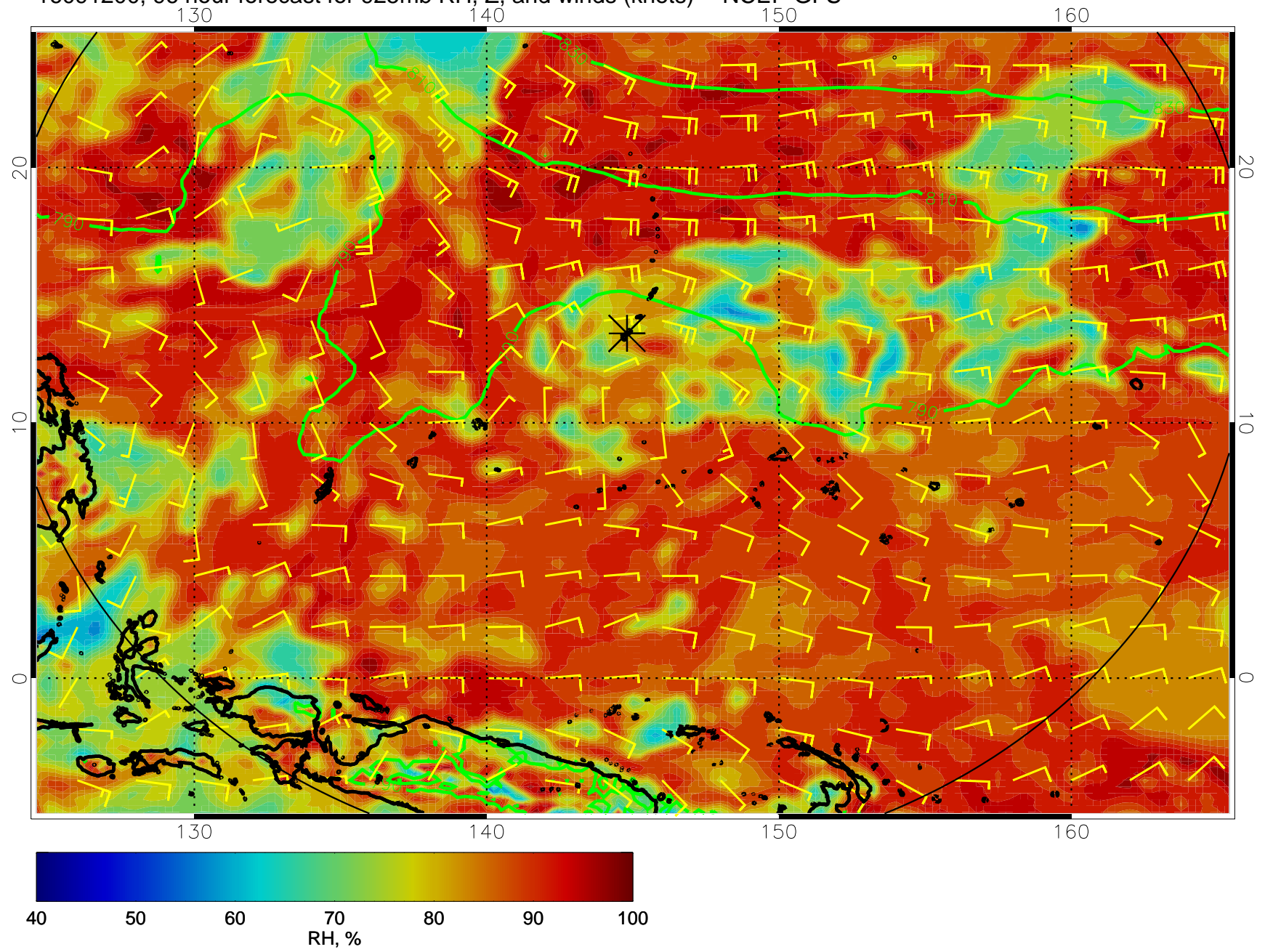
16091200, 96 hour forecast for 925mb RH, Z, and winds (knots) -- NCEP GFS
