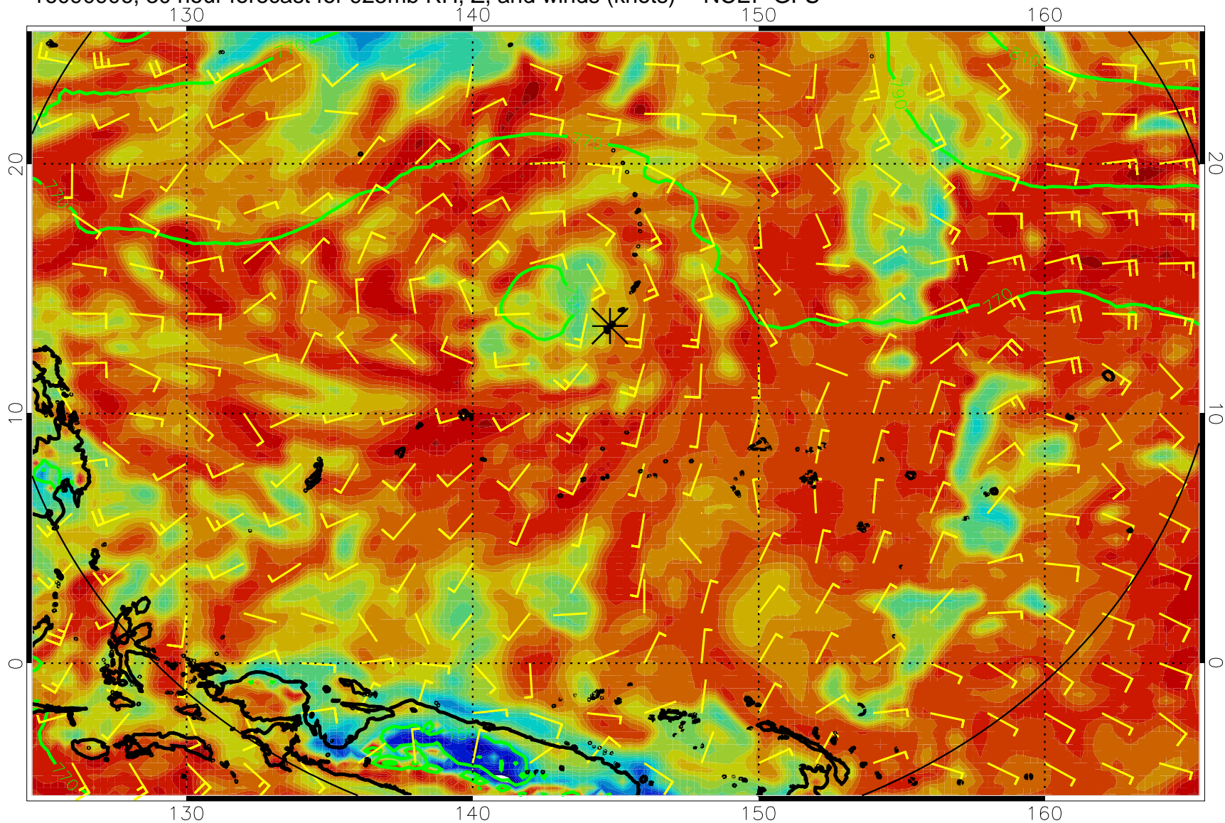
16090906, 30 hour forecast for 925mb RH, Z, and winds (knots) -- NCEP GFS
