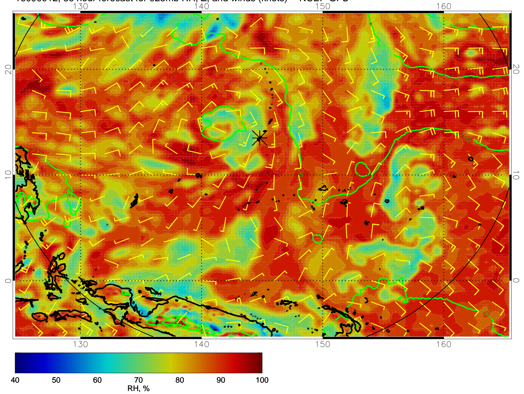
16090912, 36 hour forecast for 925mb RH, Z, and winds (knots) -- NCEP GFS
