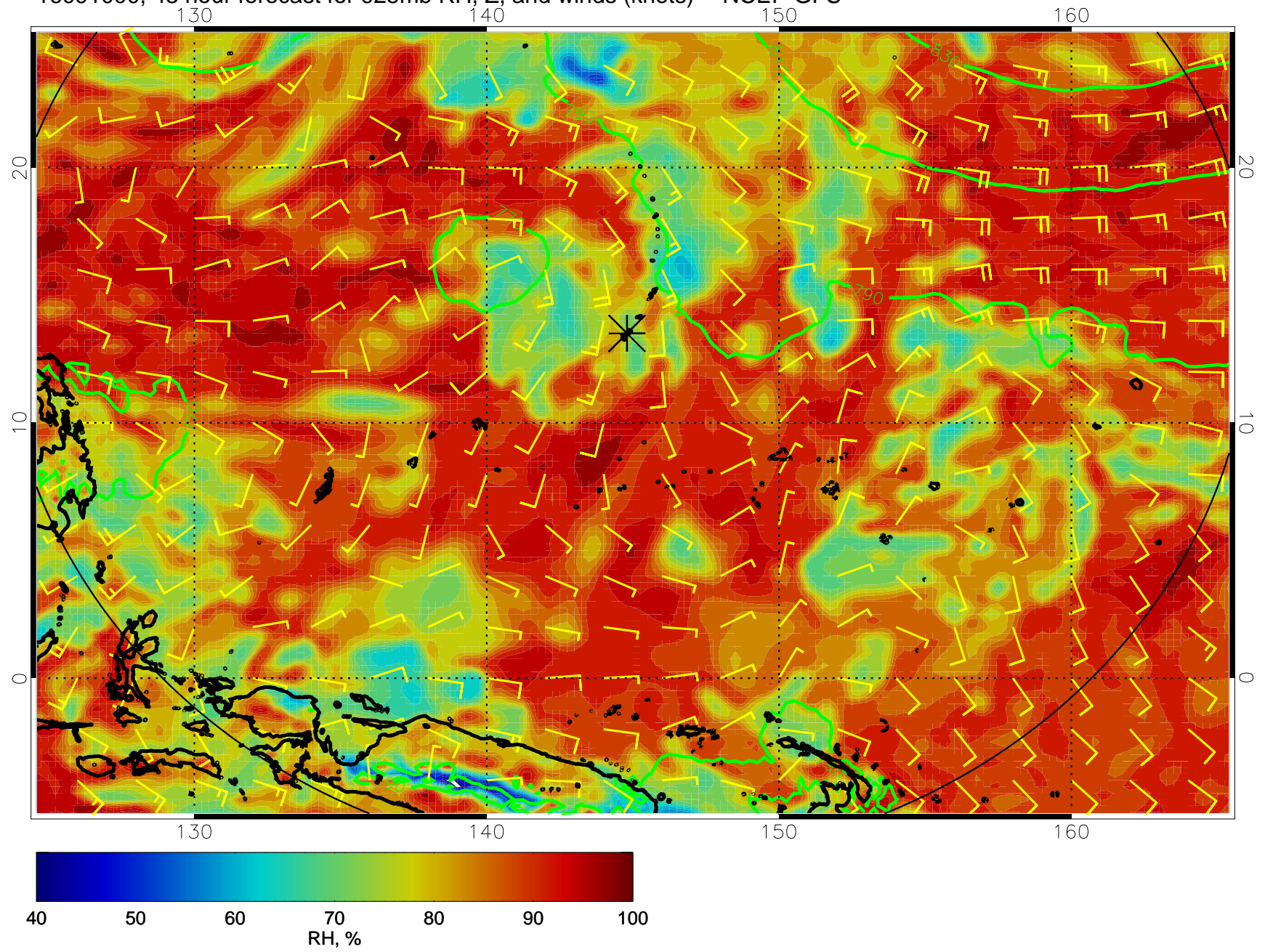
16091000, 48 hour forecast for 925mb RH, Z, and winds (knots) -- NCEP GFS
