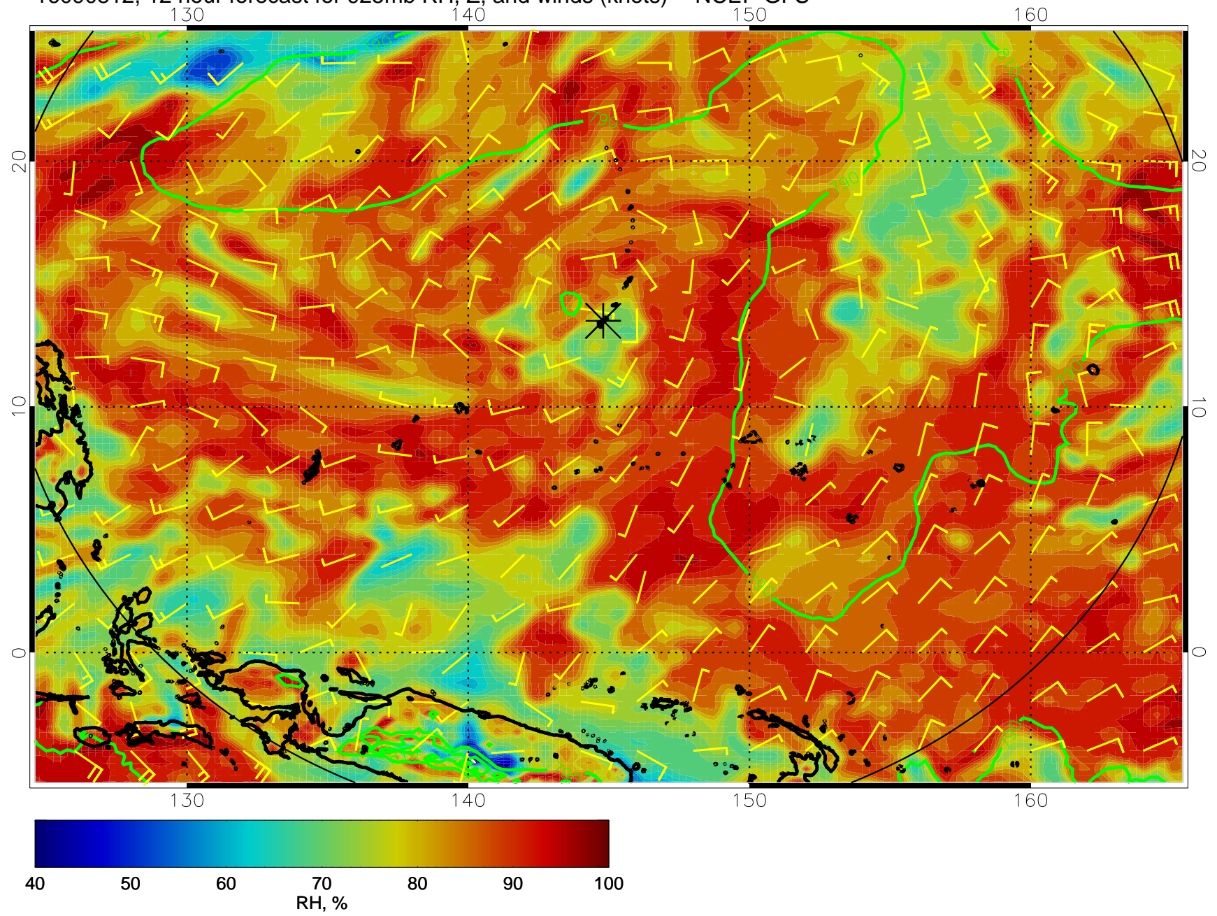
16090812, 12 hour forecast for 925mb RH, Z, and winds (knots) -- NCEP GFS
