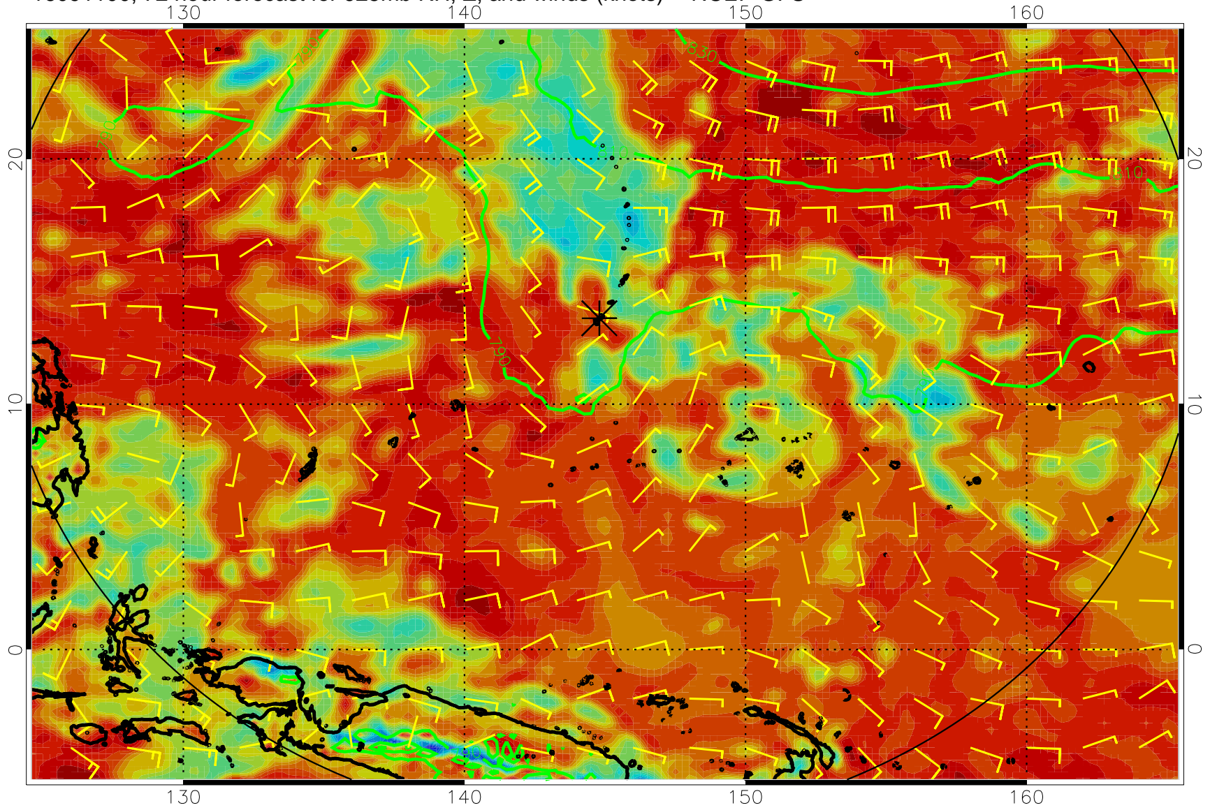
16091100, 72 hour forecast for 925mb RH, Z, and winds (knots) -- NCEP GFS
