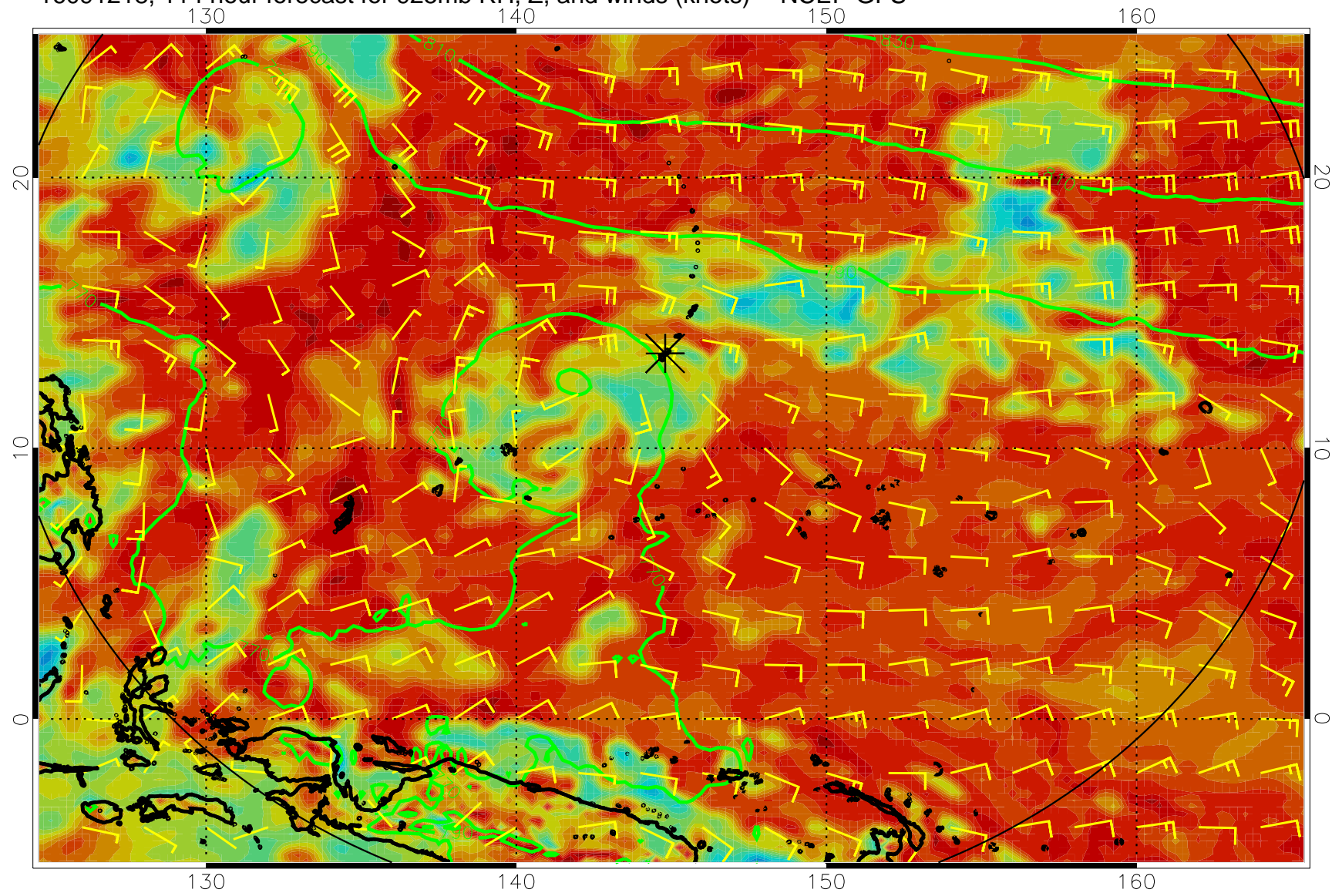
16091218, 114 hour forecast for 925mb RH, Z, and winds (knots) -- NCEP GFS
