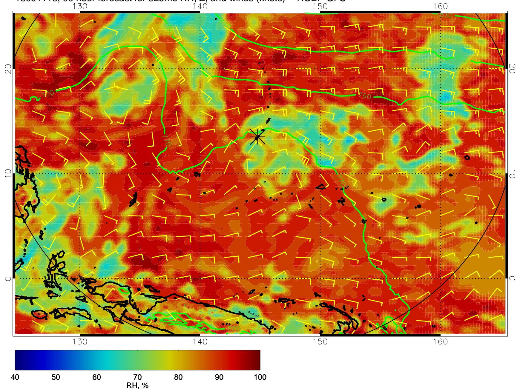
16091118, 90 hour forecast for 925mb RH, Z, and winds (knots) -- NCEP GFS
