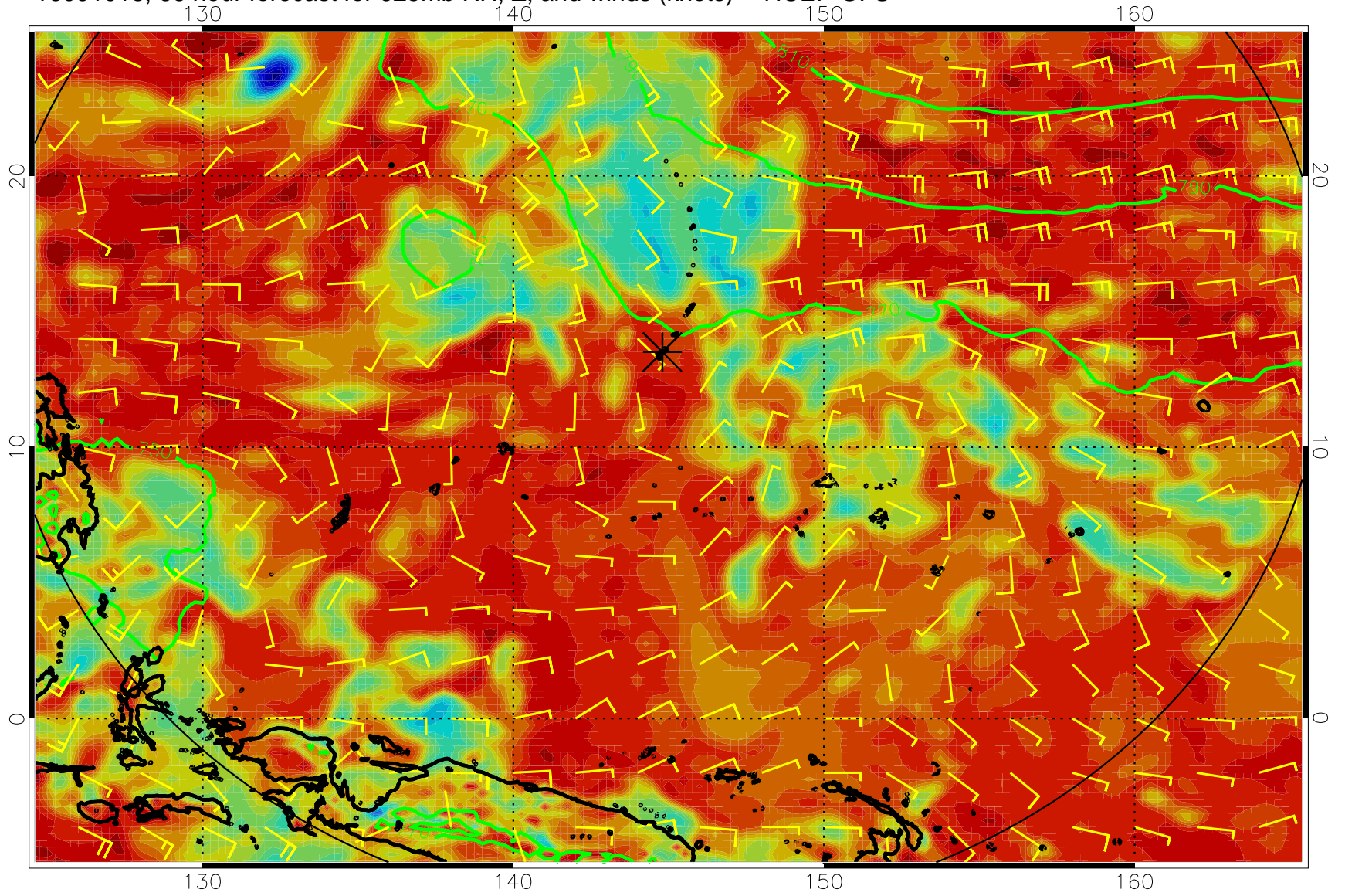
16091018, 66 hour forecast for 925mb RH, Z, and winds (knots) -- NCEP GFS
