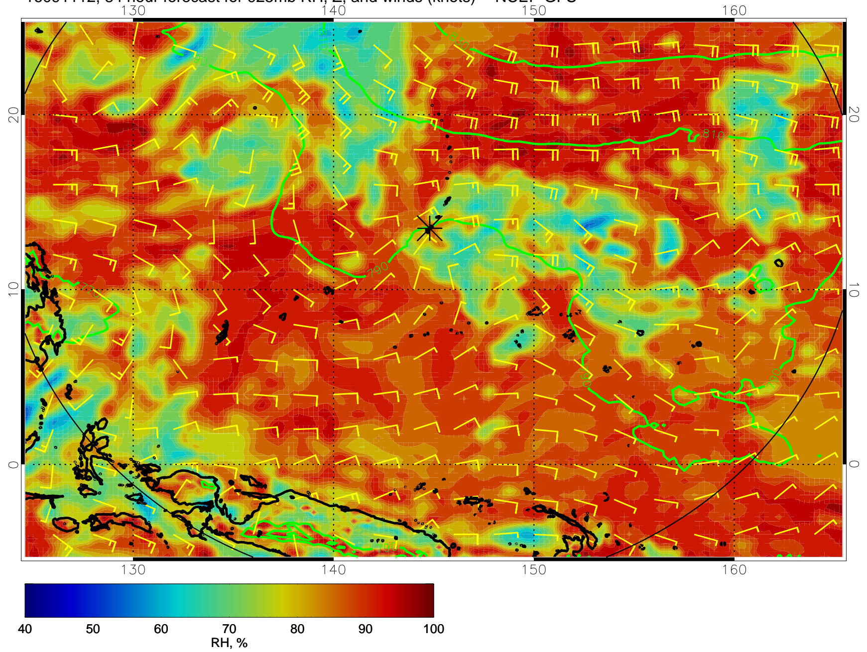
16091112, 84 hour forecast for 925mb RH, Z, and winds (knots) -- NCEP GFS
