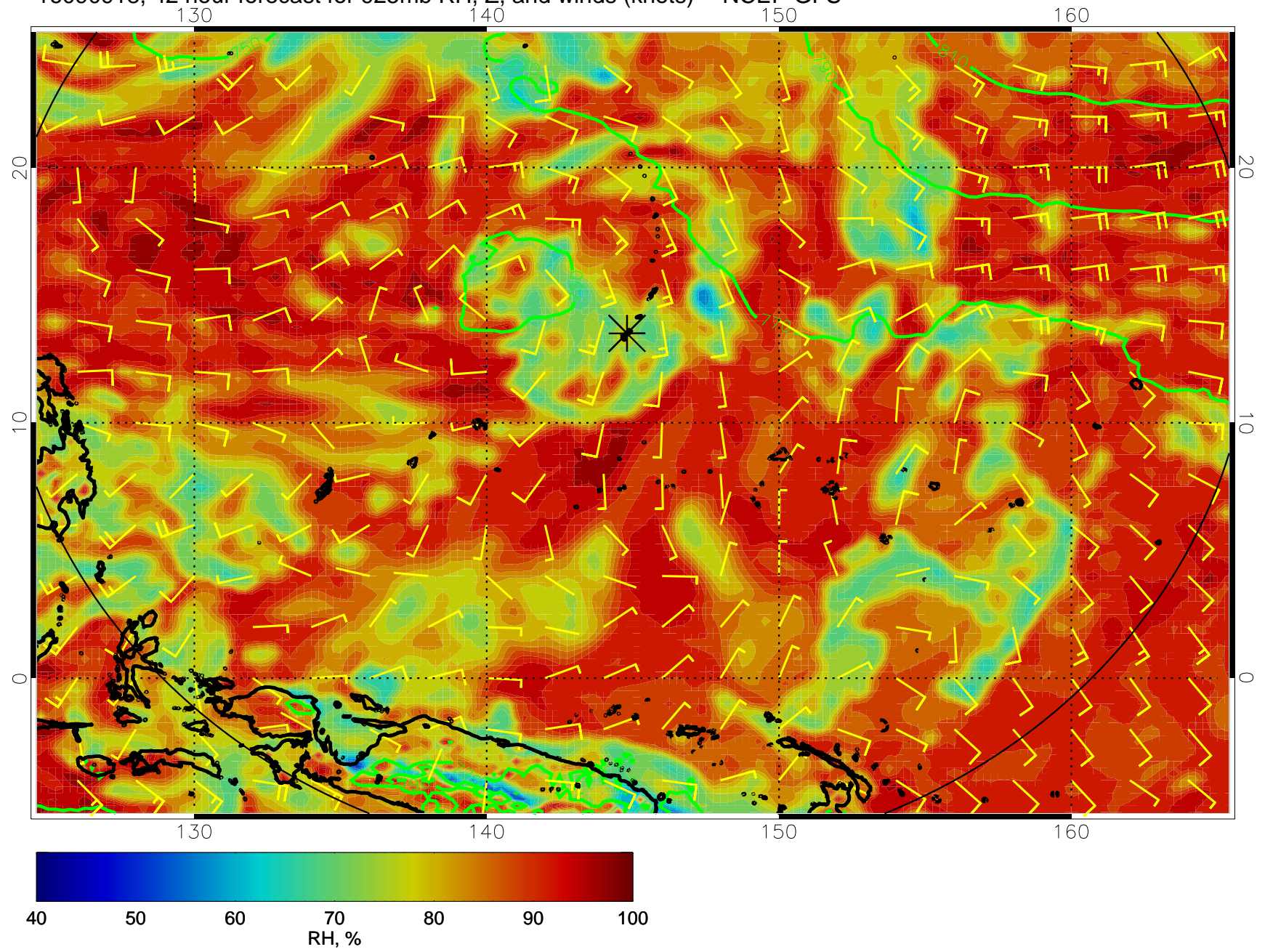
16090918, 42 hour forecast for 925mb RH, Z, and winds (knots) -- NCEP GFS
