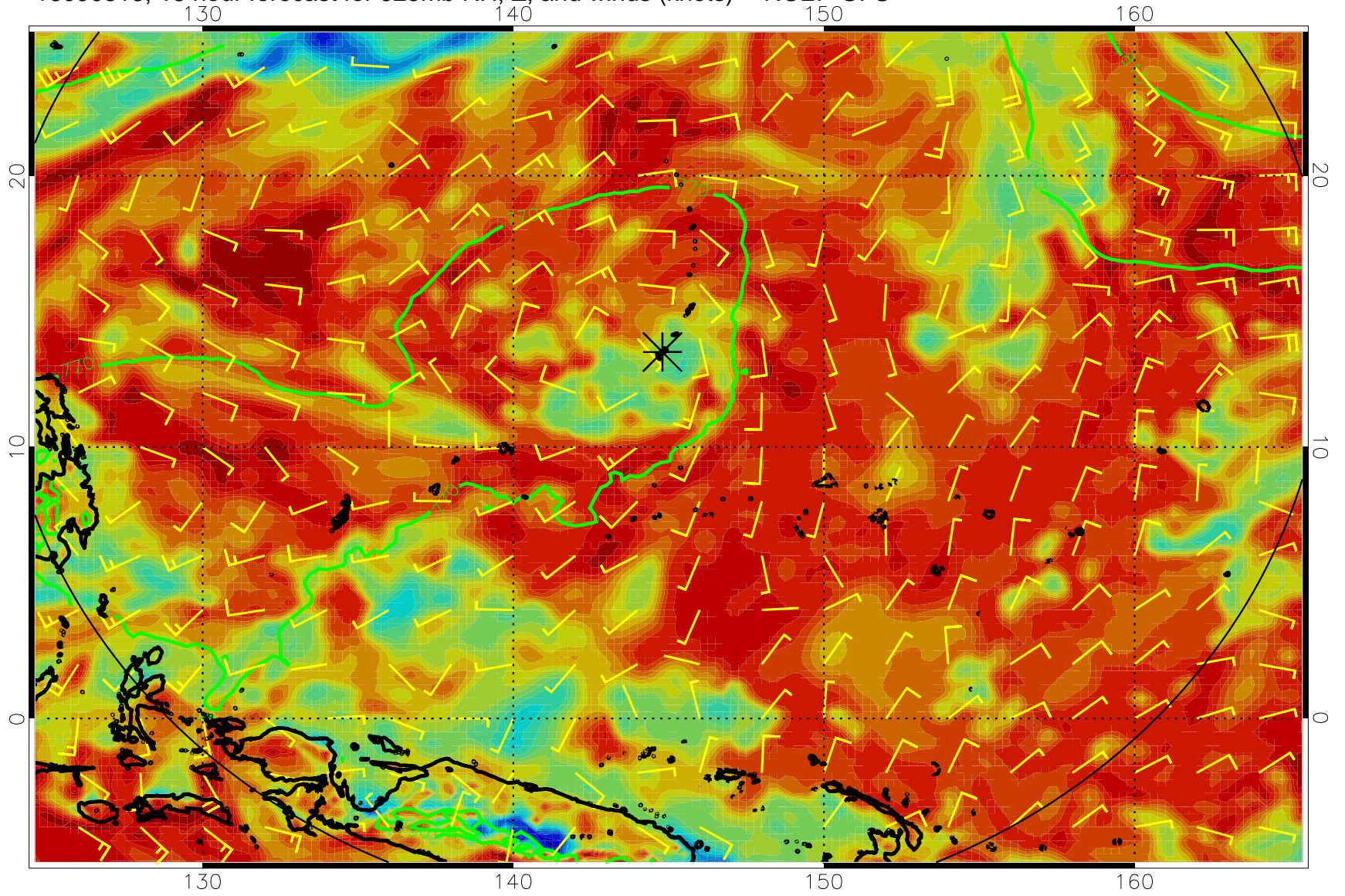
16090818, 18 hour forecast for 925mb RH, Z, and winds (knots) -- NCEP GFS
