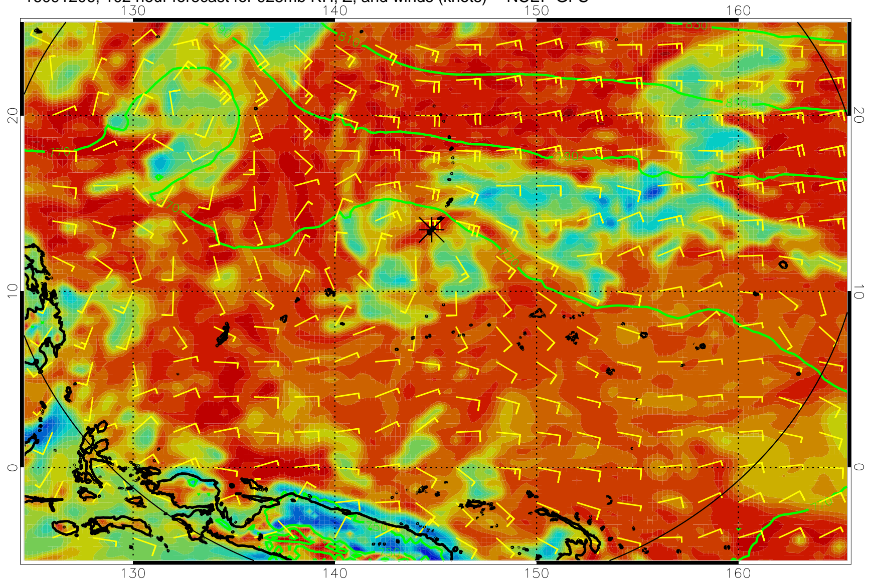
16091206, 102 hour forecast for 925mb RH, Z, and winds (knots) -- NCEP GFS
