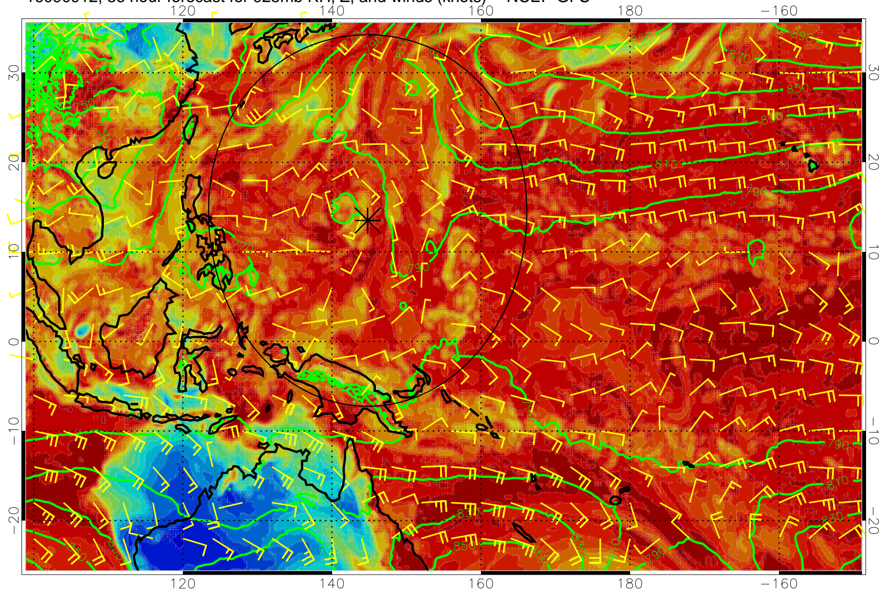
16090912, 36 hour forecast for 925mb RH, Z, and winds (knots) -- NCEP GFS
