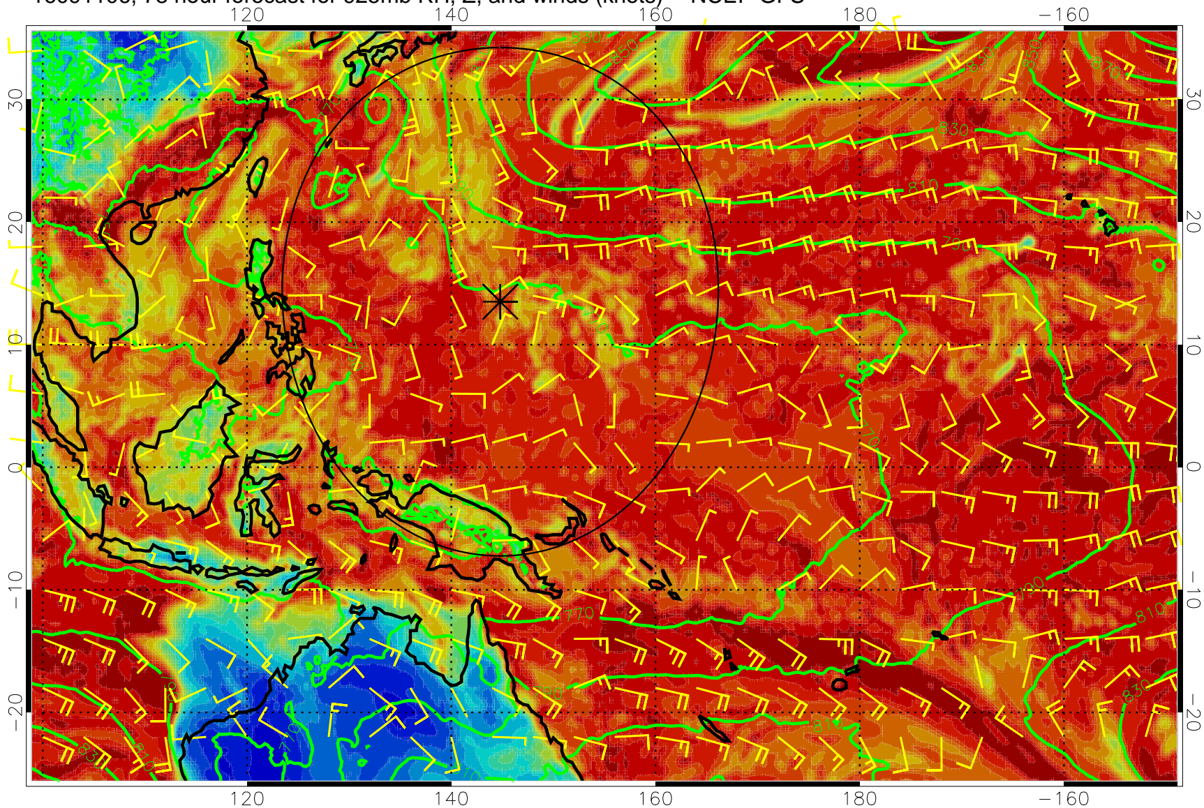
16091106, 78 hour forecast for 925mb RH, Z, and winds (knots) -- NCEP GFS
