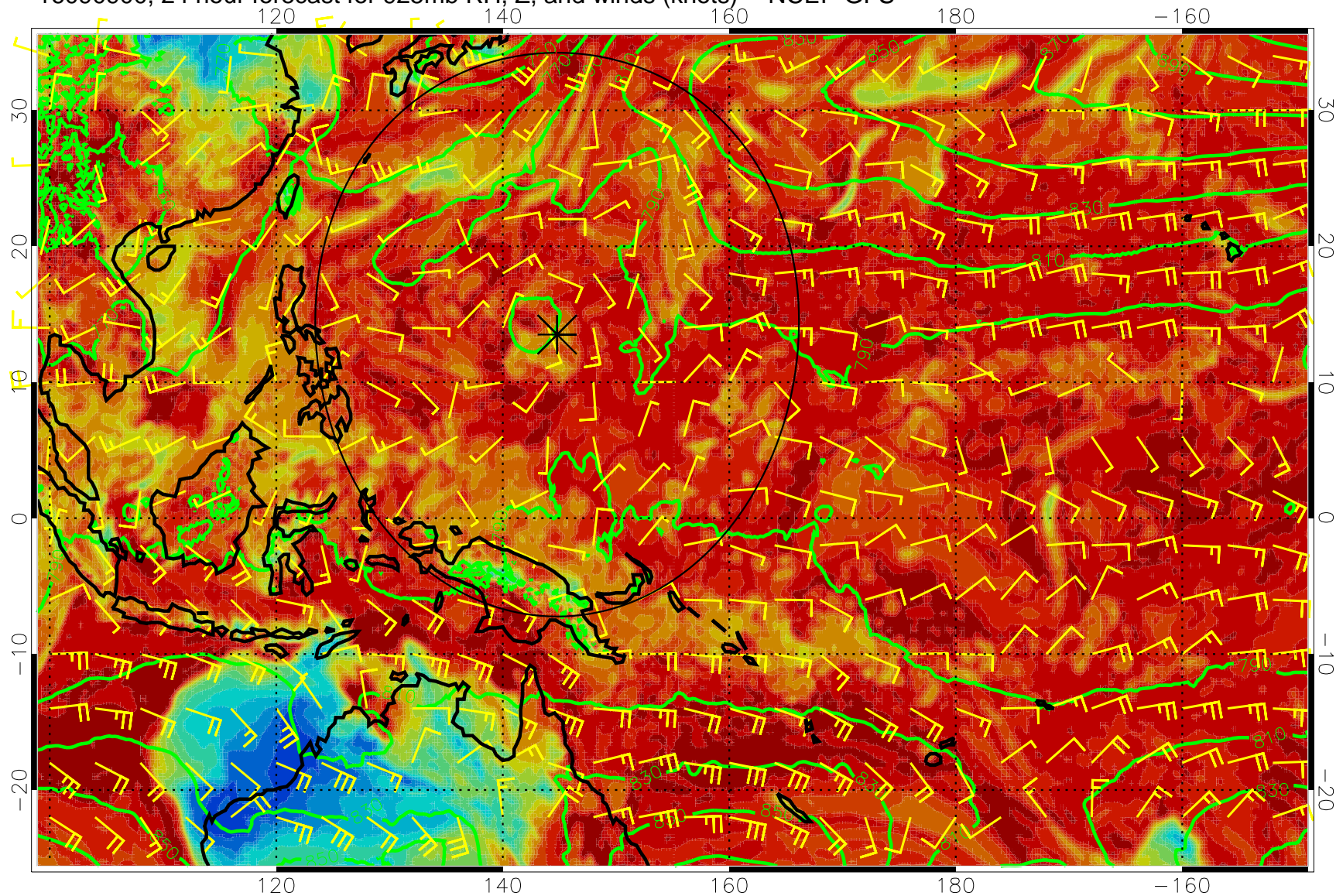
16090900, 24 hour forecast for 925mb RH, Z, and winds (knots) -- NCEP GFS
