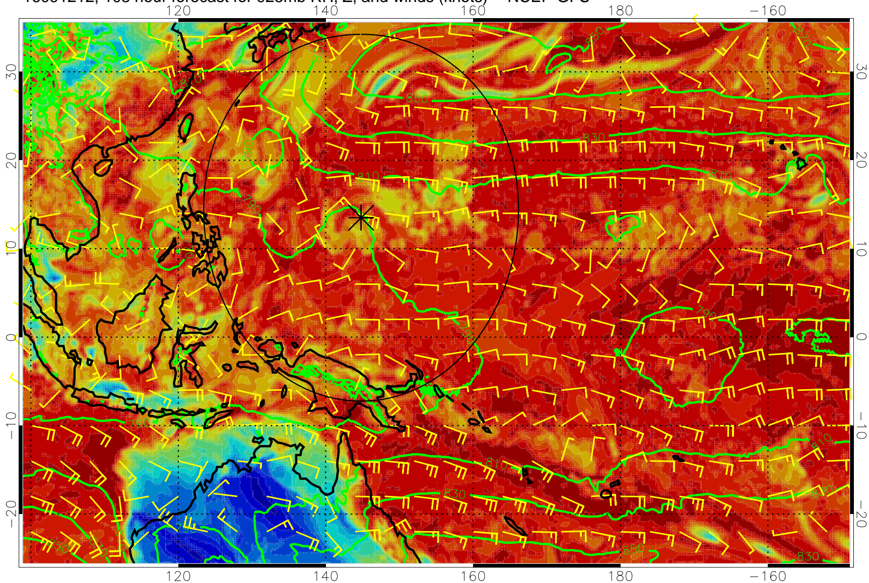
16091212, 108 hour forecast for 925mb RH, Z, and winds (knots) -- NCEP GFS
