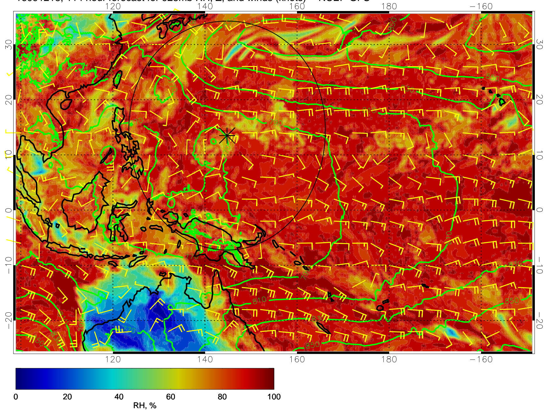
16091218, 114 hour forecast for 925mb RH, Z, and winds (knots) -- NCEP GFS
