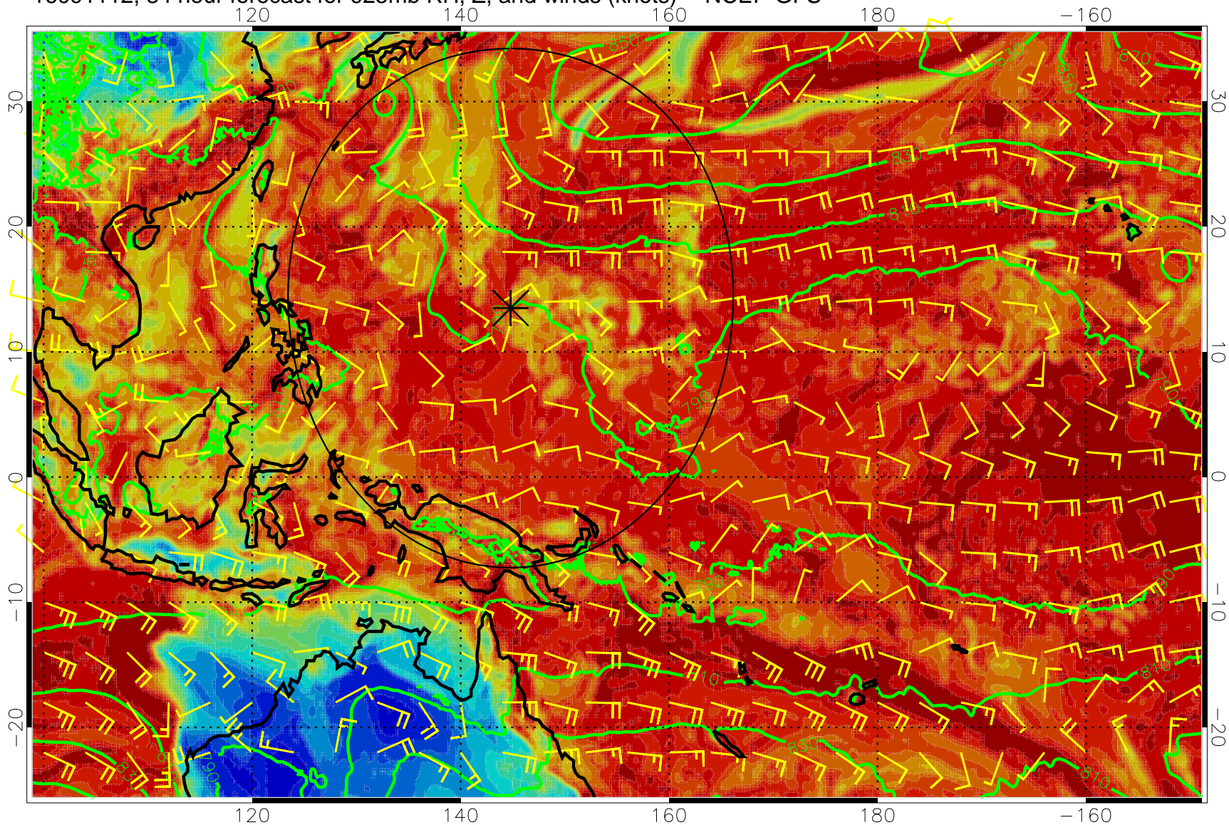
16091112, 84 hour forecast for 925mb RH, Z, and winds (knots) -- NCEP GFS
