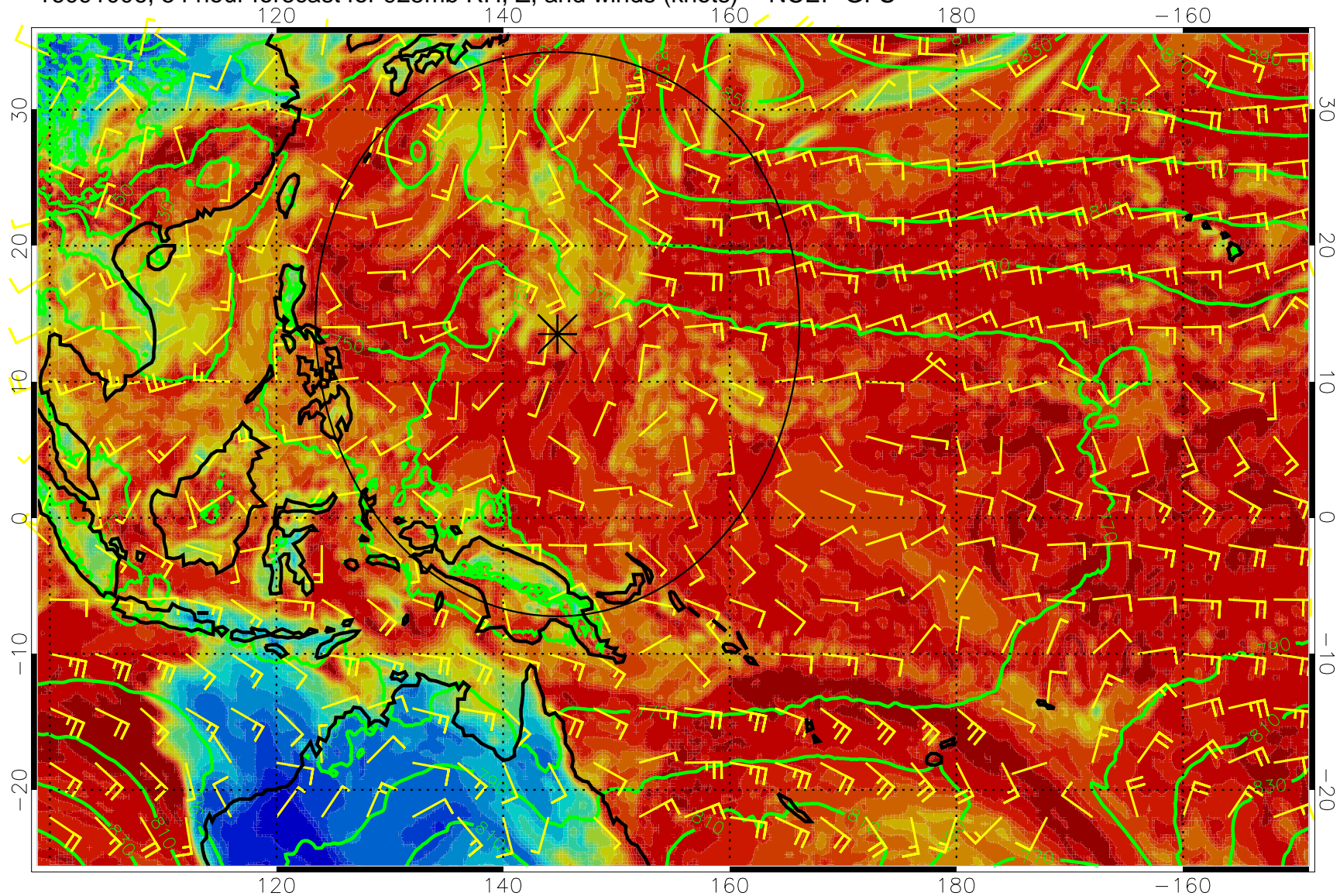
16091006, 54 hour forecast for 925mb RH, Z, and winds (knots) -- NCEP GFS
