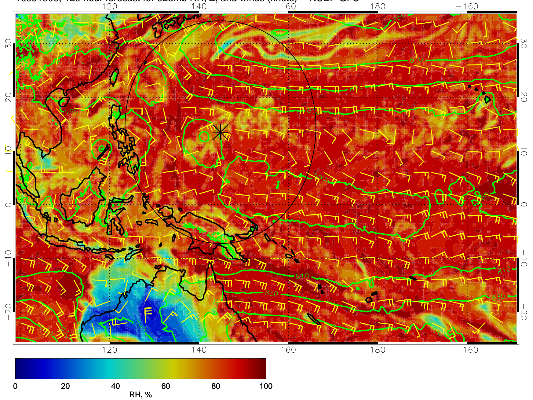
16091300, 120 hour forecast for 925mb RH, Z, and winds (knots) -- NCEP GFS
