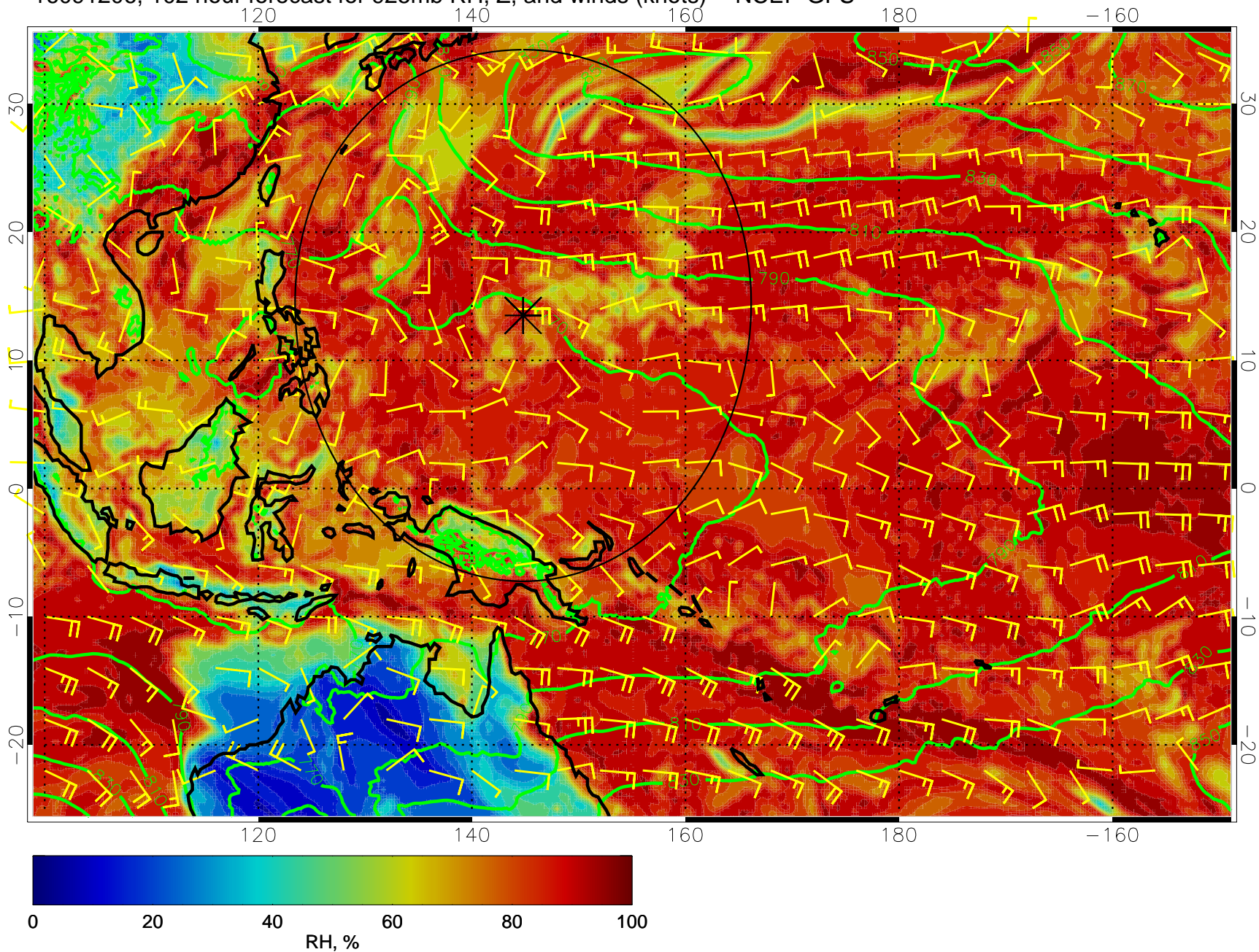
16091206, 102 hour forecast for 925mb RH, Z, and winds (knots) -- NCEP GFS
