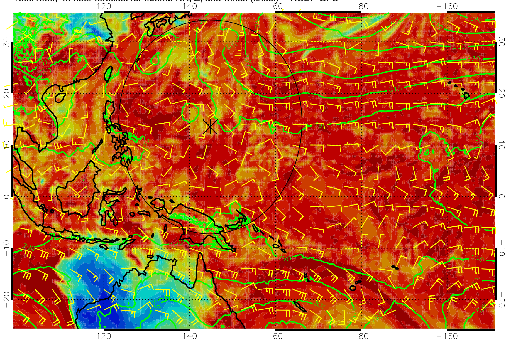
16091000, 48 hour forecast for 925mb RH, Z, and winds (knots) -- NCEP GFS
