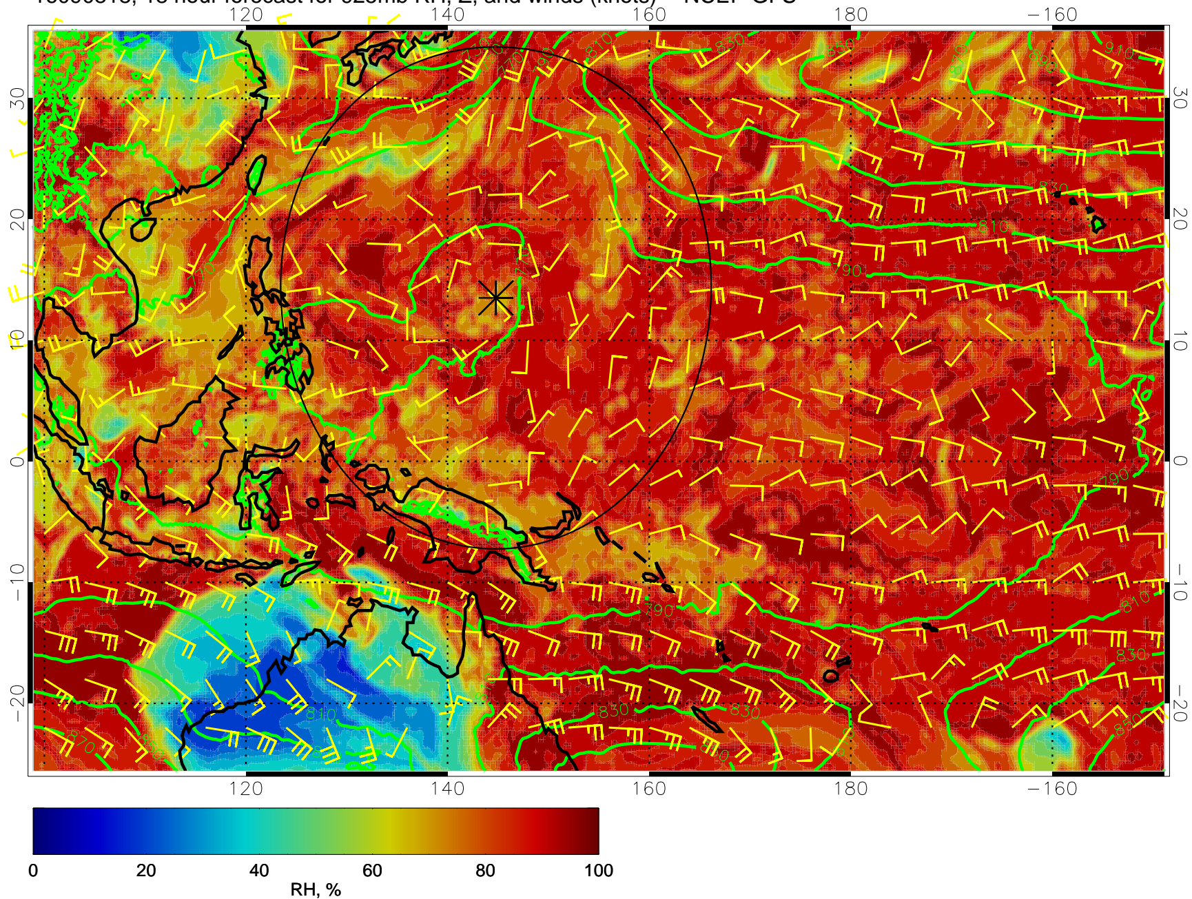
16090818, 18 hour forecast for 925mb RH, Z, and winds (knots) -- NCEP GFS
