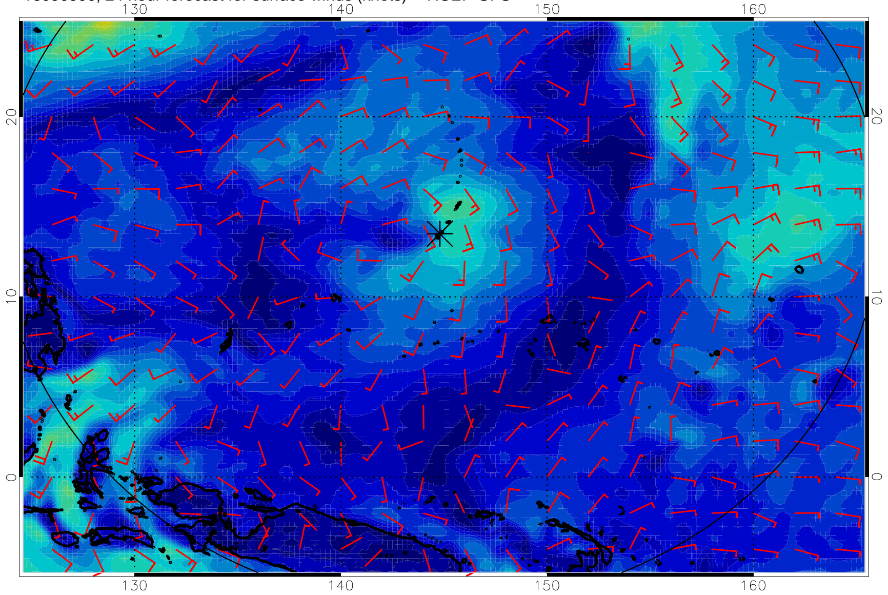
16090900, 24 hour forecast for surface winds (knots) -- NCEP GFS
