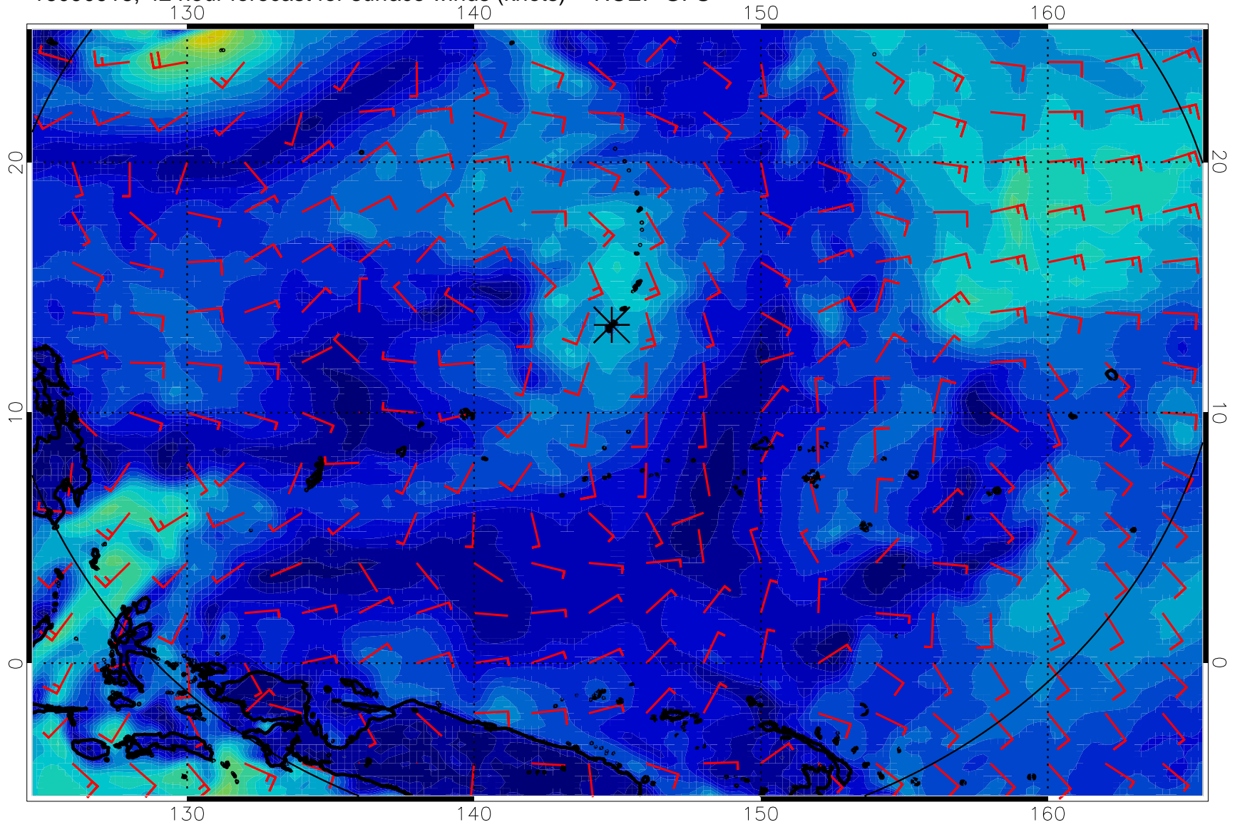
16090918, 42 hour forecast for surface winds (knots) -- NCEP GFS
