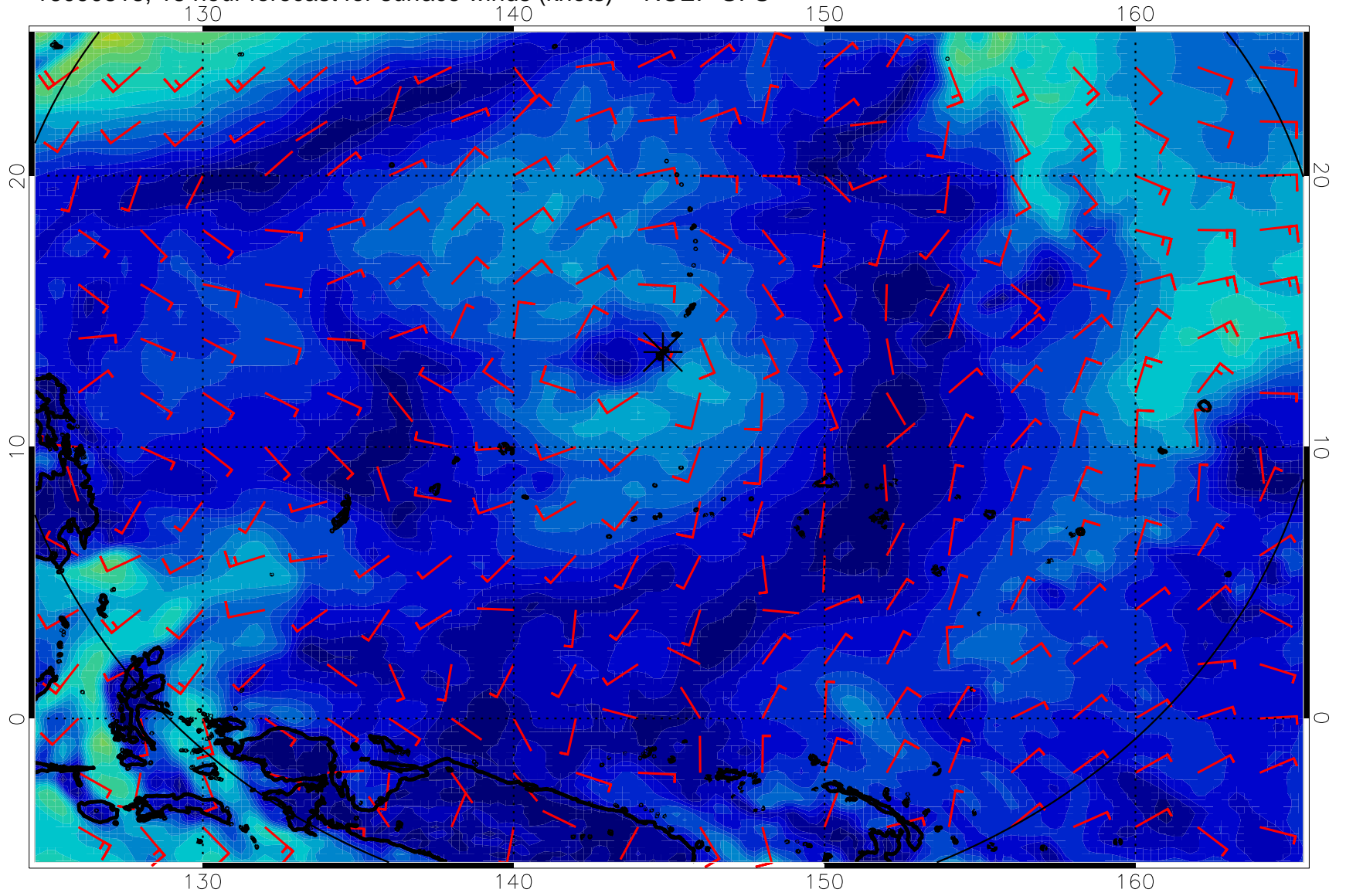
16090818, 18 hour forecast for surface winds (knots) -- NCEP GFS
