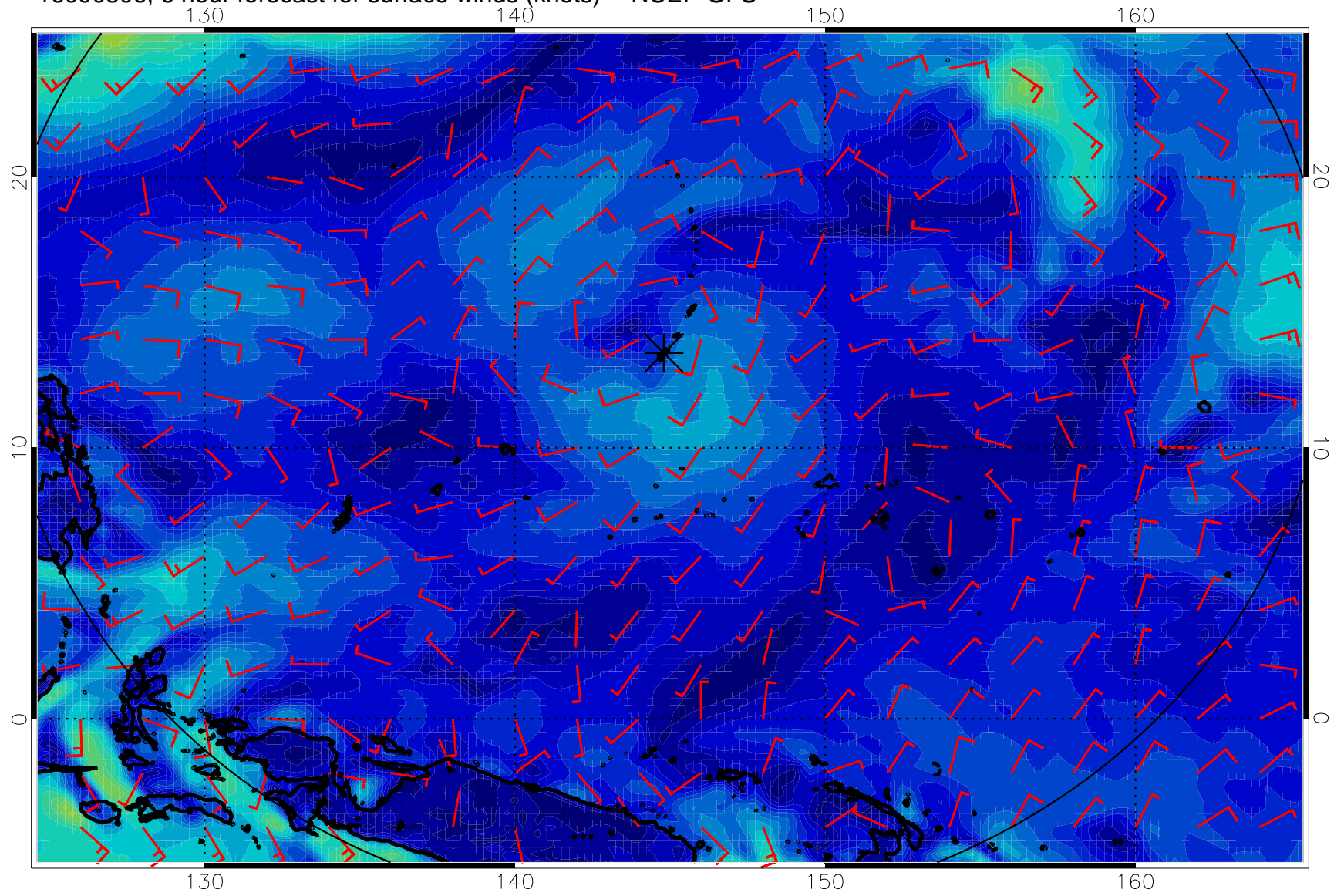
16090806, 6 hour forecast for surface winds (knots) -- NCEP GFS
