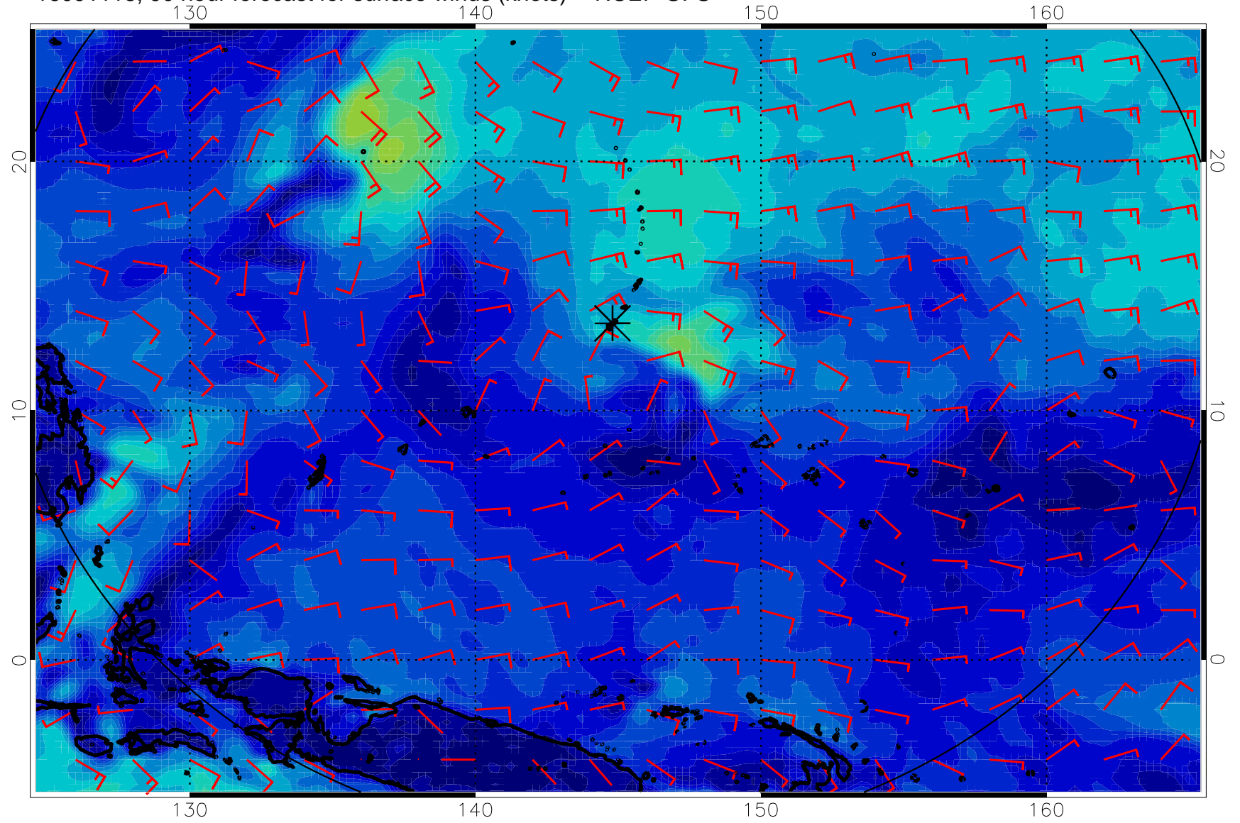
16091118, 90 hour forecast for surface winds (knots) -- NCEP GFS
