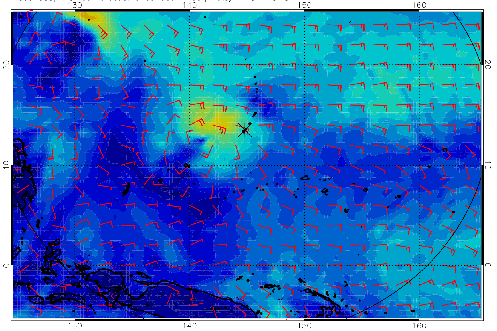
16091300, 120 hour forecast for surface winds (knots) -- NCEP GFS
