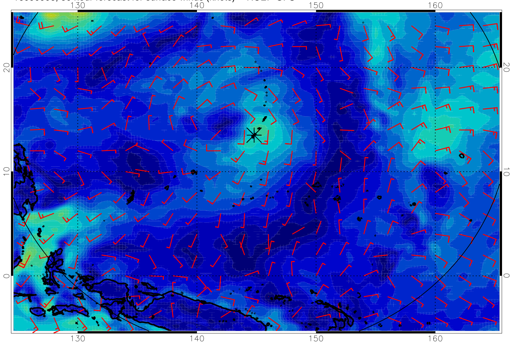
16090906, 30 hour forecast for surface winds (knots) -- NCEP GFS
