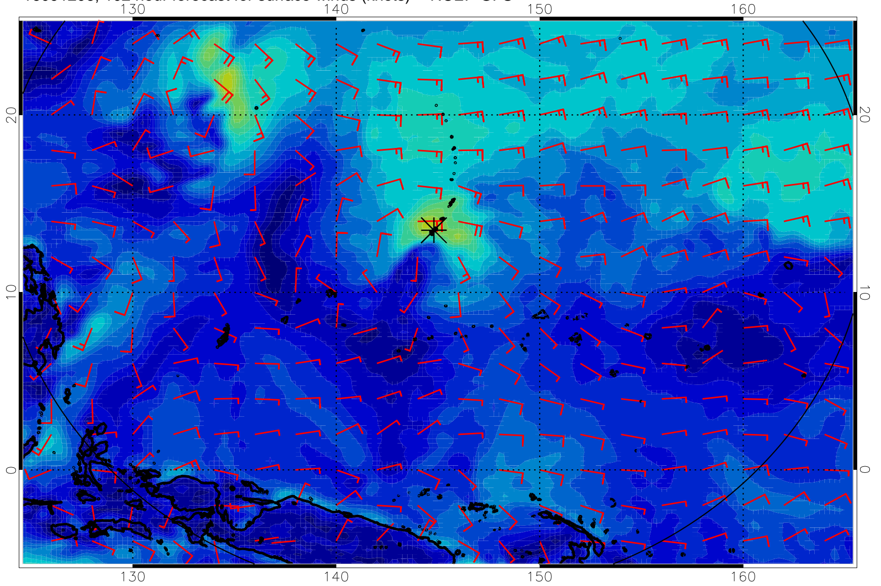
16091206, 102 hour forecast for surface winds (knots) -- NCEP GFS
