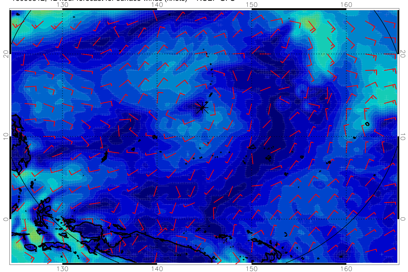
16090812, 12 hour forecast for surface winds (knots) -- NCEP GFS
