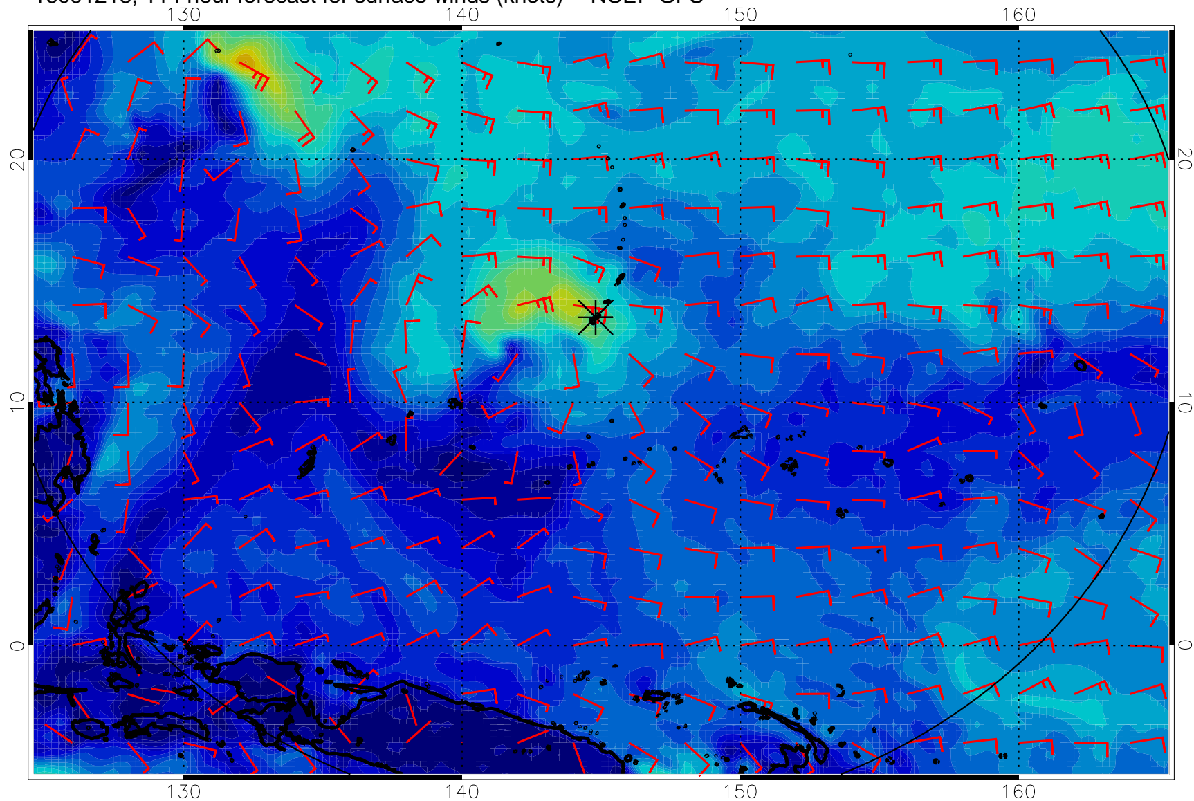
16091218, 114 hour forecast for surface winds (knots) -- NCEP GFS
