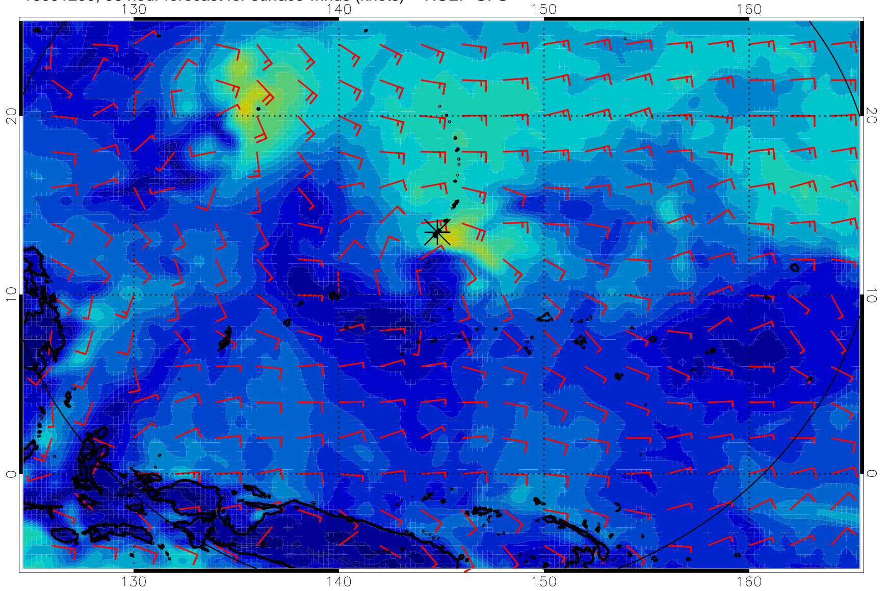
16091200, 96 hour forecast for surface winds (knots) -- NCEP GFS
