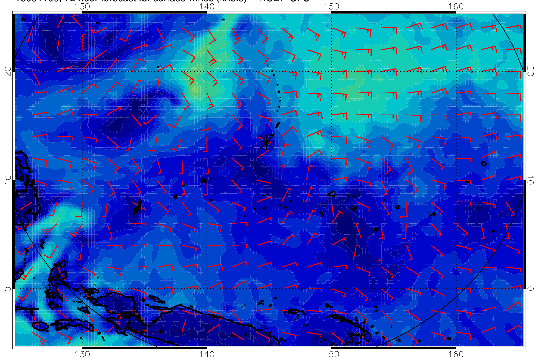
16091100, 72 hour forecast for surface winds (knots) -- NCEP GFS
