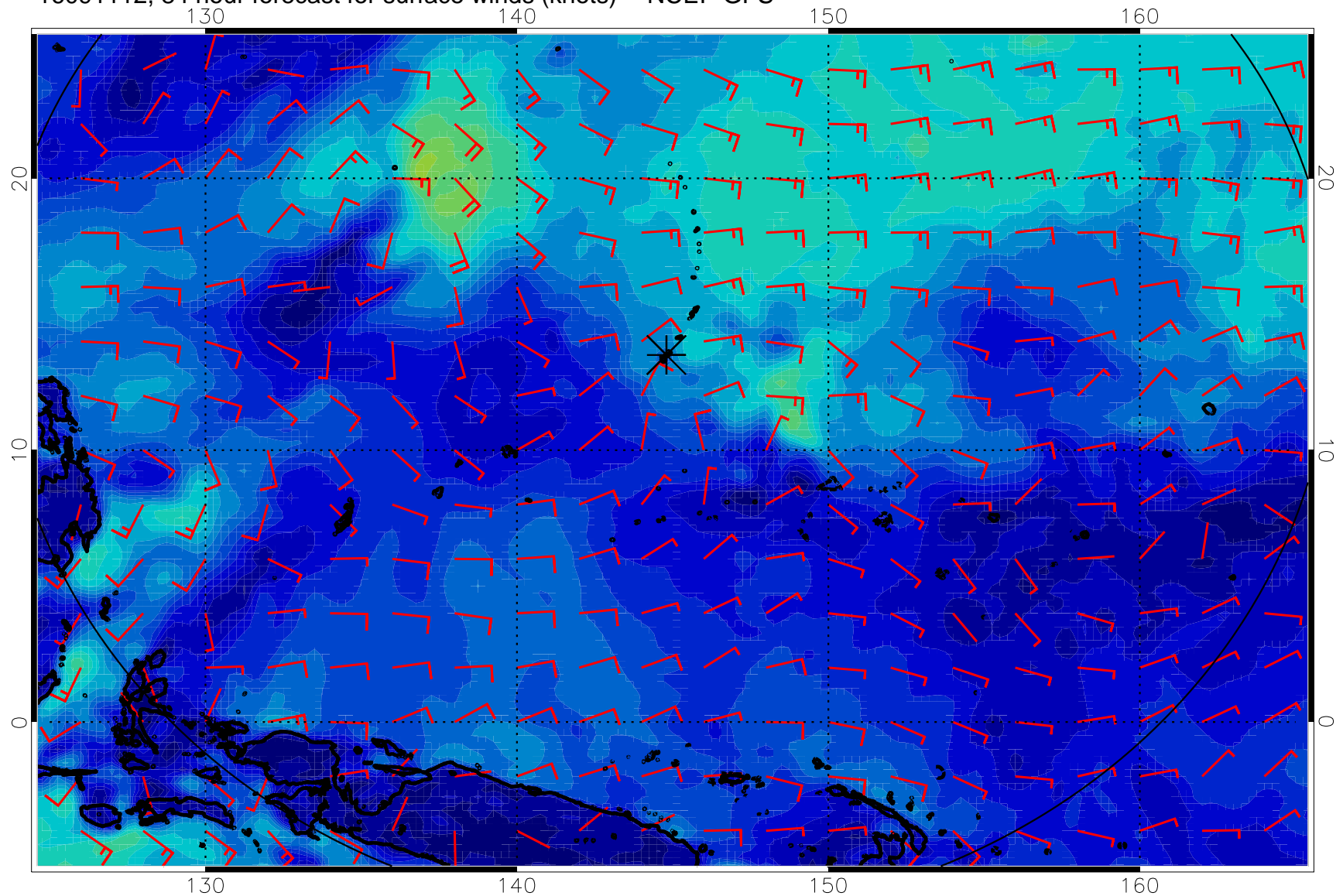
16091112, 84 hour forecast for surface winds (knots) -- NCEP GFS
