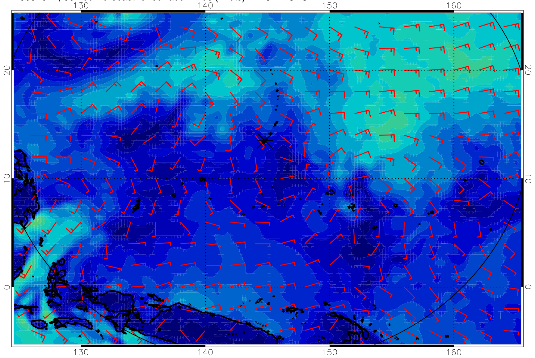
16091012, 60 hour forecast for surface winds (knots) -- NCEP GFS
