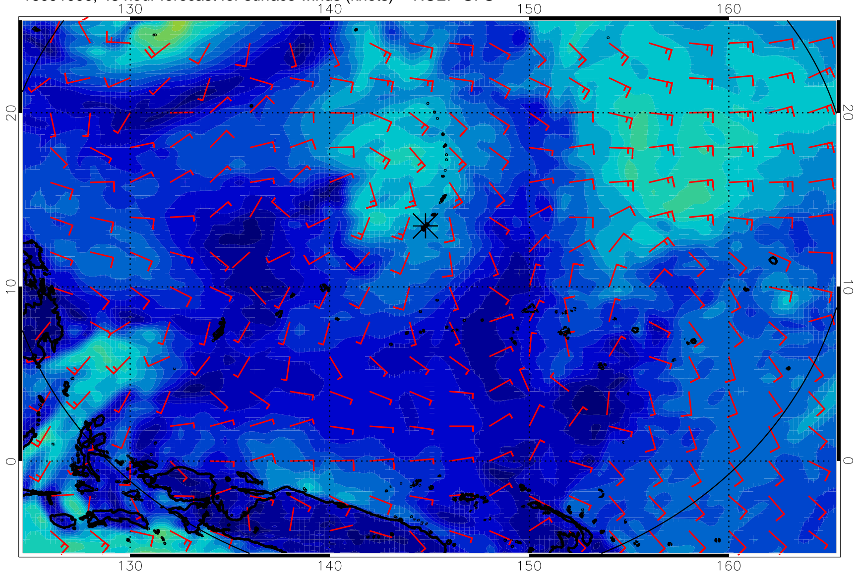
16091000, 48 hour forecast for surface winds (knots) -- NCEP GFS
