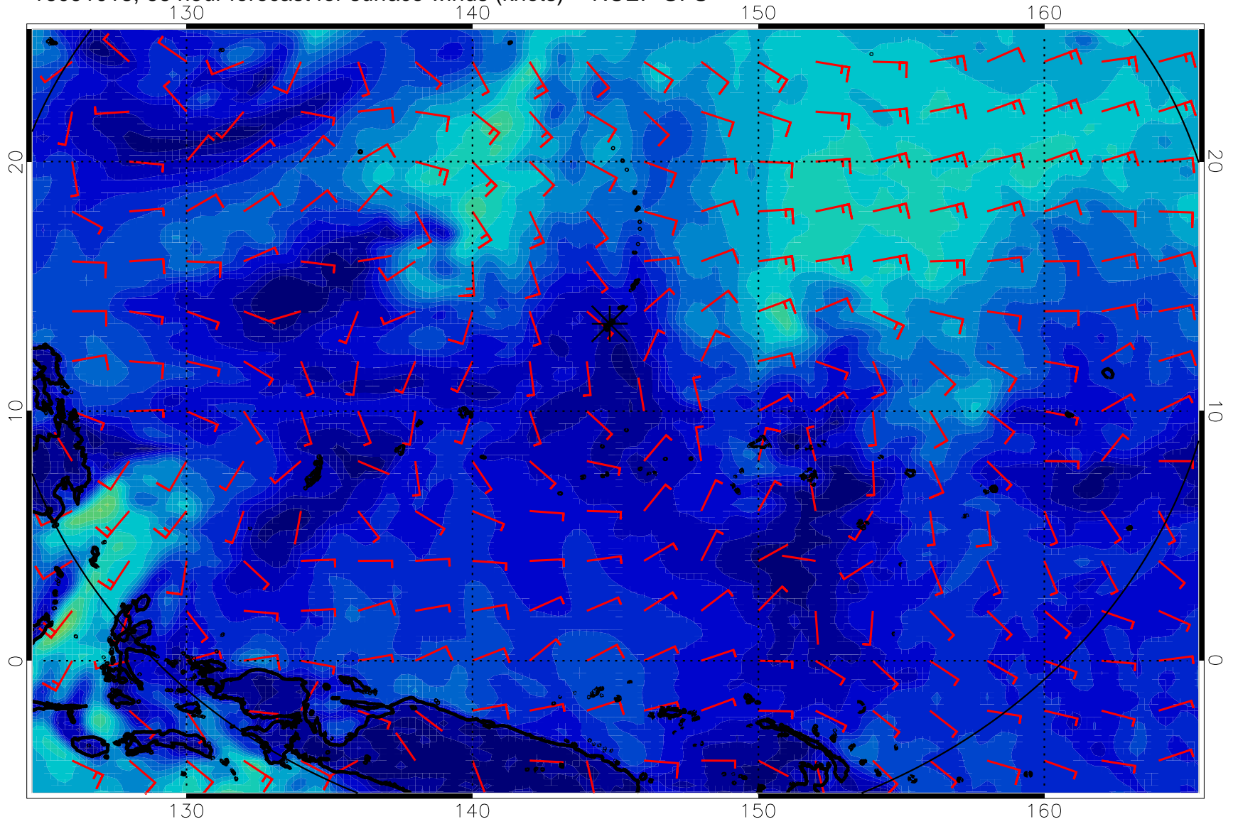
16091018, 66 hour forecast for surface winds (knots) -- NCEP GFS
