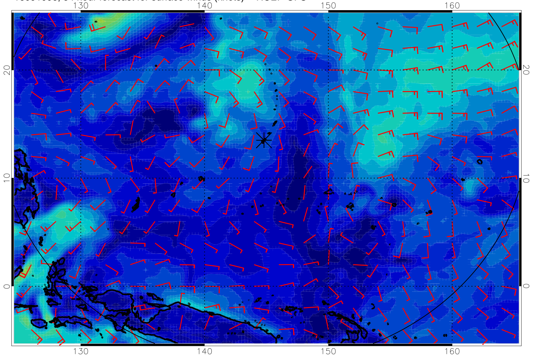
16091006, 54 hour forecast for surface winds (knots) -- NCEP GFS
