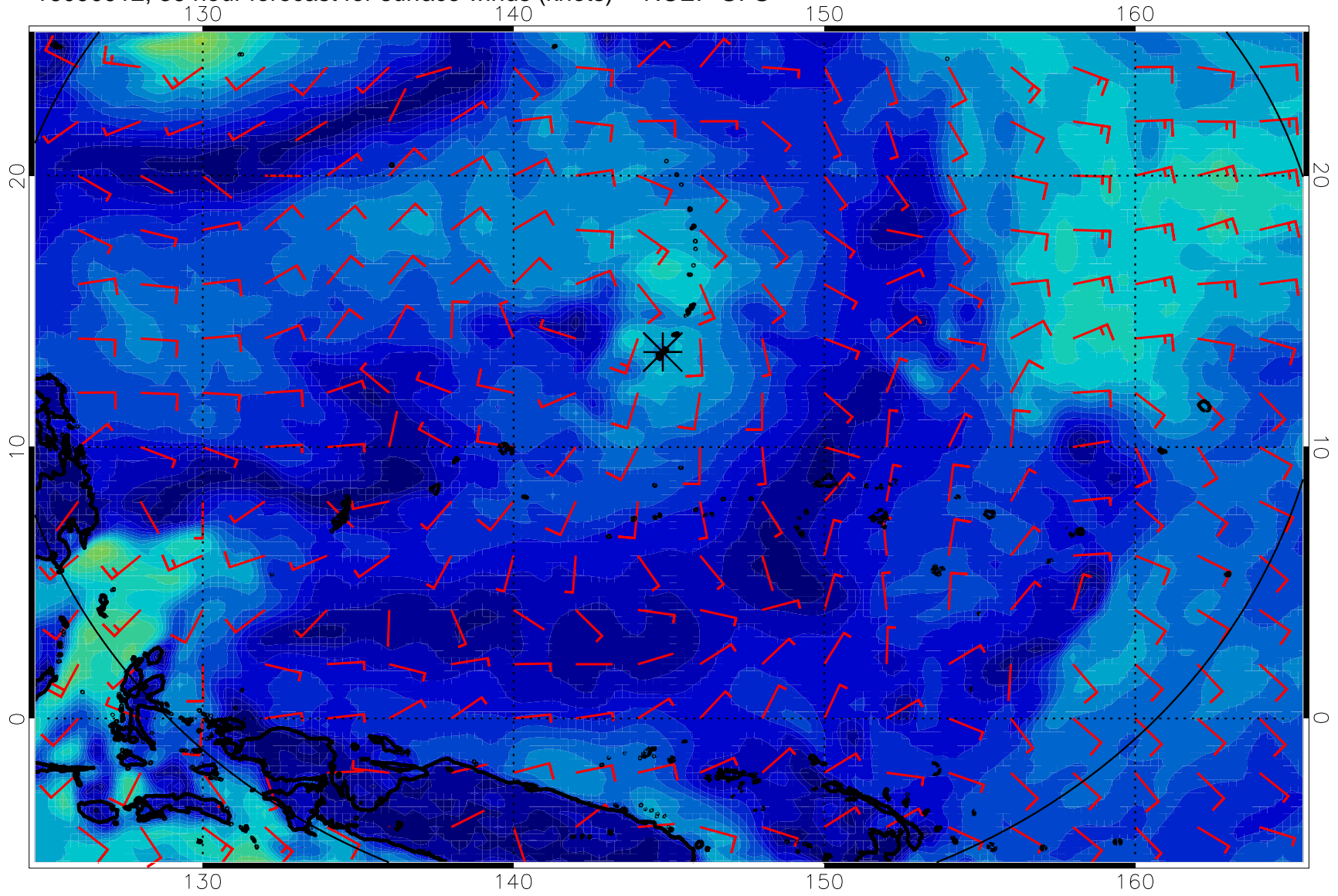
16090912, 36 hour forecast for surface winds (knots) -- NCEP GFS
