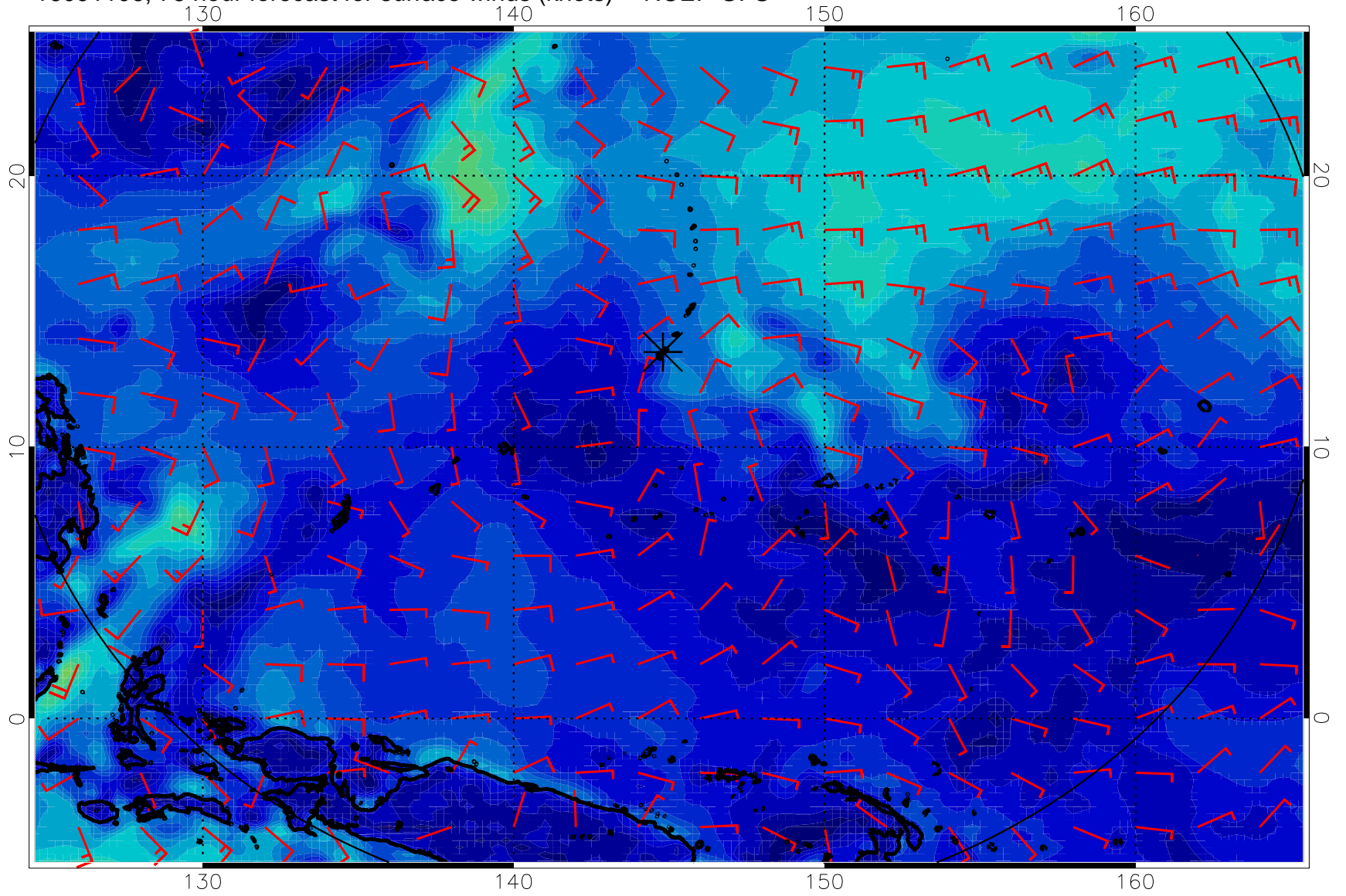
16091106, 78 hour forecast for surface winds (knots) -- NCEP GFS
