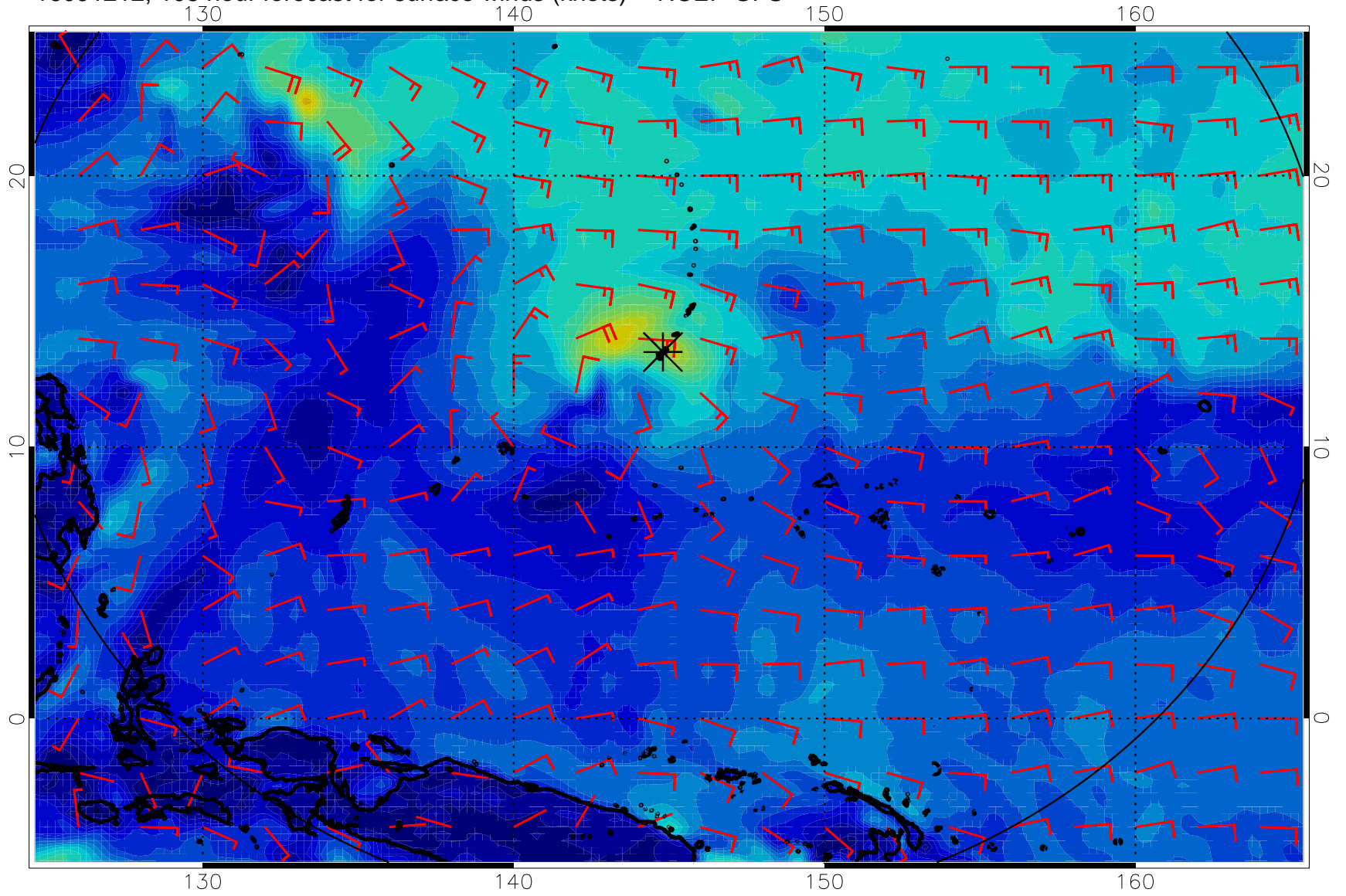
16091212, 108 hour forecast for surface winds (knots) -- NCEP GFS
