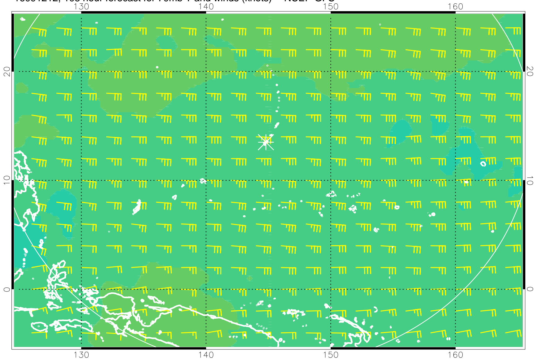
16091212, 108 hour forecast for 70mb T and winds (knots) -- NCEP GFS
