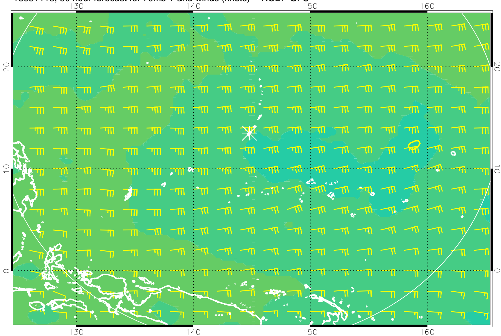
16091118, 90 hour forecast for 70mb T and winds (knots) -- NCEP GFS
