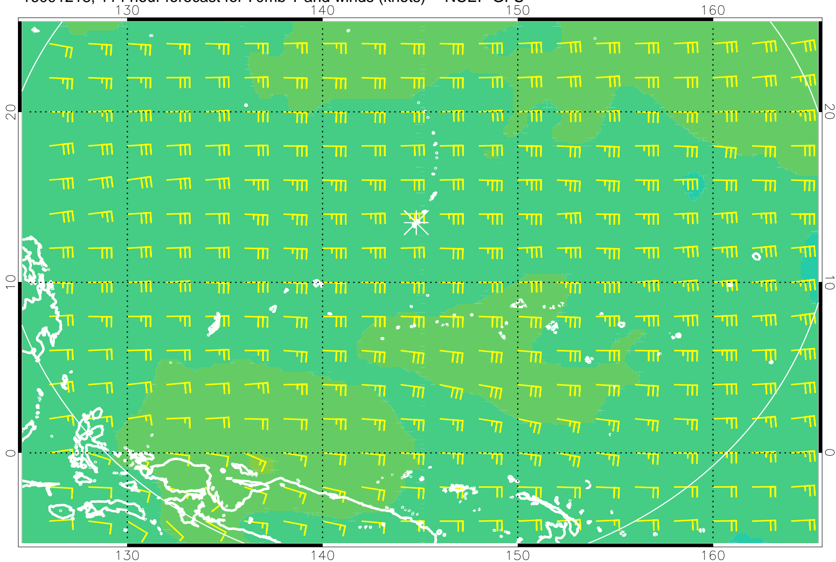
16091218, 114 hour forecast for 70mb T and winds (knots) -- NCEP GFS
