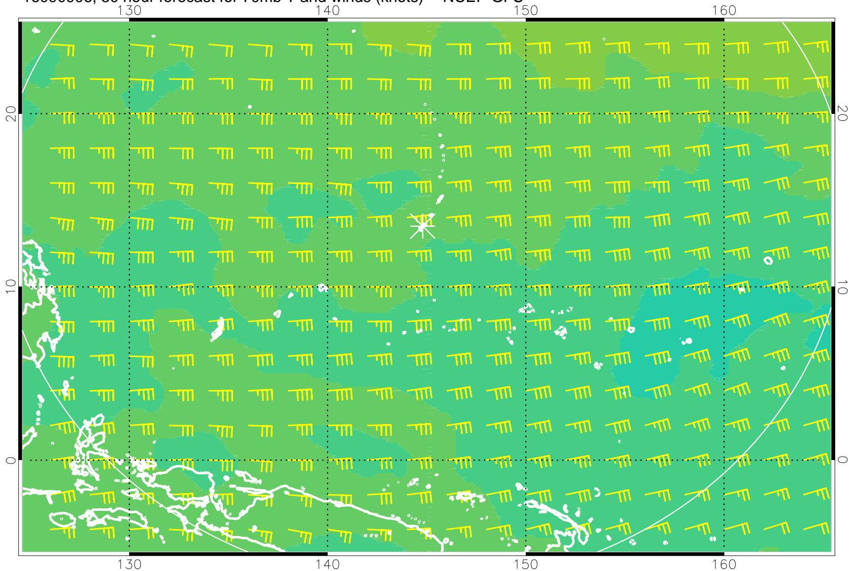
16090906, 30 hour forecast for 70mb T and winds (knots) -- NCEP GFS
