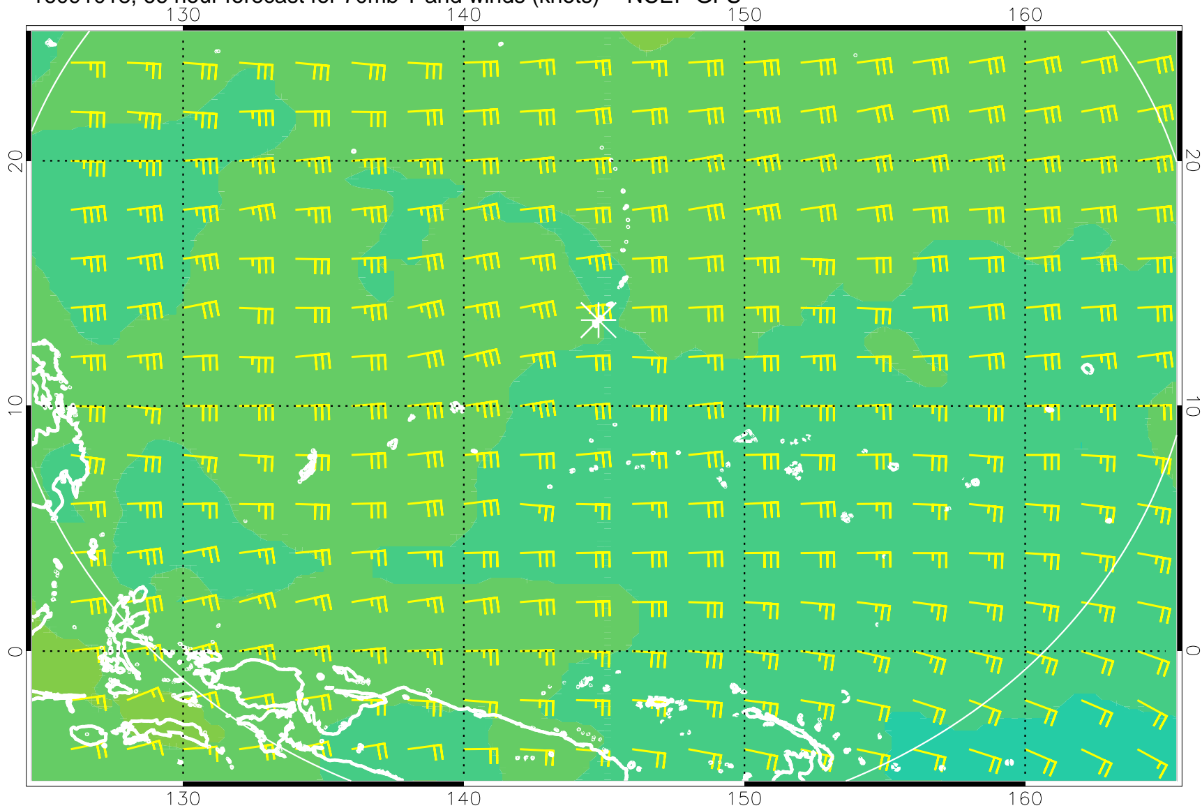
16091018, 66 hour forecast for 70mb T and winds (knots) -- NCEP GFS
