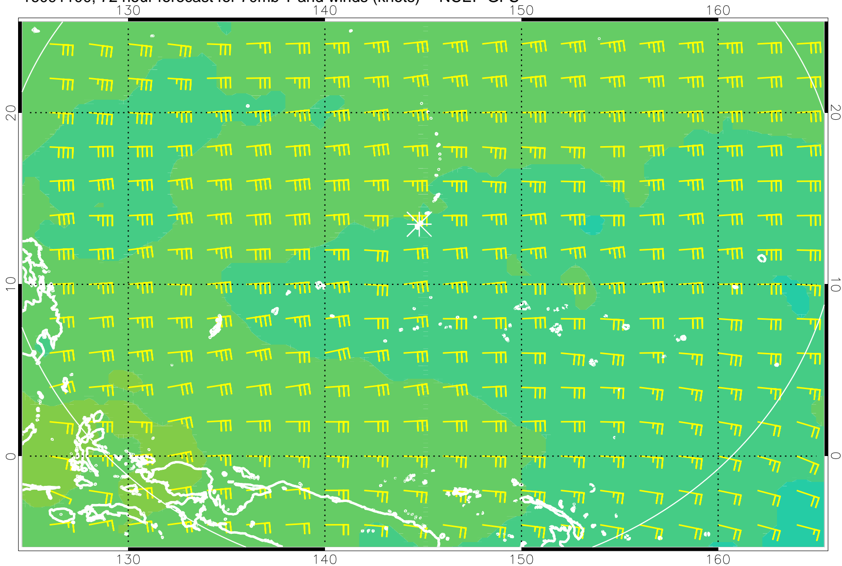
16091100, 72 hour forecast for 70mb T and winds (knots) -- NCEP GFS
