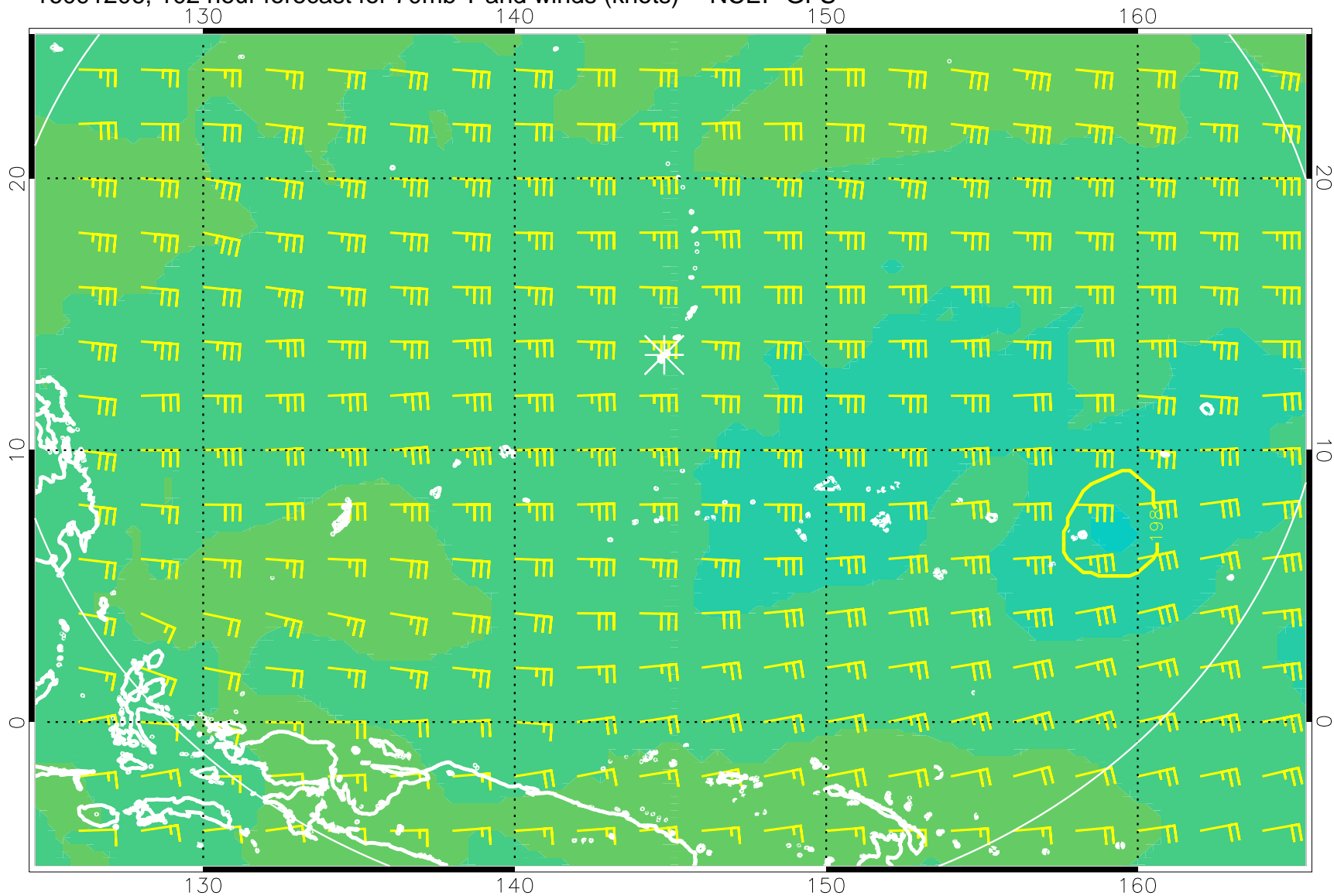
16091206, 102 hour forecast for 70mb T and winds (knots) -- NCEP GFS
