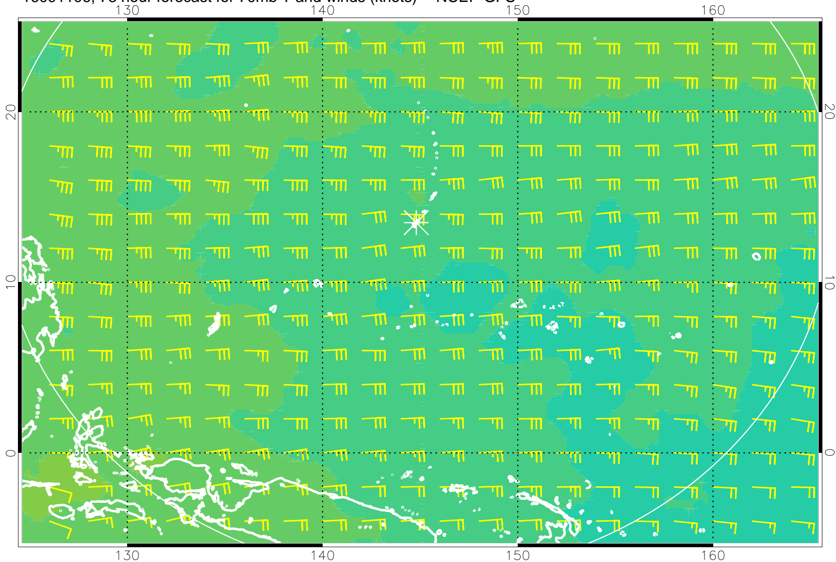
16091106, 78 hour forecast for 70mb T and winds (knots) -- NCEP GFS
