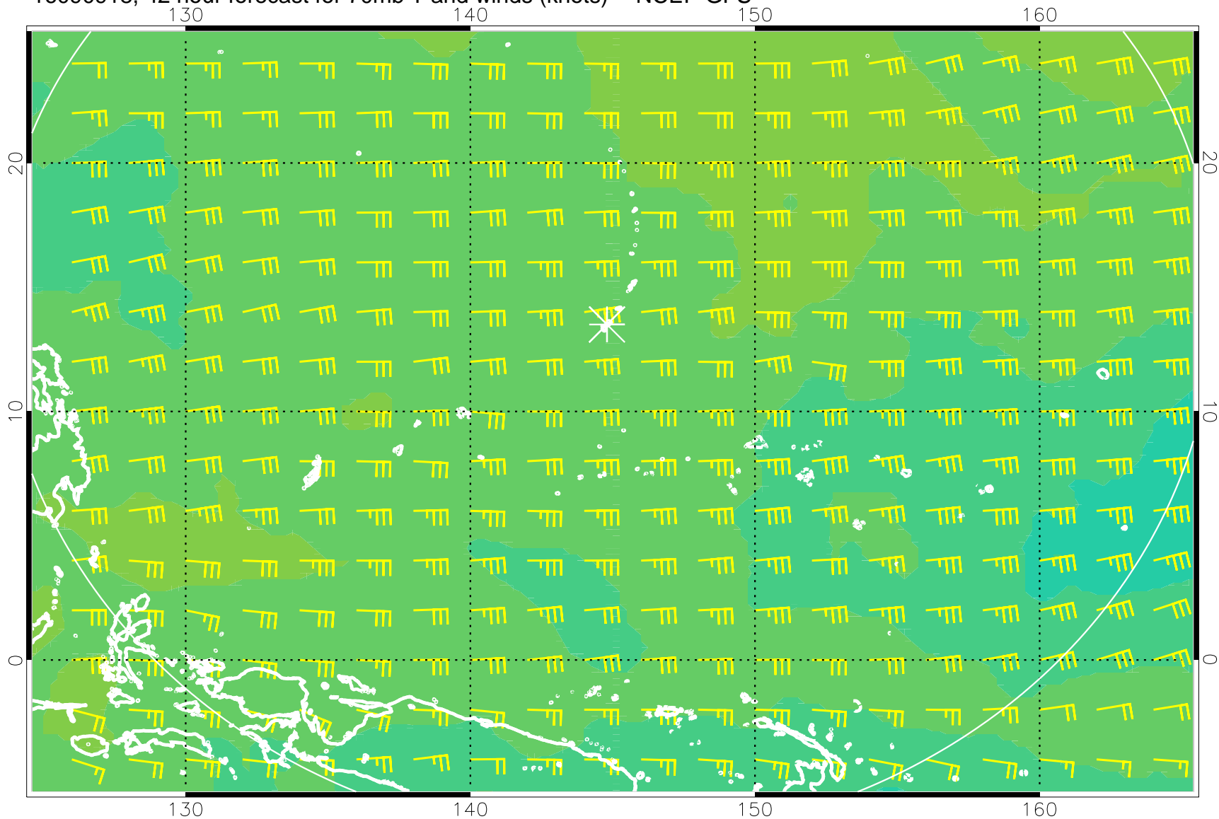
16090918, 42 hour forecast for 70mb T and winds (knots) -- NCEP GFS
