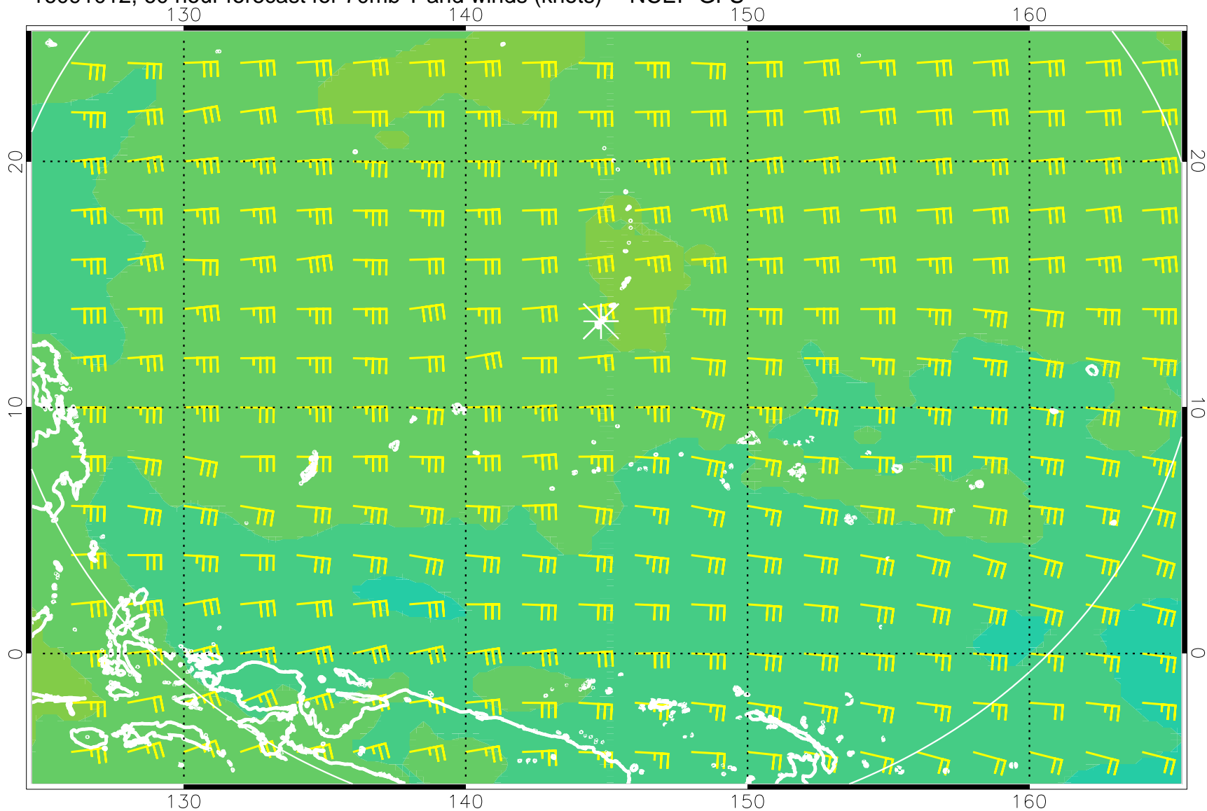
16091012, 60 hour forecast for 70mb T and winds (knots) -- NCEP GFS
