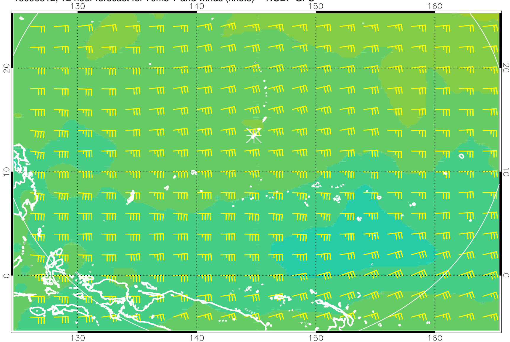
16090812, 12 hour forecast for 70mb T and winds (knots) -- NCEP GFS
