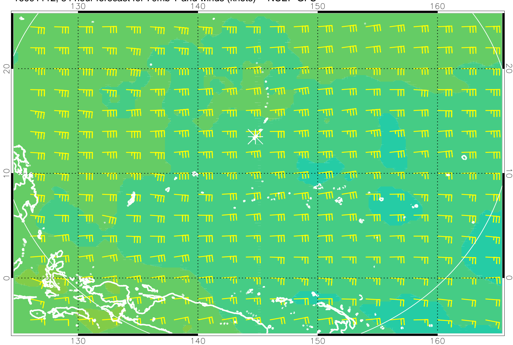
16091112, 84 hour forecast for 70mb T and winds (knots) -- NCEP GFS
