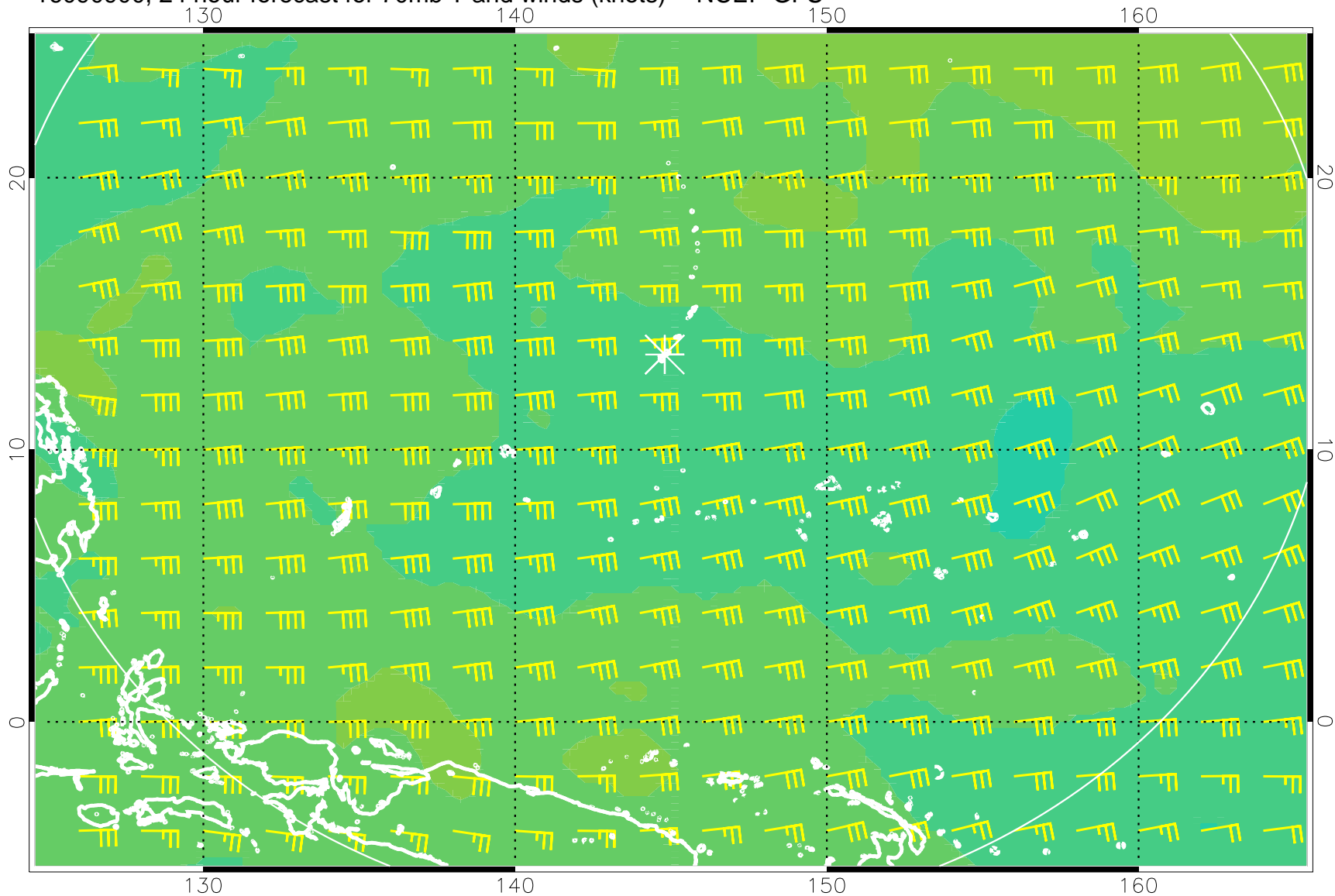
16090900, 24 hour forecast for 70mb T and winds (knots) -- NCEP GFS
