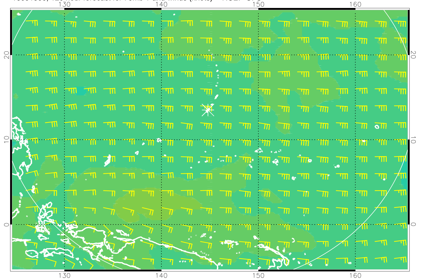
16091300, 120 hour forecast for 70mb T and winds (knots) -- NCEP GFS
