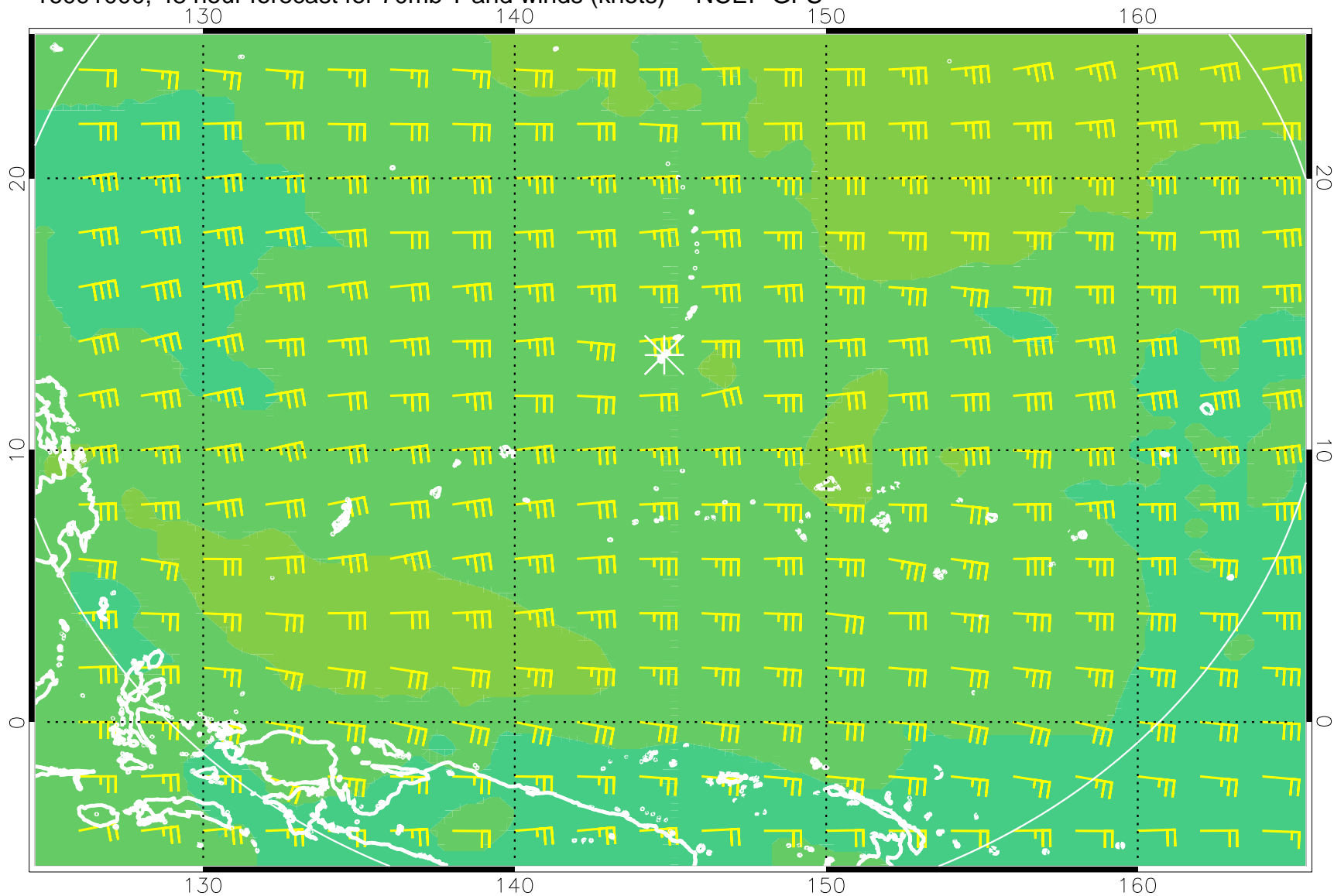
16091000, 48 hour forecast for 70mb T and winds (knots) -- NCEP GFS
