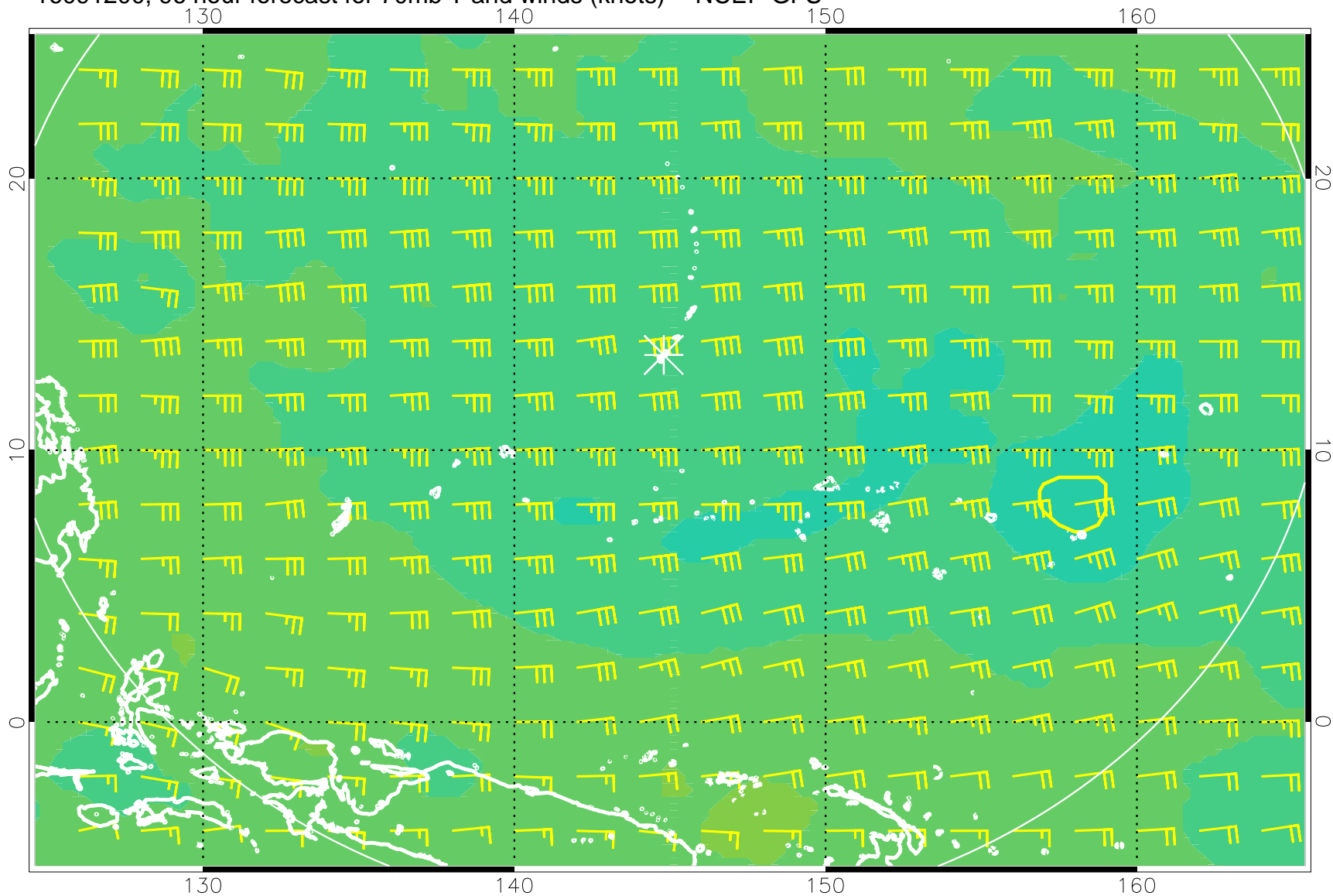
16091200, 96 hour forecast for 70mb T and winds (knots) -- NCEP GFS
