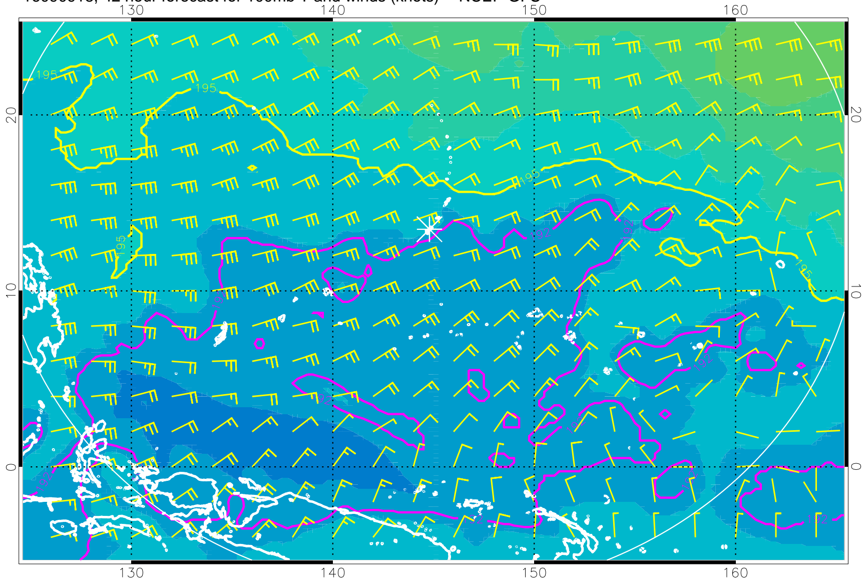
16090918, 42 hour forecast for 100mb T and winds (knots) -- NCEP GFS
