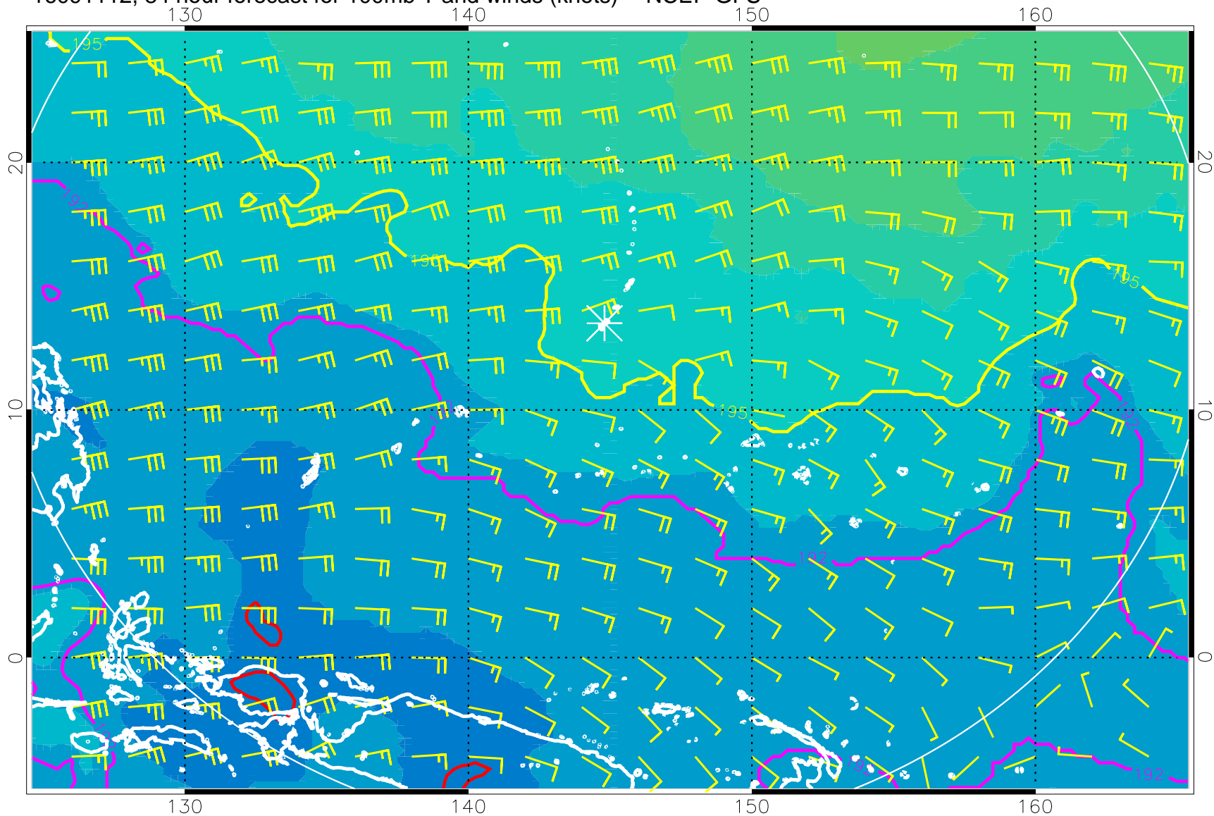
16091112, 84 hour forecast for 100mb T and winds (knots) -- NCEP GFS
