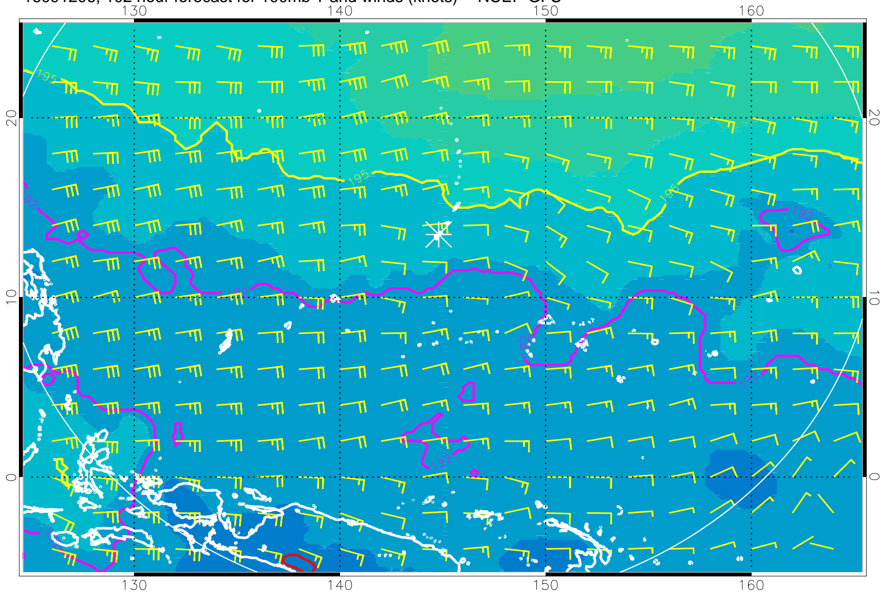
16091206, 102 hour forecast for 100mb T and winds (knots) -- NCEP GFS
