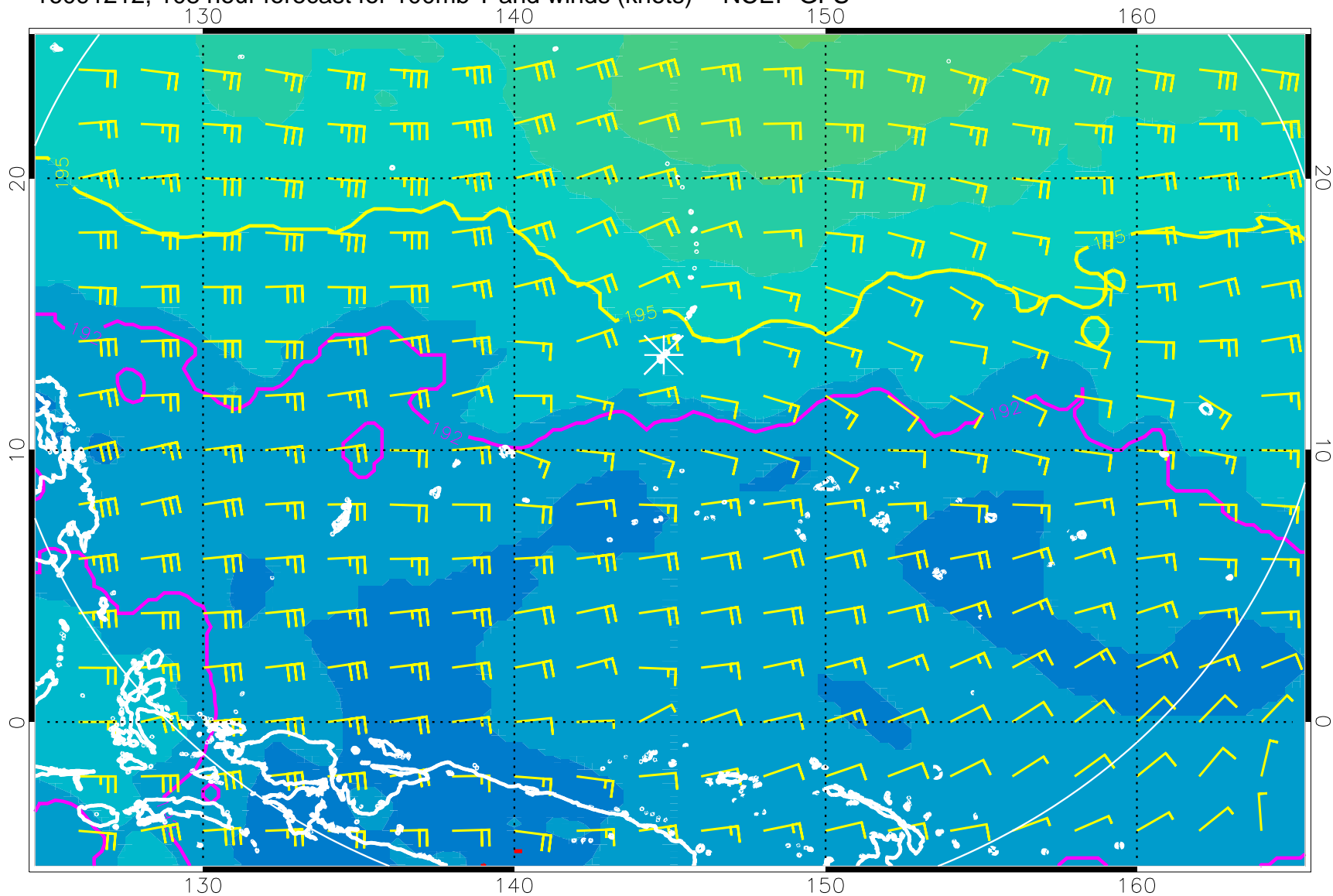
16091212, 108 hour forecast for 100mb T and winds (knots) -- NCEP GFS
