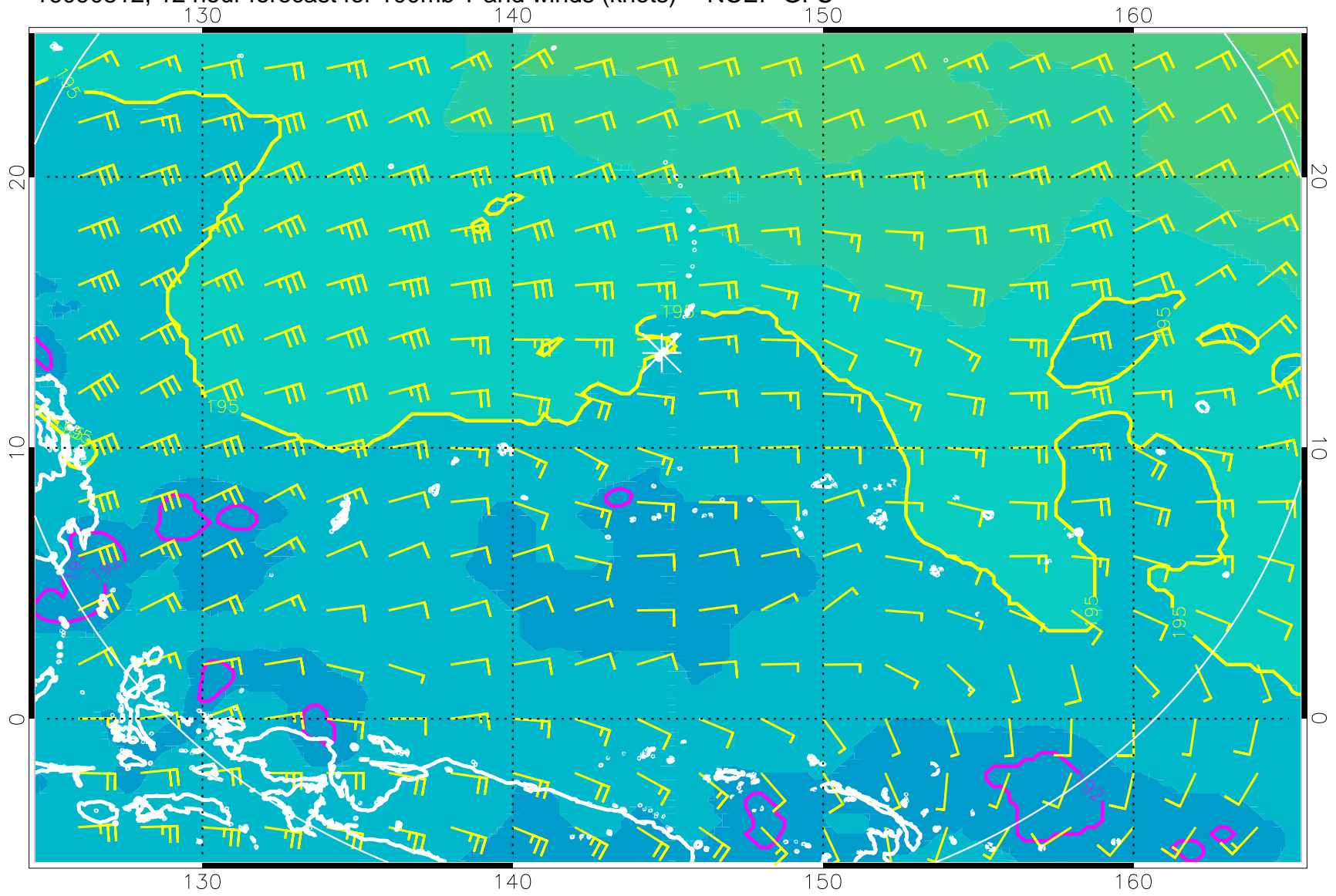
16090812, 12 hour forecast for 100mb T and winds (knots) -- NCEP GFS
