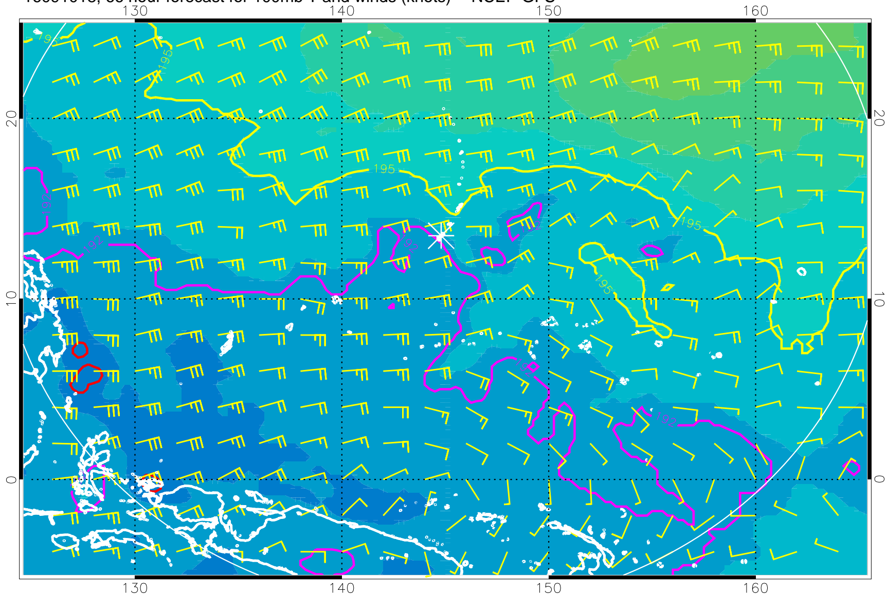
16091018, 66 hour forecast for 100mb T and winds (knots) -- NCEP GFS
