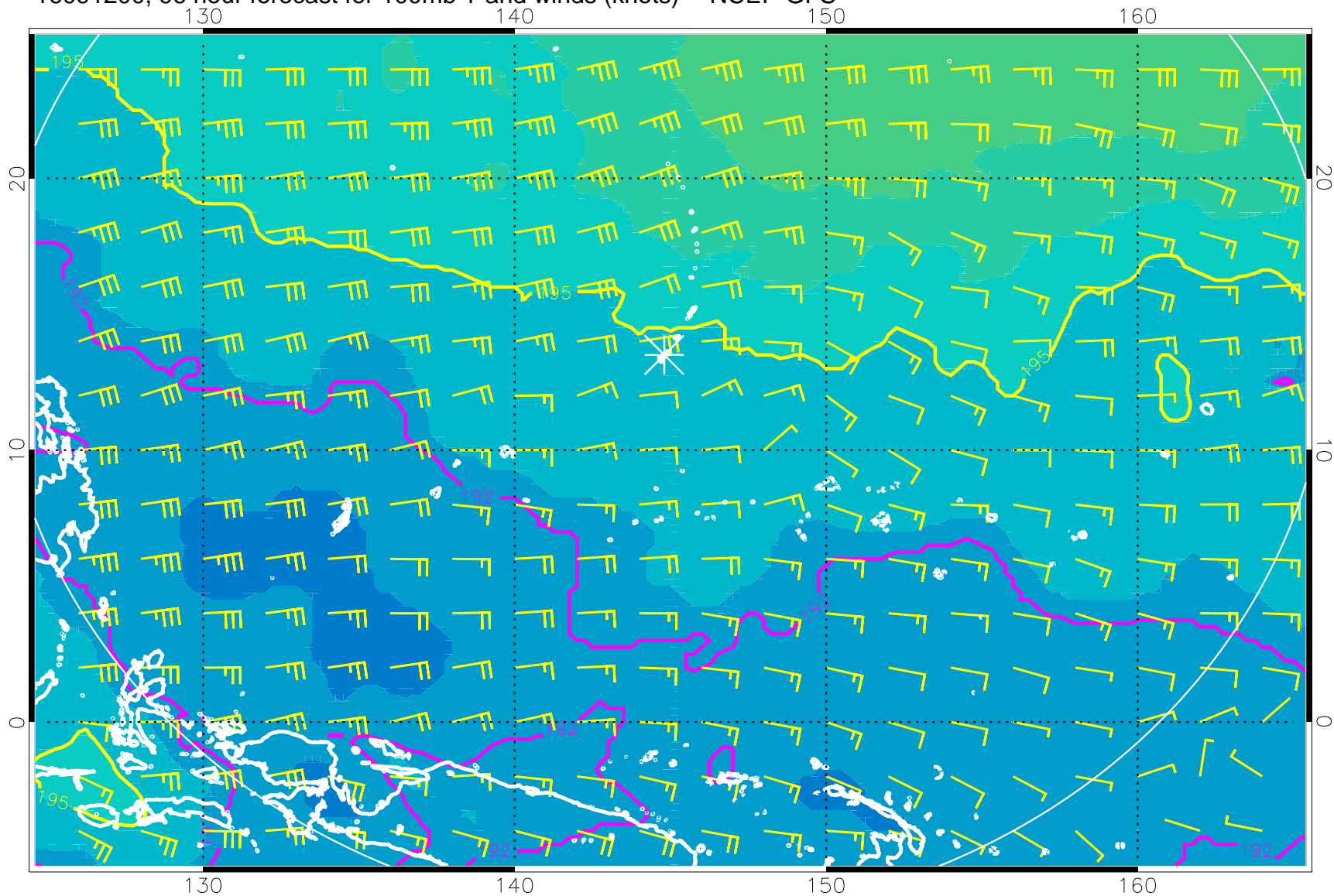
16091200, 96 hour forecast for 100mb T and winds (knots) -- NCEP GFS
