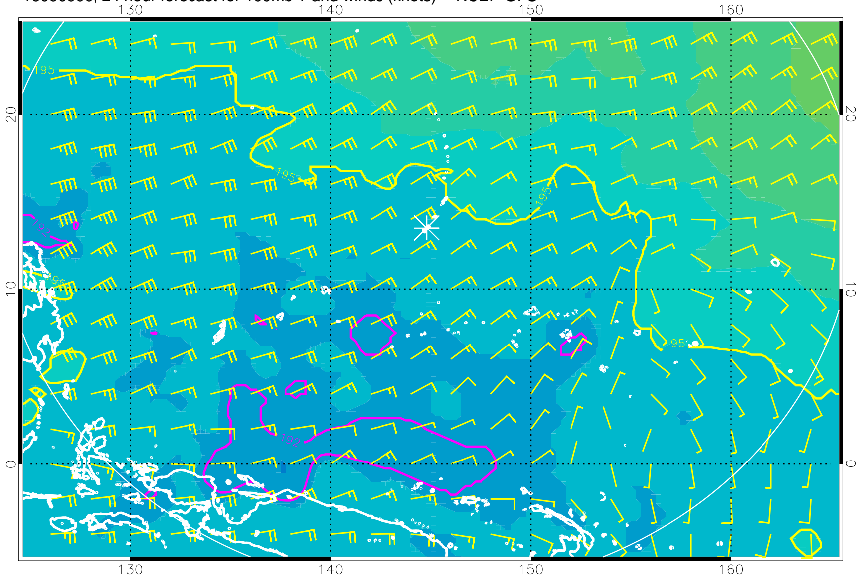
16090900, 24 hour forecast for 100mb T and winds (knots) -- NCEP GFS
