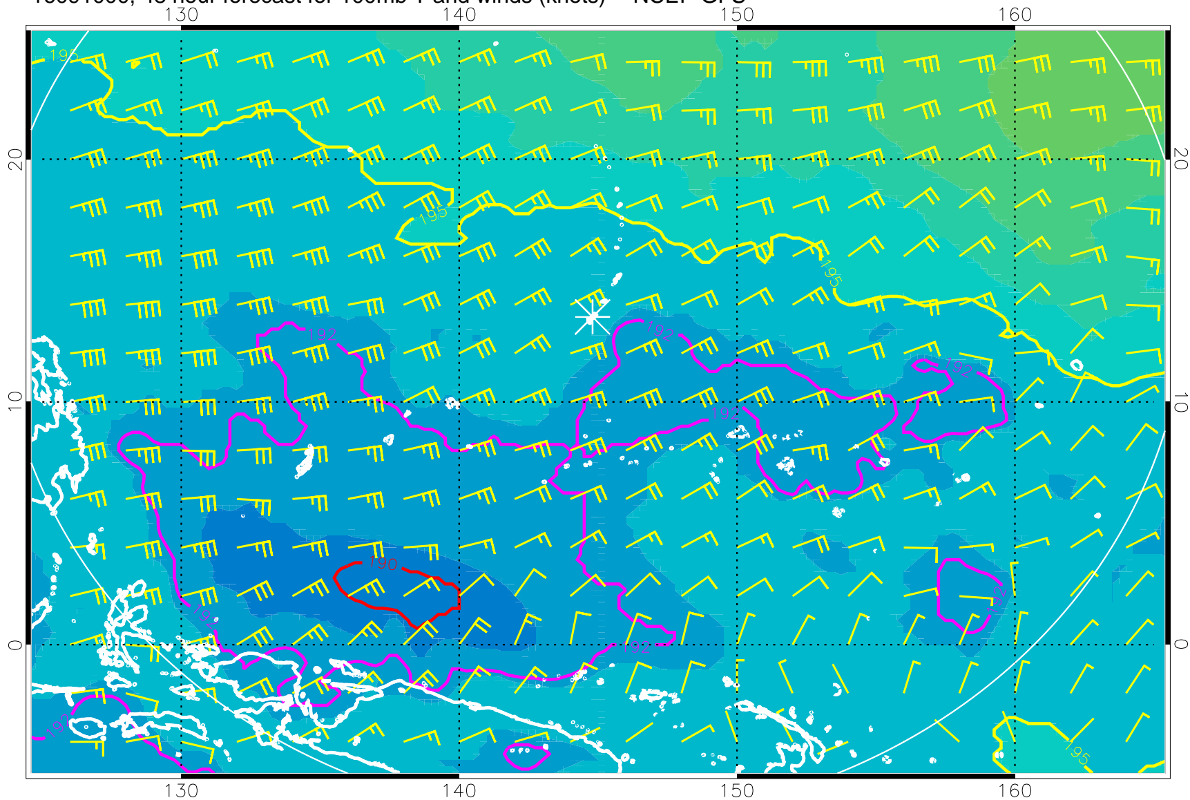
16091000, 48 hour forecast for 100mb T and winds (knots) -- NCEP GFS
