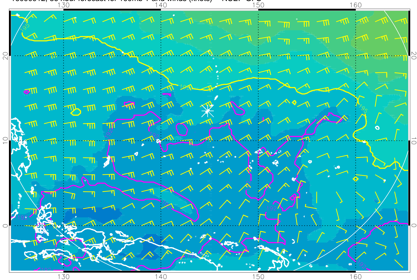
16090912, 36 hour forecast for 100mb T and winds (knots) -- NCEP GFS
