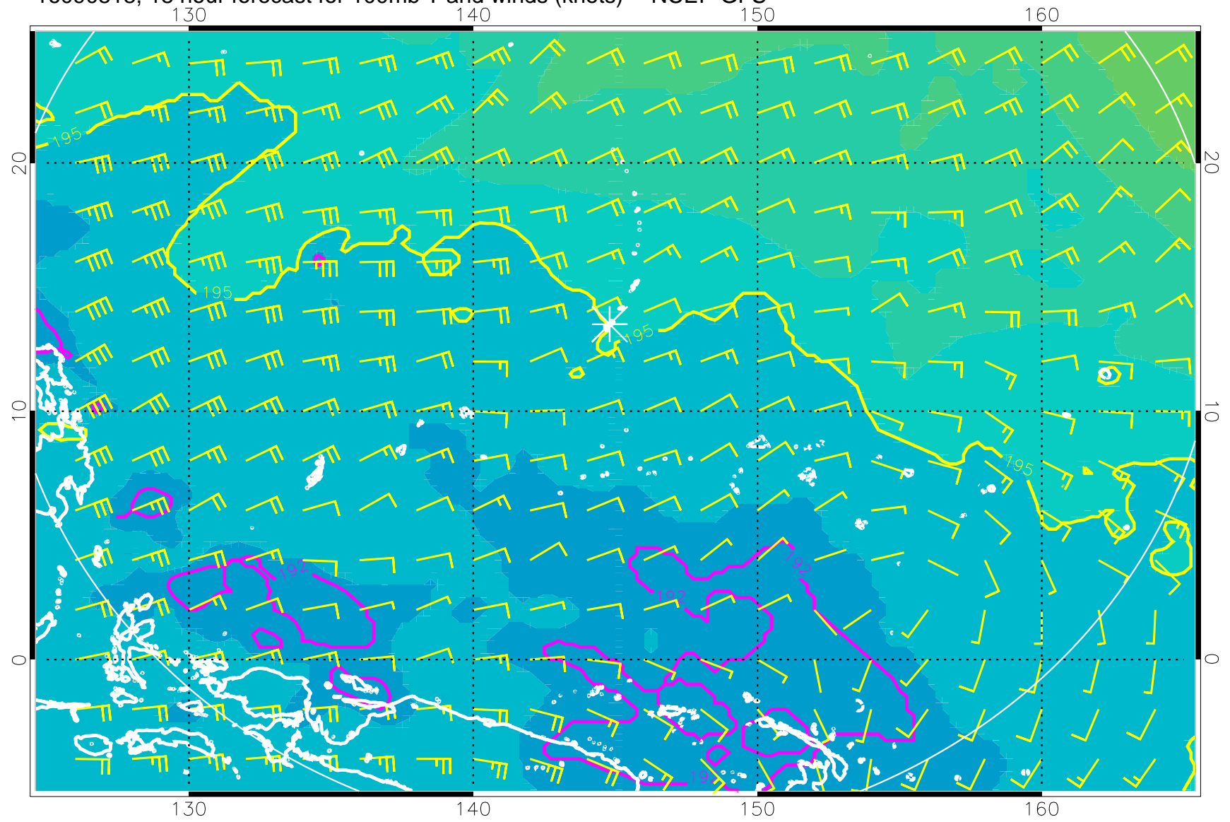
16090818, 18 hour forecast for 100mb T and winds (knots) -- NCEP GFS
