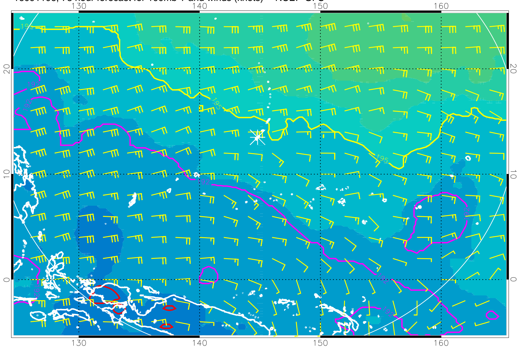
16091106, 78 hour forecast for 100mb T and winds (knots) -- NCEP GFS
