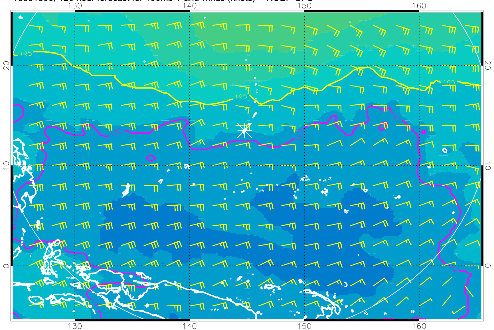
16091300, 120 hour forecast for 100mb T and winds (knots) -- NCEP GFS
