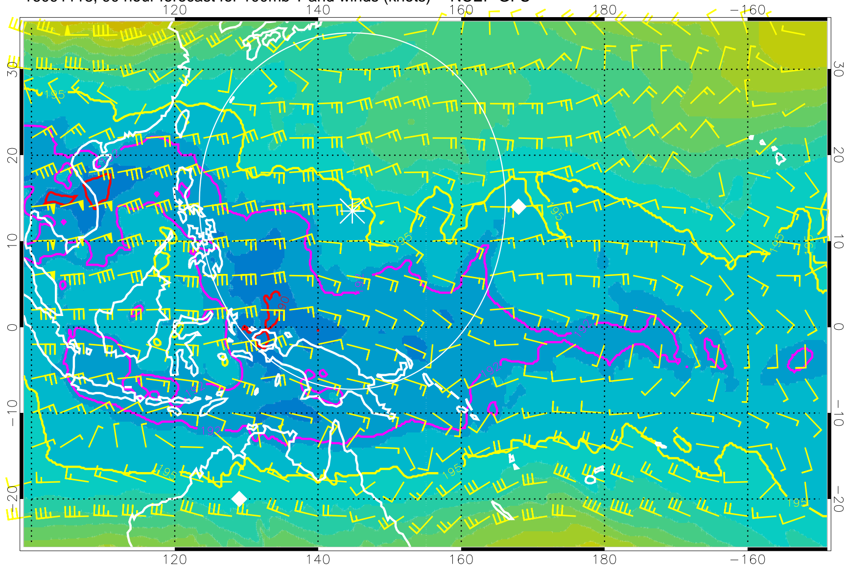
16091118, 90 hour forecast for 100mb T and winds (knots) -- NCEP GFS
