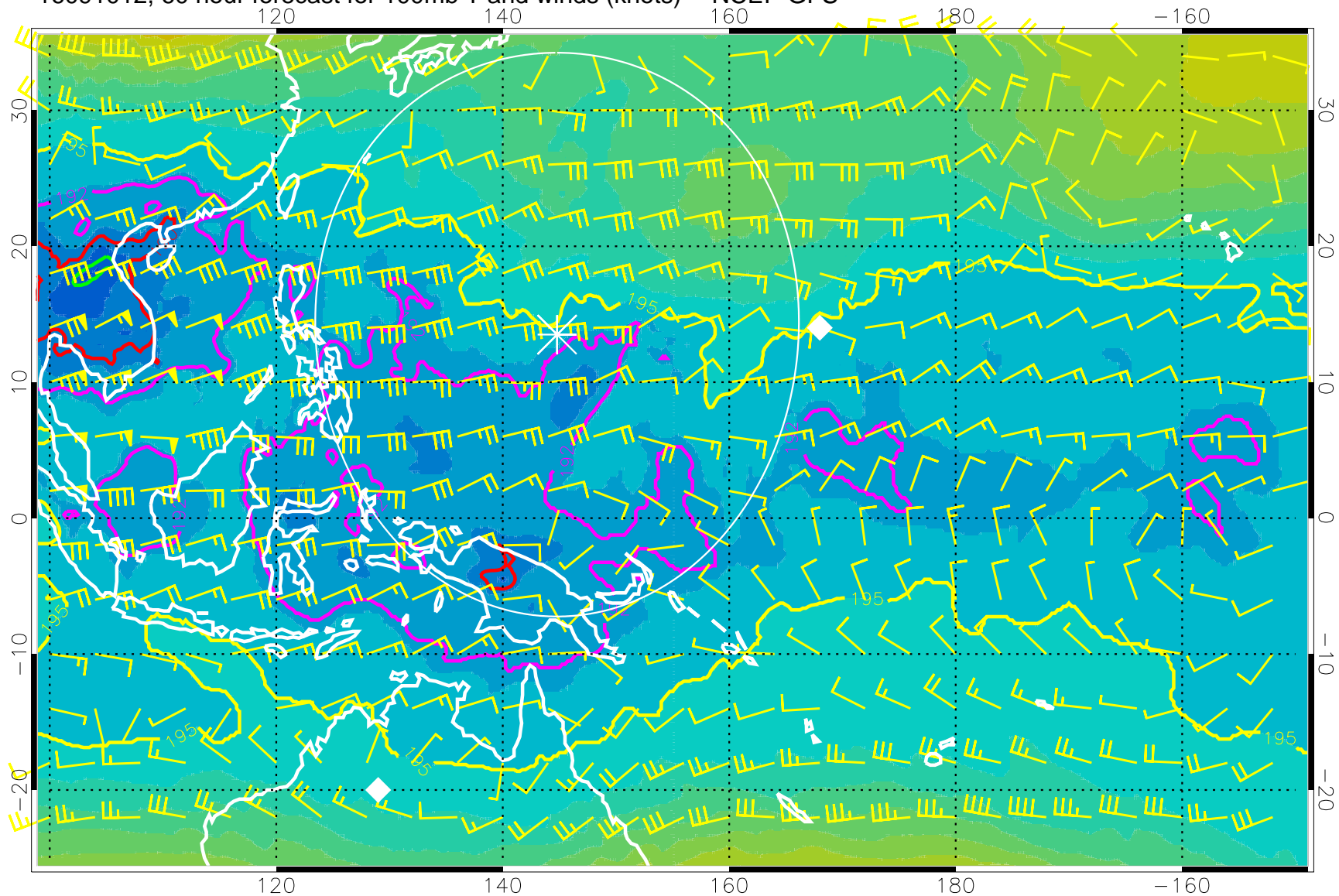
16091012, 60 hour forecast for 100mb T and winds (knots) -- NCEP GFS
