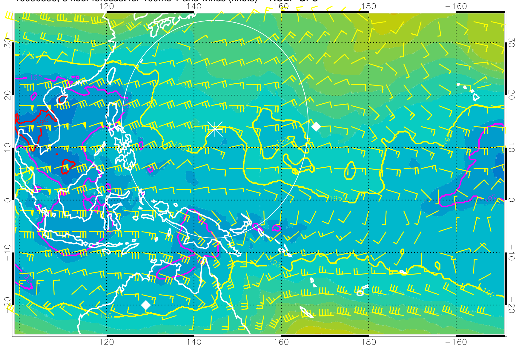
16090806, 6 hour forecast for 100mb T and winds (knots) -- NCEP GFS
