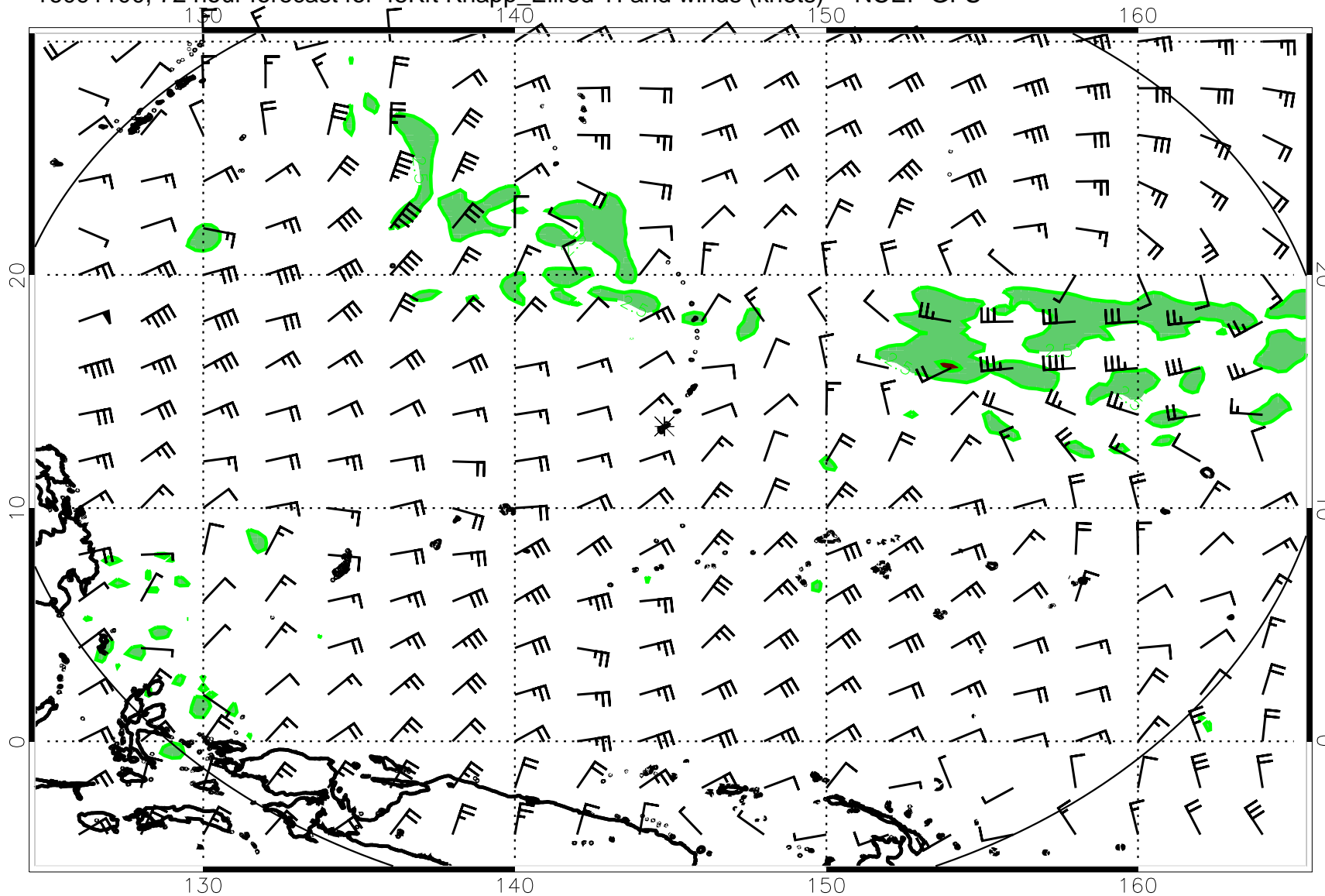
16091100, 72 hour forecast for 45Kft Knapp_Ellrod TI and winds (knots) -- NCEP GFS
