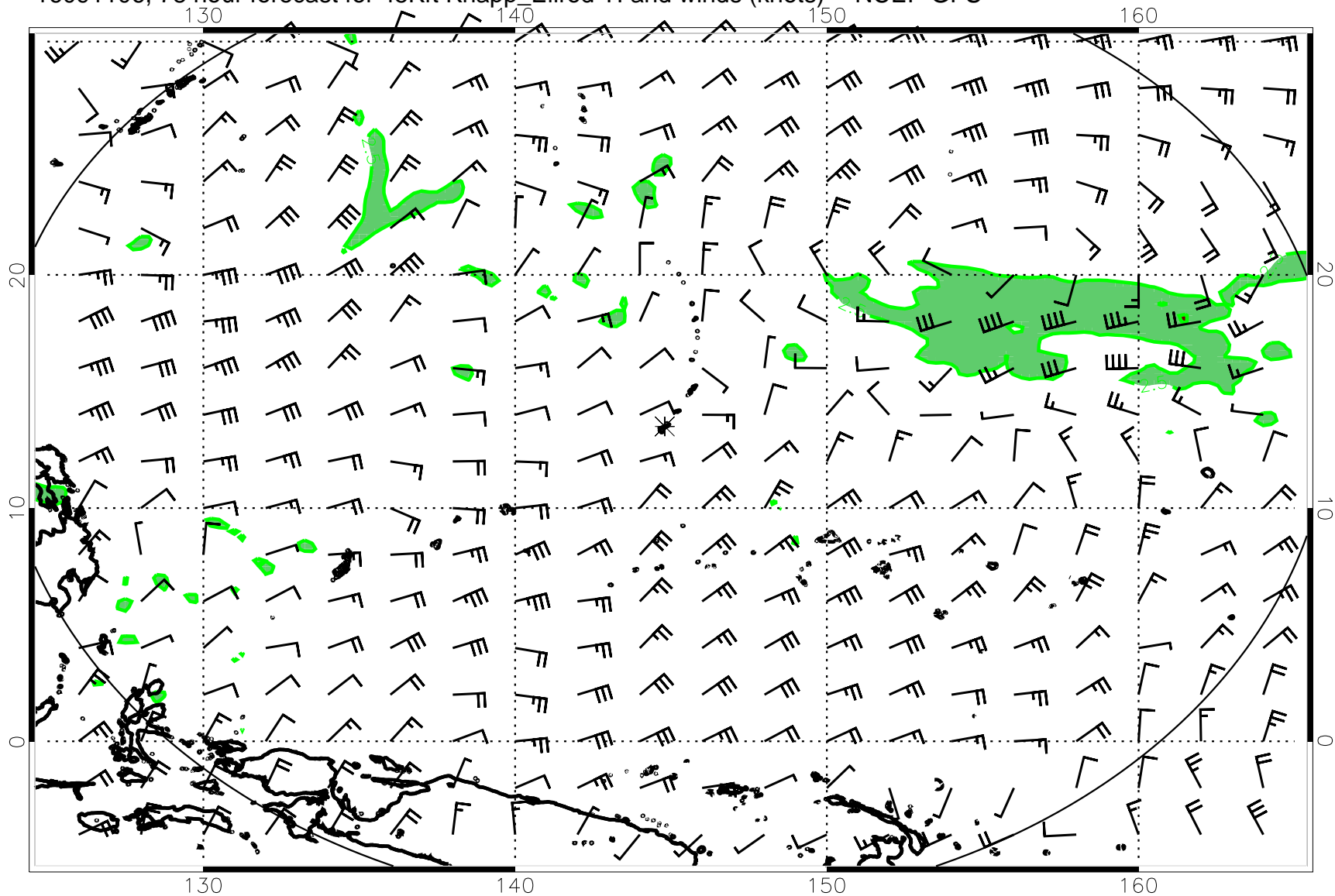
16091106, 78 hour forecast for 45Kft Knapp_Ellrod TI and winds (knots) -- NCEP GFS
