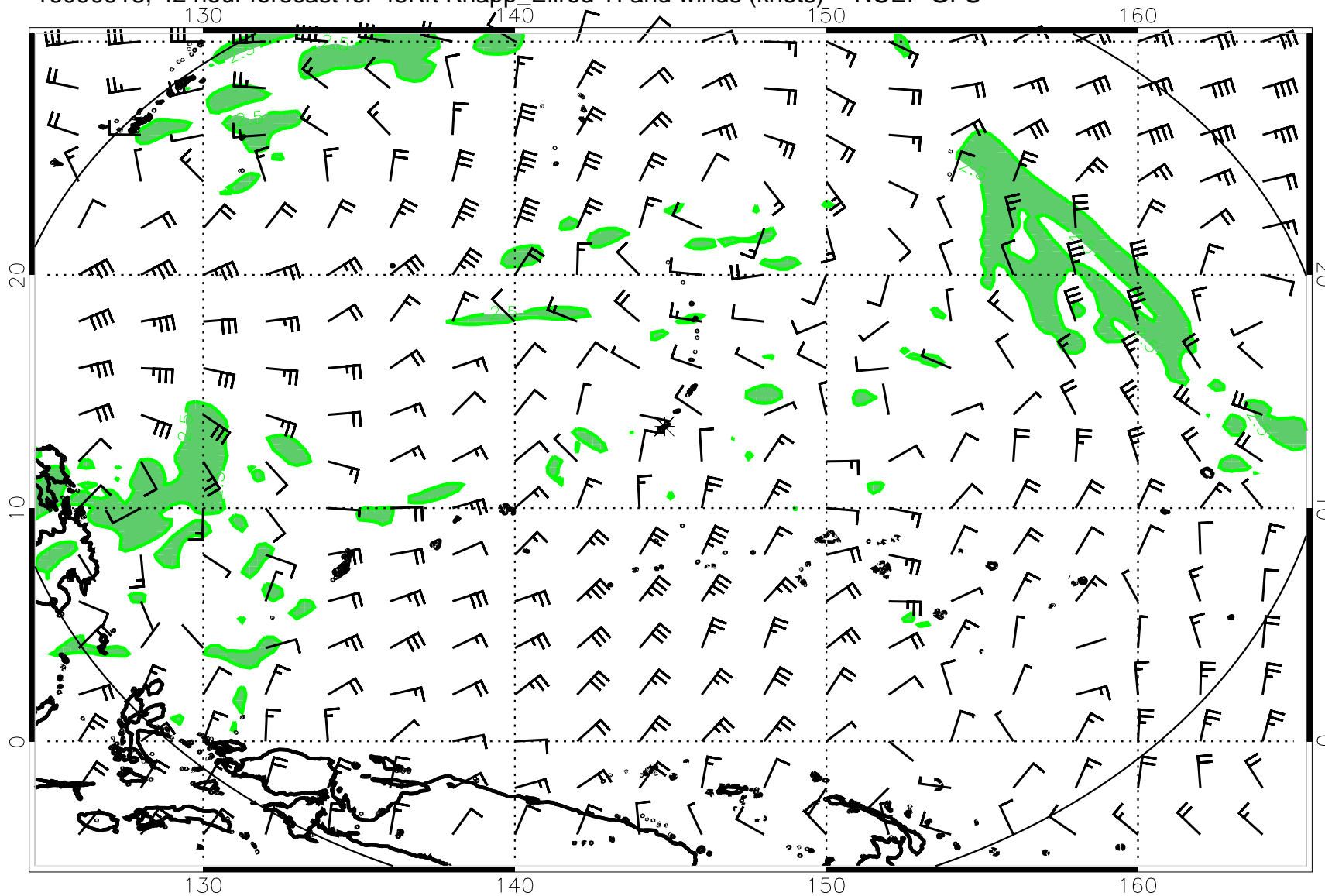
16090918, 42 hour forecast for 45Kft Knapp_Ellrod TI and winds (knots) -- NCEP GFS
