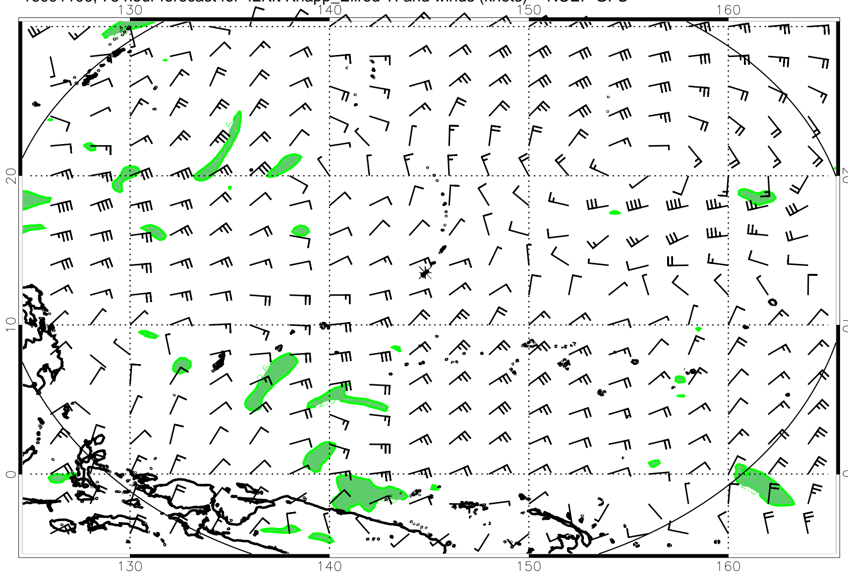
16091106, 78 hour forecast for 42Kft Knapp_Ellrod TI and winds (knots) -- NCEP GFS
