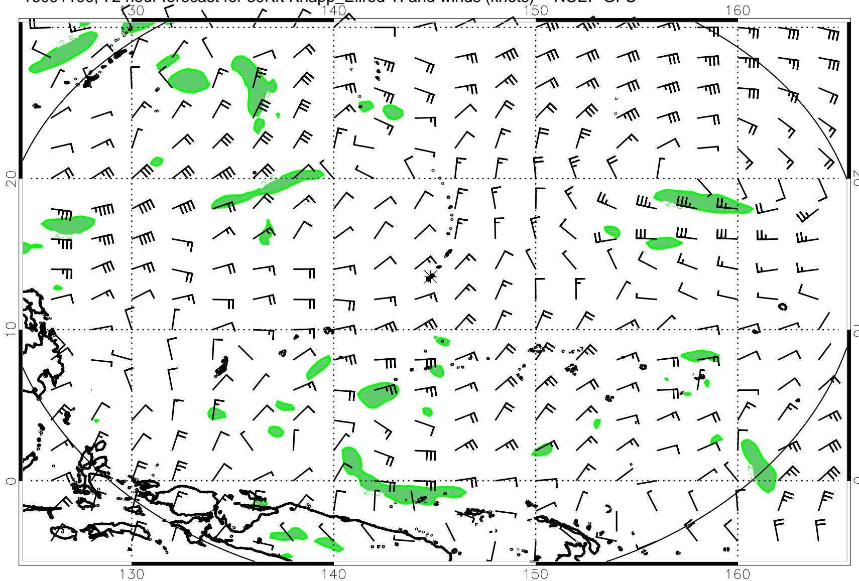
16091100, 72 hour forecast for 39Kft Knapp_Ellrod TI and winds (knots) -- NCEP GFS
