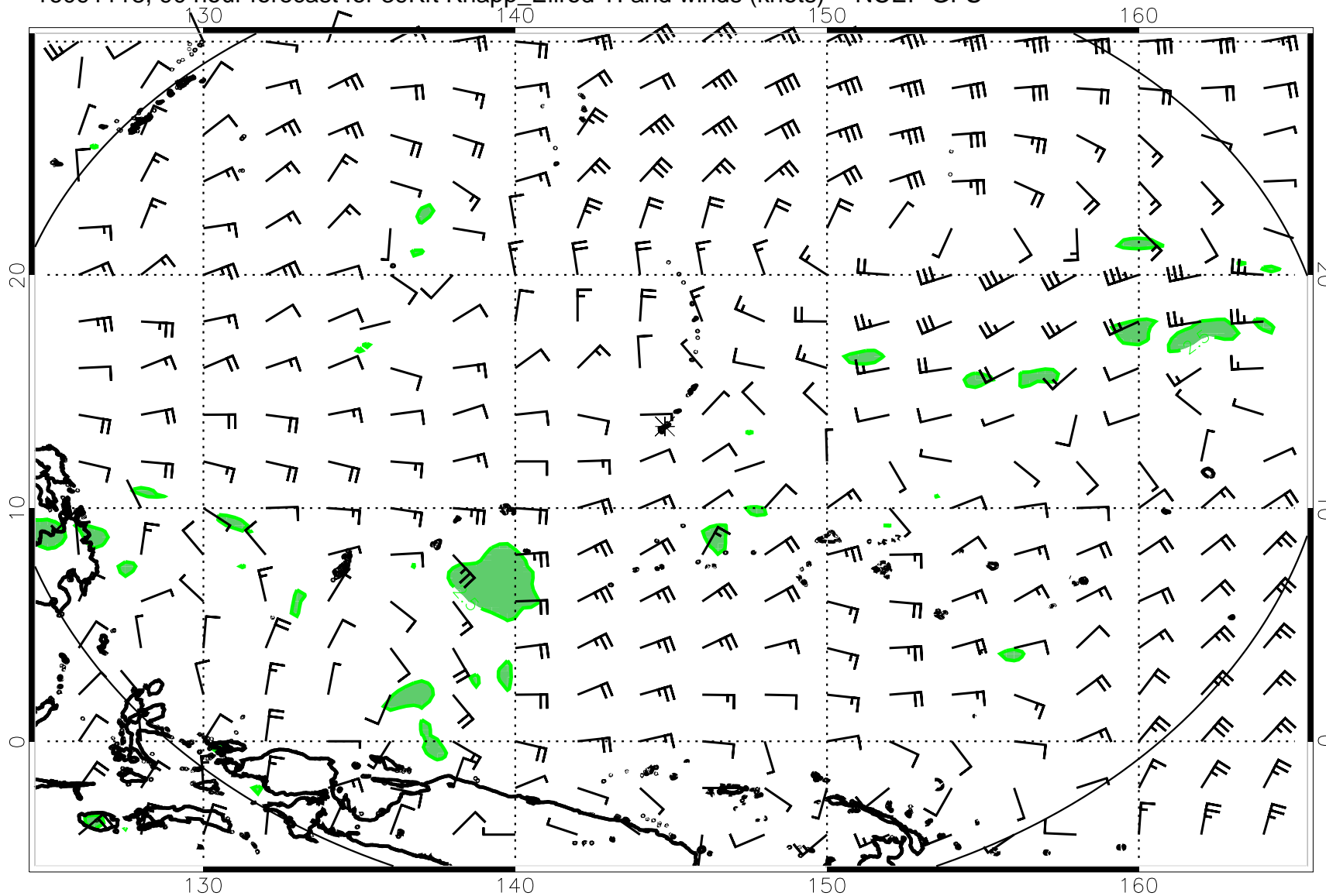
16091118, 90 hour forecast for 39Kft Knapp_Ellrod TI and winds (knots) -- NCEP GFS
