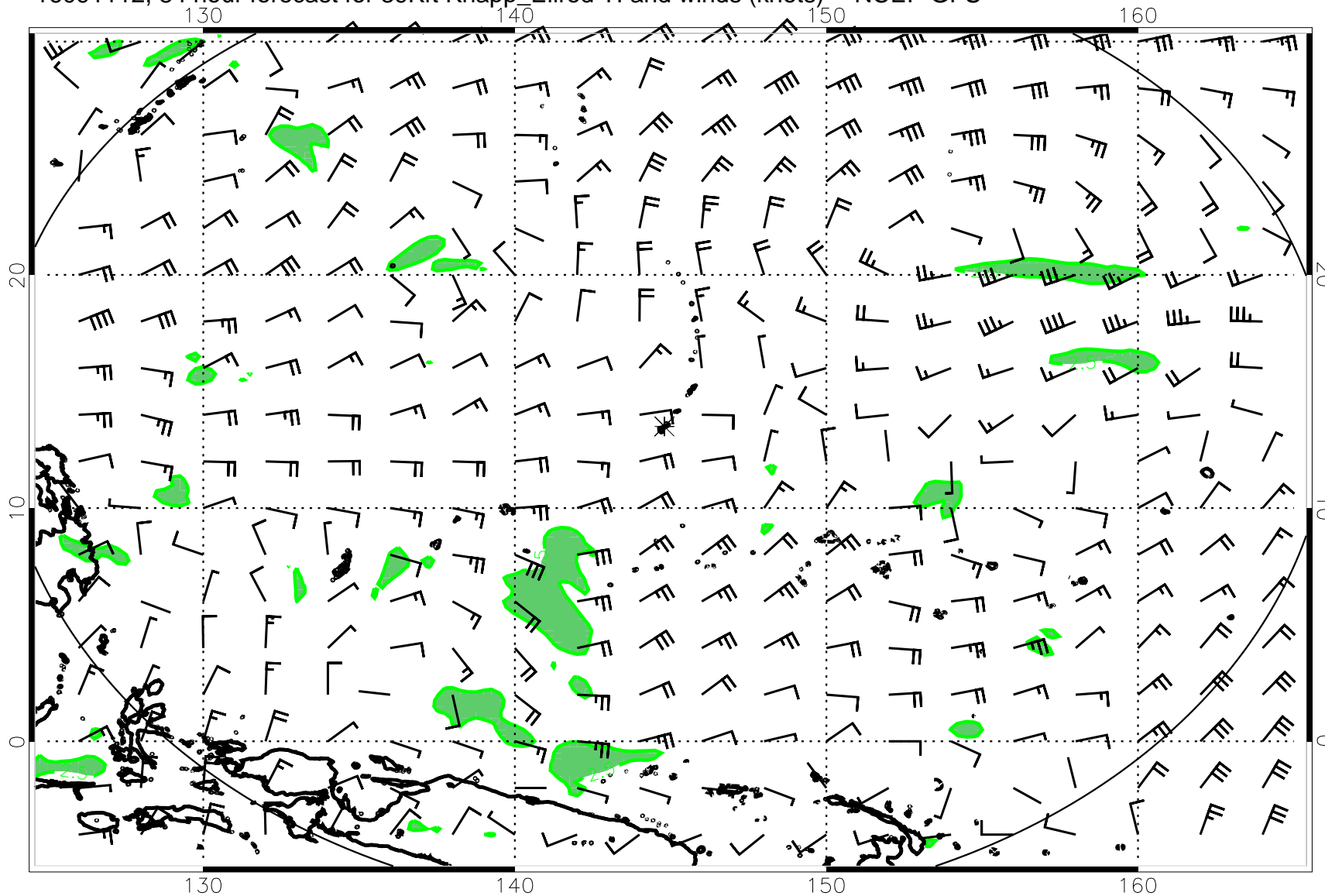
16091112, 84 hour forecast for 39Kft Knapp_Ellrod TI and winds (knots) -- NCEP GFS
