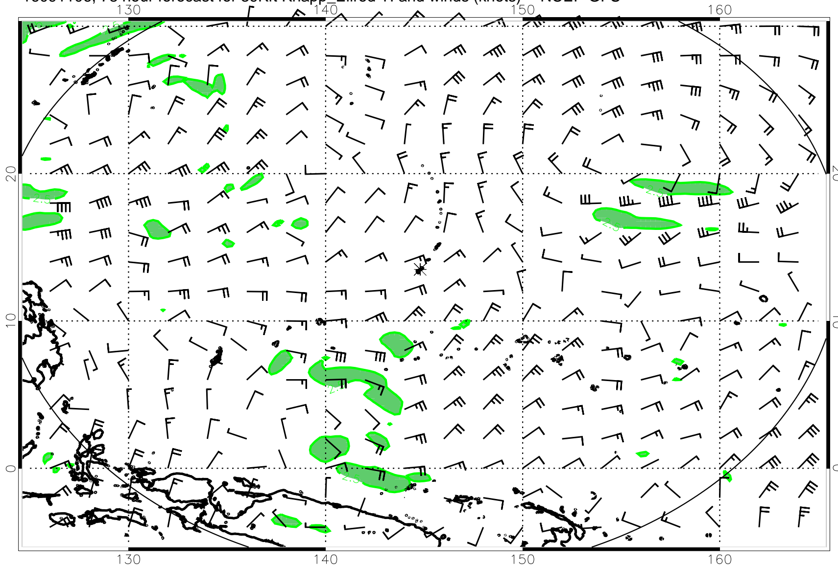
16091106, 78 hour forecast for 39Kft Knapp_Ellrod TI and winds (knots) -- NCEP GFS
