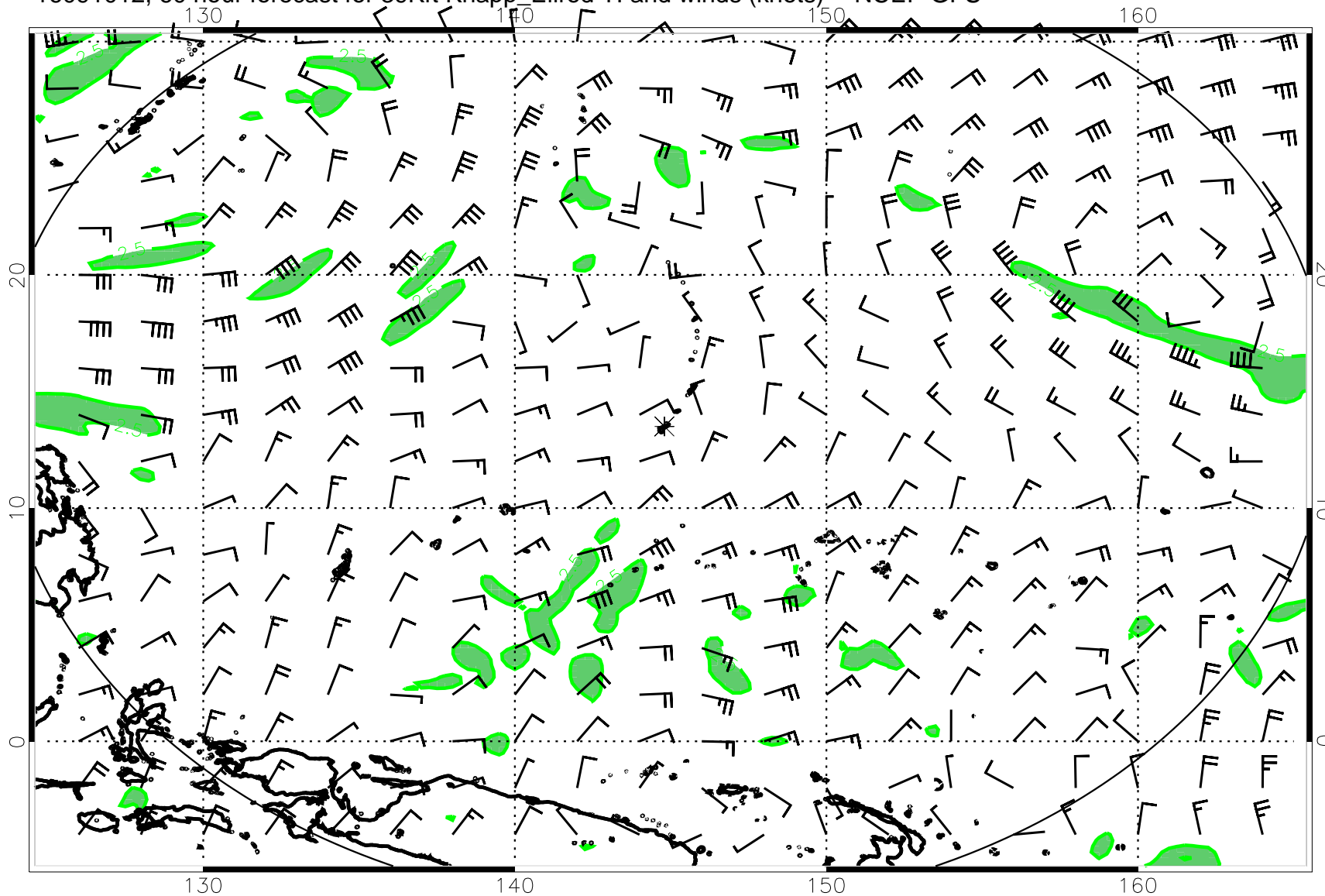
16091012, 60 hour forecast for 39Kft Knapp_Ellrod TI and winds (knots) -- NCEP GFS
