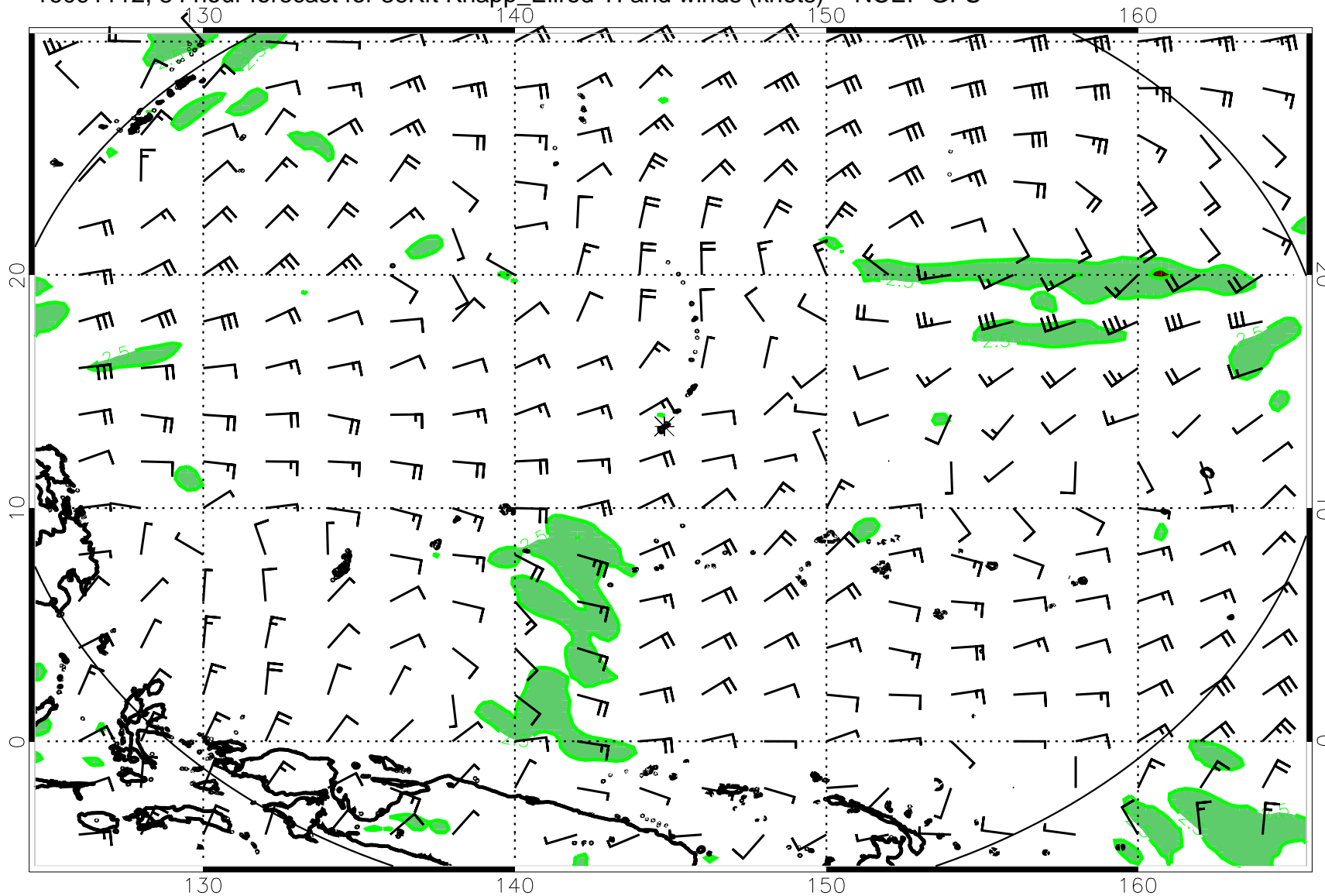
16091112, 84 hour forecast for 36Kft Knapp_Ellrod TI and winds (knots) -- NCEP GFS
