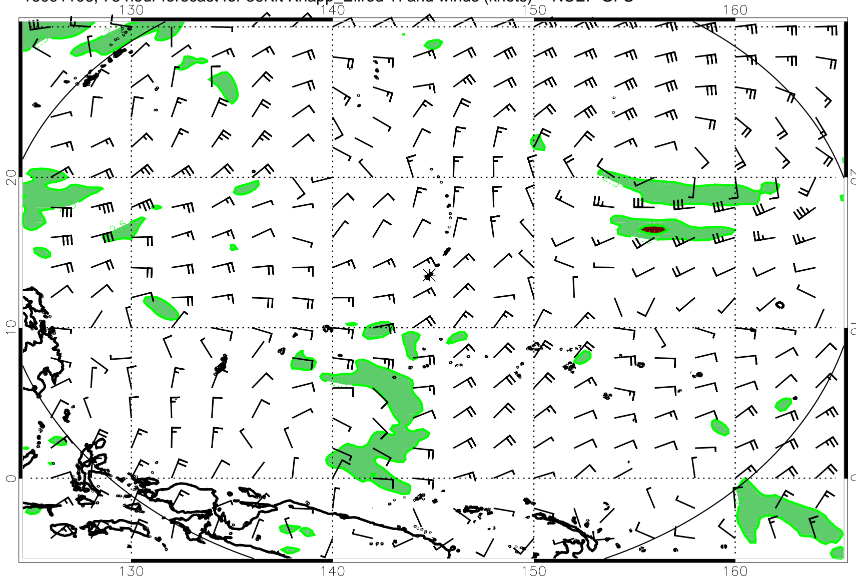
16091106, 78 hour forecast for 36Kft Knapp_Ellrod TI and winds (knots) -- NCEP GFS
