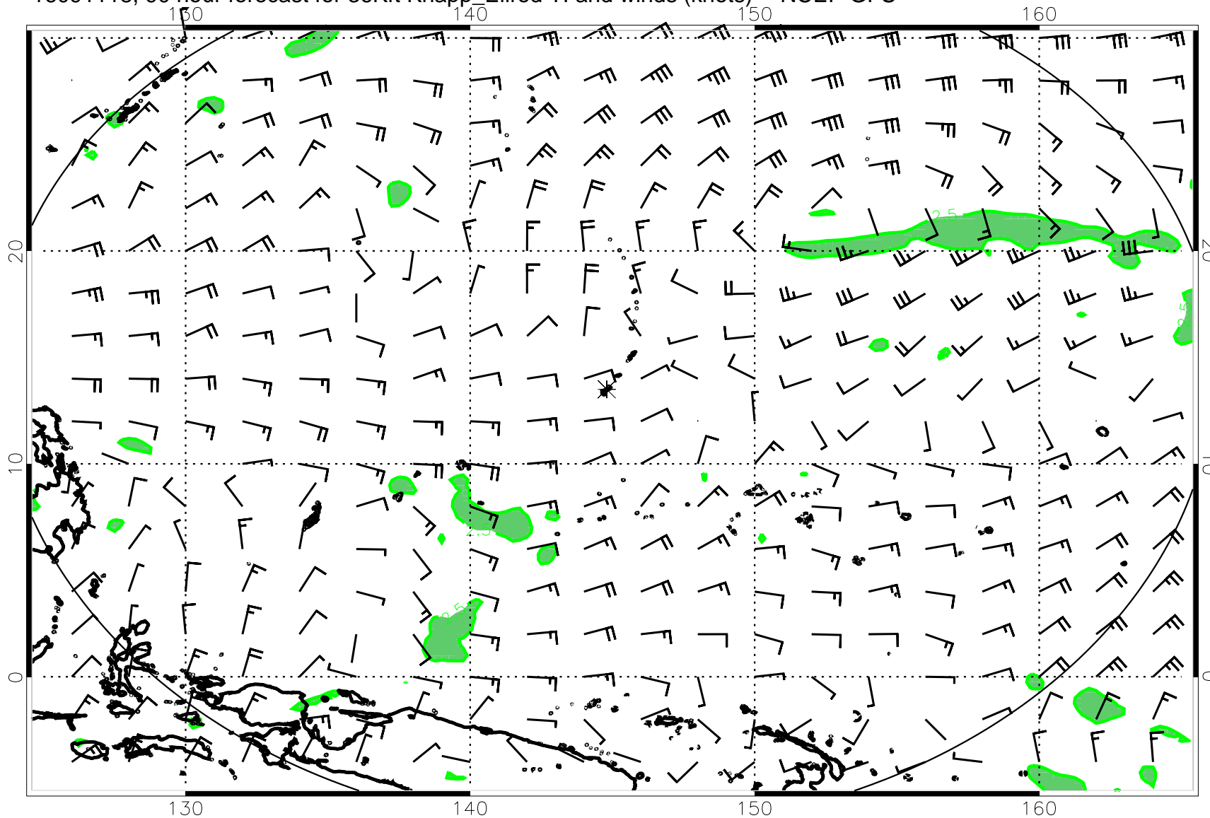
16091118, 90 hour forecast for 36Kft Knapp_Ellrod TI and winds (knots) -- NCEP GFS
