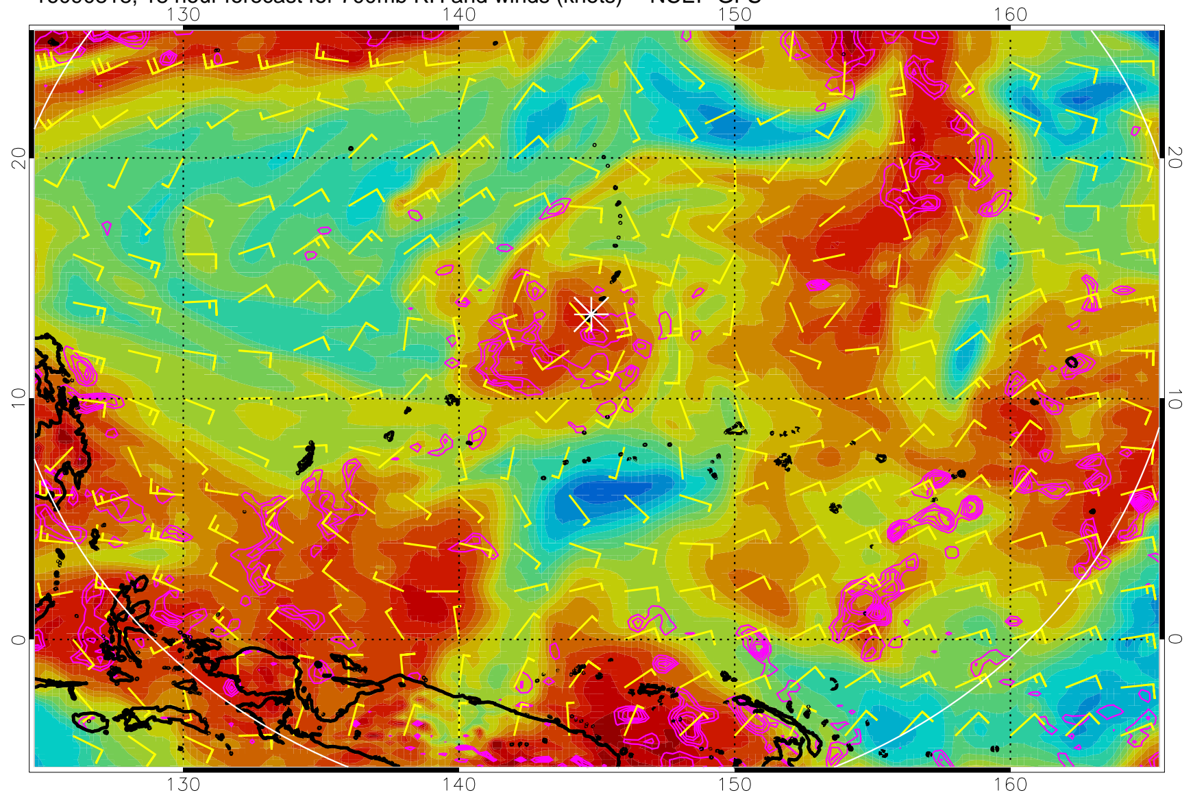
16090818, 18 hour forecast for 700mb RH and winds (knots) -- NCEP GFS
