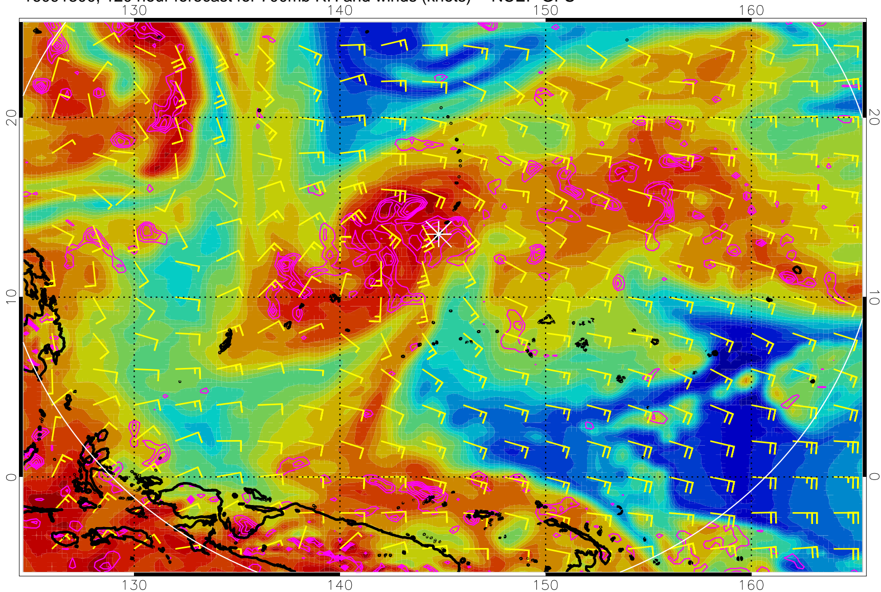
16091300, 120 hour forecast for 700mb RH and winds (knots) -- NCEP GFS
