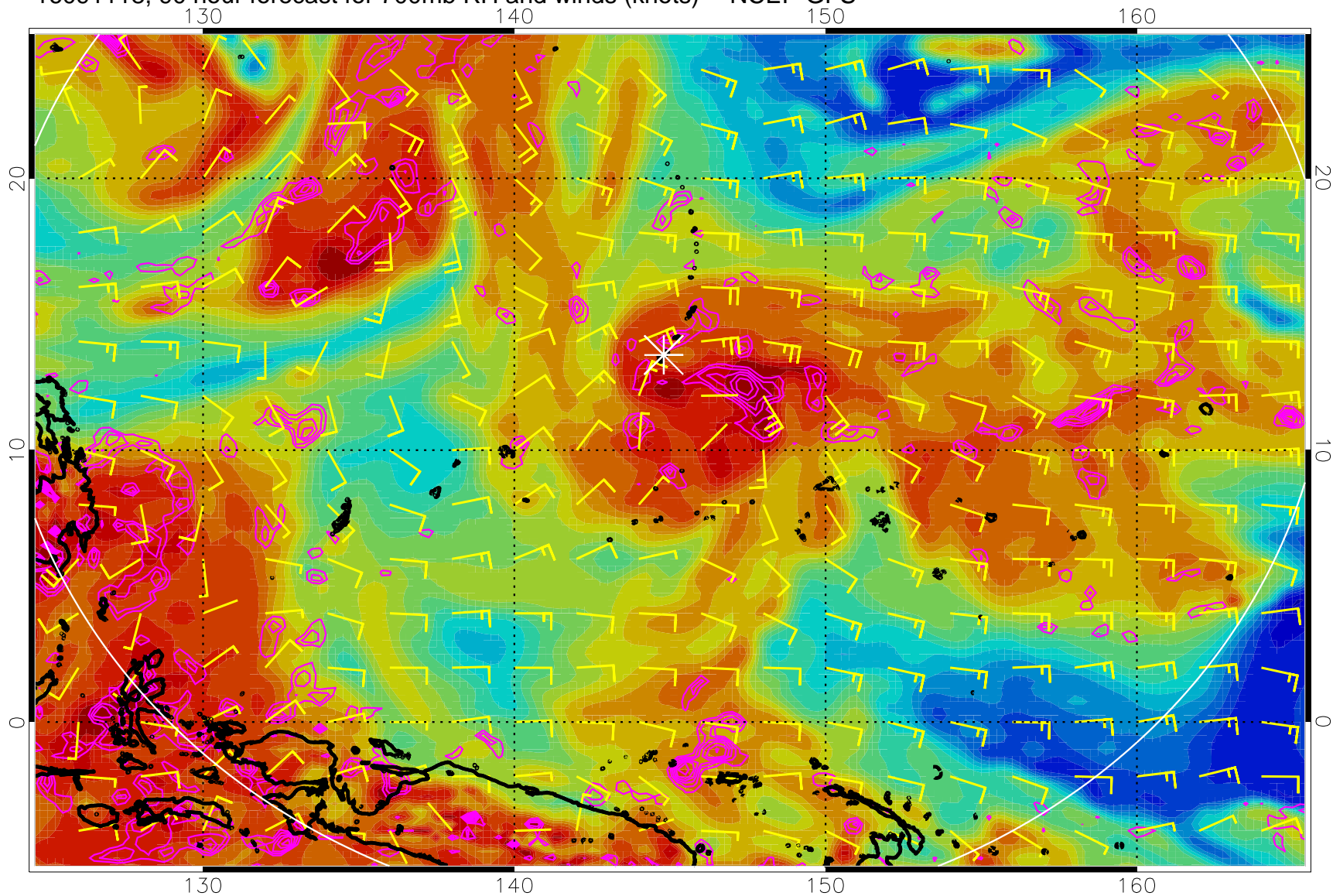
16091118, 90 hour forecast for 700mb RH and winds (knots) -- NCEP GFS
