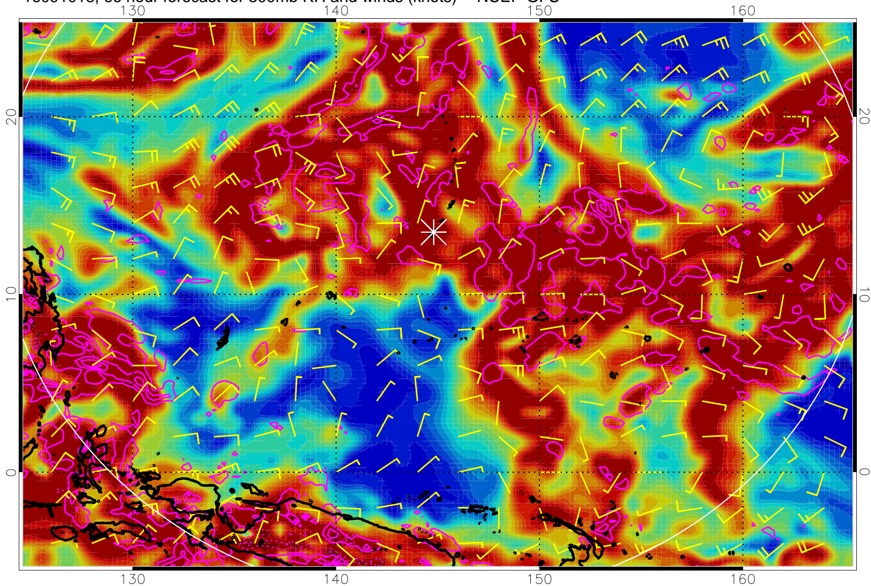
16091018, 66 hour forecast for 300mb RH and winds (knots) -- NCEP GFS
