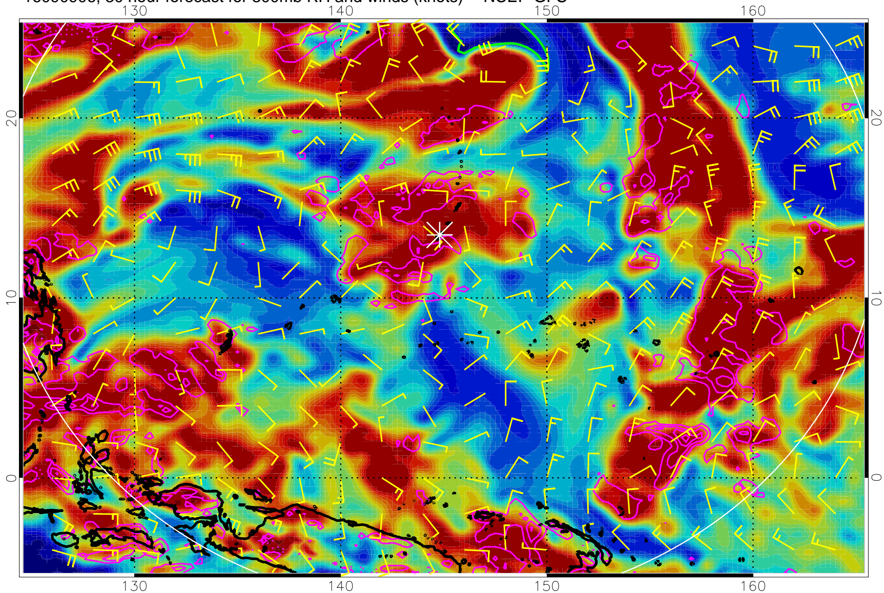
16090906, 30 hour forecast for 300mb RH and winds (knots) -- NCEP GFS
