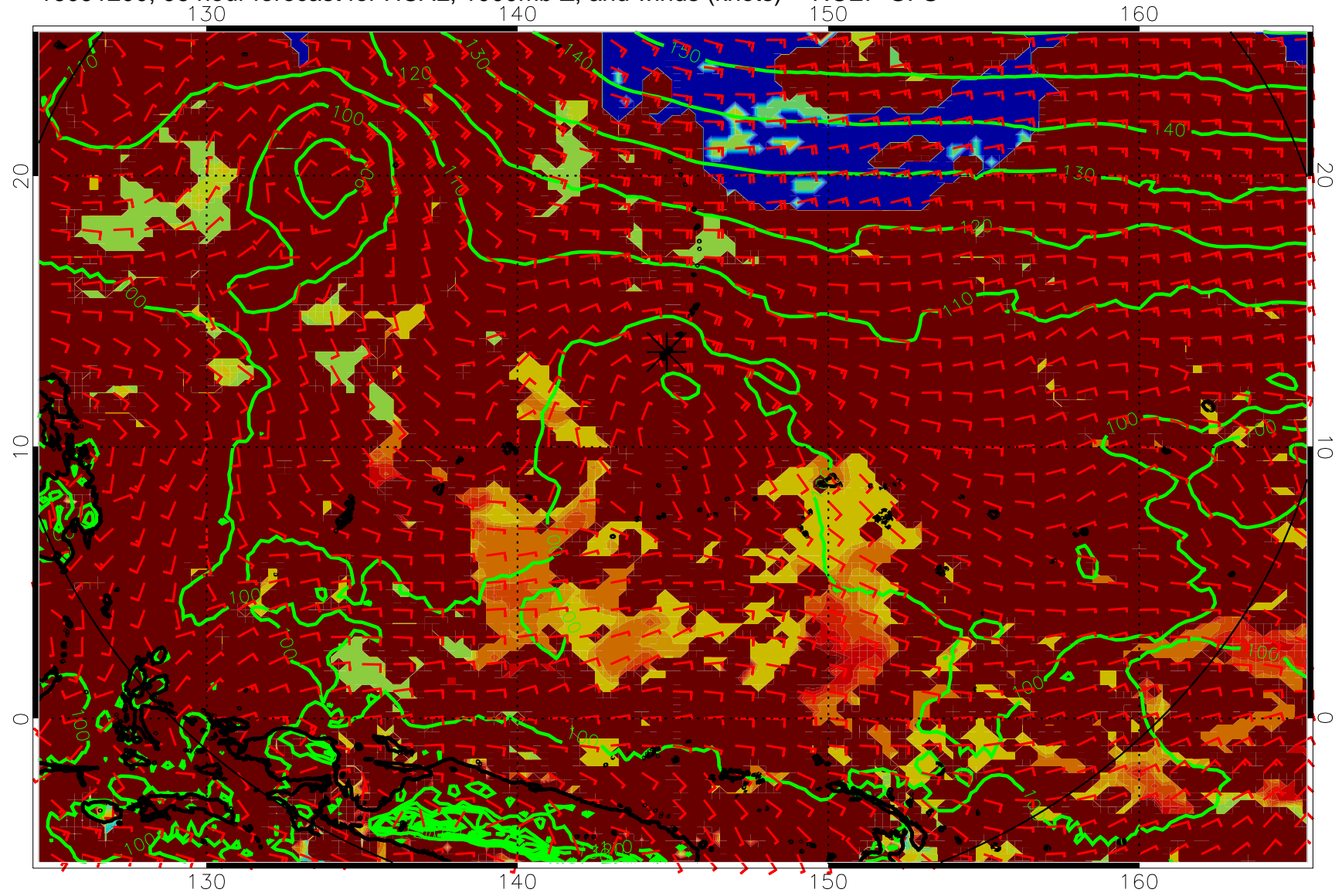
16091200, 96 hour forecast for HCAL, 1000mb Z, and winds (knots) -- NCEP GFS
