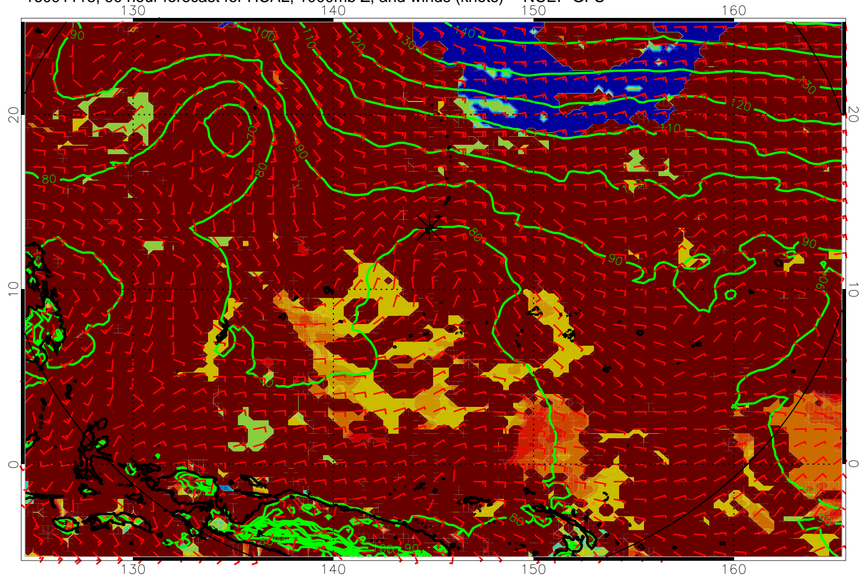
16091118, 90 hour forecast for HCAL, 1000mb Z, and winds (knots) -- NCEP GFS
