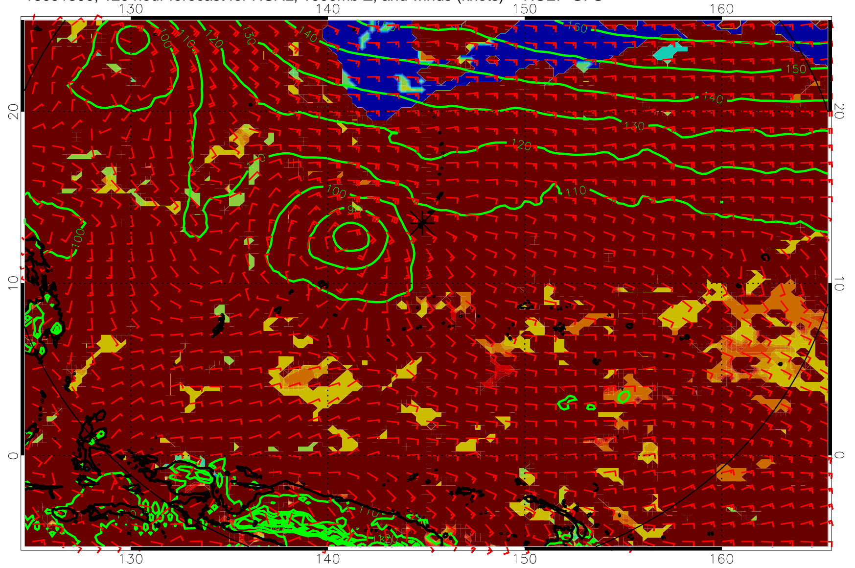
16091300, 120 hour forecast for HCAL, 1000mb Z, and winds (knots) -- NCEP GFS
