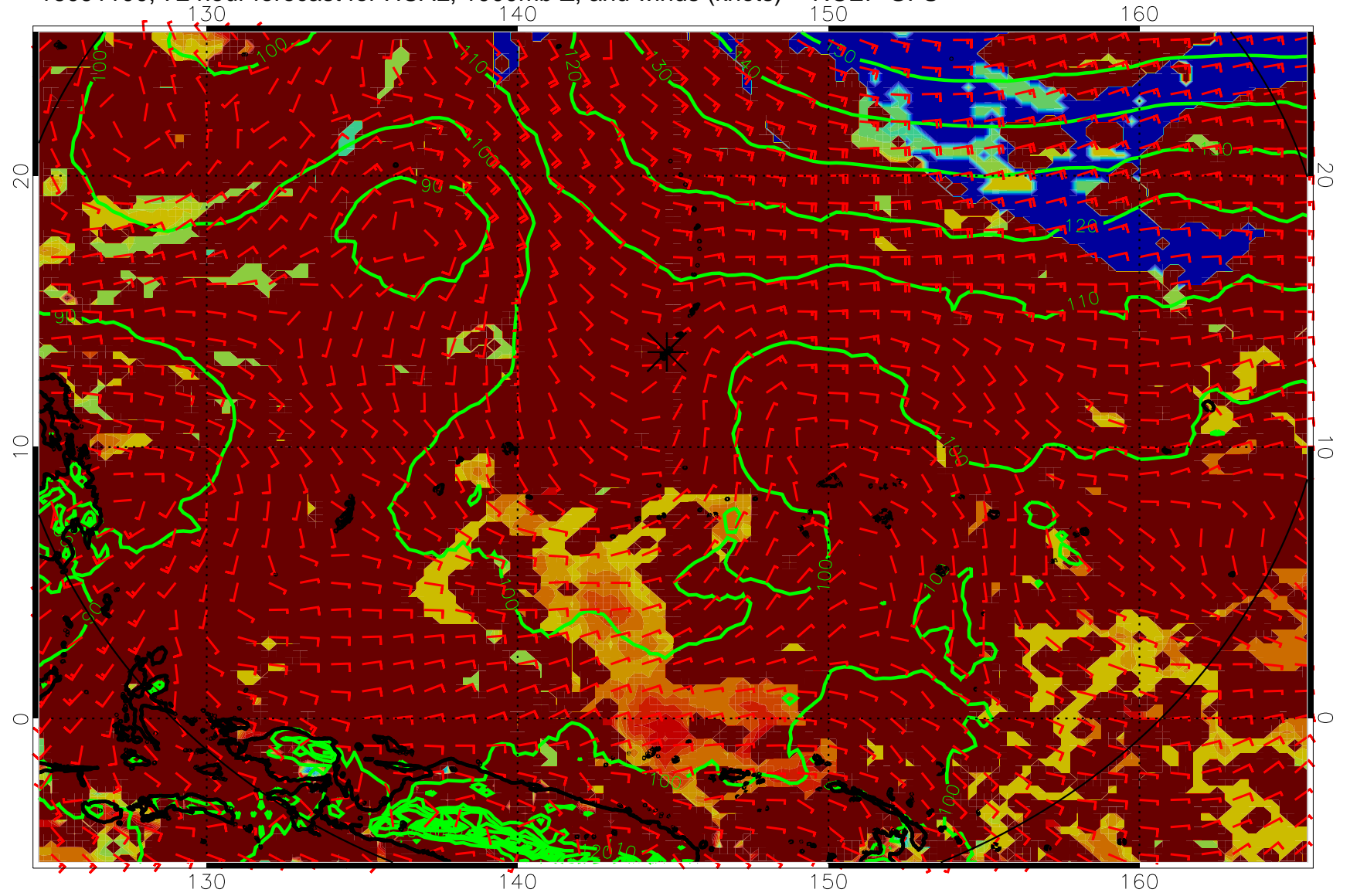
16091100, 72 hour forecast for HCAL, 1000mb Z, and winds (knots) -- NCEP GFS
