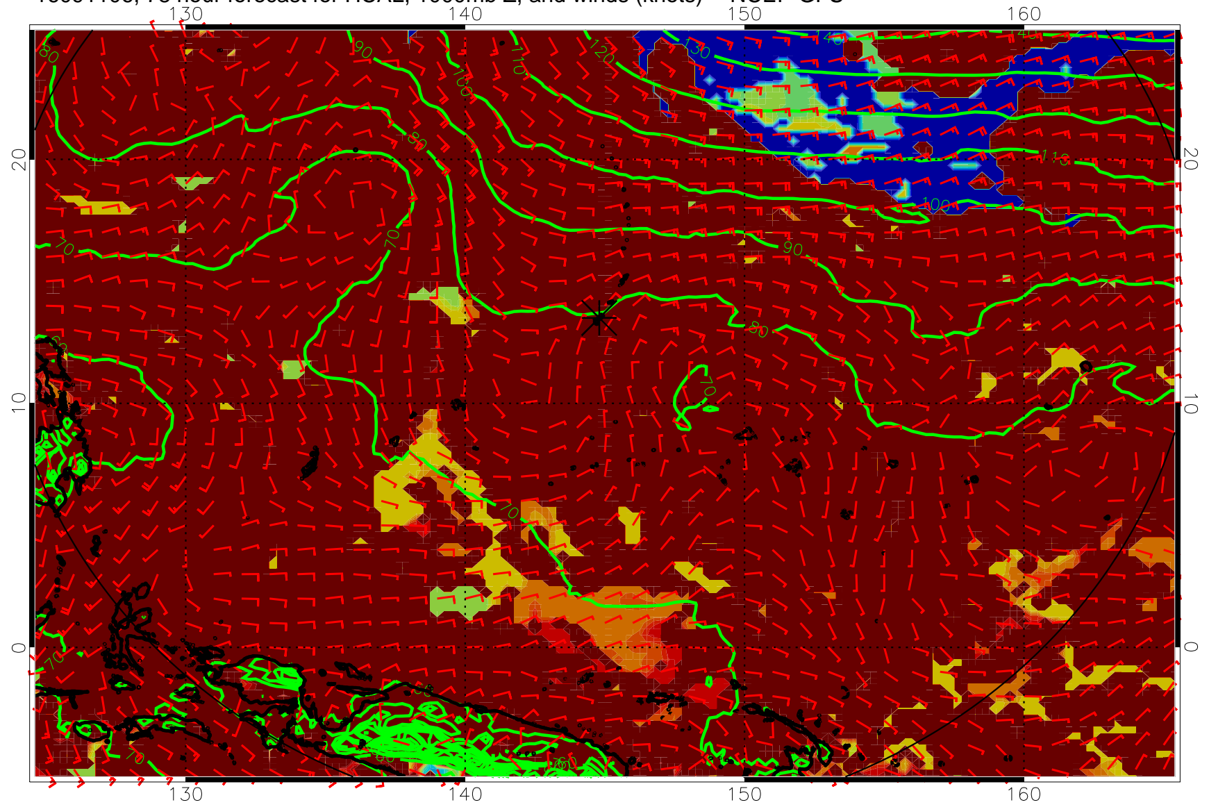
16091106, 78 hour forecast for HCAL, 1000mb Z, and winds (knots) -- NCEP GFS
