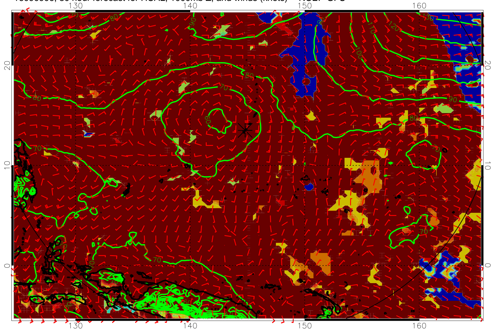
16090906, 30 hour forecast for HCAL, 1000mb Z, and winds (knots) -- NCEP GFS
