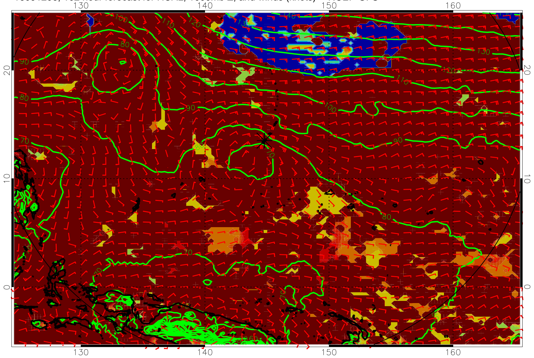
16091206, 102 hour forecast for HCAL, 1000mb Z, and winds (knots) -- NCEP GFS
