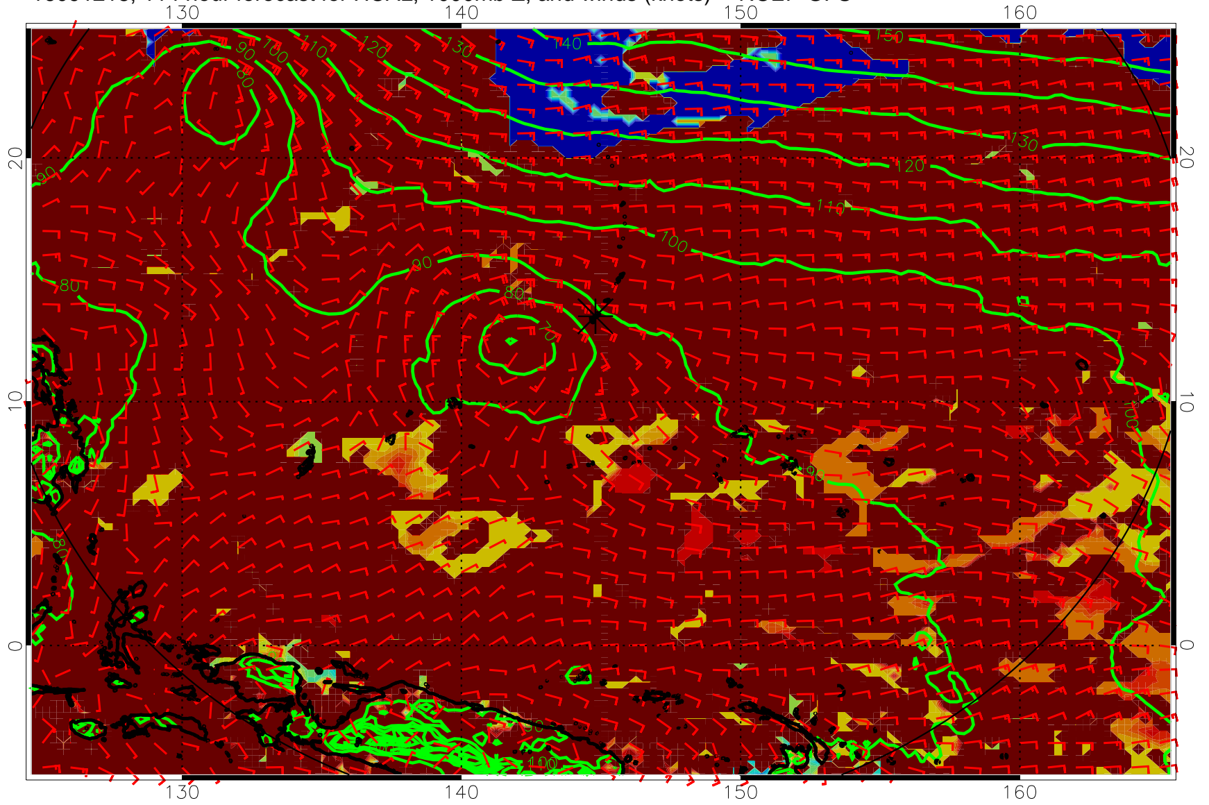
16091218, 114 hour forecast for HCAL, 1000mb Z, and winds (knots) -- NCEP GFS
