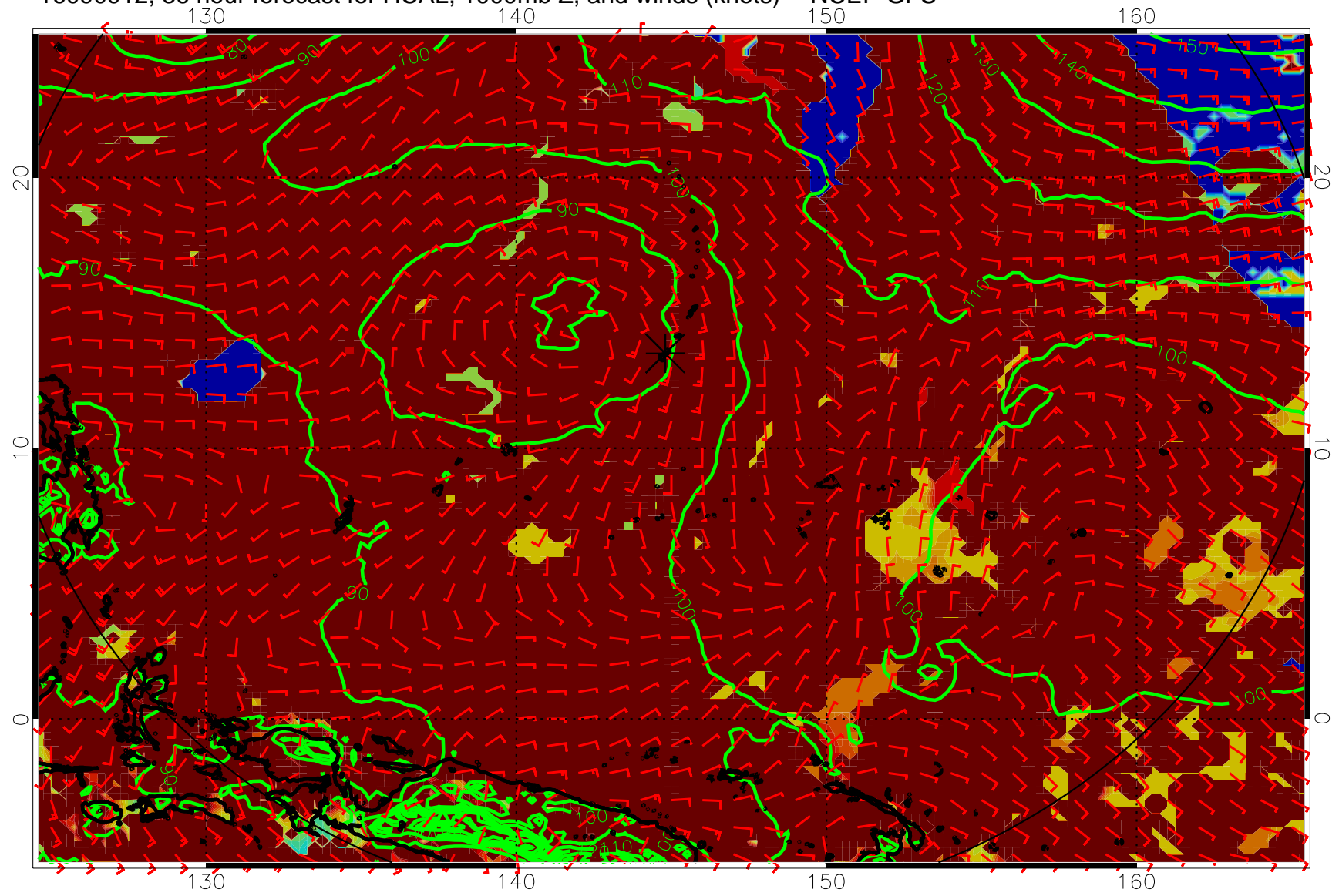
16090912, 36 hour forecast for HCAL, 1000mb Z, and winds (knots) -- NCEP GFS
