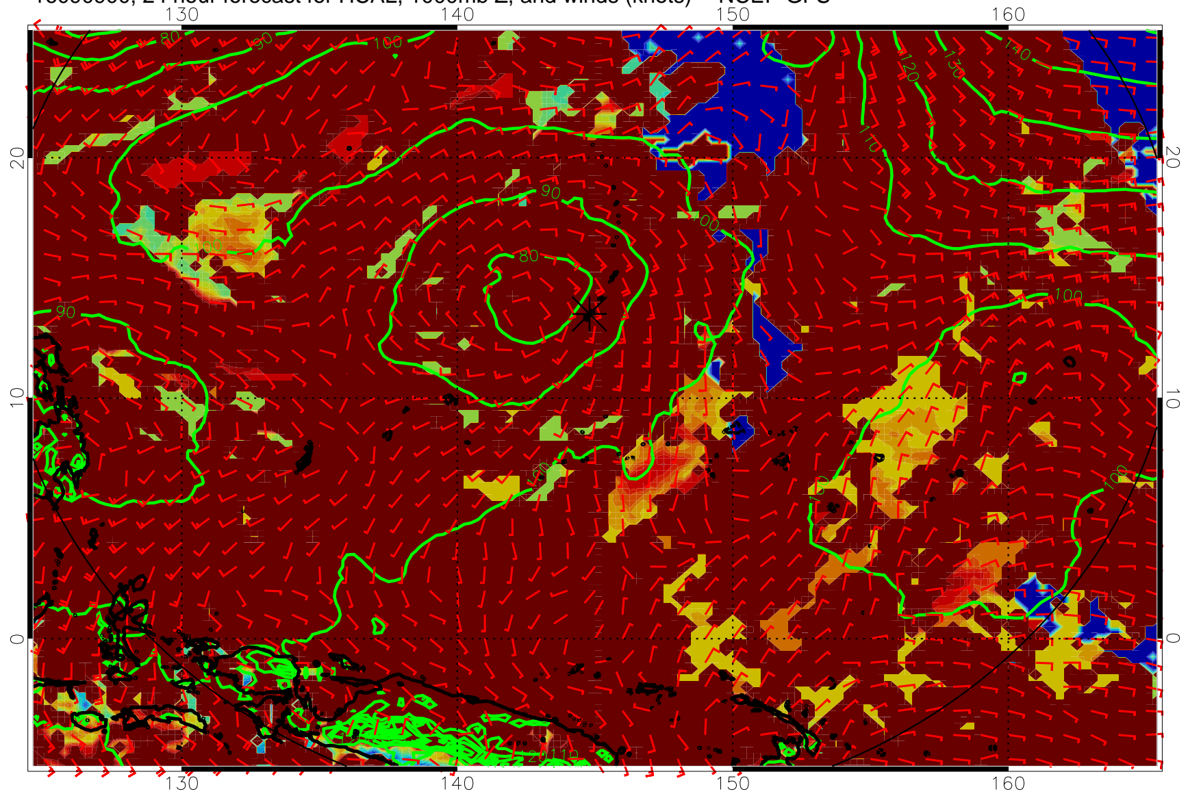
16090900, 24 hour forecast for HCAL, 1000mb Z, and winds (knots) -- NCEP GFS
