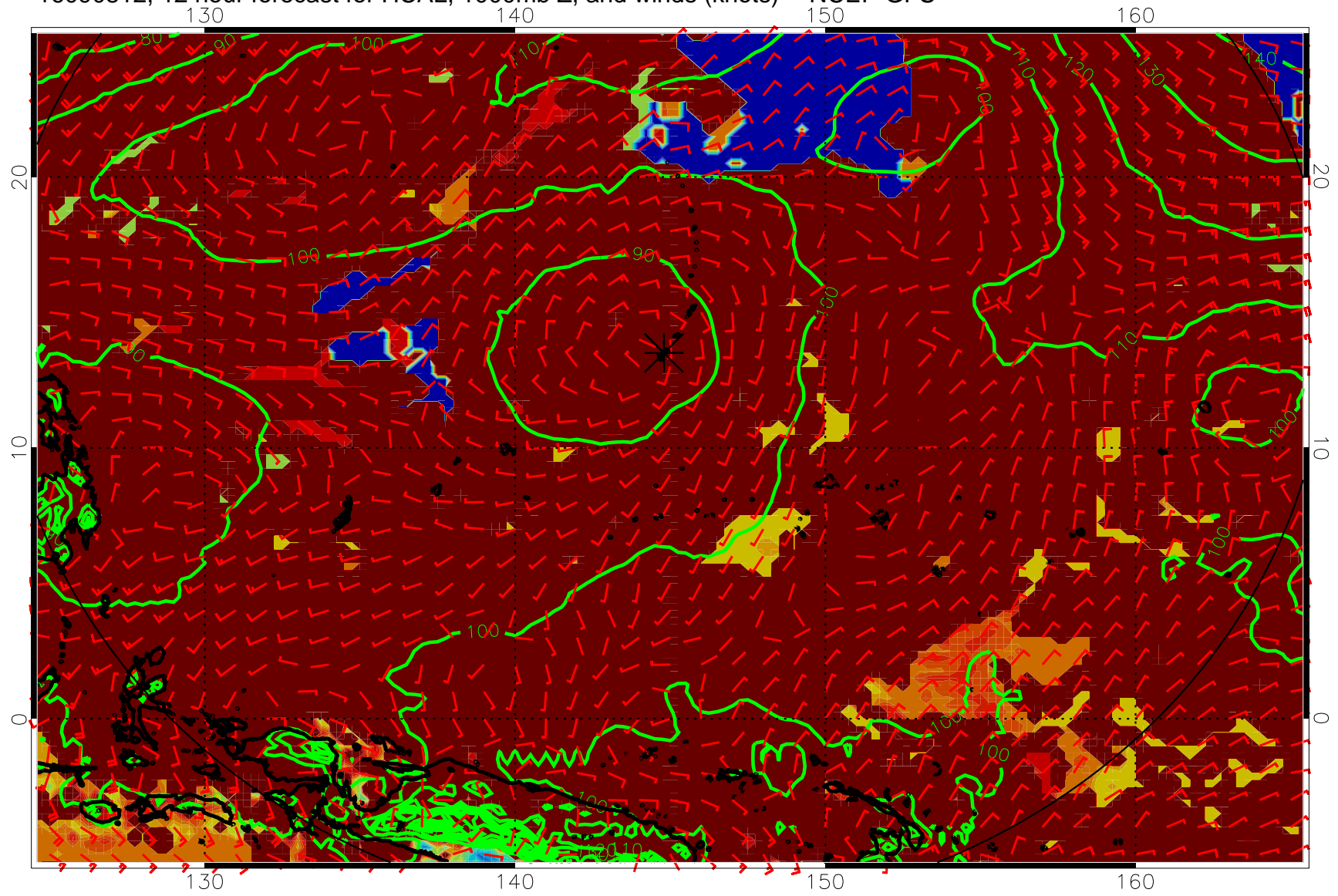
16090812, 12 hour forecast for HCAL, 1000mb Z, and winds (knots) -- NCEP GFS
