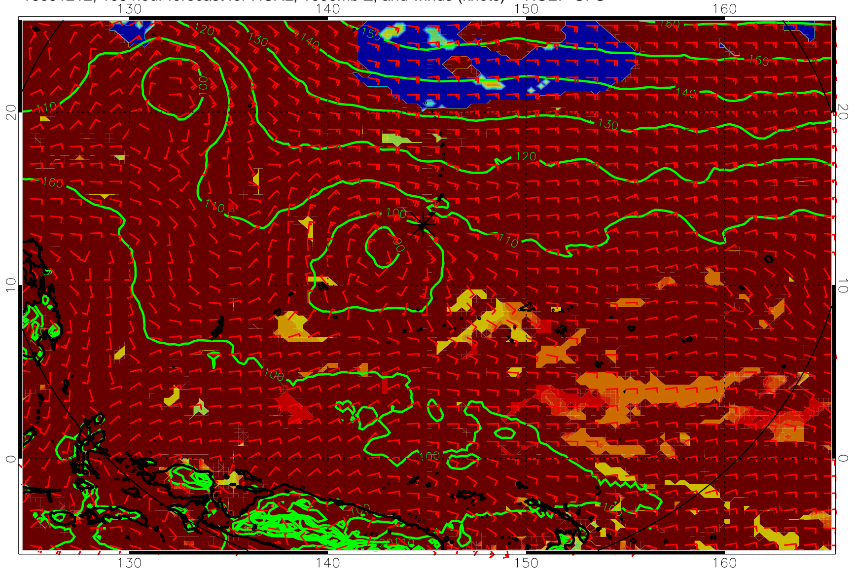
16091212, 108 hour forecast for HCAL, 1000mb Z, and winds (knots) -- NCEP GFS
