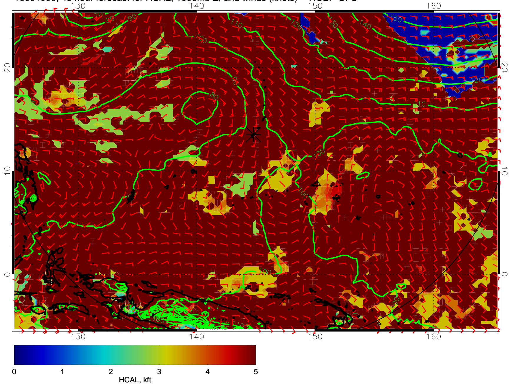
16091000, 48 hour forecast for HCAL, 1000mb Z, and winds (knots) -- NCEP GFS
