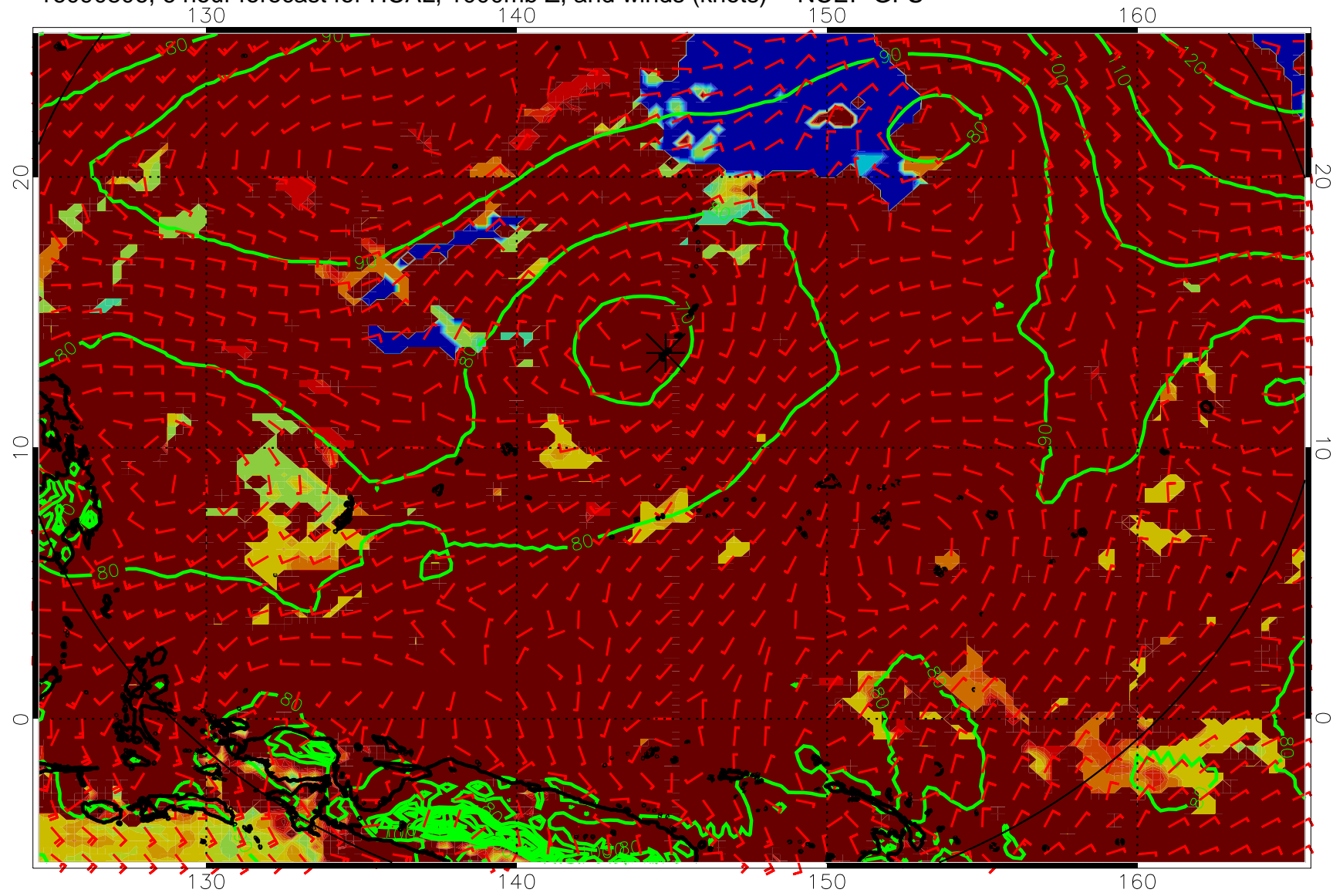
16090806, 6 hour forecast for HCAL, 1000mb Z, and winds (knots) -- NCEP GFS
