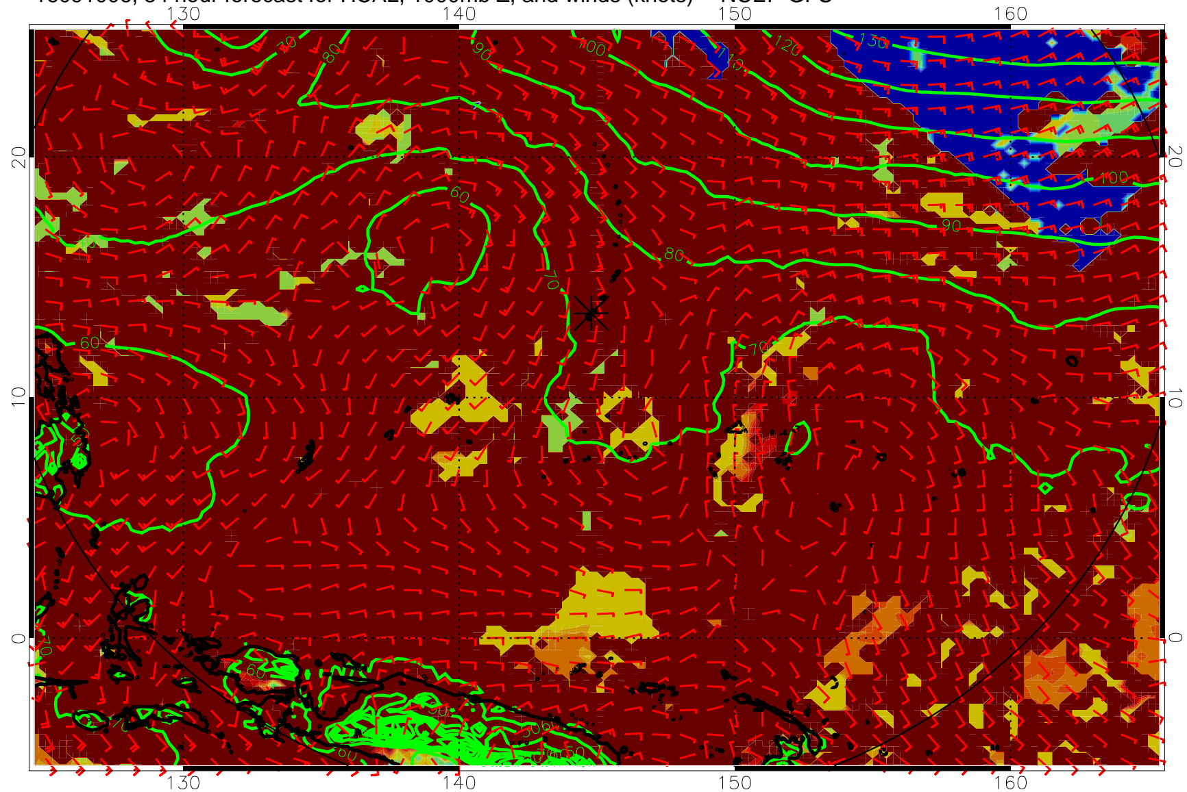
16091006, 54 hour forecast for HCAL, 1000mb Z, and winds (knots) -- NCEP GFS
