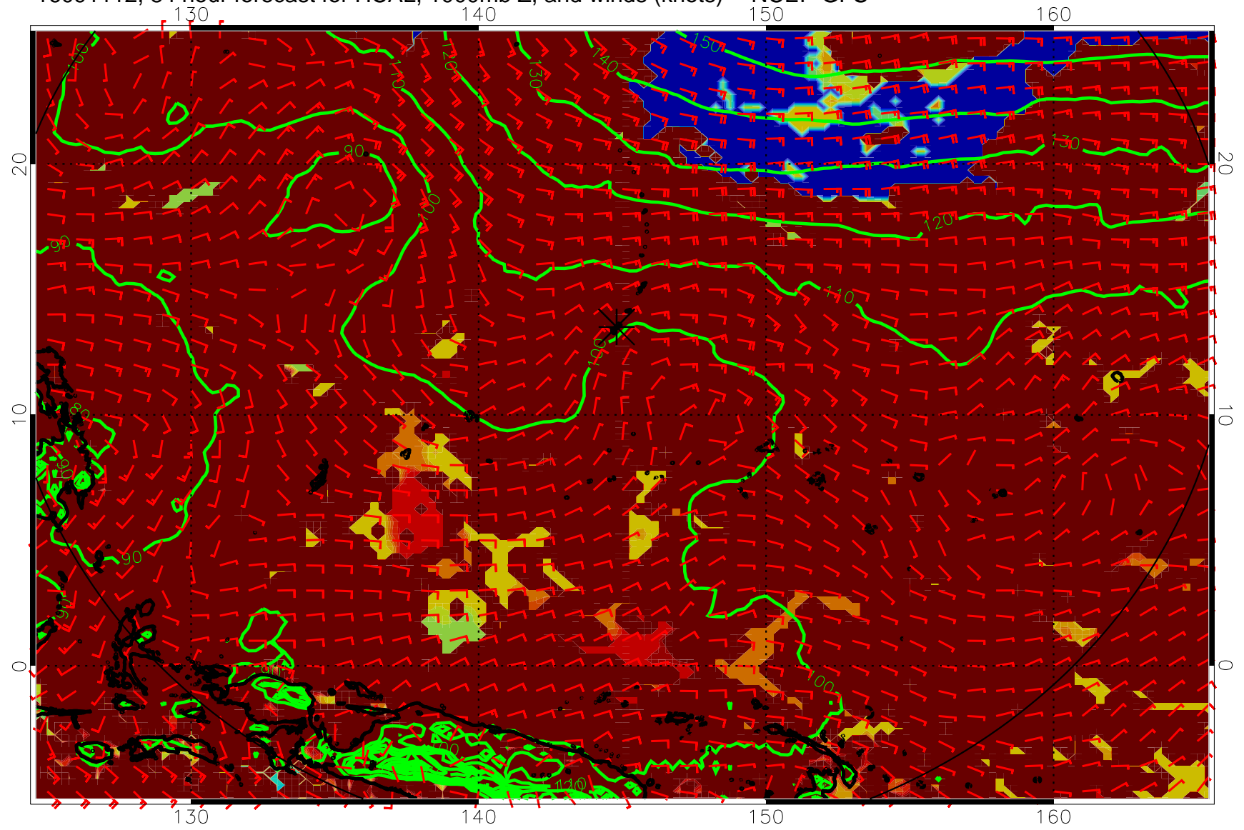
16091112, 84 hour forecast for HCAL, 1000mb Z, and winds (knots) -- NCEP GFS
