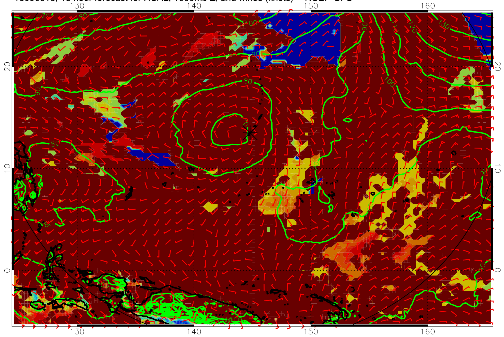
16090818, 18 hour forecast for HCAL, 1000mb Z, and winds (knots) -- NCEP GFS
