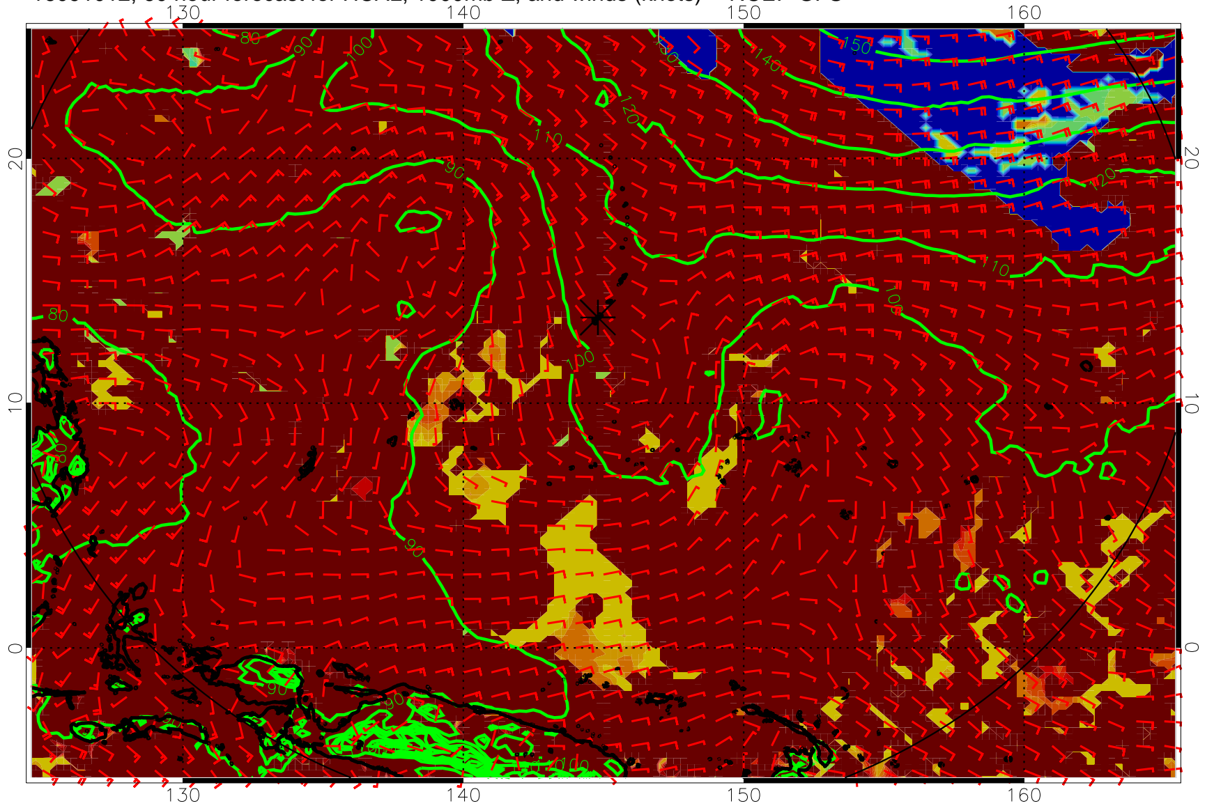
16091012, 60 hour forecast for HCAL, 1000mb Z, and winds (knots) -- NCEP GFS
