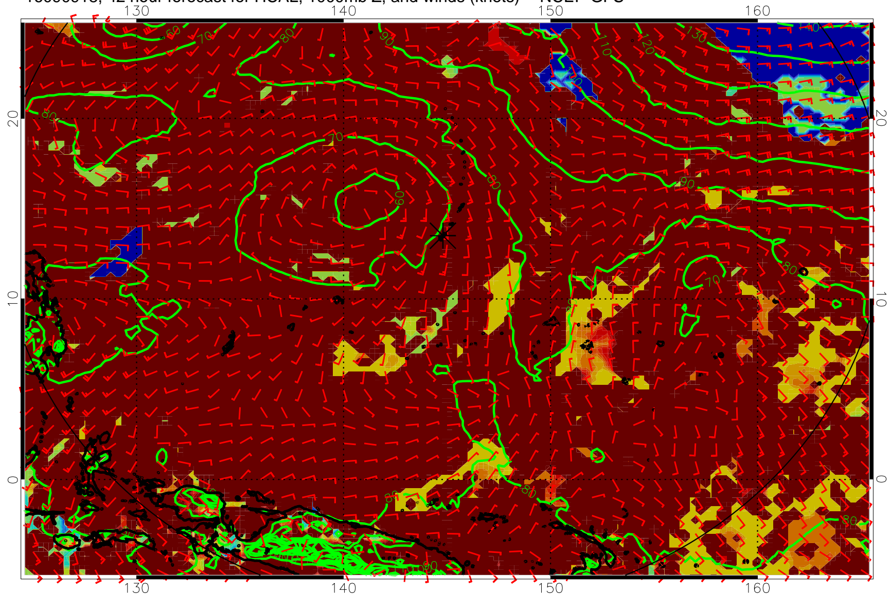
16090918, 42 hour forecast for HCAL, 1000mb Z, and winds (knots) -- NCEP GFS
