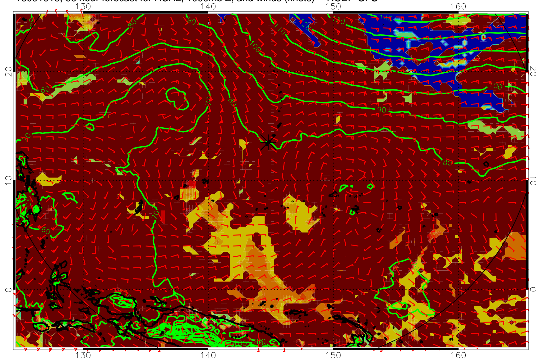
16091018, 66 hour forecast for HCAL, 1000mb Z, and winds (knots) -- NCEP GFS
