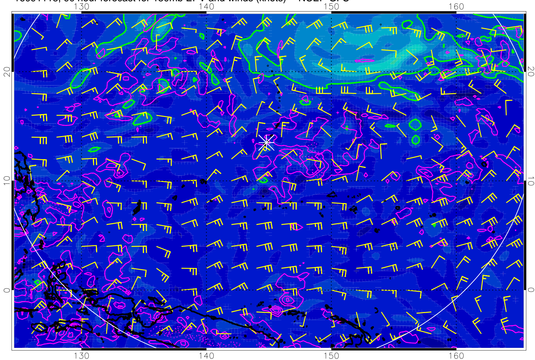
16091118, 90 hour forecast for 150mb EPV and winds (knots) -- NCEP GFS
