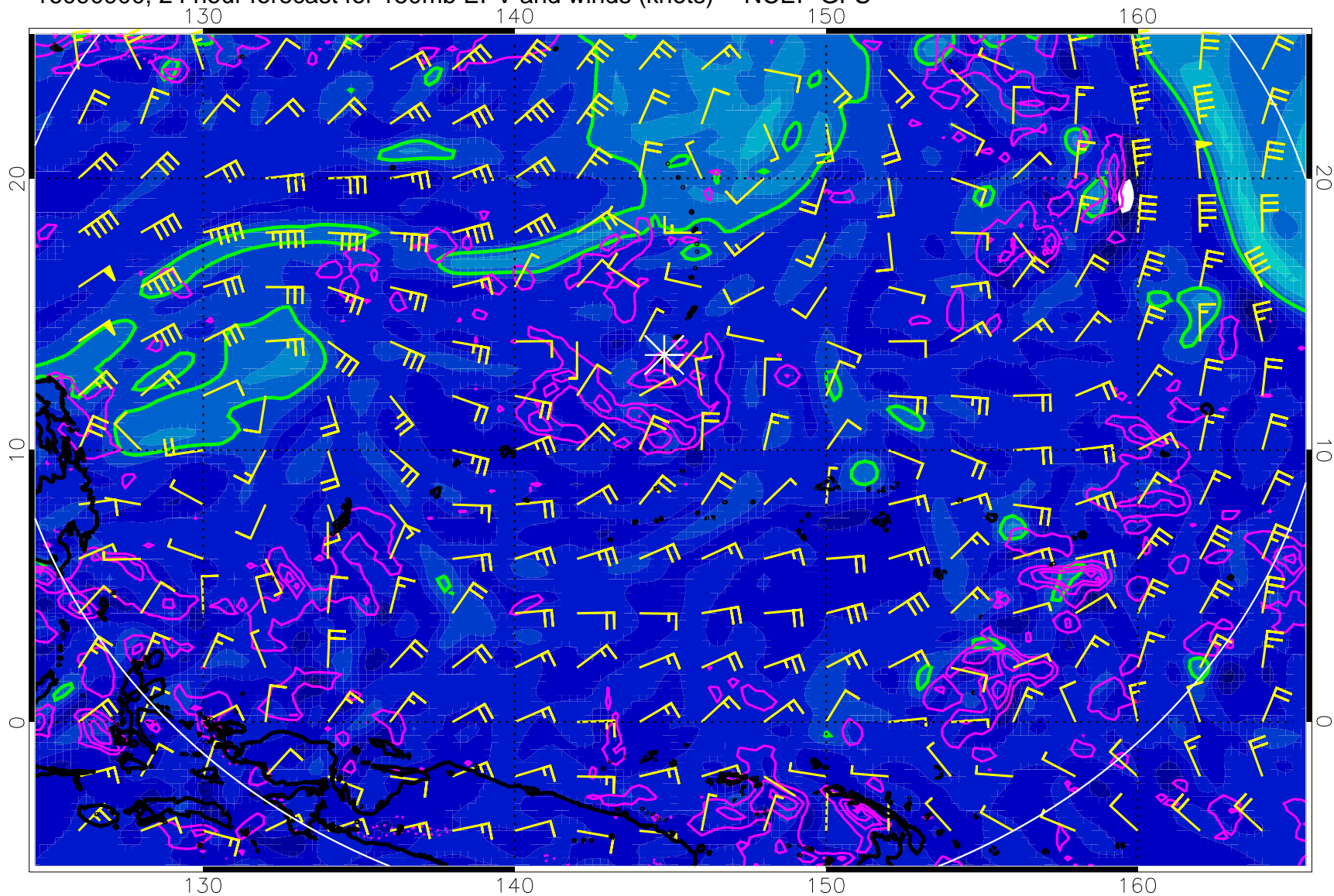
16090900, 24 hour forecast for 150mb EPV and winds (knots) -- NCEP GFS
