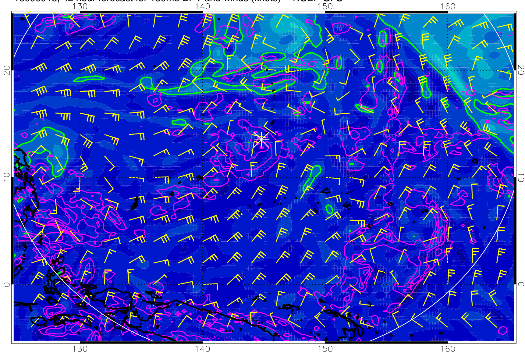
16090918, 42 hour forecast for 150mb EPV and winds (knots) -- NCEP GFS
