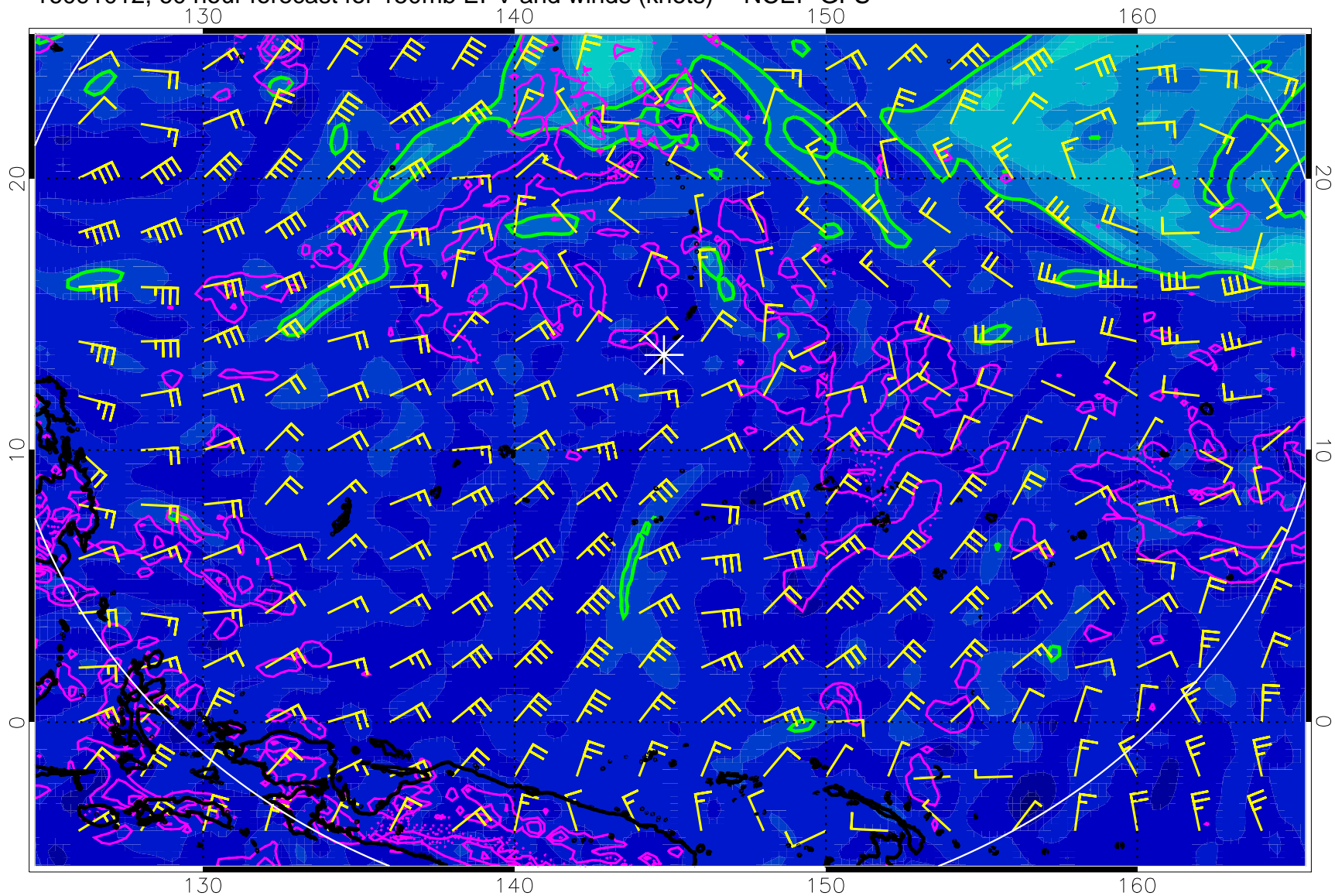
16091012, 60 hour forecast for 150mb EPV and winds (knots) -- NCEP GFS
