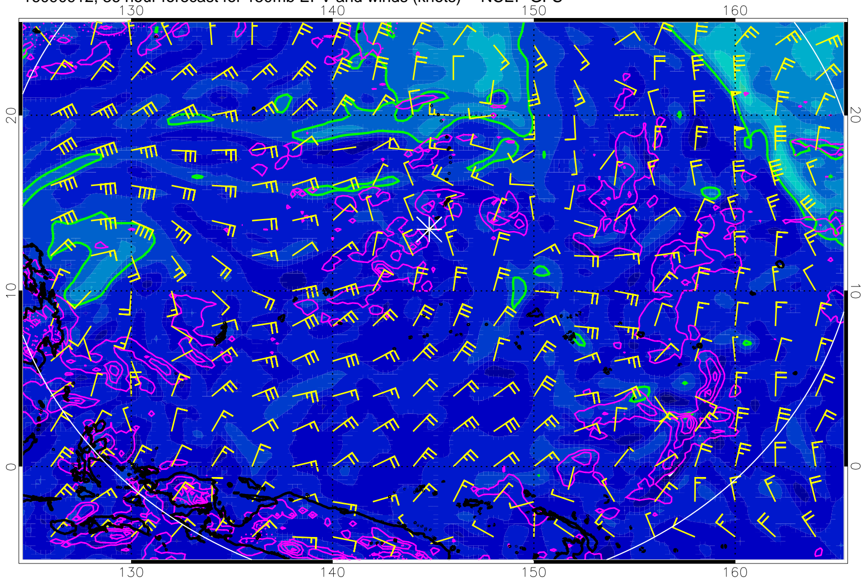
16090912, 36 hour forecast for 150mb EPV and winds (knots) -- NCEP GFS
