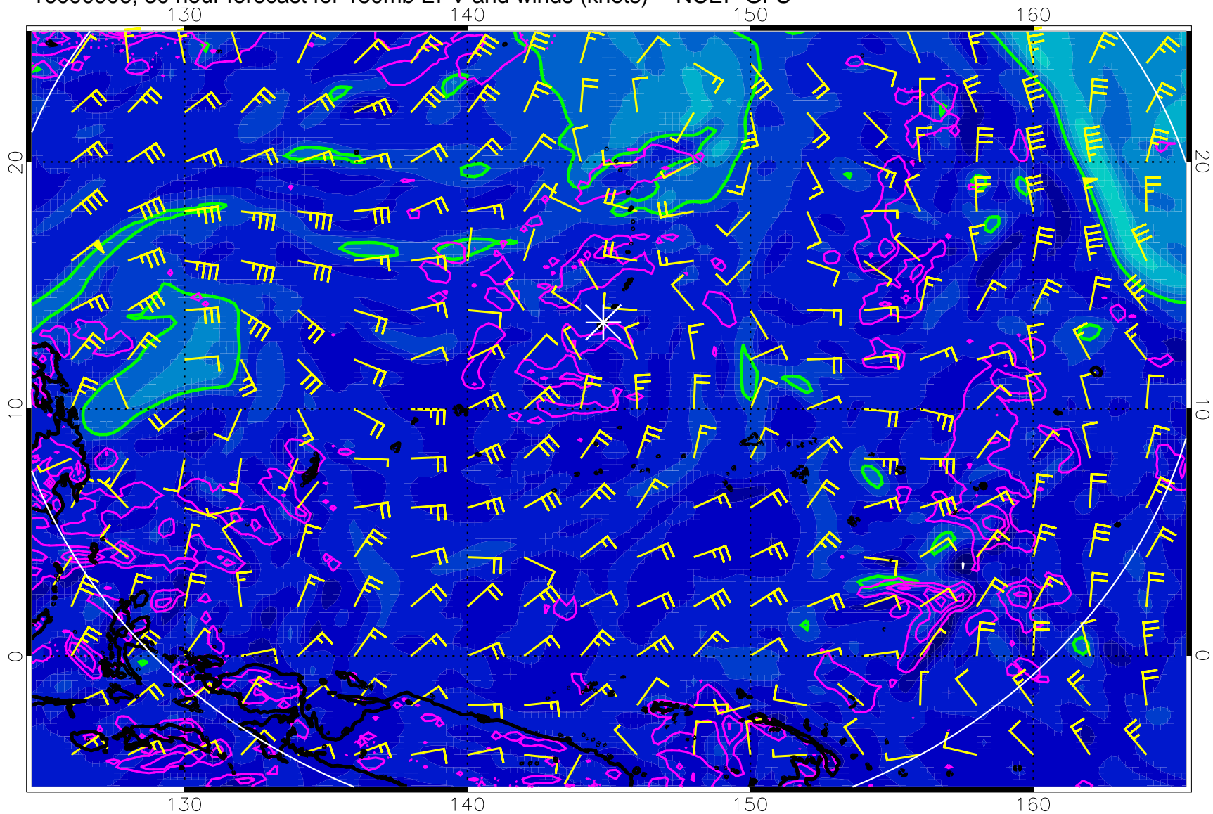
16090906, 30 hour forecast for 150mb EPV and winds (knots) -- NCEP GFS
