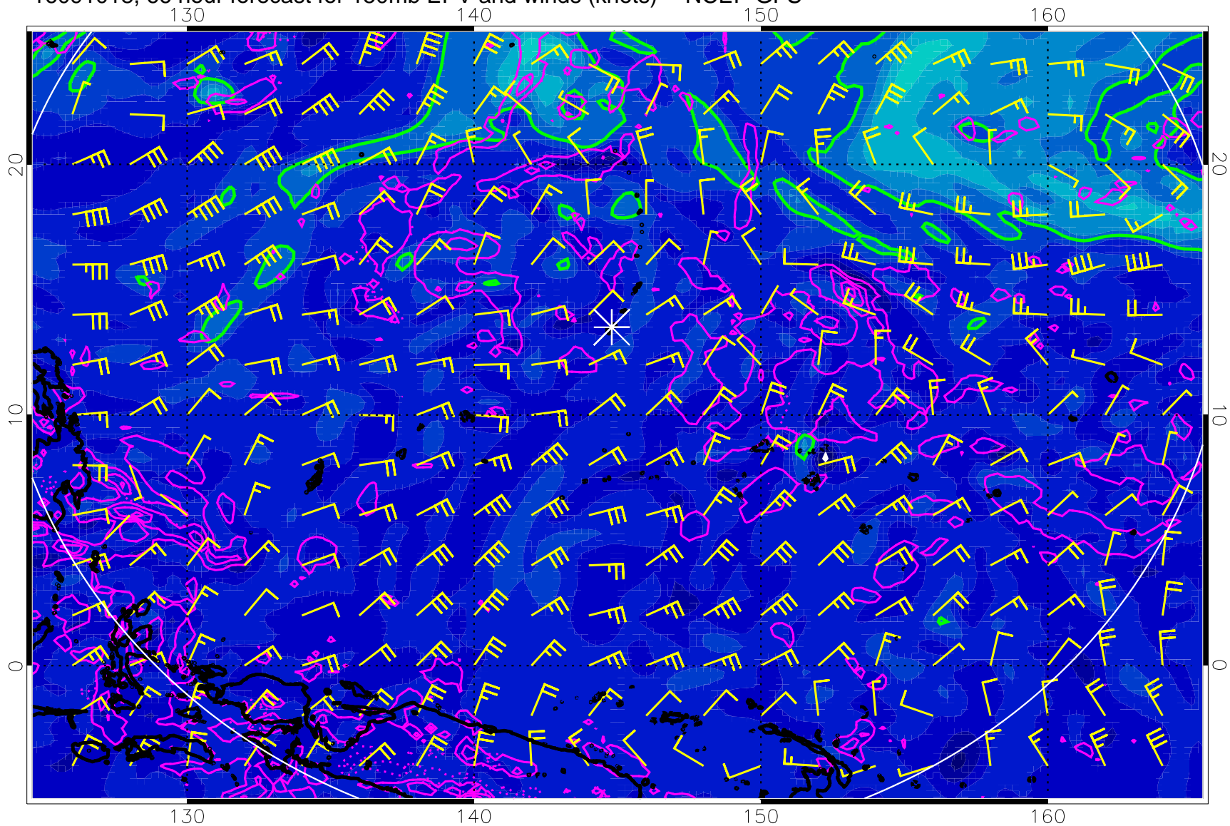
16091018, 66 hour forecast for 150mb EPV and winds (knots) -- NCEP GFS
