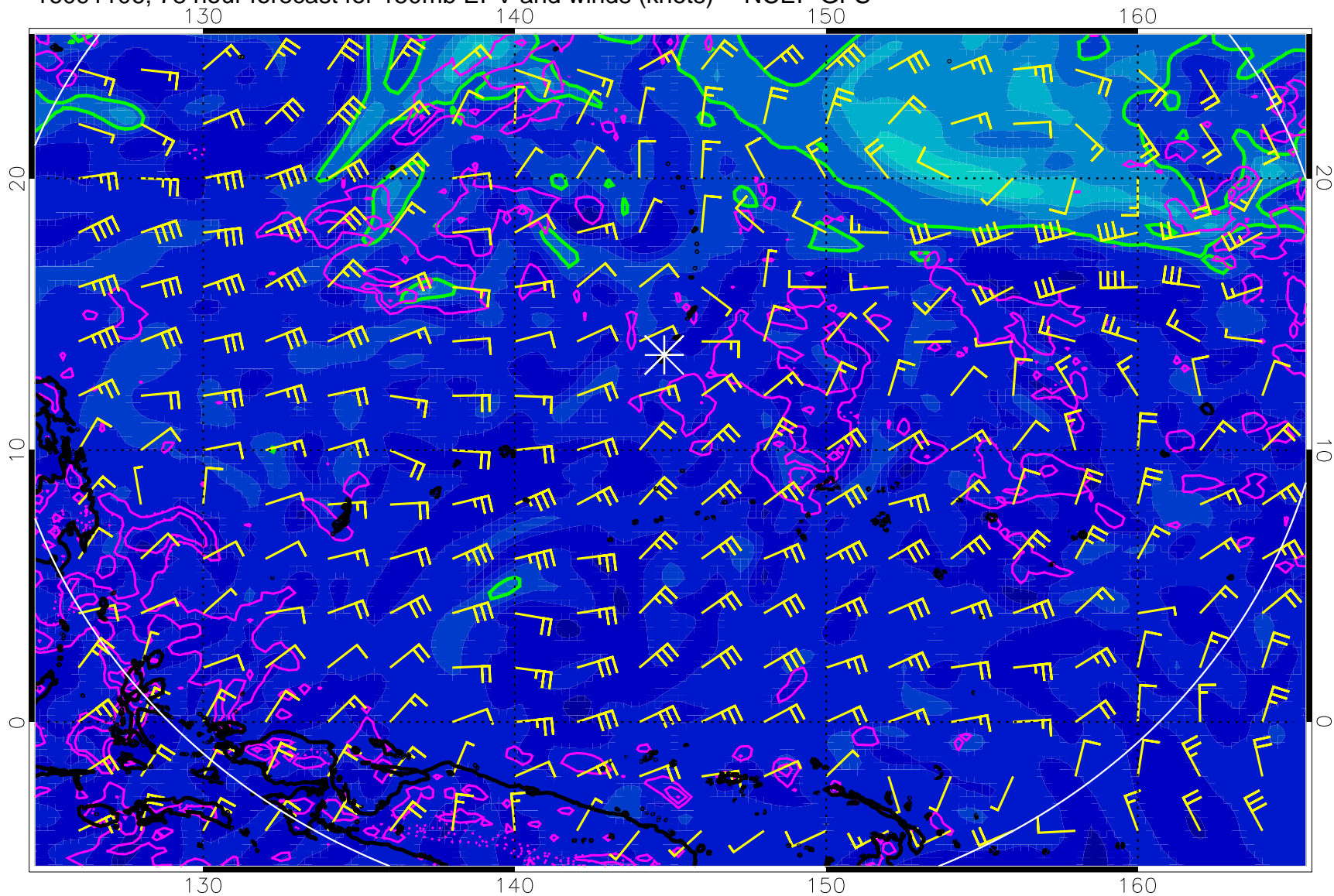
16091106, 78 hour forecast for 150mb EPV and winds (knots) -- NCEP GFS
