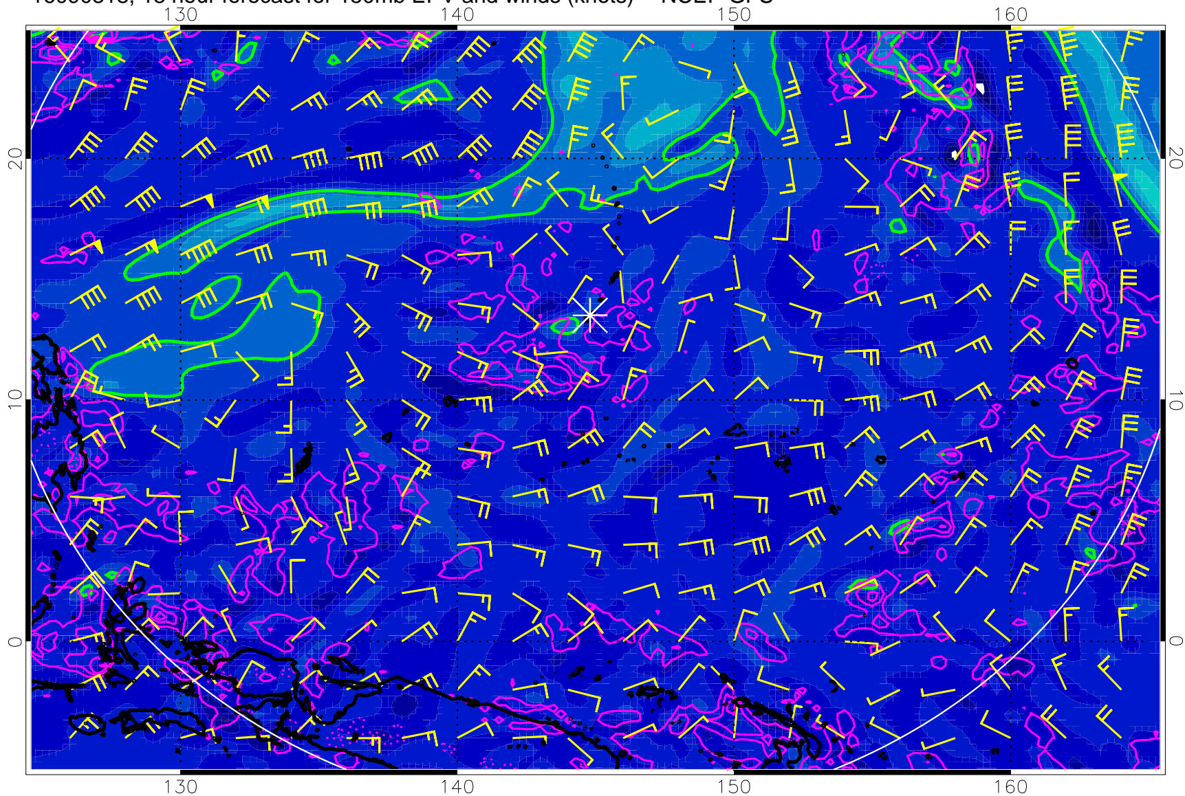
16090818, 18 hour forecast for 150mb EPV and winds (knots) -- NCEP GFS
