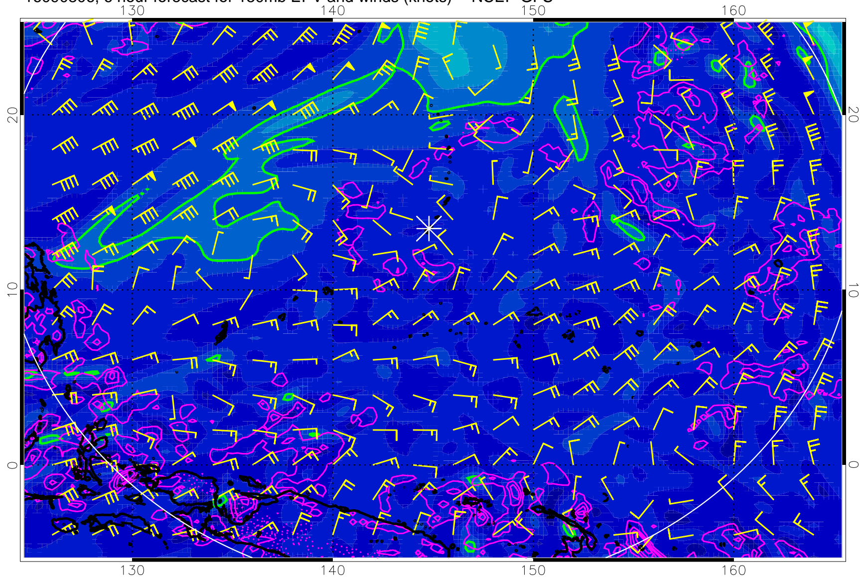
16090806, 6 hour forecast for 150mb EPV and winds (knots) -- NCEP GFS
