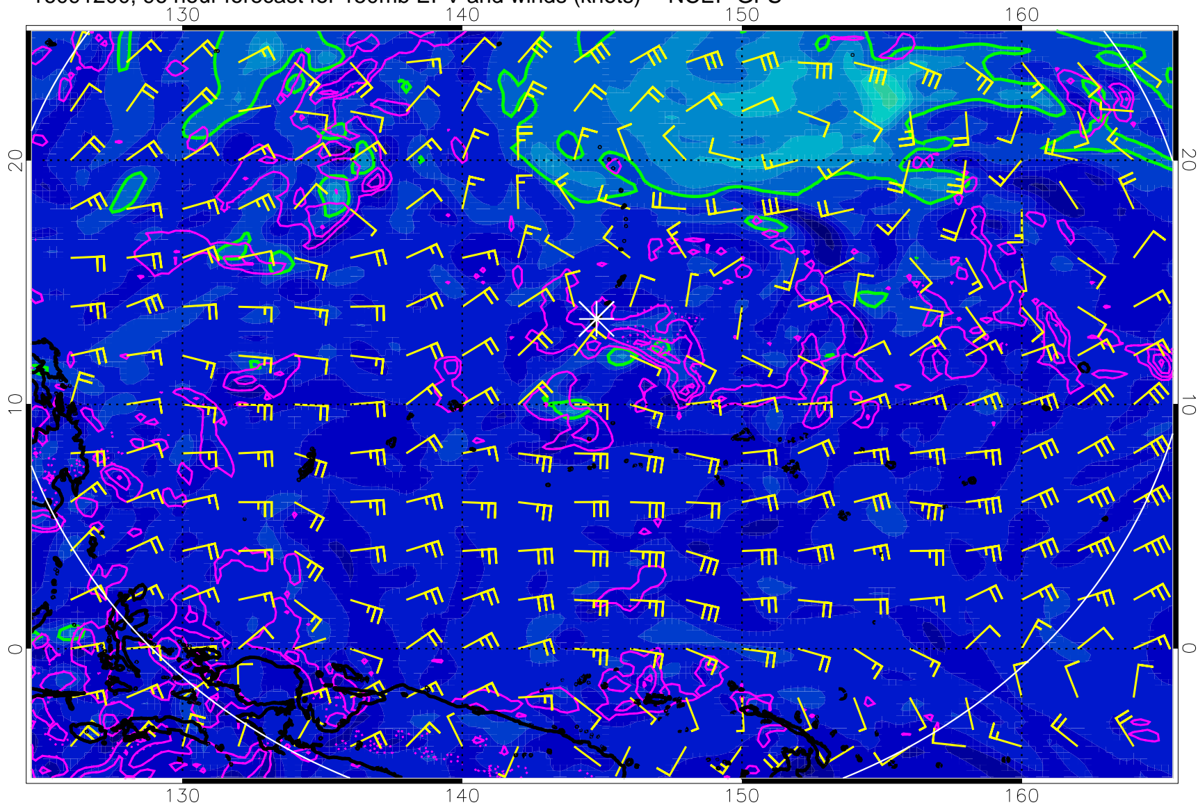
16091200, 96 hour forecast for 150mb EPV and winds (knots) -- NCEP GFS
