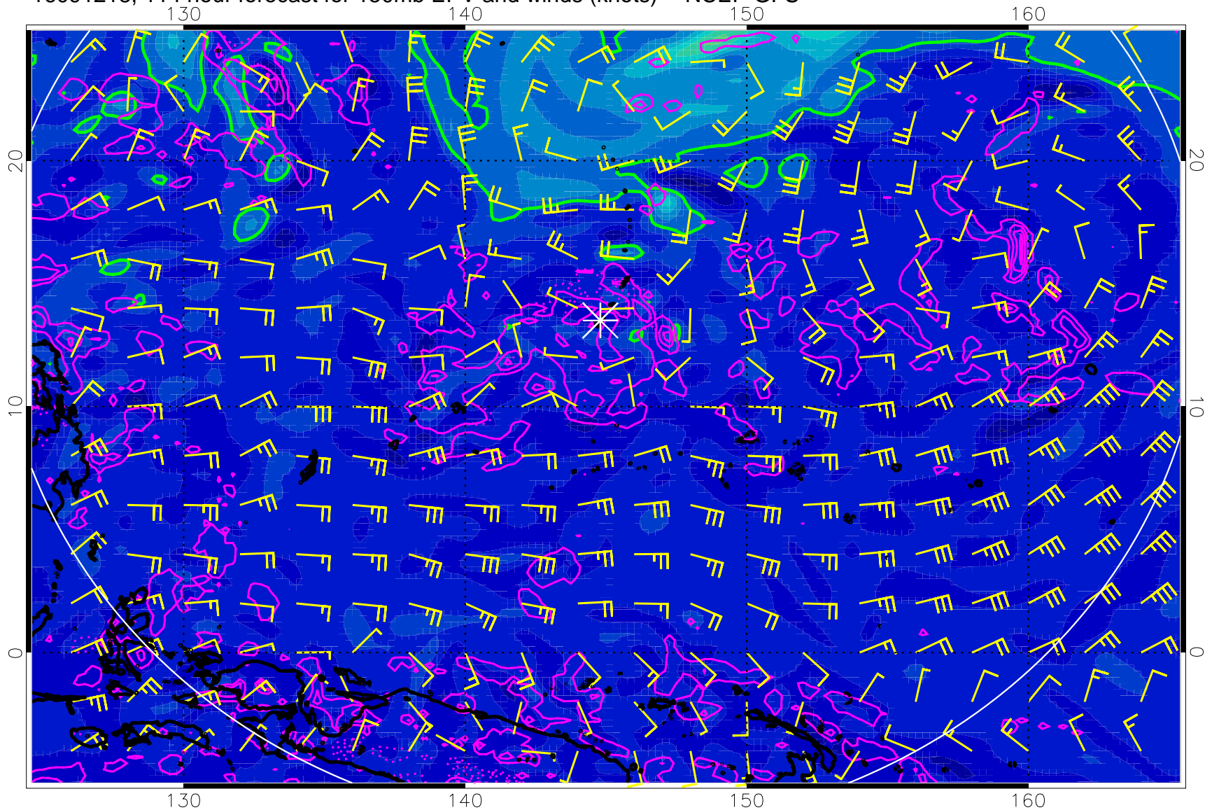
16091218, 114 hour forecast for 150mb EPV and winds (knots) -- NCEP GFS
