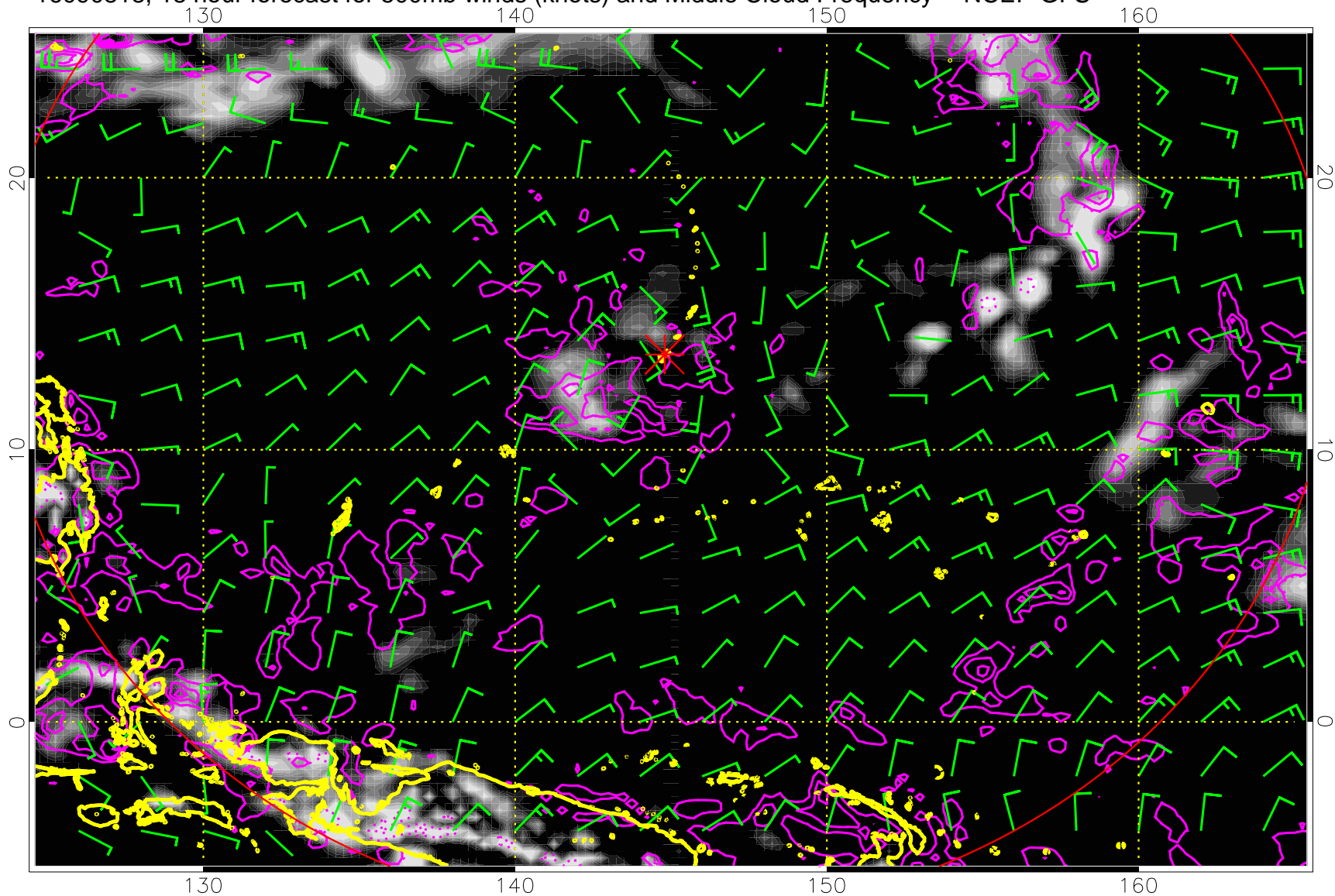
16090818, 18 hour forecast for 500mb winds (knots) and Middle Cloud Frequency -- NCEP GFS
