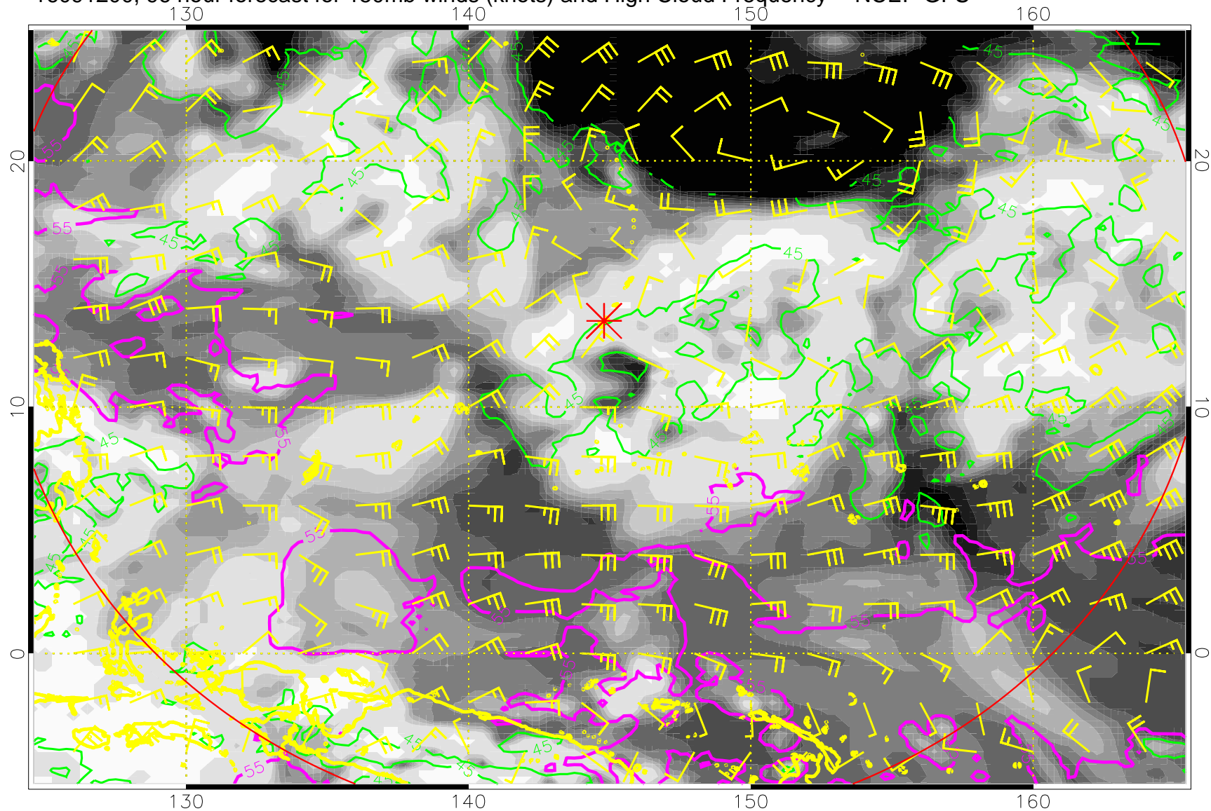
16091200, 96 hour forecast for 150mb winds (knots) and High Cloud Frequency -- NCEP GFS
