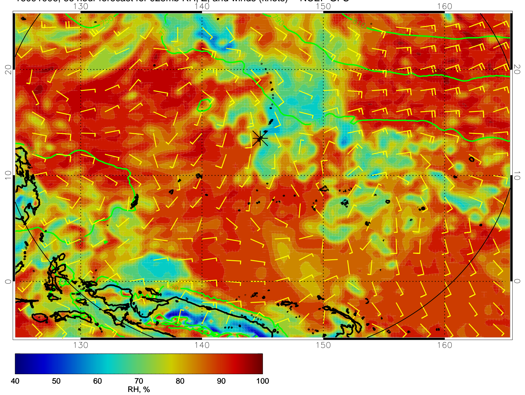
16091006, 66 hour forecast for 925mb RH, Z, and winds (knots) -- NCEP GFS
