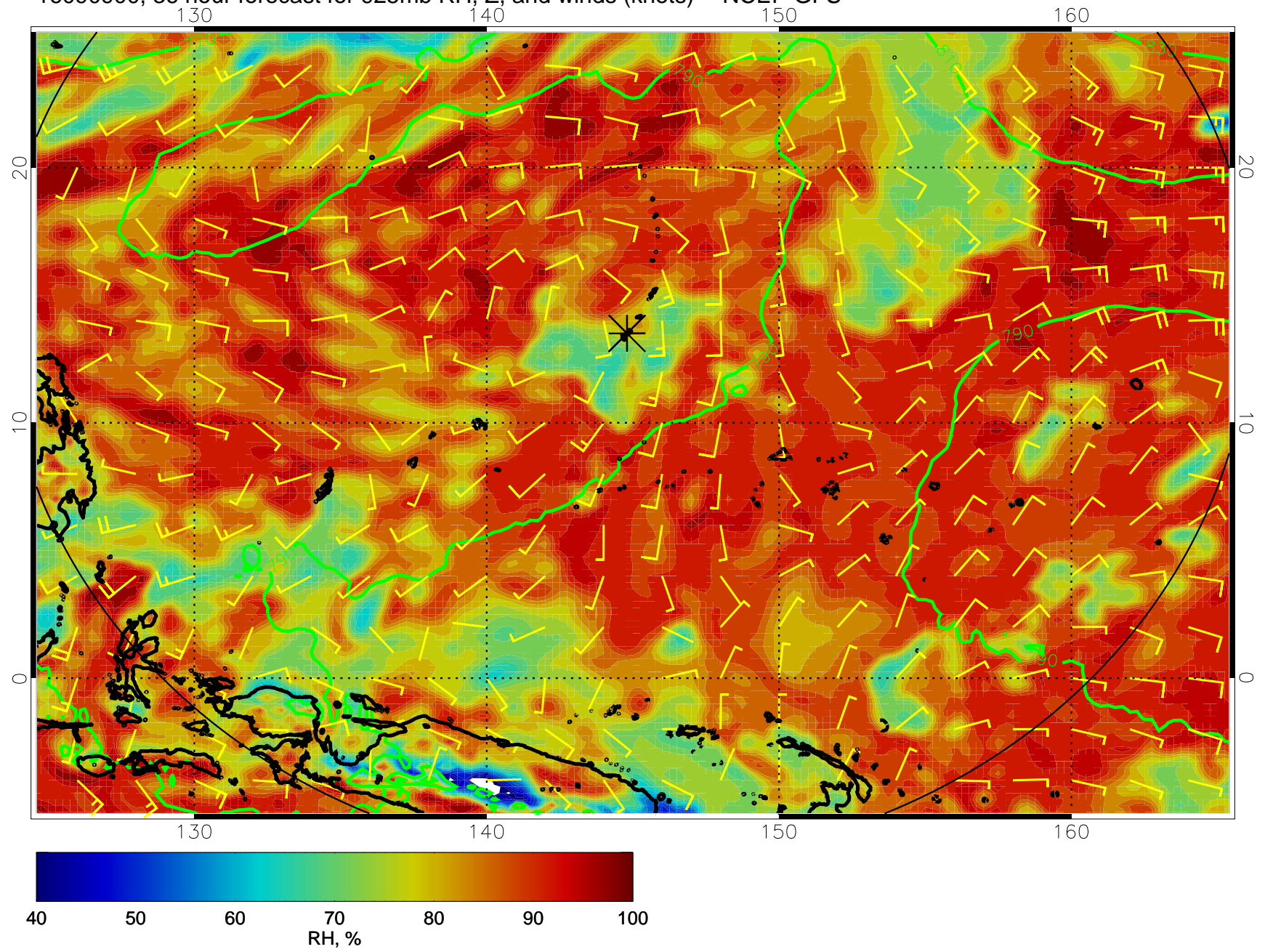
16090900, 36 hour forecast for 925mb RH, Z, and winds (knots) -- NCEP GFS
