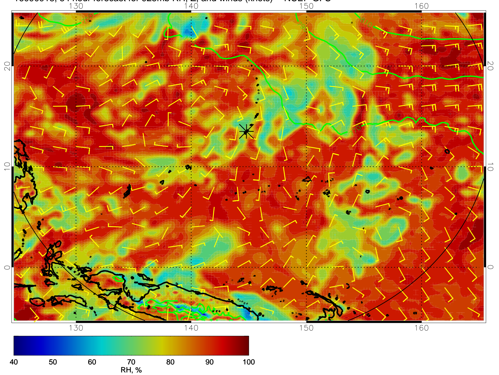
16090918, 54 hour forecast for 925mb RH, Z, and winds (knots) -- NCEP GFS
