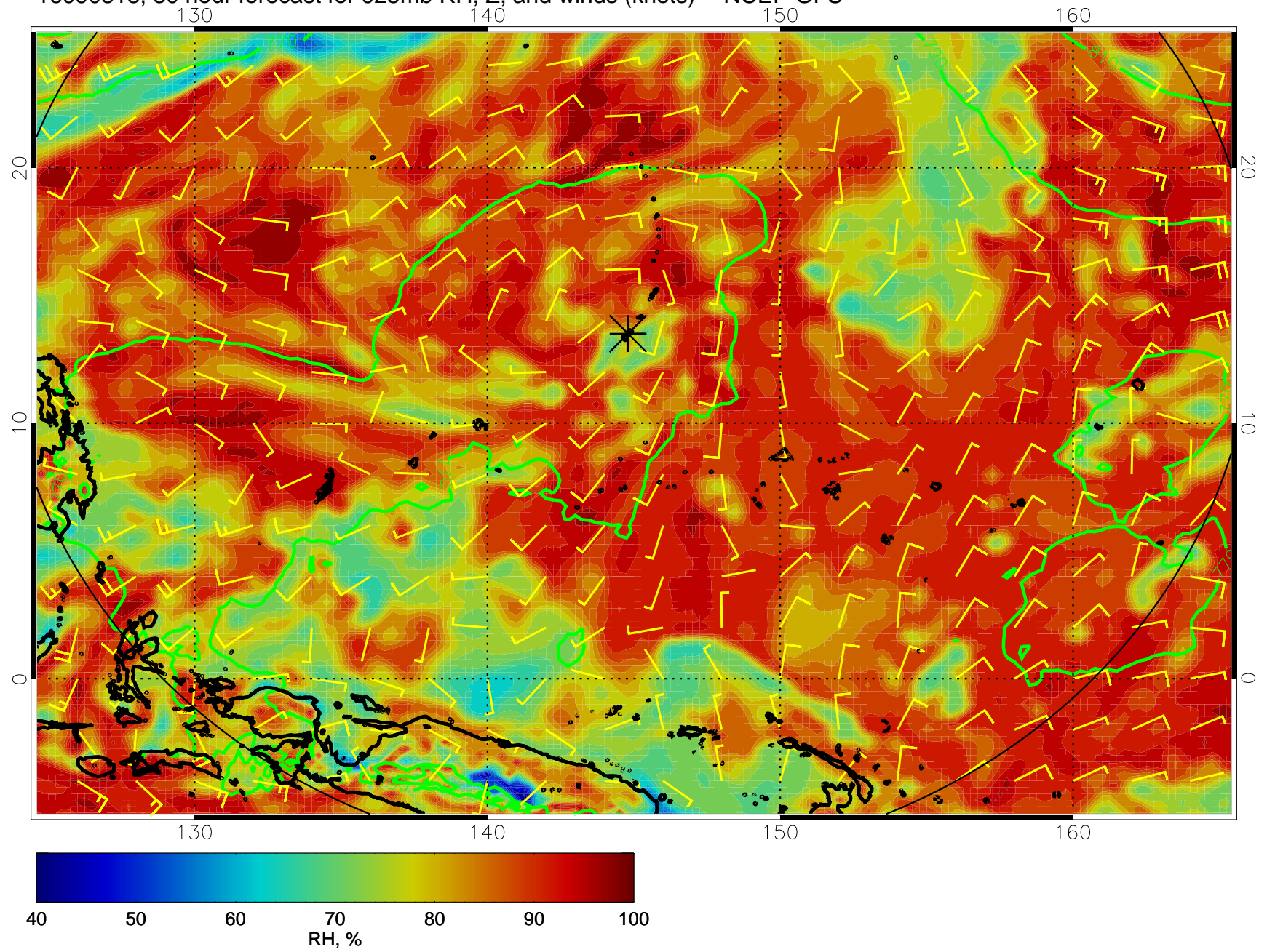
16090818, 30 hour forecast for 925mb RH, Z, and winds (knots) -- NCEP GFS
