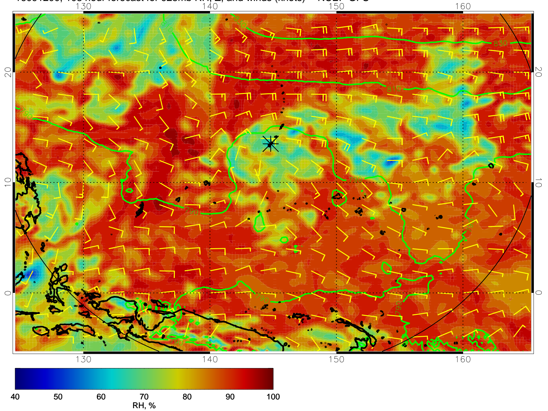
16091200, 108 hour forecast for 925mb RH, Z, and winds (knots) -- NCEP GFS
