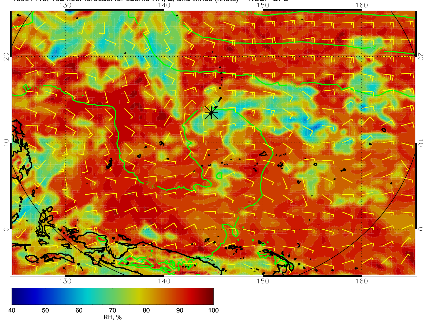
16091118, 102 hour forecast for 925mb RH, Z, and winds (knots) -- NCEP GFS
