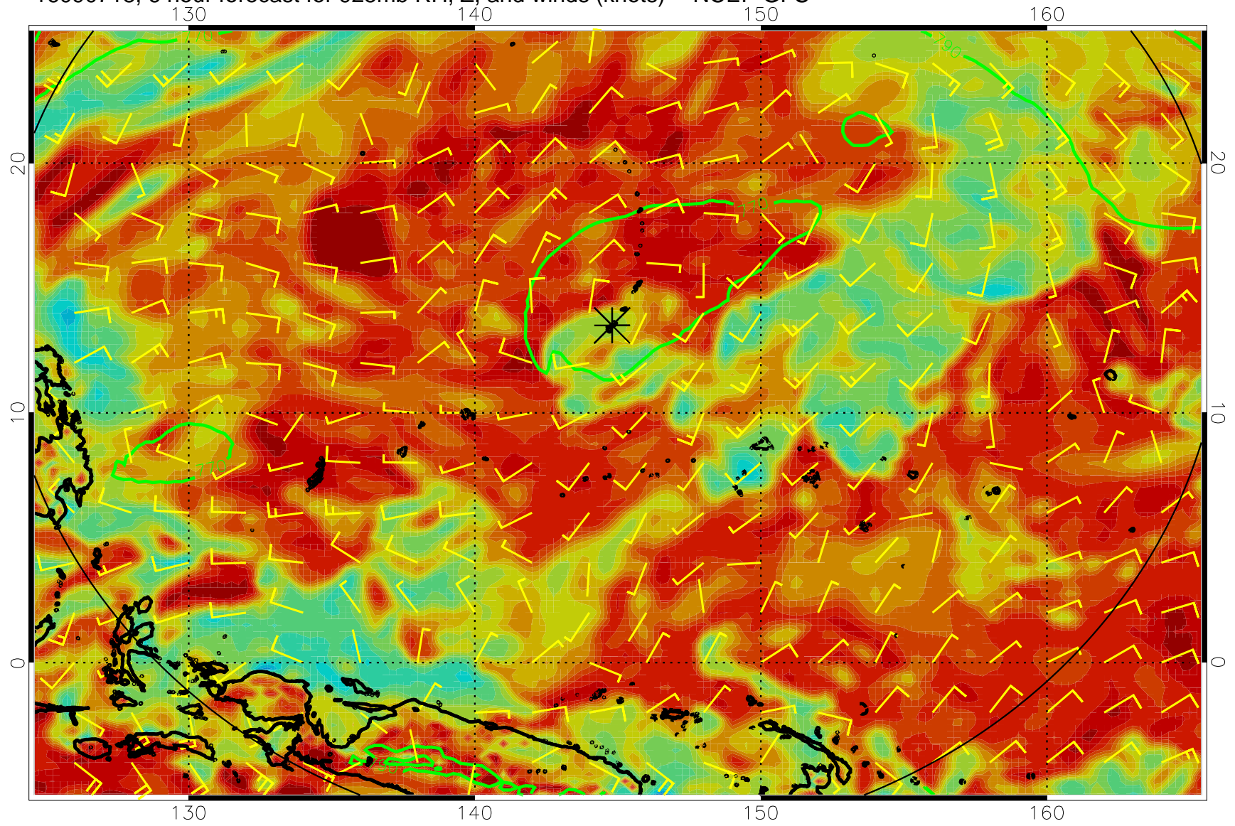
16090718, 6 hour forecast for 925mb RH, Z, and winds (knots) -- NCEP GFS
