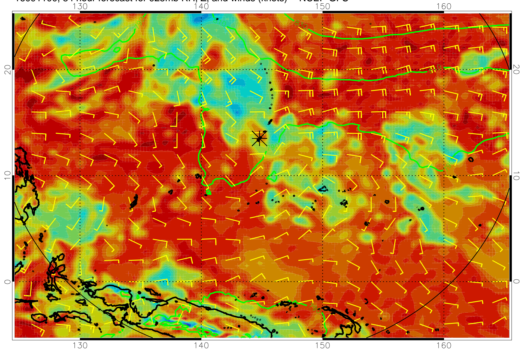
16091100, 84 hour forecast for 925mb RH, Z, and winds (knots) -- NCEP GFS
