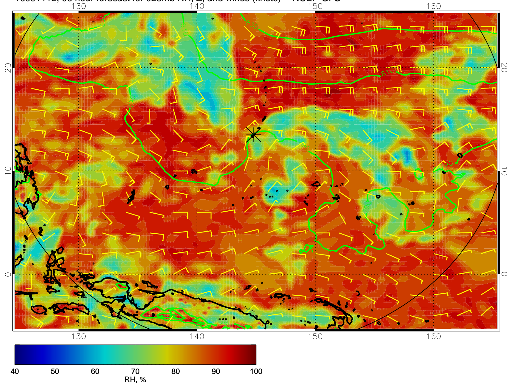
16091112, 96 hour forecast for 925mb RH, Z, and winds (knots) -- NCEP GFS
