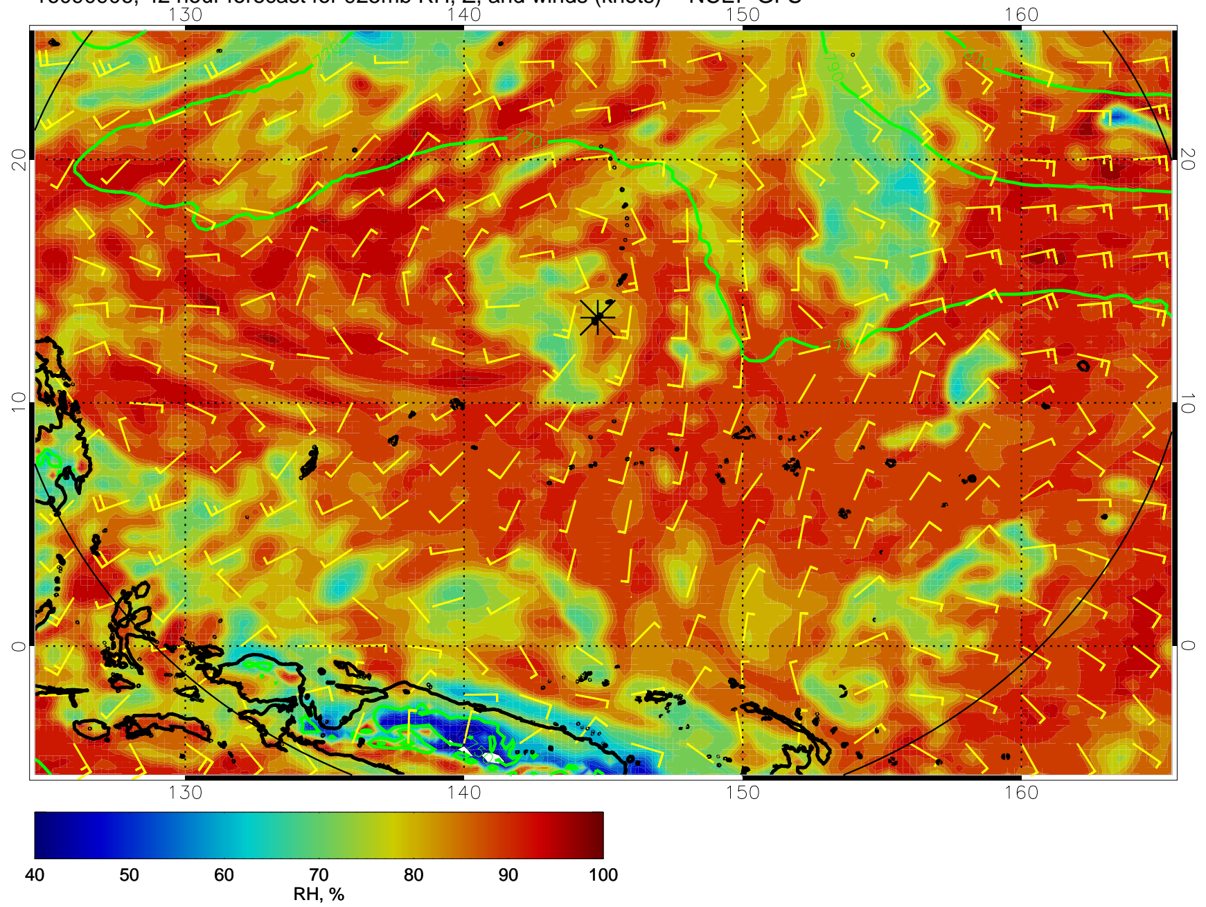
16090906, 42 hour forecast for 925mb RH, Z, and winds (knots) -- NCEP GFS
