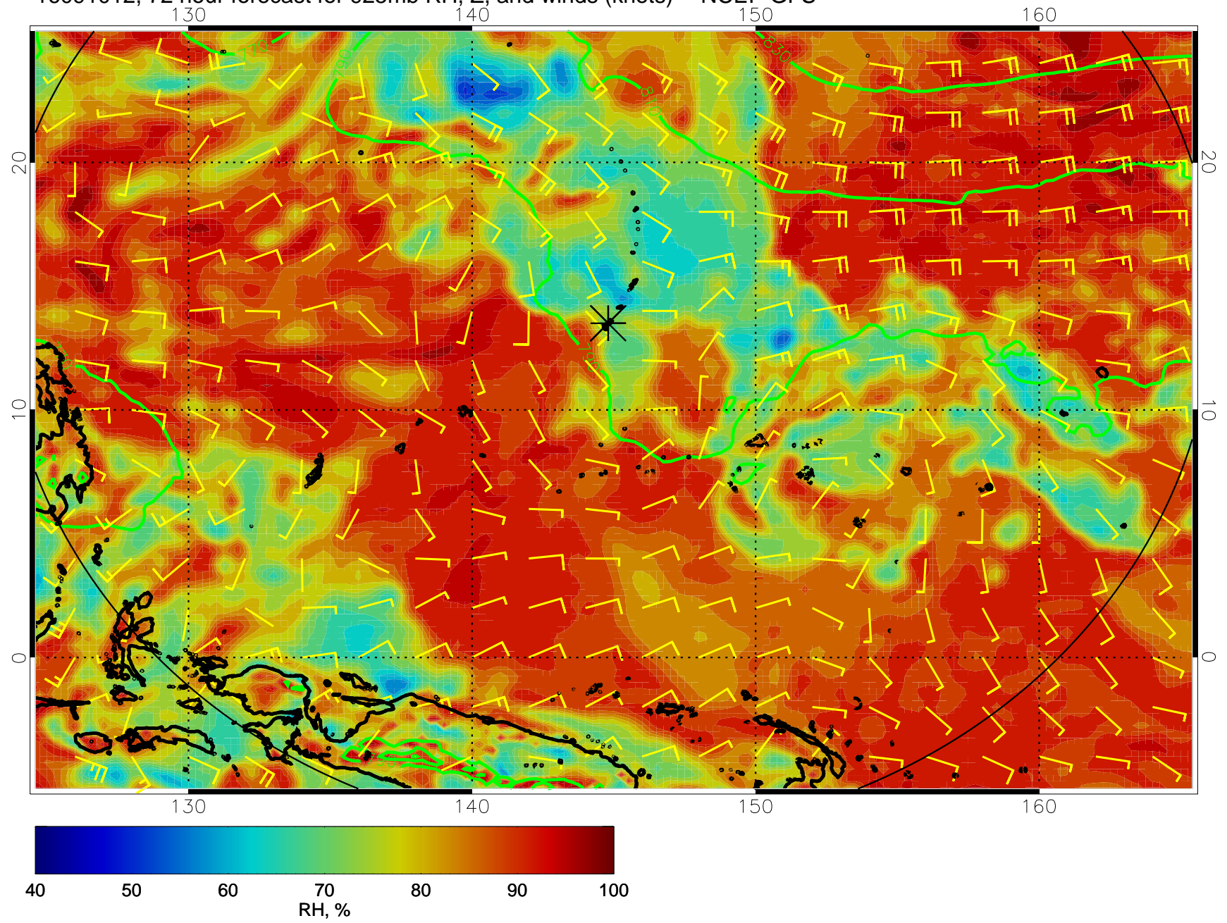
16091012, 72 hour forecast for 925mb RH, Z, and winds (knots) -- NCEP GFS
