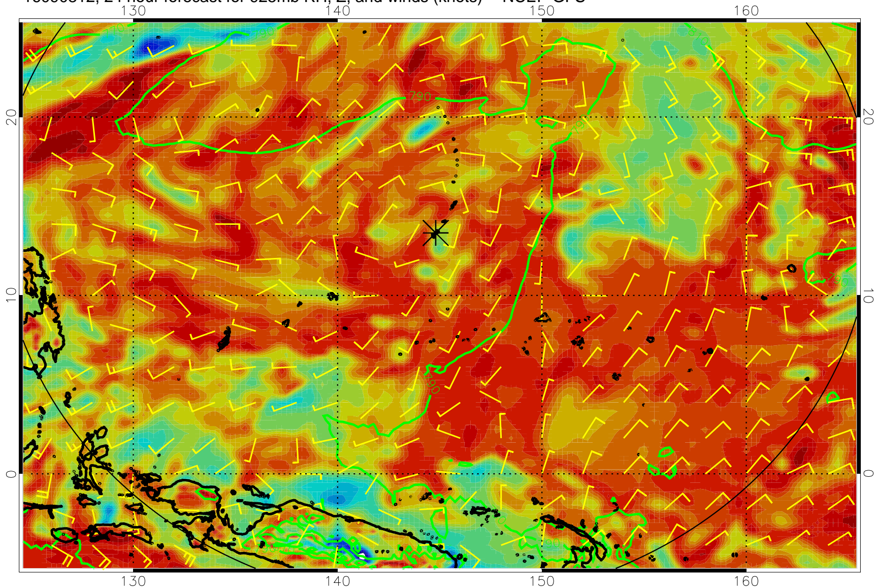
16090812, 24 hour forecast for 925mb RH, Z, and winds (knots) -- NCEP GFS
