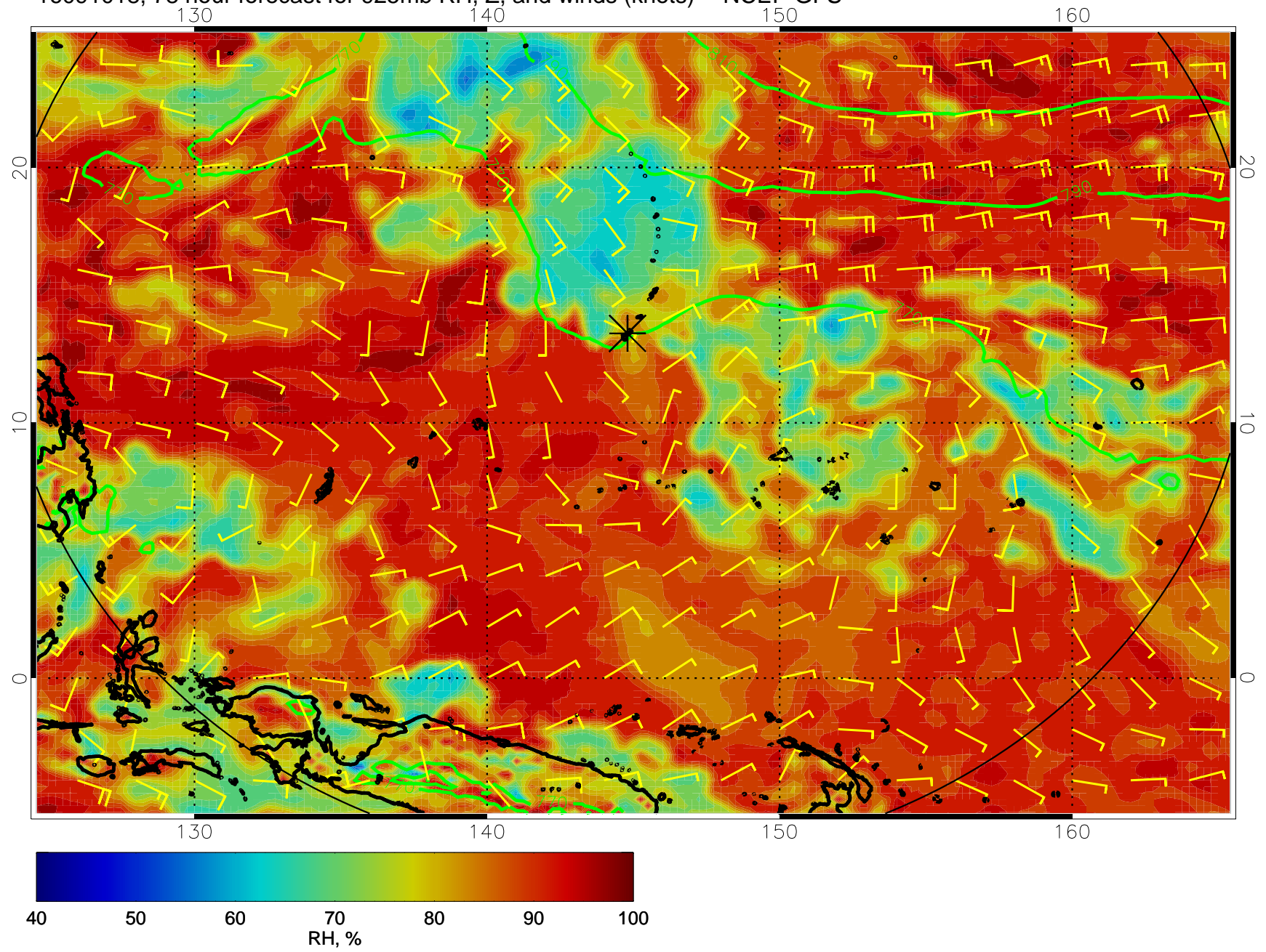
16091018, 78 hour forecast for 925mb RH, Z, and winds (knots) -- NCEP GFS
