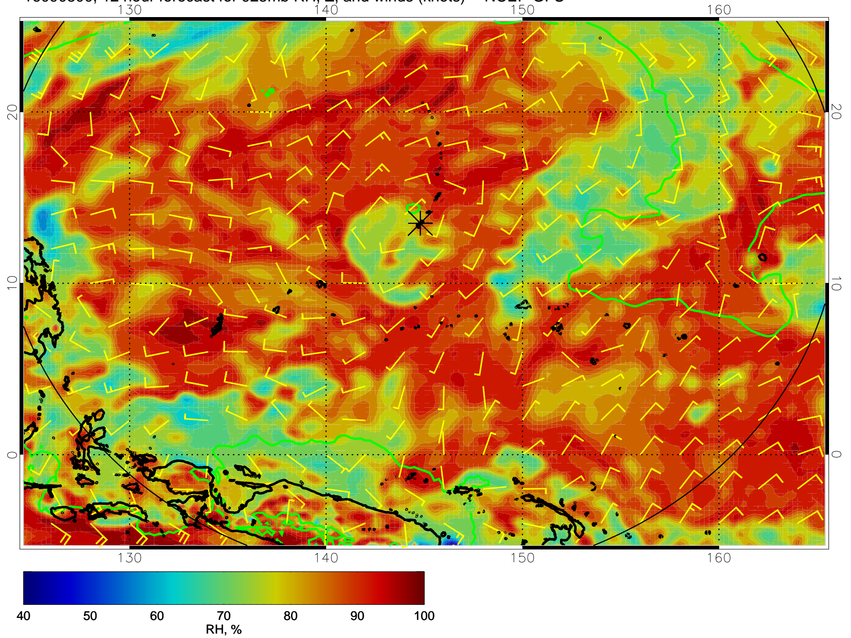
16090800, 12 hour forecast for 925mb RH, Z, and winds (knots) -- NCEP GFS
