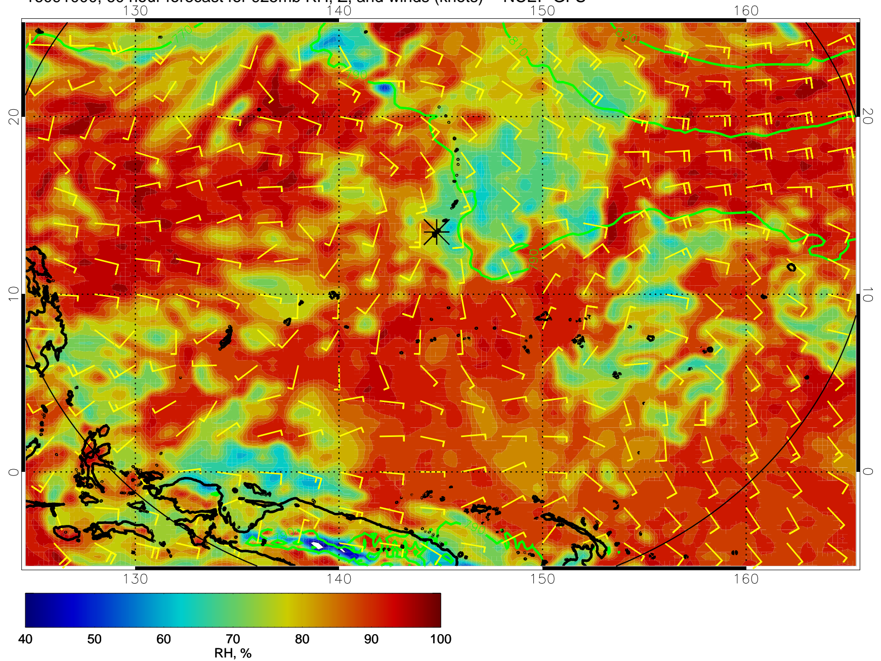
16091000, 60 hour forecast for 925mb RH, Z, and winds (knots) -- NCEP GFS
