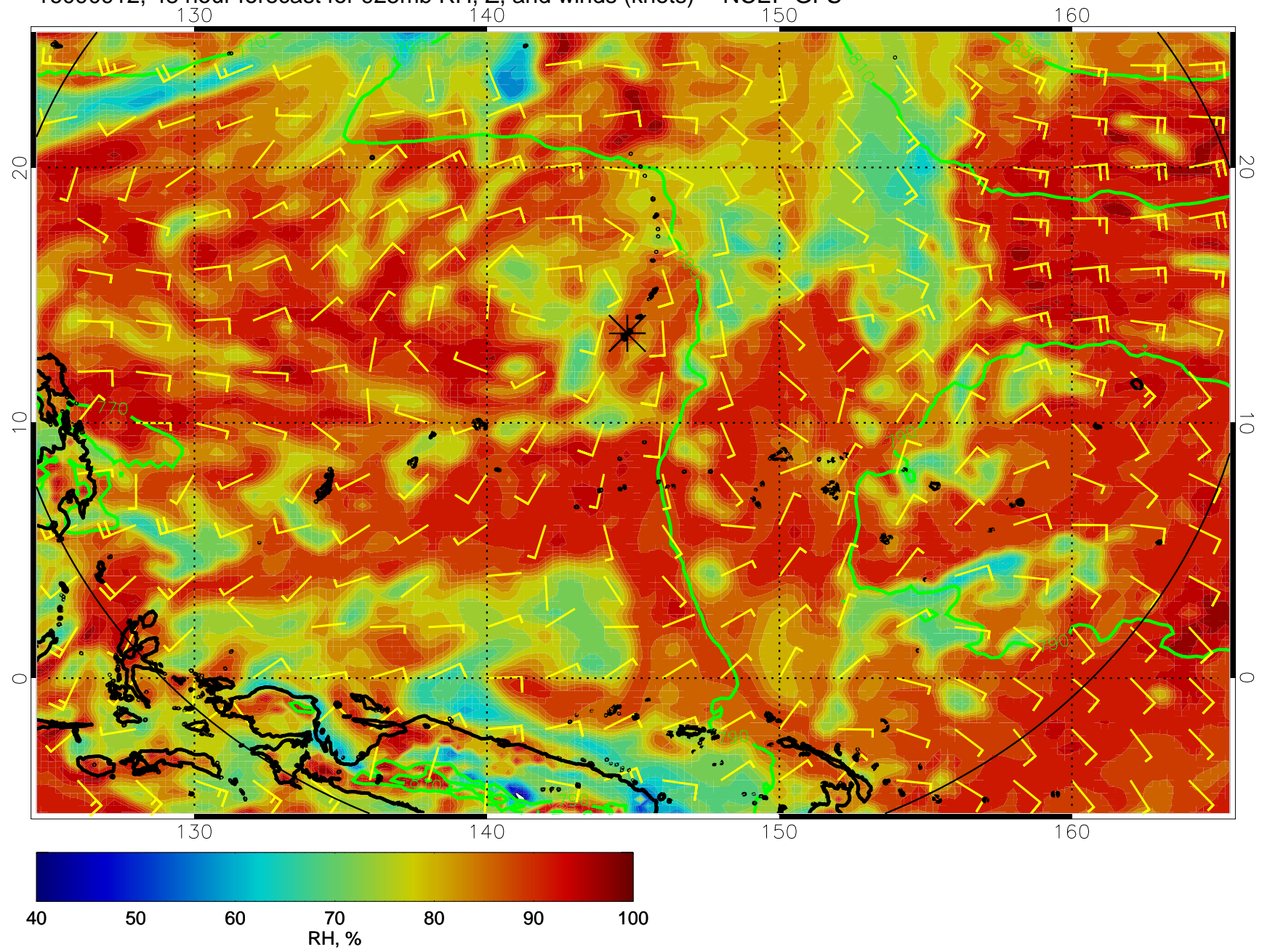
16090912, 48 hour forecast for 925mb RH, Z, and winds (knots) -- NCEP GFS
