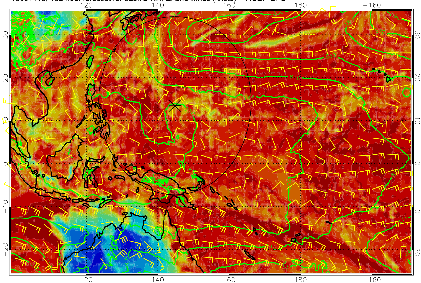
16091118, 102 hour forecast for 925mb RH, Z, and winds (knots) -- NCEP GFS
