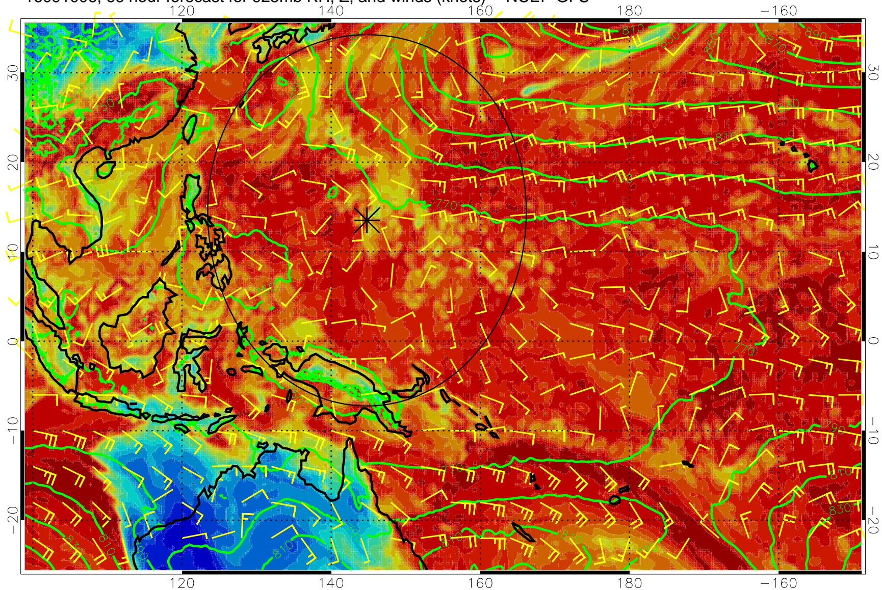
16091006, 66 hour forecast for 925mb RH, Z, and winds (knots) -- NCEP GFS
