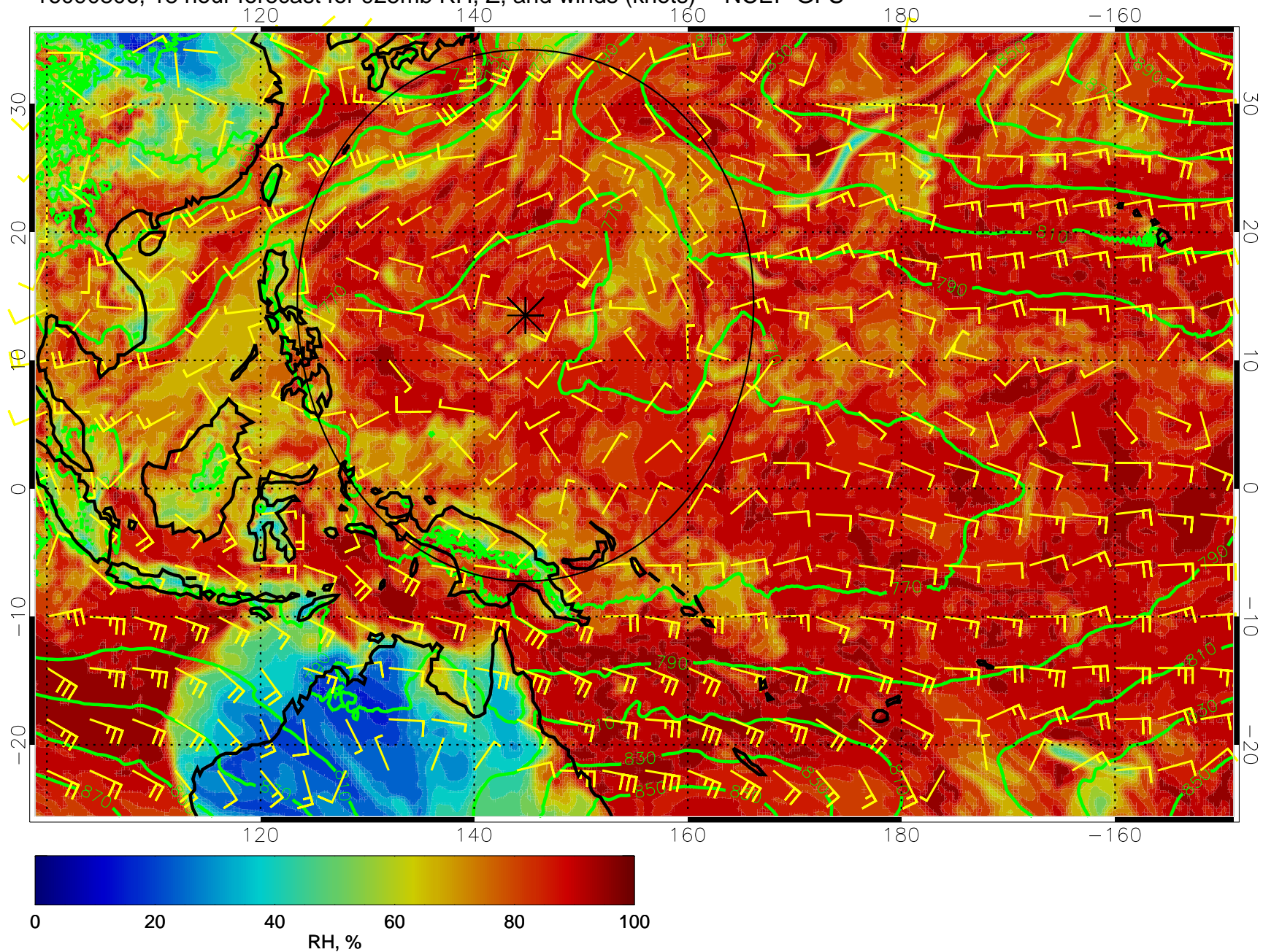
16090806, 18 hour forecast for 925mb RH, Z, and winds (knots) -- NCEP GFS
