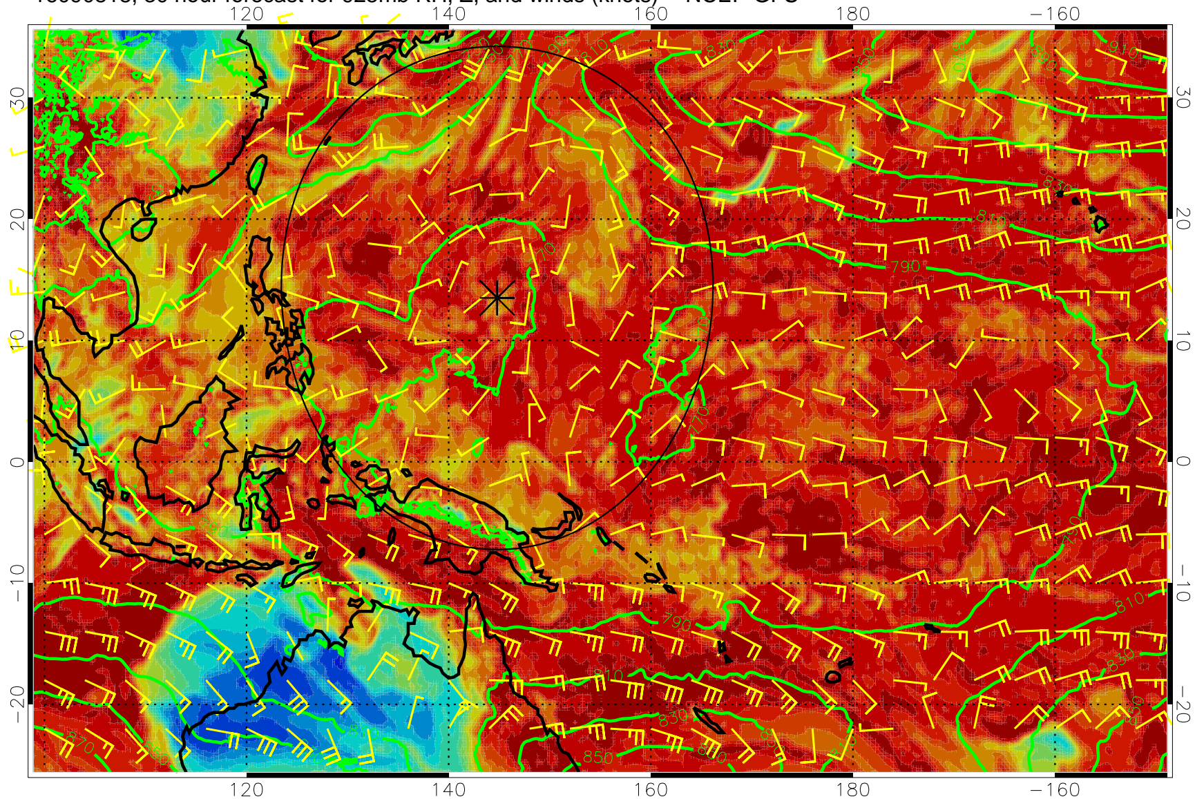
16090818, 30 hour forecast for 925mb RH, Z, and winds (knots) -- NCEP GFS
