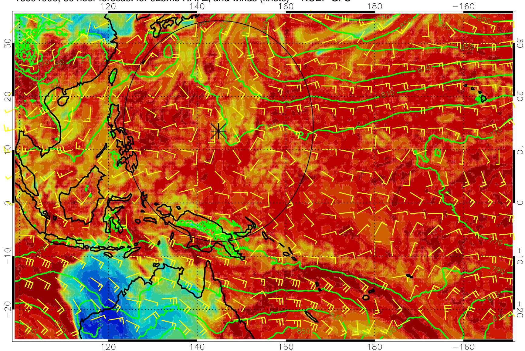
16091000, 60 hour forecast for 925mb RH, Z, and winds (knots) -- NCEP GFS
