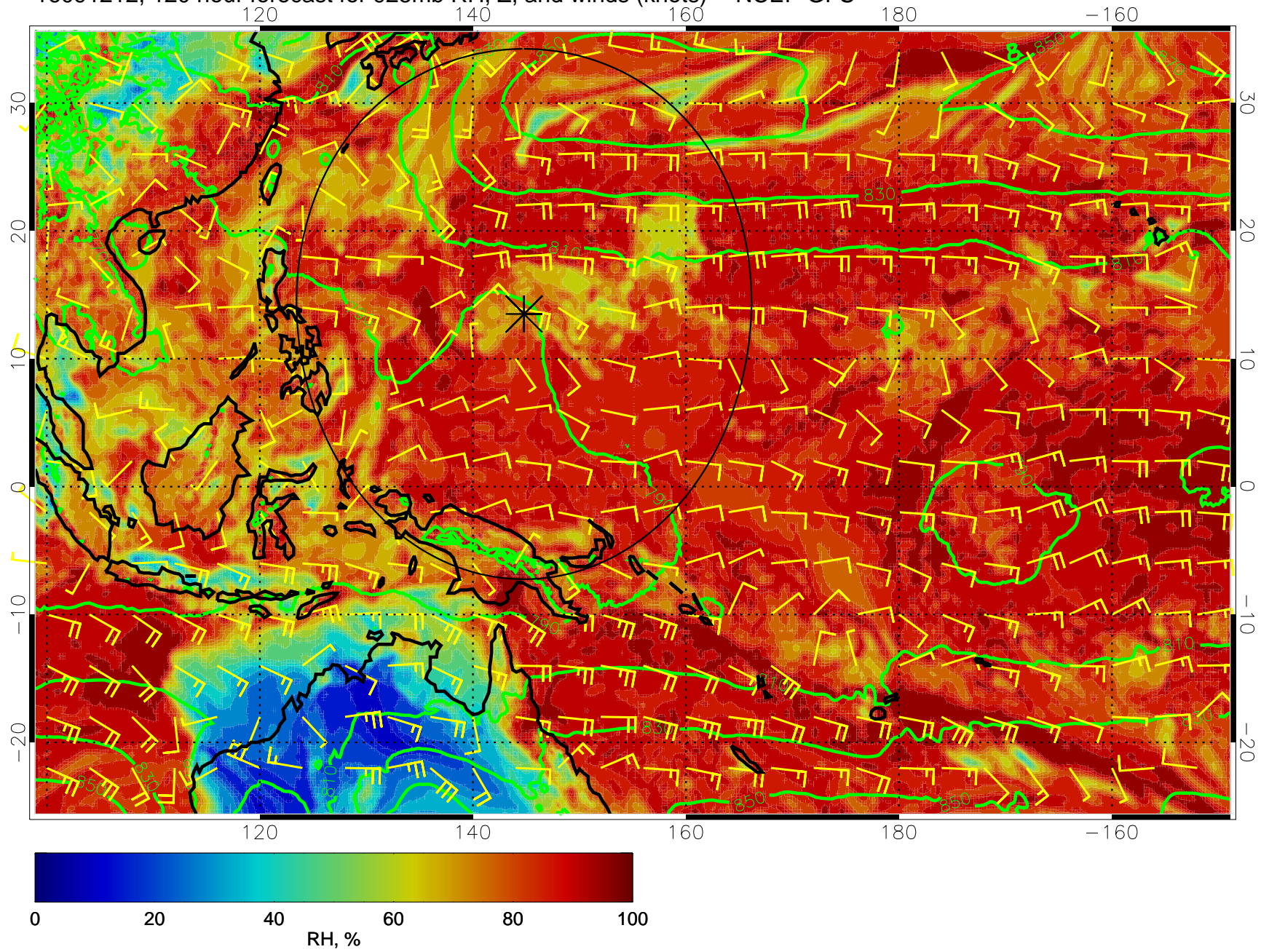
16091212, 120 hour forecast for 925mb RH, Z, and winds (knots) -- NCEP GFS
