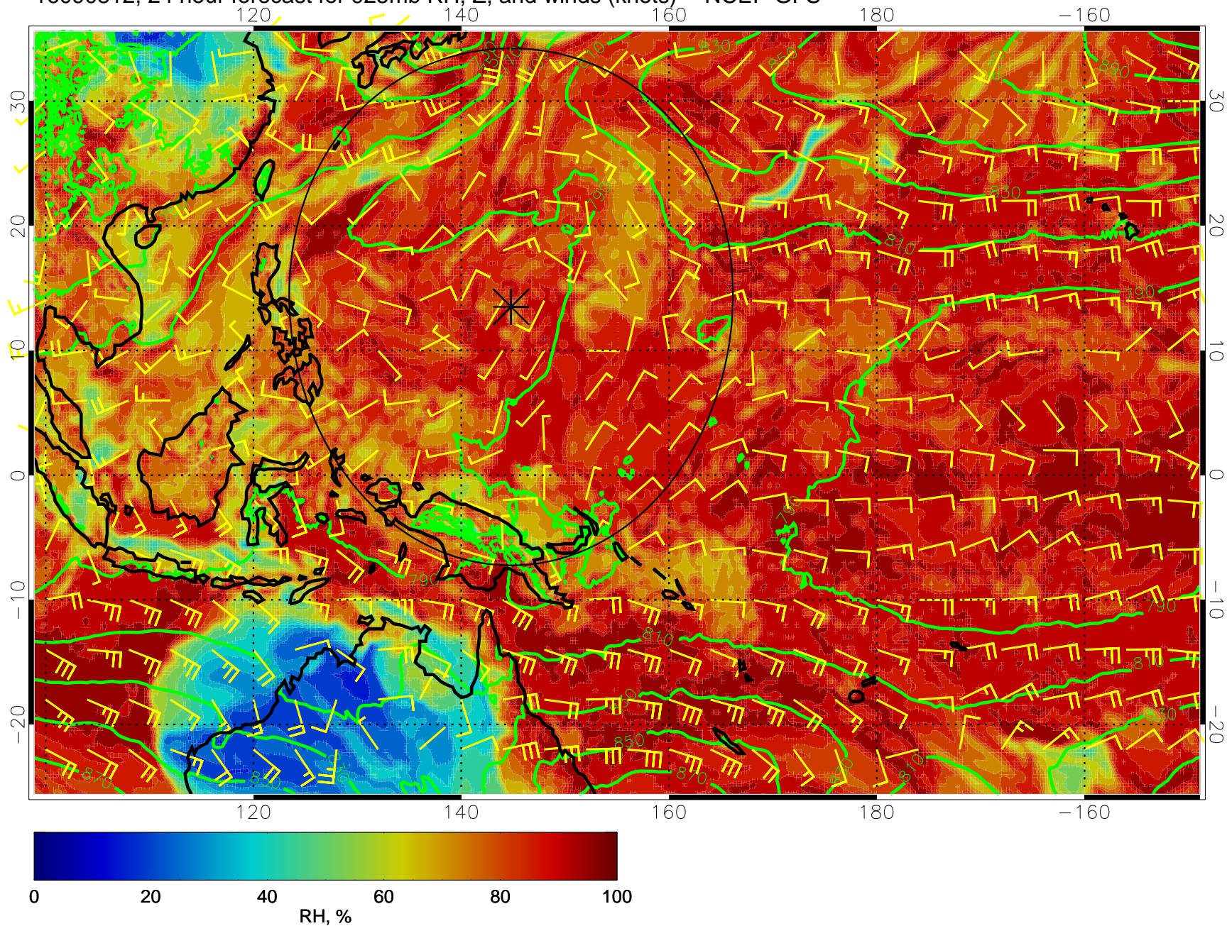
16090812, 24 hour forecast for 925mb RH, Z, and winds (knots) -- NCEP GFS
