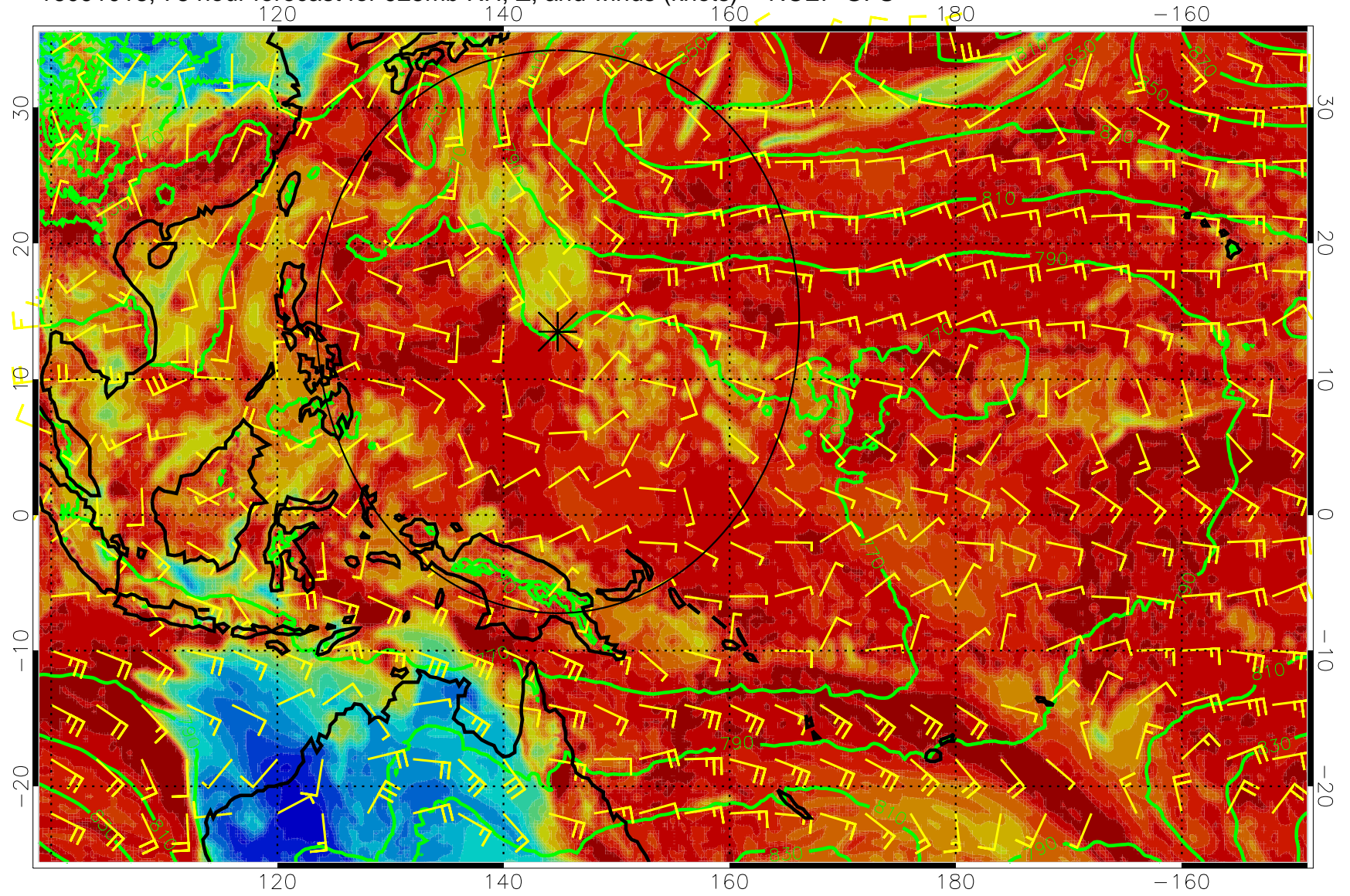
16091018, 78 hour forecast for 925mb RH, Z, and winds (knots) -- NCEP GFS
