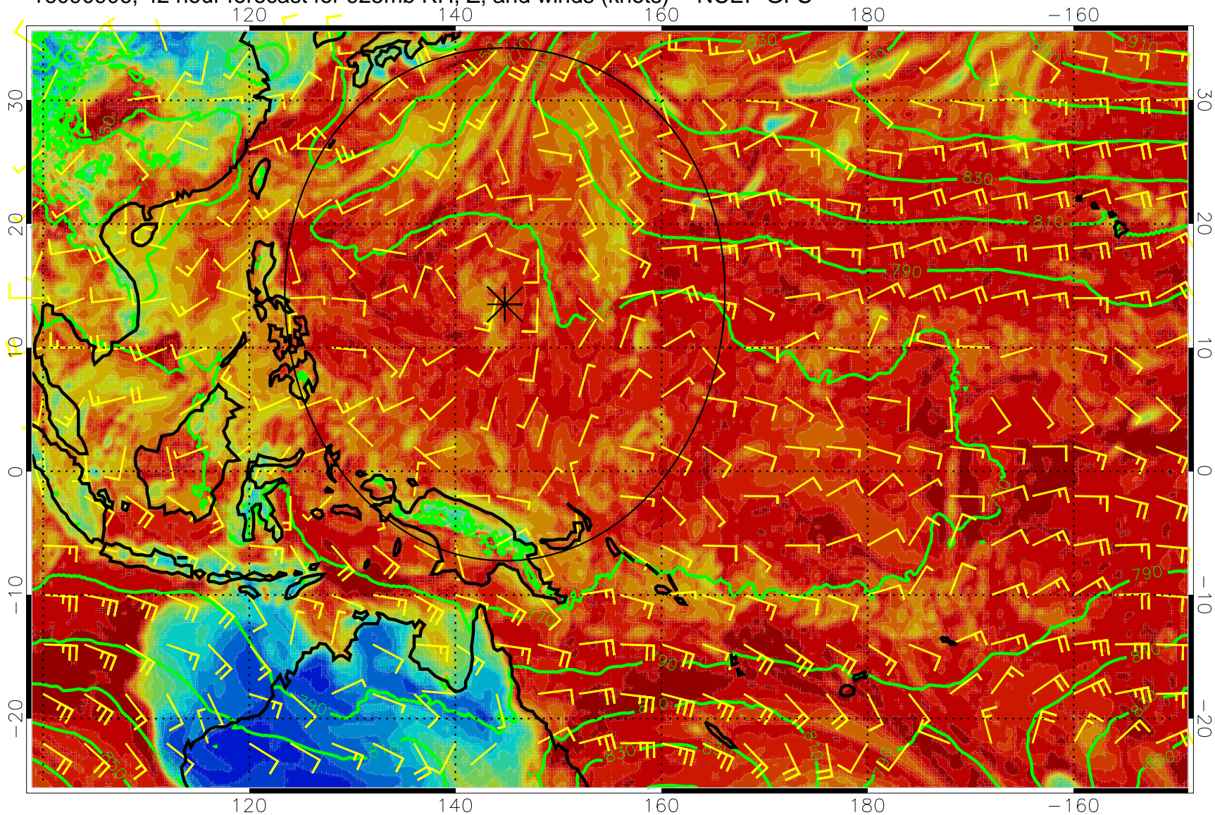
16090906, 42 hour forecast for 925mb RH, Z, and winds (knots) -- NCEP GFS
