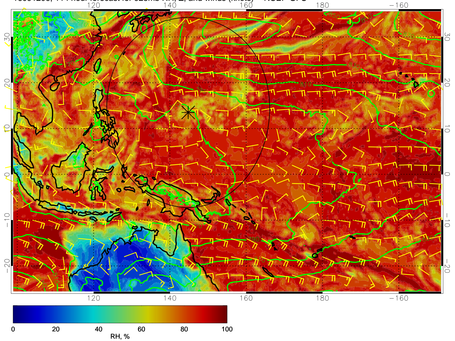
16091206, 114 hour forecast for 925mb RH, Z, and winds (knots) -- NCEP GFS
