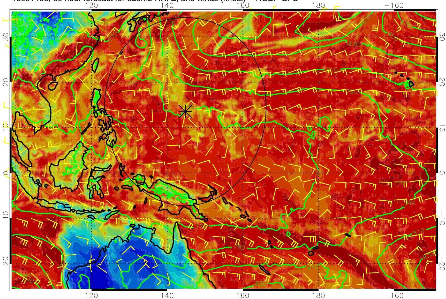
16091106, 90 hour forecast for 925mb RH, Z, and winds (knots) -- NCEP GFS
