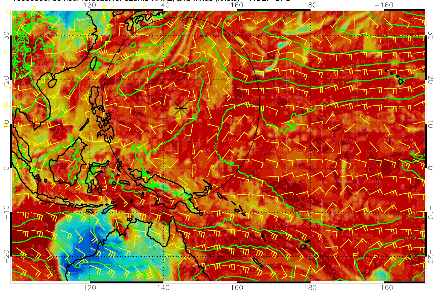
16090900, 36 hour forecast for 925mb RH, Z, and winds (knots) -- NCEP GFS
