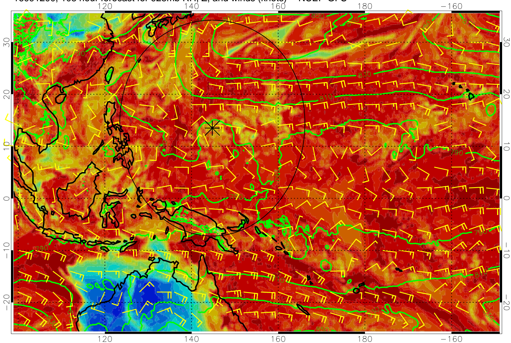
16091200, 108 hour forecast for 925mb RH, Z, and winds (knots) -- NCEP GFS
