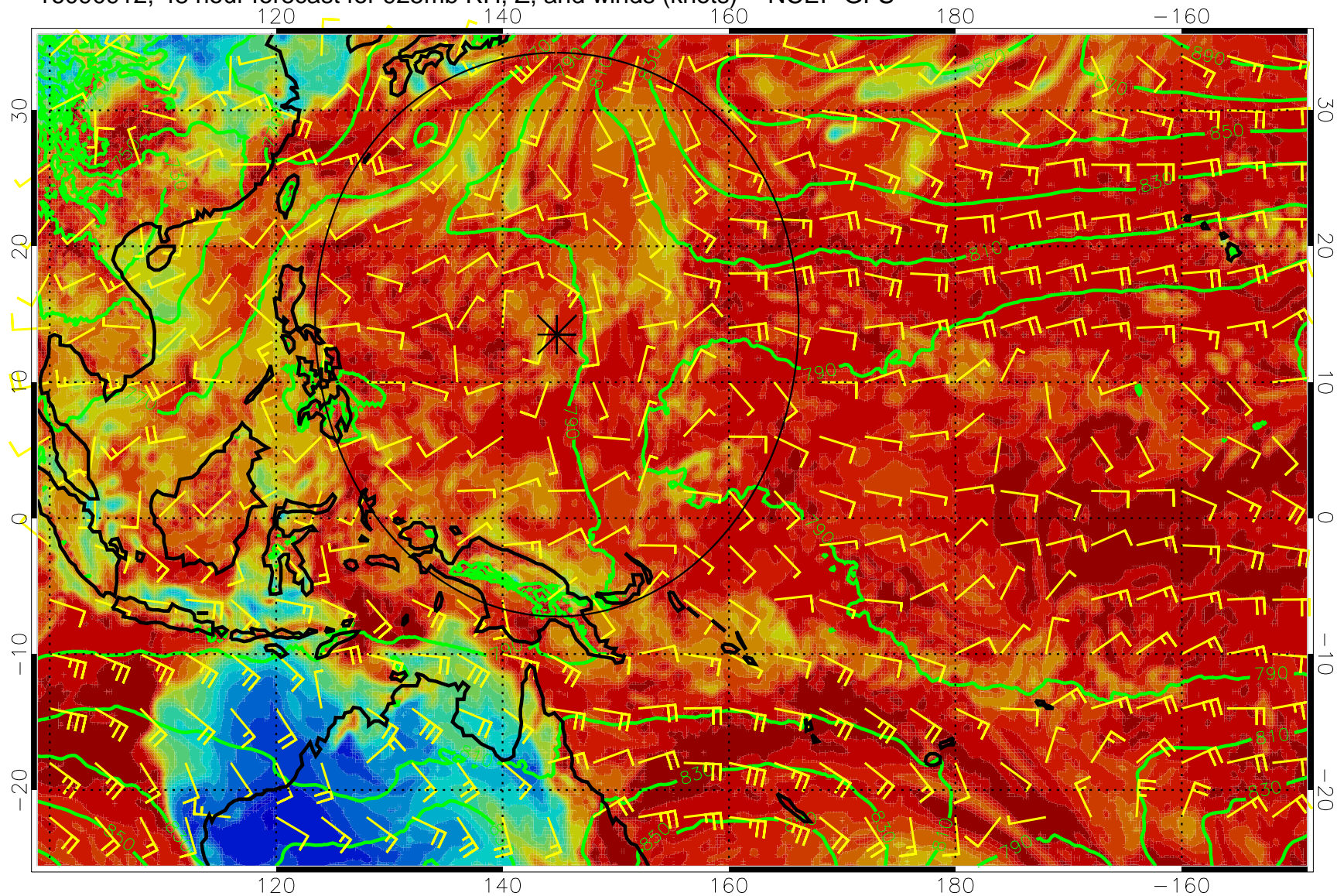
16090912, 48 hour forecast for 925mb RH, Z, and winds (knots) -- NCEP GFS
