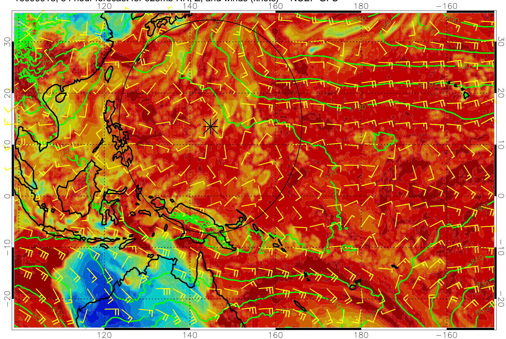
16090918, 54 hour forecast for 925mb RH, Z, and winds (knots) -- NCEP GFS
