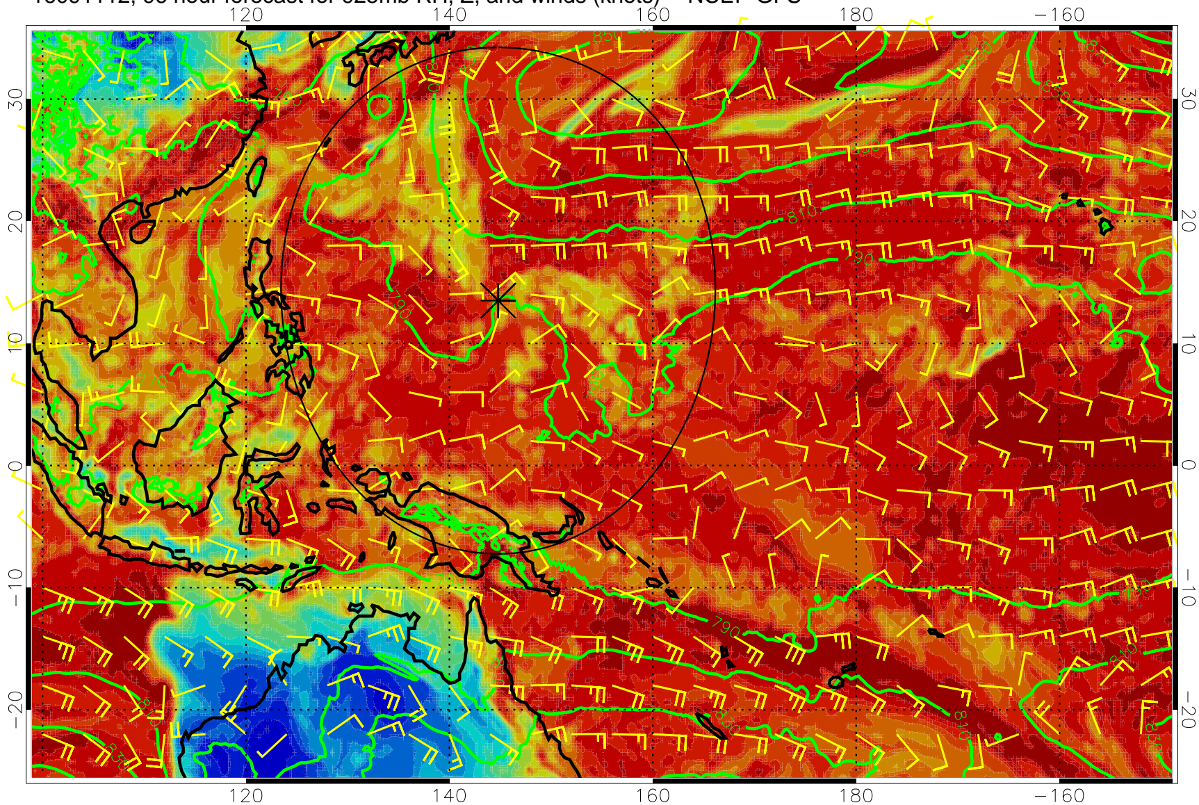
16091112, 96 hour forecast for 925mb RH, Z, and winds (knots) -- NCEP GFS
