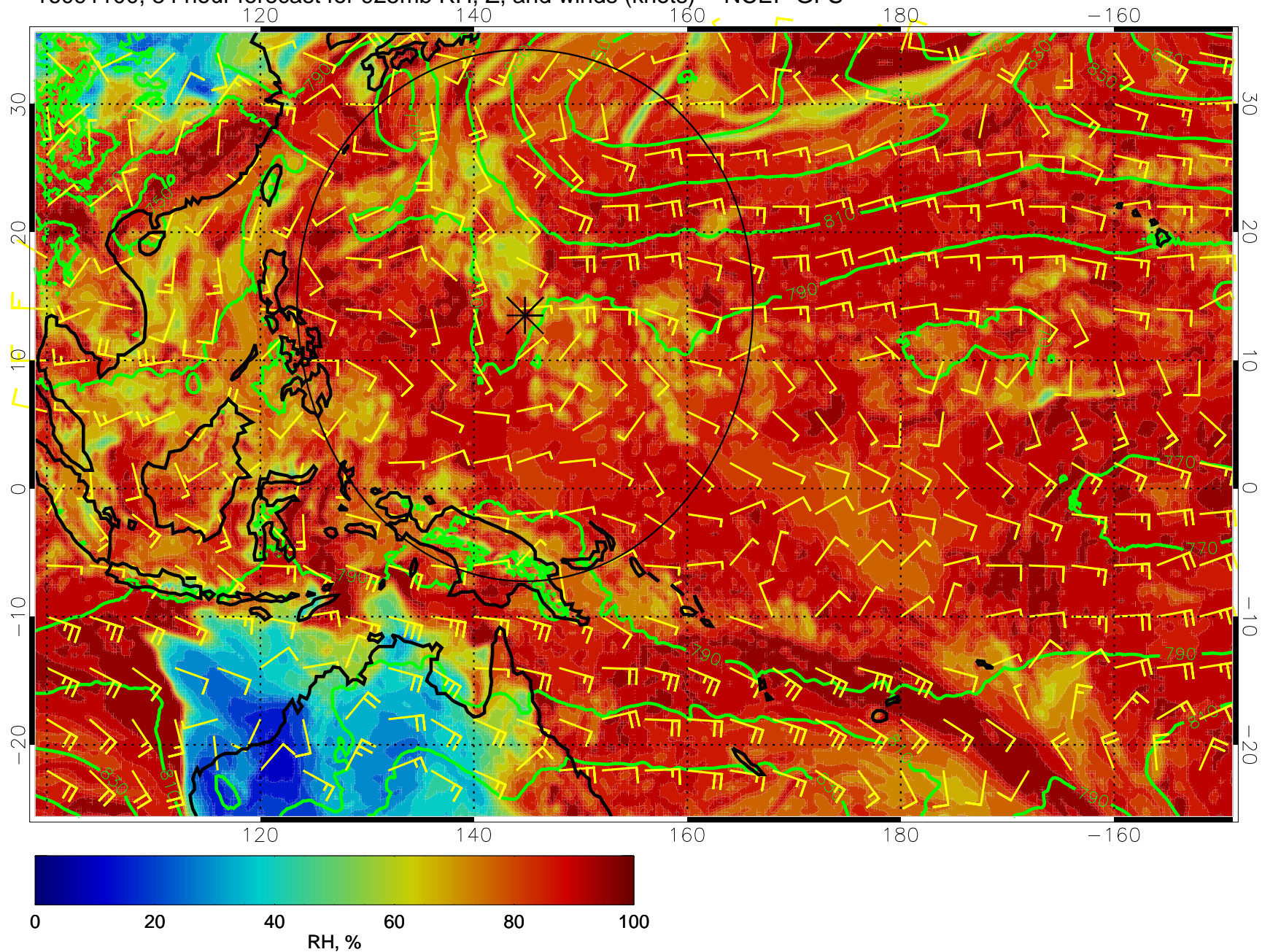
16091100, 84 hour forecast for 925mb RH, Z, and winds (knots) -- NCEP GFS
