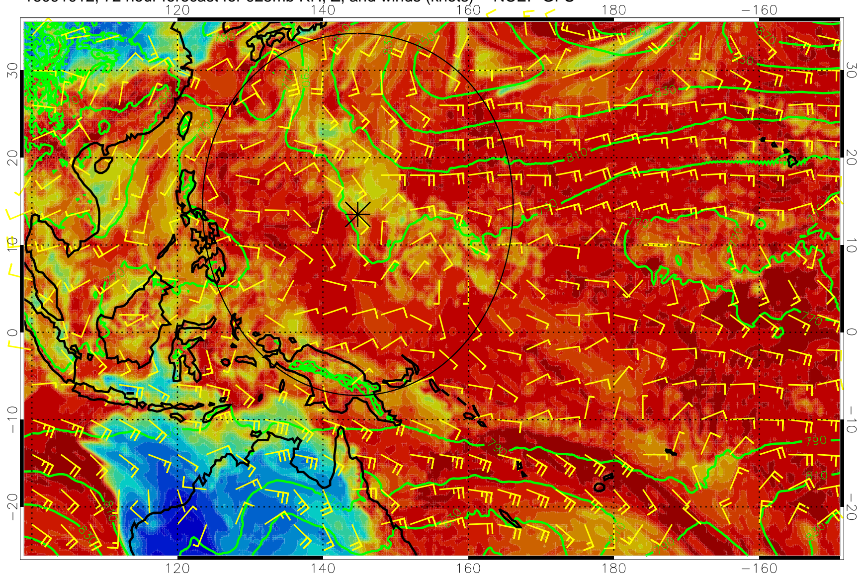
16091012, 72 hour forecast for 925mb RH, Z, and winds (knots) -- NCEP GFS
