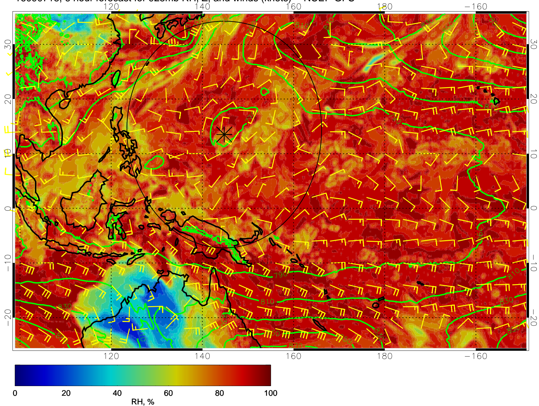
16090718, 6 hour forecast for 925mb RH, Z, and winds (knots) -- NCEP GFS
