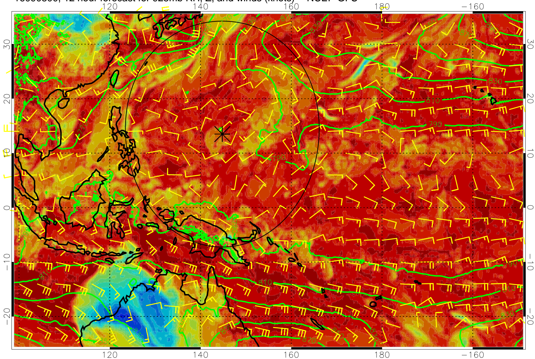
16090800, 12 hour forecast for 925mb RH, Z, and winds (knots) -- NCEP GFS
