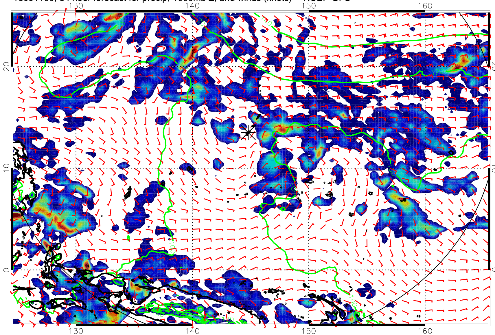
16091100, 84 hour forecast for precip, 1000mb Z, and winds (knots) -- NCEP GFS
