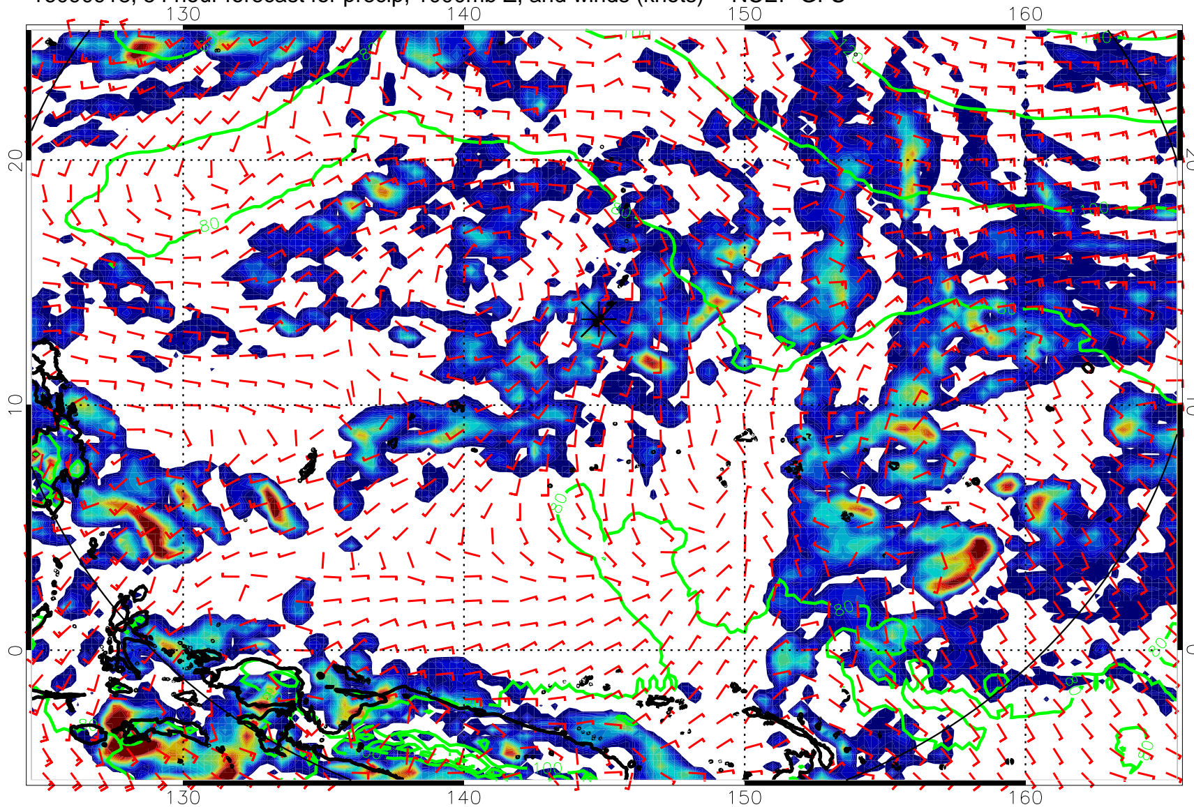
16090918, 54 hour forecast for precip, 1000mb Z, and winds (knots) -- NCEP GFS
