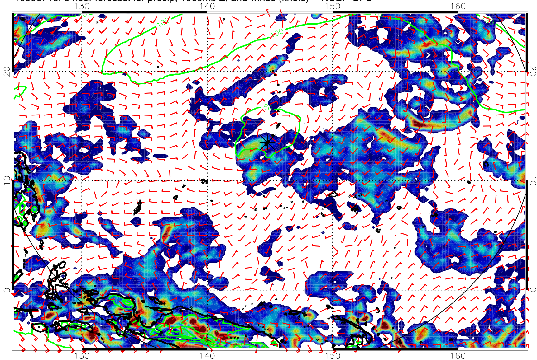
16090718, 6 hour forecast for precip, 1000mb Z, and winds (knots) -- NCEP GFS
