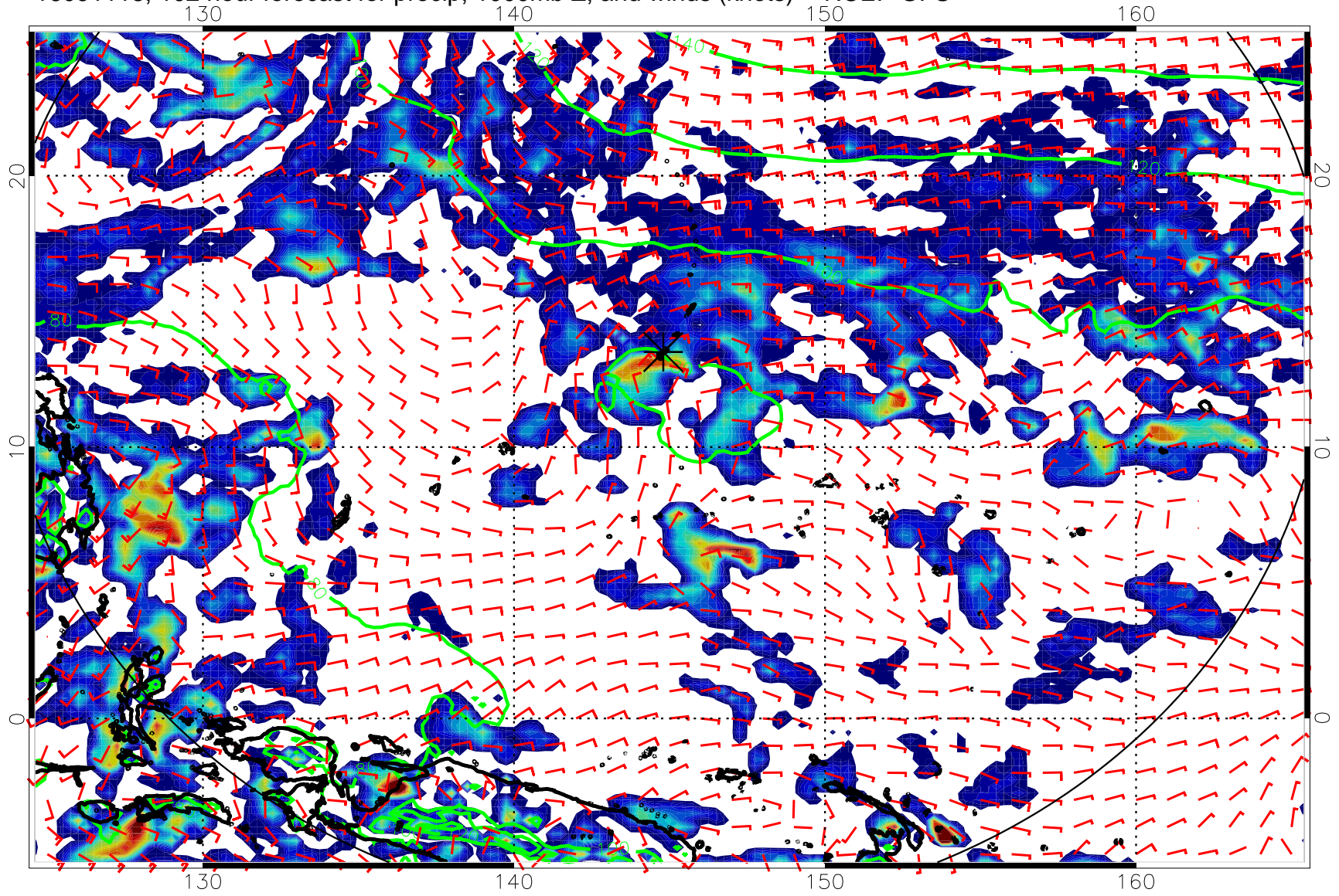
16091118, 102 hour forecast for precip, 1000mb Z, and winds (knots) -- NCEP GFS
