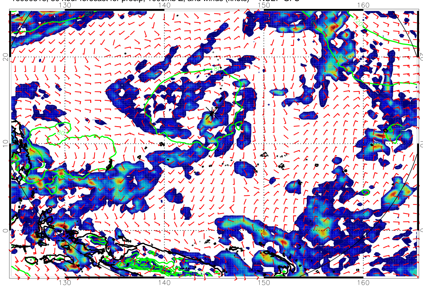
16090818, 30 hour forecast for precip, 1000mb Z, and winds (knots) -- NCEP GFS
