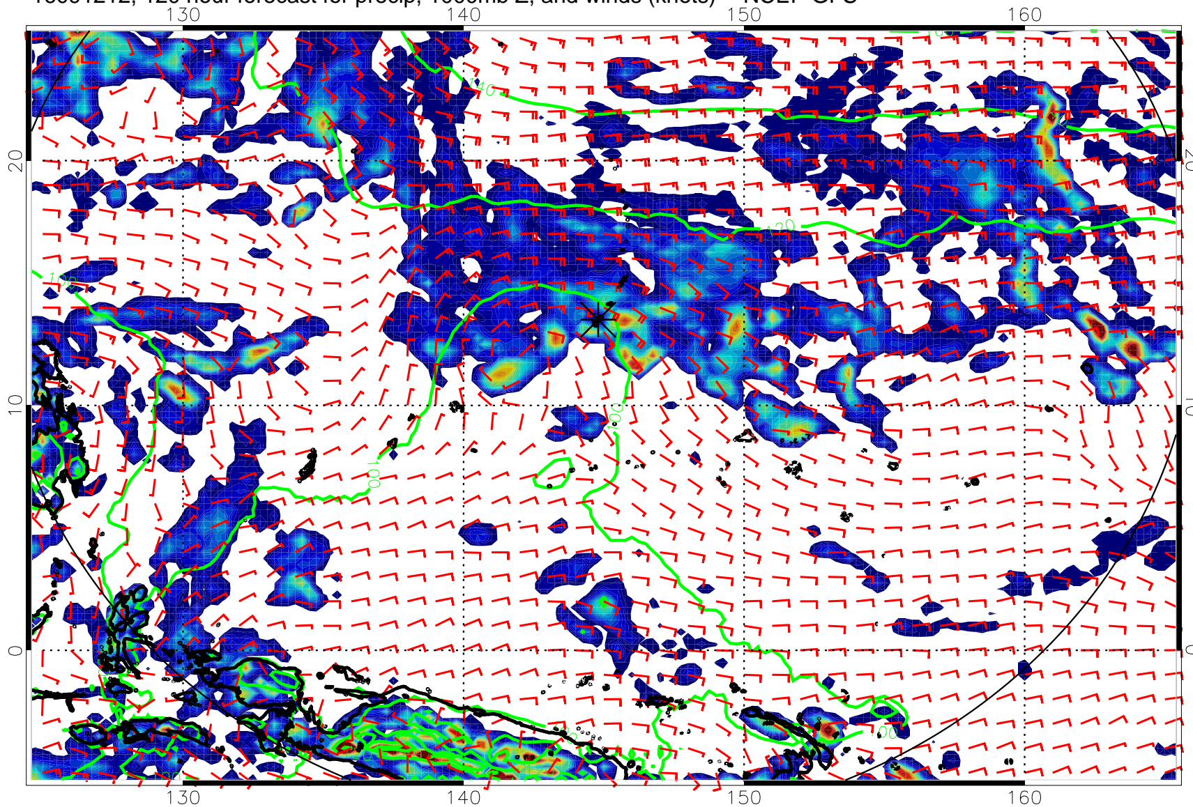
16091212, 120 hour forecast for precip, 1000mb Z, and winds (knots) -- NCEP GFS
