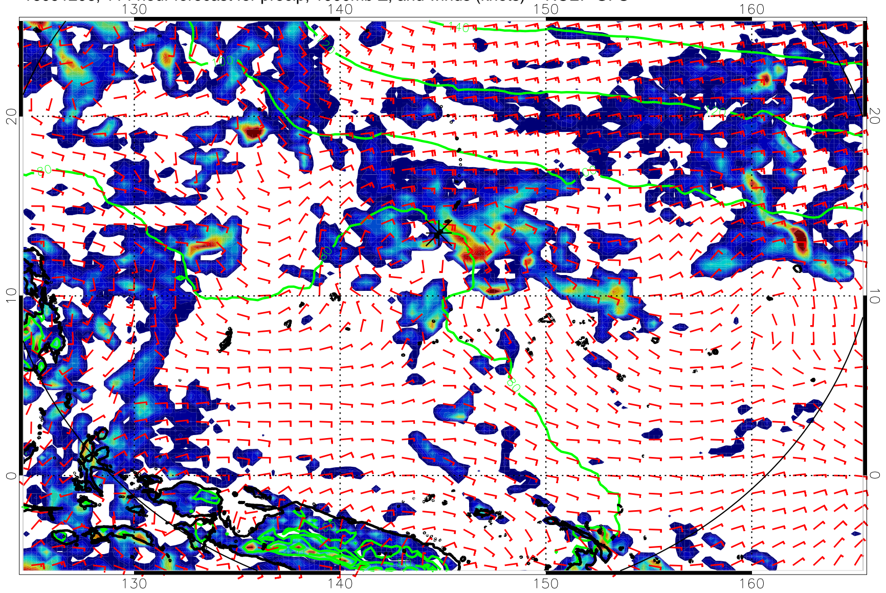
16091206, 114 hour forecast for precip, 1000mb Z, and winds (knots) -- NCEP GFS
