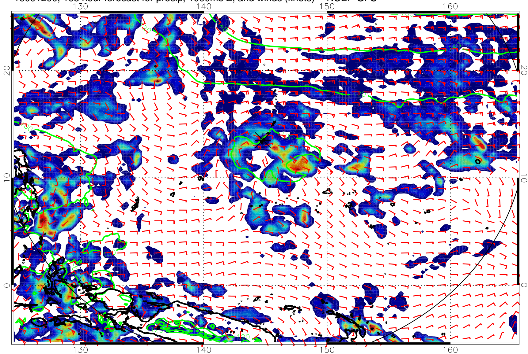
16091200, 108 hour forecast for precip, 1000mb Z, and winds (knots) -- NCEP GFS
