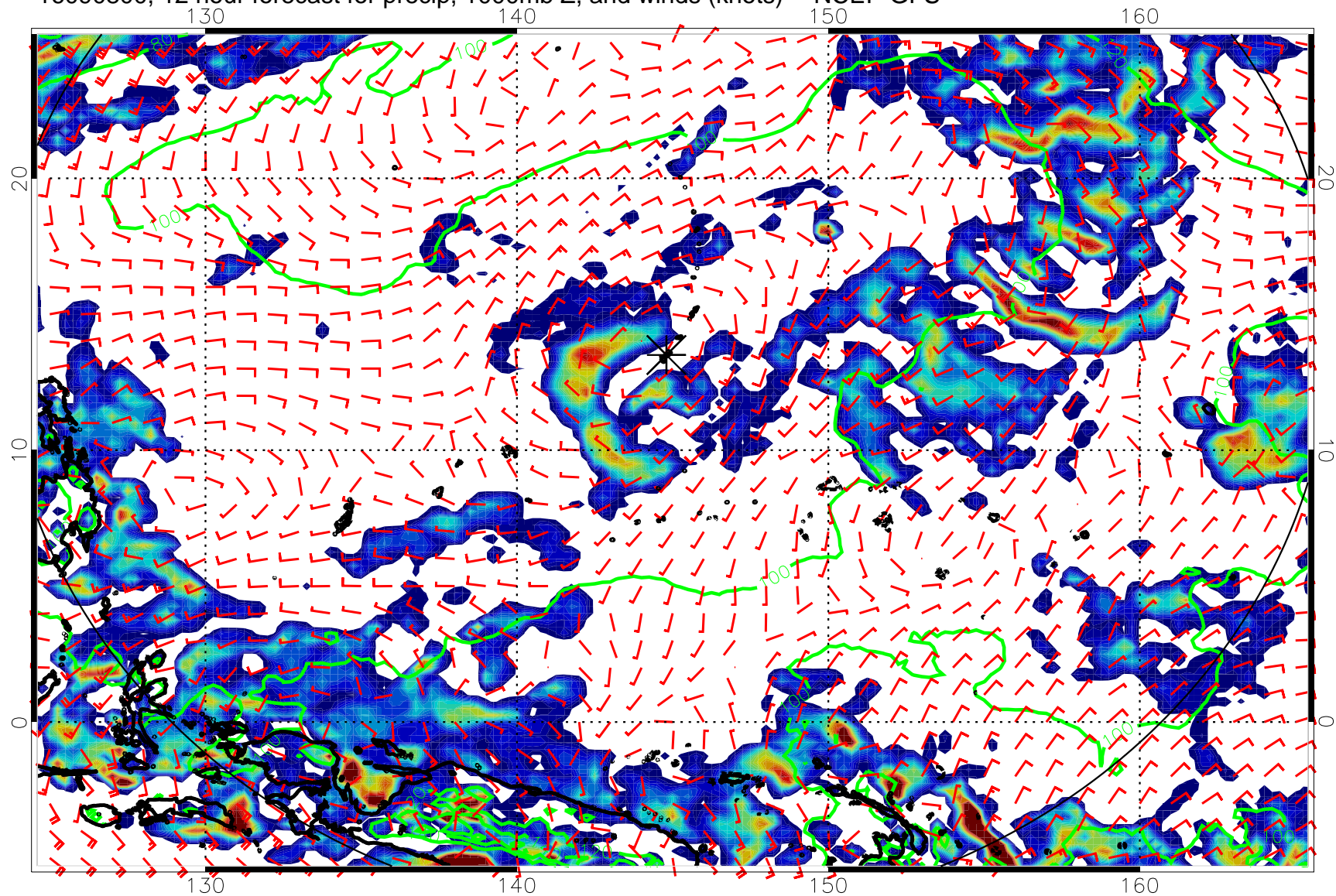
16090800, 12 hour forecast for precip, 1000mb Z, and winds (knots) -- NCEP GFS
