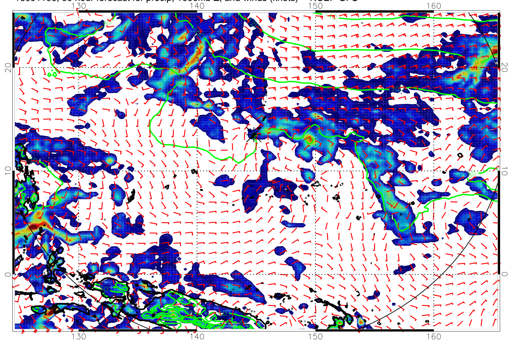
16091106, 90 hour forecast for precip, 1000mb Z, and winds (knots) -- NCEP GFS
