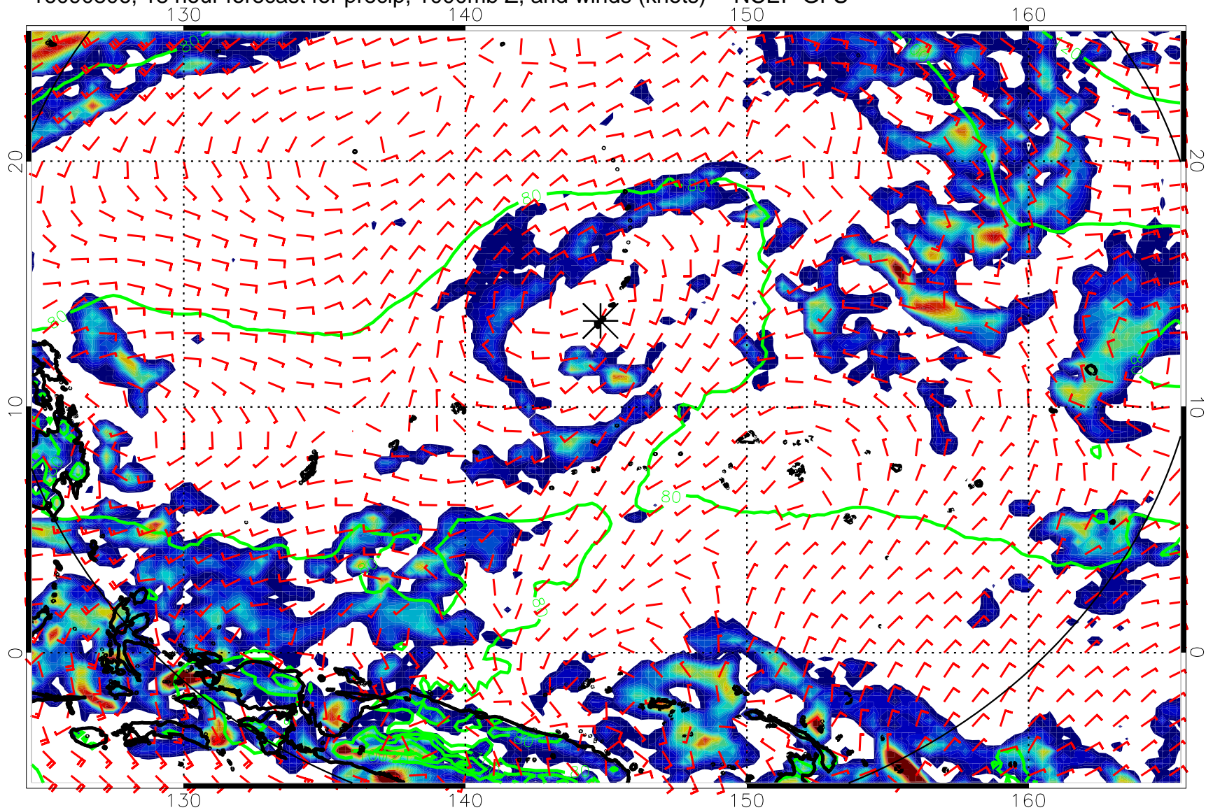
16090806, 18 hour forecast for precip, 1000mb Z, and winds (knots) -- NCEP GFS
