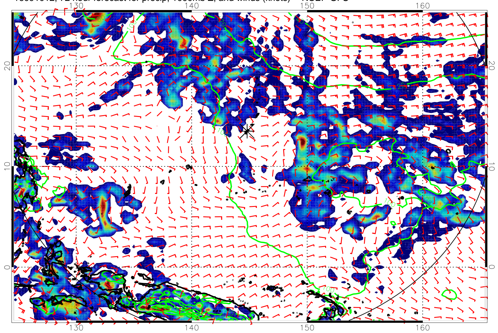
16091012, 72 hour forecast for precip, 1000mb Z, and winds (knots) -- NCEP GFS
