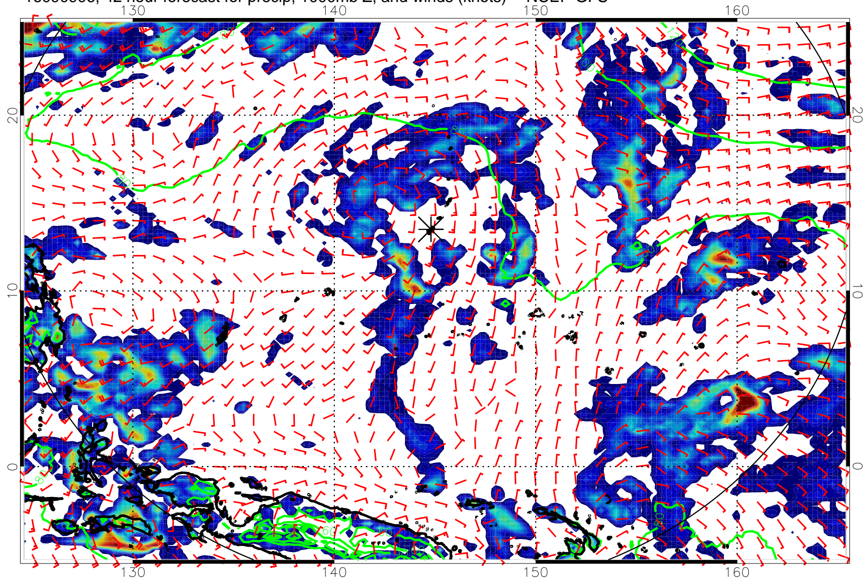
16090906, 42 hour forecast for precip, 1000mb Z, and winds (knots) -- NCEP GFS
