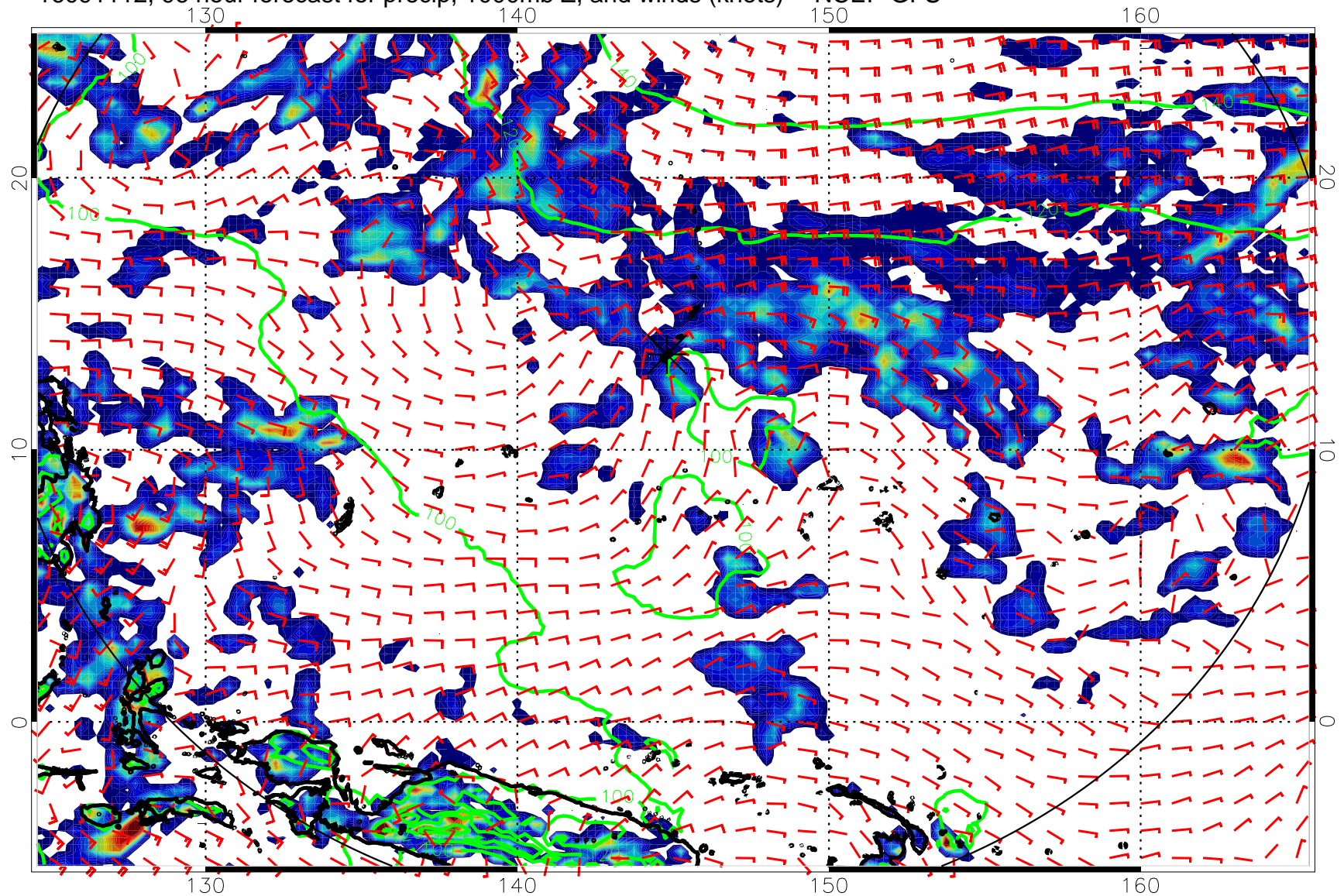
16091112, 96 hour forecast for precip, 1000mb Z, and winds (knots) -- NCEP GFS
