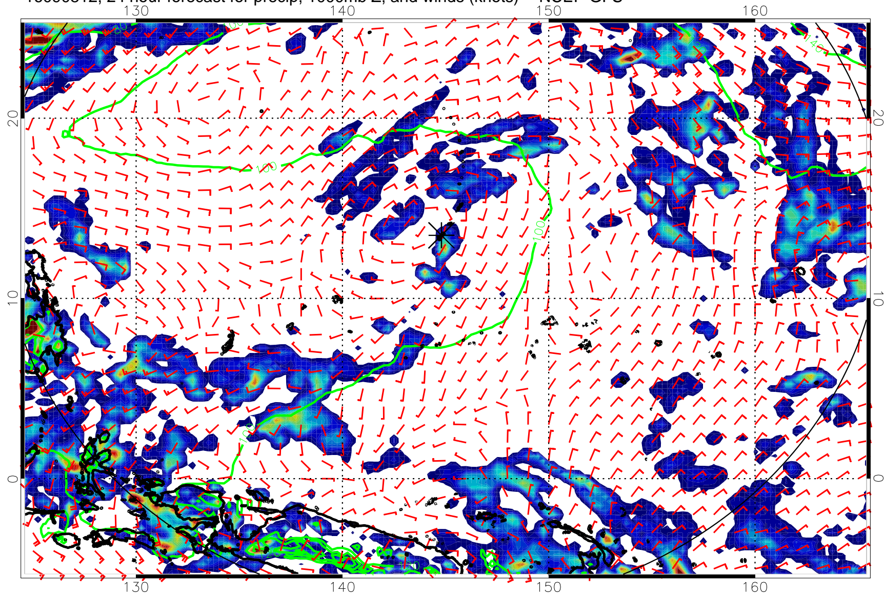
16090812, 24 hour forecast for precip, 1000mb Z, and winds (knots) -- NCEP GFS
