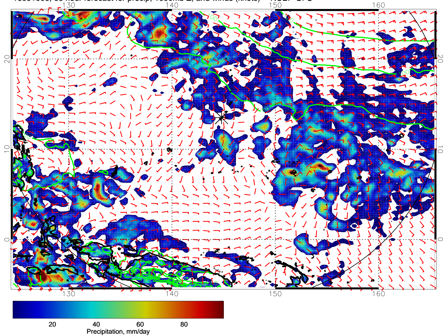
16091006, 66 hour forecast for precip, 1000mb Z, and winds (knots) -- NCEP GFS
