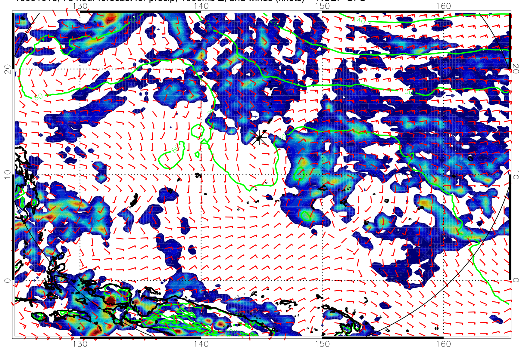
16091018, 78 hour forecast for precip, 1000mb Z, and winds (knots) -- NCEP GFS
