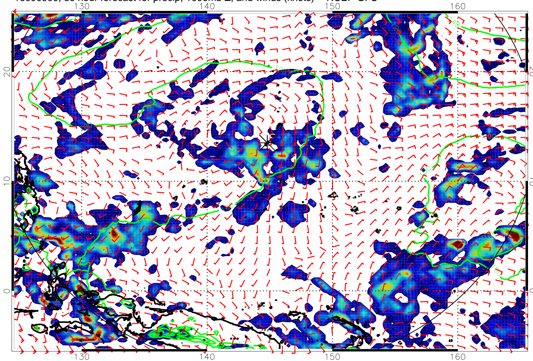
16090900, 36 hour forecast for precip, 1000mb Z, and winds (knots) -- NCEP GFS
