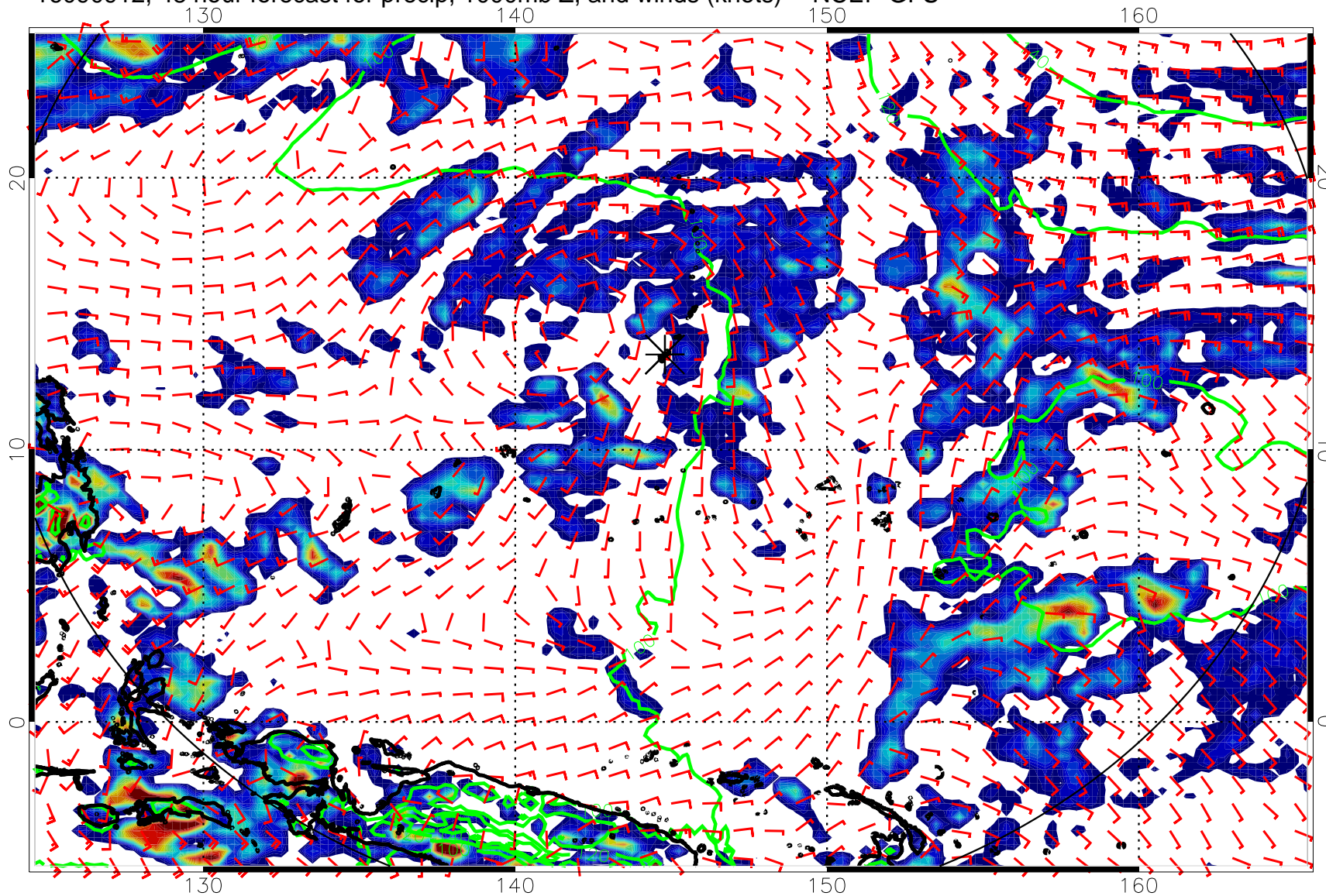
16090912, 48 hour forecast for precip, 1000mb Z, and winds (knots) -- NCEP GFS
