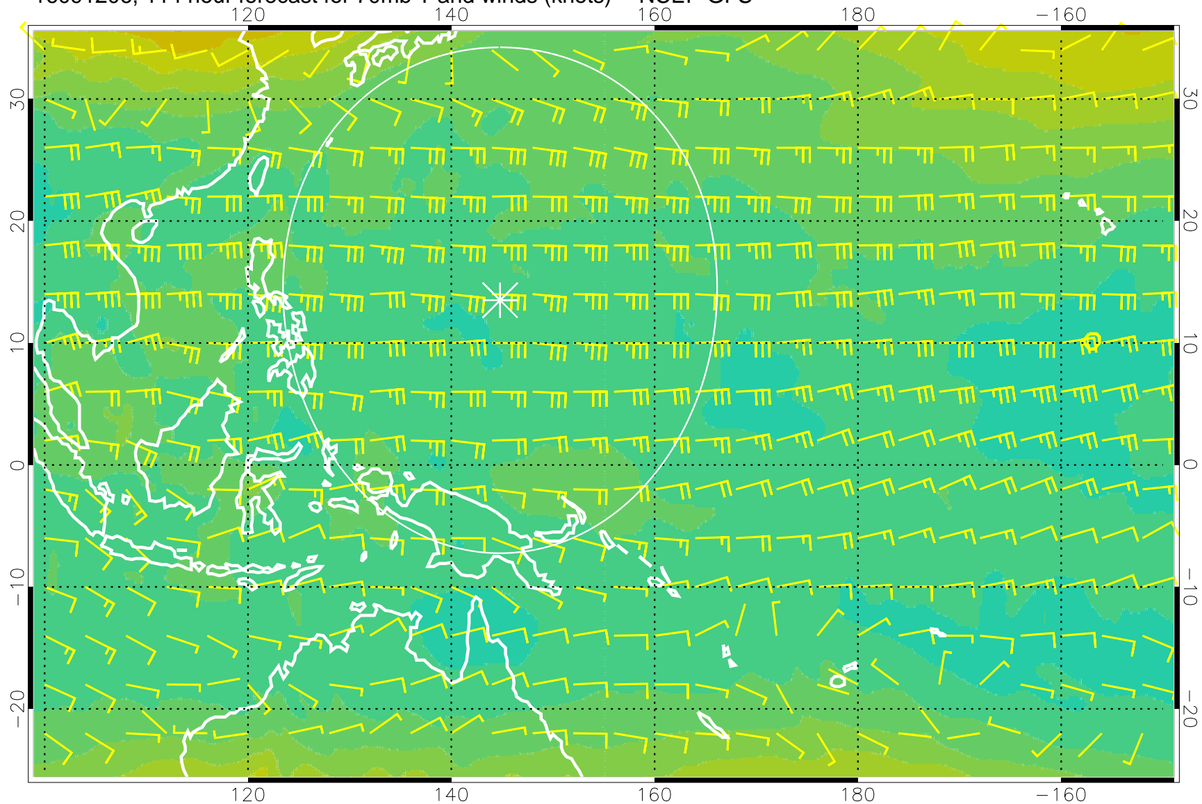
16091206, 114 hour forecast for 70mb T and winds (knots) -- NCEP GFS
