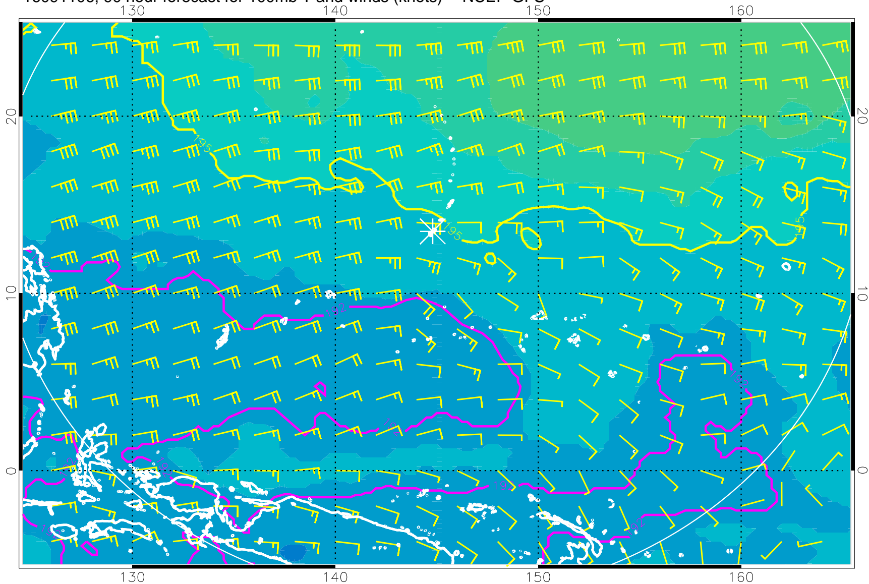
16091106, 90 hour forecast for 100mb T and winds (knots) -- NCEP GFS
