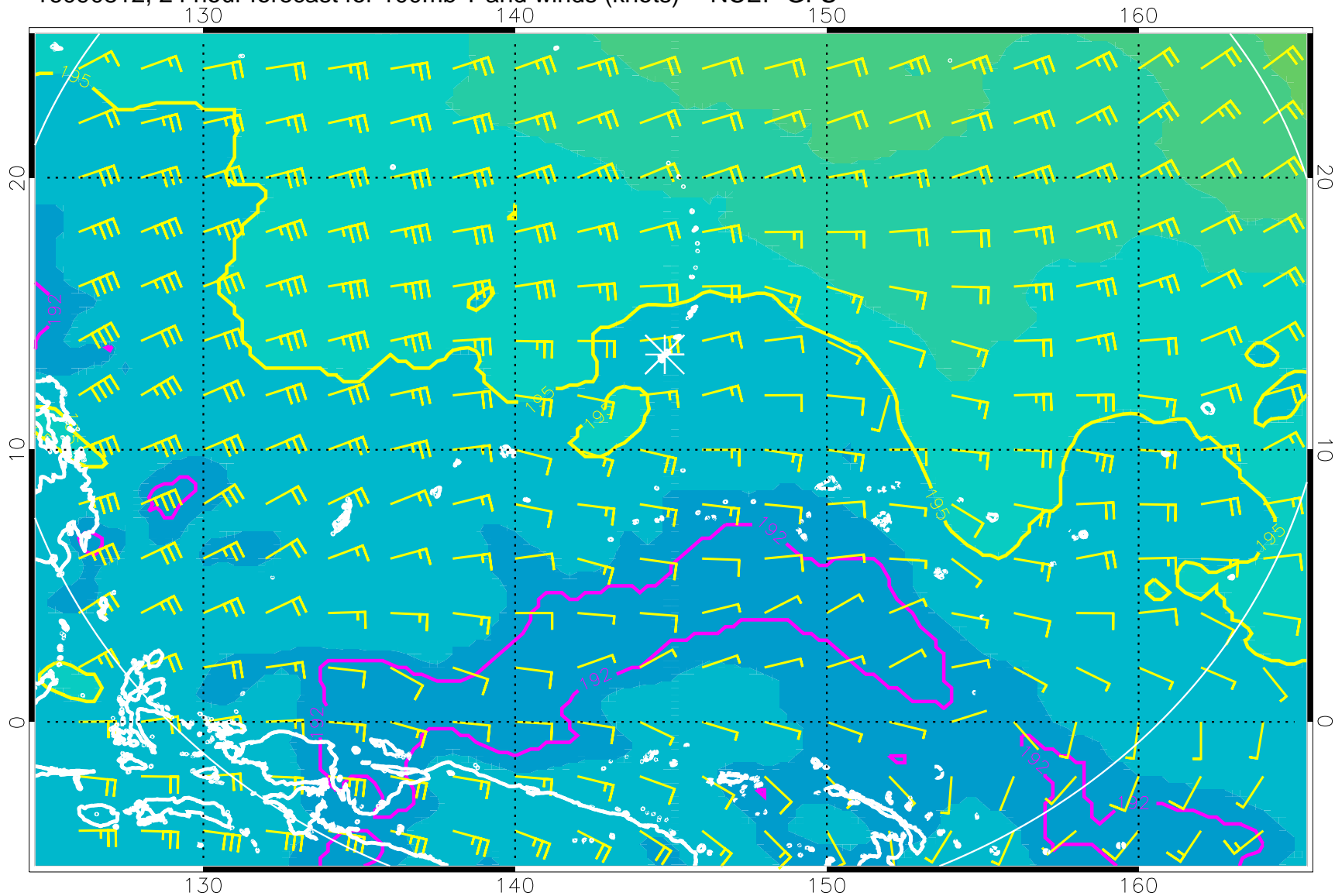
16090812, 24 hour forecast for 100mb T and winds (knots) -- NCEP GFS
