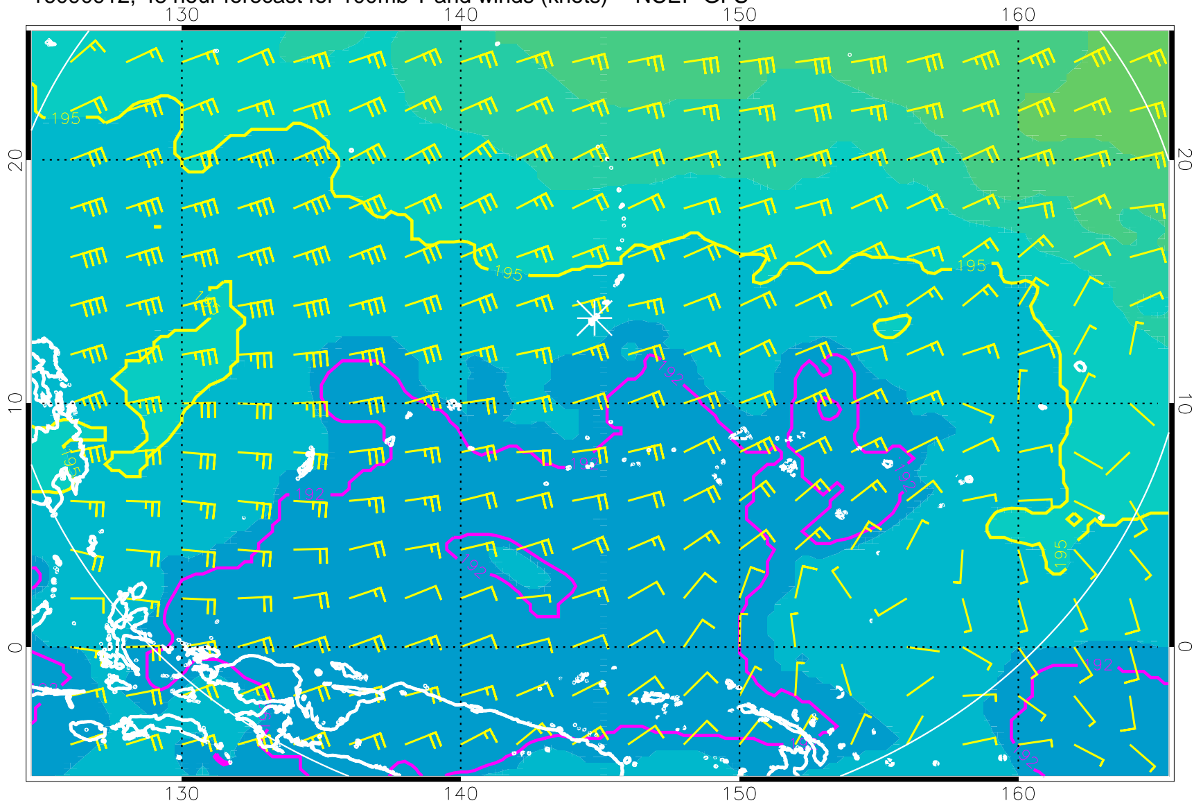
16090912, 48 hour forecast for 100mb T and winds (knots) -- NCEP GFS
