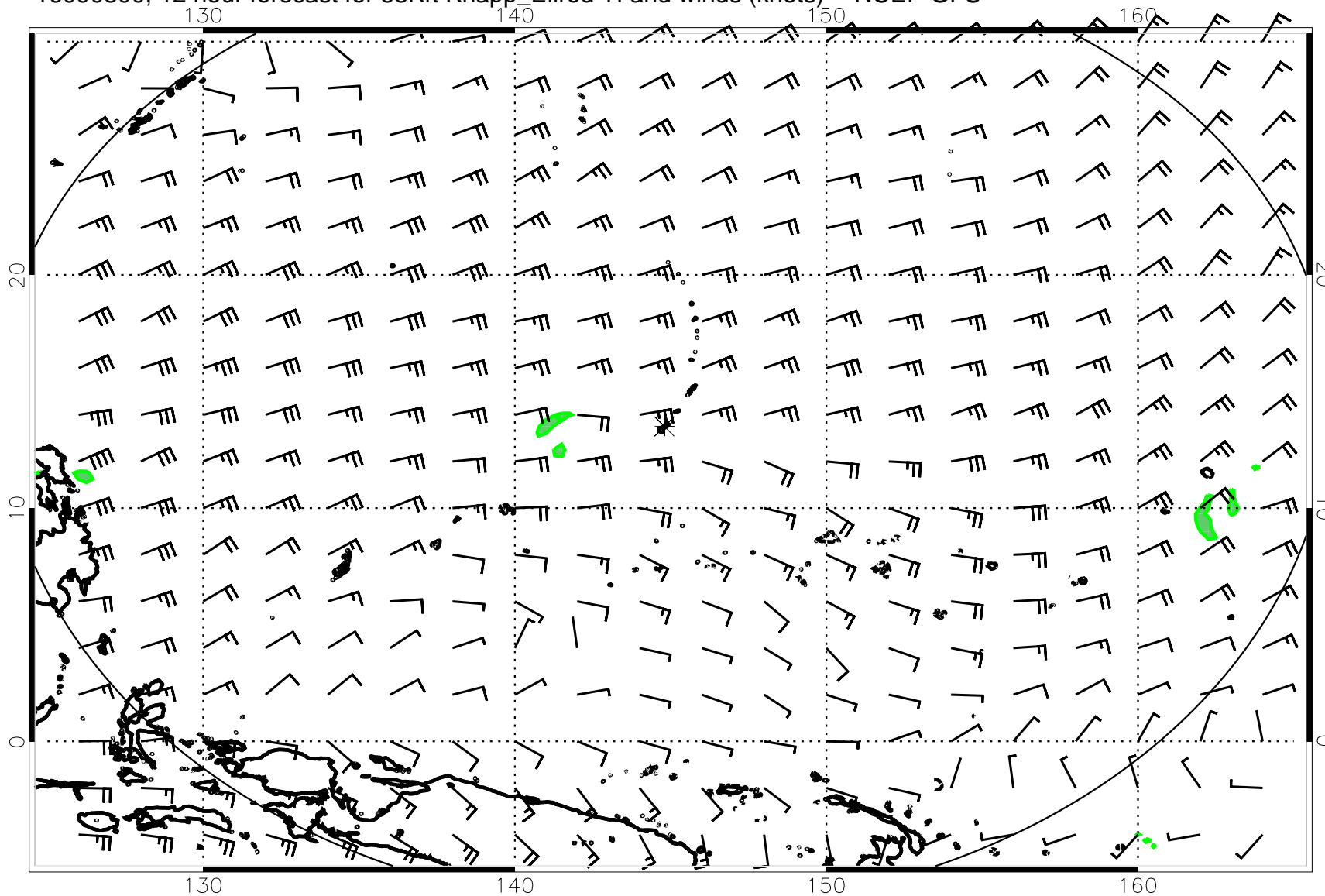
16090800, 12 hour forecast for 53Kft Knapp_Ellrod TI and winds (knots) -- NCEP GFS
