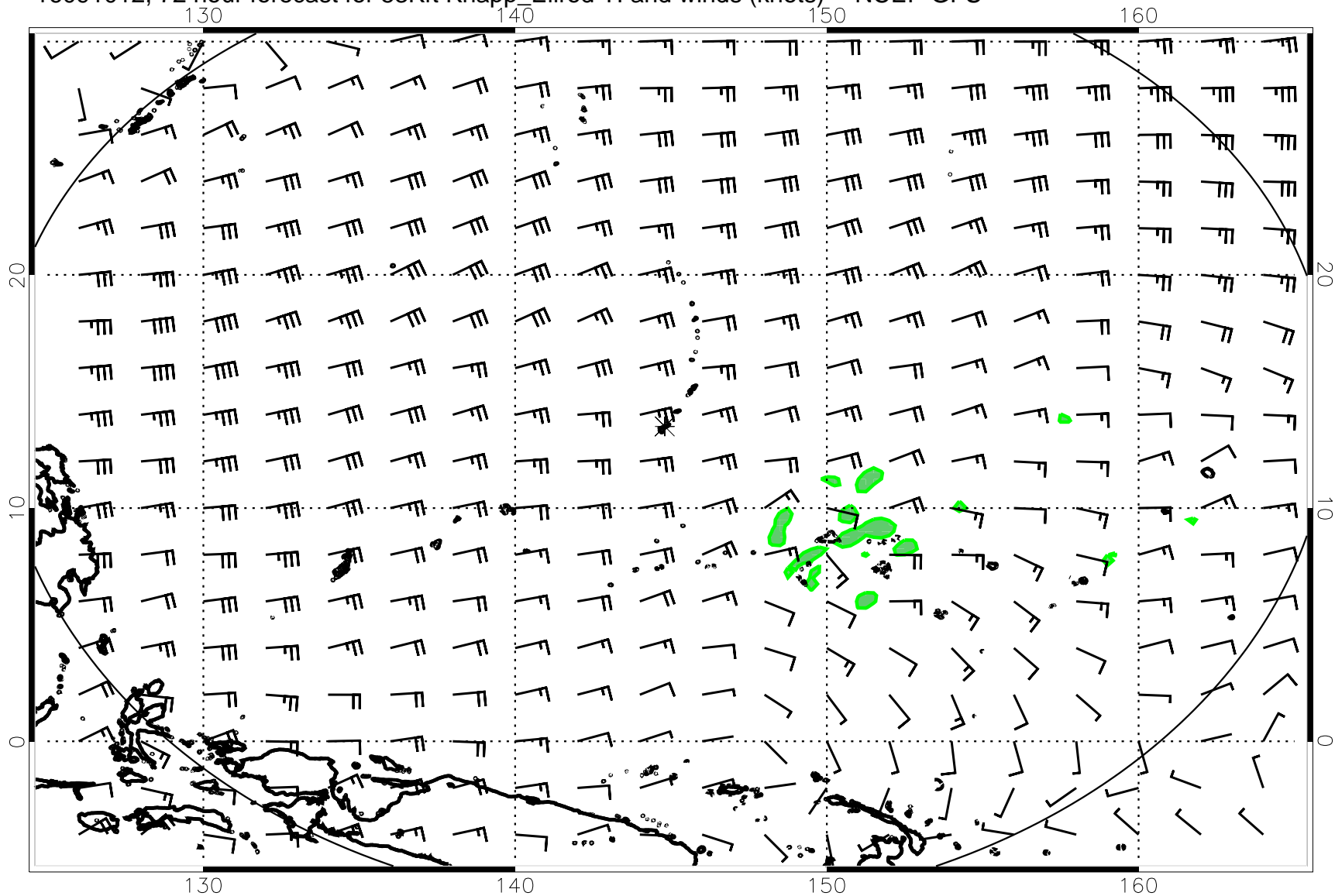
16091012, 72 hour forecast for 53Kft Knapp_Ellrod TI and winds (knots) -- NCEP GFS
