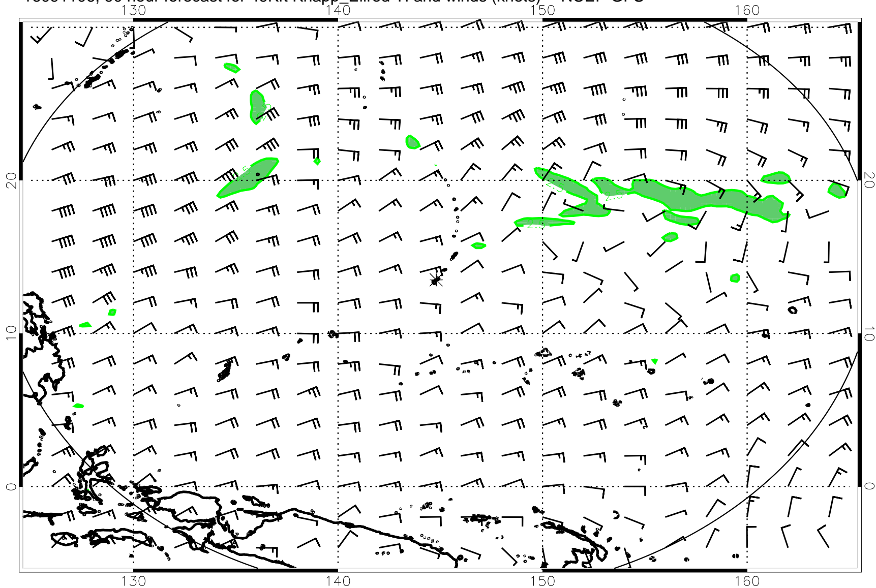
16091106, 90 hour forecast for 49Kft Knapp_Ellrod TI and winds (knots) -- NCEP GFS
