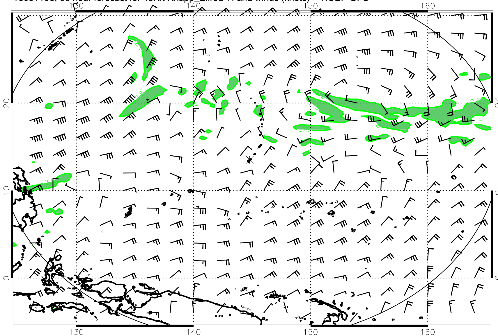
16091106, 90 hour forecast for 45Kft Knapp_Ellrod TI and winds (knots) -- NCEP GFS
