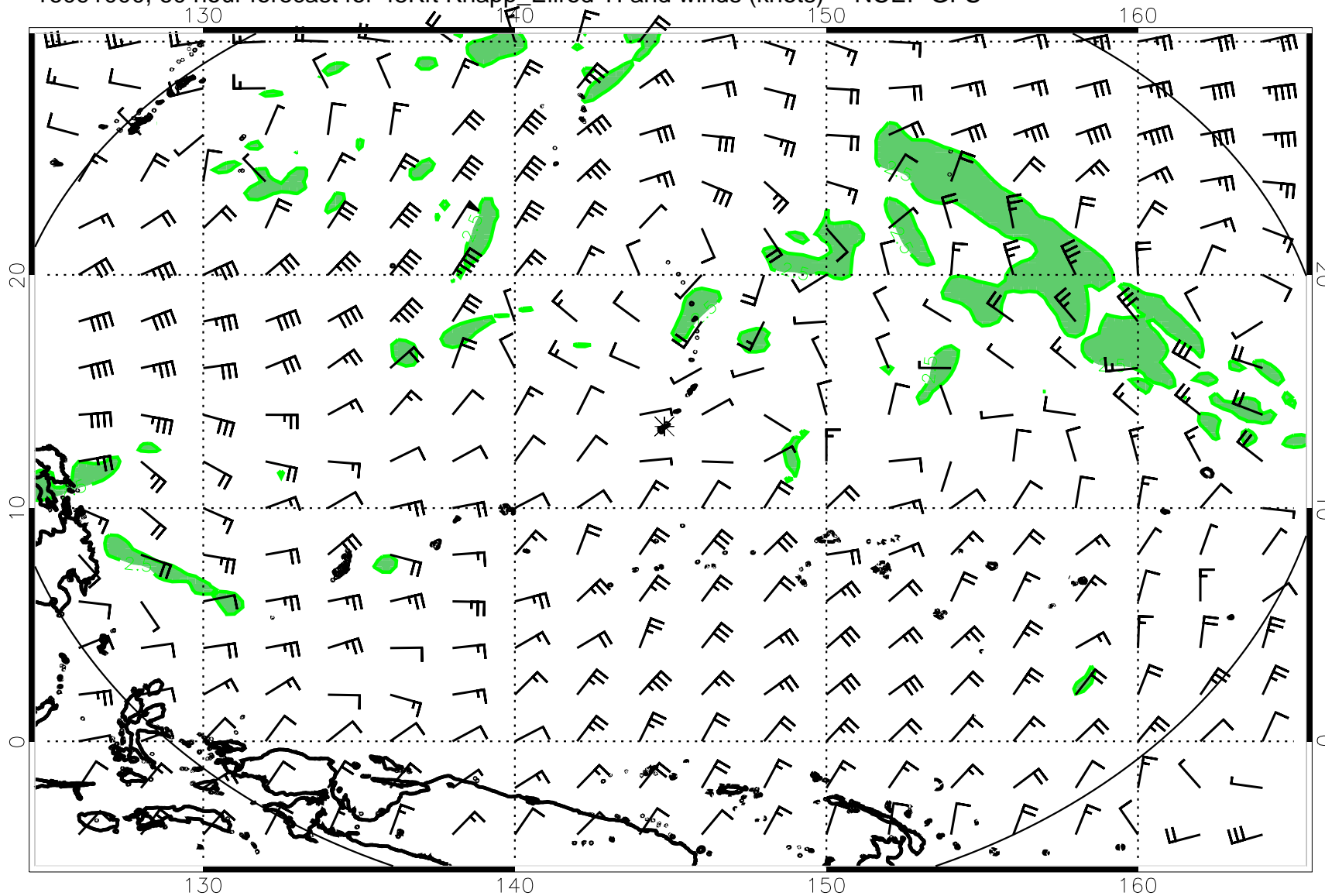
16091000, 60 hour forecast for 45Kft Knapp_Ellrod TI and winds (knots) -- NCEP GFS
