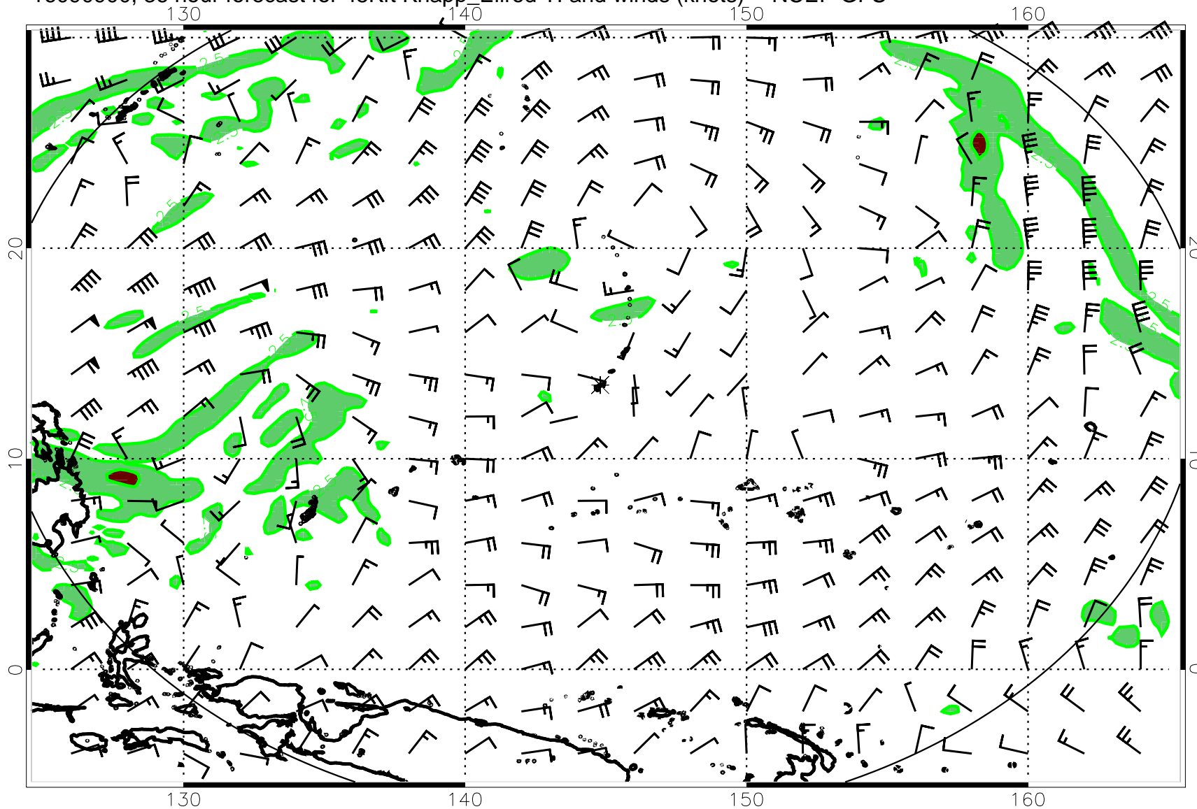
16090900, 36 hour forecast for 45Kft Knapp_Ellrod TI and winds (knots) -- NCEP GFS
