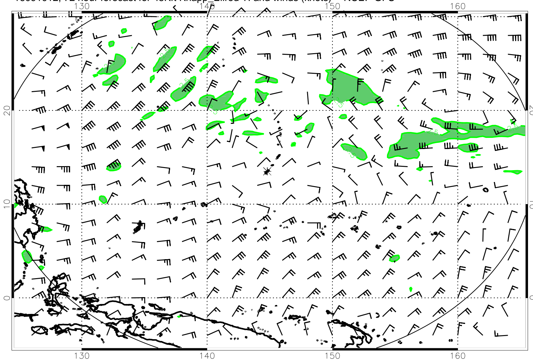
16091012, 72 hour forecast for 45Kft Knapp_Ellrod TI and winds (knots) -- NCEP GFS
