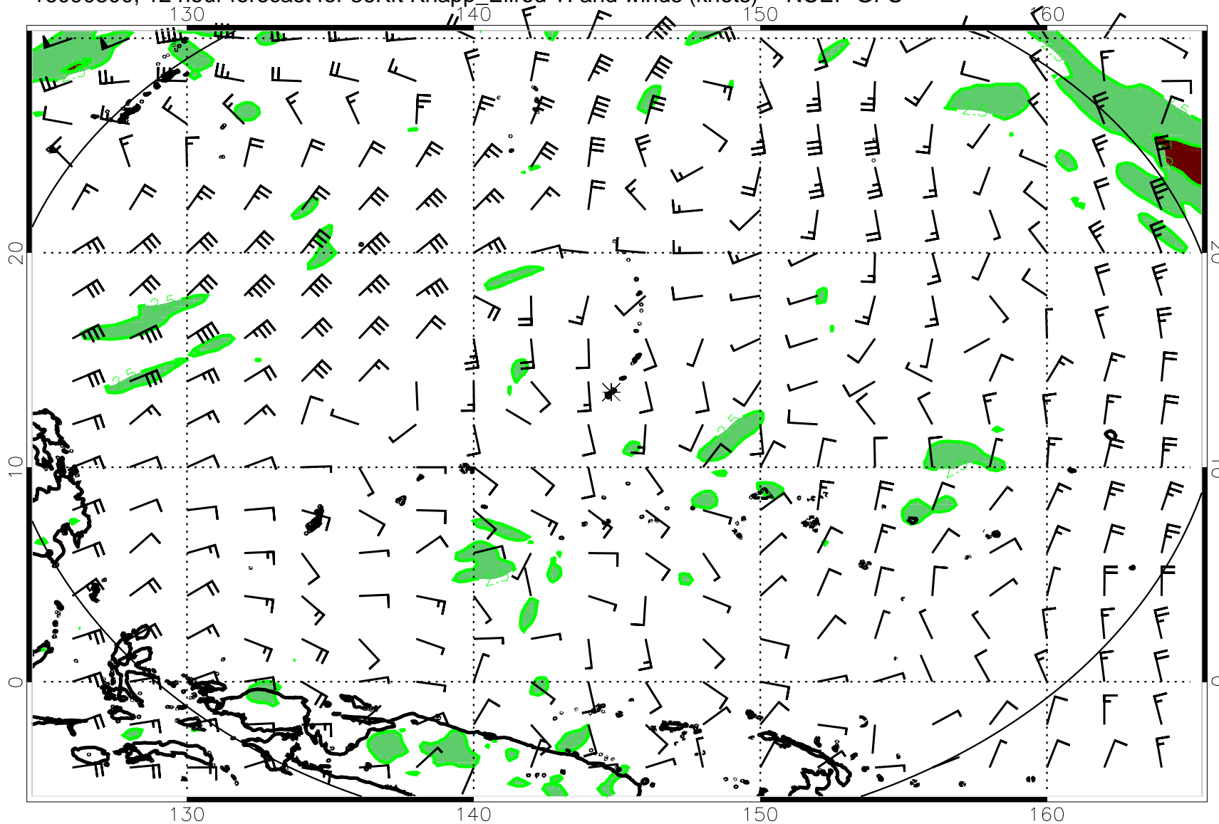
16090800, 12 hour forecast for 36Kft Knapp_Ellrod TI and winds (knots) -- NCEP GFS
