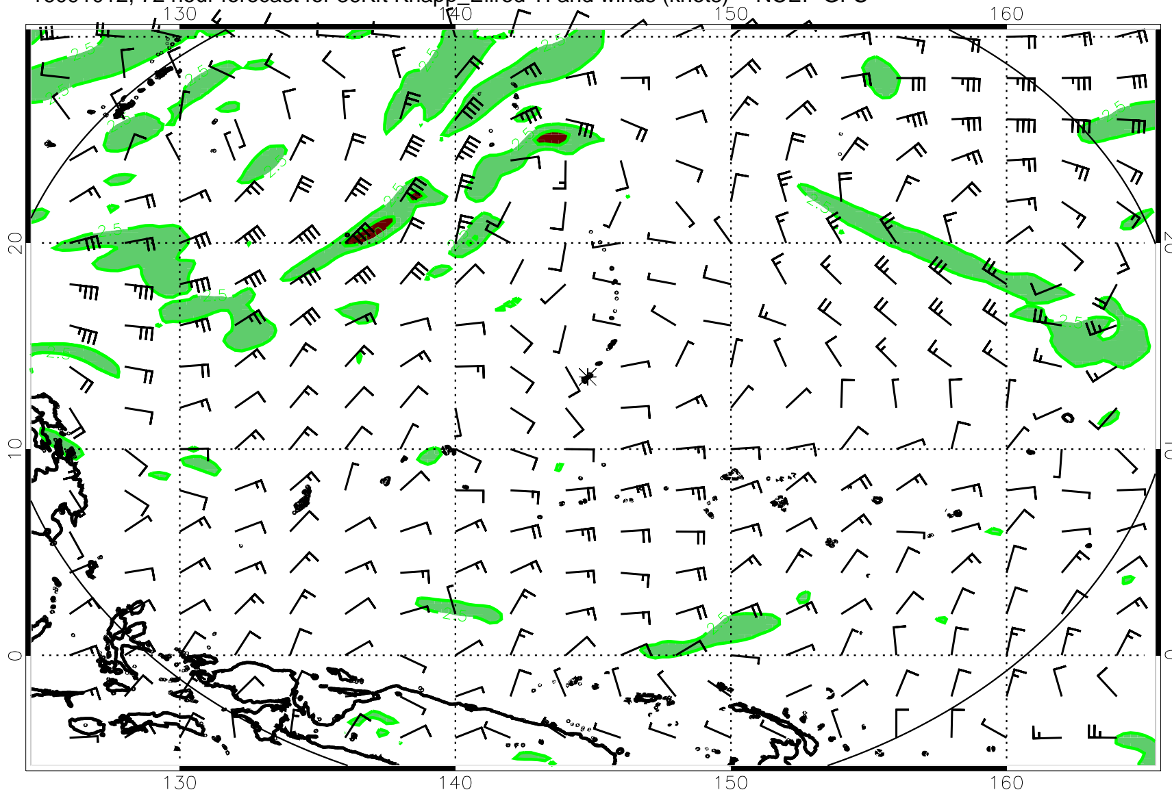
16091012, 72 hour forecast for 36Kft Knapp_Ellrod TI and winds (knots) -- NCEP GFS
