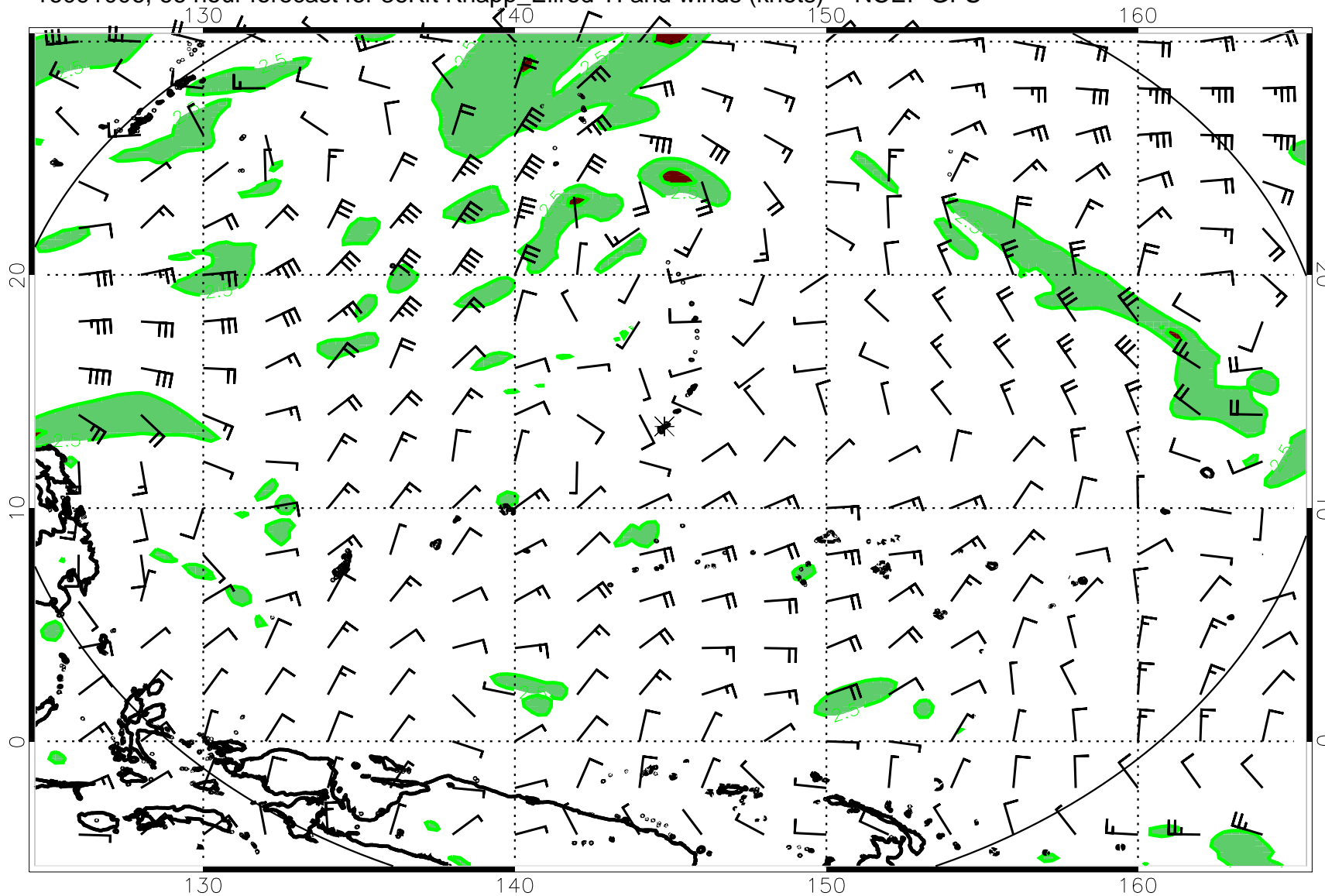
16091006, 66 hour forecast for 36Kft Knapp_Ellrod TI and winds (knots) -- NCEP GFS
