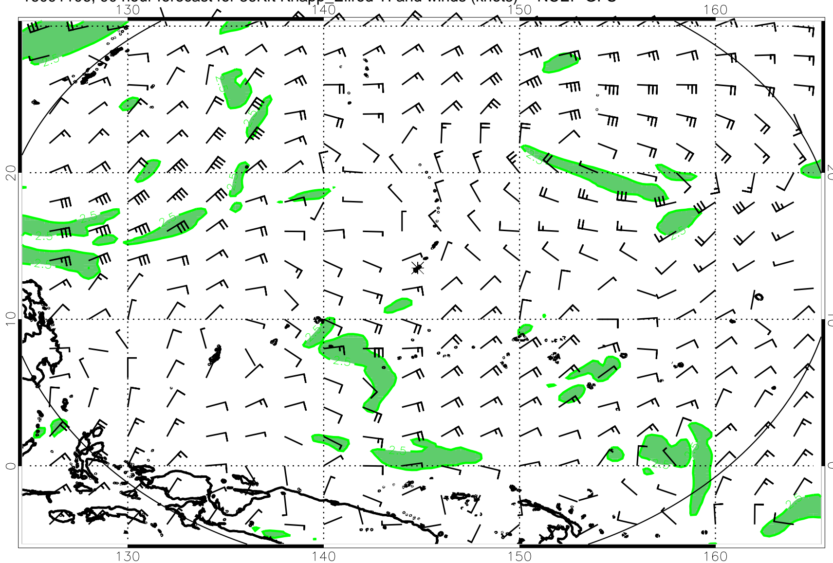
16091106, 90 hour forecast for 36Kft Knapp_Ellrod TI and winds (knots) -- NCEP GFS
