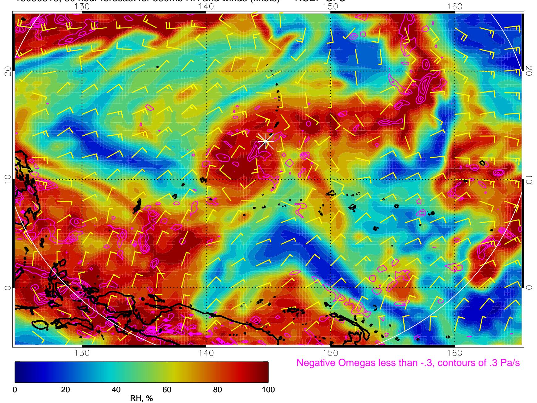
16090818, 30 hour forecast for 500mb RH and winds (knots) -- NCEP GFS
