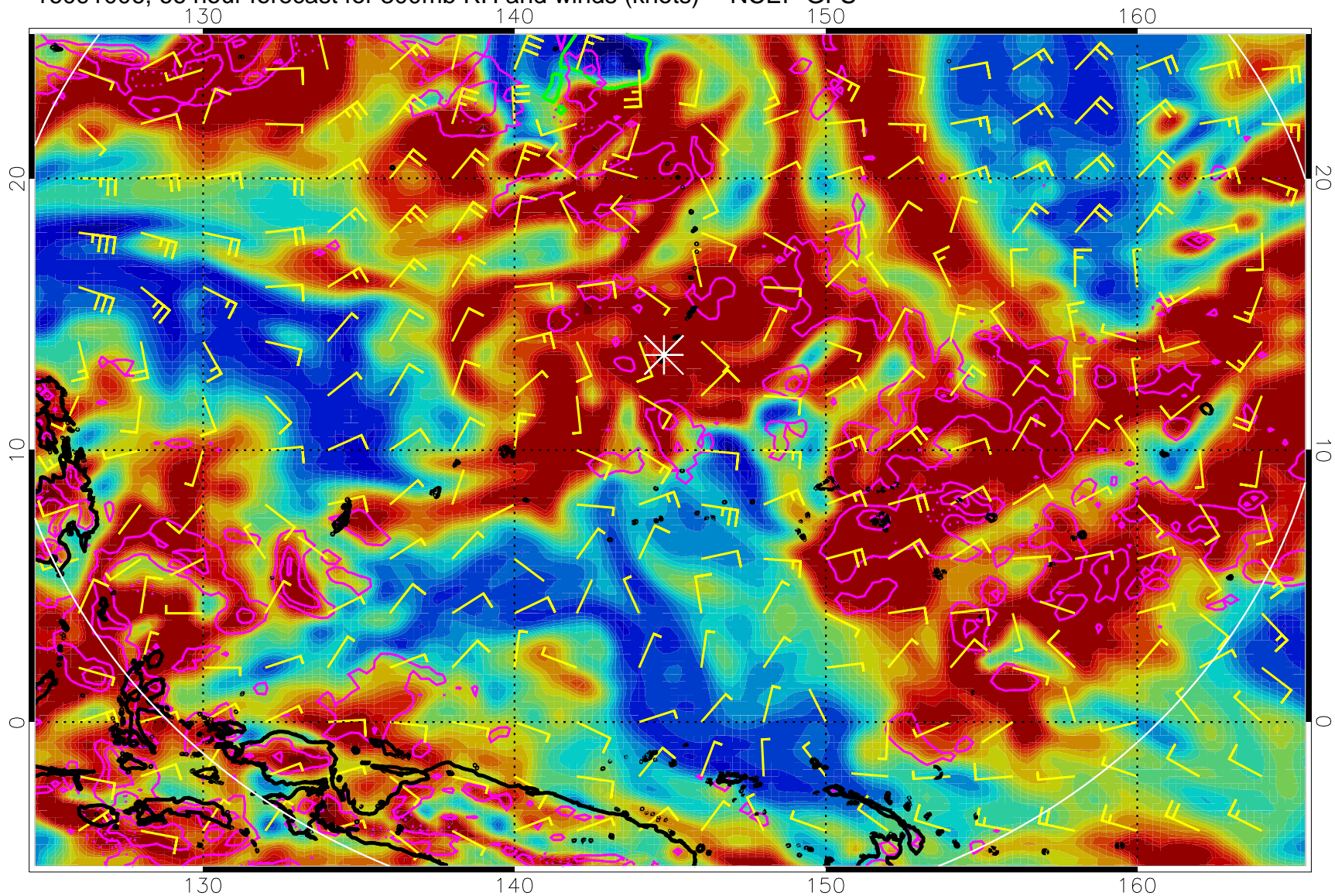
16091006, 66 hour forecast for 300mb RH and winds (knots) -- NCEP GFS
