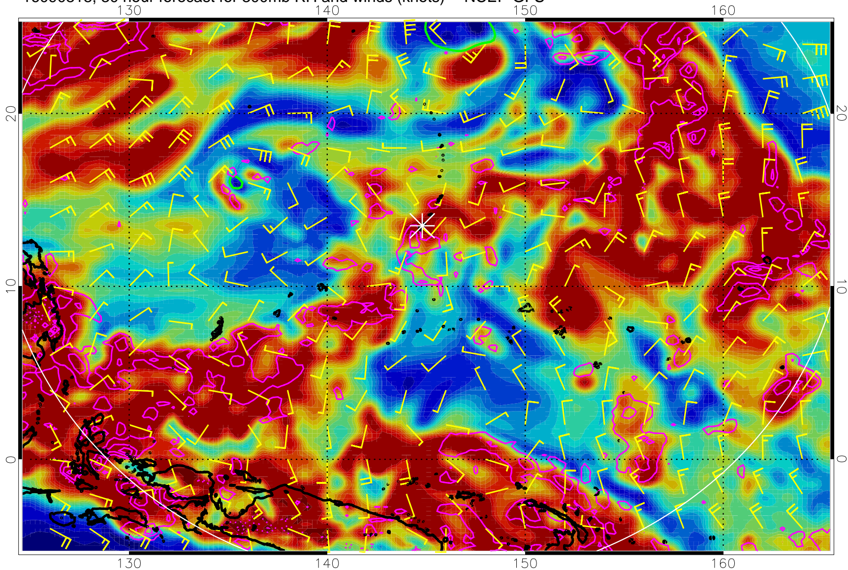
16090818, 30 hour forecast for 300mb RH and winds (knots) -- NCEP GFS
