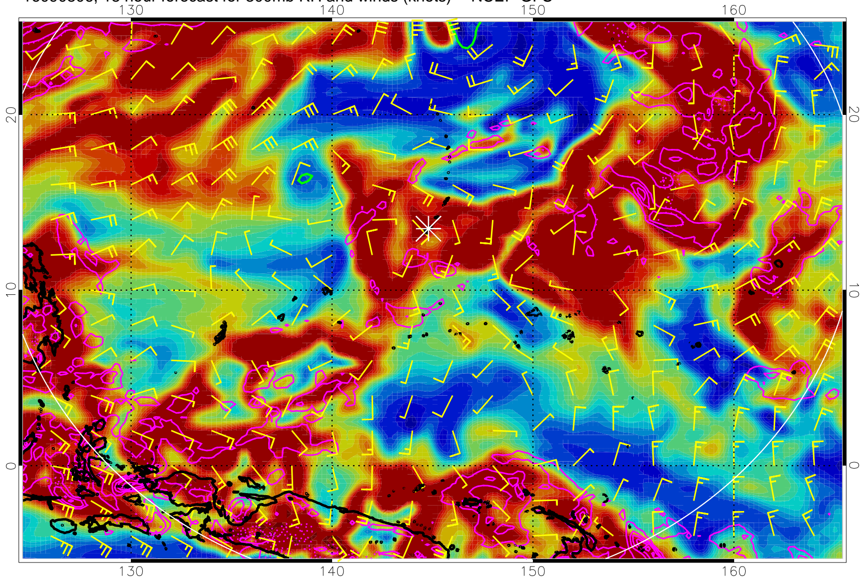
16090806, 18 hour forecast for 300mb RH and winds (knots) -- NCEP GFS
