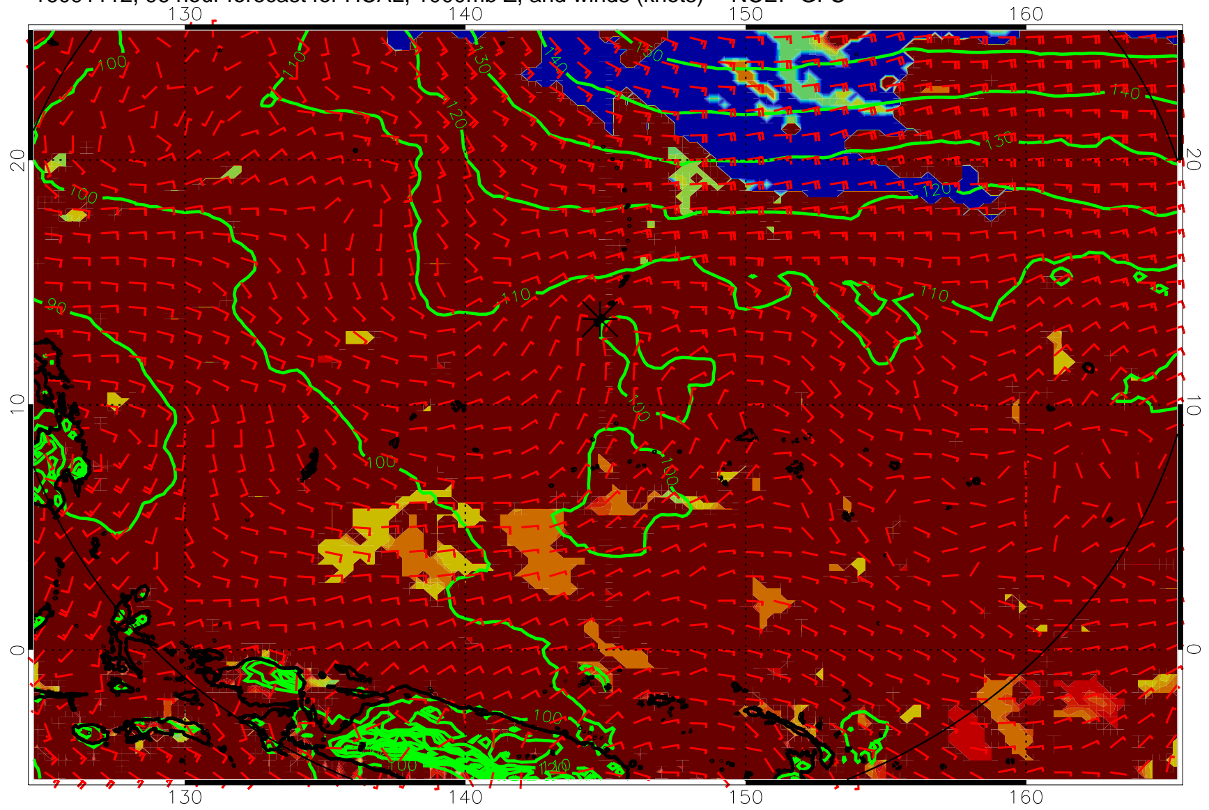
16091112, 96 hour forecast for HCAL, 1000mb Z, and winds (knots) -- NCEP GFS
