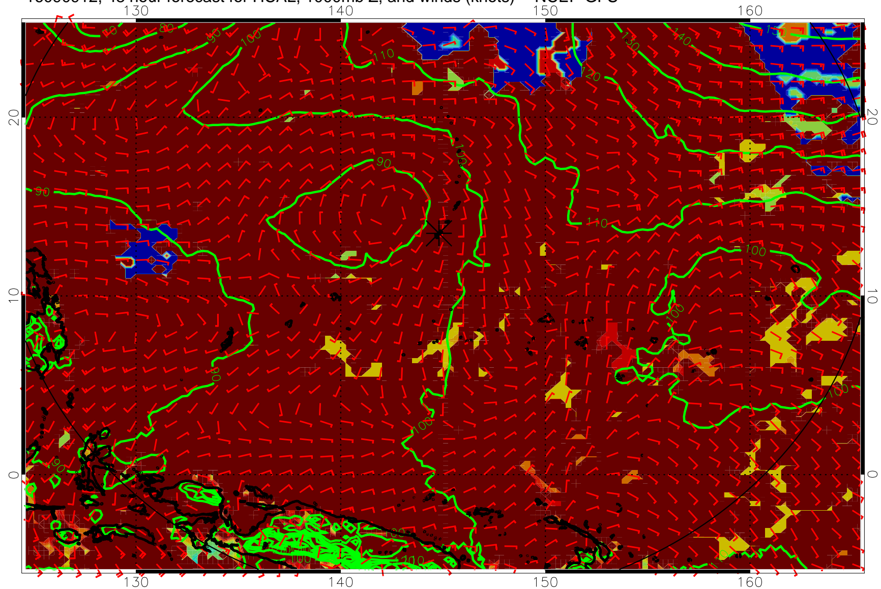
16090912, 48 hour forecast for HCAL, 1000mb Z, and winds (knots) -- NCEP GFS
