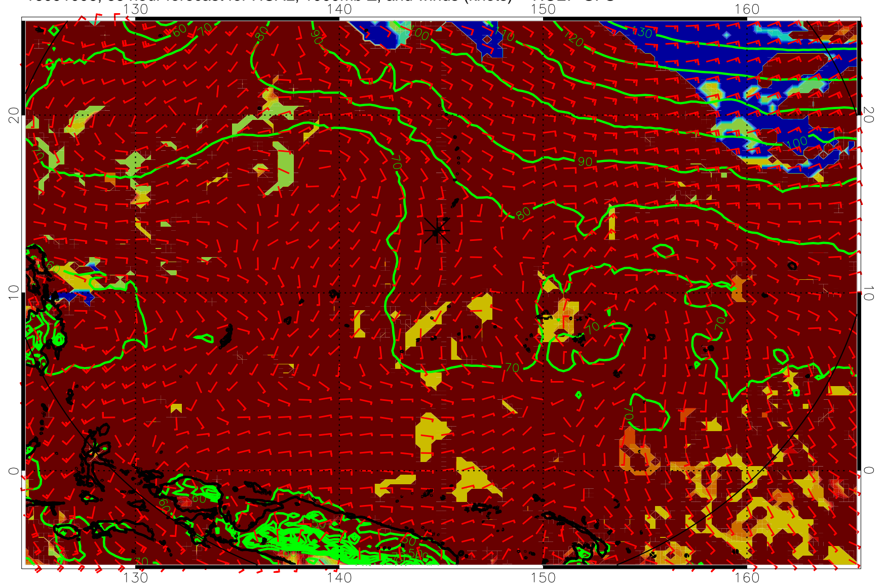
16091006, 66 hour forecast for HCAL, 1000mb Z, and winds (knots) -- NCEP GFS
