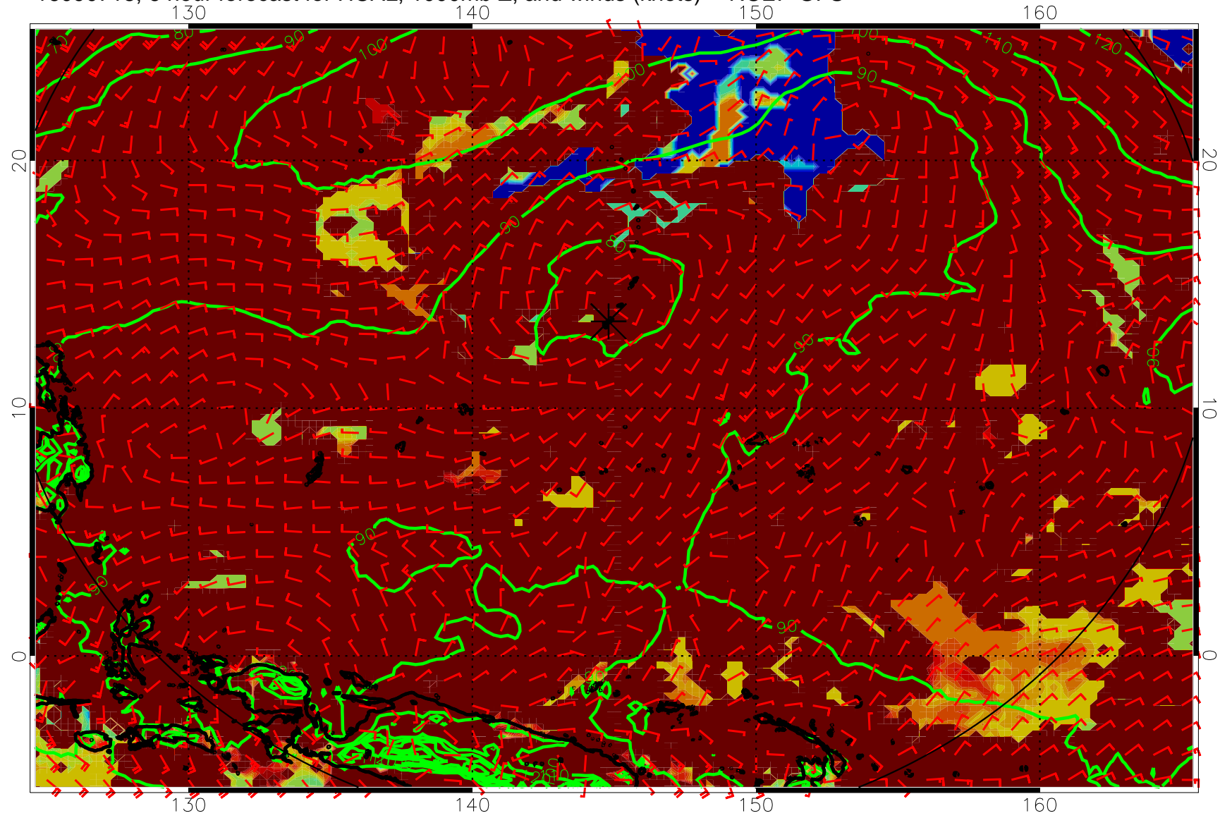
16090718, 6 hour forecast for HCAL, 1000mb Z, and winds (knots) -- NCEP GFS
