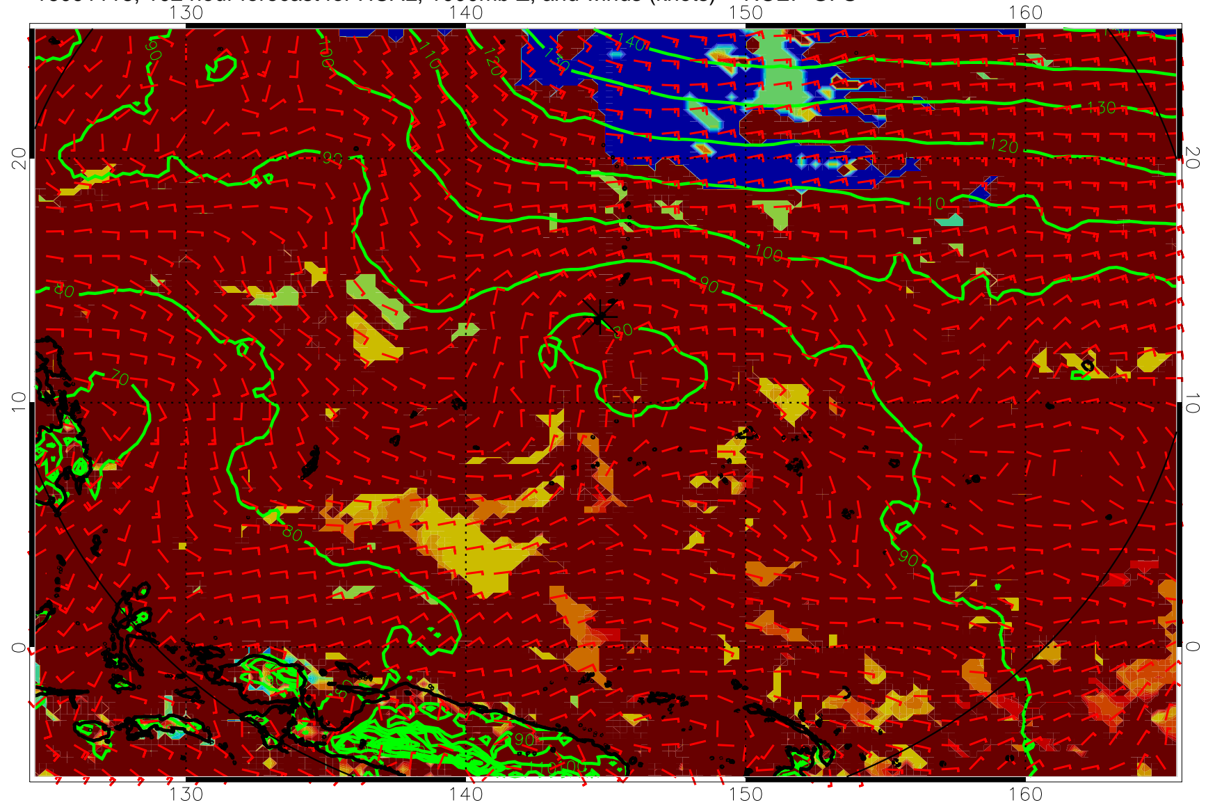
16091118, 102 hour forecast for HCAL, 1000mb Z, and winds (knots) -- NCEP GFS
