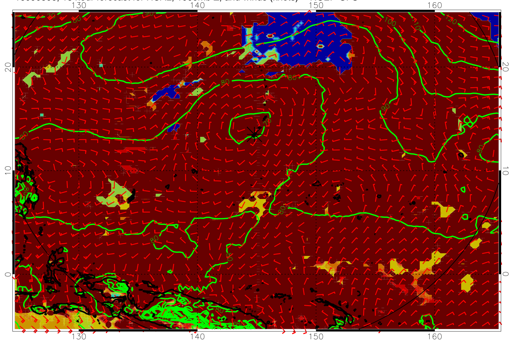
16090806, 18 hour forecast for HCAL, 1000mb Z, and winds (knots) -- NCEP GFS
