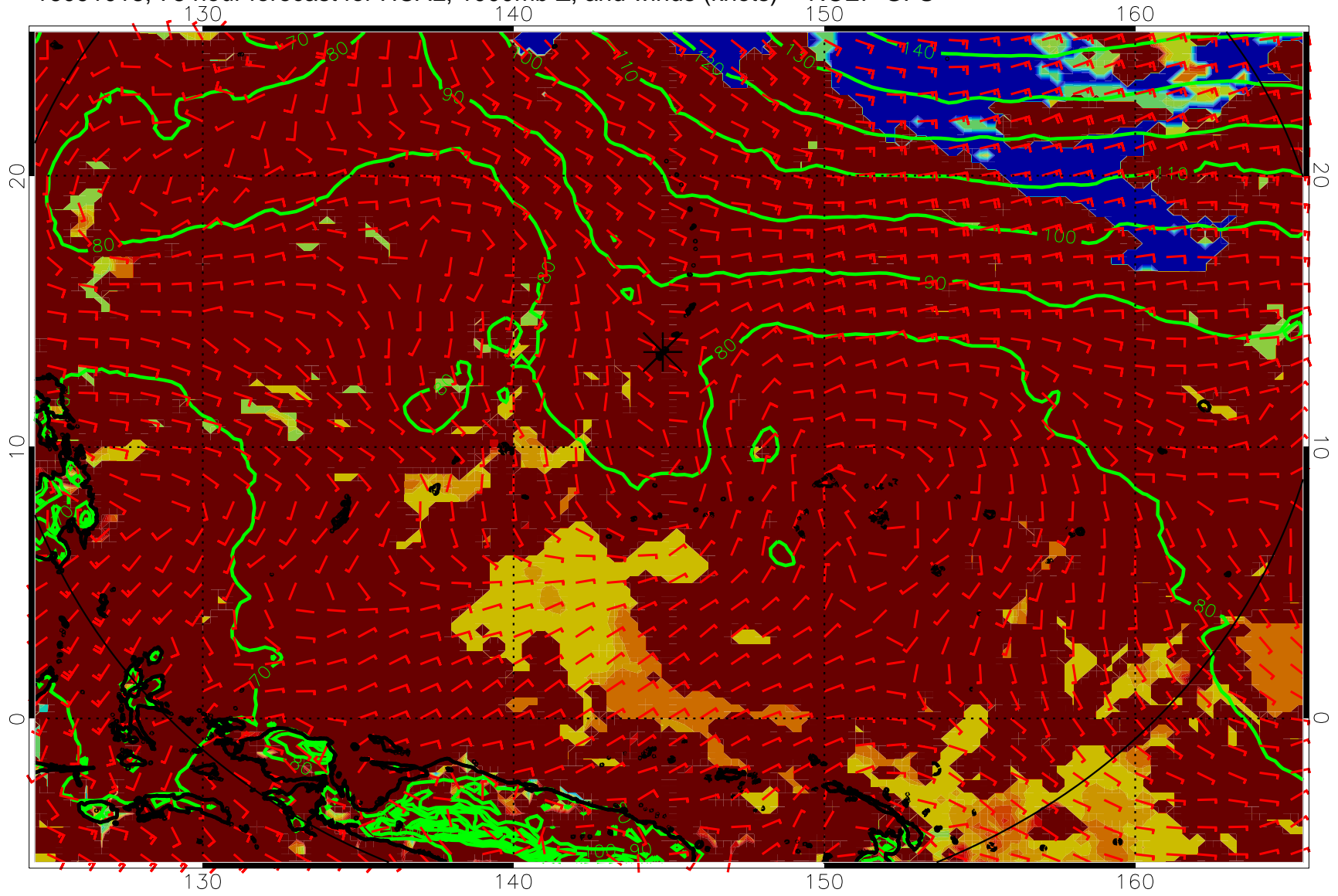
16091018, 78 hour forecast for HCAL, 1000mb Z, and winds (knots) -- NCEP GFS
