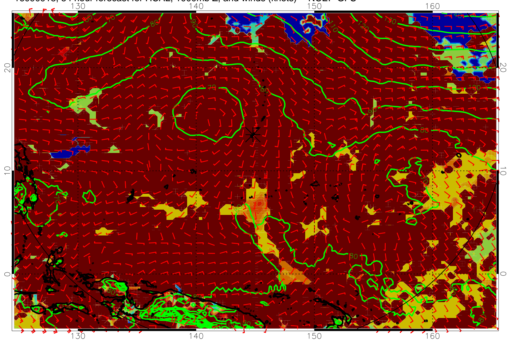
16090918, 54 hour forecast for HCAL, 1000mb Z, and winds (knots) -- NCEP GFS
