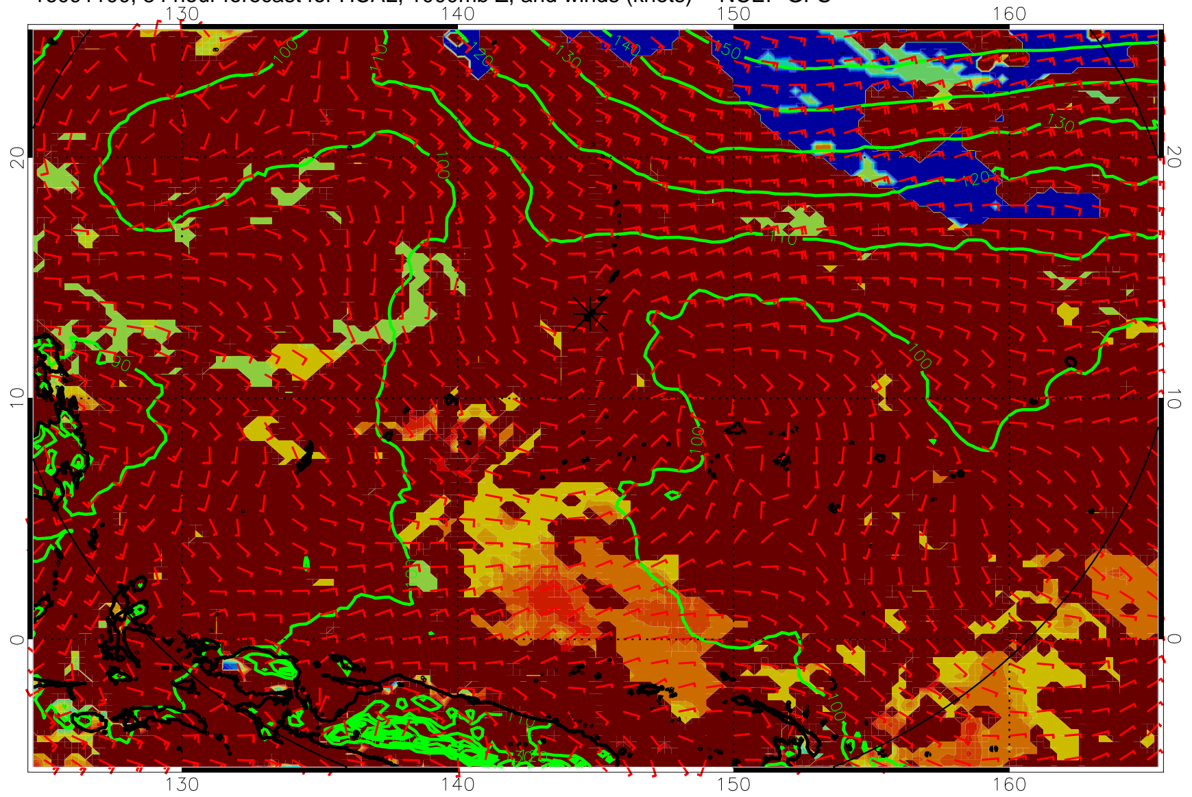
16091100, 84 hour forecast for HCAL, 1000mb Z, and winds (knots) -- NCEP GFS
