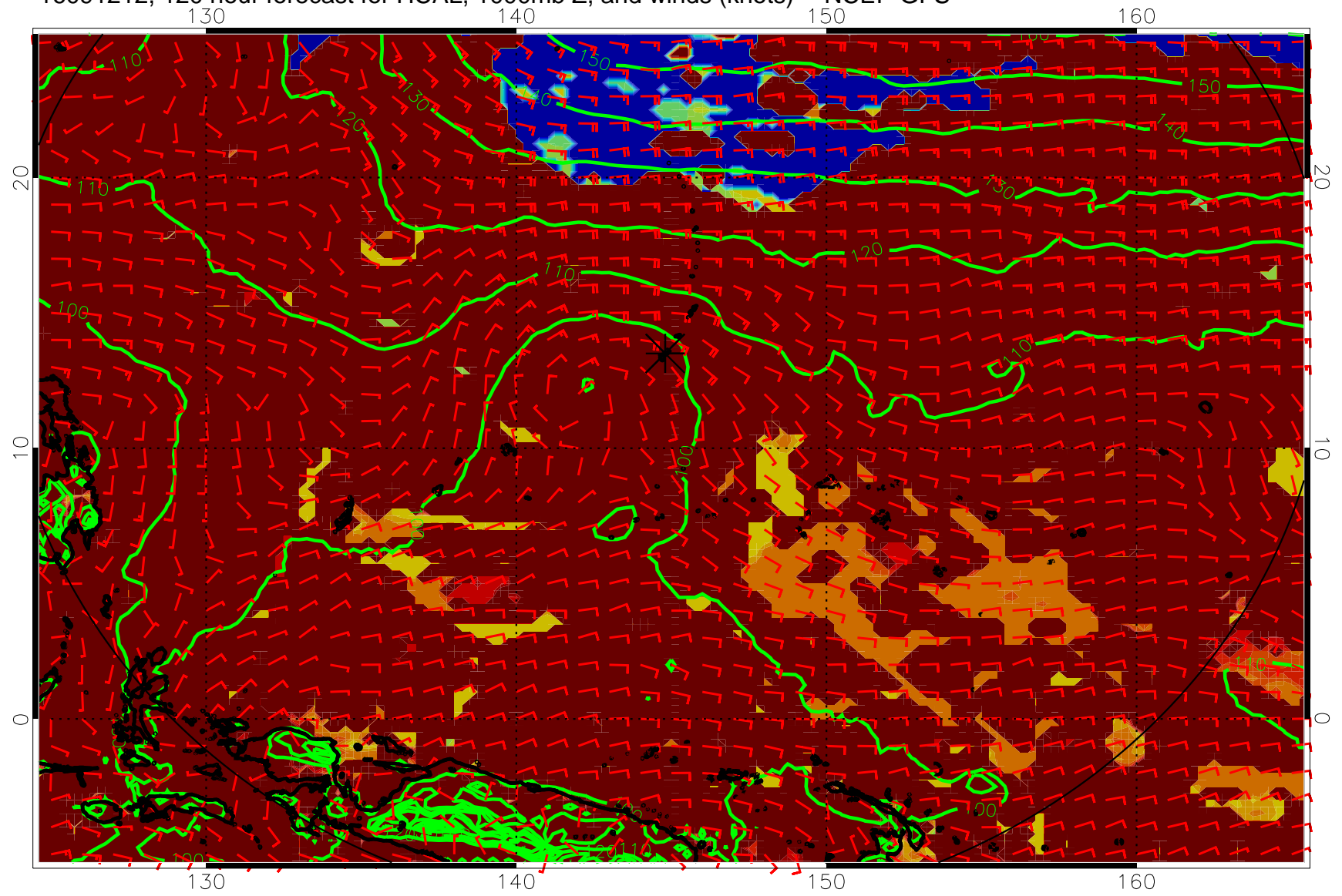
16091212, 120 hour forecast for HCAL, 1000mb Z, and winds (knots) -- NCEP GFS
