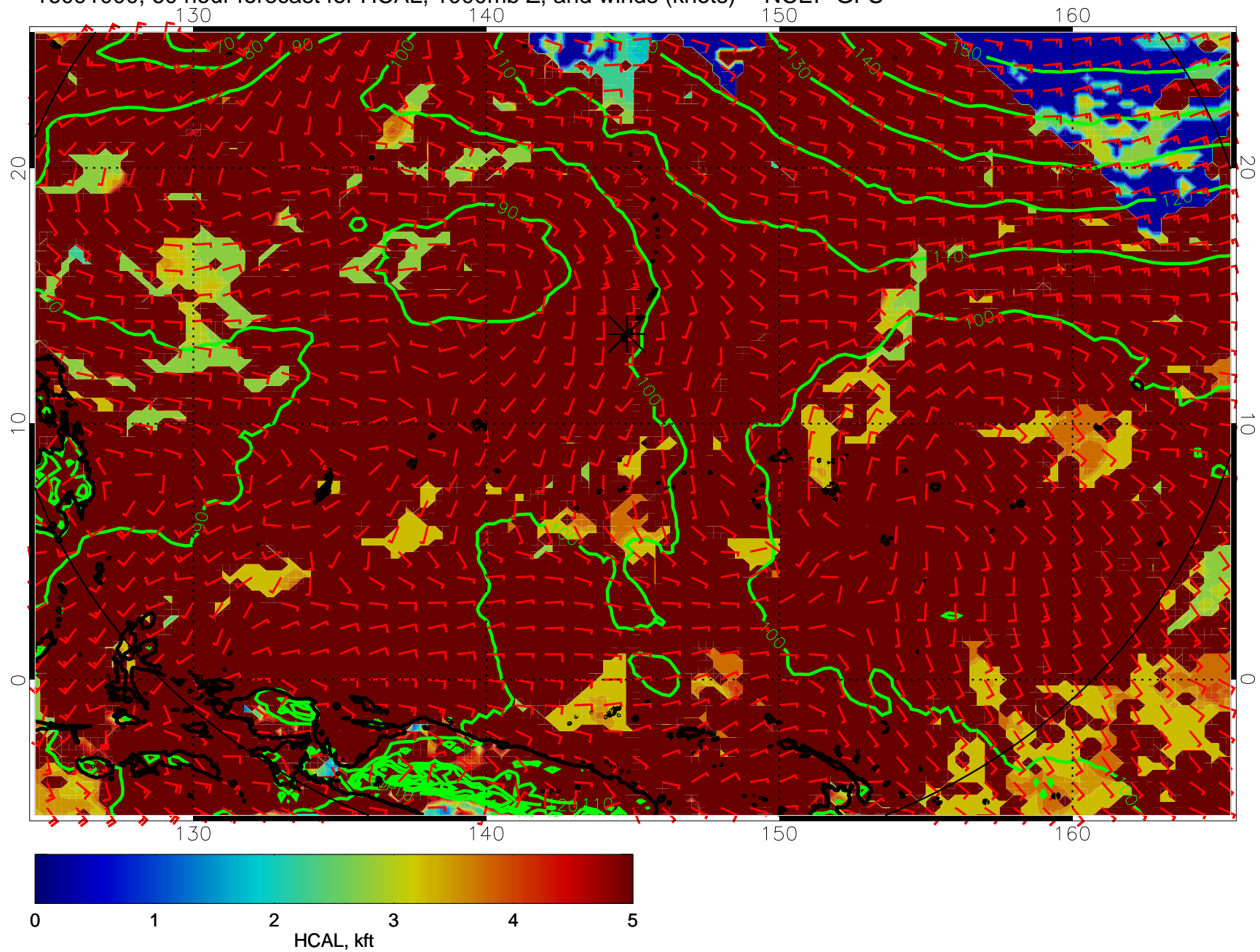
16091000, 60 hour forecast for HCAL, 1000mb Z, and winds (knots) -- NCEP GFS
