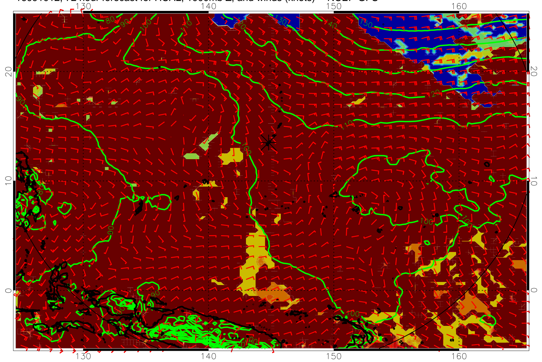
16091012, 72 hour forecast for HCAL, 1000mb Z, and winds (knots) -- NCEP GFS
