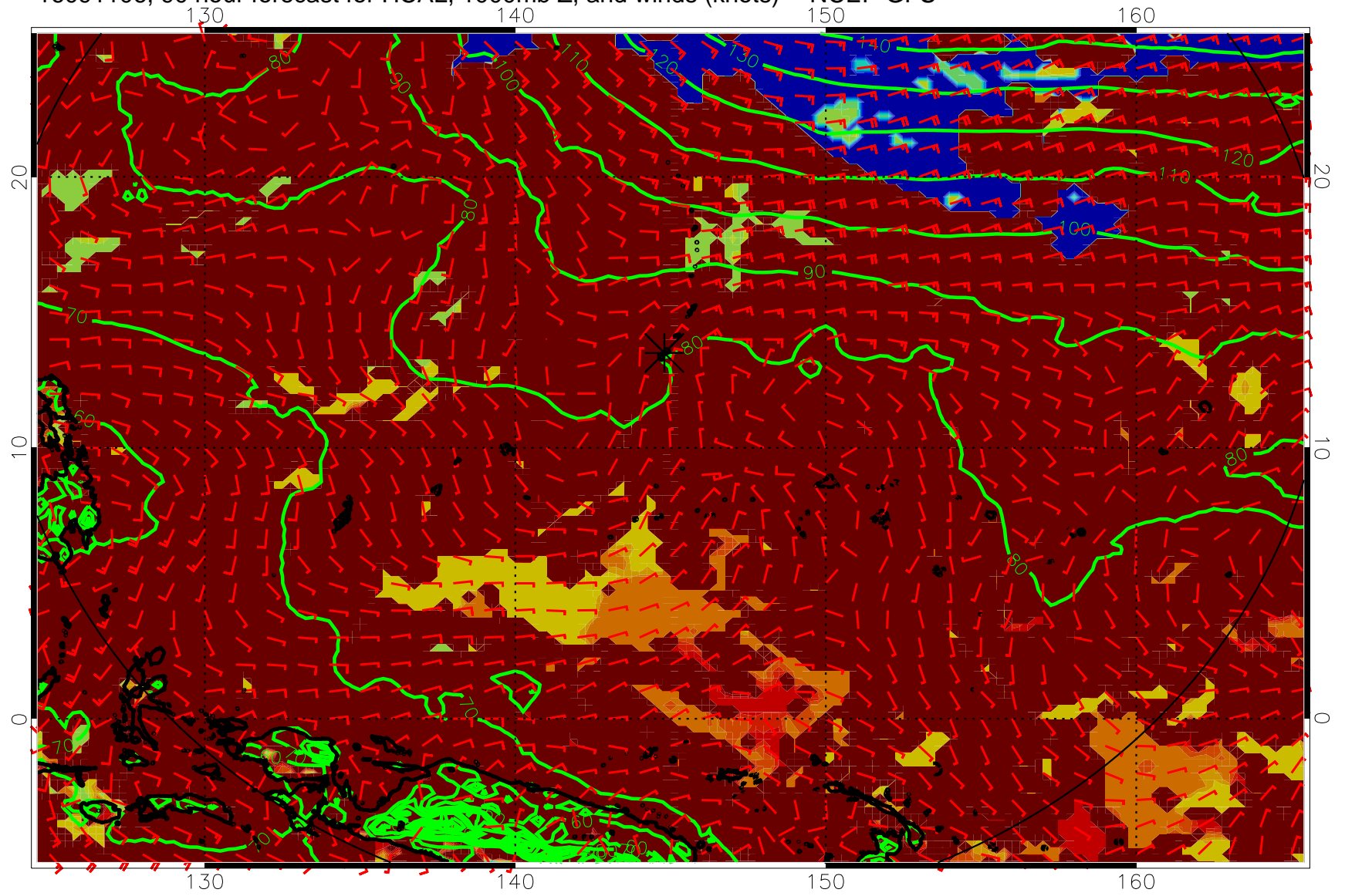
16091106, 90 hour forecast for HCAL, 1000mb Z, and winds (knots) -- NCEP GFS
