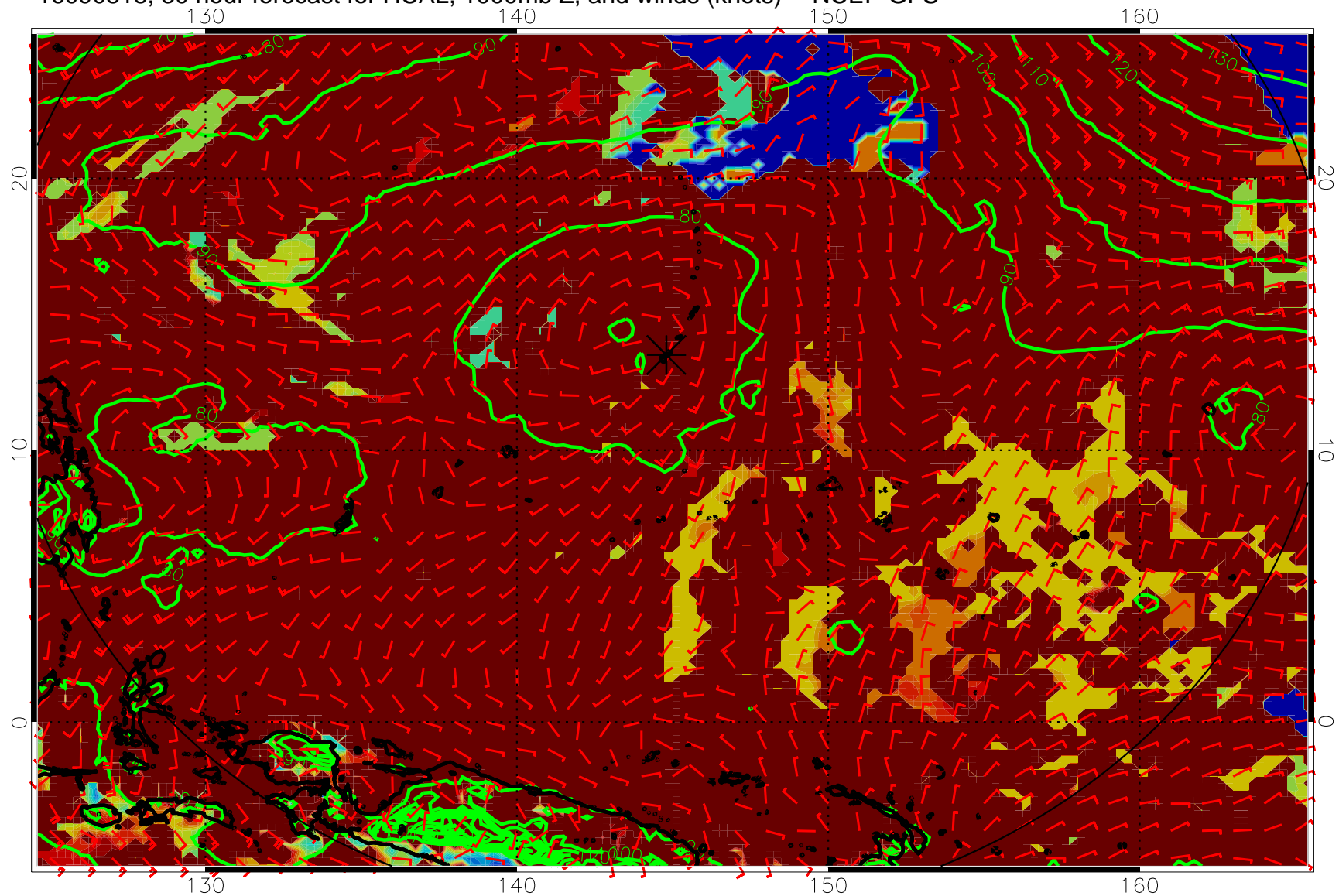
16090818, 30 hour forecast for HCAL, 1000mb Z, and winds (knots) -- NCEP GFS
