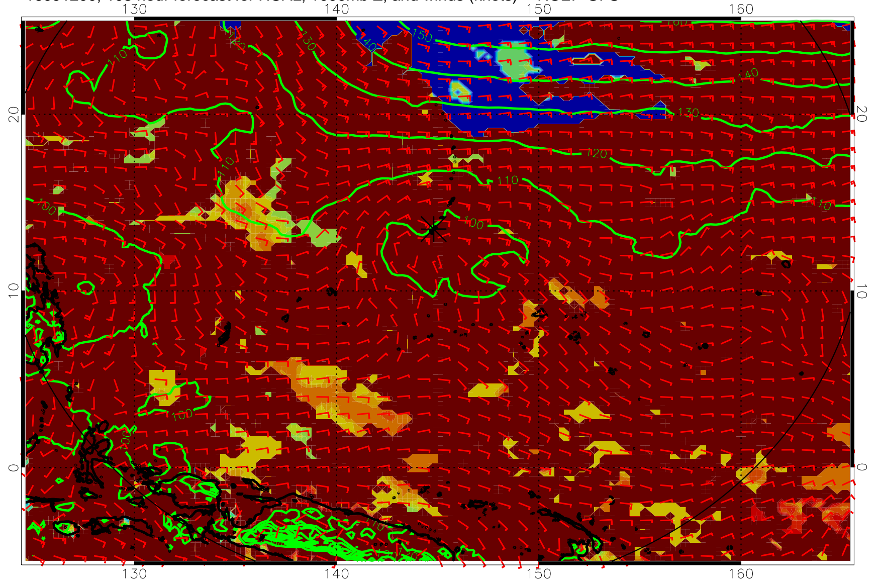
16091200, 108 hour forecast for HCAL, 1000mb Z, and winds (knots) -- NCEP GFS
