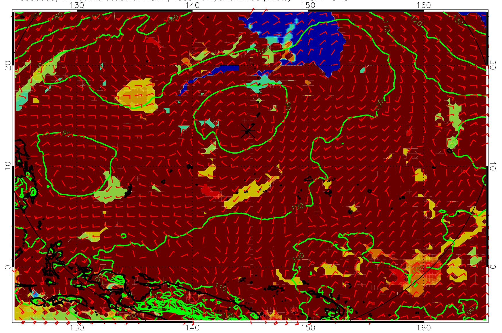
16090800, 12 hour forecast for HCAL, 1000mb Z, and winds (knots) -- NCEP GFS
