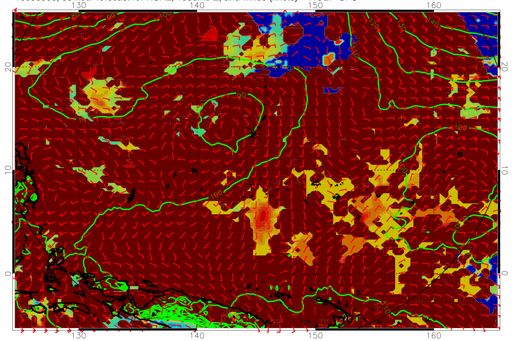
16090900, 36 hour forecast for HCAL, 1000mb Z, and winds (knots) -- NCEP GFS
