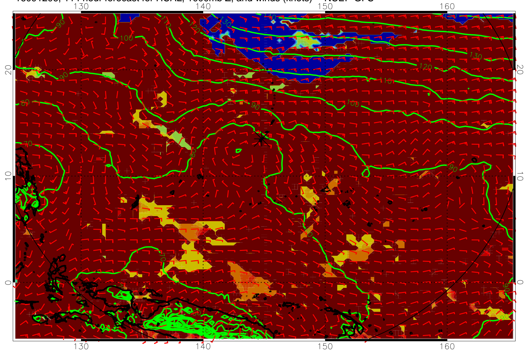
16091206, 114 hour forecast for HCAL, 1000mb Z, and winds (knots) -- NCEP GFS
