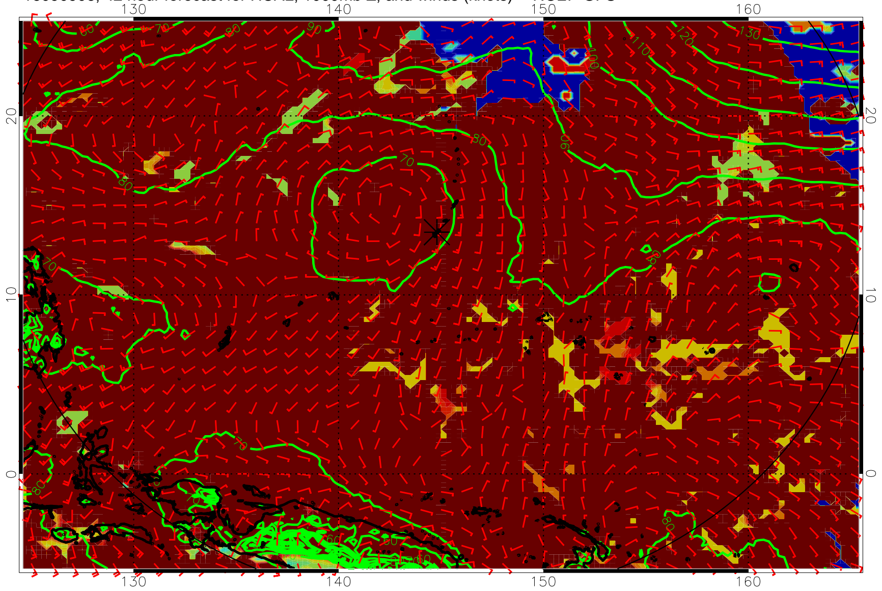
16090906, 42 hour forecast for HCAL, 1000mb Z, and winds (knots) -- NCEP GFS
