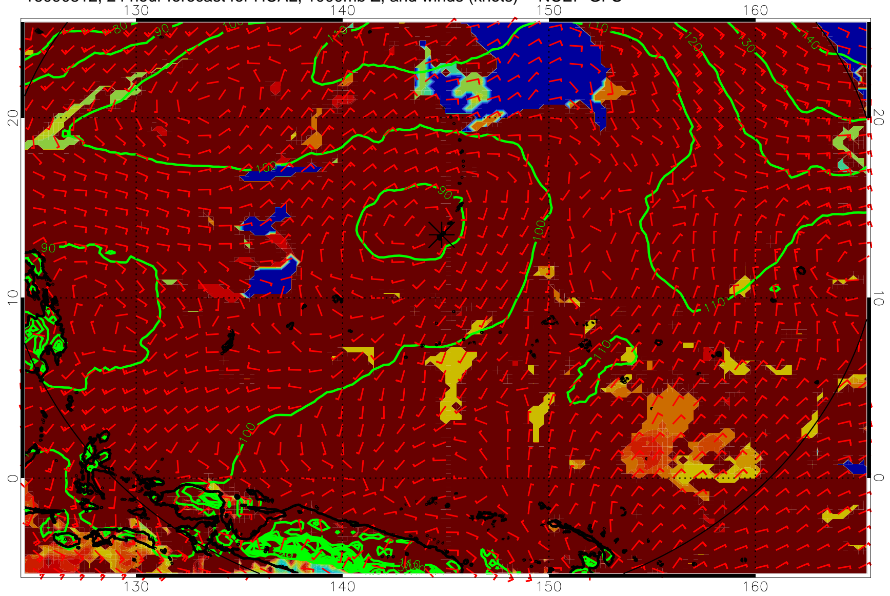
16090812, 24 hour forecast for HCAL, 1000mb Z, and winds (knots) -- NCEP GFS
