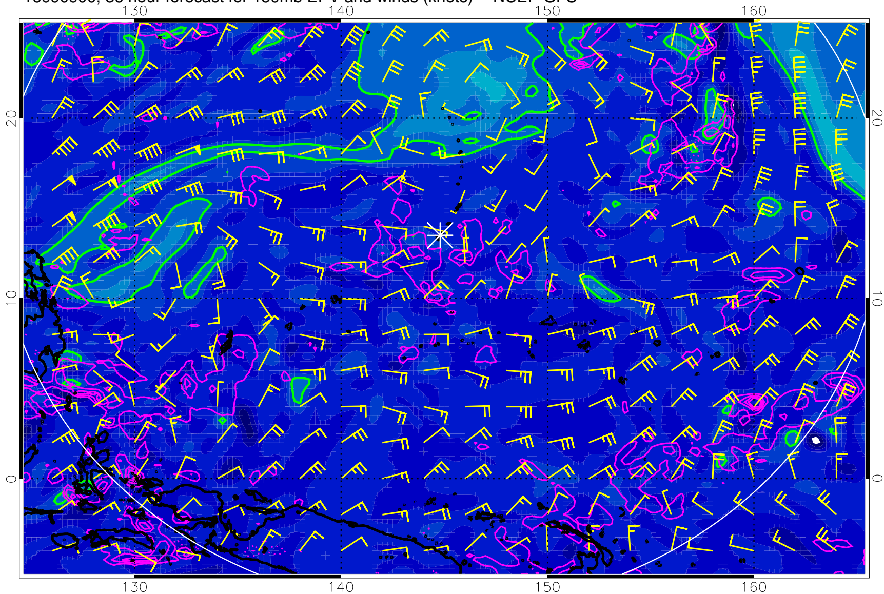
16090900, 36 hour forecast for 150mb EPV and winds (knots) -- NCEP GFS
