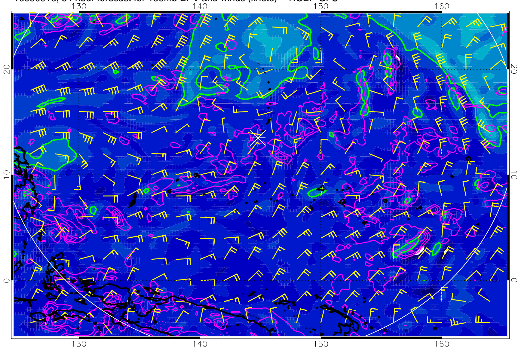
16090918, 54 hour forecast for 150mb EPV and winds (knots) -- NCEP GFS
