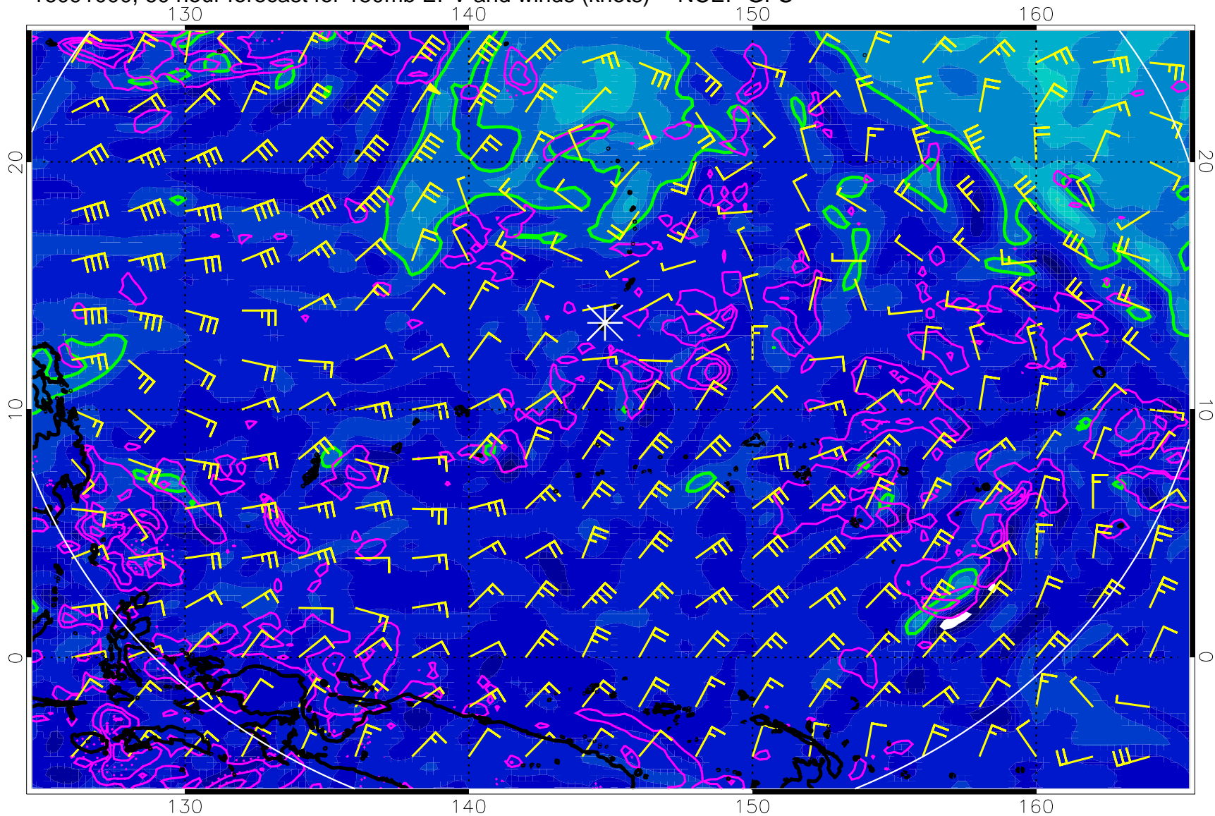
16091000, 60 hour forecast for 150mb EPV and winds (knots) -- NCEP GFS
