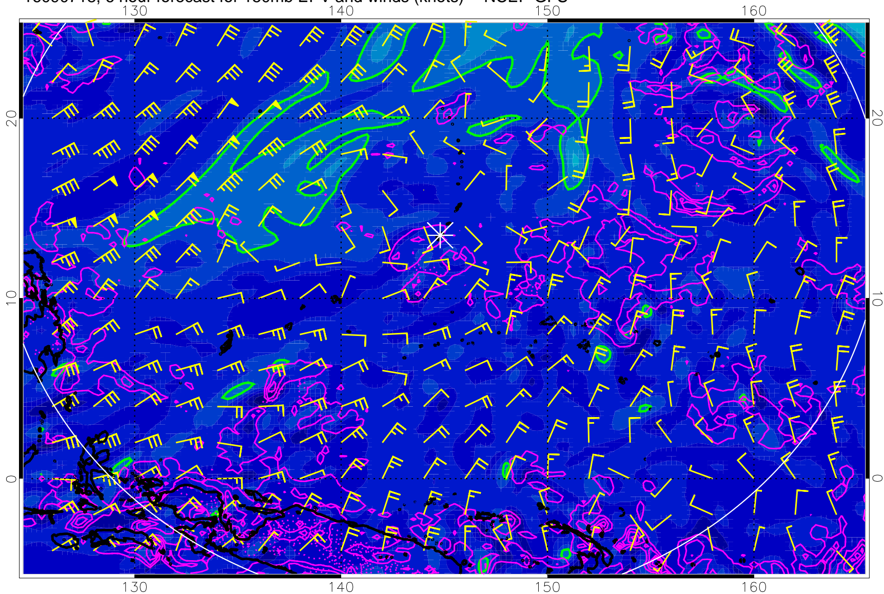
16090718, 6 hour forecast for 150mb EPV and winds (knots) -- NCEP GFS
