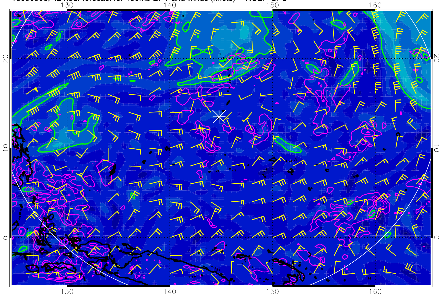
16090906, 42 hour forecast for 150mb EPV and winds (knots) -- NCEP GFS
