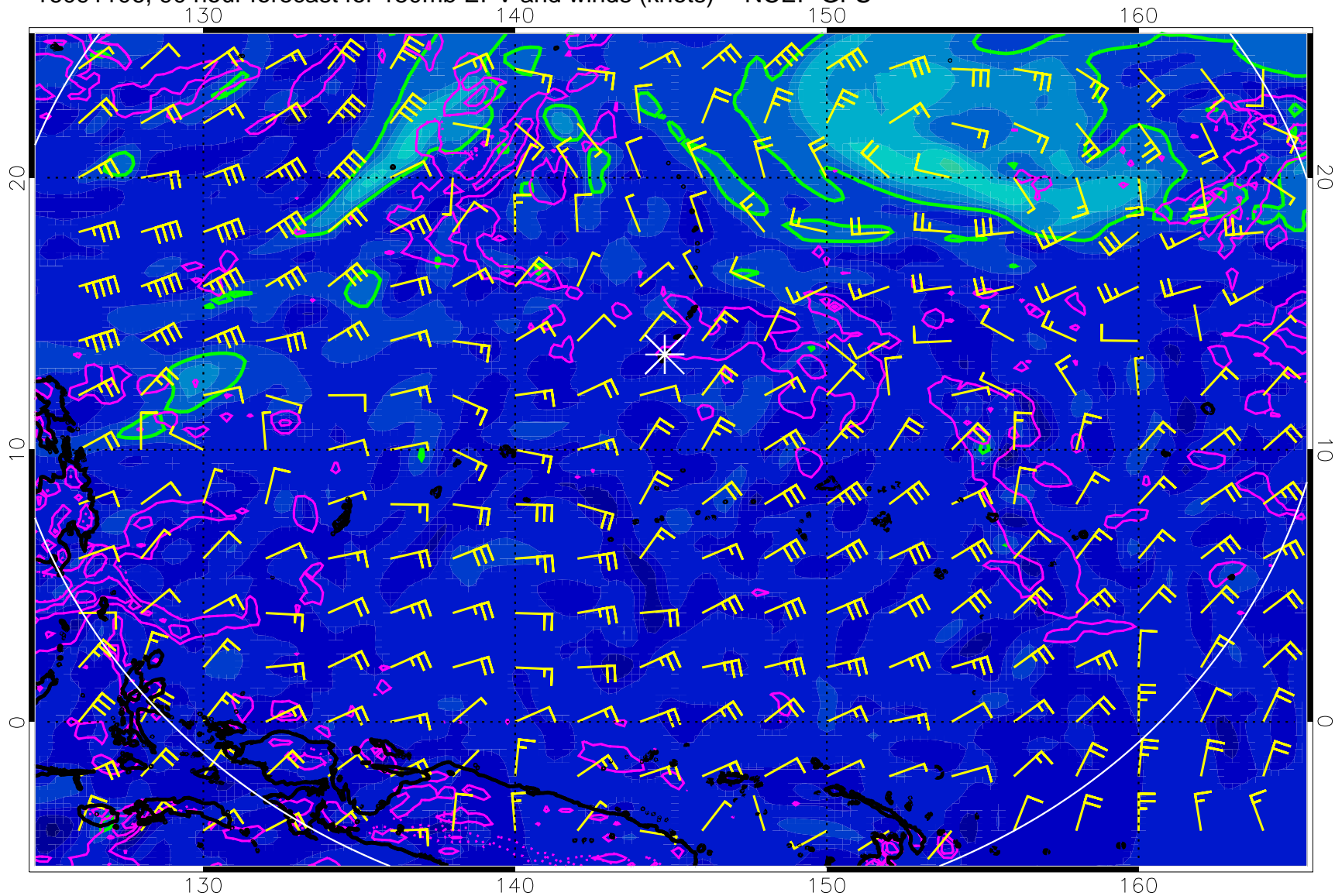
16091106, 90 hour forecast for 150mb EPV and winds (knots) -- NCEP GFS
