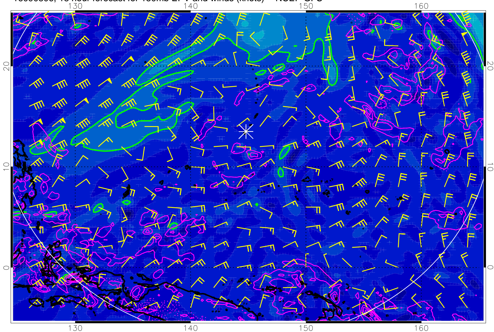
16090806, 18 hour forecast for 150mb EPV and winds (knots) -- NCEP GFS
