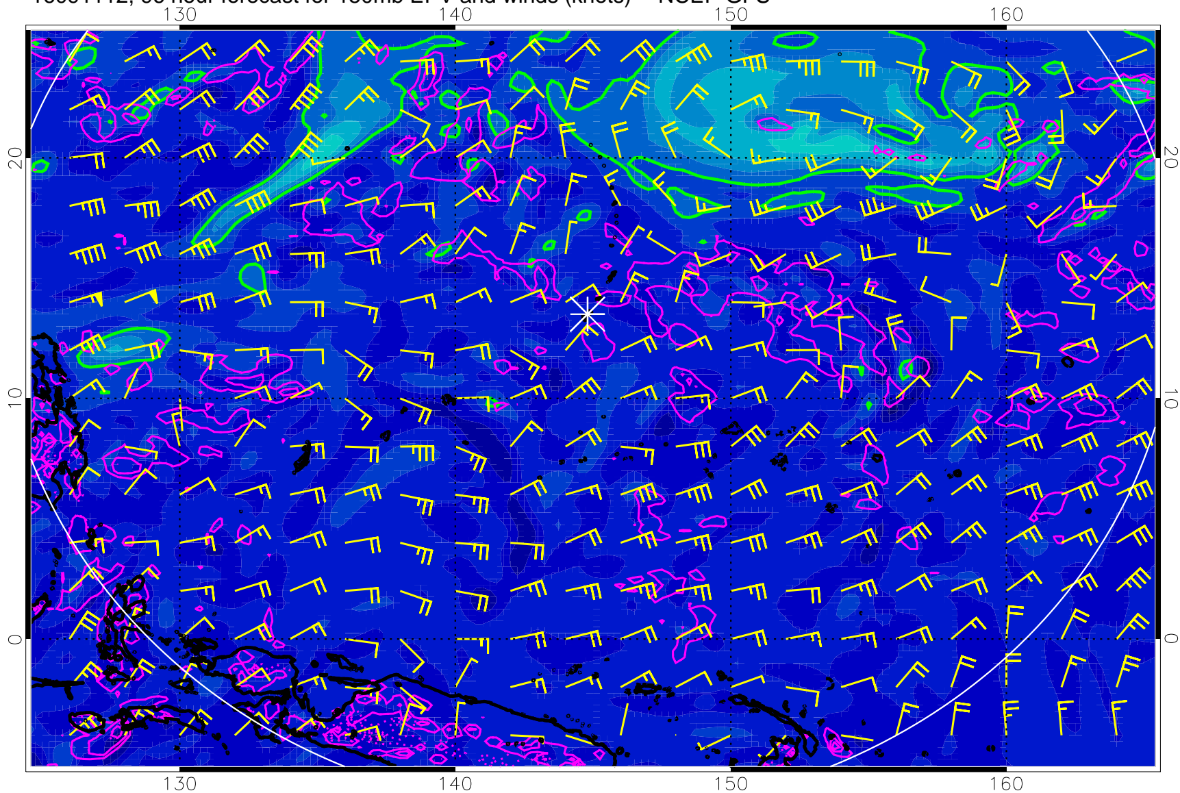
16091112, 96 hour forecast for 150mb EPV and winds (knots) -- NCEP GFS
