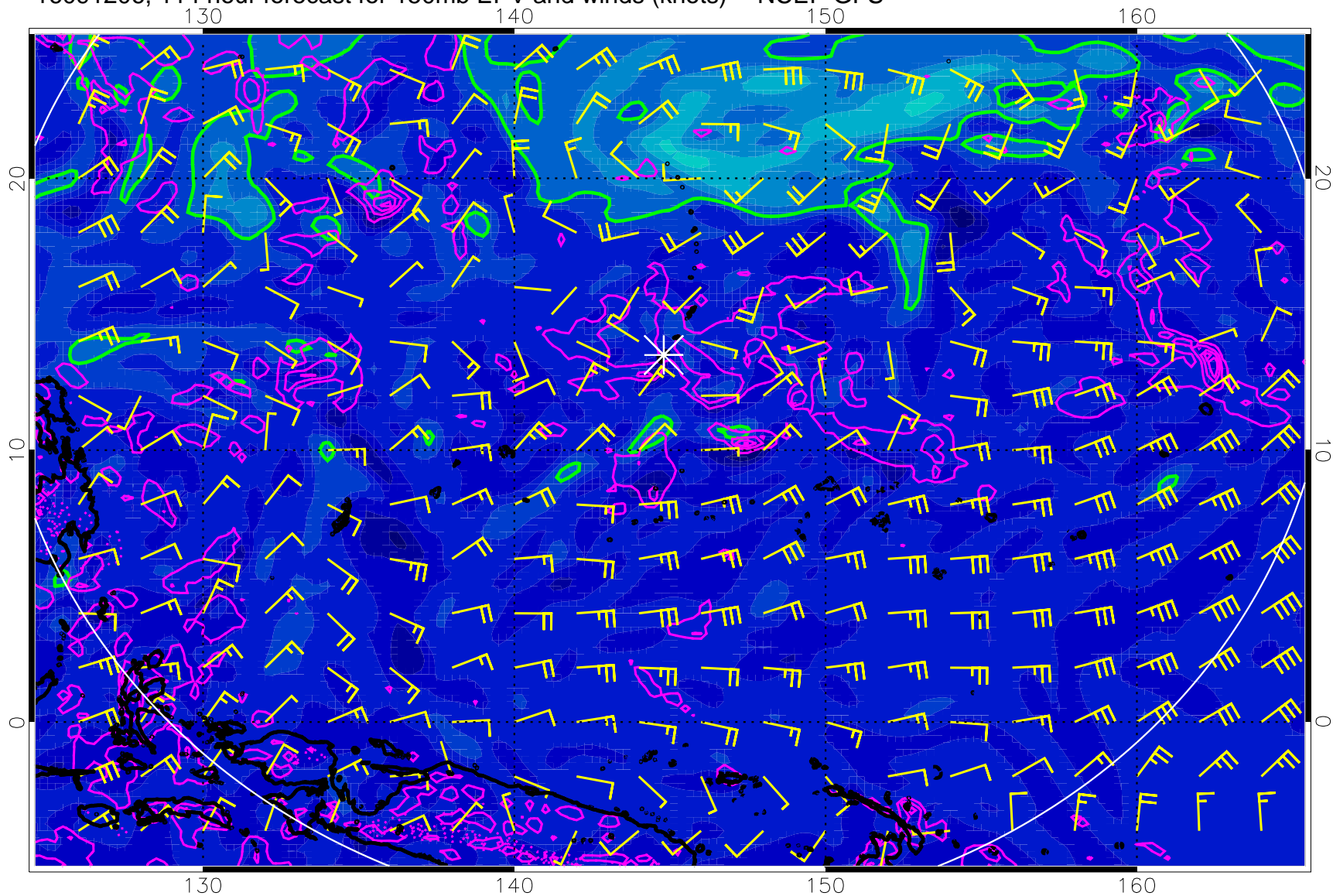
16091206, 114 hour forecast for 150mb EPV and winds (knots) -- NCEP GFS
