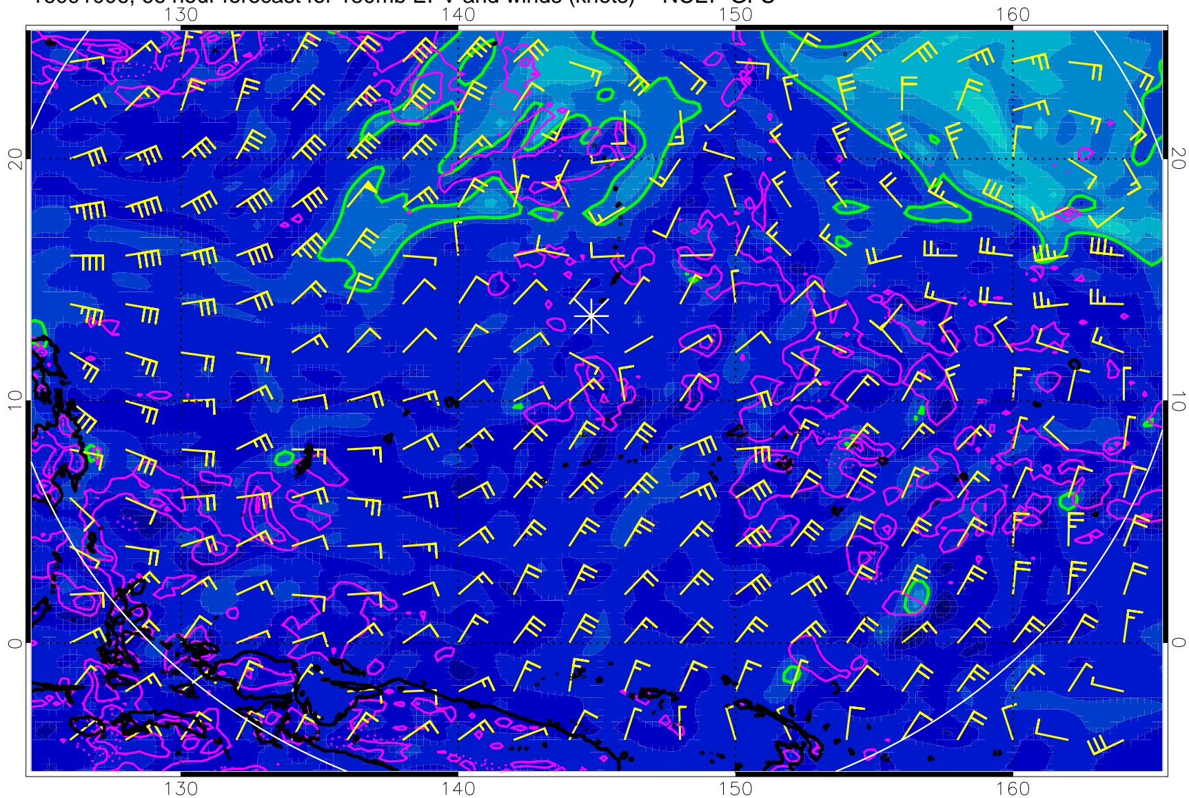
16091006, 66 hour forecast for 150mb EPV and winds (knots) -- NCEP GFS
