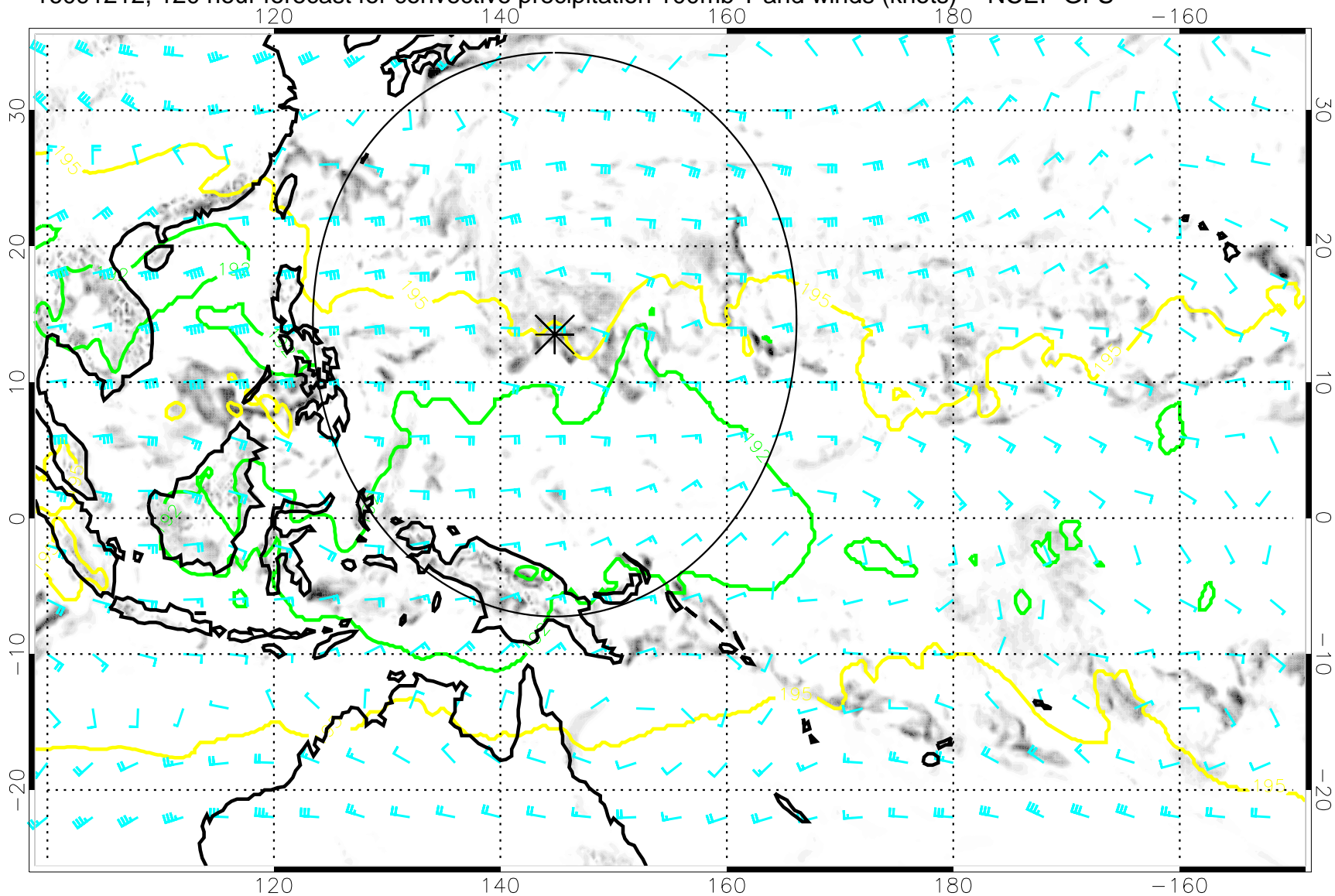
16091212, 120 hour forecast for convective precipitation 100mb T and winds (knots) -- NCEP GFS
