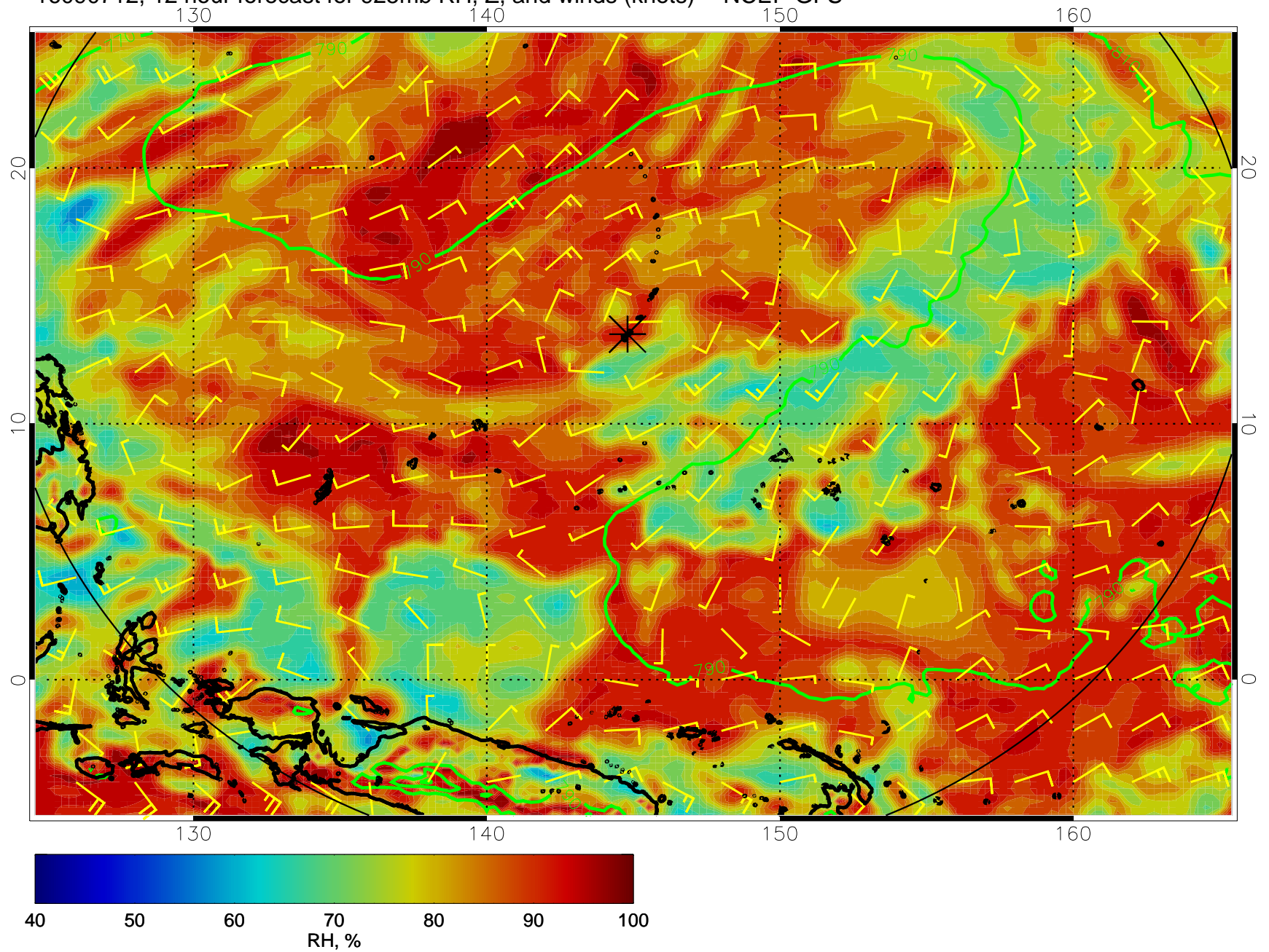
16090712, 12 hour forecast for 925mb RH, Z, and winds (knots) -- NCEP GFS
