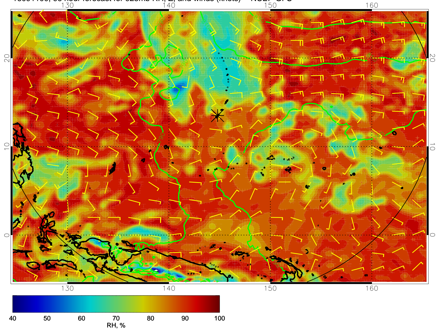
16091100, 96 hour forecast for 925mb RH, Z, and winds (knots) -- NCEP GFS
