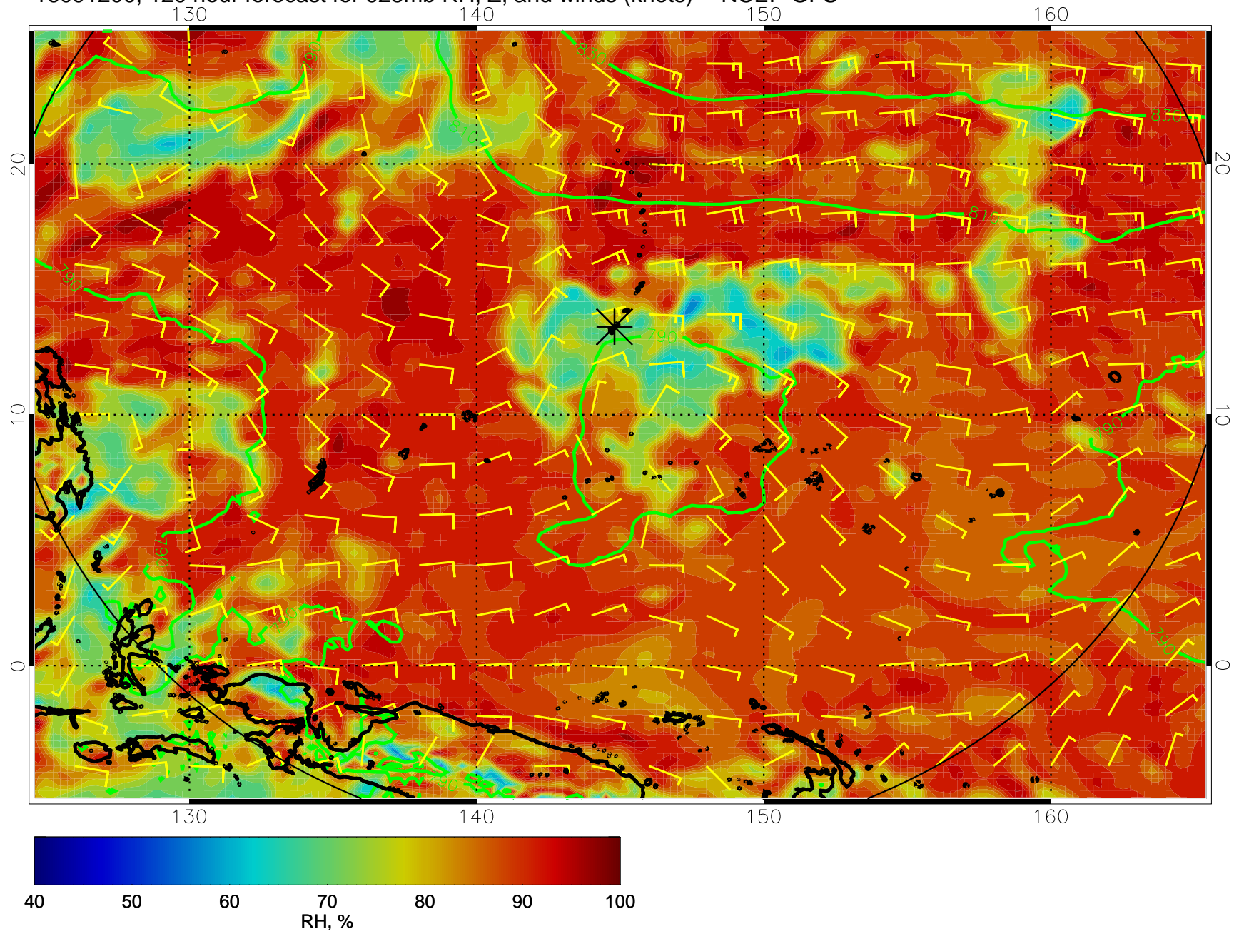
16091200, 120 hour forecast for 925mb RH, Z, and winds (knots) -- NCEP GFS
