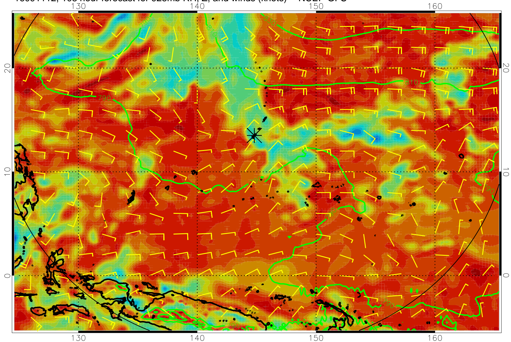
16091112, 108 hour forecast for 925mb RH, Z, and winds (knots) -- NCEP GFS
