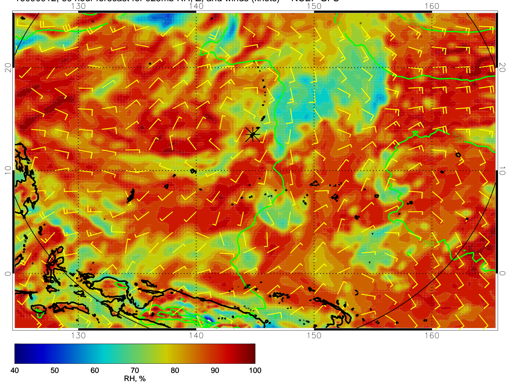
16090912, 60 hour forecast for 925mb RH, Z, and winds (knots) -- NCEP GFS
