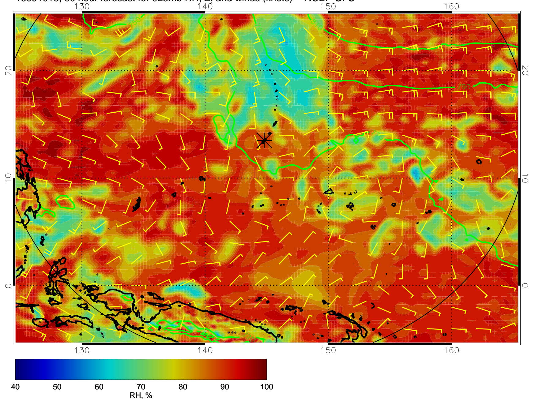
16091018, 90 hour forecast for 925mb RH, Z, and winds (knots) -- NCEP GFS
