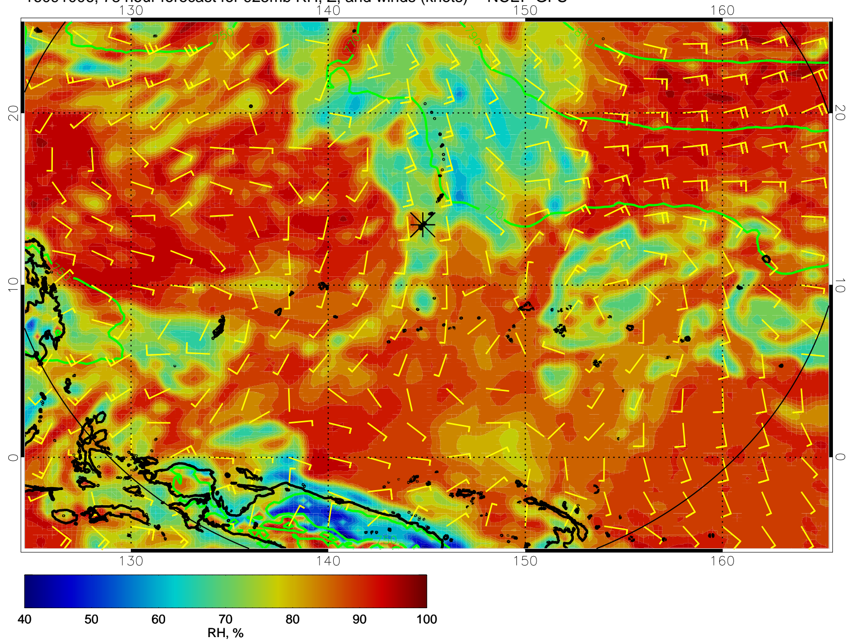
16091006, 78 hour forecast for 925mb RH, Z, and winds (knots) -- NCEP GFS
