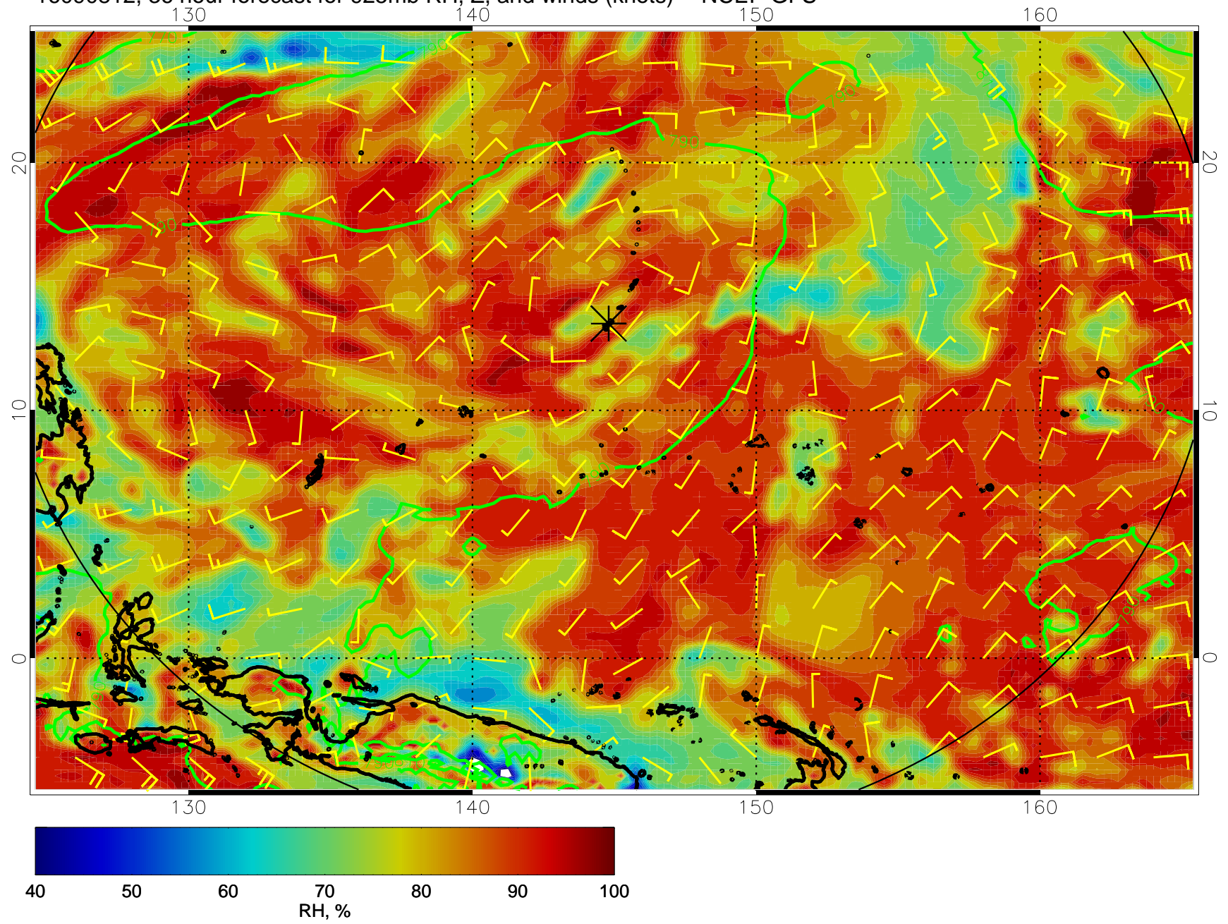
16090812, 36 hour forecast for 925mb RH, Z, and winds (knots) -- NCEP GFS
