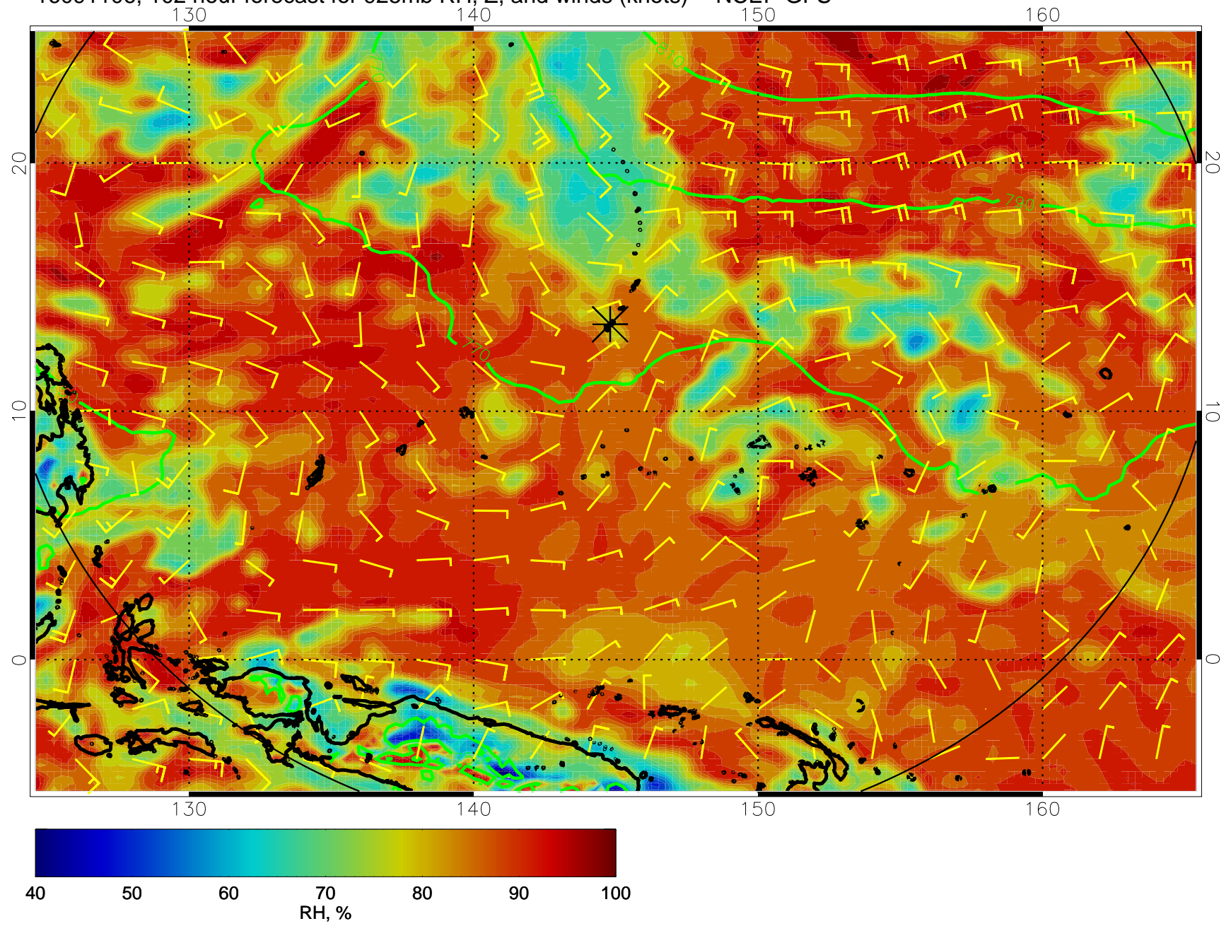
16091106, 102 hour forecast for 925mb RH, Z, and winds (knots) -- NCEP GFS
