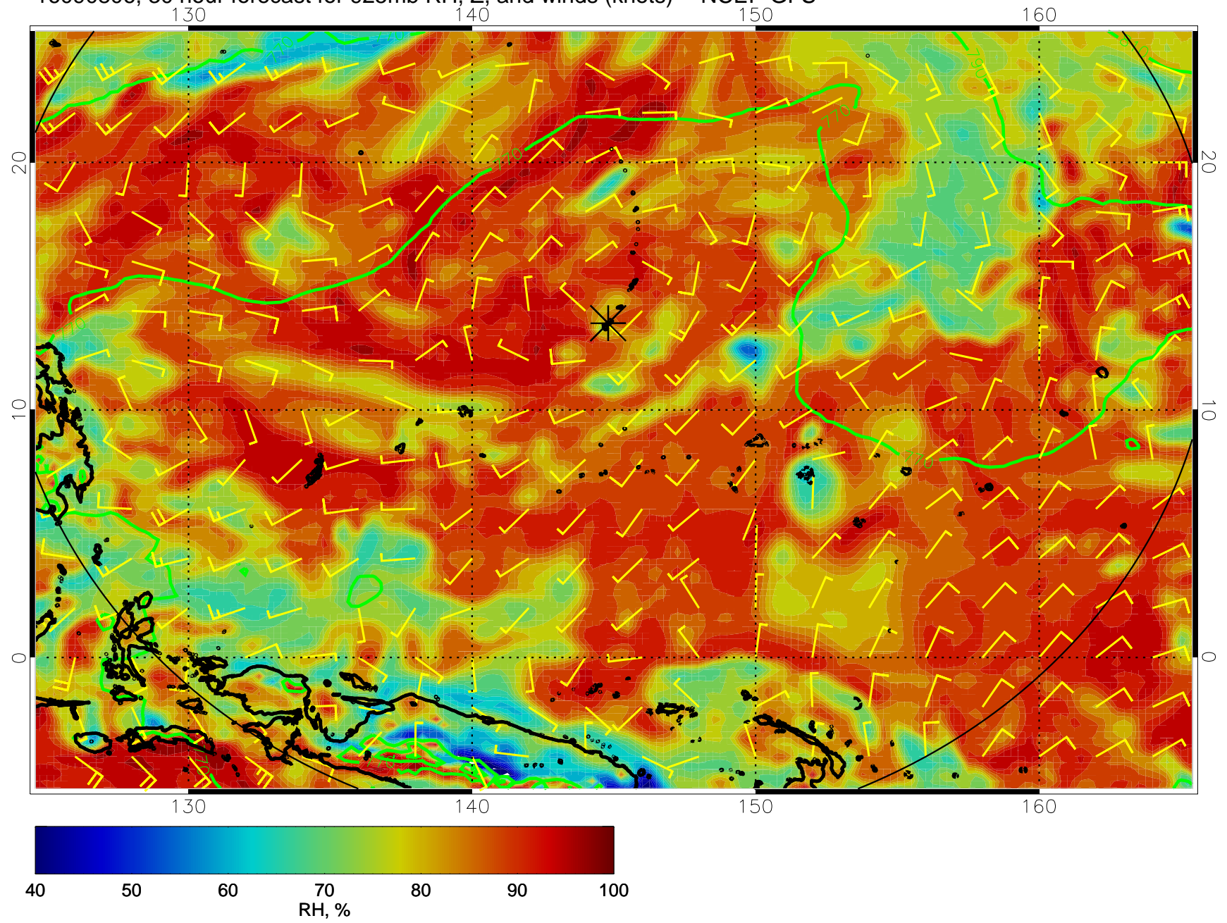
16090806, 30 hour forecast for 925mb RH, Z, and winds (knots) -- NCEP GFS
