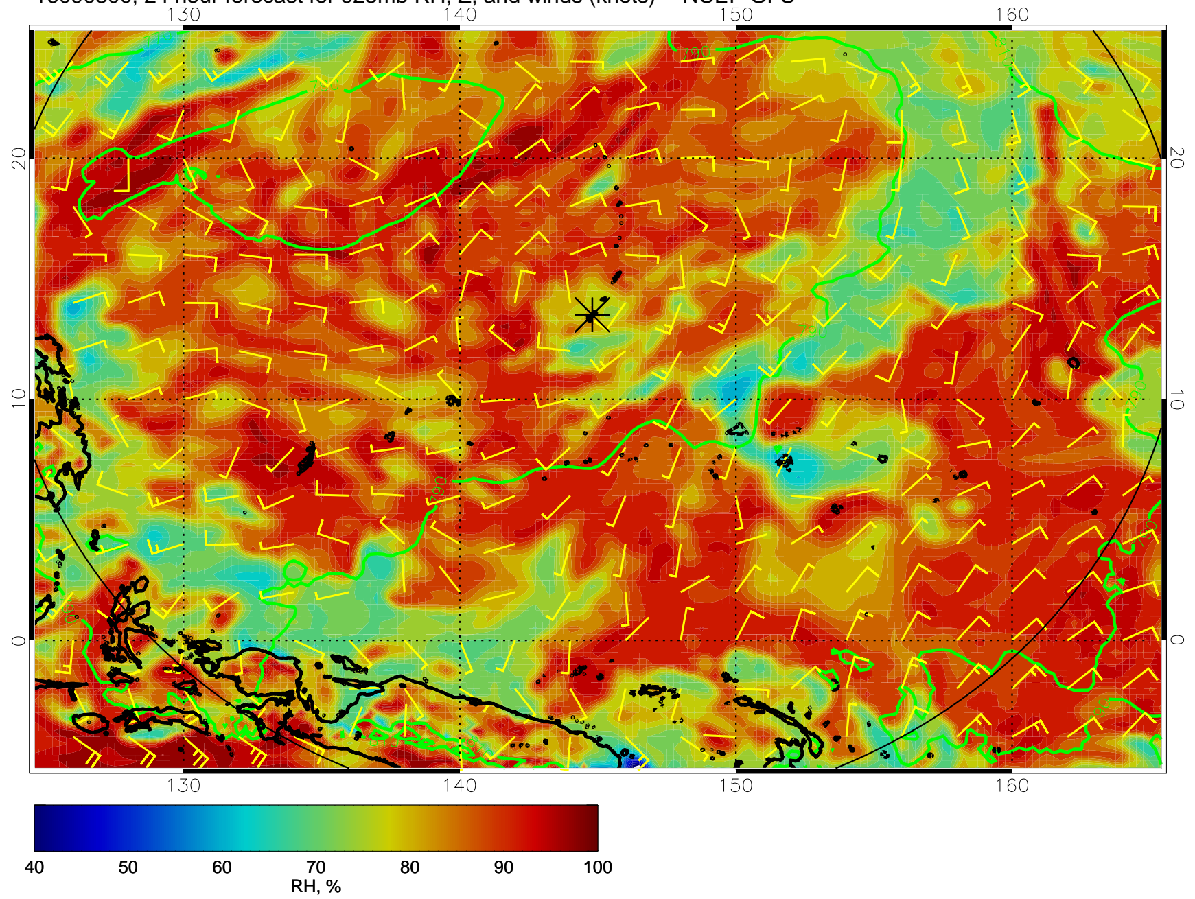
16090800, 24 hour forecast for 925mb RH, Z, and winds (knots) -- NCEP GFS
