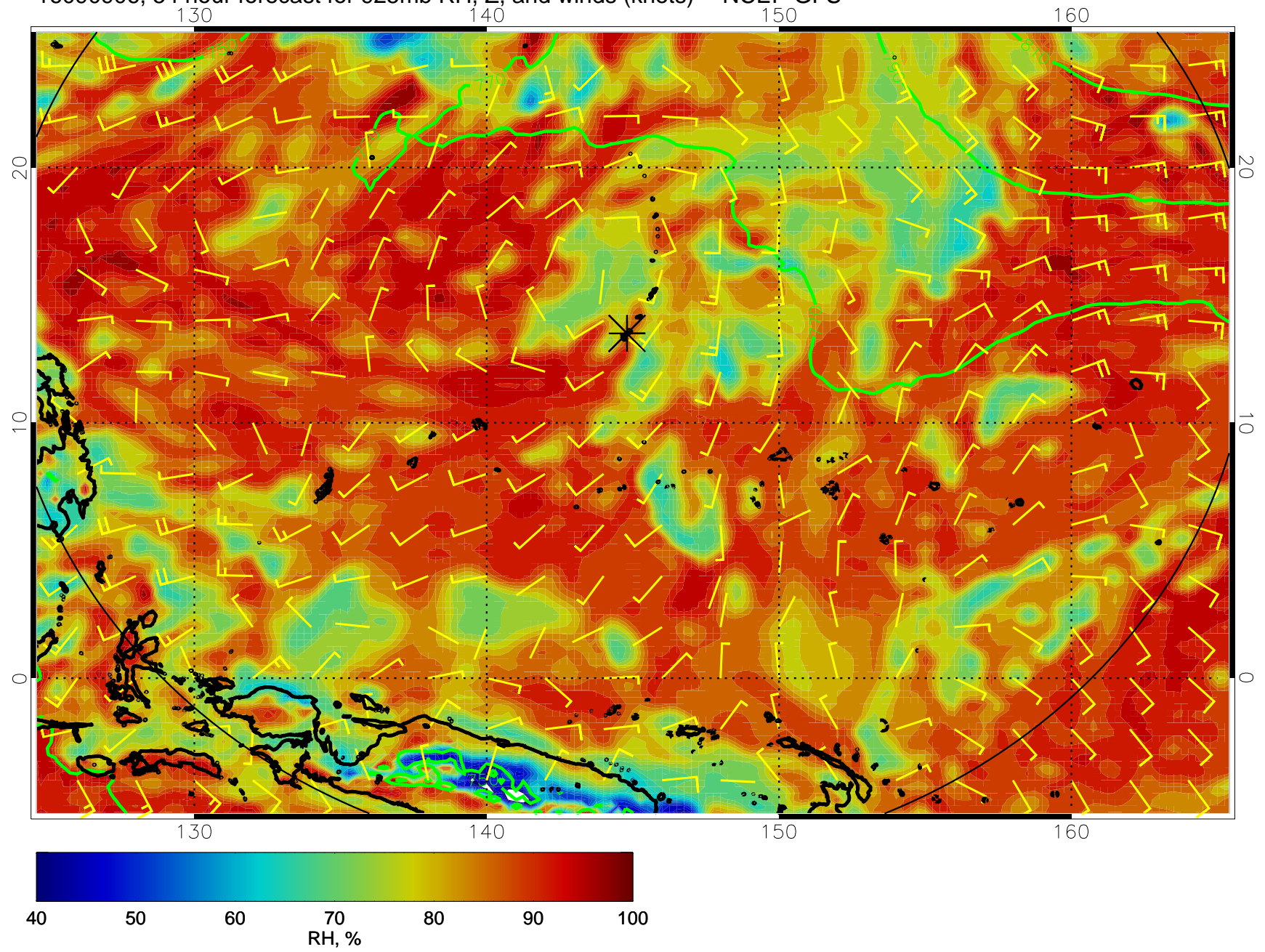
16090906, 54 hour forecast for 925mb RH, Z, and winds (knots) -- NCEP GFS
