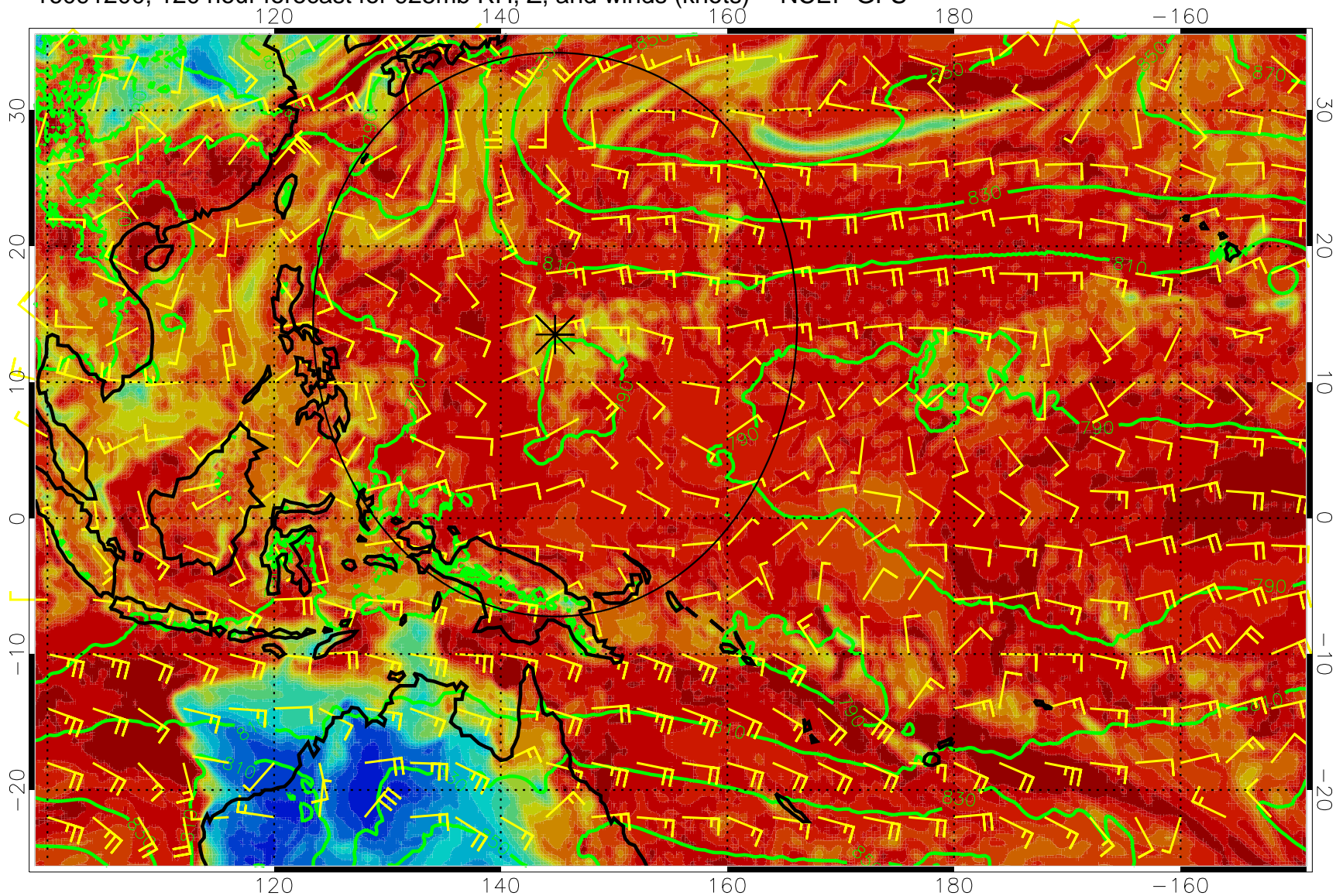
16091200, 120 hour forecast for 925mb RH, Z, and winds (knots) -- NCEP GFS
