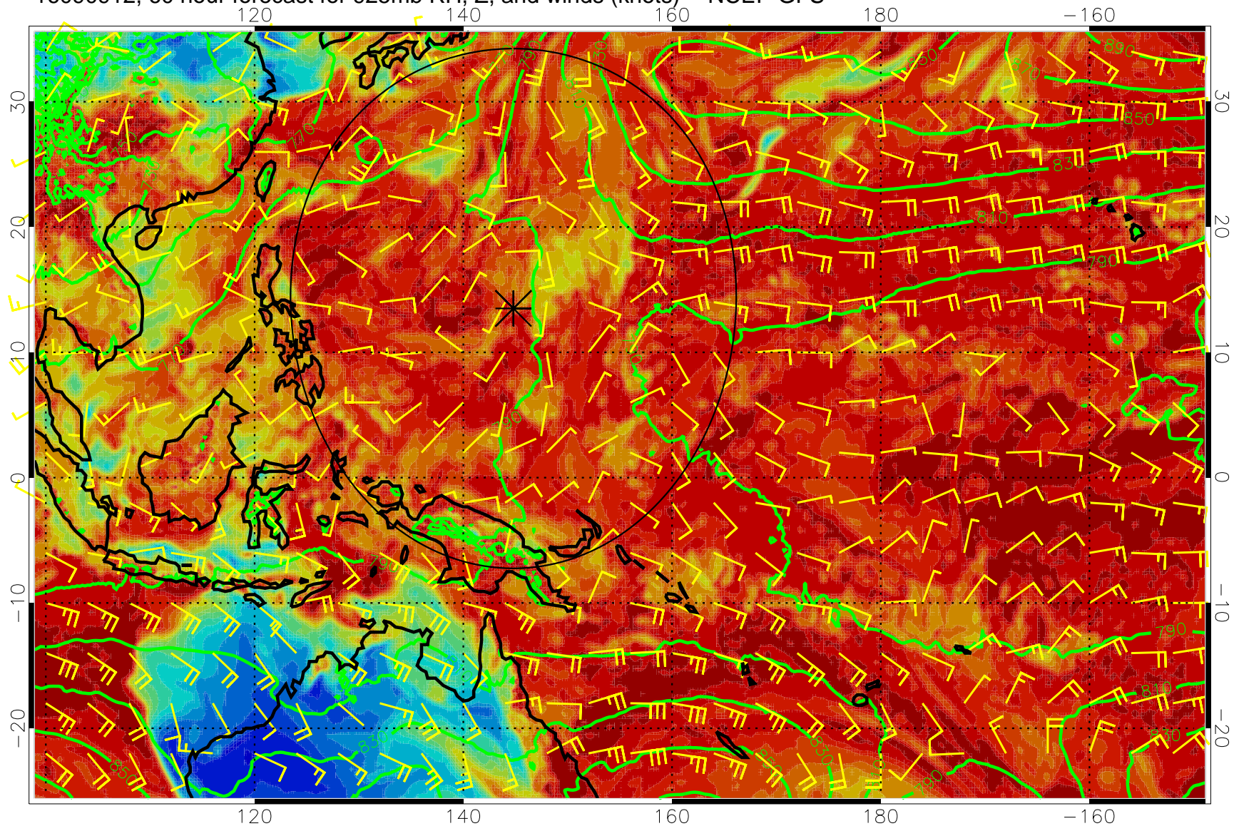
16090912, 60 hour forecast for 925mb RH, Z, and winds (knots) -- NCEP GFS
