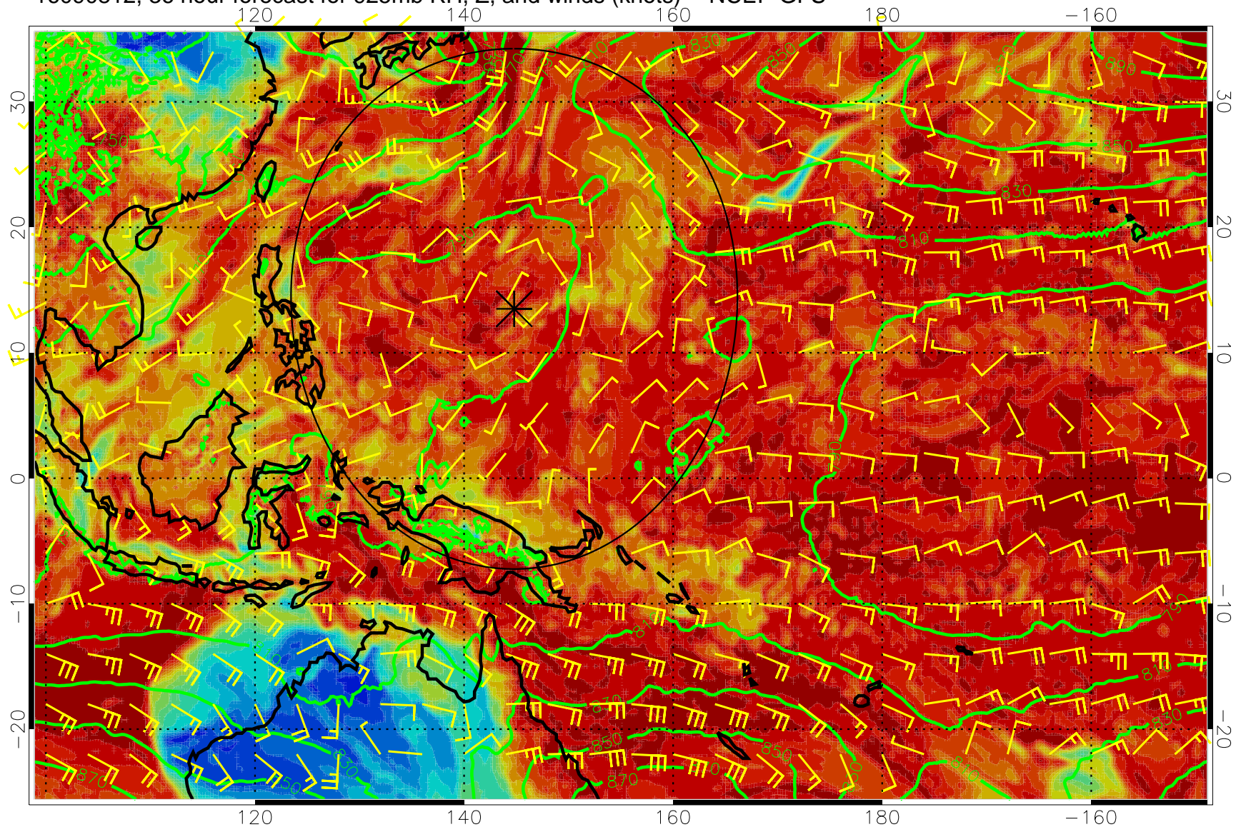
16090812, 36 hour forecast for 925mb RH, Z, and winds (knots) -- NCEP GFS
