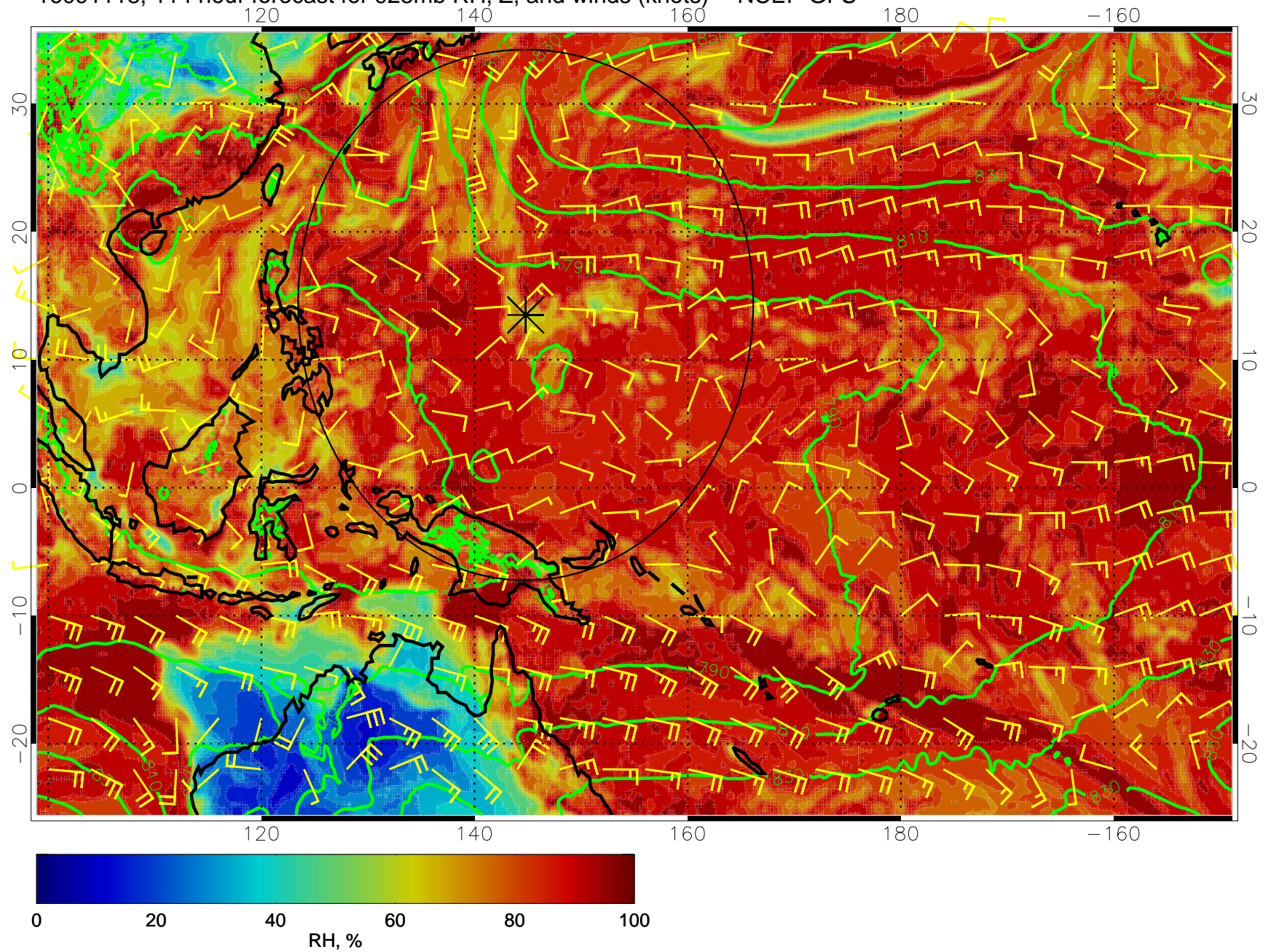
16091118, 114 hour forecast for 925mb RH, Z, and winds (knots) -- NCEP GFS
