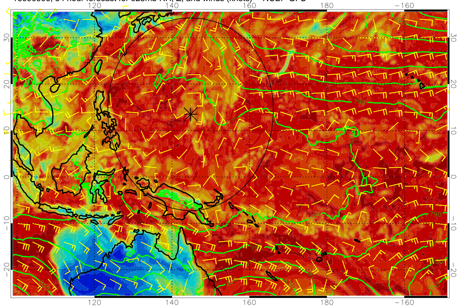
16090906, 54 hour forecast for 925mb RH, Z, and winds (knots) -- NCEP GFS
