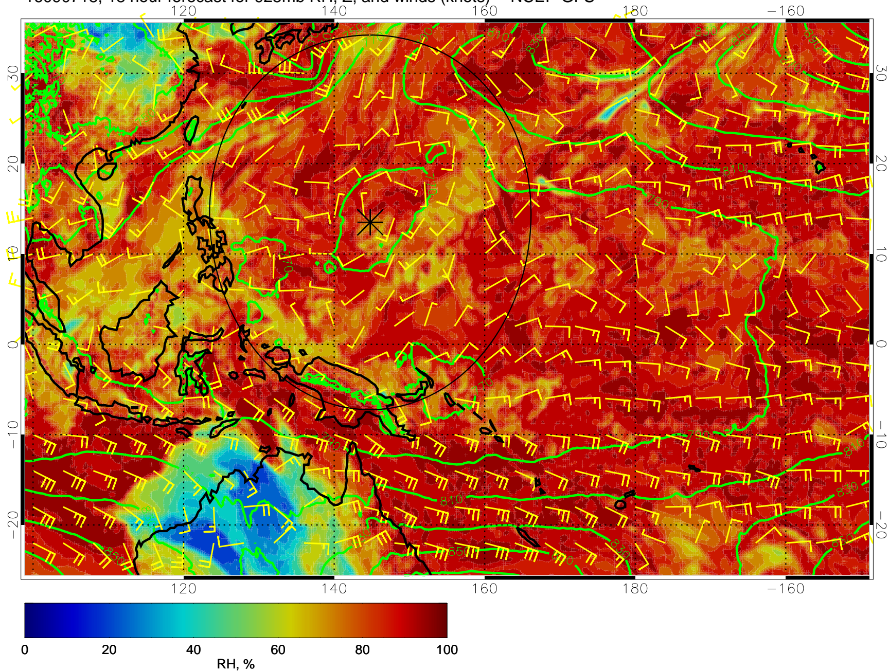
16090718, 18 hour forecast for 925mb RH, Z, and winds (knots) -- NCEP GFS
