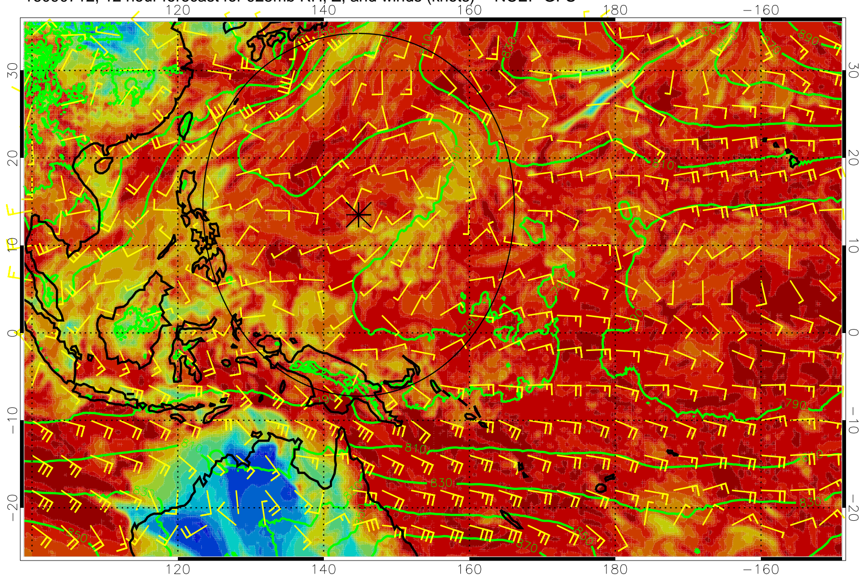
16090712, 12 hour forecast for 925mb RH, Z, and winds (knots) -- NCEP GFS
