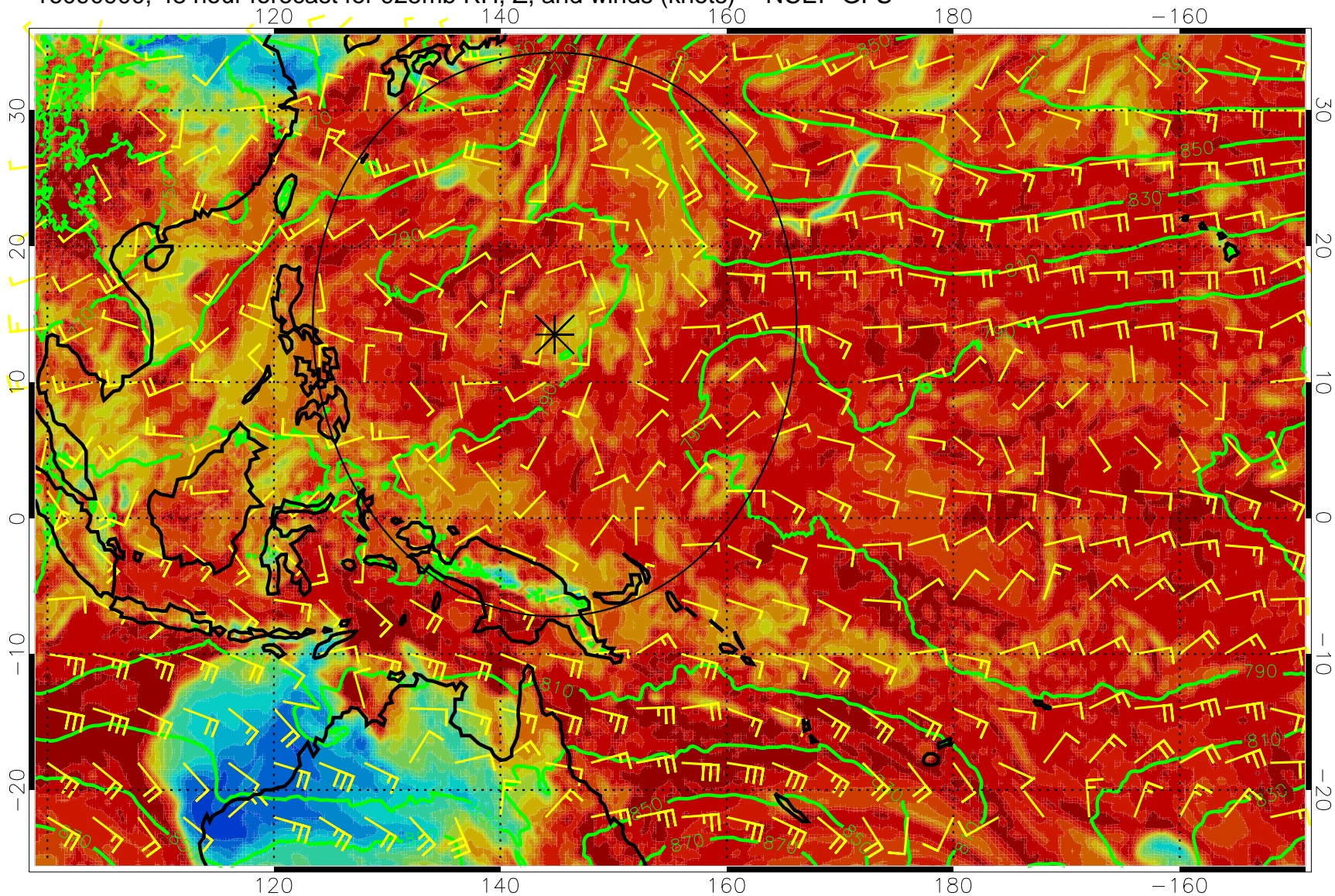
16090900, 48 hour forecast for 925mb RH, Z, and winds (knots) -- NCEP GFS
