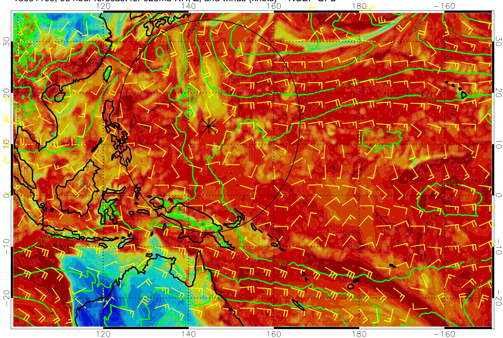
16091100, 96 hour forecast for 925mb RH, Z, and winds (knots) -- NCEP GFS
