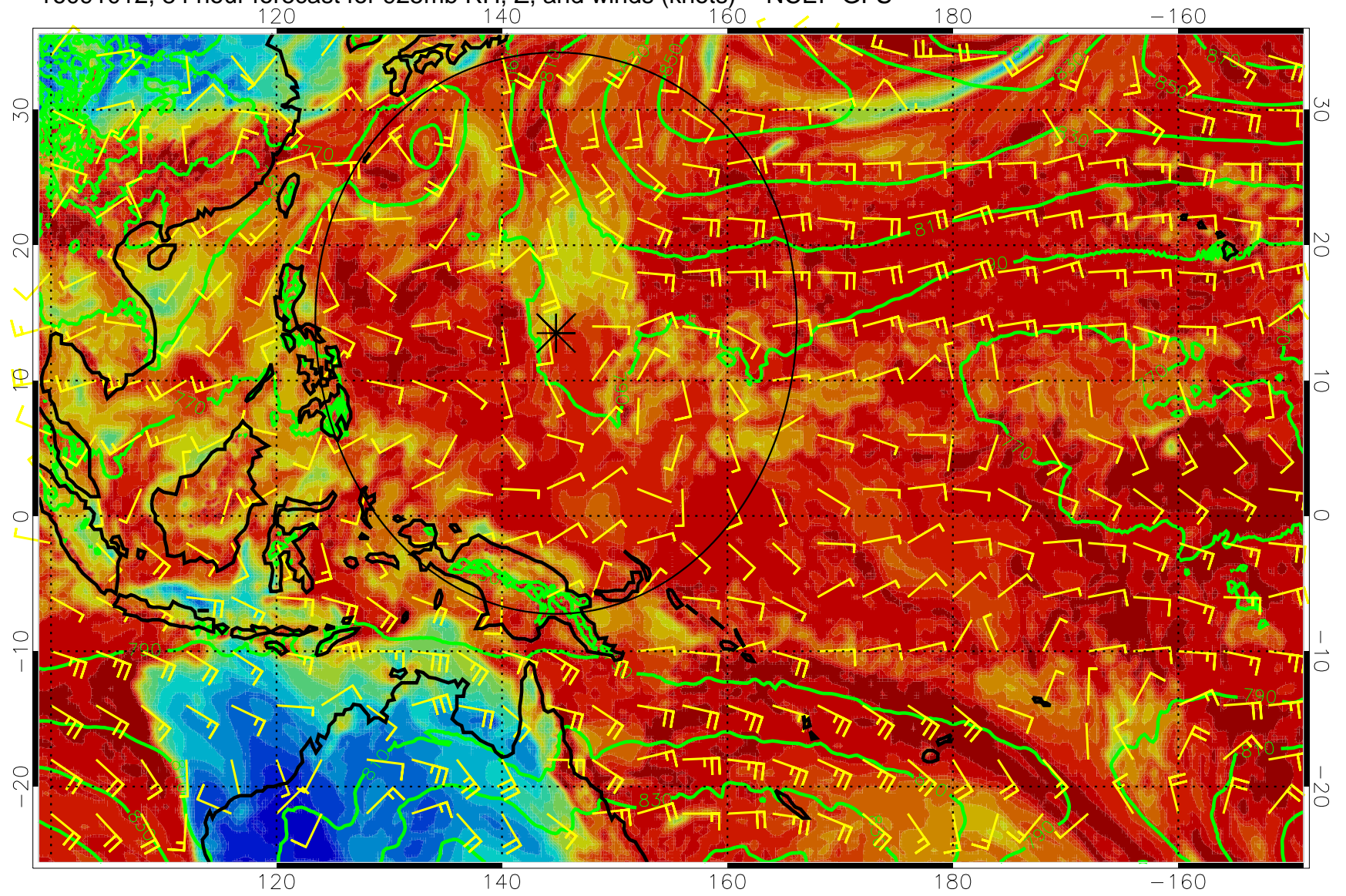
16091012, 84 hour forecast for 925mb RH, Z, and winds (knots) -- NCEP GFS
