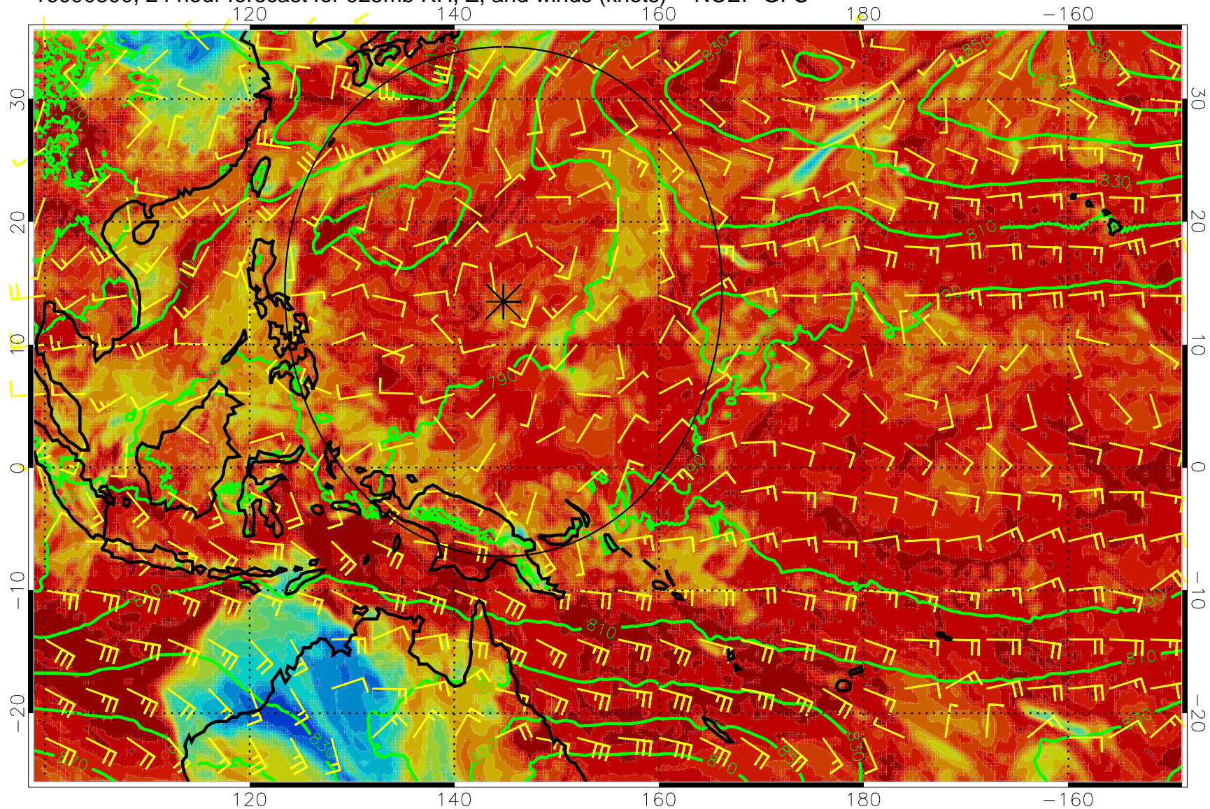
16090800, 24 hour forecast for 925mb RH, Z, and winds (knots) -- NCEP GFS
