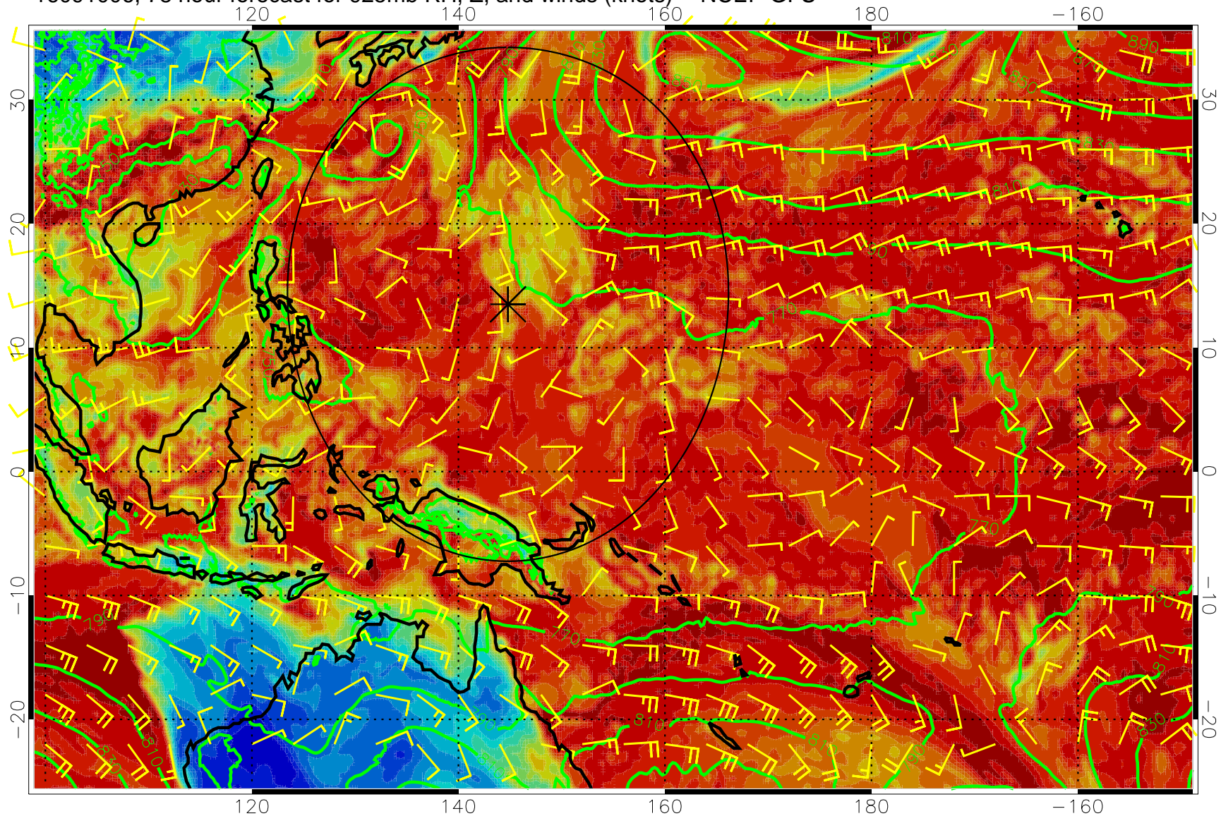
16091006, 78 hour forecast for 925mb RH, Z, and winds (knots) -- NCEP GFS
