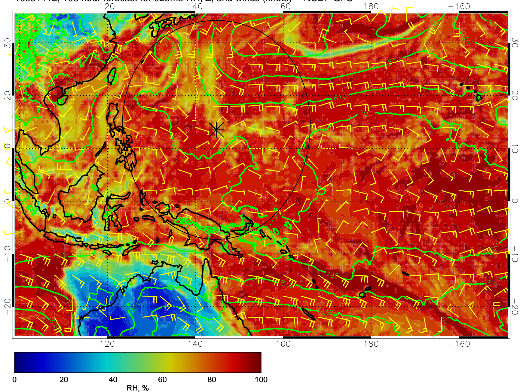
16091112, 108 hour forecast for 925mb RH, Z, and winds (knots) -- NCEP GFS
