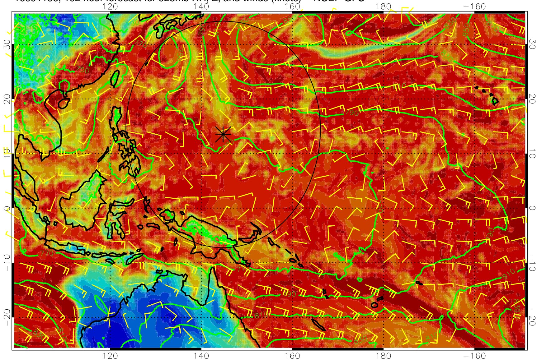
16091106, 102 hour forecast for 925mb RH, Z, and winds (knots) -- NCEP GFS
