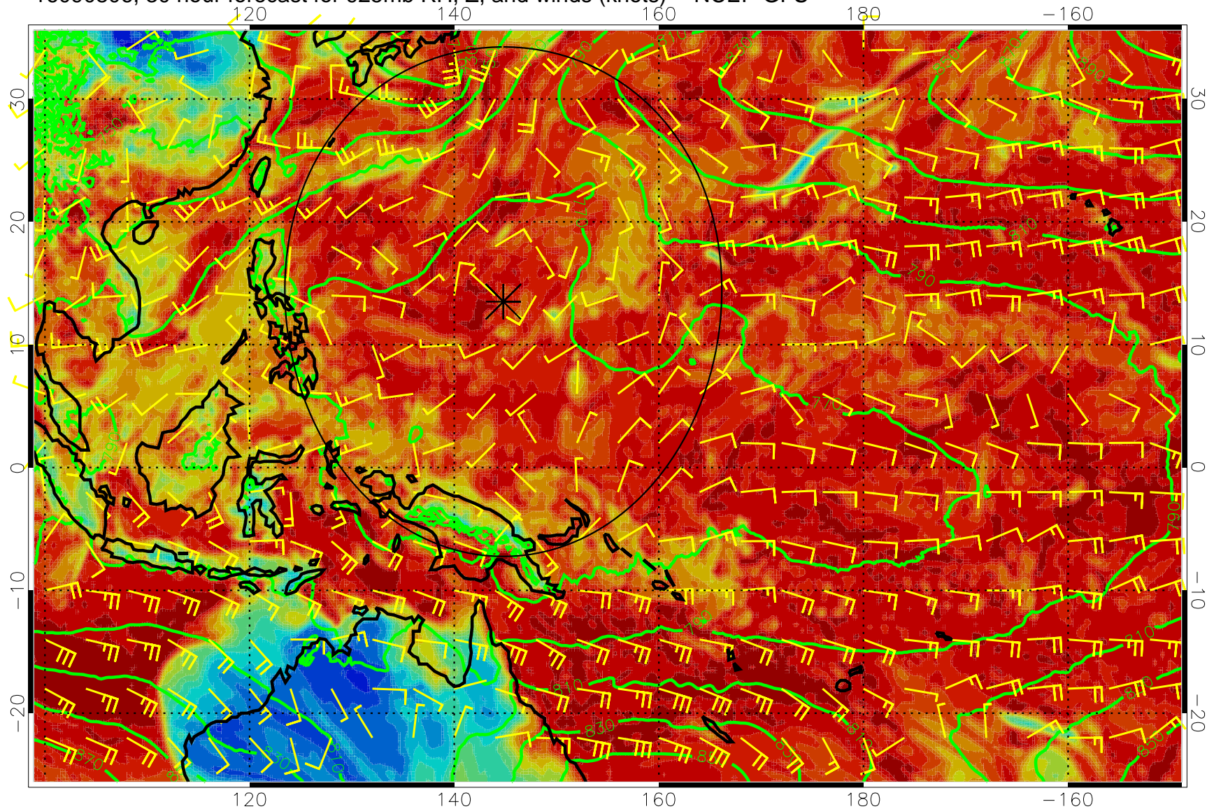
16090806, 30 hour forecast for 925mb RH, Z, and winds (knots) -- NCEP GFS
