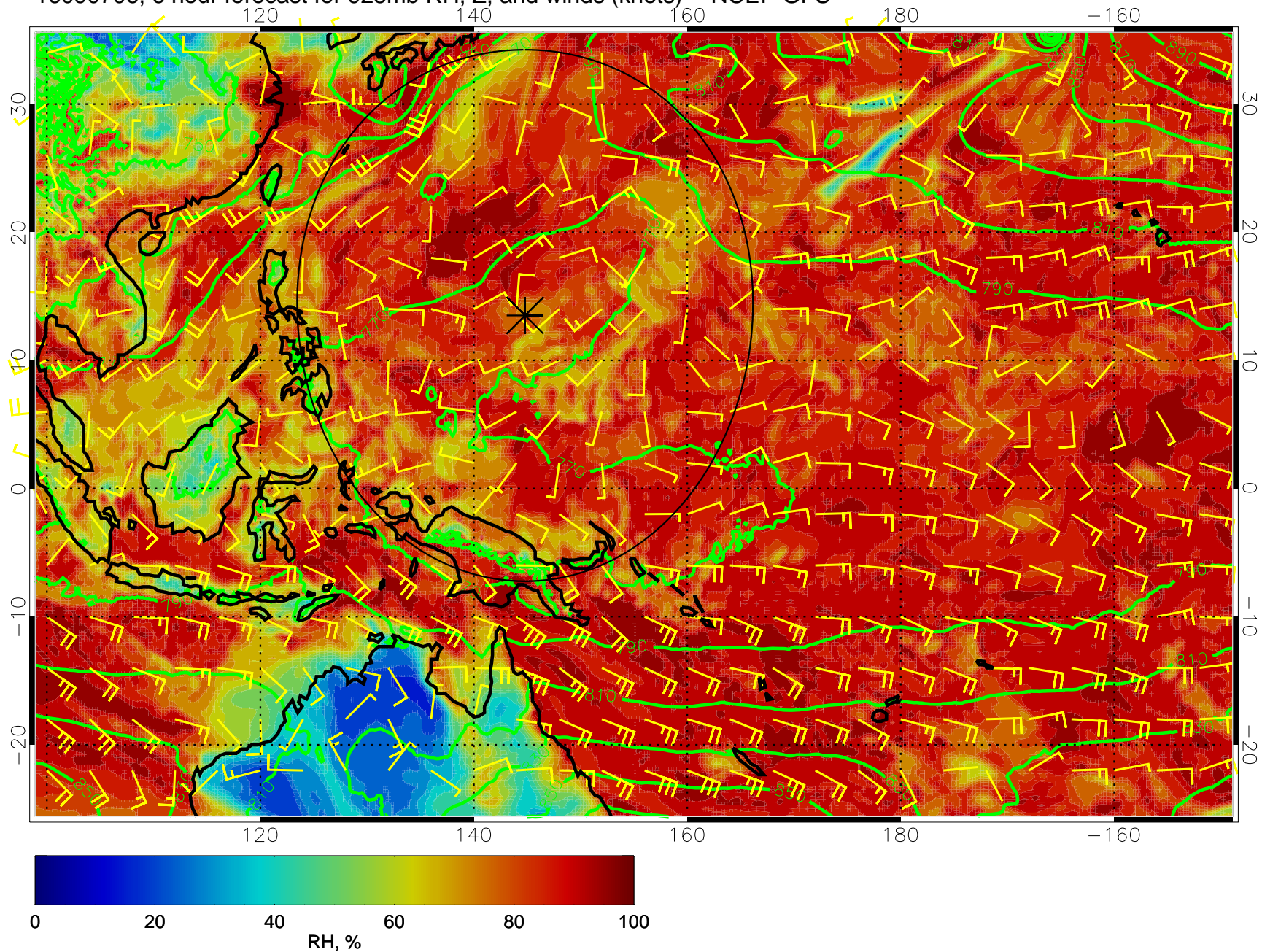
16090706, 6 hour forecast for 925mb RH, Z, and winds (knots) -- NCEP GFS
