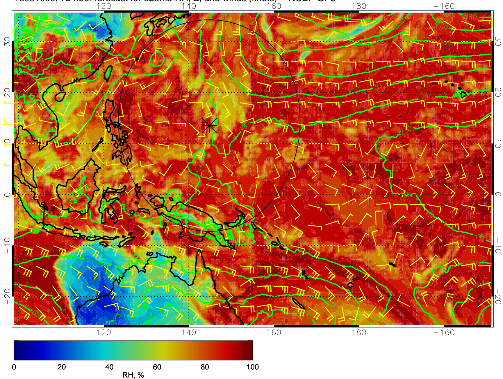
16091000, 72 hour forecast for 925mb RH, Z, and winds (knots) -- NCEP GFS
