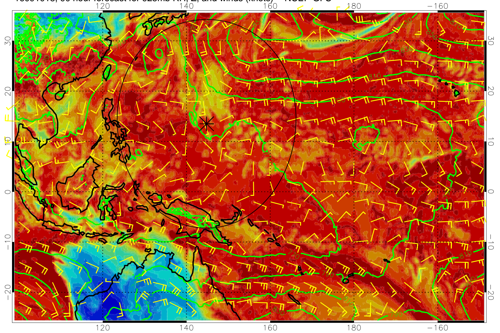
16091018, 90 hour forecast for 925mb RH, Z, and winds (knots) -- NCEP GFS
