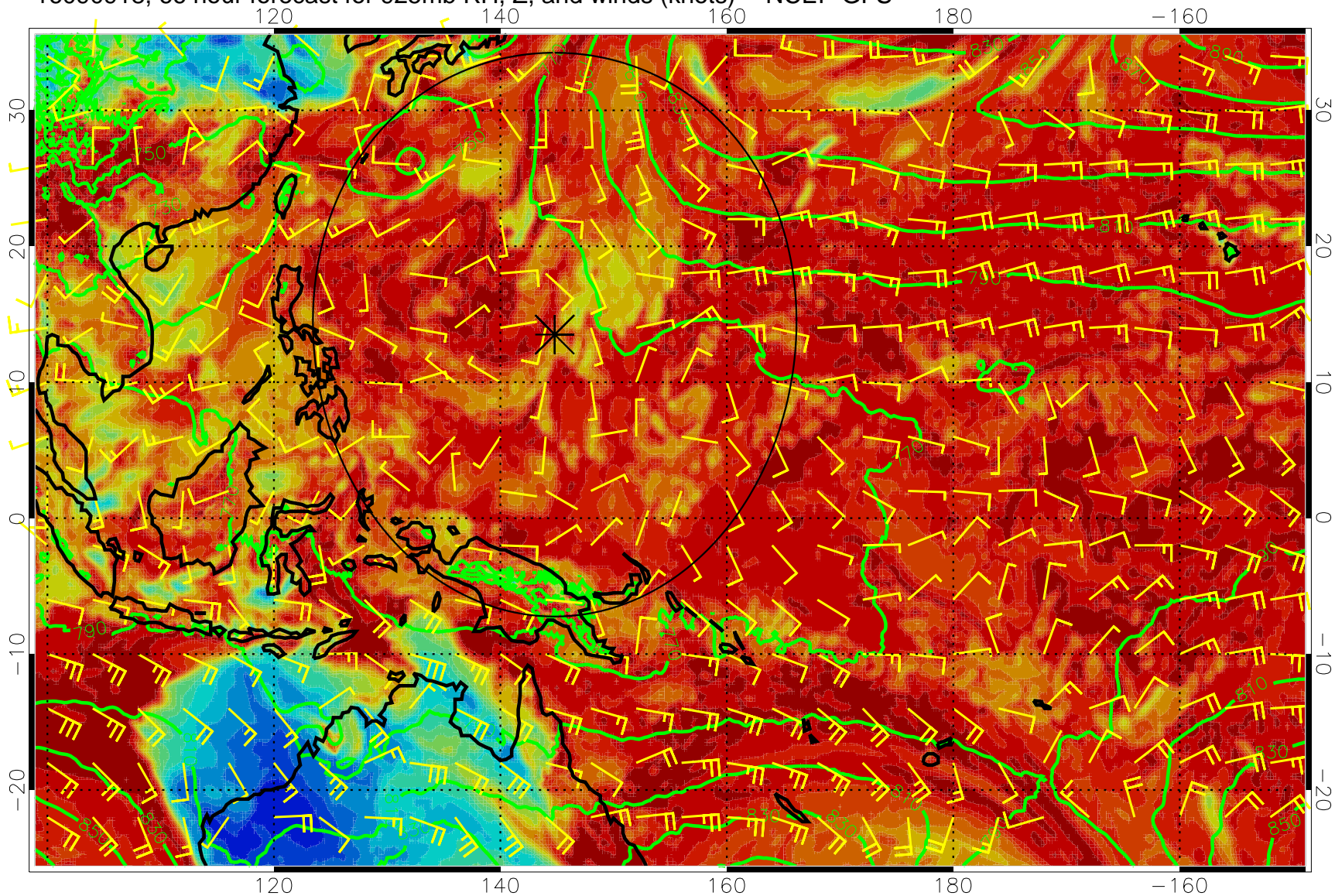
16090918, 66 hour forecast for 925mb RH, Z, and winds (knots) -- NCEP GFS
