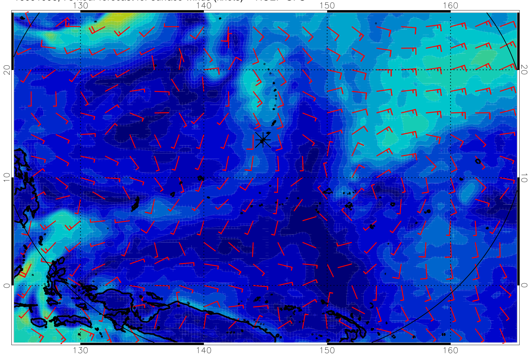
16091006, 78 hour forecast for surface winds (knots) -- NCEP GFS
