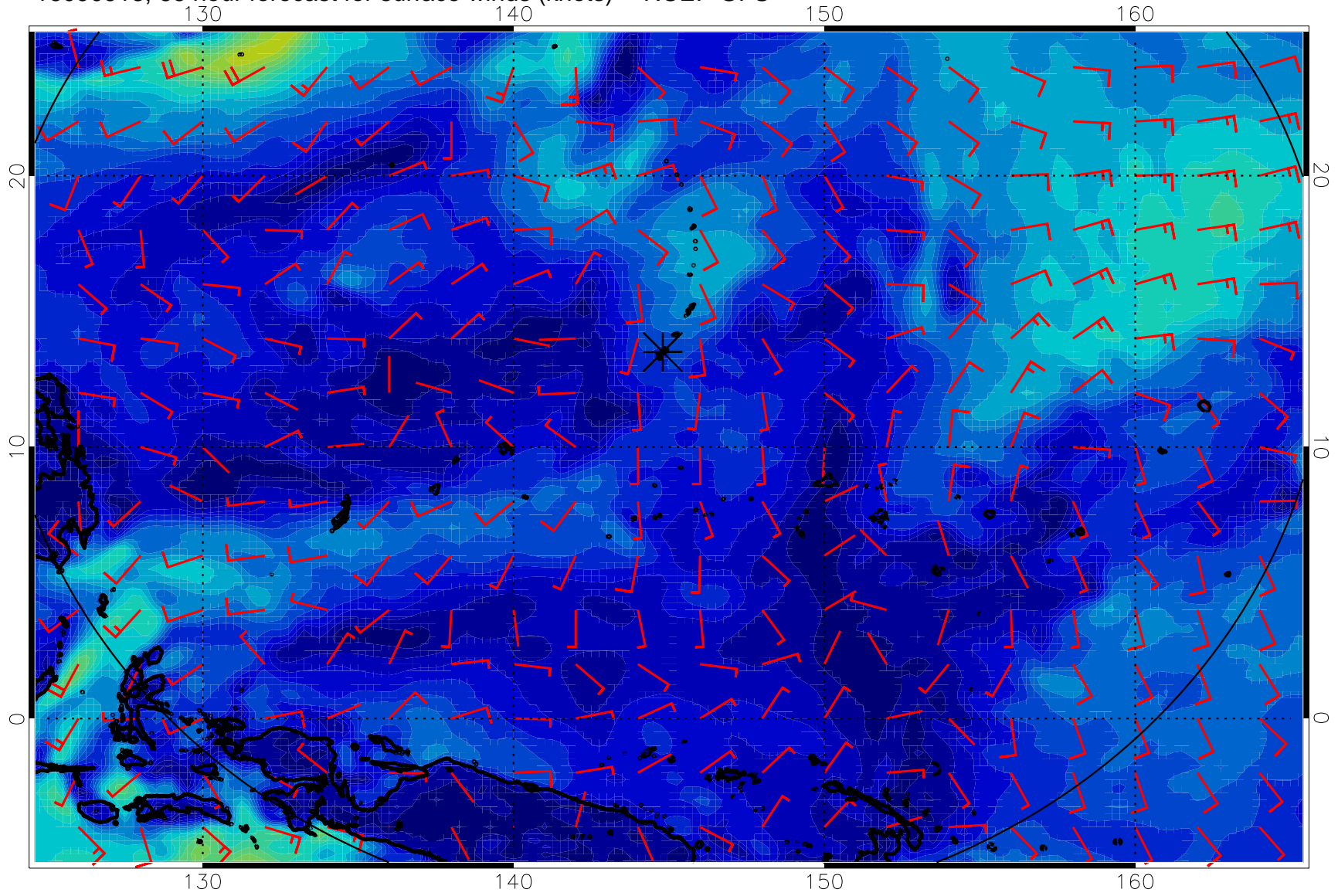
16090918, 66 hour forecast for surface winds (knots) -- NCEP GFS
