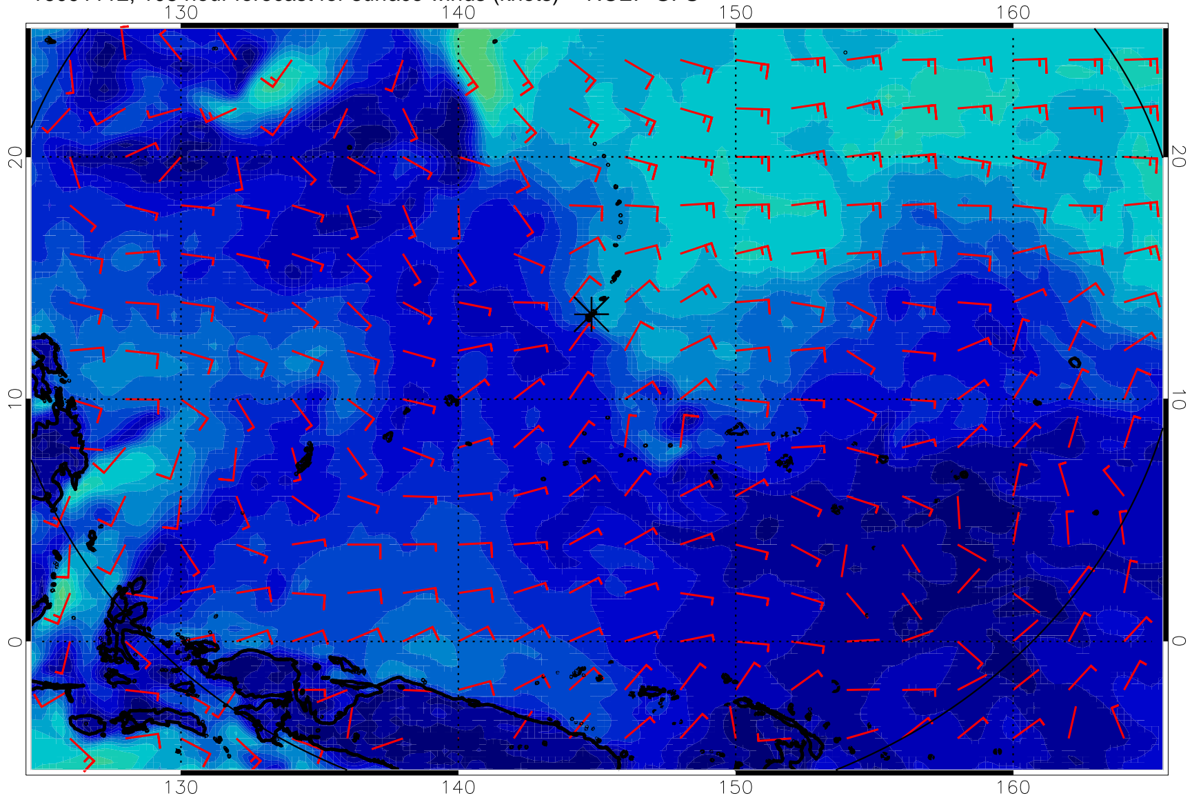
16091112, 108 hour forecast for surface winds (knots) -- NCEP GFS
