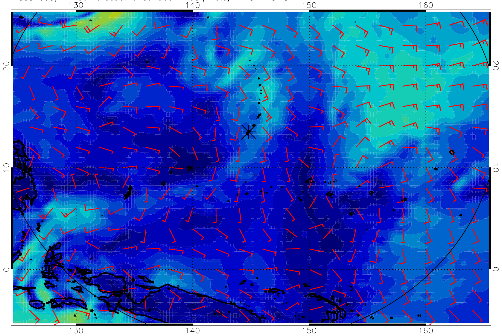
16091000, 72 hour forecast for surface winds (knots) -- NCEP GFS
