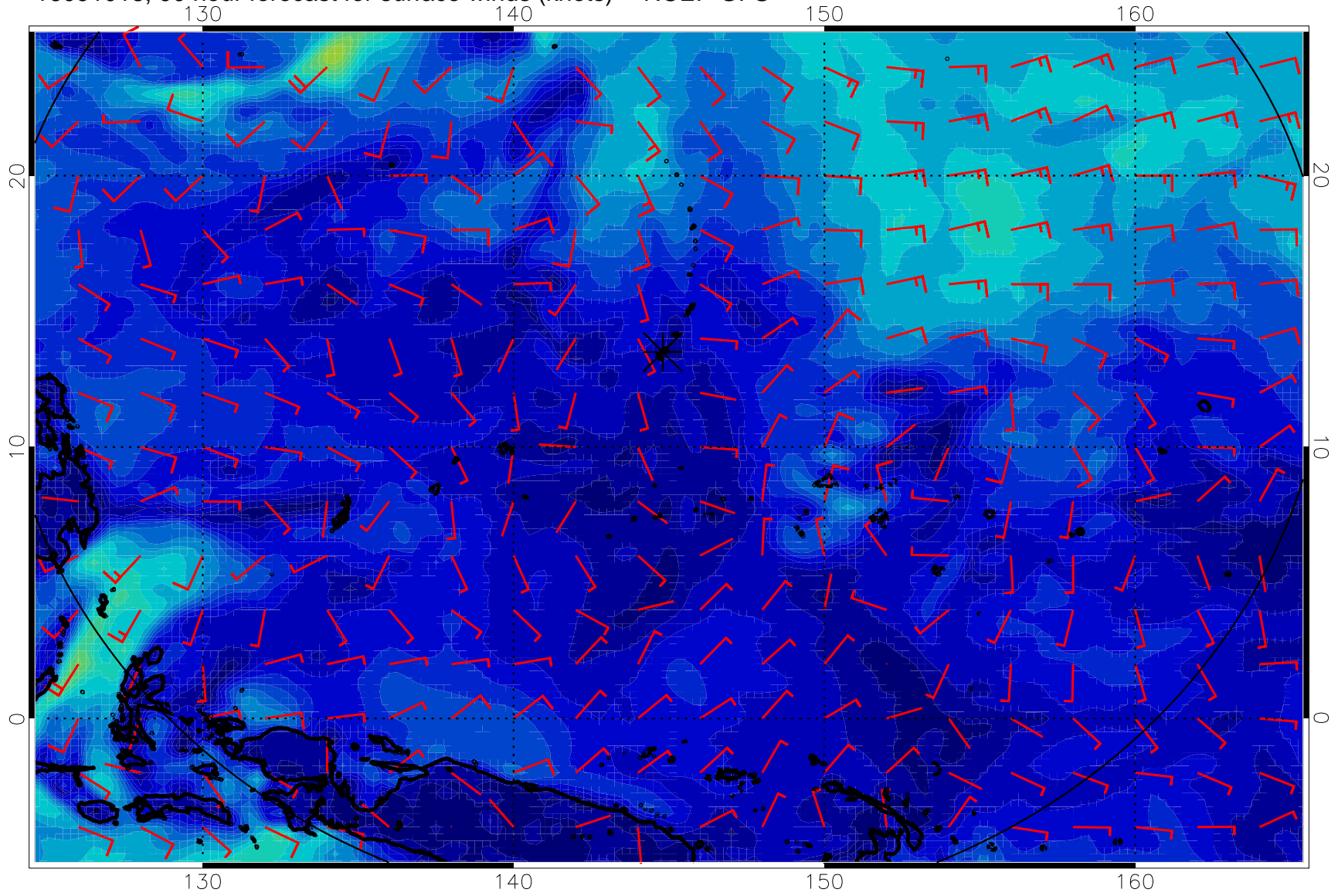
16091018, 90 hour forecast for surface winds (knots) -- NCEP GFS
