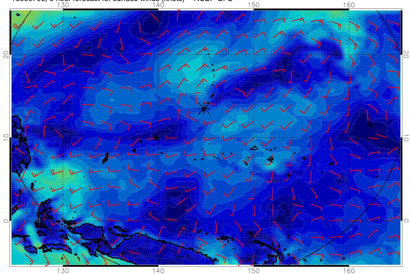
16090706, 6 hour forecast for surface winds (knots) -- NCEP GFS
