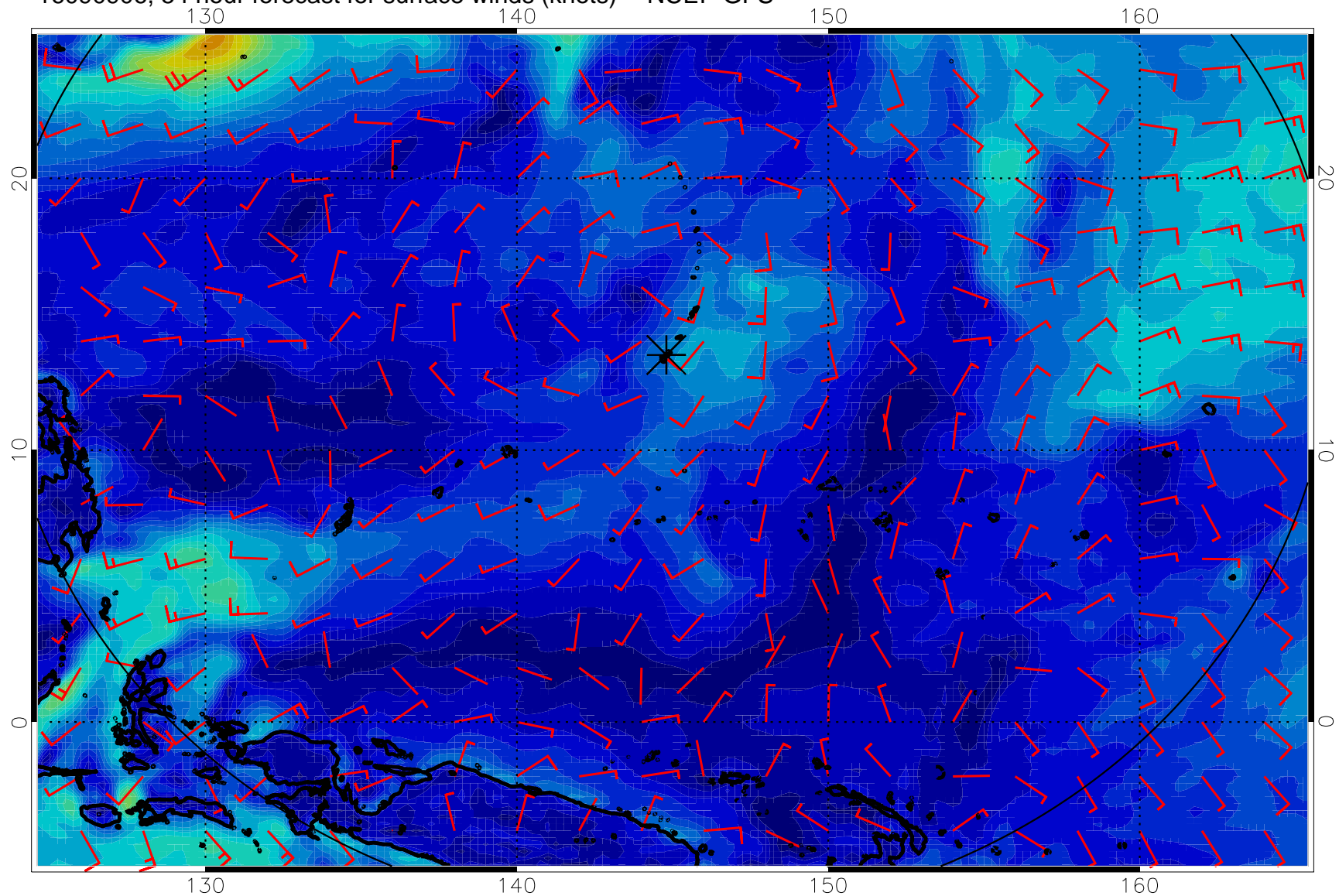
16090906, 54 hour forecast for surface winds (knots) -- NCEP GFS
