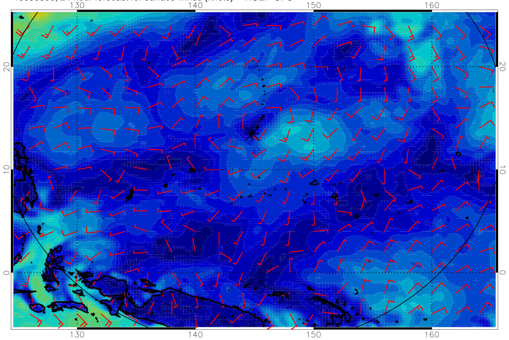
16090800, 24 hour forecast for surface winds (knots) -- NCEP GFS
