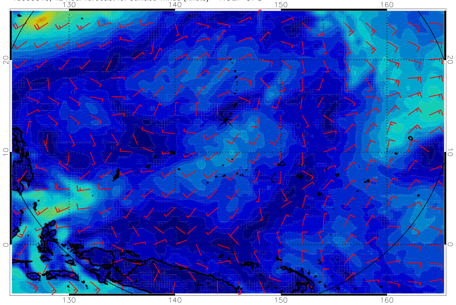
16090818, 42 hour forecast for surface winds (knots) -- NCEP GFS
