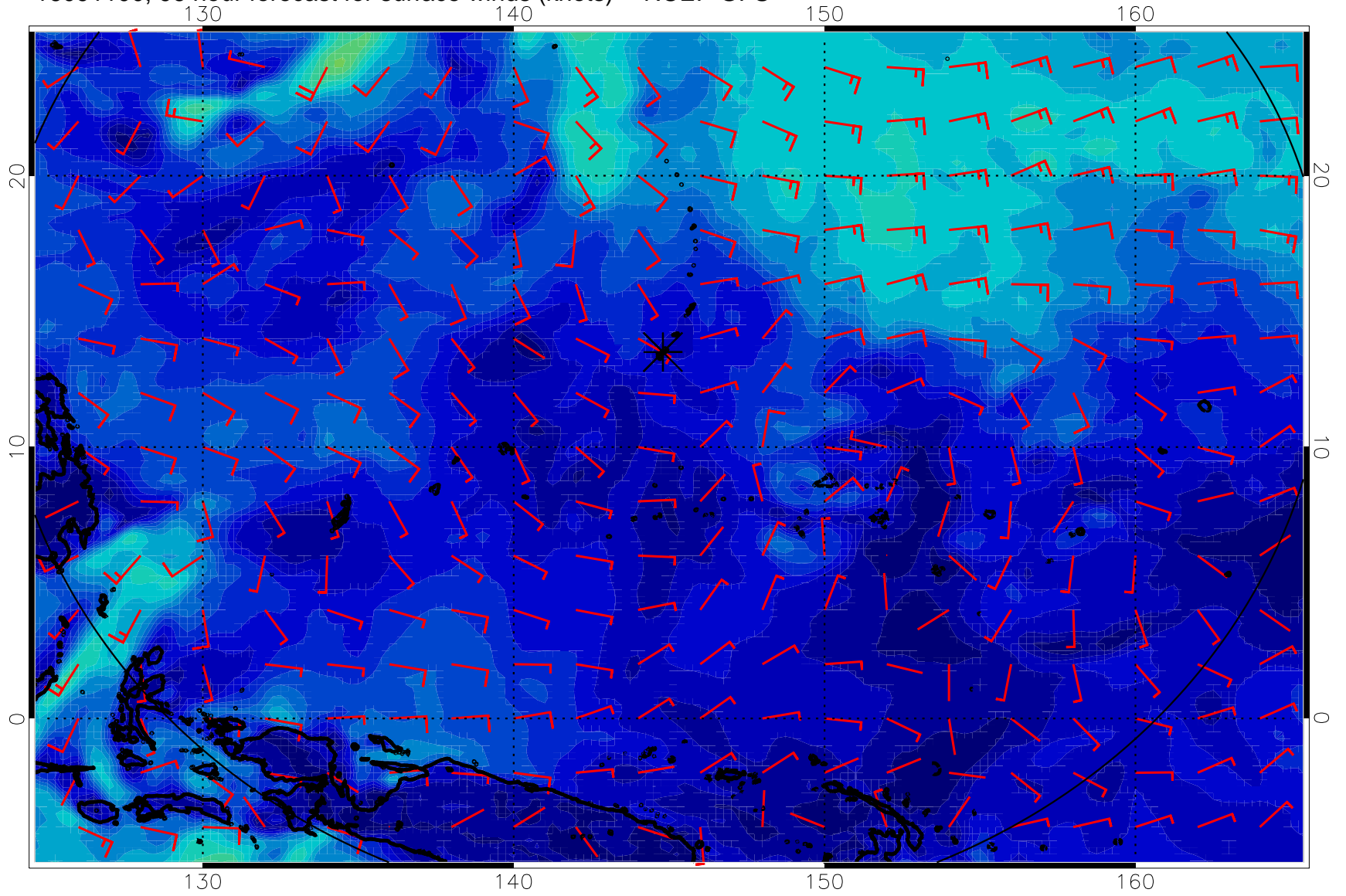
16091100, 96 hour forecast for surface winds (knots) -- NCEP GFS
