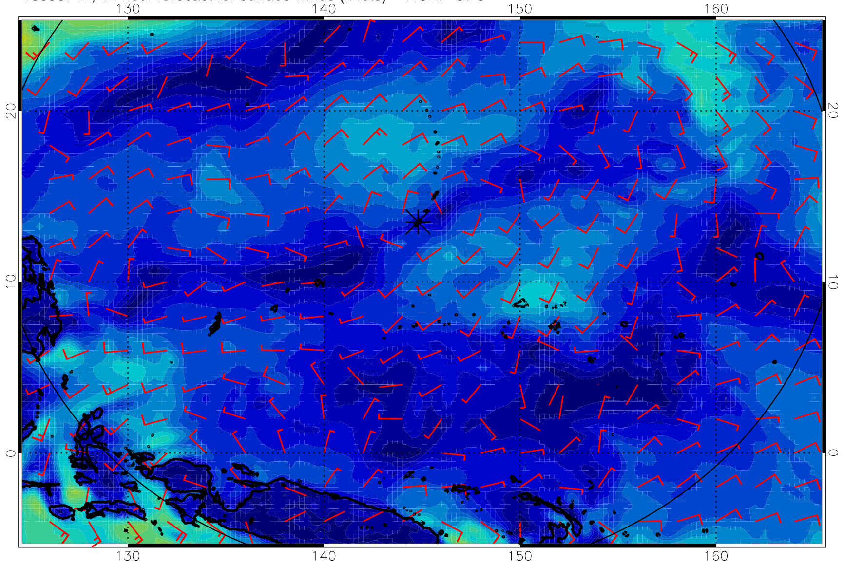
16090712, 12 hour forecast for surface winds (knots) -- NCEP GFS
