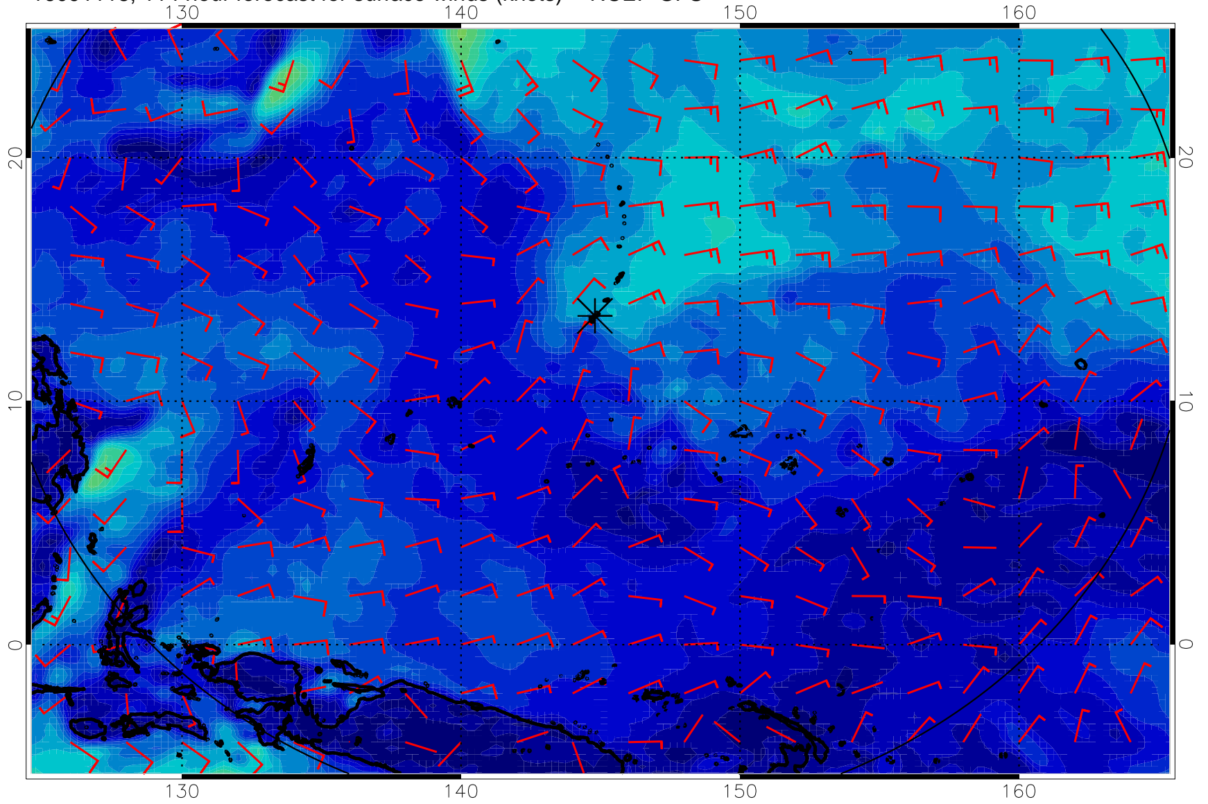
16091118, 114 hour forecast for surface winds (knots) -- NCEP GFS
