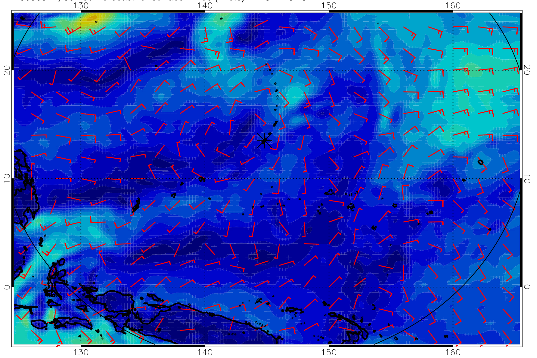
16090912, 60 hour forecast for surface winds (knots) -- NCEP GFS
