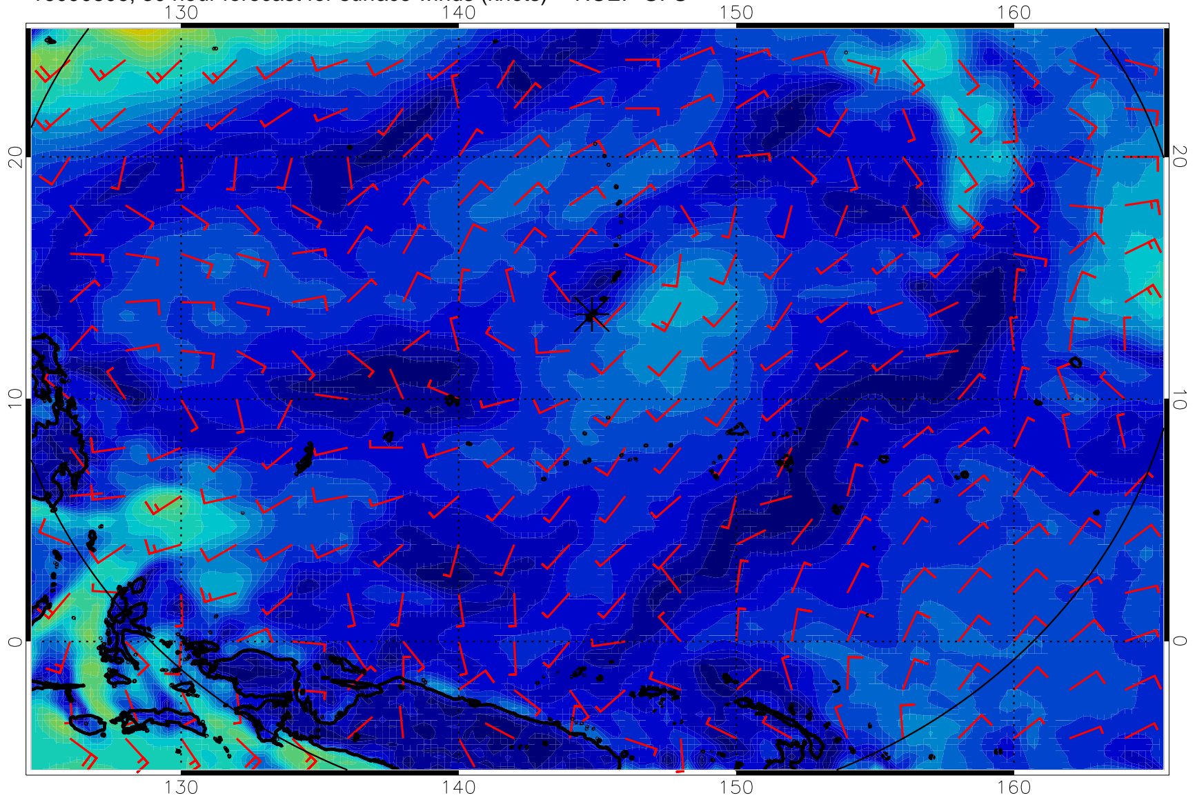
16090806, 30 hour forecast for surface winds (knots) -- NCEP GFS
