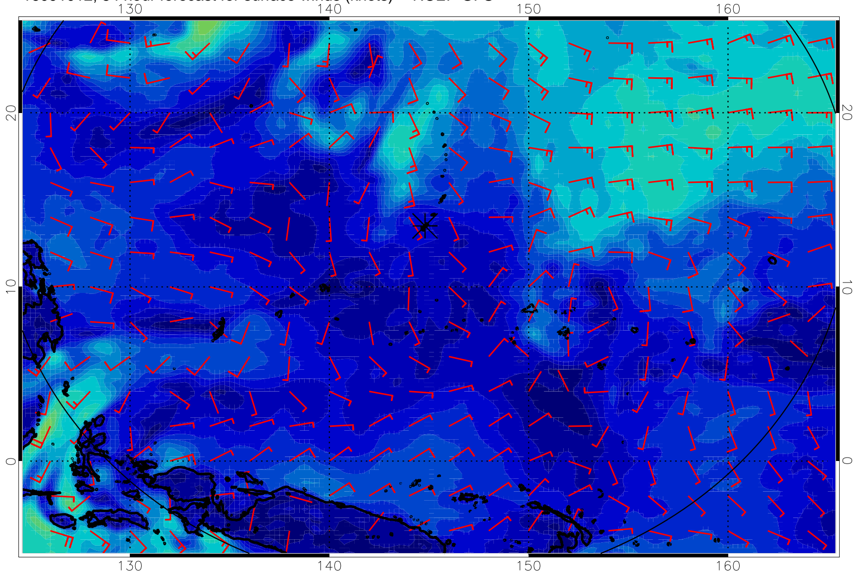
16091012, 84 hour forecast for surface winds (knots) -- NCEP GFS
