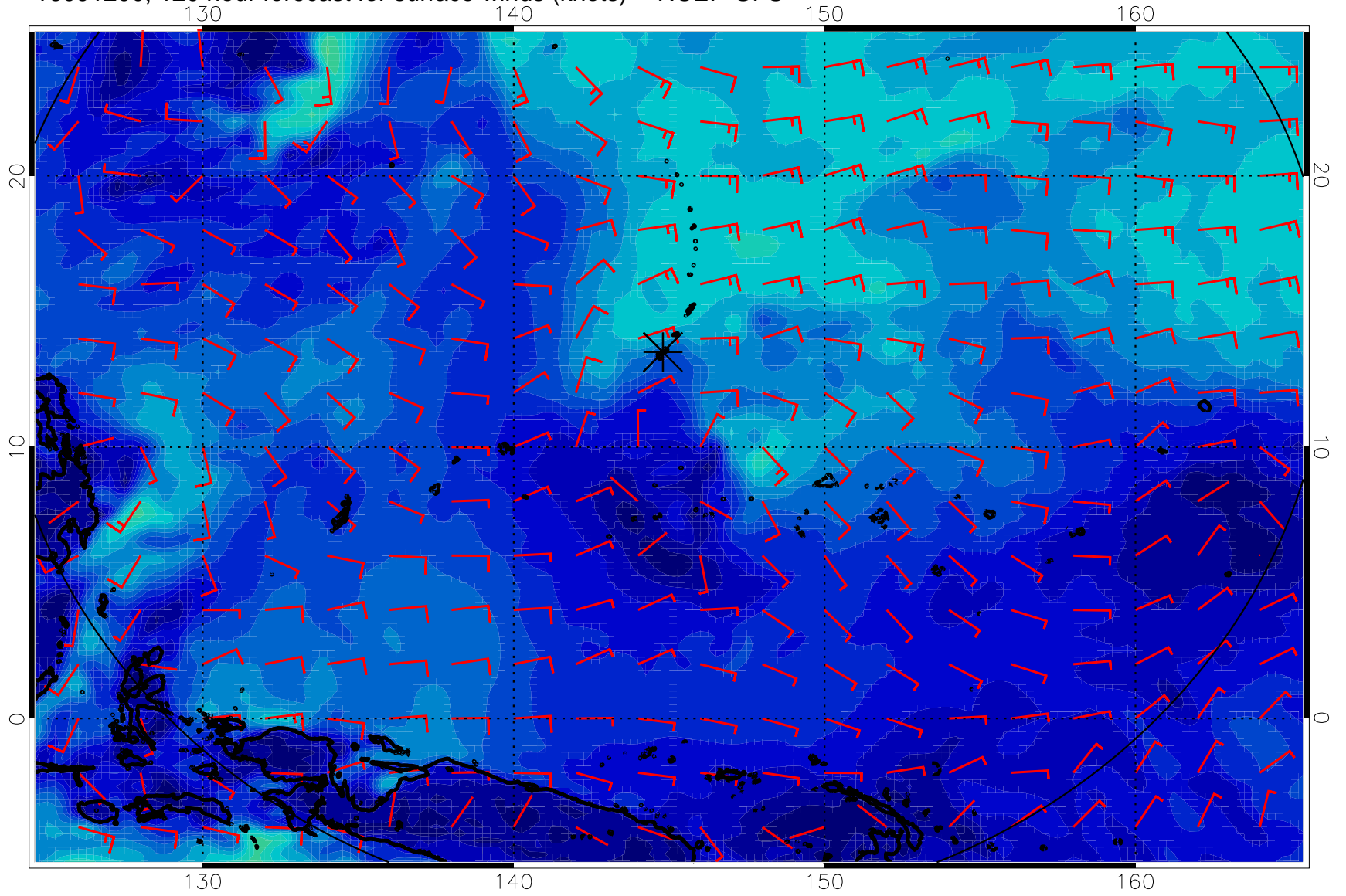
16091200, 120 hour forecast for surface winds (knots) -- NCEP GFS
