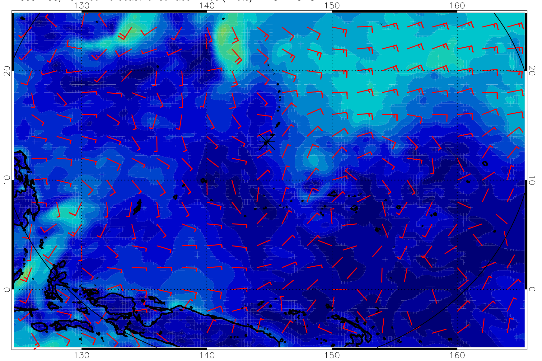
16091106, 102 hour forecast for surface winds (knots) -- NCEP GFS
