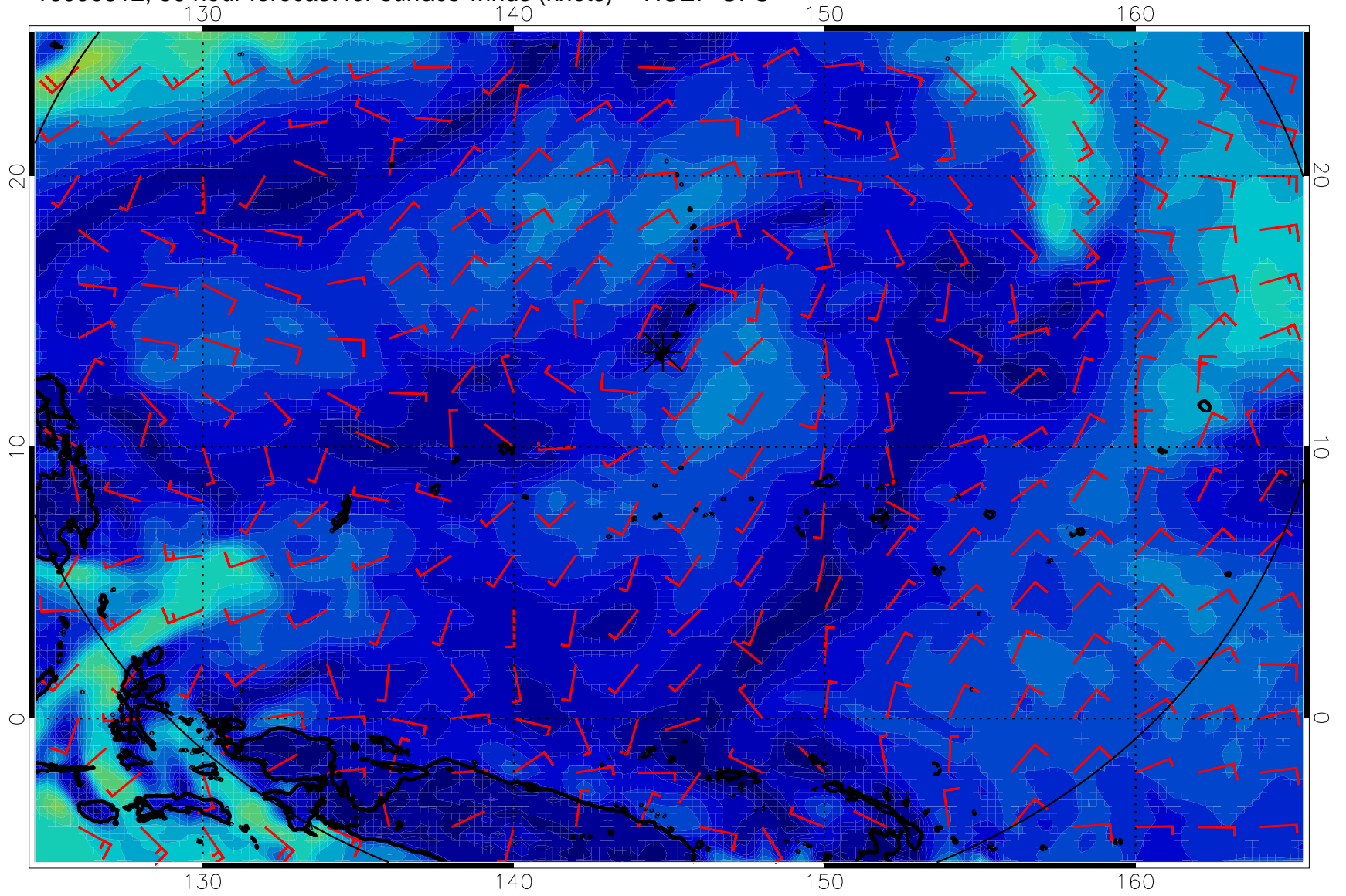
16090812, 36 hour forecast for surface winds (knots) -- NCEP GFS
