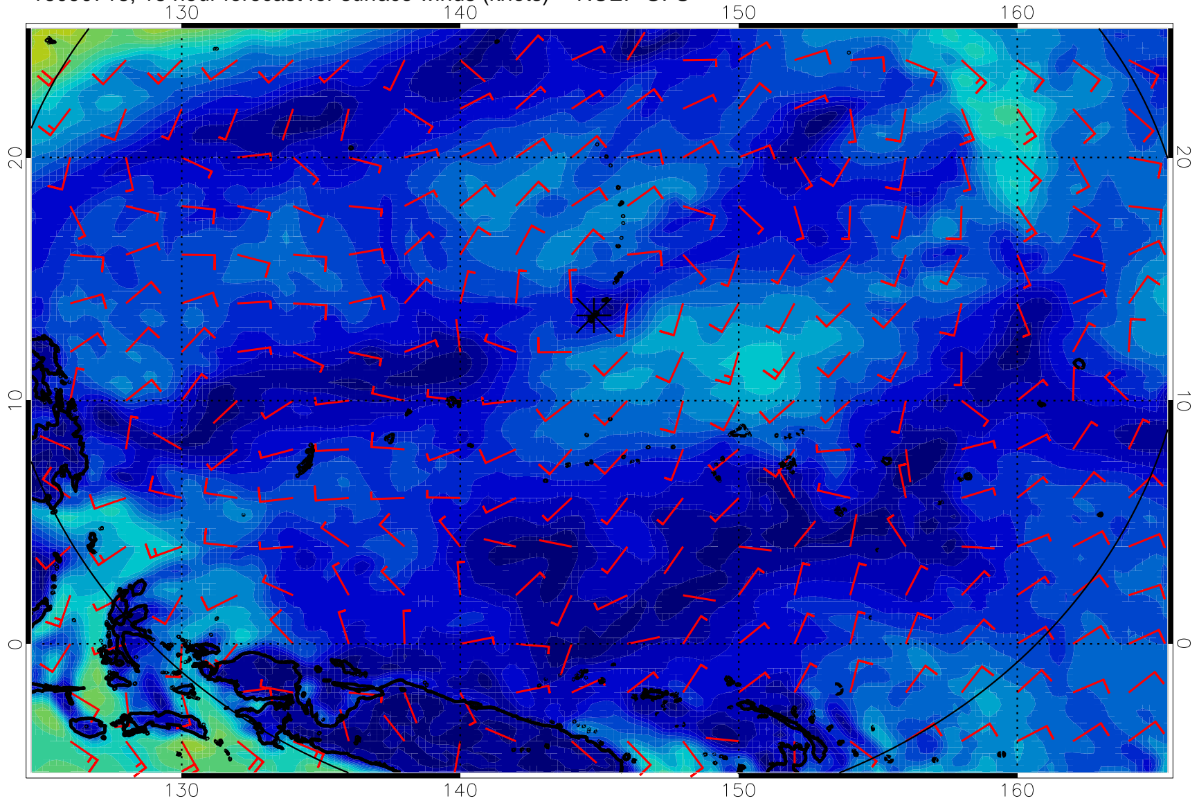
16090718, 18 hour forecast for surface winds (knots) -- NCEP GFS
