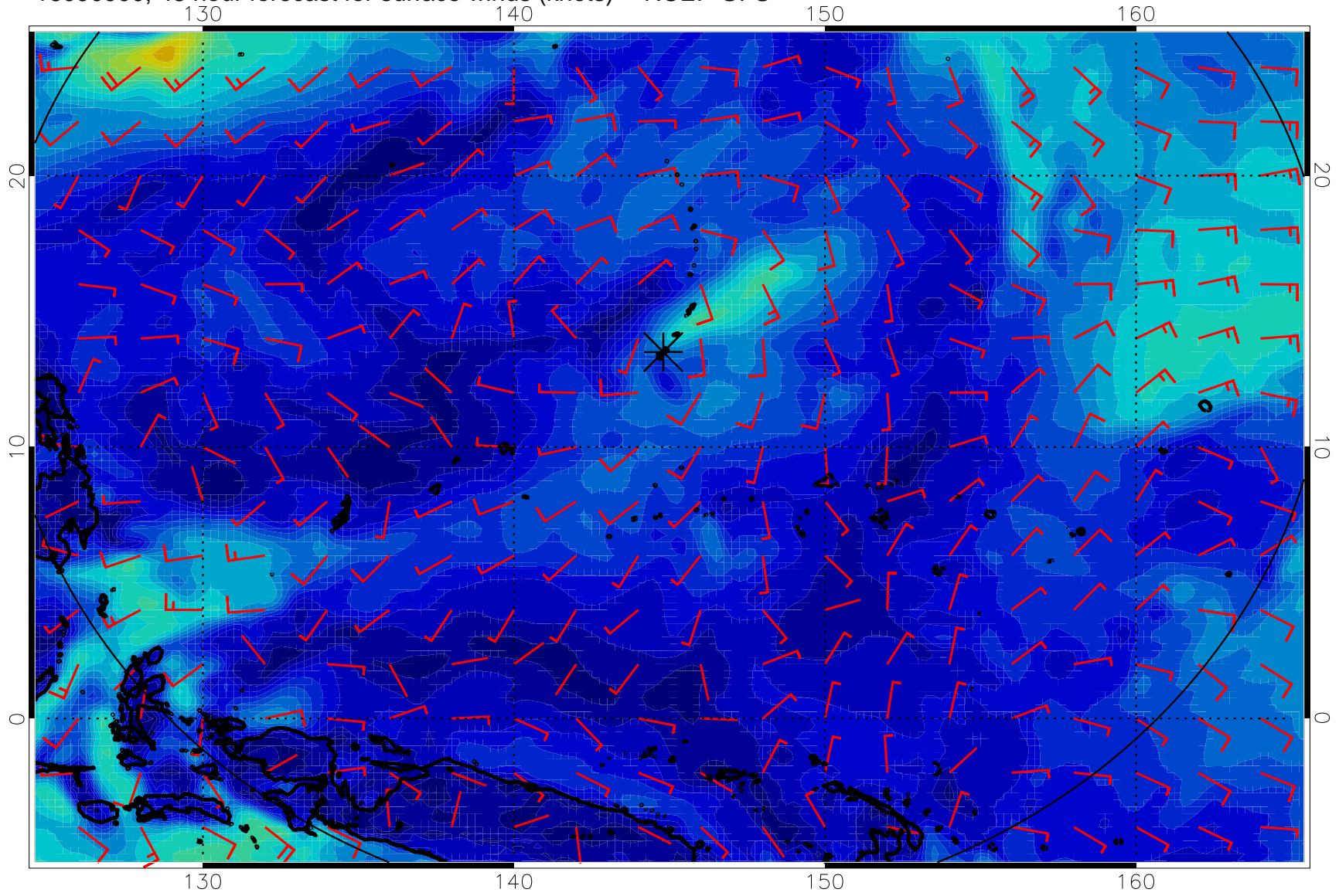
16090900, 48 hour forecast for surface winds (knots) -- NCEP GFS
