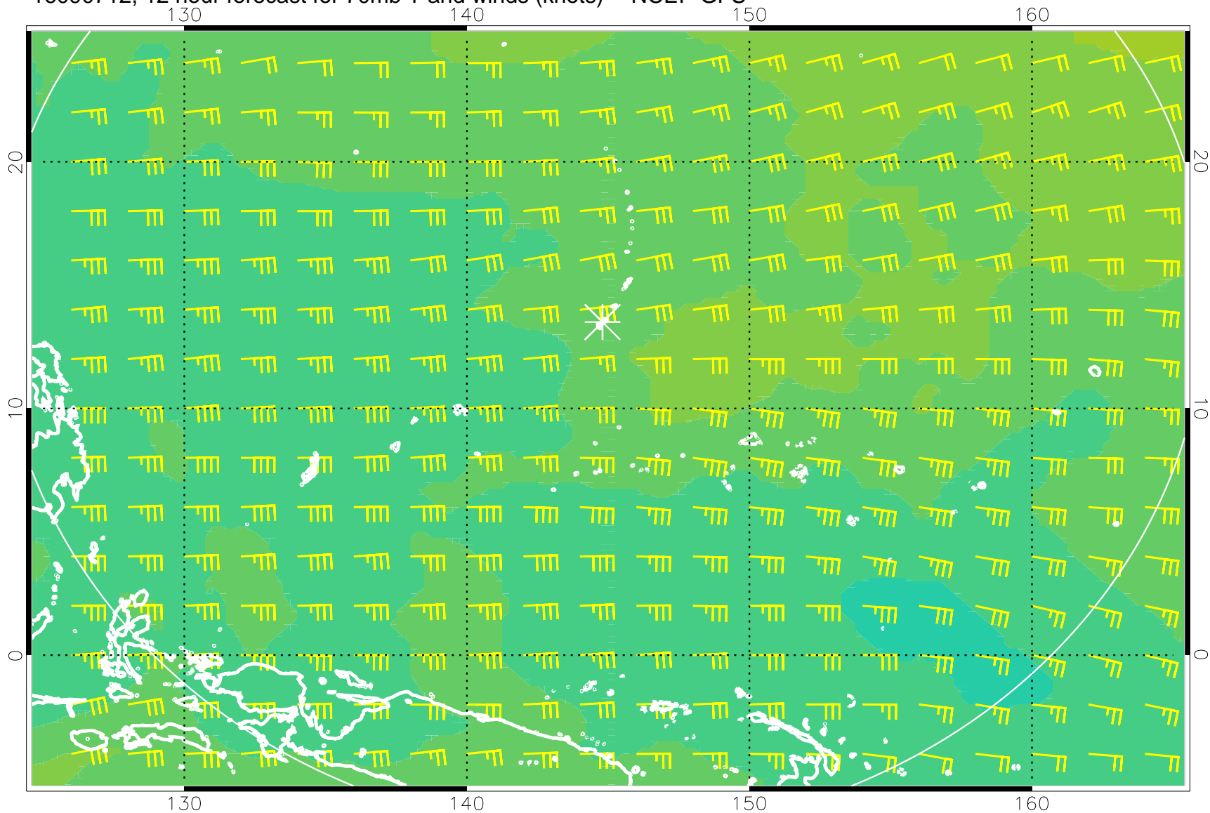
16090712, 12 hour forecast for 70mb T and winds (knots) -- NCEP GFS
