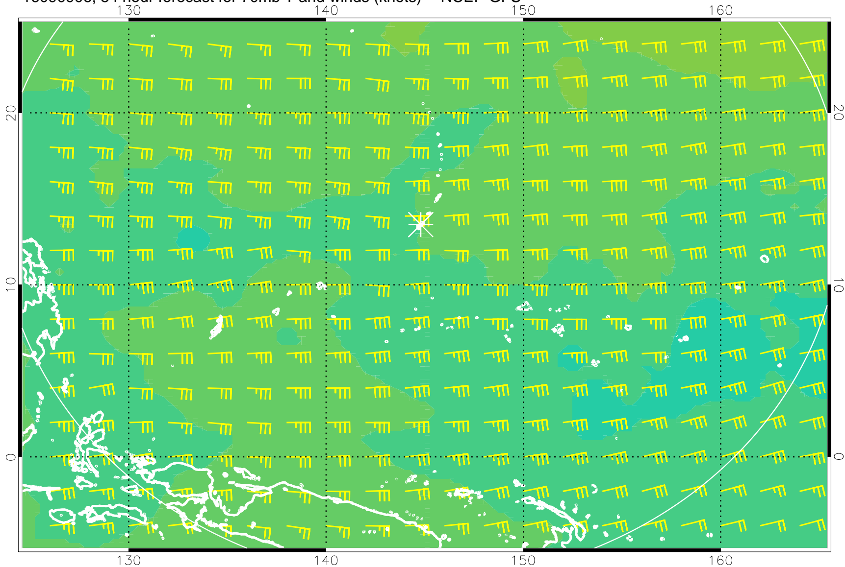
16090906, 54 hour forecast for 70mb T and winds (knots) -- NCEP GFS
