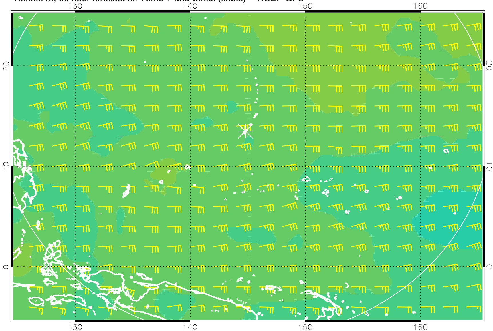
16090918, 66 hour forecast for 70mb T and winds (knots) -- NCEP GFS
