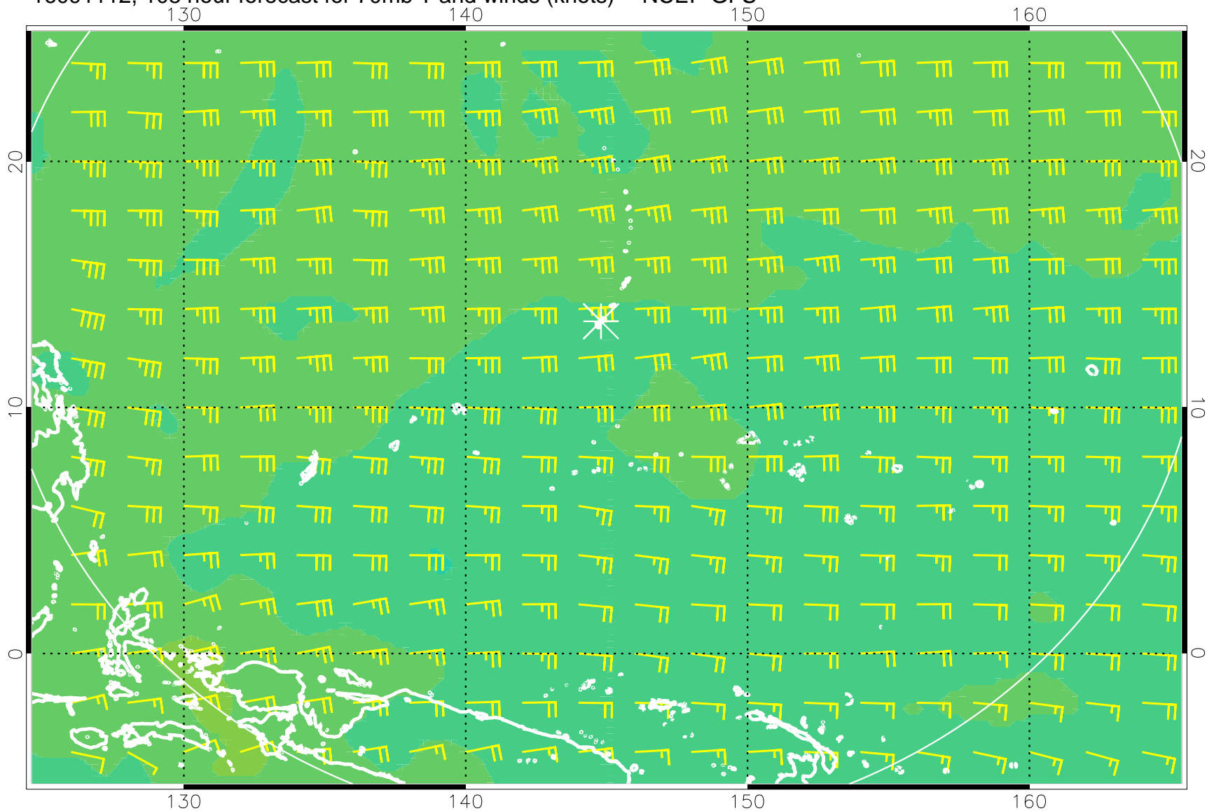
16091112, 108 hour forecast for 70mb T and winds (knots) -- NCEP GFS
