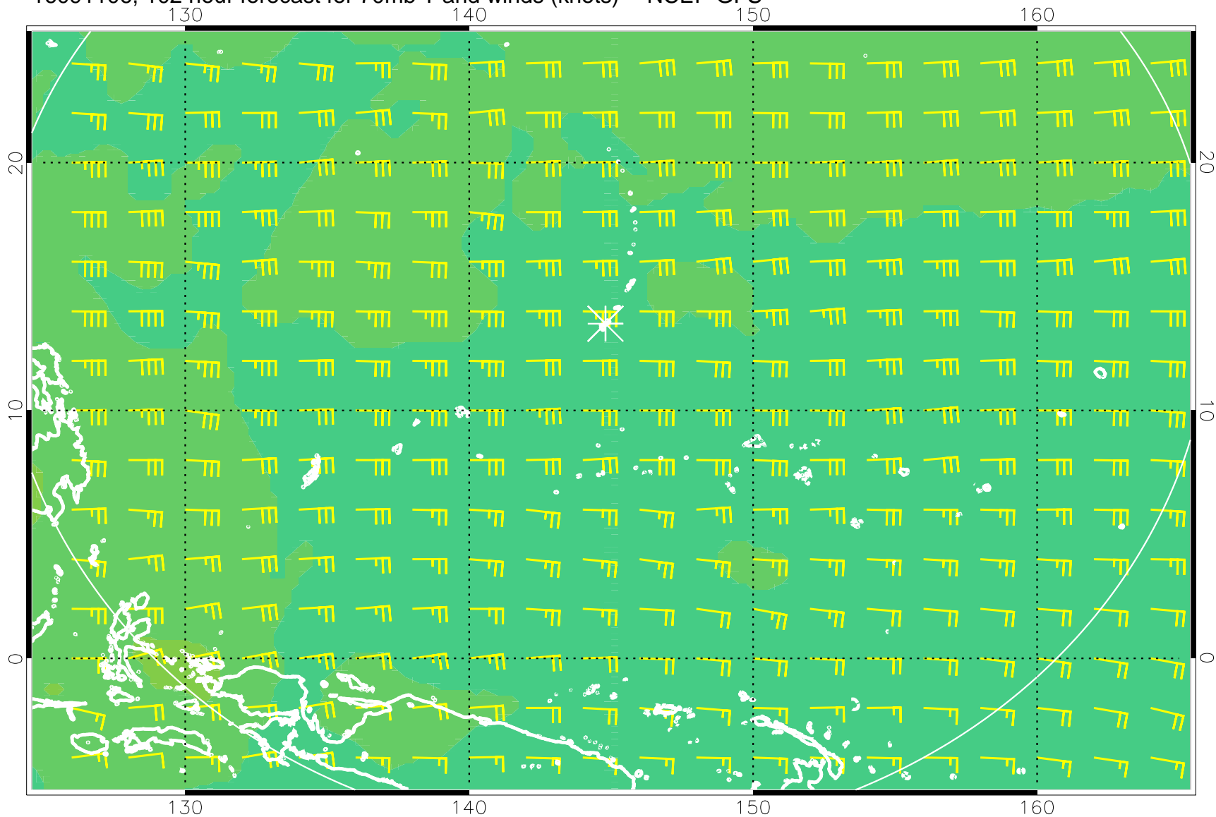
16091106, 102 hour forecast for 70mb T and winds (knots) -- NCEP GFS
