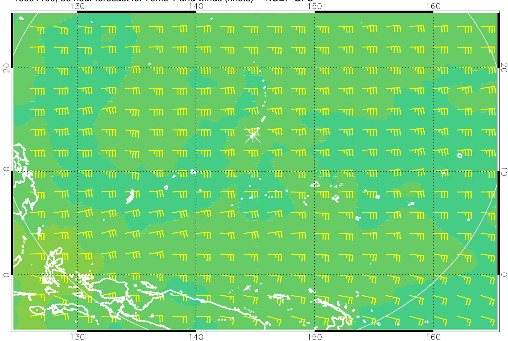
16091100, 96 hour forecast for 70mb T and winds (knots) -- NCEP GFS
