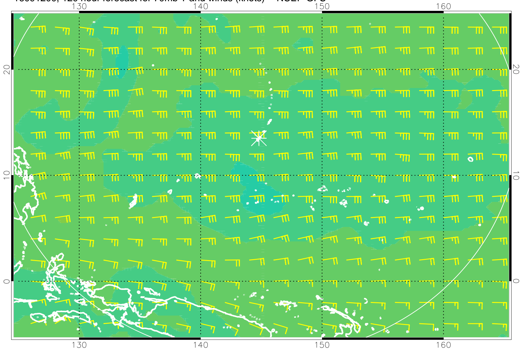
16091200, 120 hour forecast for 70mb T and winds (knots) -- NCEP GFS
