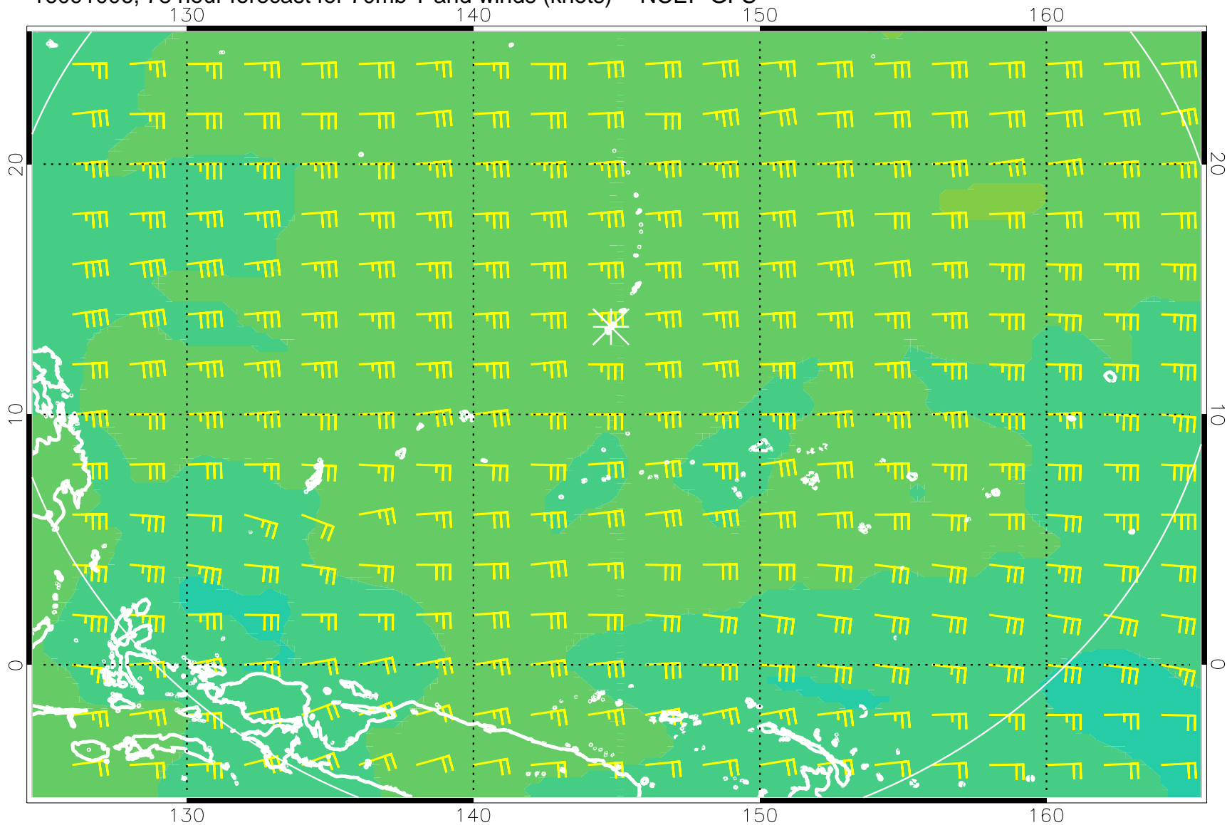
16091006, 78 hour forecast for 70mb T and winds (knots) -- NCEP GFS
