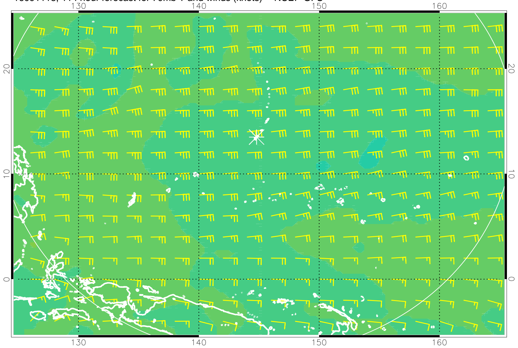
16091118, 114 hour forecast for 70mb T and winds (knots) -- NCEP GFS
