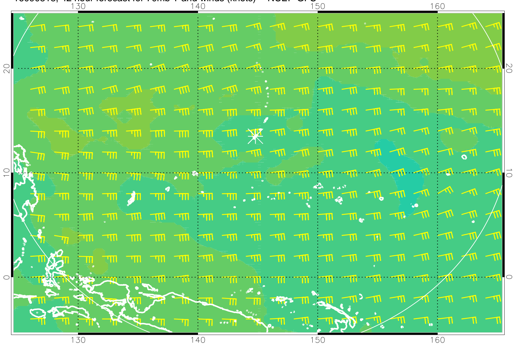
16090818, 42 hour forecast for 70mb T and winds (knots) -- NCEP GFS
