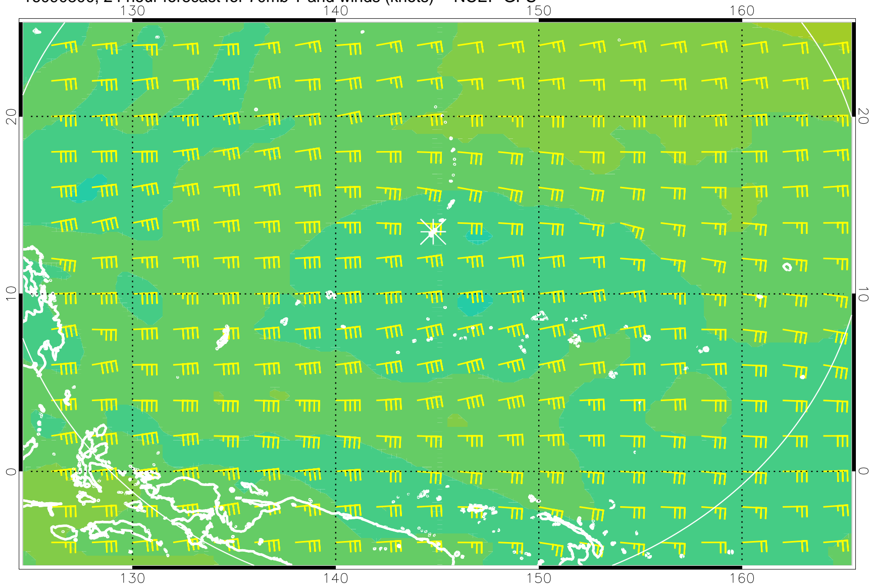
16090800, 24 hour forecast for 70mb T and winds (knots) -- NCEP GFS
