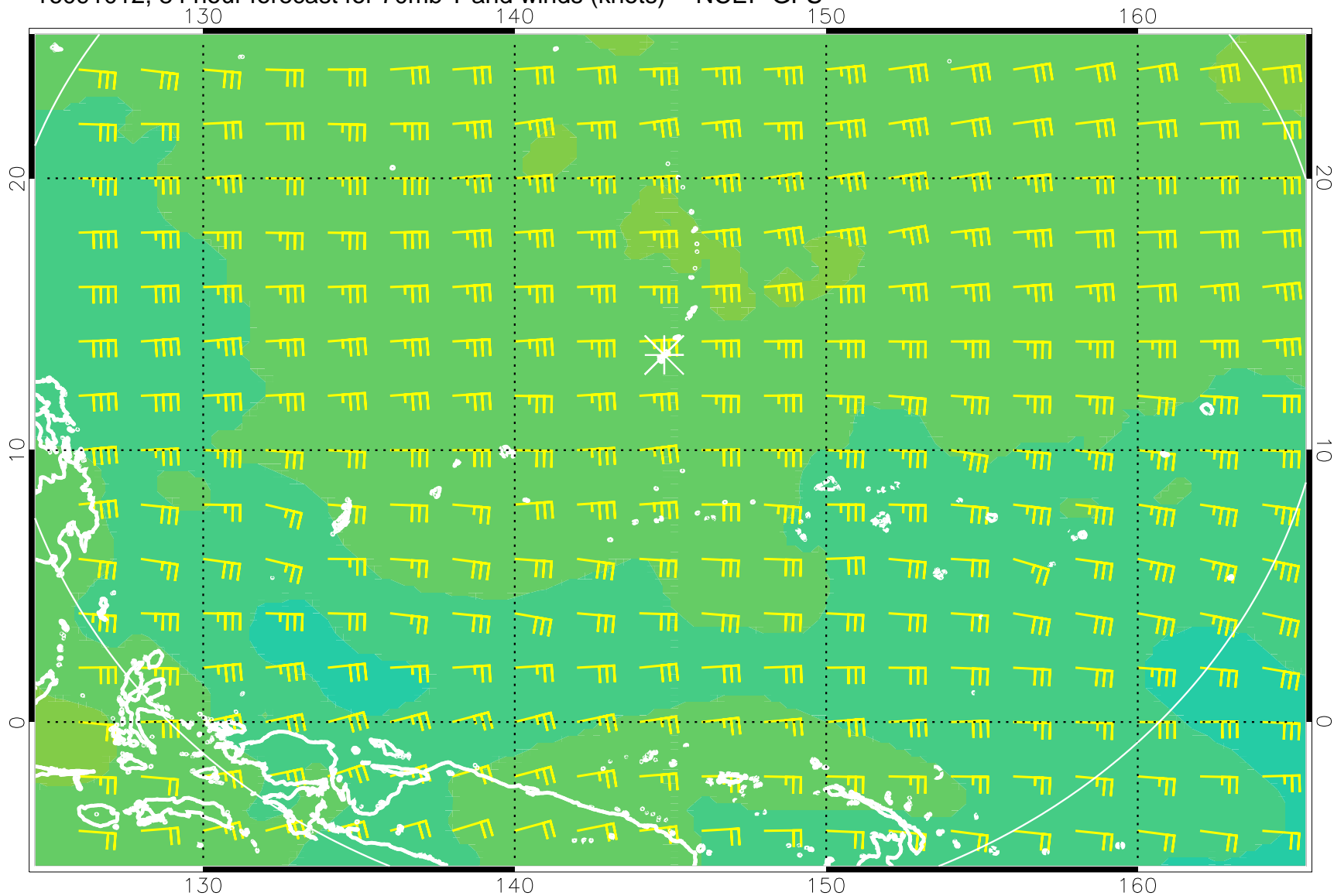
16091012, 84 hour forecast for 70mb T and winds (knots) -- NCEP GFS
