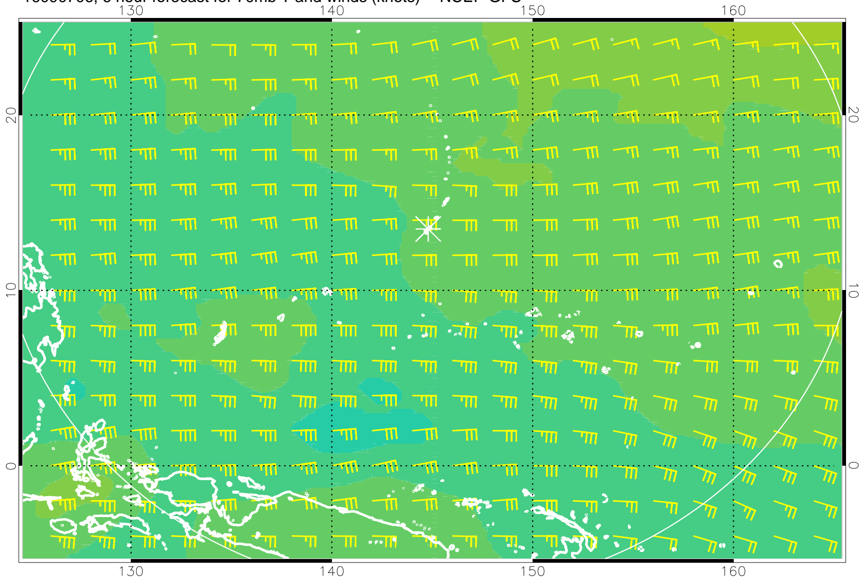
16090706, 6 hour forecast for 70mb T and winds (knots) -- NCEP GFS
