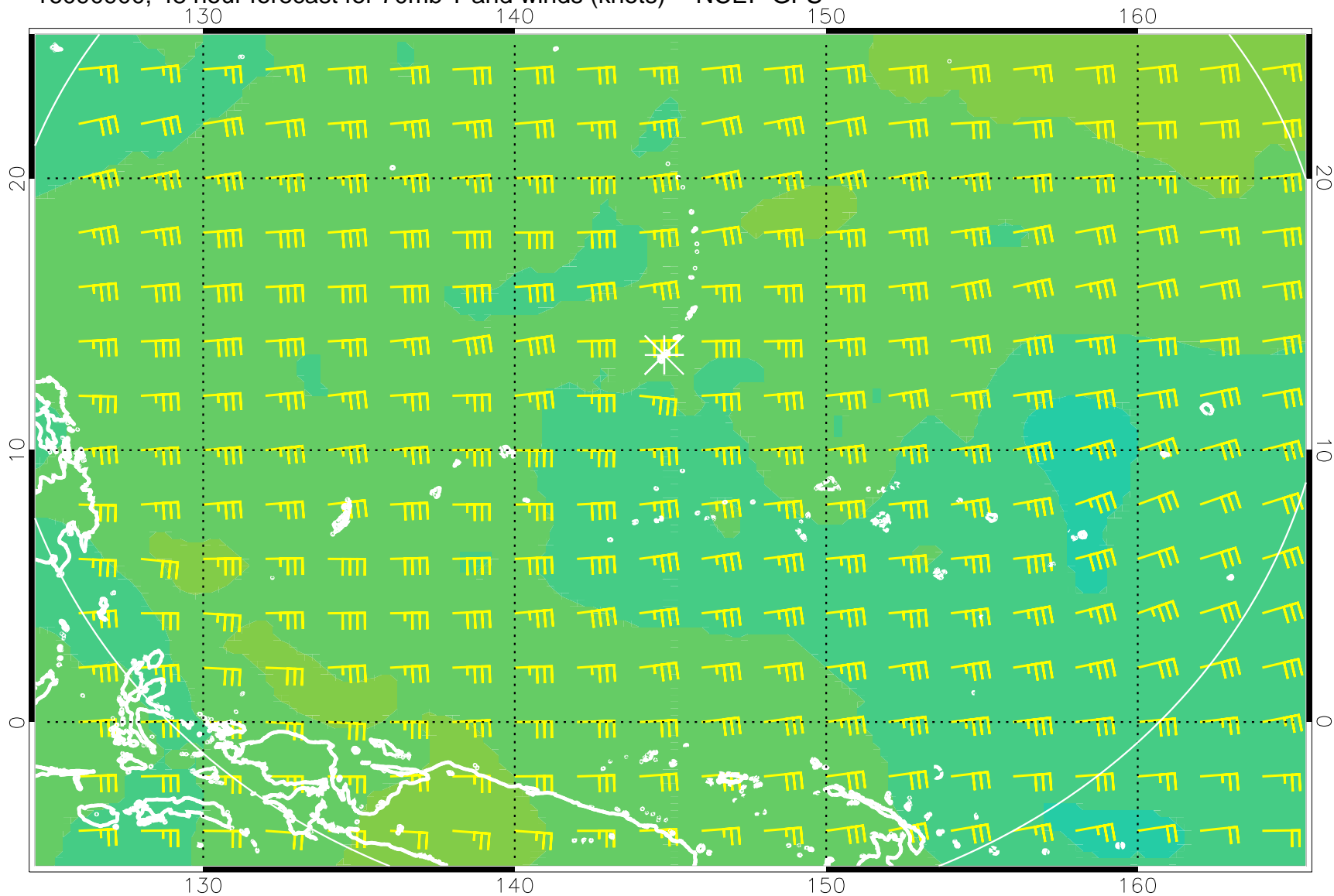
16090900, 48 hour forecast for 70mb T and winds (knots) -- NCEP GFS
