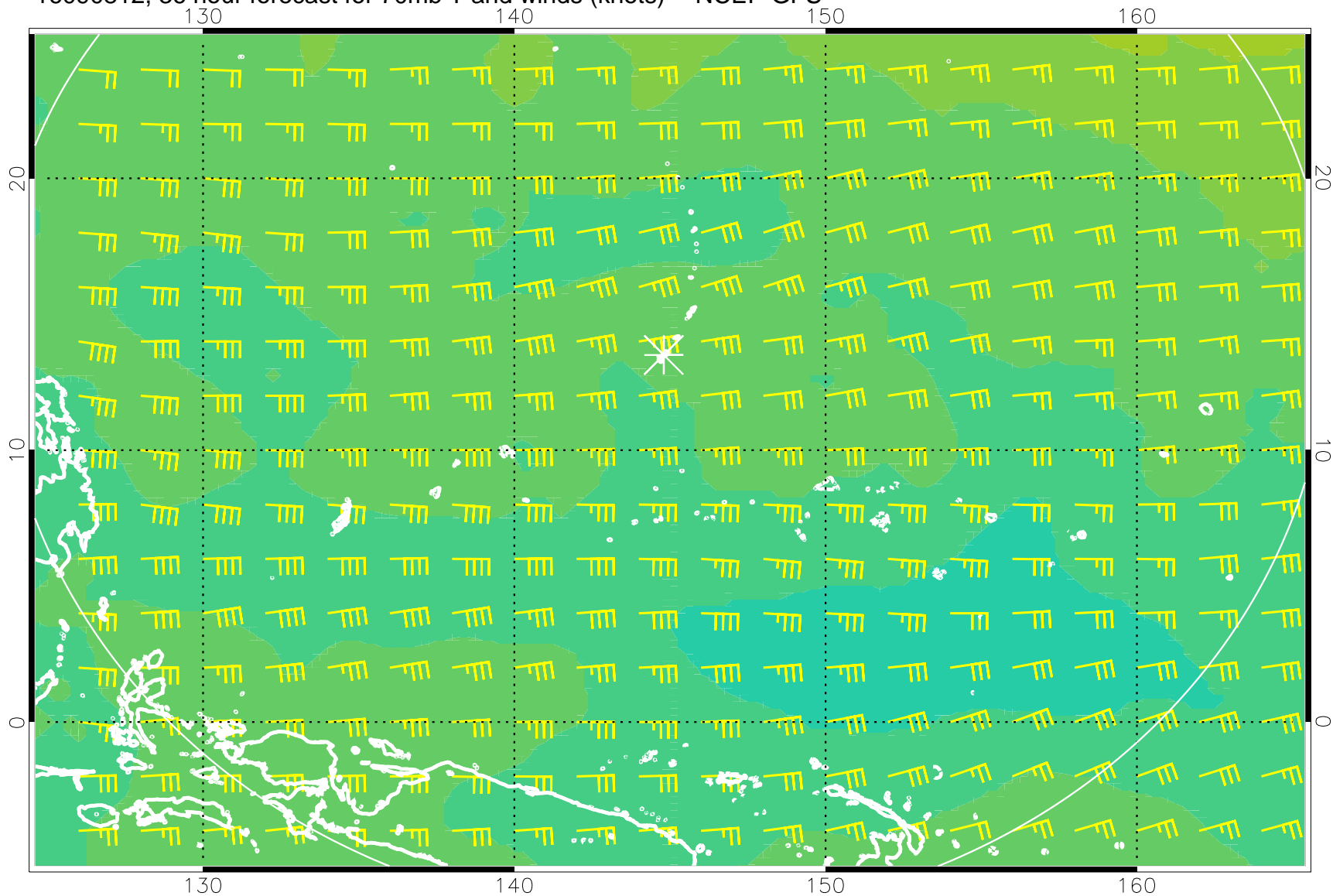
16090812, 36 hour forecast for 70mb T and winds (knots) -- NCEP GFS
