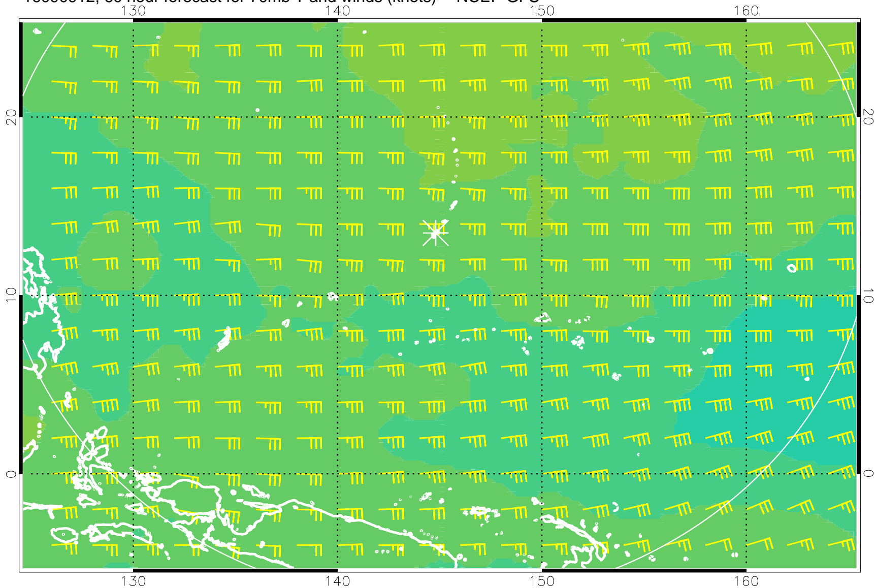
16090912, 60 hour forecast for 70mb T and winds (knots) -- NCEP GFS
