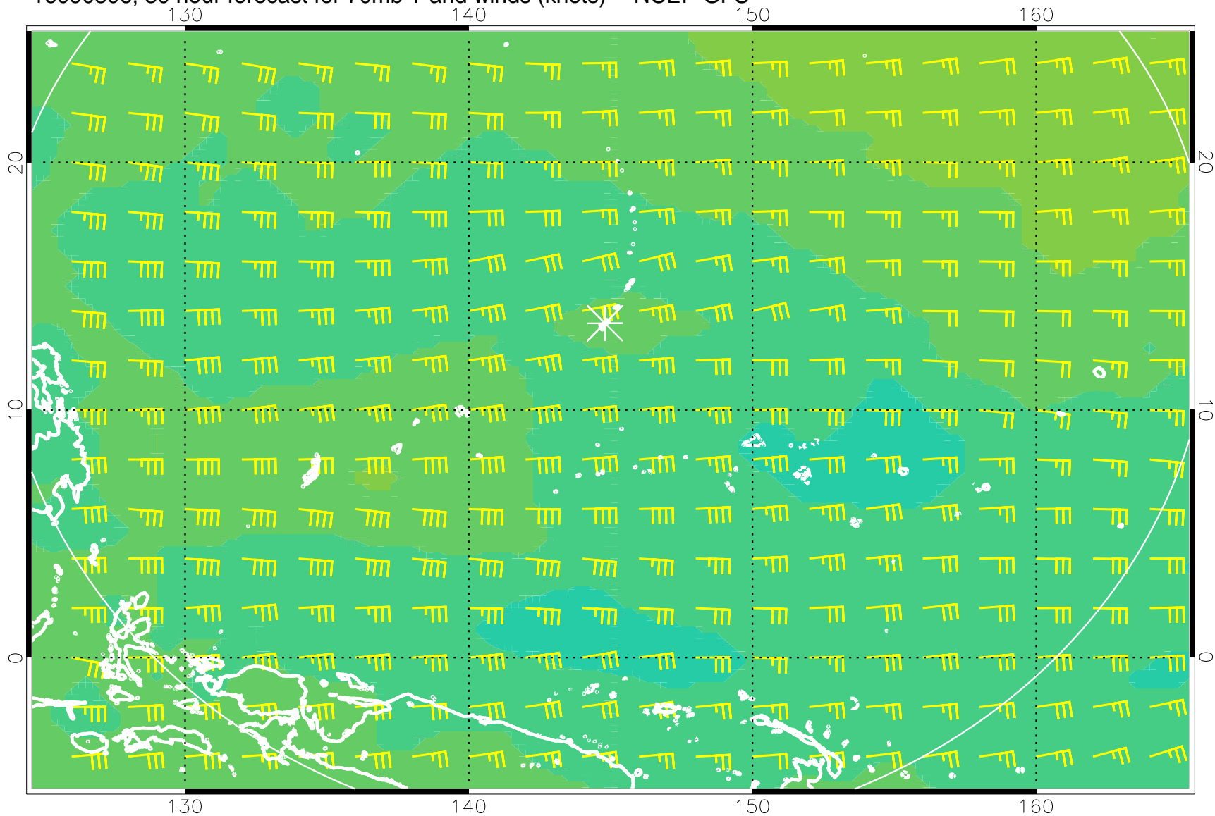
16090806, 30 hour forecast for 70mb T and winds (knots) -- NCEP GFS
