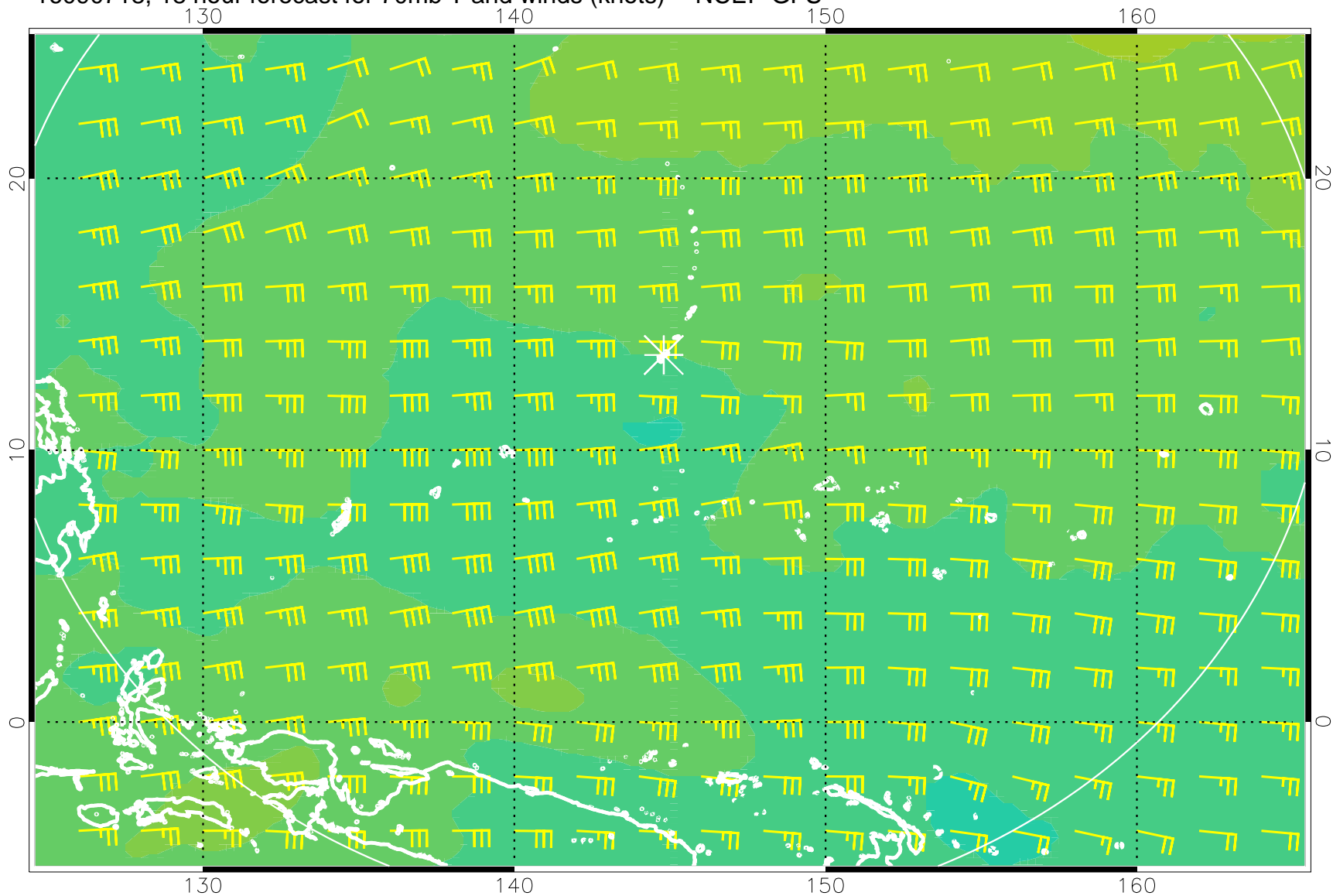
16090718, 18 hour forecast for 70mb T and winds (knots) -- NCEP GFS
