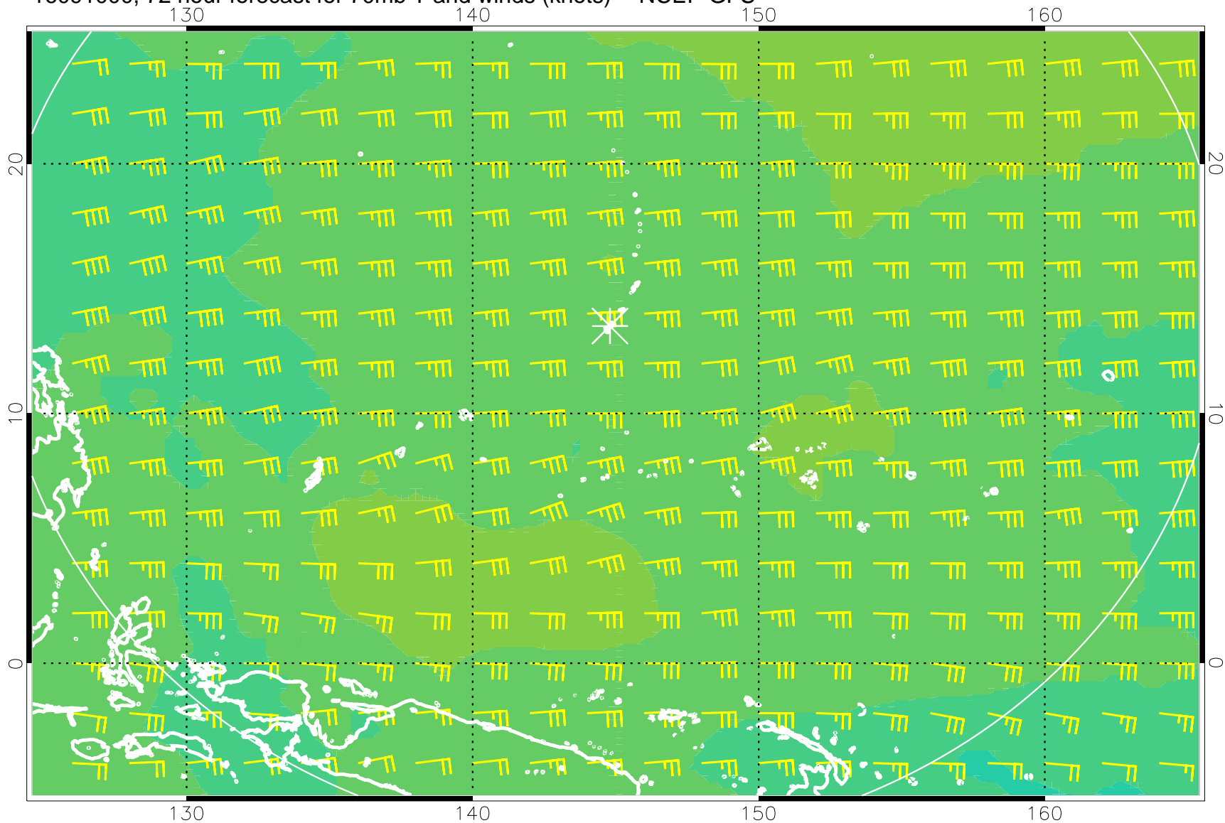
16091000, 72 hour forecast for 70mb T and winds (knots) -- NCEP GFS
