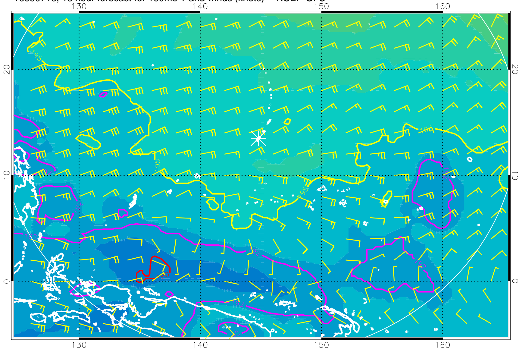
16090718, 18 hour forecast for 100mb T and winds (knots) -- NCEP GFS
