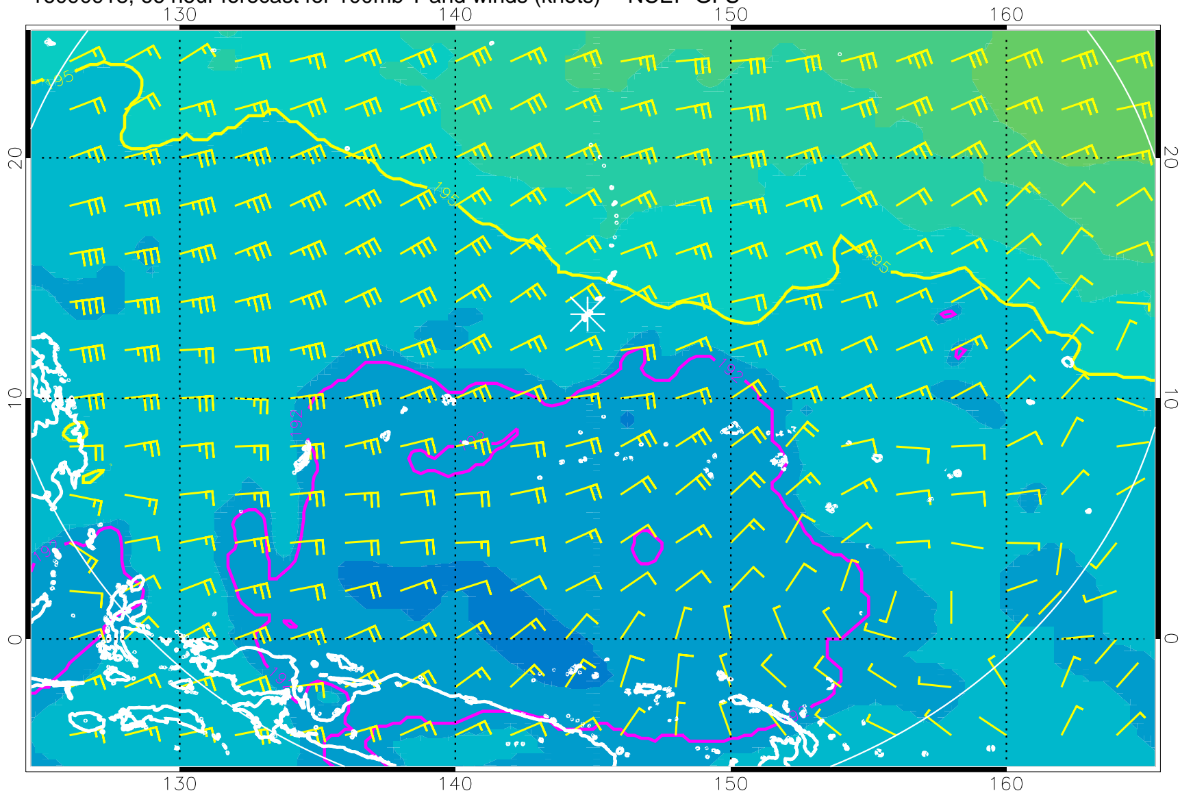
16090918, 66 hour forecast for 100mb T and winds (knots) -- NCEP GFS
