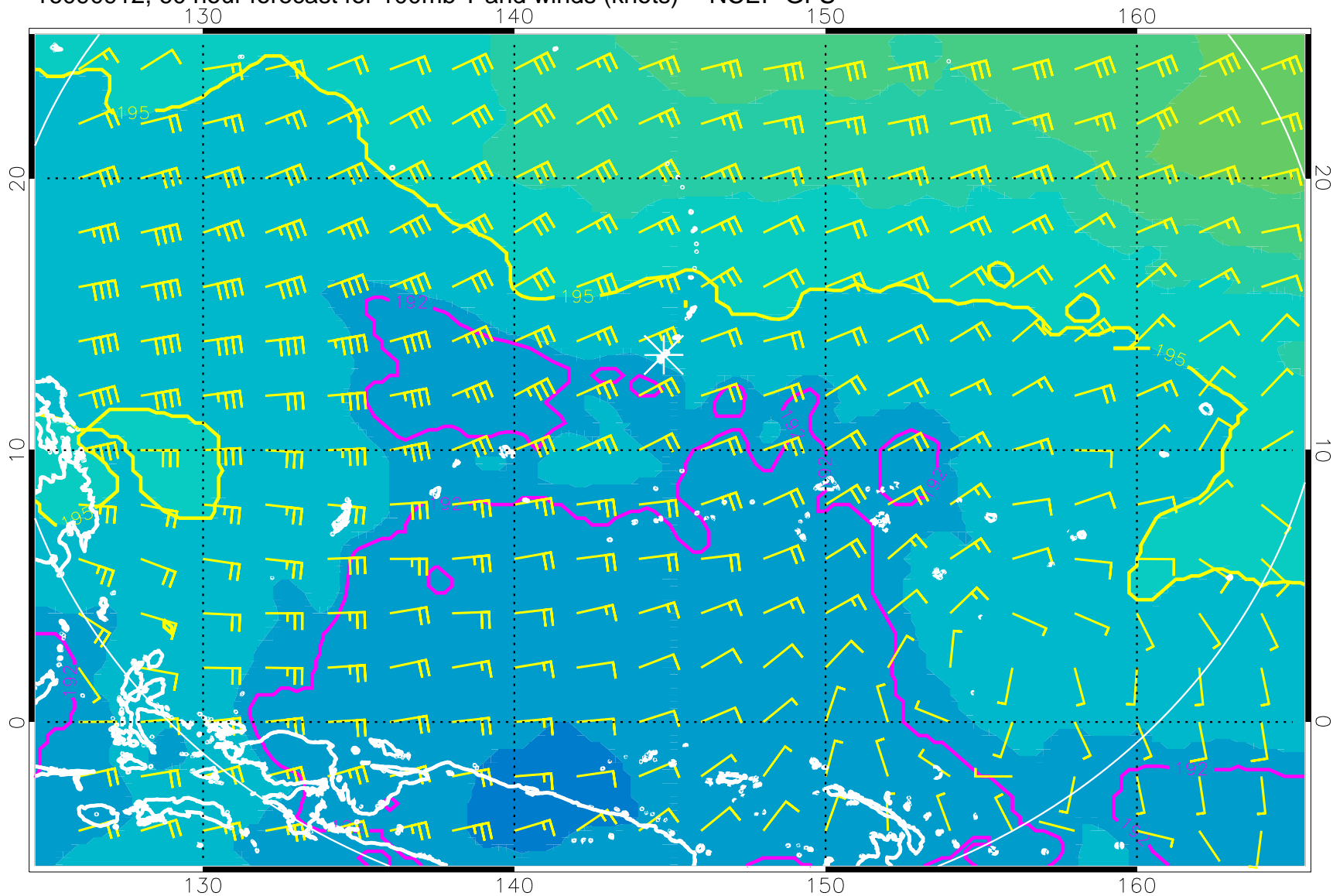
16090912, 60 hour forecast for 100mb T and winds (knots) -- NCEP GFS
