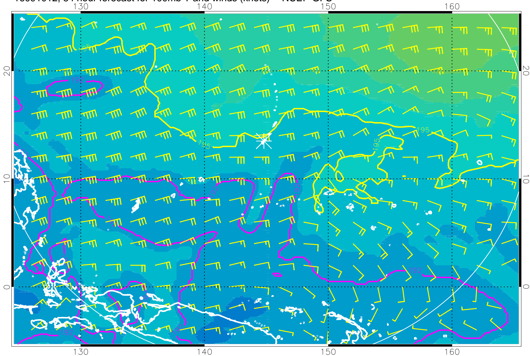
16091012, 84 hour forecast for 100mb T and winds (knots) -- NCEP GFS
