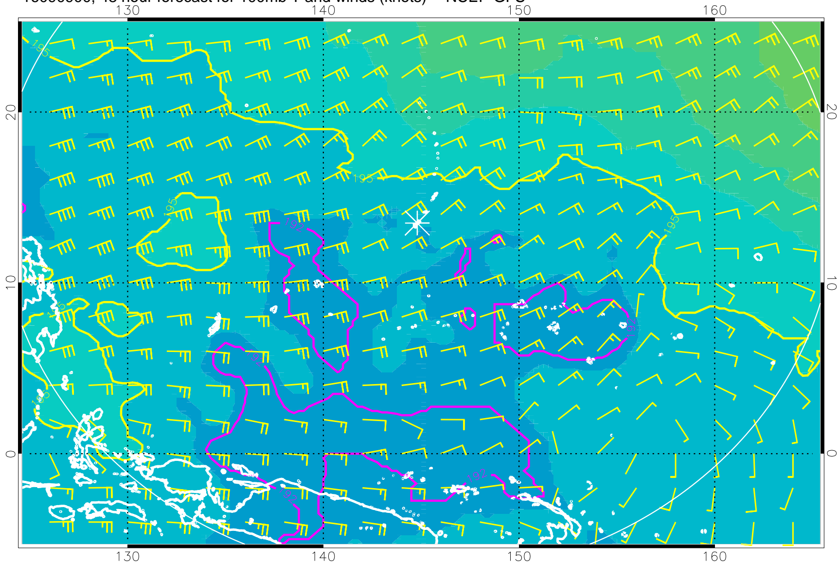
16090900, 48 hour forecast for 100mb T and winds (knots) -- NCEP GFS
