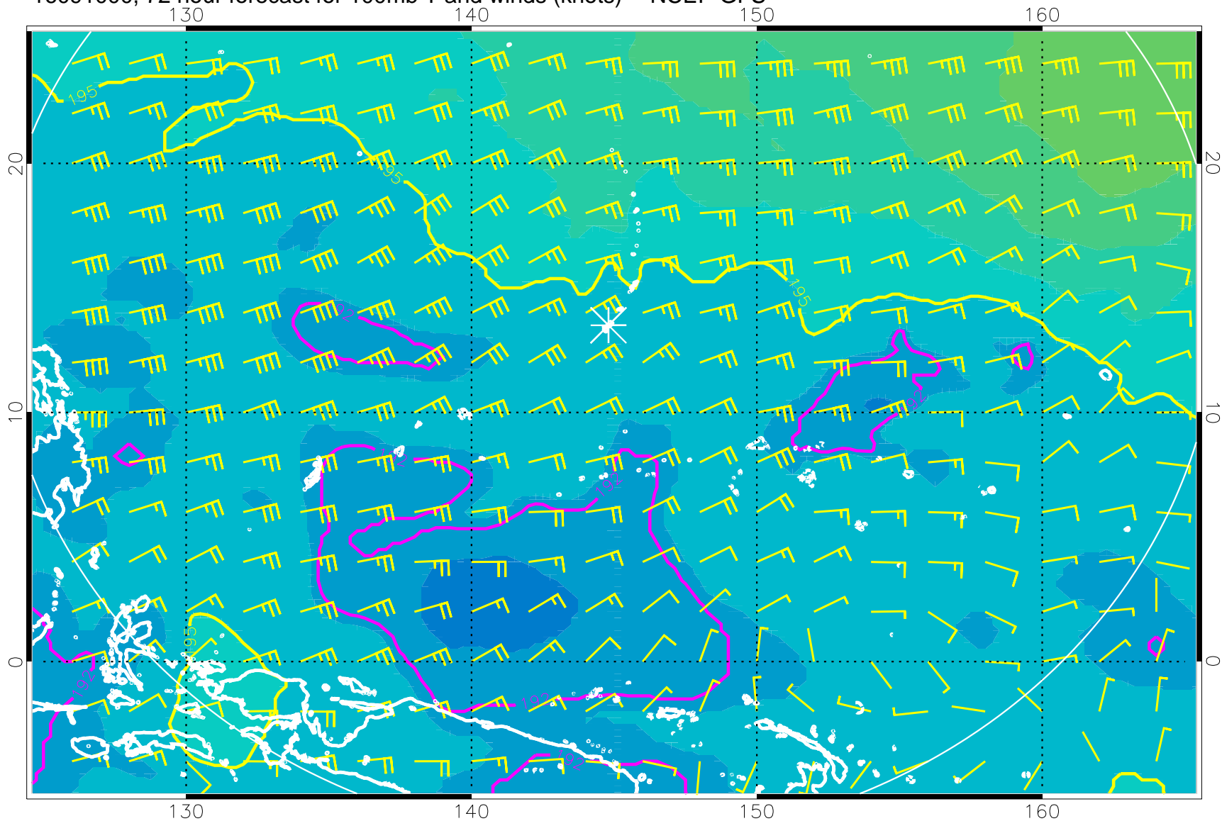
16091000, 72 hour forecast for 100mb T and winds (knots) -- NCEP GFS
