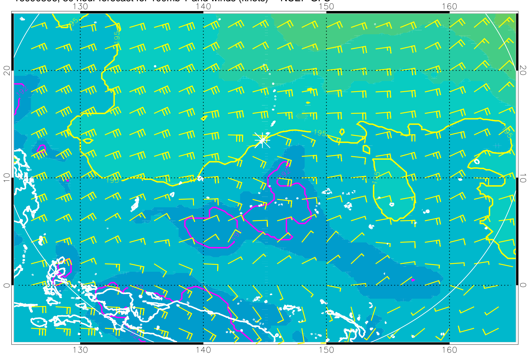
16090806, 30 hour forecast for 100mb T and winds (knots) -- NCEP GFS
