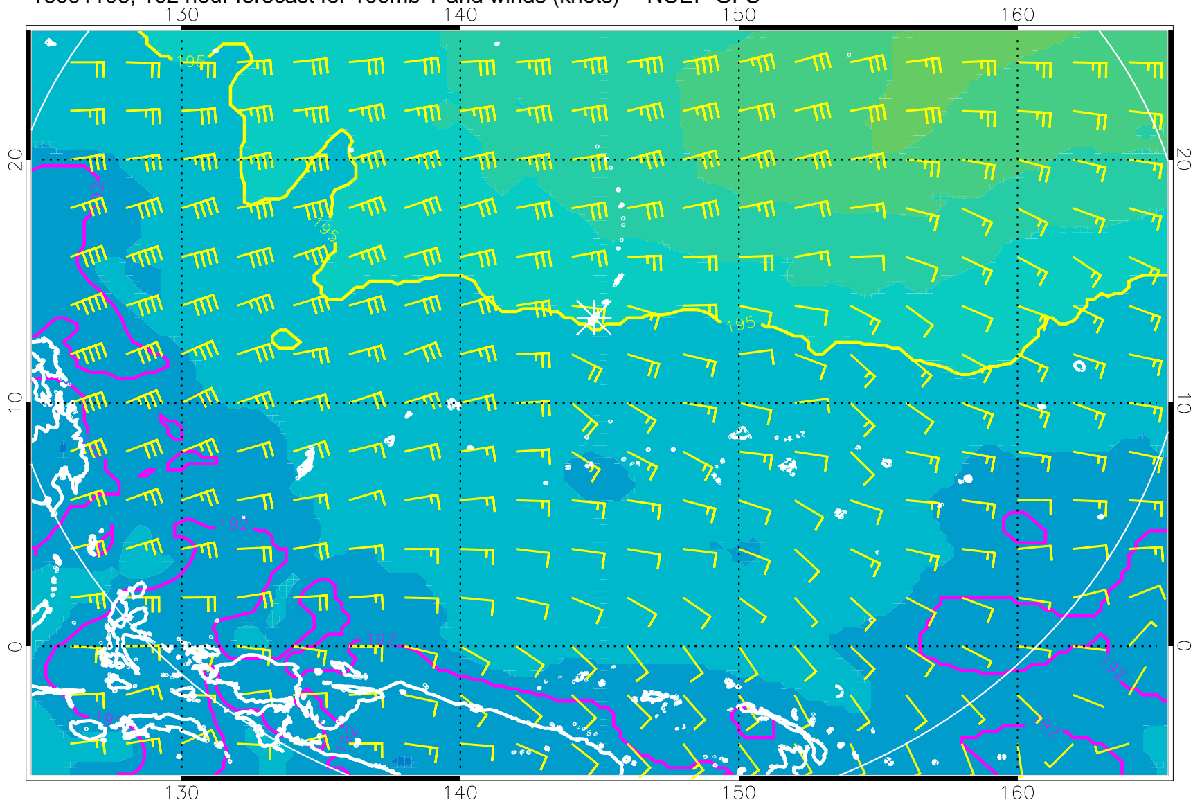
16091106, 102 hour forecast for 100mb T and winds (knots) -- NCEP GFS
