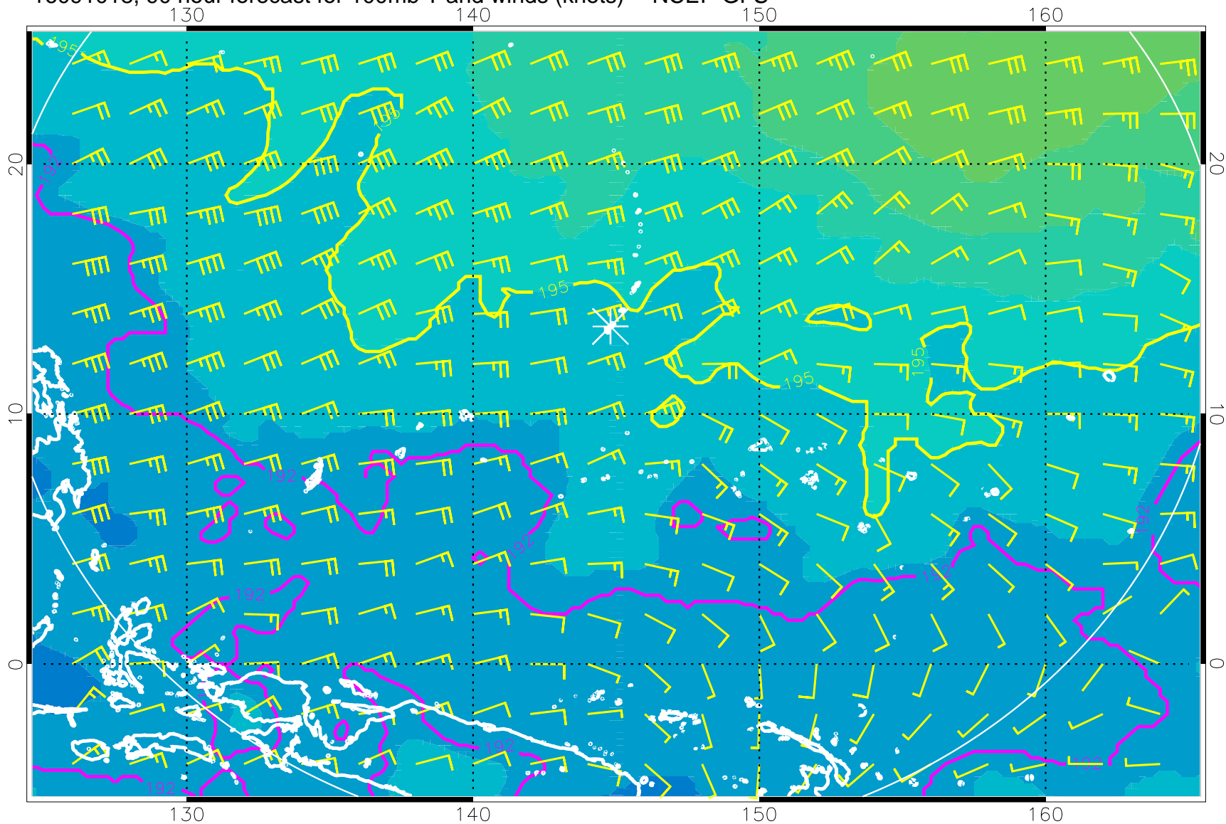
16091018, 90 hour forecast for 100mb T and winds (knots) -- NCEP GFS
