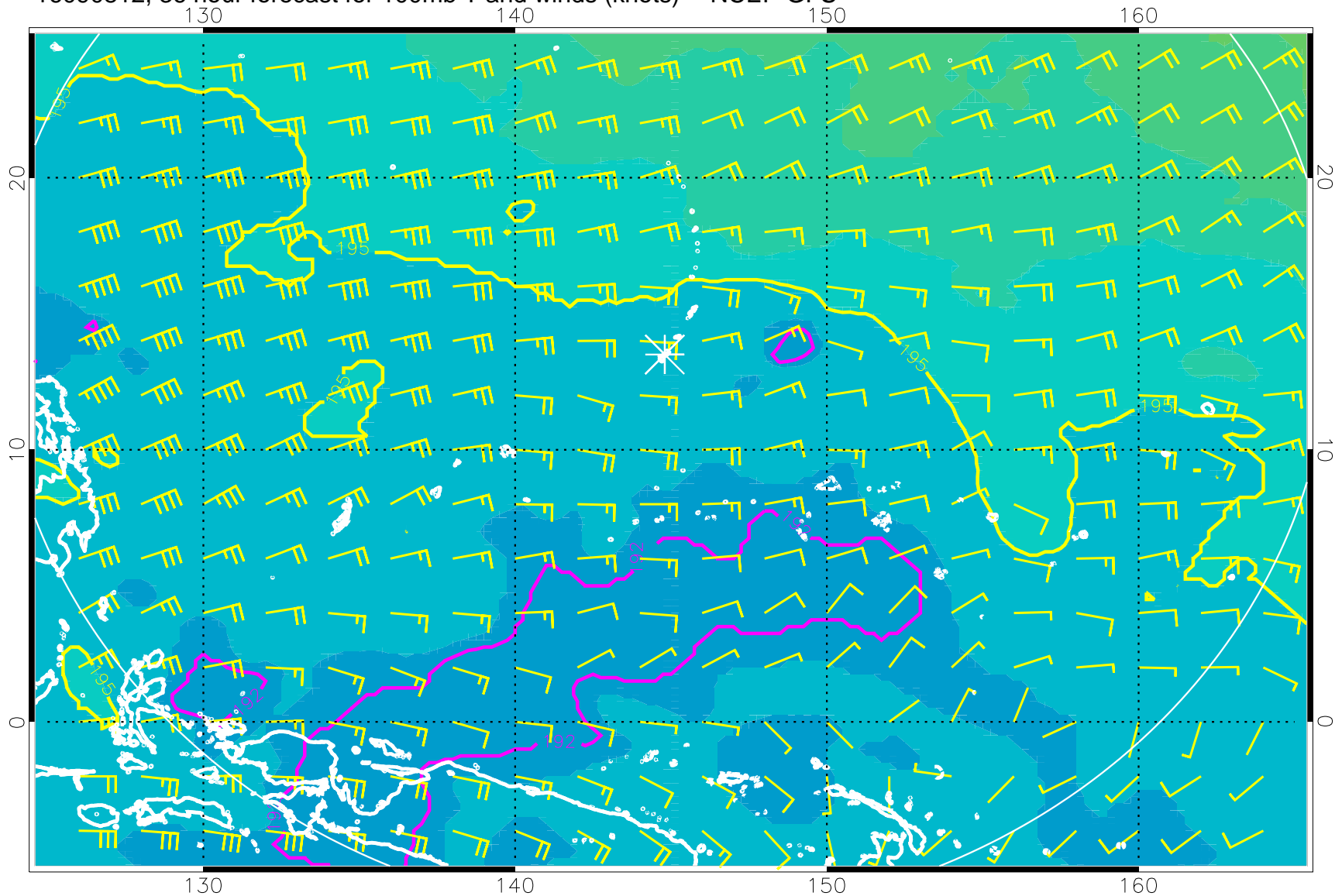
16090812, 36 hour forecast for 100mb T and winds (knots) -- NCEP GFS
