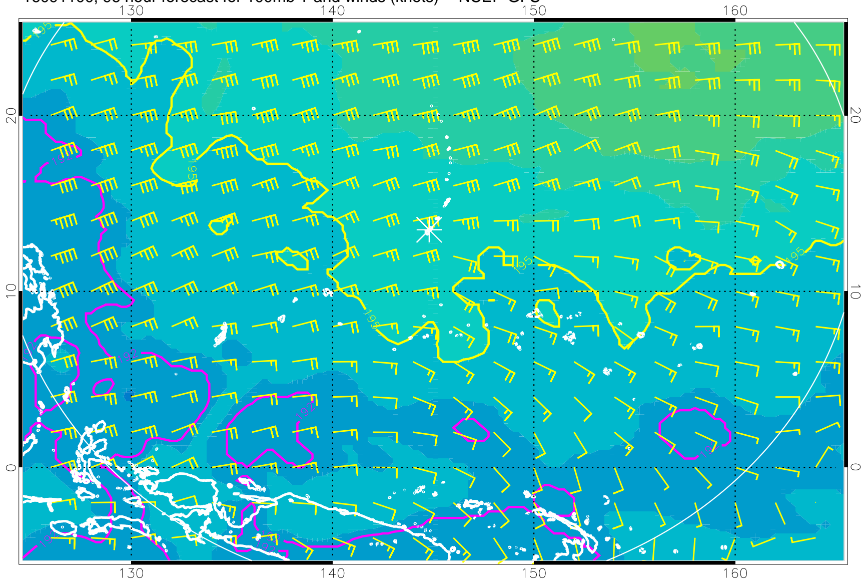
16091100, 96 hour forecast for 100mb T and winds (knots) -- NCEP GFS
