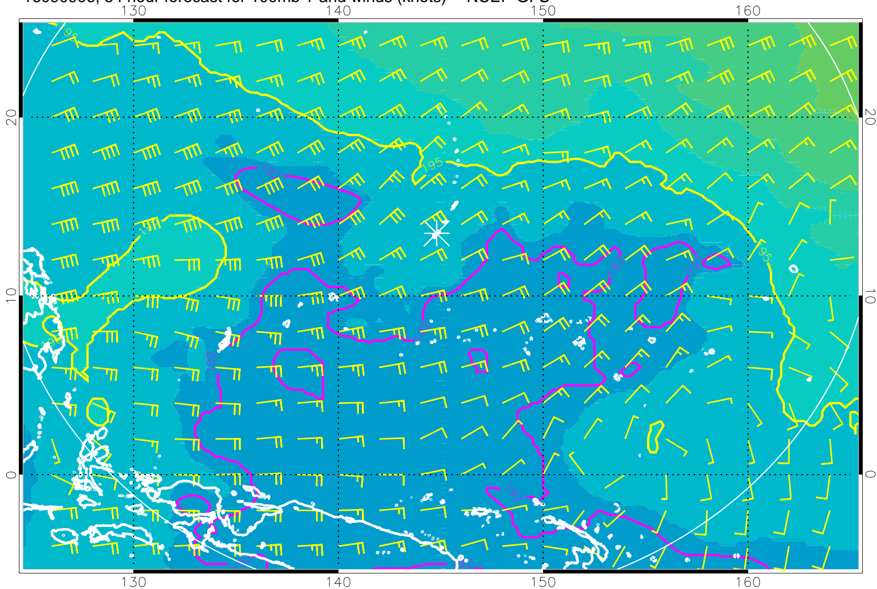
16090906, 54 hour forecast for 100mb T and winds (knots) -- NCEP GFS
