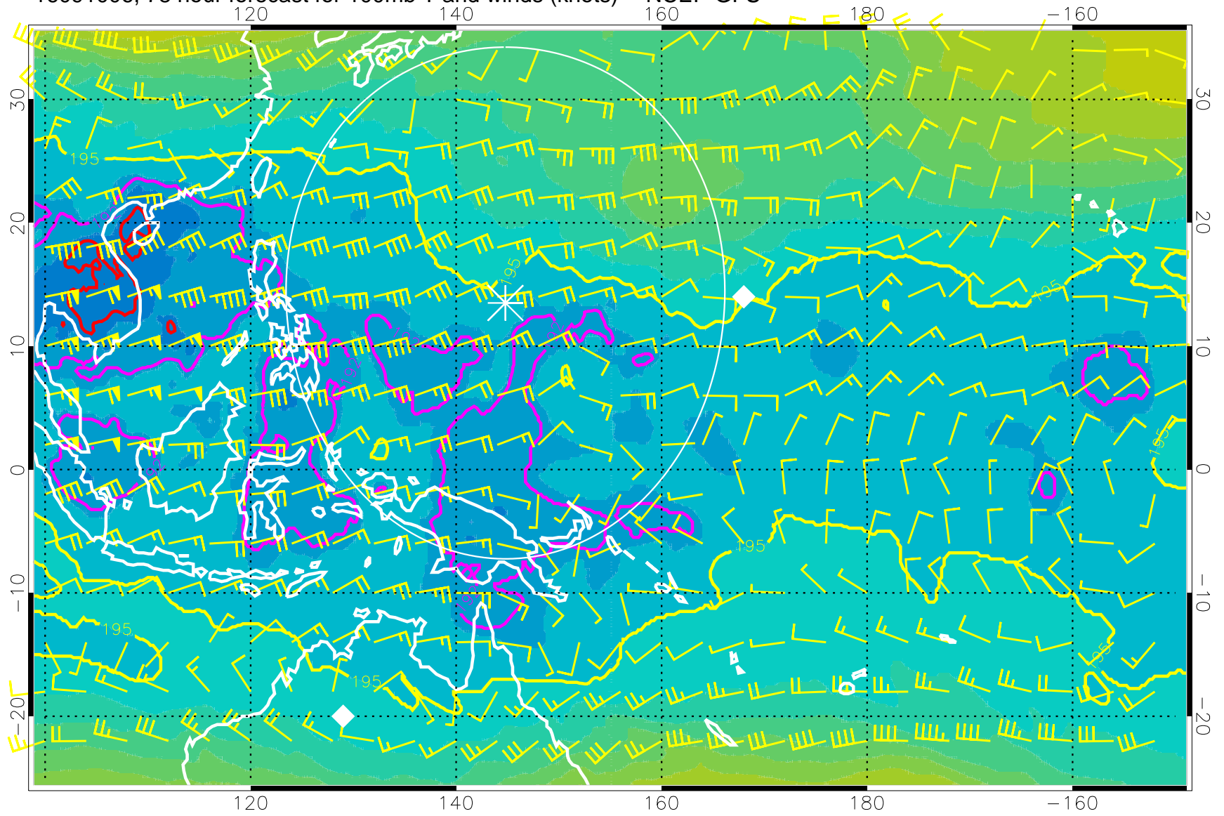
16091006, 78 hour forecast for 100mb T and winds (knots) -- NCEP GFS
