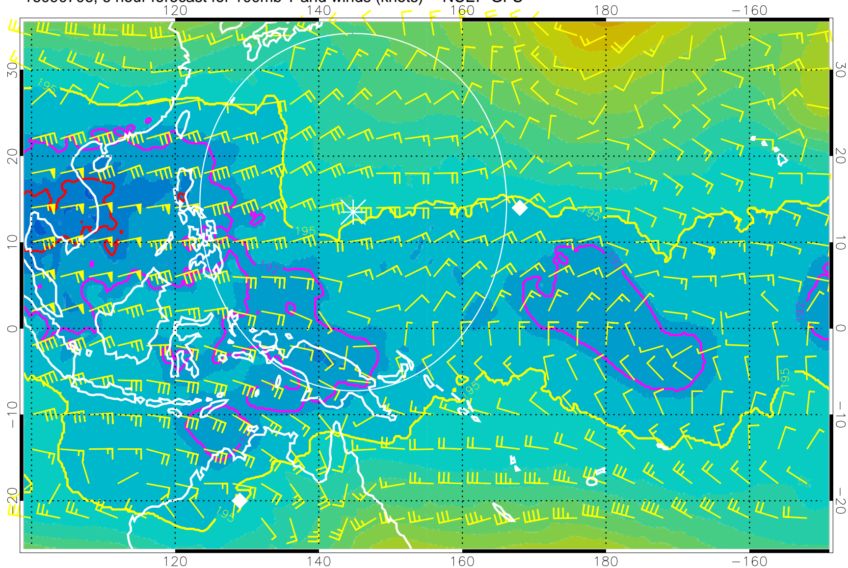
16090706, 6 hour forecast for 100mb T and winds (knots) -- NCEP GFS
