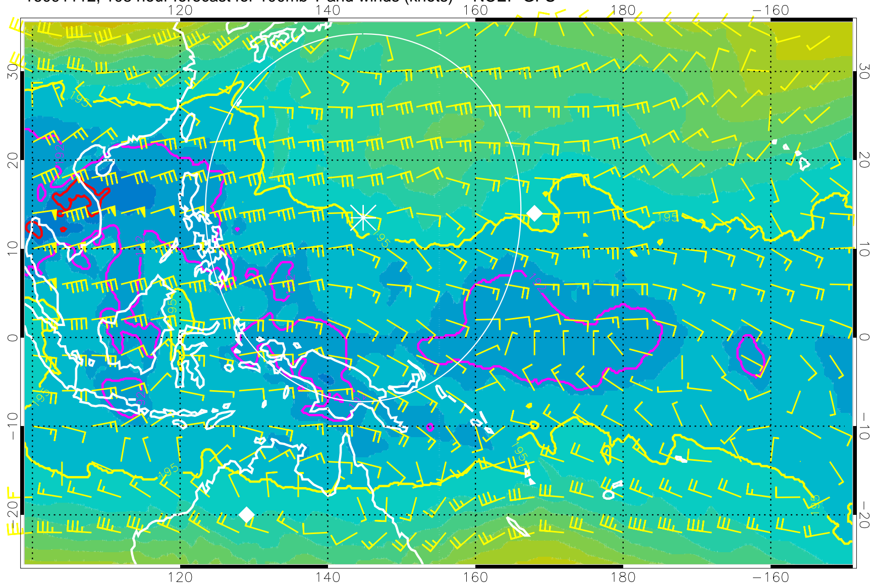
16091112, 108 hour forecast for 100mb T and winds (knots) -- NCEP GFS
