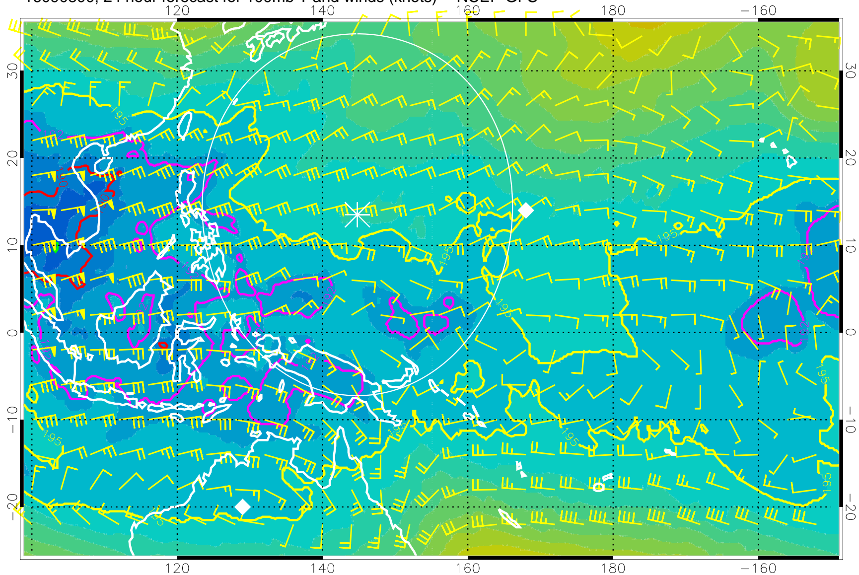
16090800, 24 hour forecast for 100mb T and winds (knots) -- NCEP GFS
