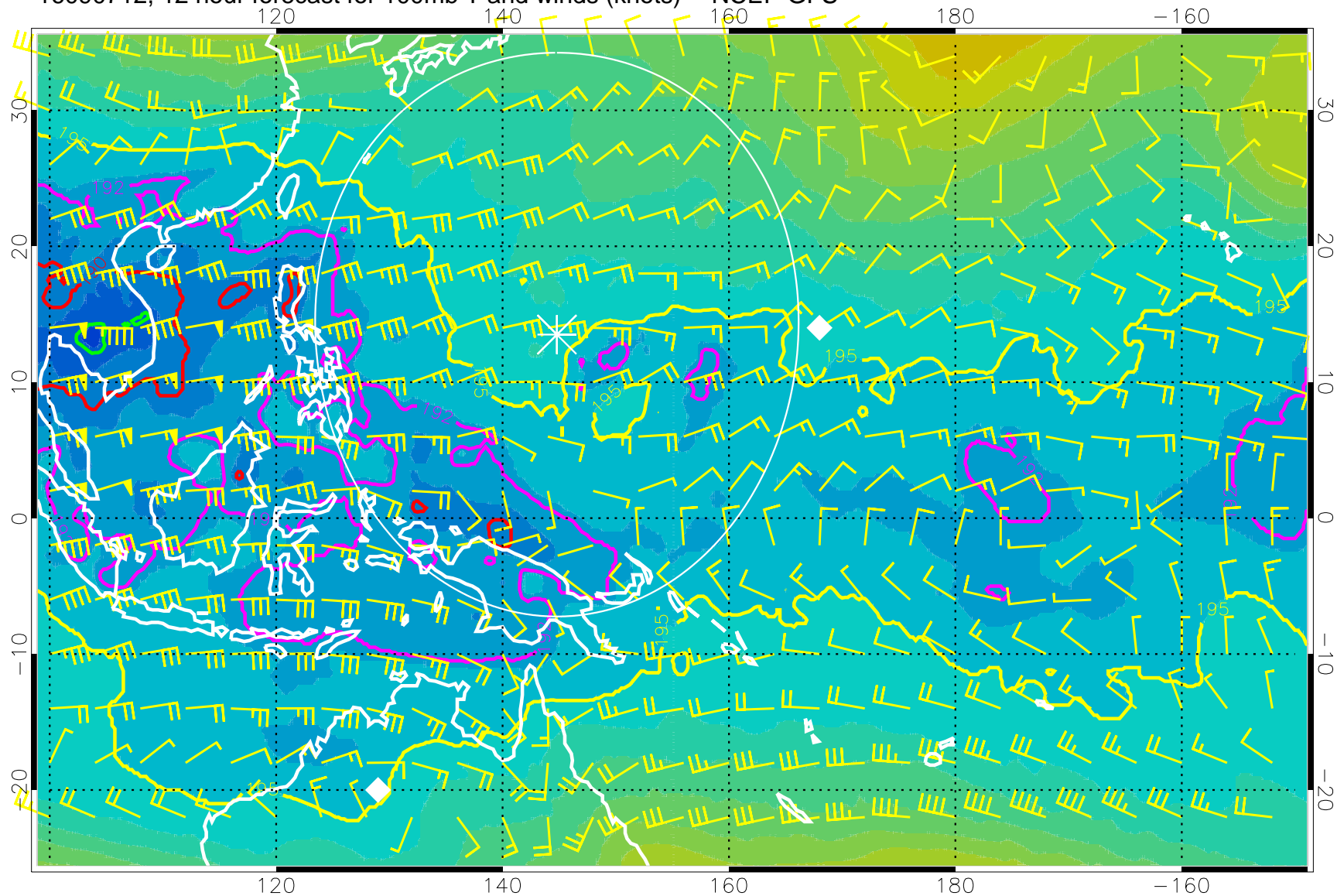
16090712, 12 hour forecast for 100mb T and winds (knots) -- NCEP GFS
