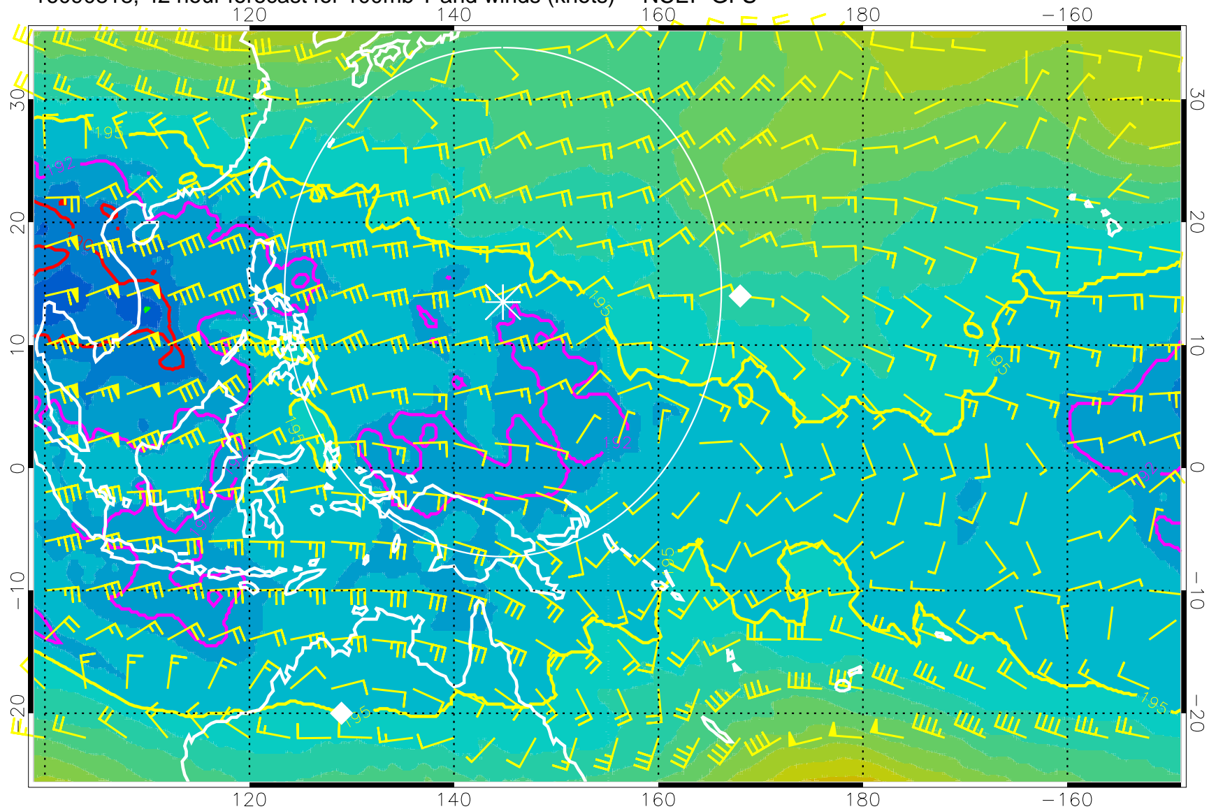
16090818, 42 hour forecast for 100mb T and winds (knots) -- NCEP GFS
