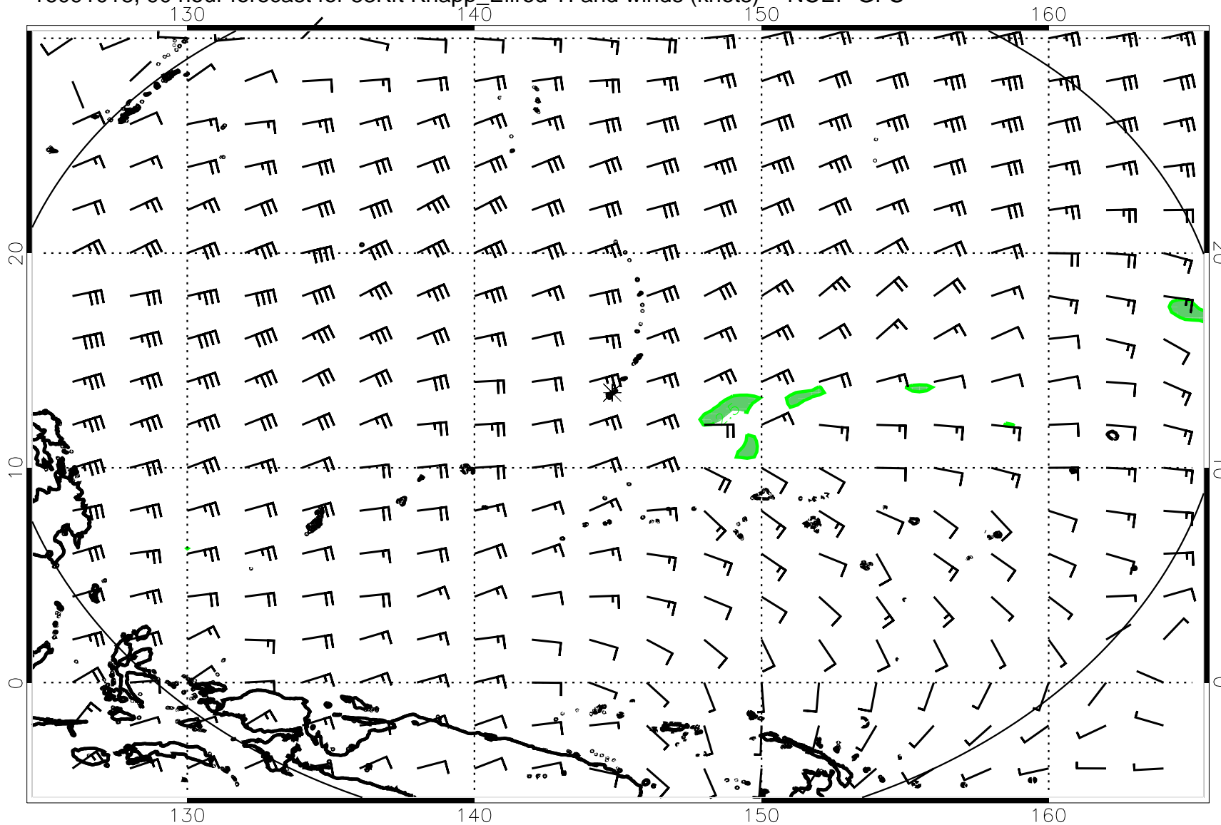
16091018, 90 hour forecast for 53Kft Knapp_Ellrod TI and winds (knots) -- NCEP GFS
