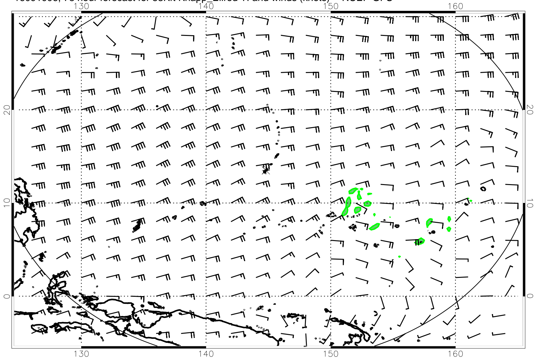
16091006, 78 hour forecast for 53Kft Knapp_Ellrod TI and winds (knots) -- NCEP GFS
