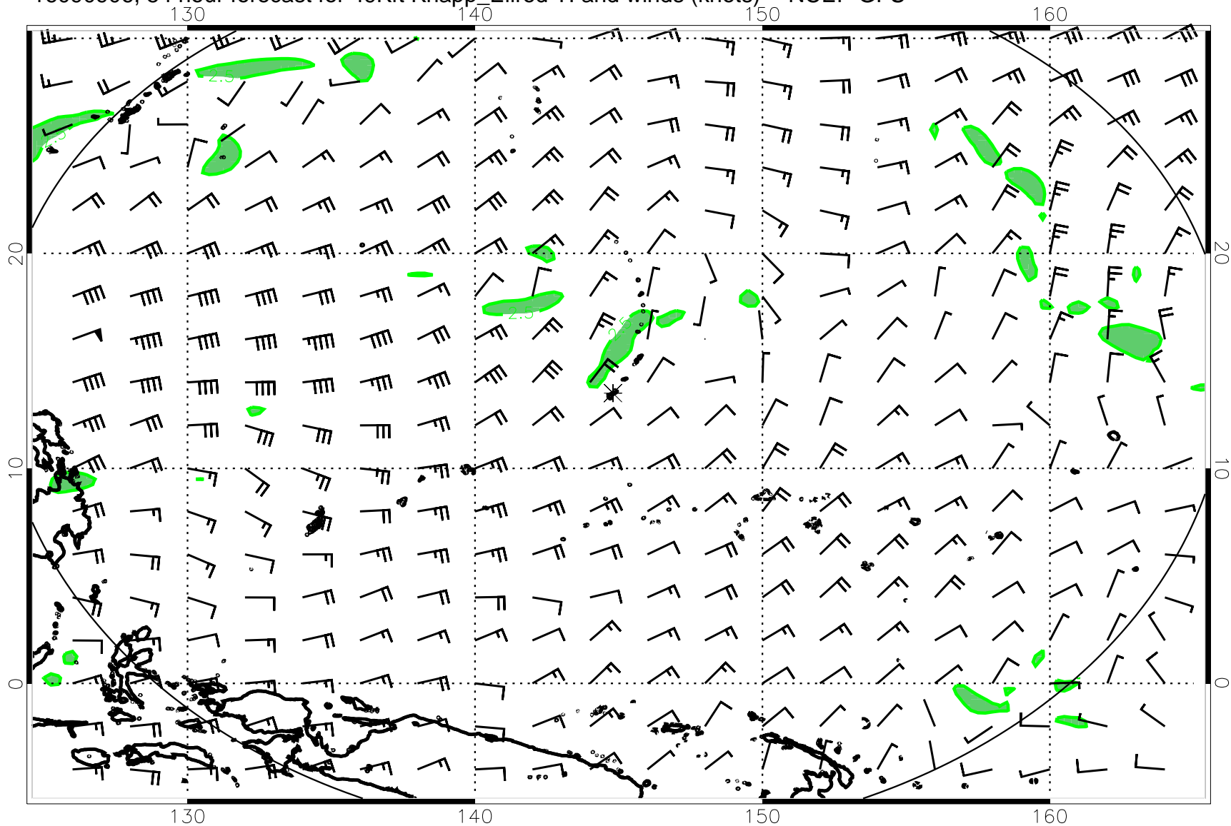
16090906, 54 hour forecast for 49Kft Knapp_Ellrod TI and winds (knots) -- NCEP GFS
