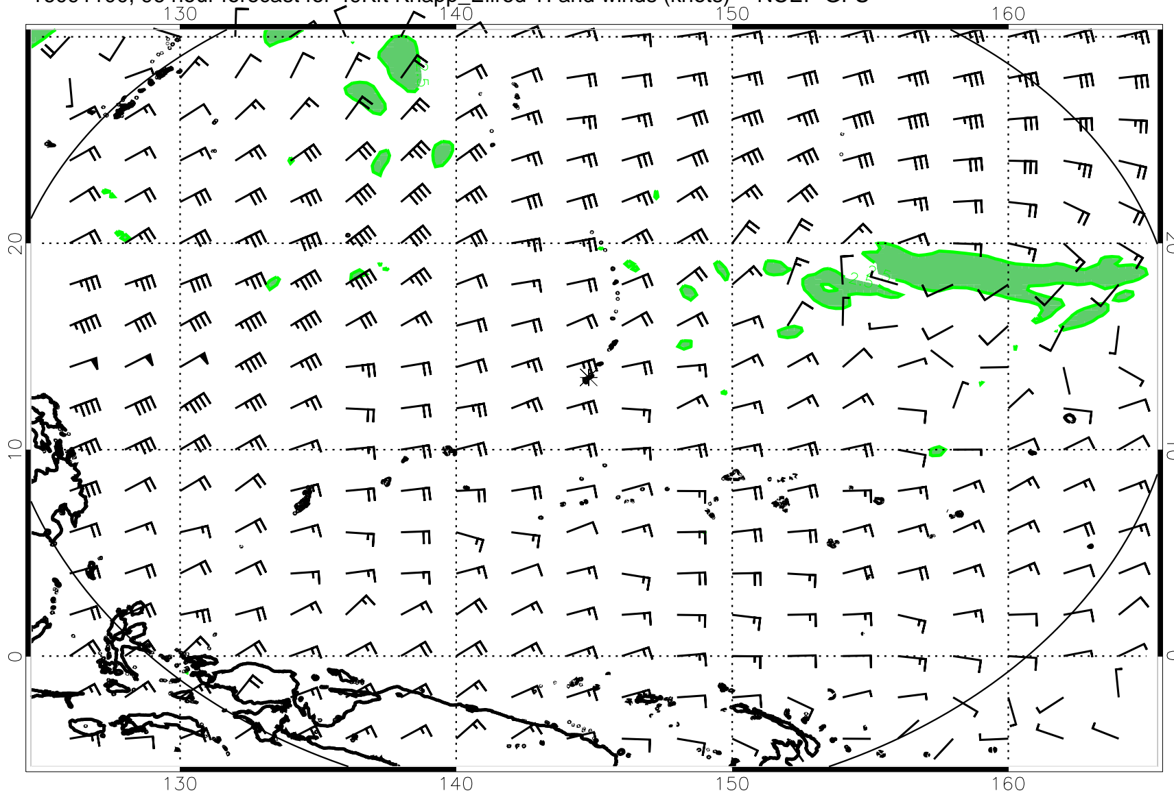
16091100, 96 hour forecast for 49Kft Knapp_Ellrod TI and winds (knots) -- NCEP GFS
