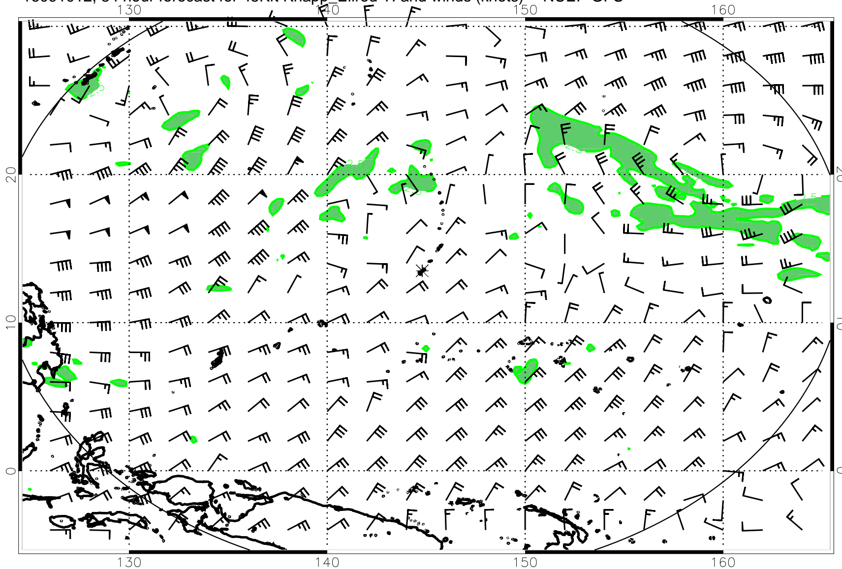
16091012, 84 hour forecast for 45Kft Knapp_Ellrod TI and winds (knots) -- NCEP GFS
