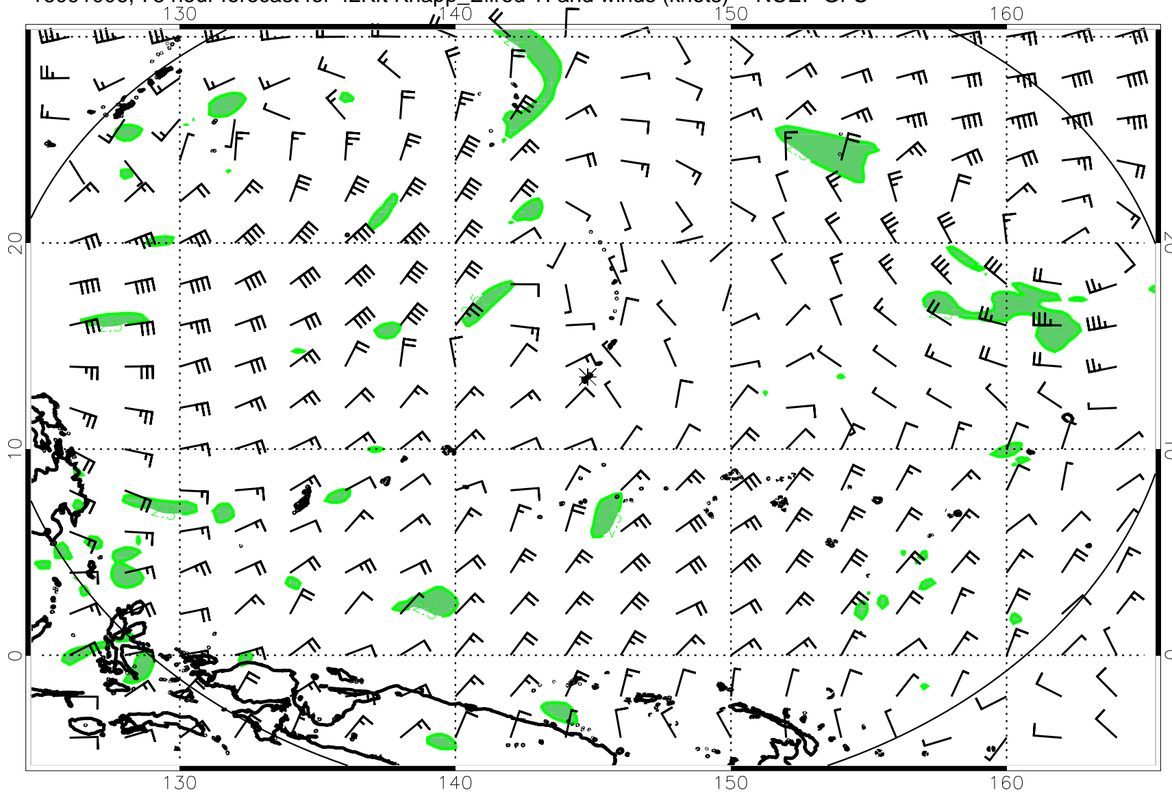
16091006, 78 hour forecast for 42Kft Knapp_Ellrod TI and winds (knots) -- NCEP GFS
