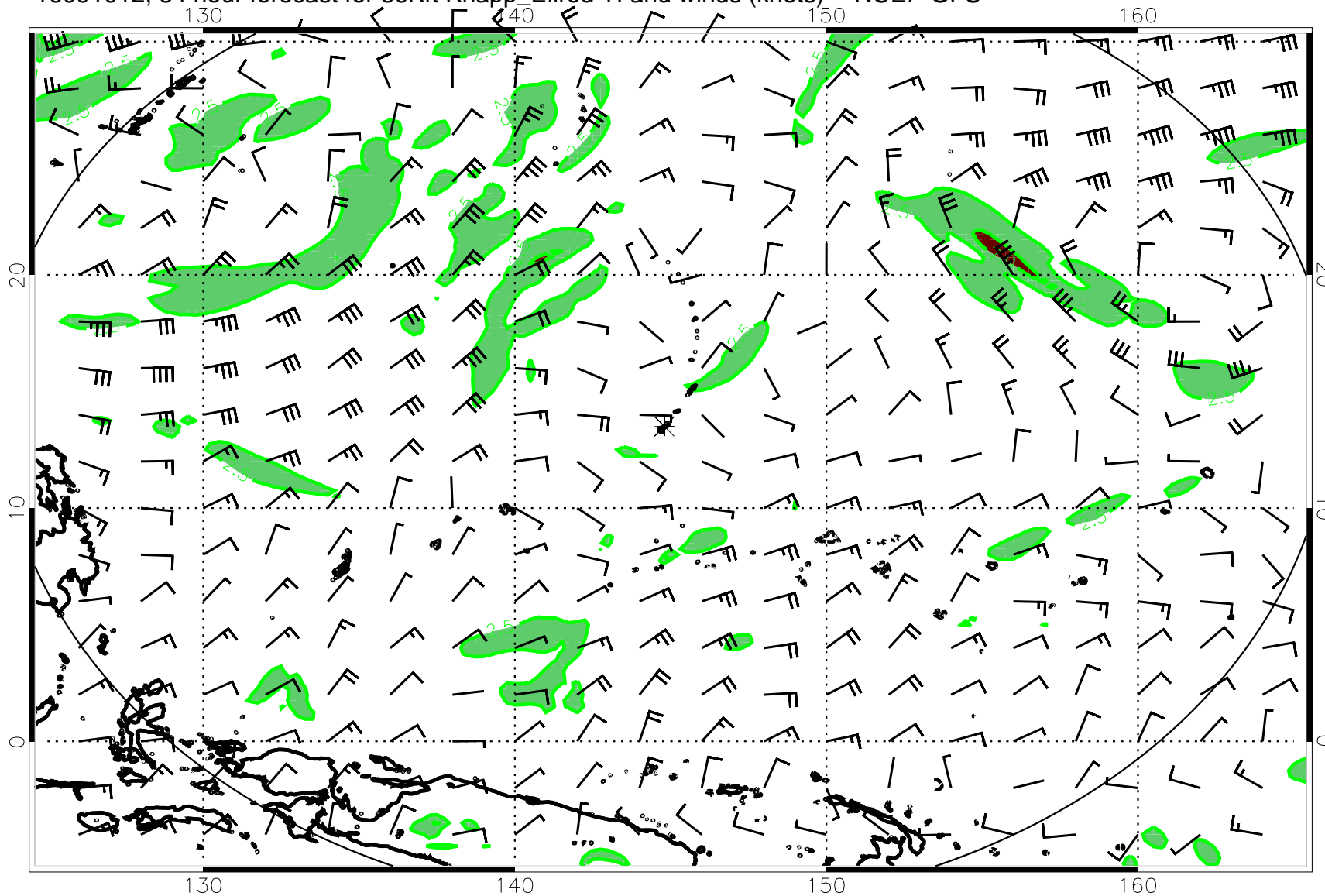
16091012, 84 hour forecast for 36Kft Knapp_Ellrod TI and winds (knots) -- NCEP GFS
