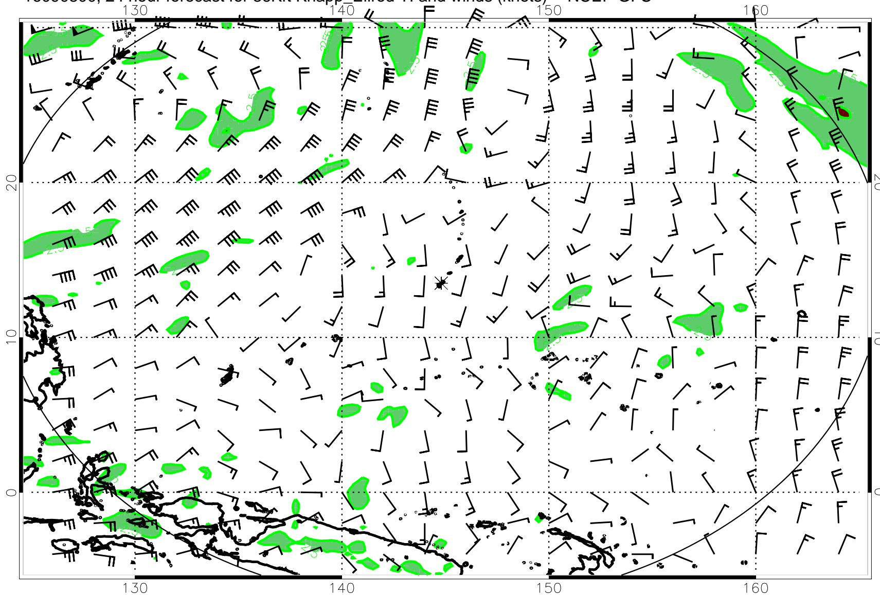
16090800, 24 hour forecast for 36Kft Knapp_Ellrod TI and winds (knots) -- NCEP GFS
