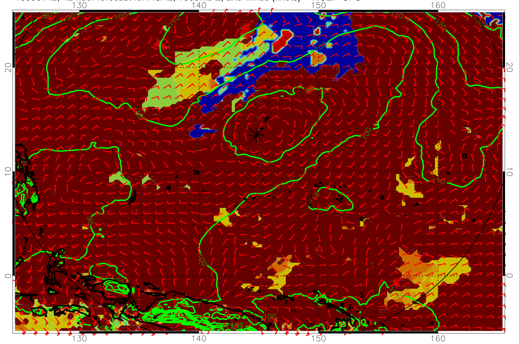
16090712, 12 hour forecast for HCAL, 1000mb Z, and winds (knots) -- NCEP GFS
