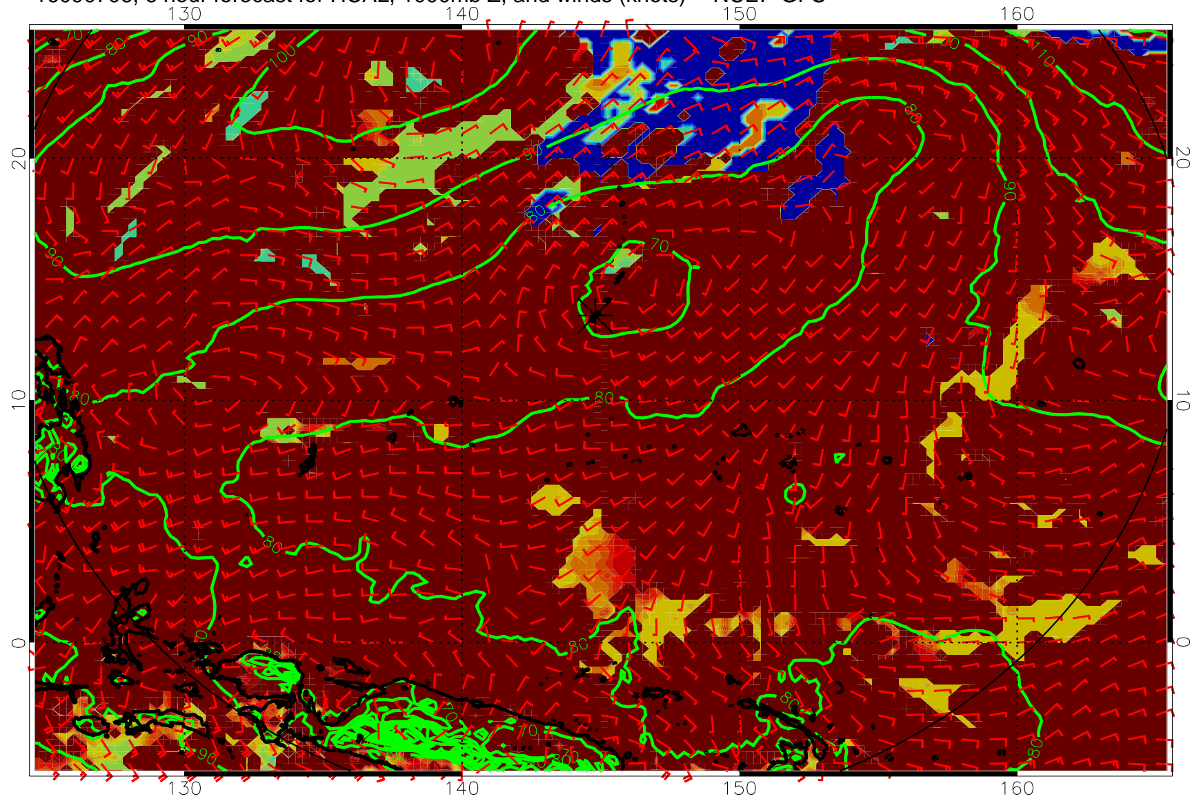
16090706, 6 hour forecast for HCAL, 1000mb Z, and winds (knots) -- NCEP GFS
