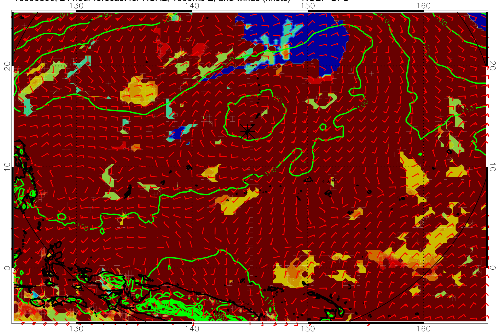
16090800, 24 hour forecast for HCAL, 1000mb Z, and winds (knots) -- NCEP GFS
