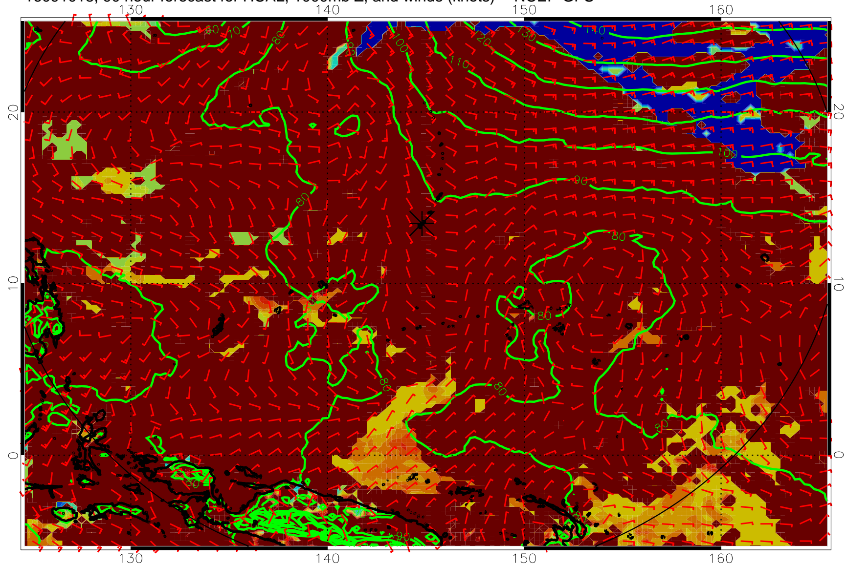
16091018, 90 hour forecast for HCAL, 1000mb Z, and winds (knots) -- NCEP GFS
