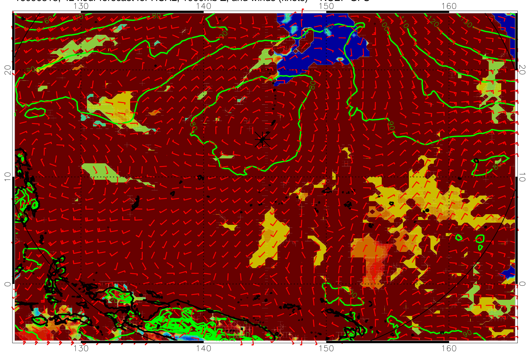
16090818, 42 hour forecast for HCAL, 1000mb Z, and winds (knots) -- NCEP GFS
