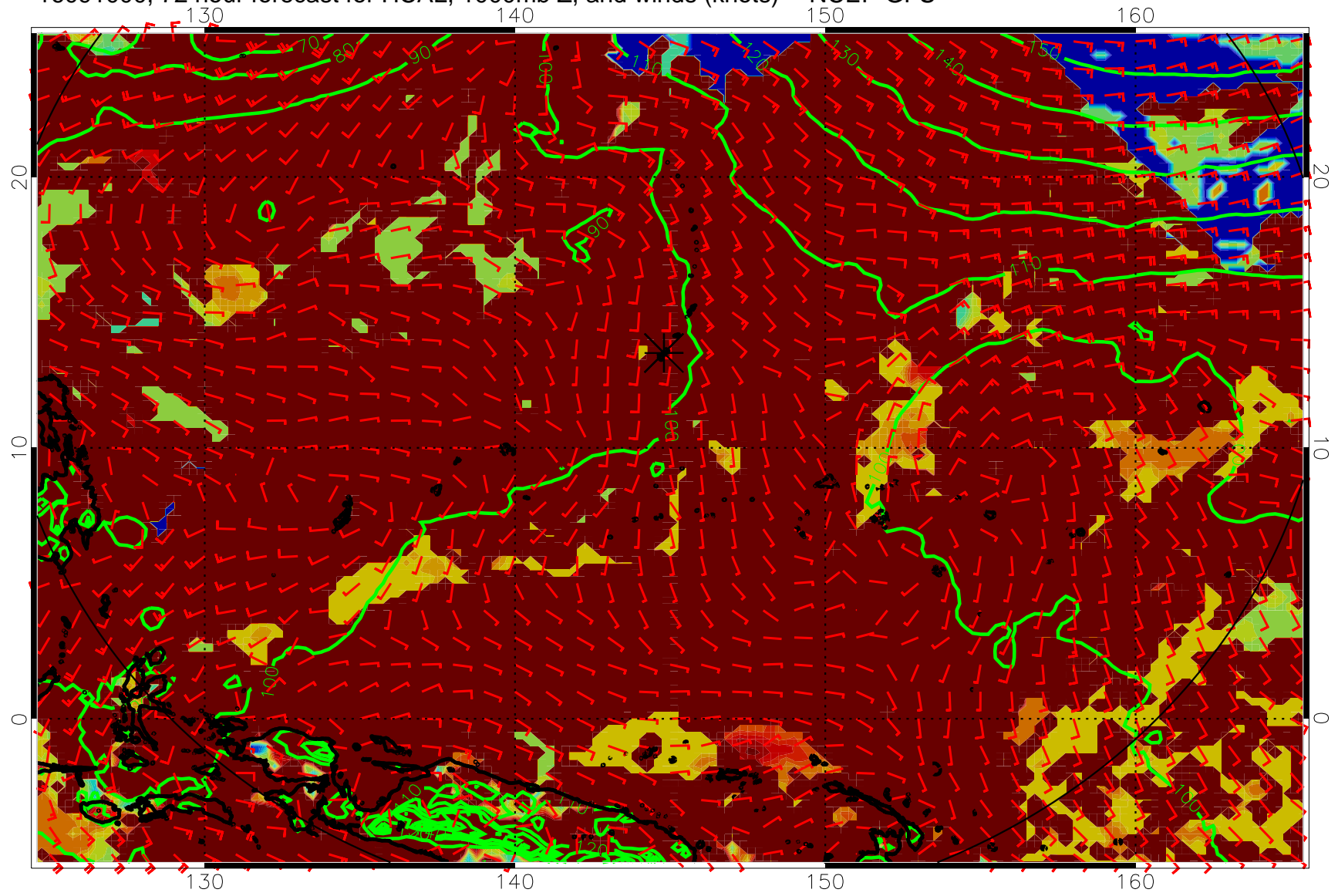
16091000, 72 hour forecast for HCAL, 1000mb Z, and winds (knots) -- NCEP GFS
