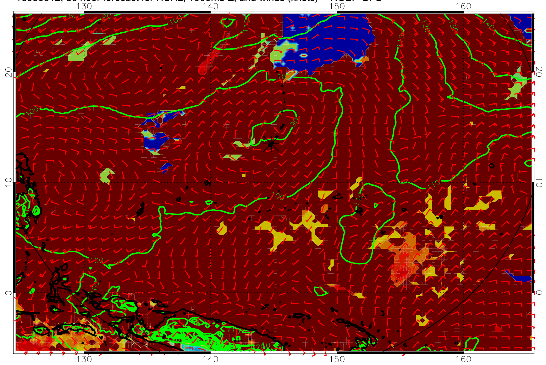
16090812, 36 hour forecast for HCAL, 1000mb Z, and winds (knots) -- NCEP GFS
