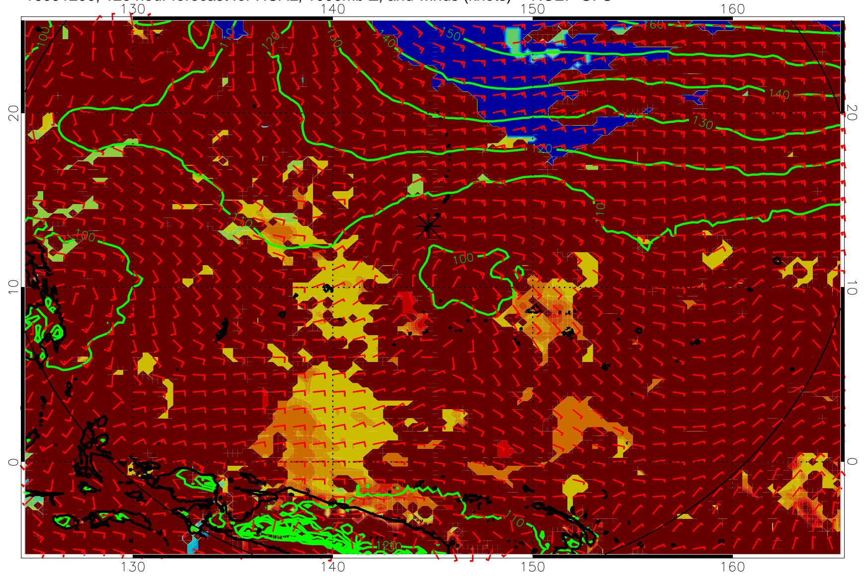
16091200, 120 hour forecast for HCAL, 1000mb Z, and winds (knots) -- NCEP GFS
