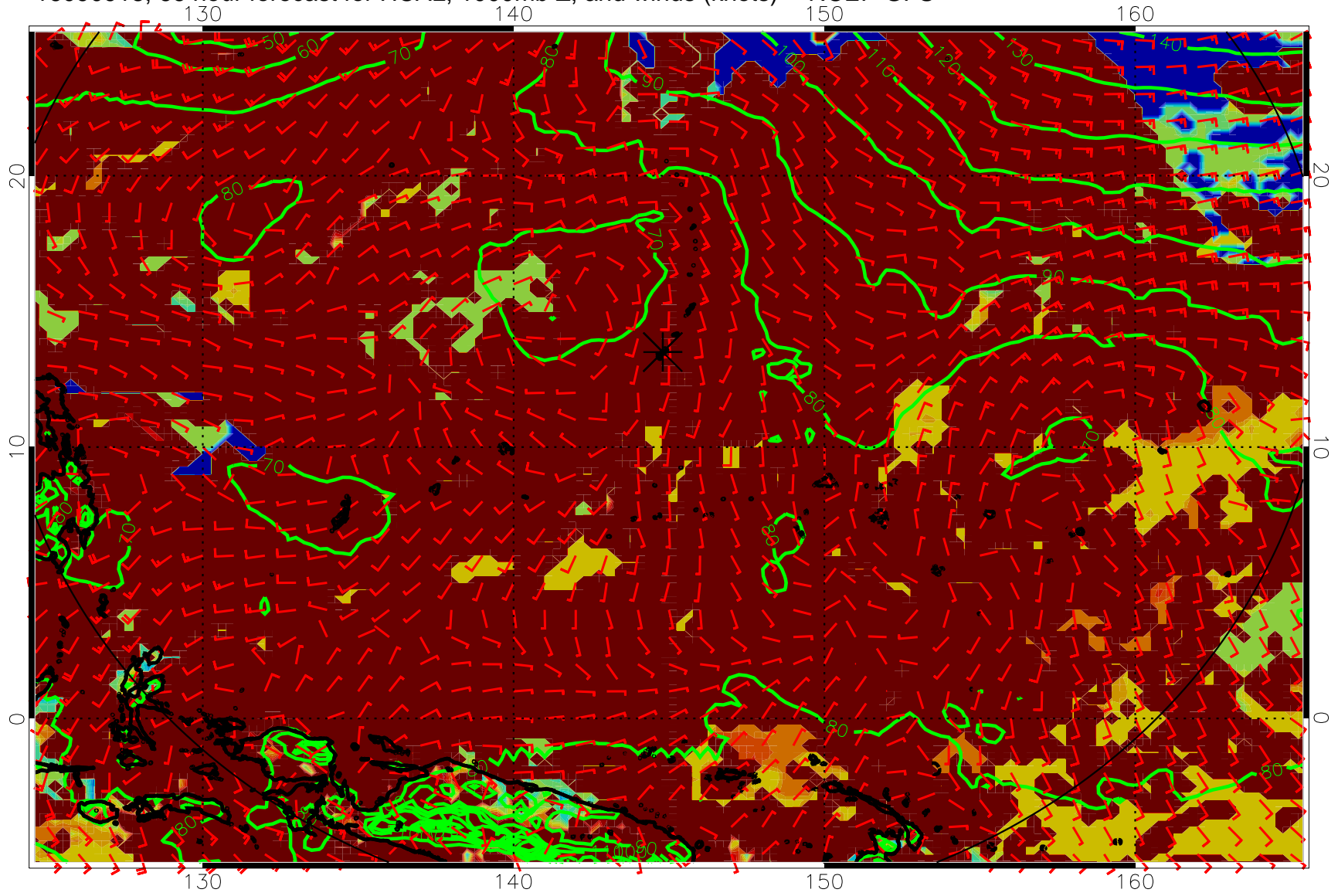
16090918, 66 hour forecast for HCAL, 1000mb Z, and winds (knots) -- NCEP GFS
