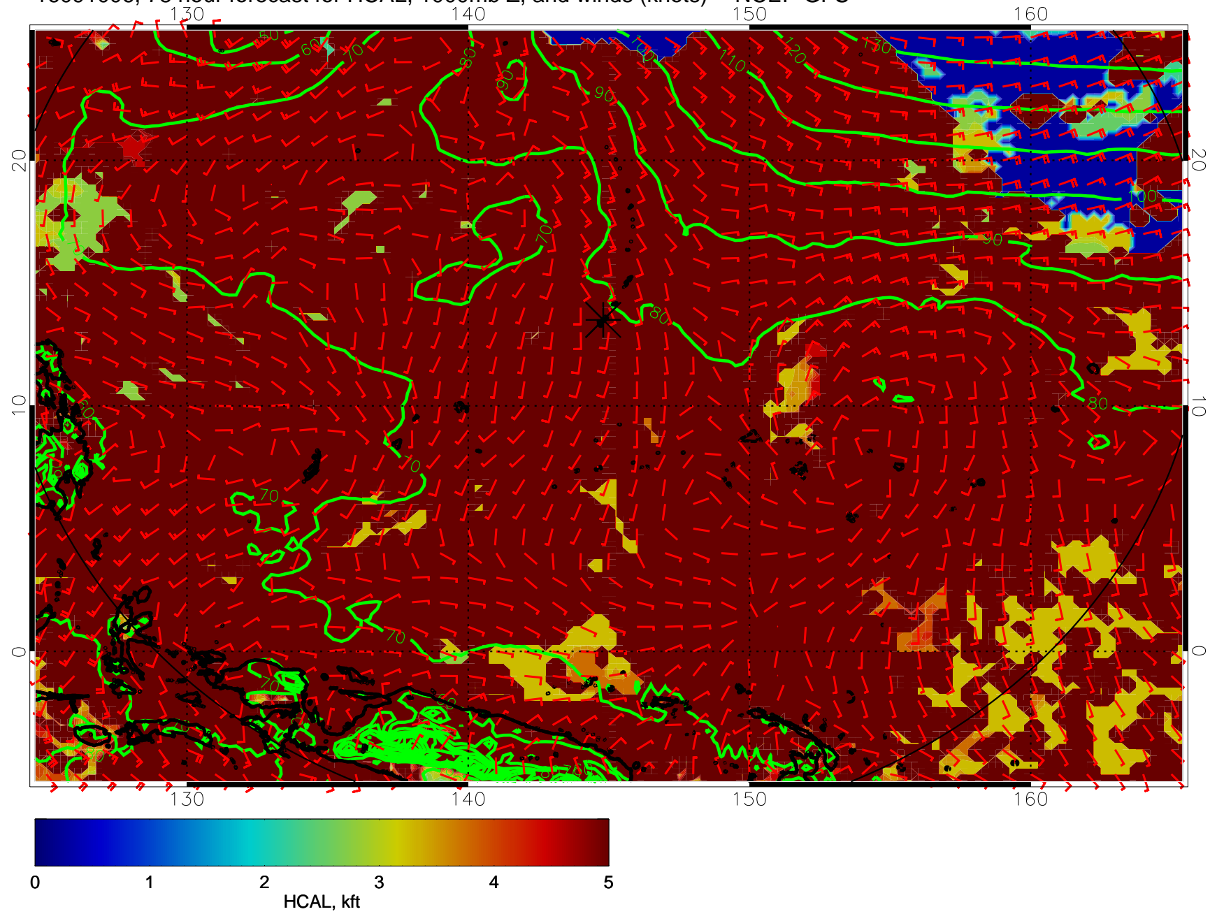
16091006, 78 hour forecast for HCAL, 1000mb Z, and winds (knots) -- NCEP GFS
