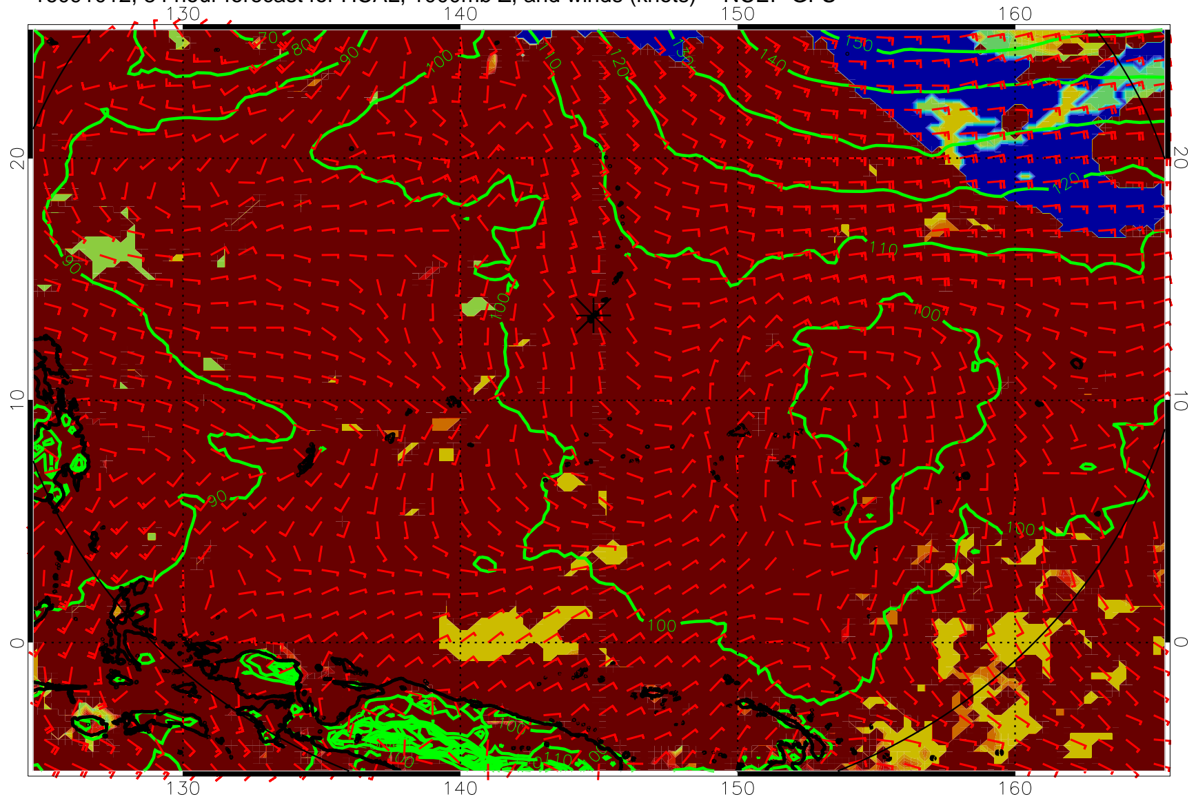
16091012, 84 hour forecast for HCAL, 1000mb Z, and winds (knots) -- NCEP GFS
