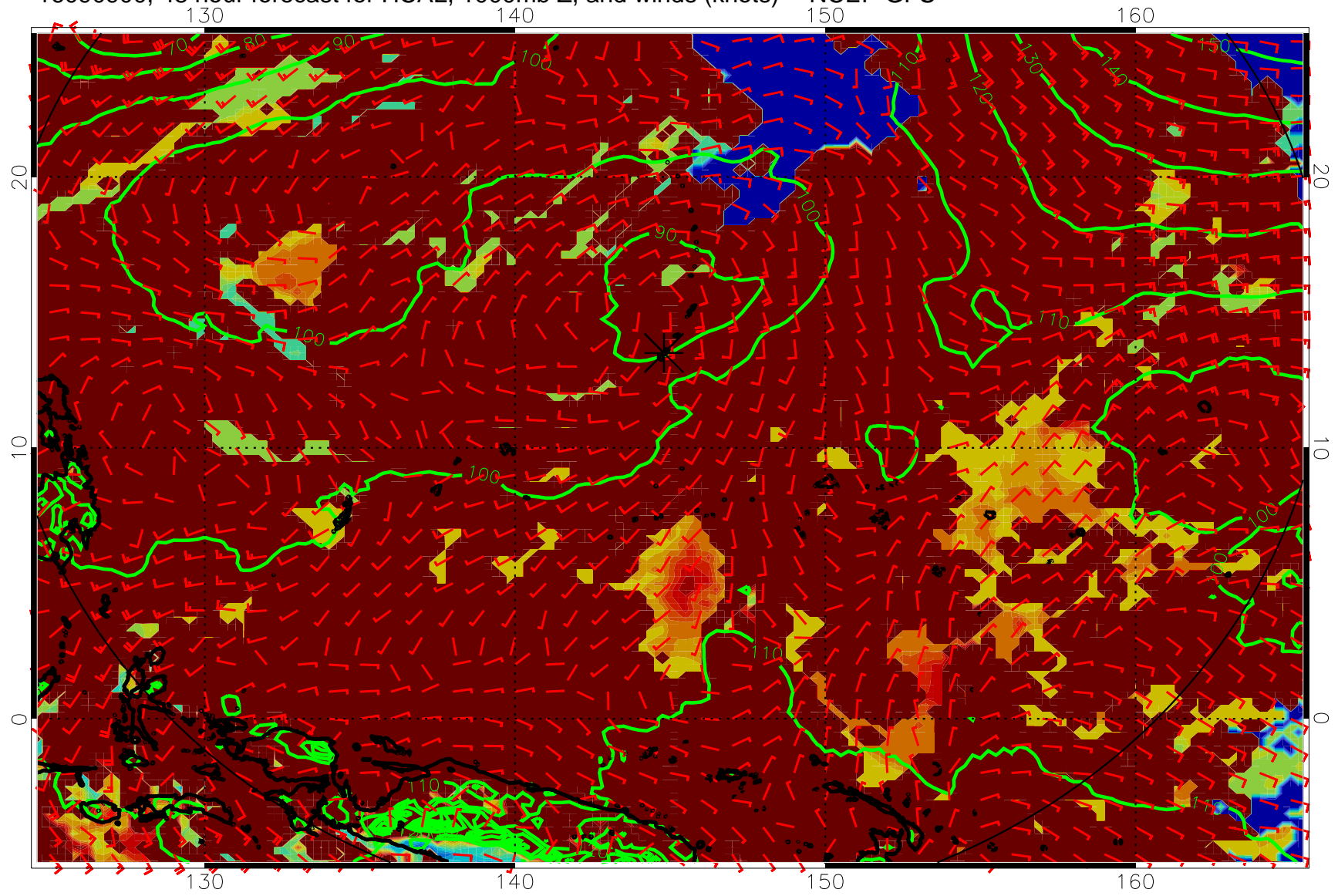
16090900, 48 hour forecast for HCAL, 1000mb Z, and winds (knots) -- NCEP GFS
