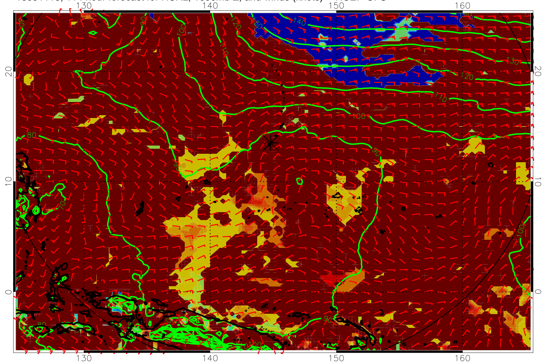
16091118, 114 hour forecast for HCAL, 1000mb Z, and winds (knots) -- NCEP GFS
