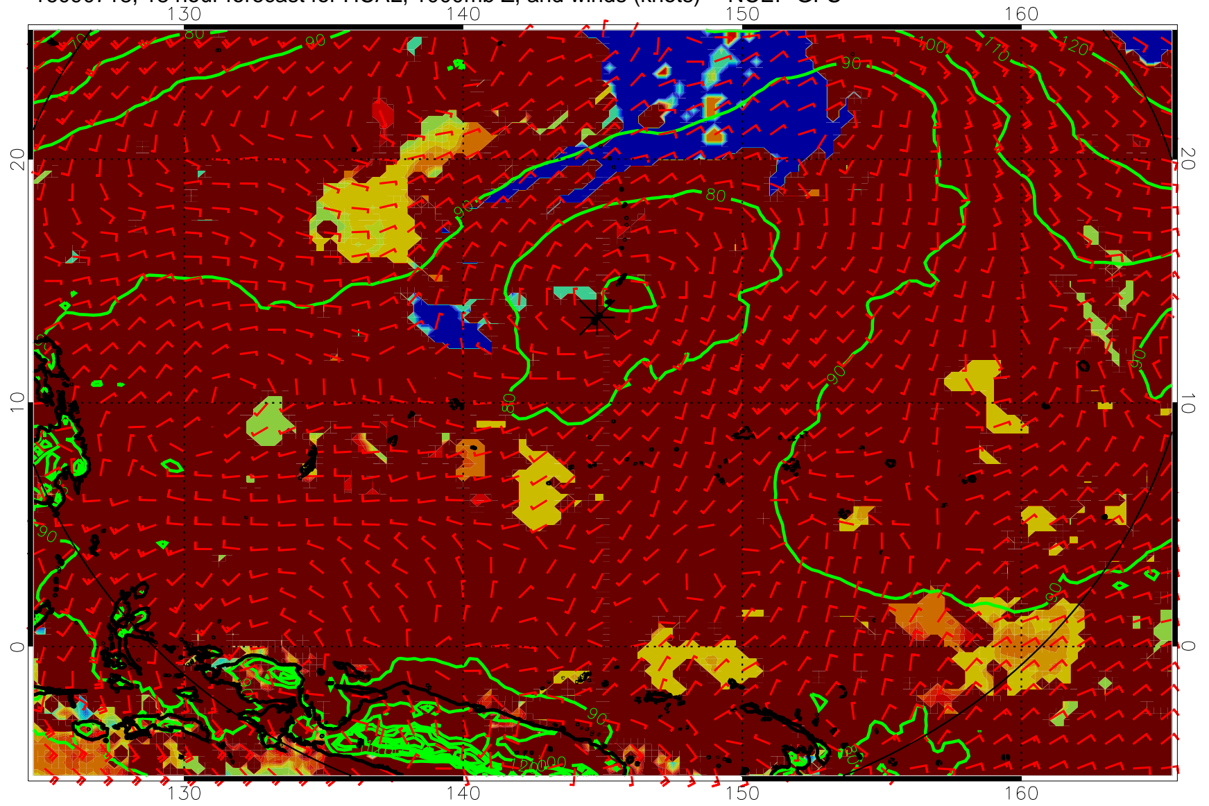
16090718, 18 hour forecast for HCAL, 1000mb Z, and winds (knots) -- NCEP GFS
