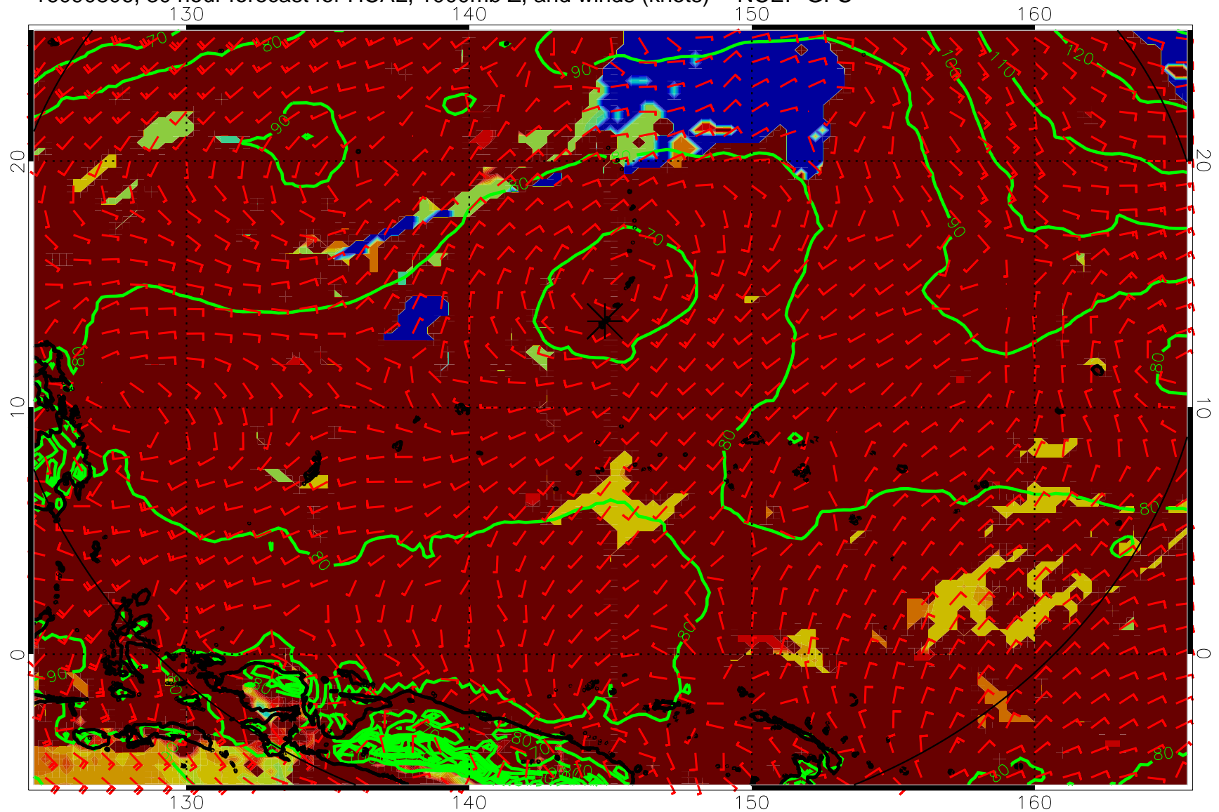
16090806, 30 hour forecast for HCAL, 1000mb Z, and winds (knots) -- NCEP GFS
