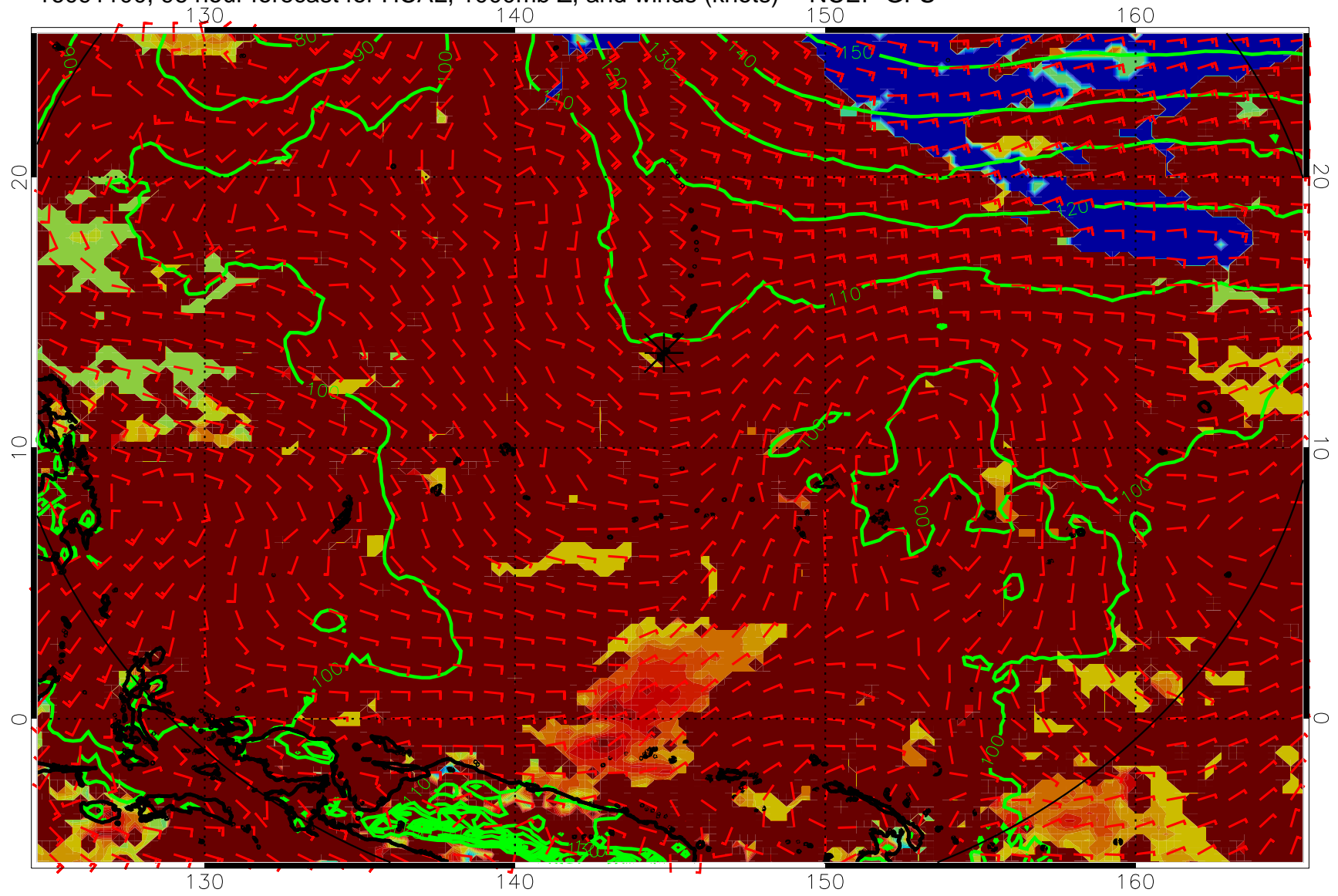
16091100, 96 hour forecast for HCAL, 1000mb Z, and winds (knots) -- NCEP GFS
