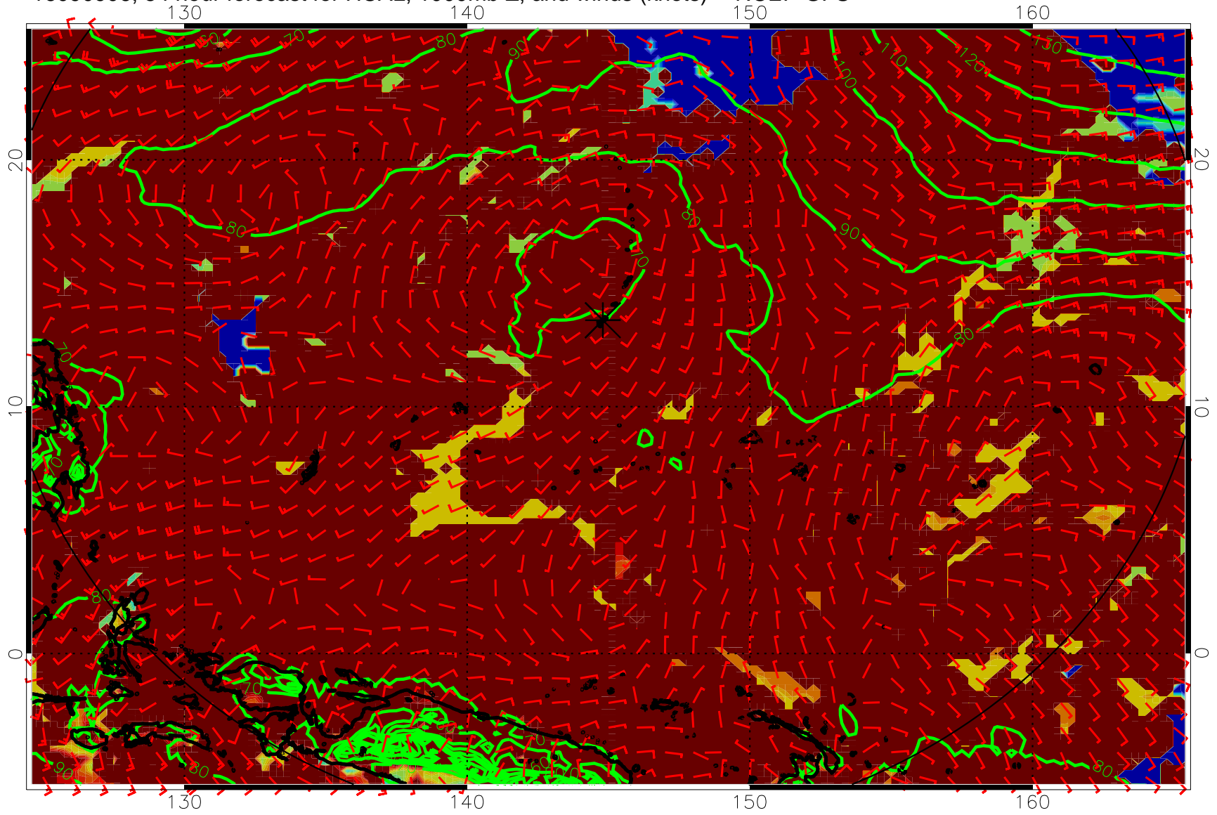
16090906, 54 hour forecast for HCAL, 1000mb Z, and winds (knots) -- NCEP GFS
