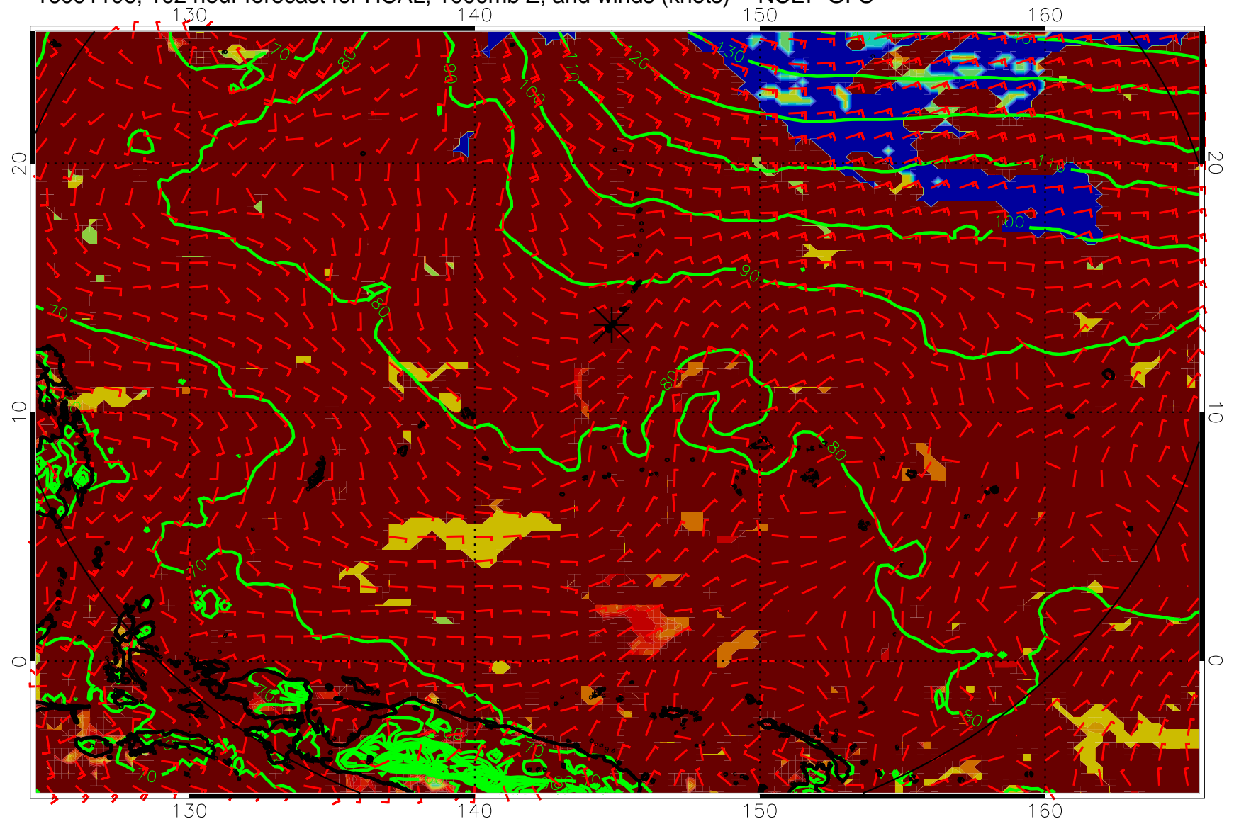
16091106, 102 hour forecast for HCAL, 1000mb Z, and winds (knots) -- NCEP GFS
