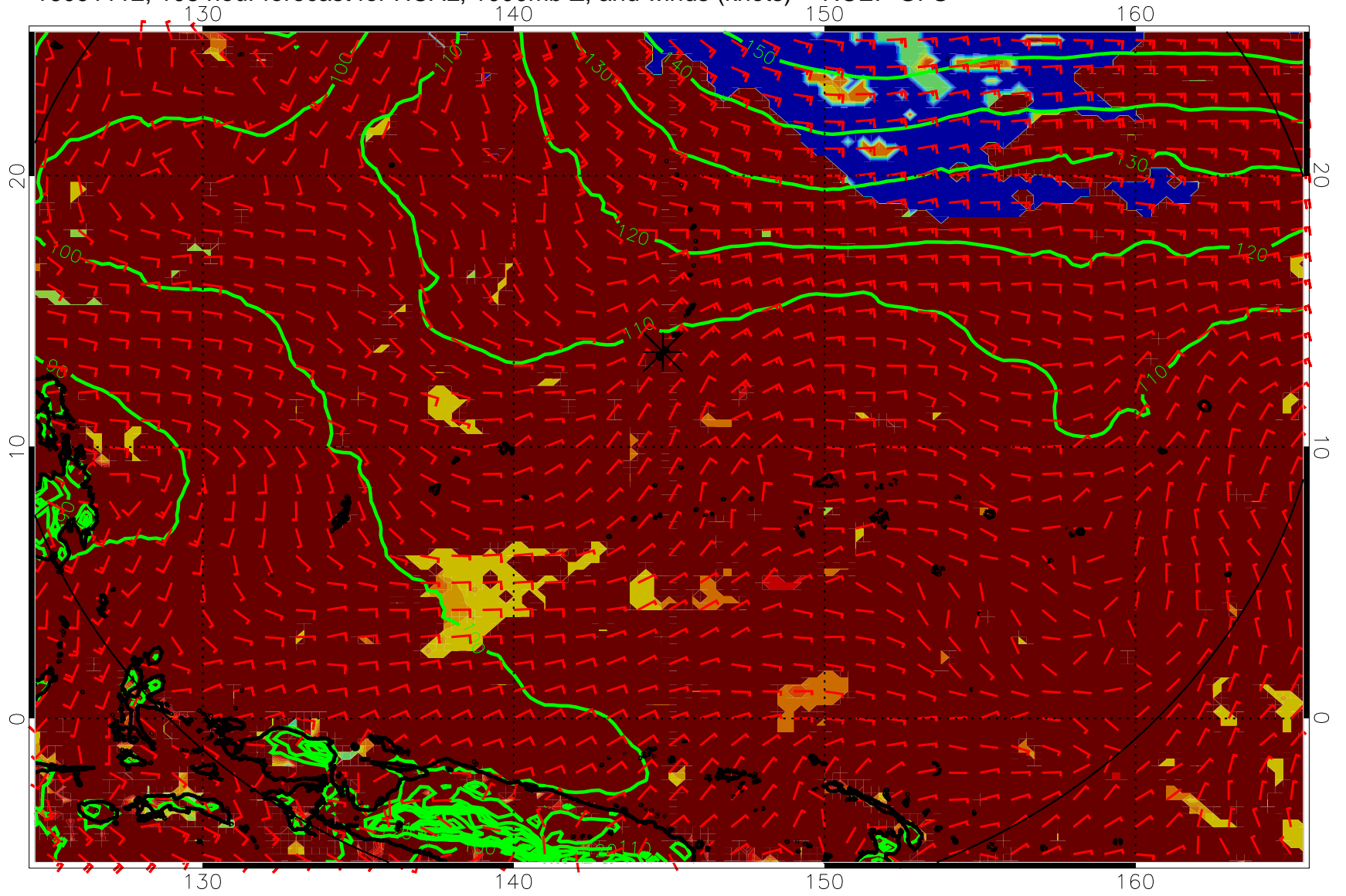
16091112, 108 hour forecast for HCAL, 1000mb Z, and winds (knots) -- NCEP GFS
