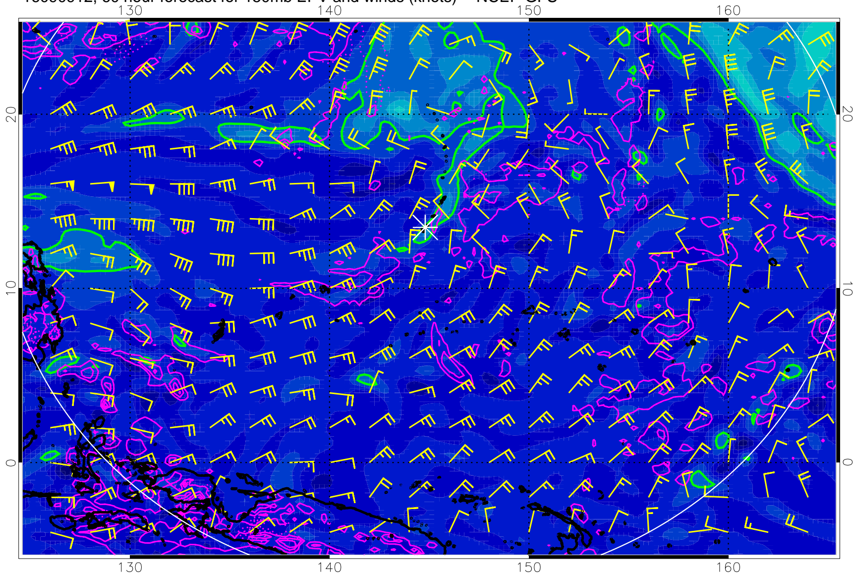
16090912, 60 hour forecast for 150mb EPV and winds (knots) -- NCEP GFS
