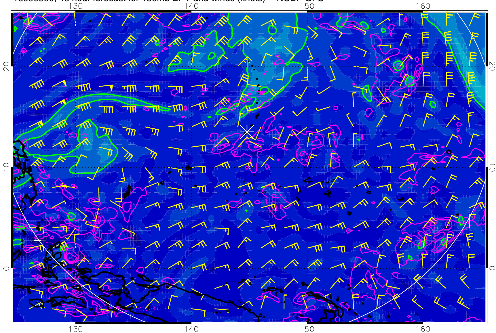
16090900, 48 hour forecast for 150mb EPV and winds (knots) -- NCEP GFS
