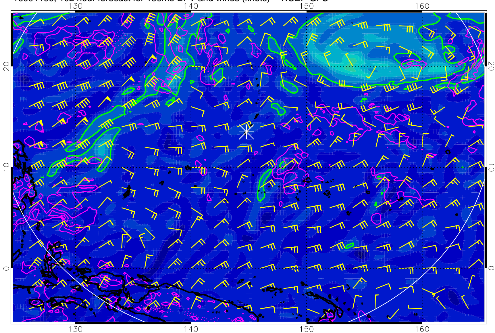
16091106, 102 hour forecast for 150mb EPV and winds (knots) -- NCEP GFS
