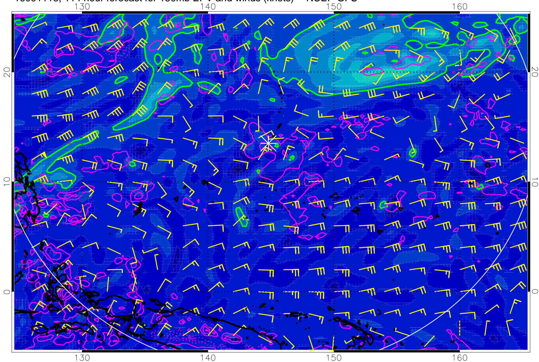
16091118, 114 hour forecast for 150mb EPV and winds (knots) -- NCEP GFS
