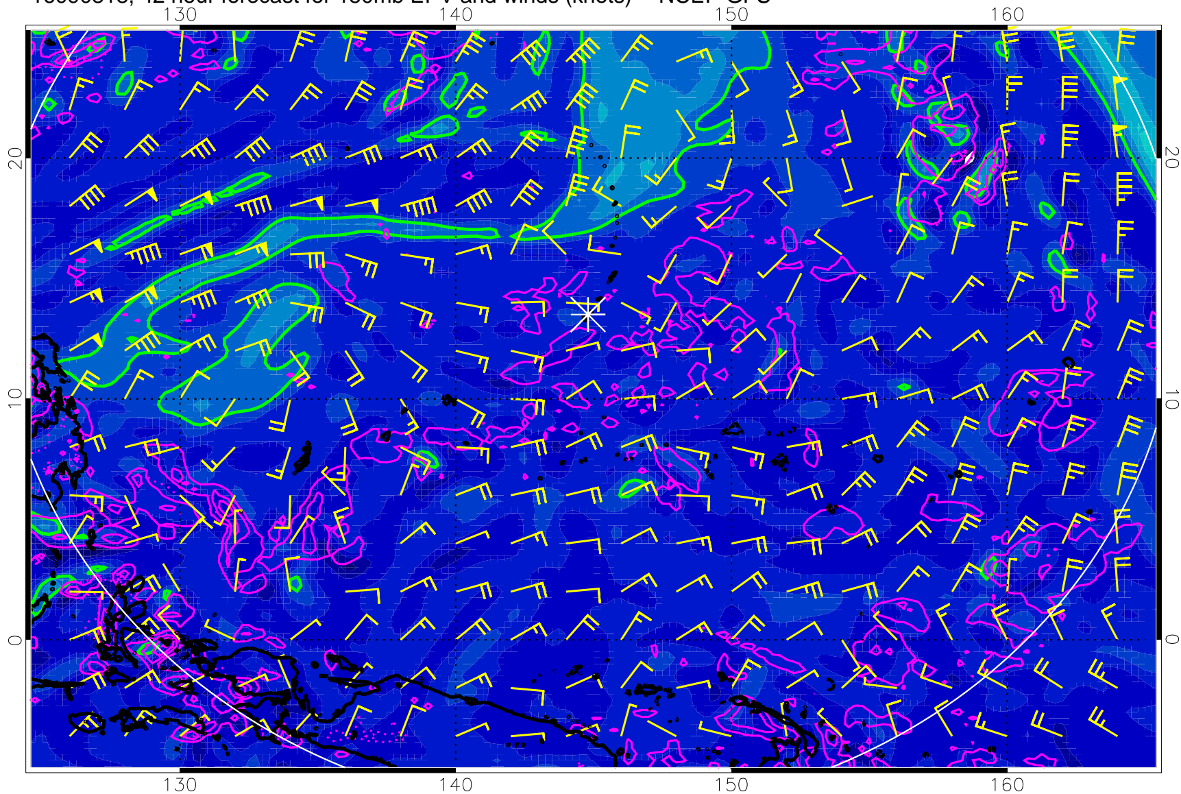
16090818, 42 hour forecast for 150mb EPV and winds (knots) -- NCEP GFS
