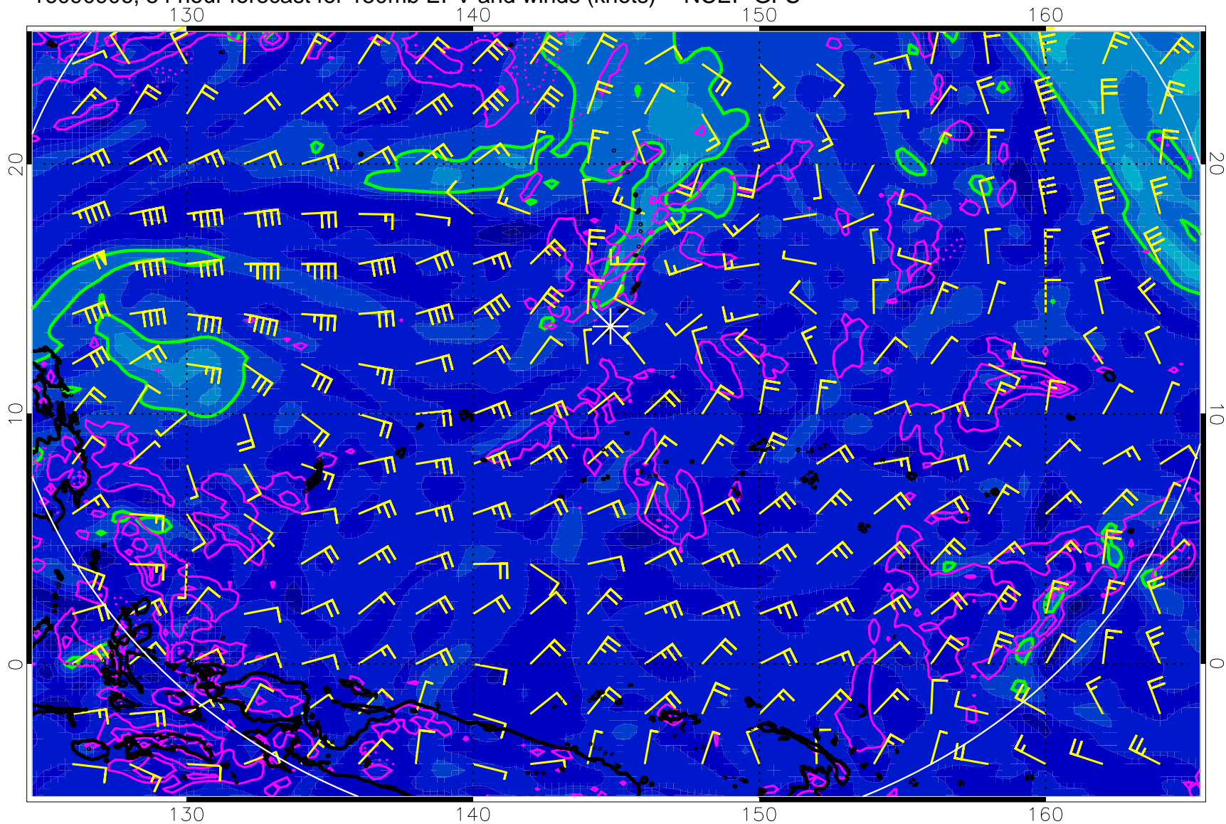
16090906, 54 hour forecast for 150mb EPV and winds (knots) -- NCEP GFS
