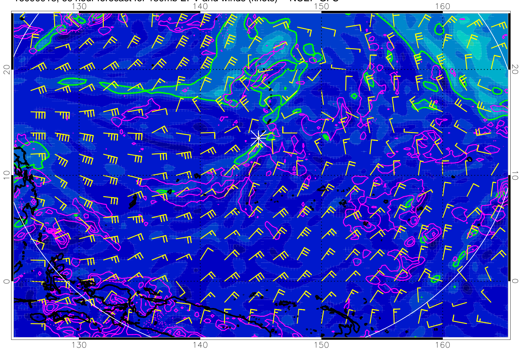
16090918, 66 hour forecast for 150mb EPV and winds (knots) -- NCEP GFS
