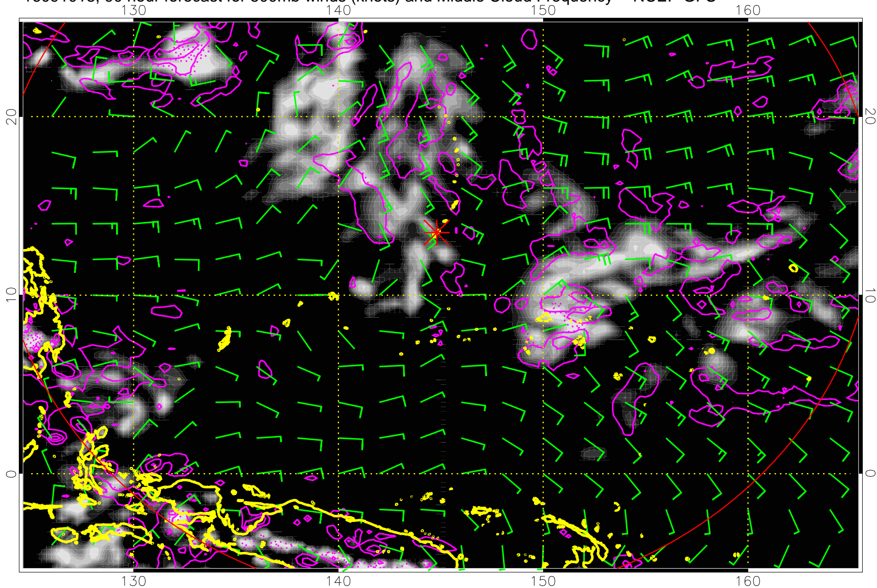
16091018, 90 hour forecast for 500mb winds (knots) and Middle Cloud Frequency -- NCEP GFS
