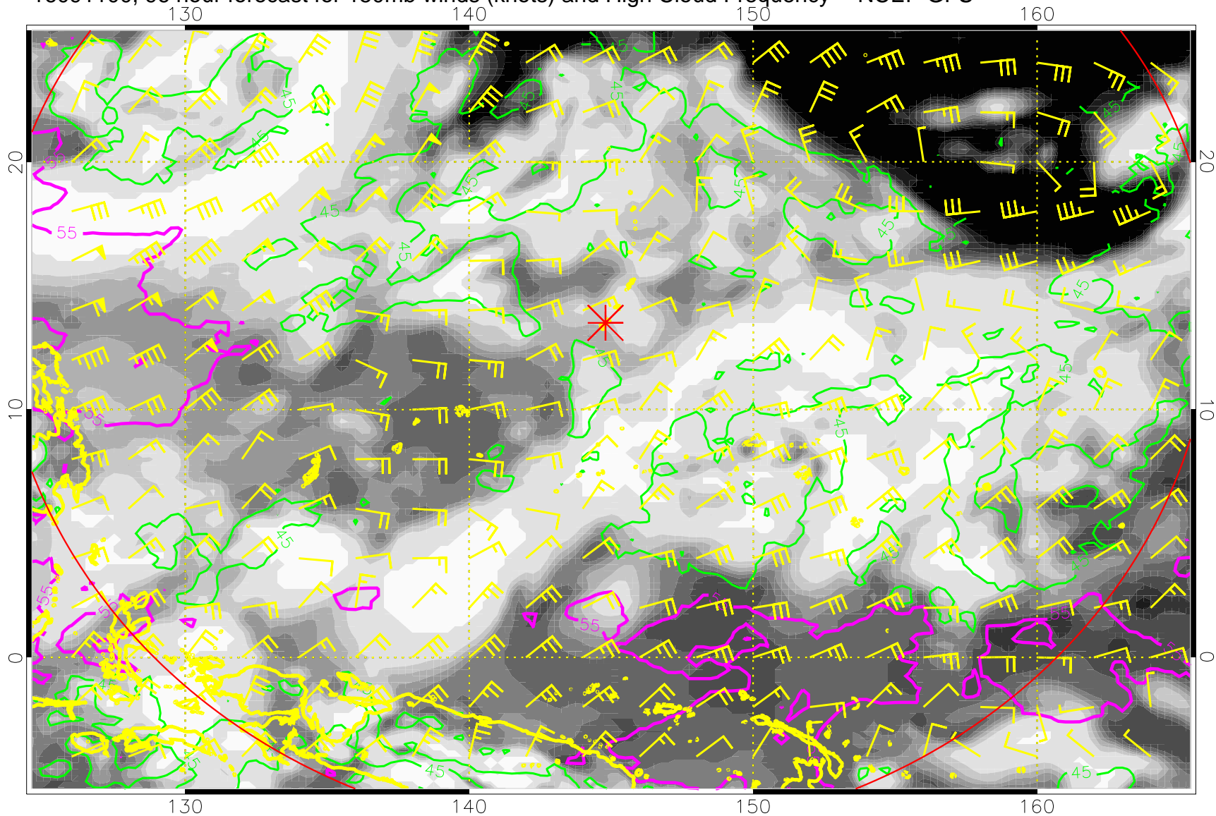
16091100, 96 hour forecast for 150mb winds (knots) and High Cloud Frequency -- NCEP GFS
