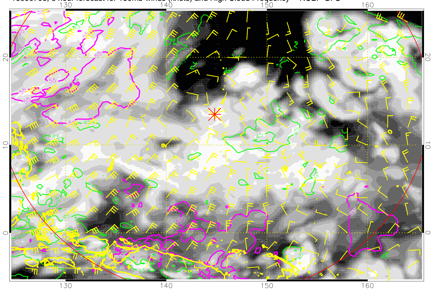
16090706, 6 hour forecast for 150mb winds (knots) and High Cloud Frequency -- NCEP GFS
