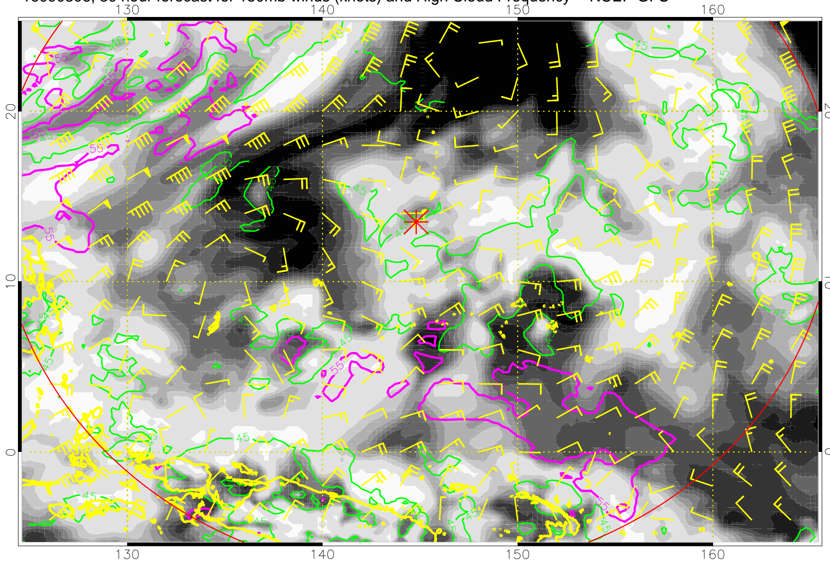
16090806, 30 hour forecast for 150mb winds (knots) and High Cloud Frequency -- NCEP GFS
