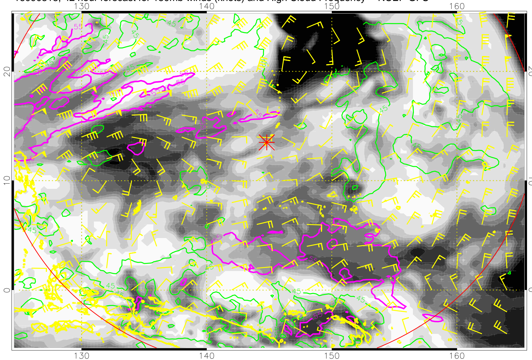
16090818, 42 hour forecast for 150mb winds (knots) and High Cloud Frequency -- NCEP GFS
