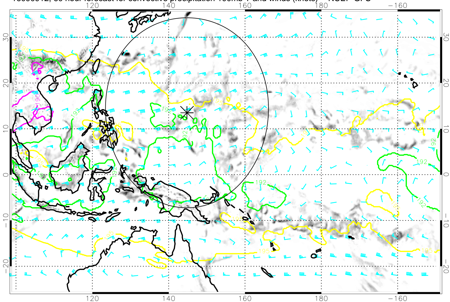
16090912, 60 hour forecast for convective precipitation 100mb T and winds (knots) -- NCEP GFS
