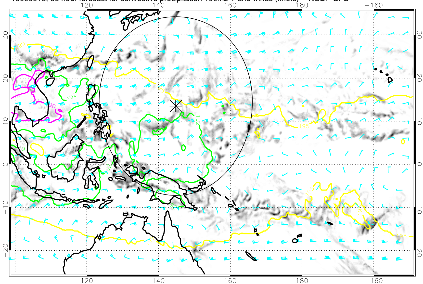
16090918, 66 hour forecast for convective precipitation 100mb T and winds (knots) -- NCEP GFS
