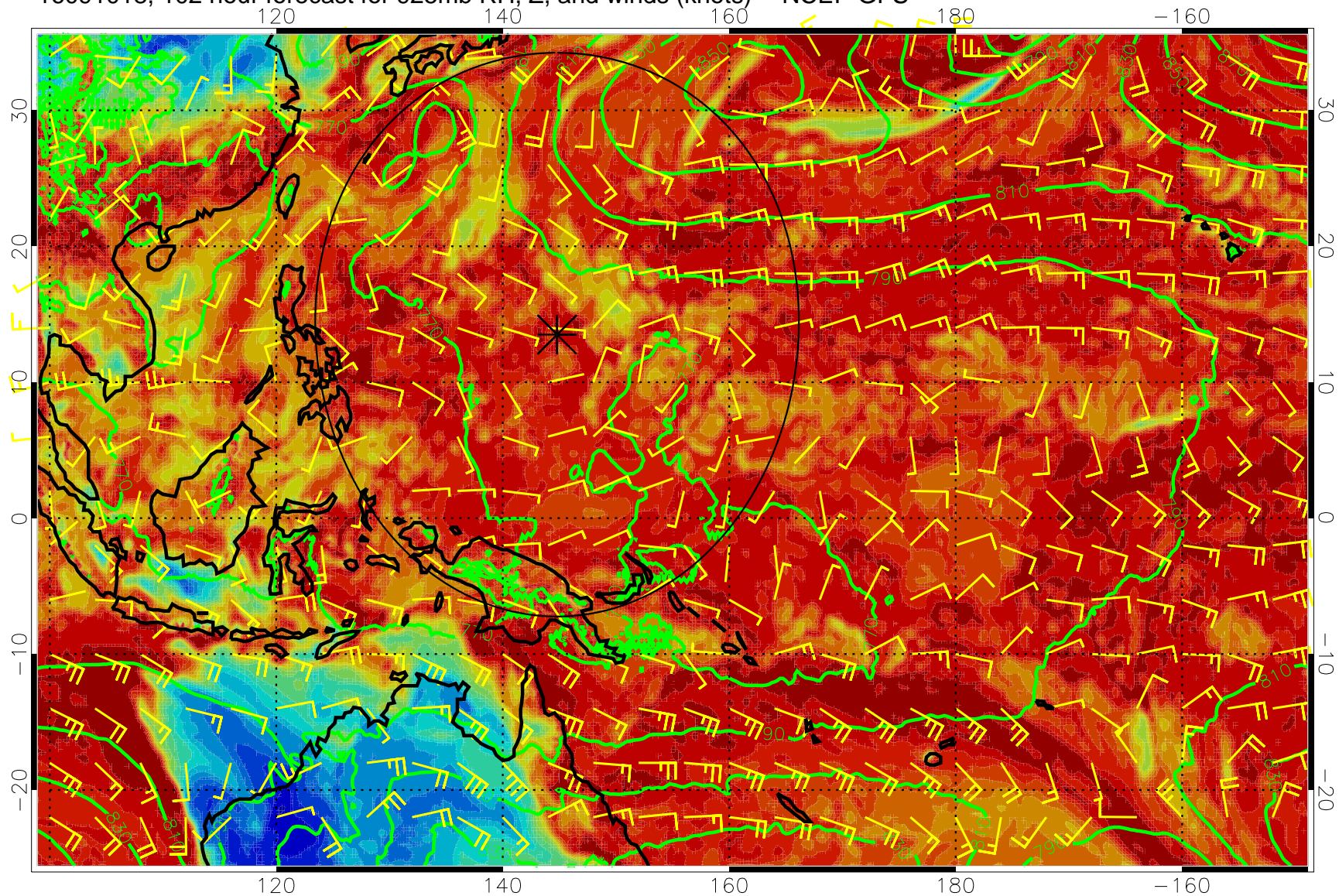
16091018, 102 hour forecast for 925mb RH, Z, and winds (knots) -- NCEP GFS
