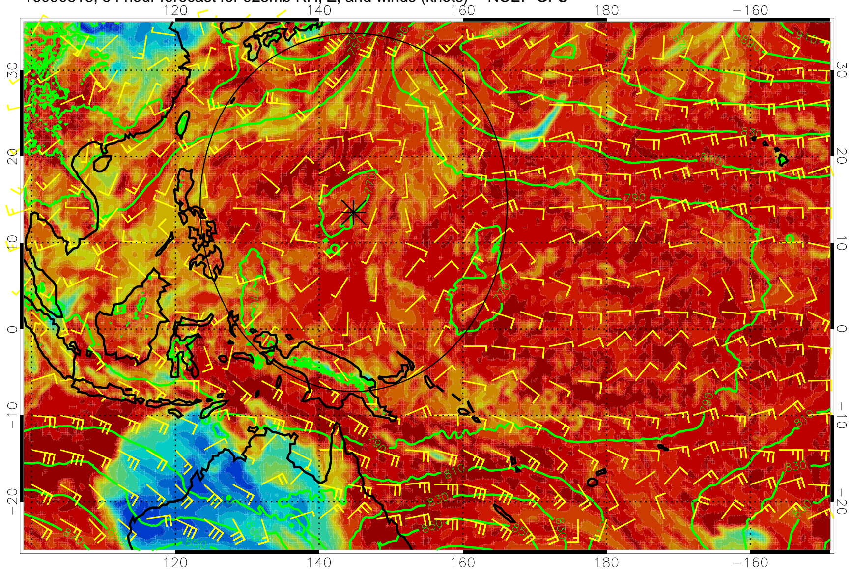
16090818, 54 hour forecast for 925mb RH, Z, and winds (knots) -- NCEP GFS
