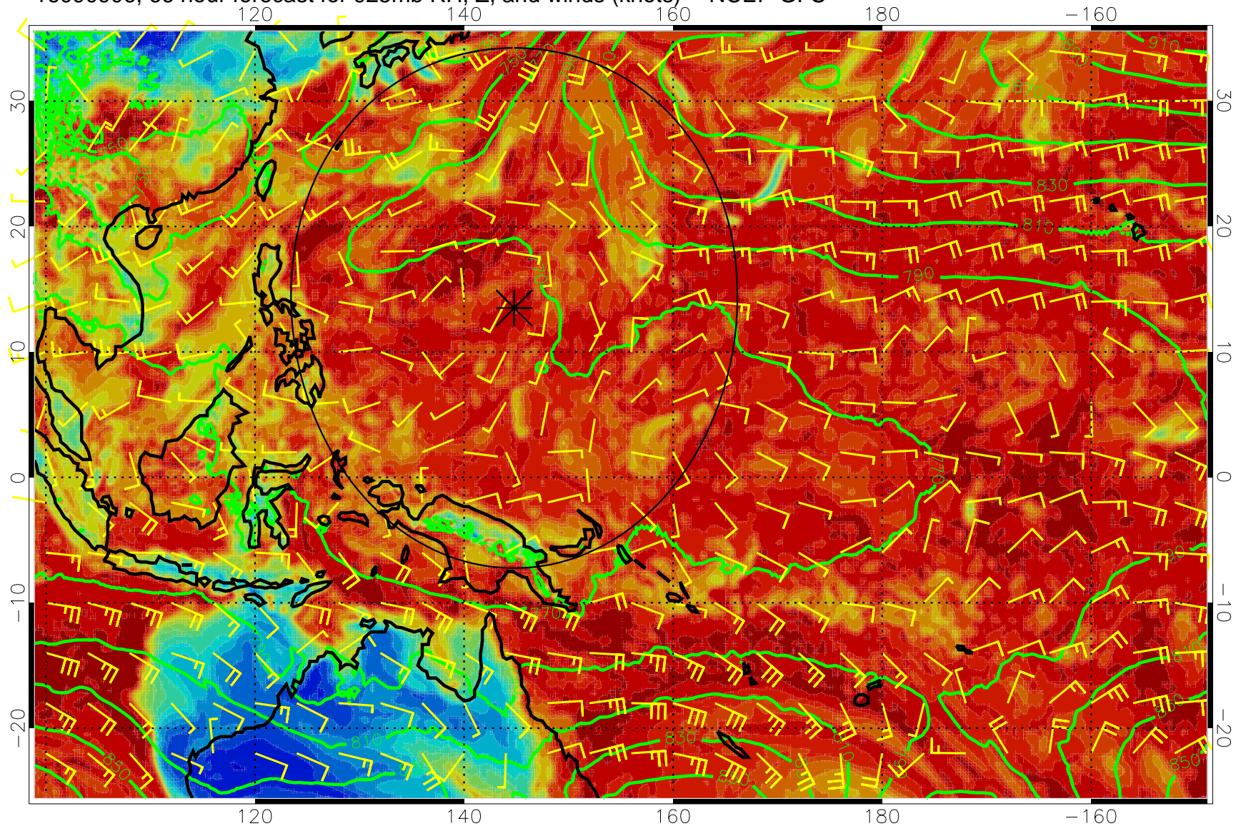
16090906, 66 hour forecast for 925mb RH, Z, and winds (knots) -- NCEP GFS
