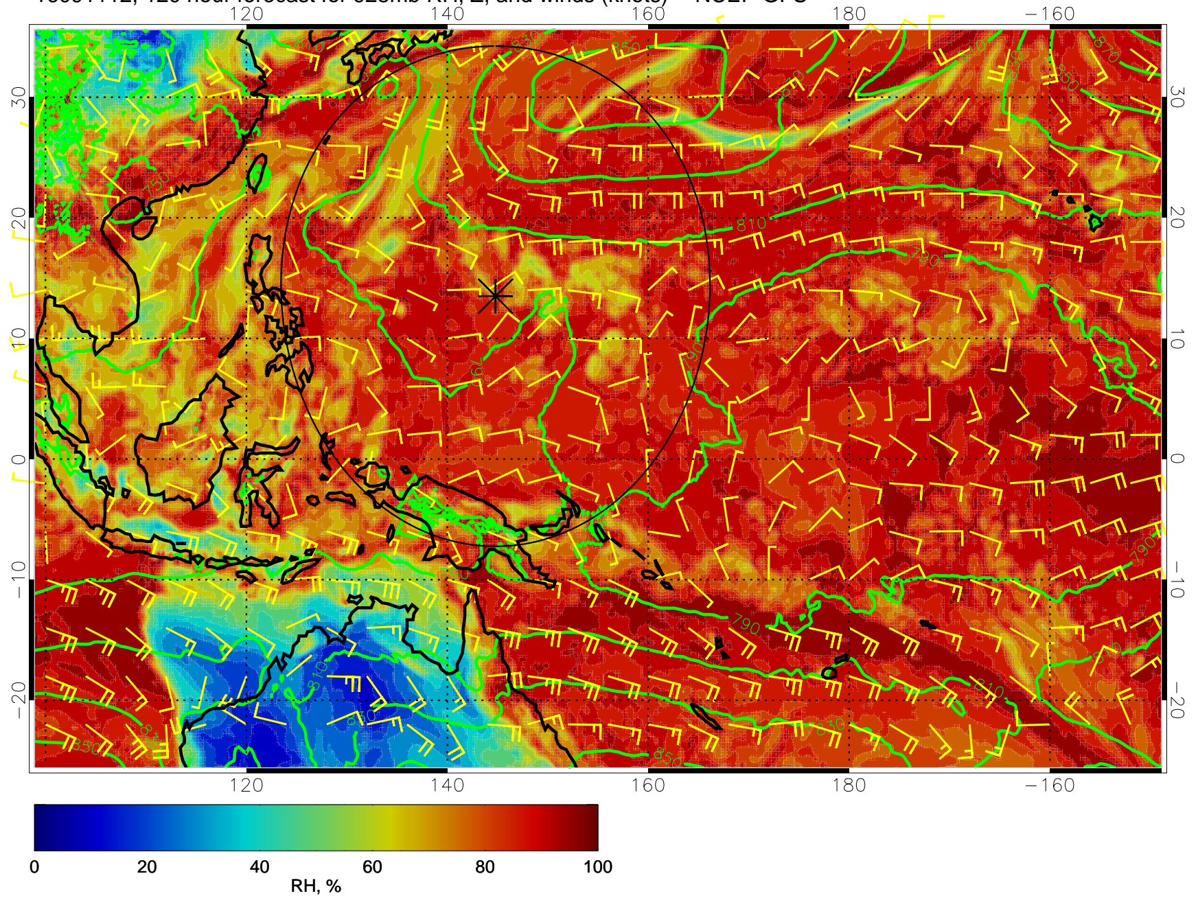
16091112, 120 hour forecast for 925mb RH, Z, and winds (knots) -- NCEP GFS
