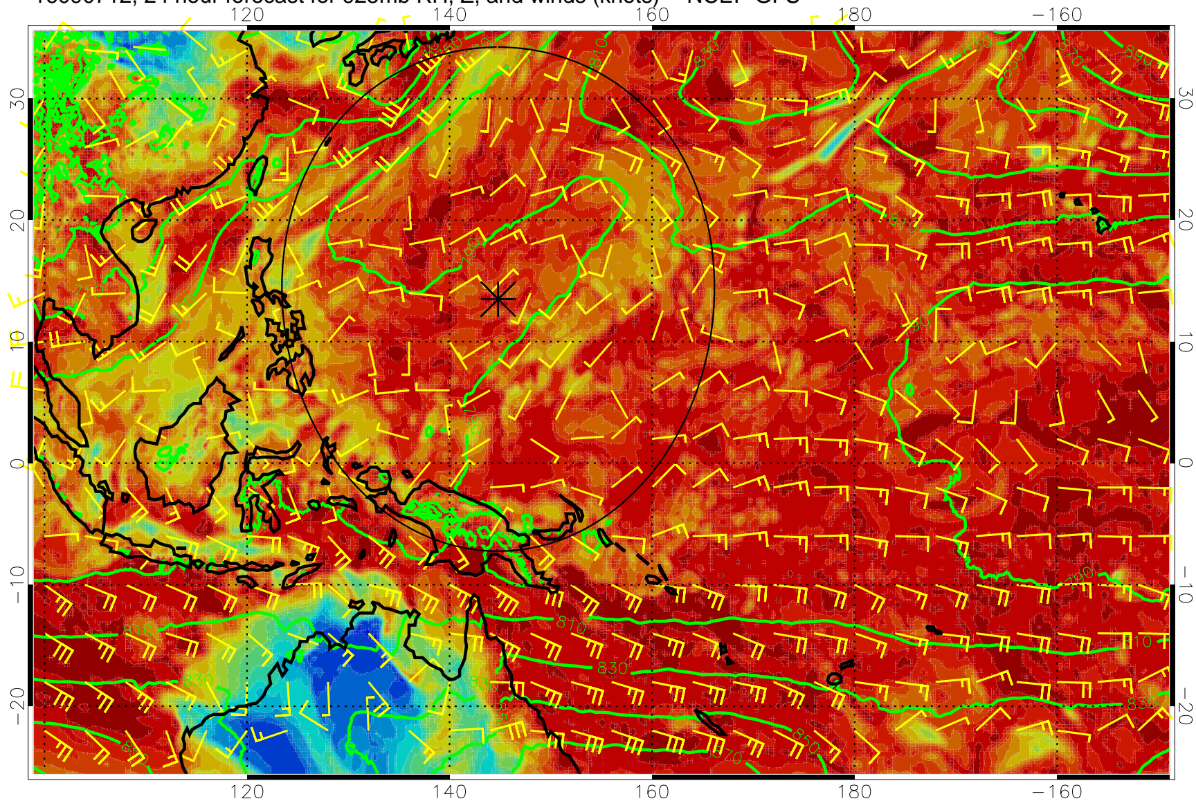
16090712, 24 hour forecast for 925mb RH, Z, and winds (knots) -- NCEP GFS
