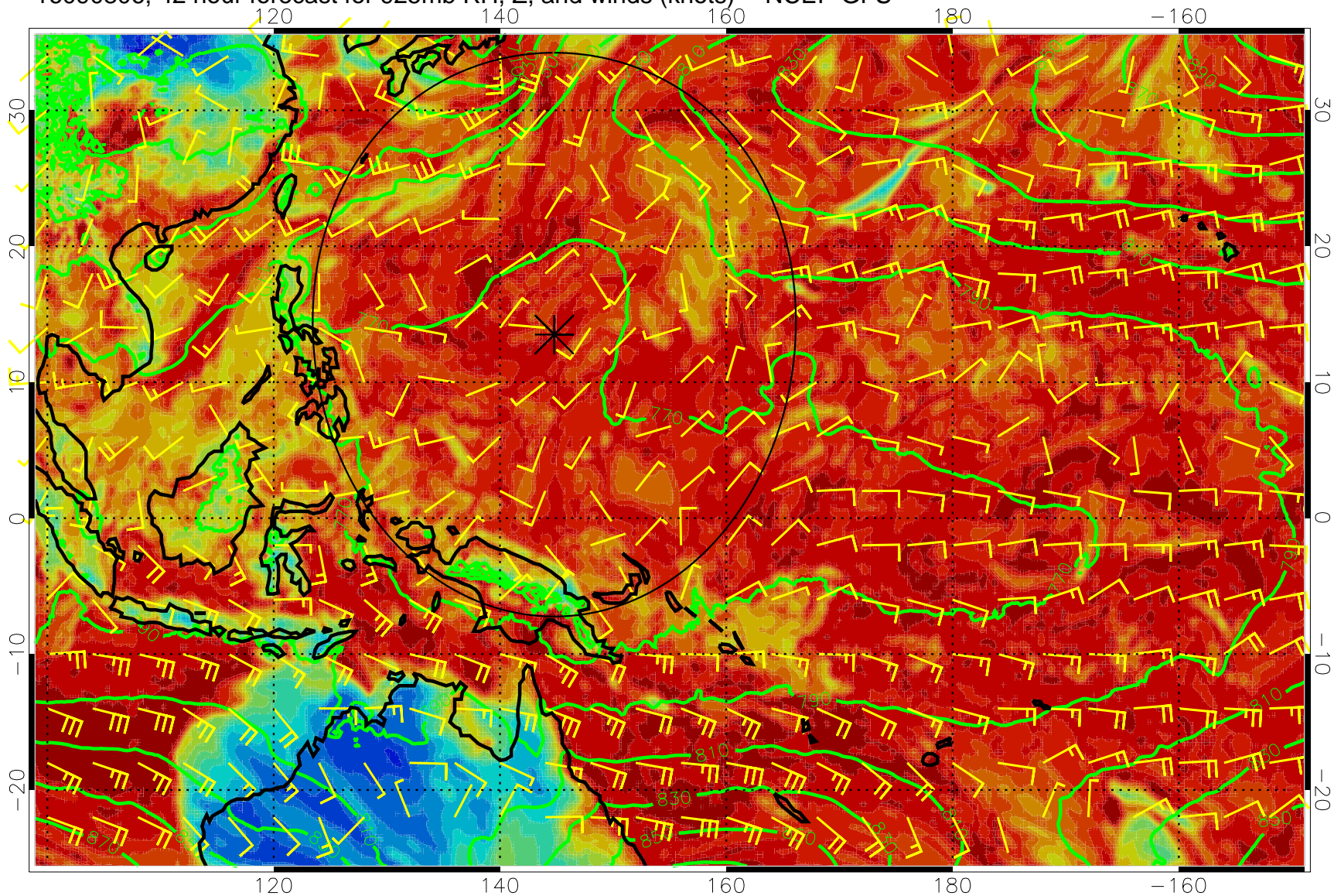
16090806, 42 hour forecast for 925mb RH, Z, and winds (knots) -- NCEP GFS
