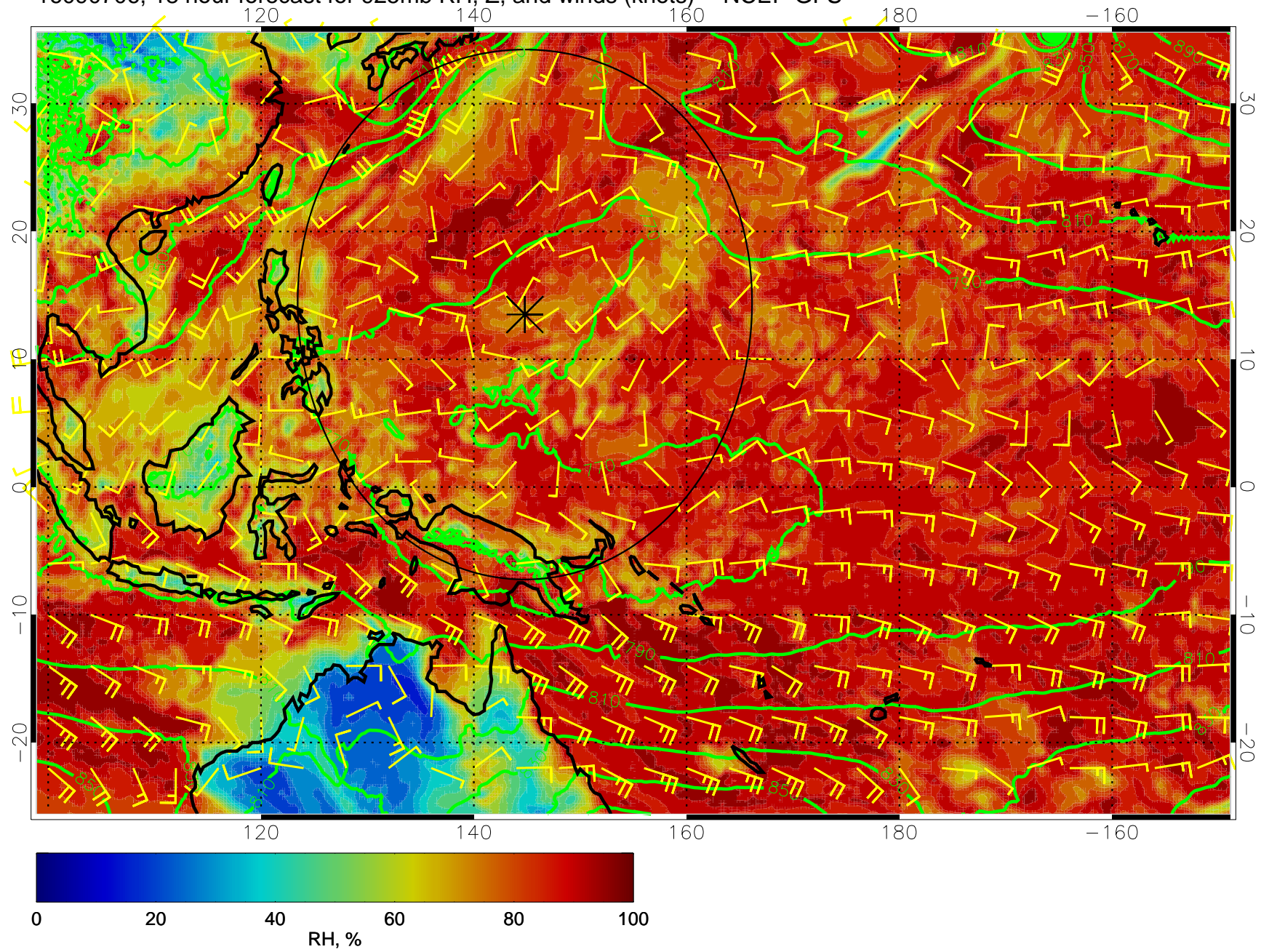
16090706, 18 hour forecast for 925mb RH, Z, and winds (knots) -- NCEP GFS
