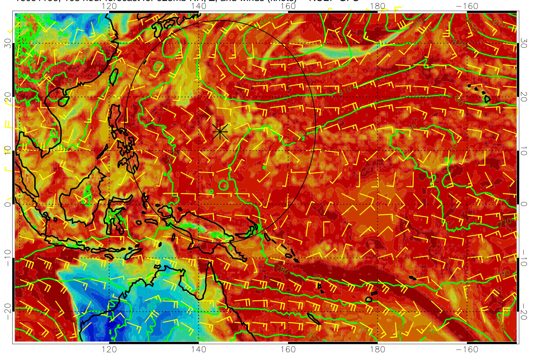
16091100, 108 hour forecast for 925mb RH, Z, and winds (knots) -- NCEP GFS
