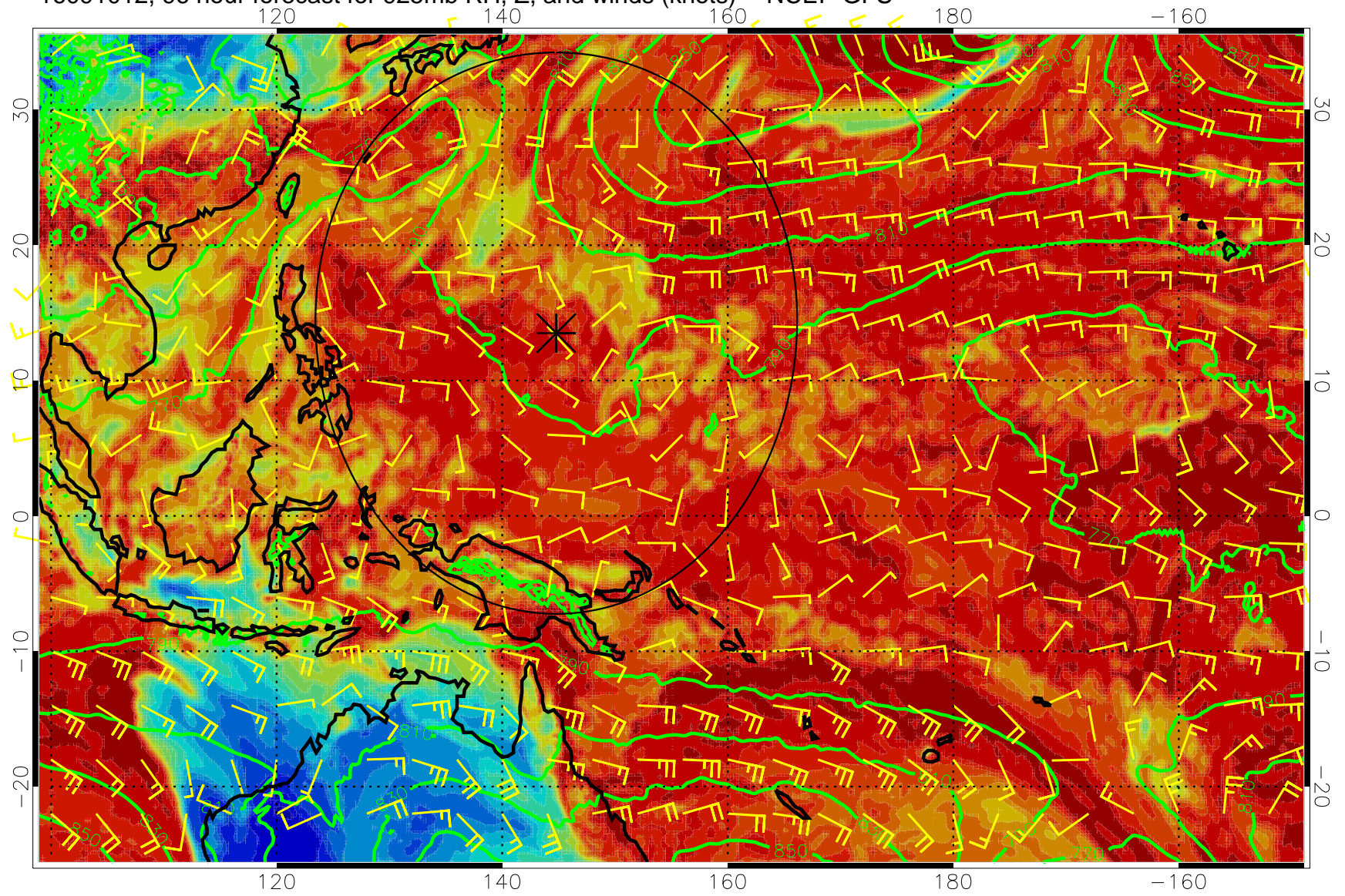
16091012, 96 hour forecast for 925mb RH, Z, and winds (knots) -- NCEP GFS
