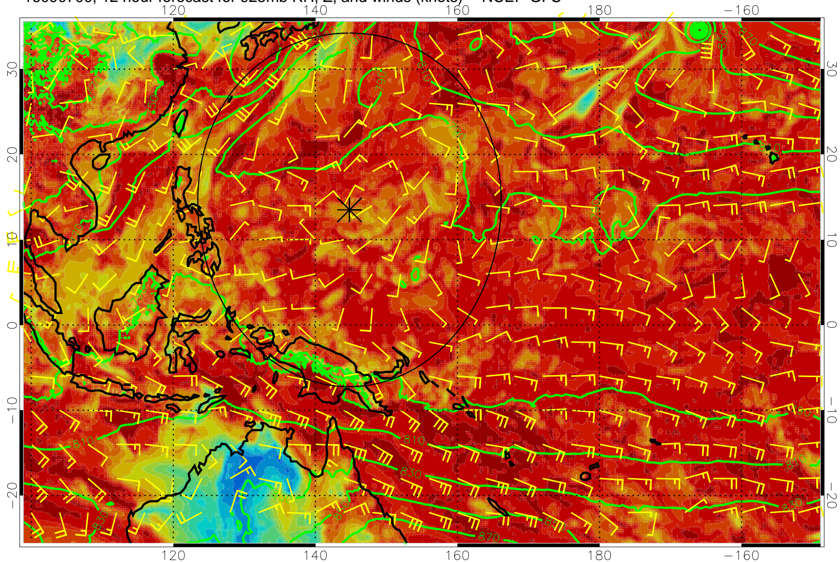
16090700, 12 hour forecast for 925mb RH, Z, and winds (knots) -- NCEP GFS
