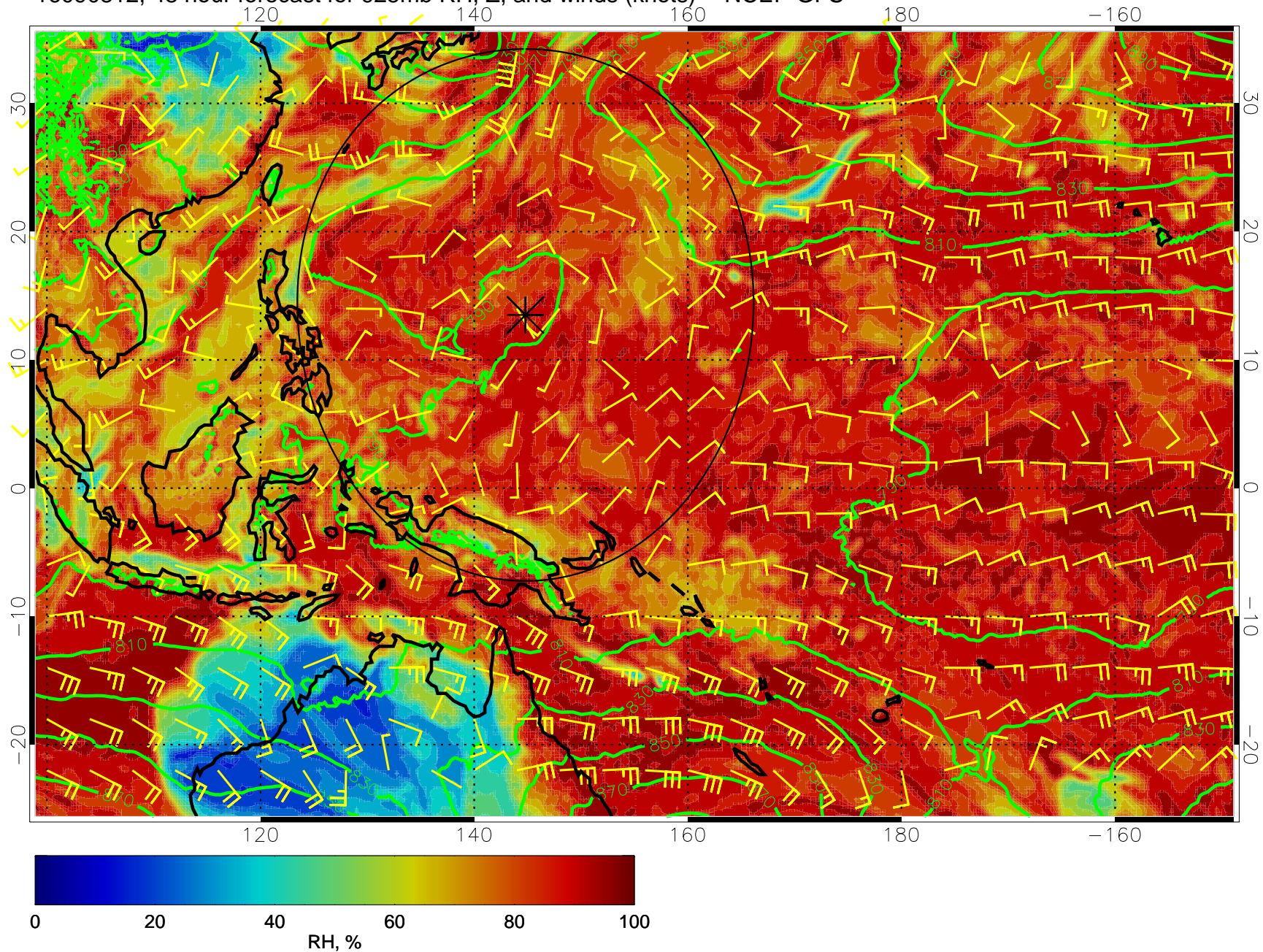
16090812, 48 hour forecast for 925mb RH, Z, and winds (knots) -- NCEP GFS
