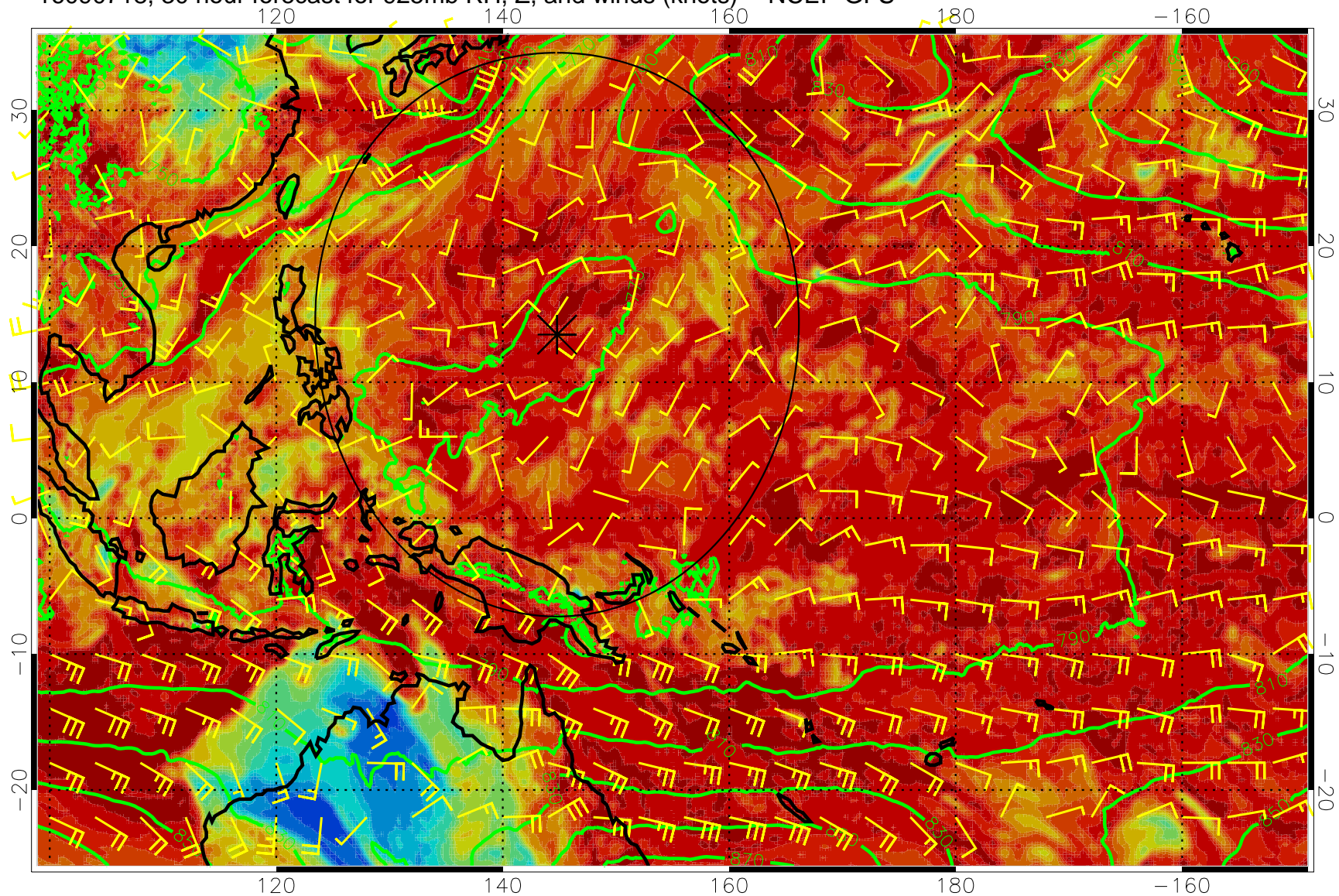
16090718, 30 hour forecast for 925mb RH, Z, and winds (knots) -- NCEP GFS
