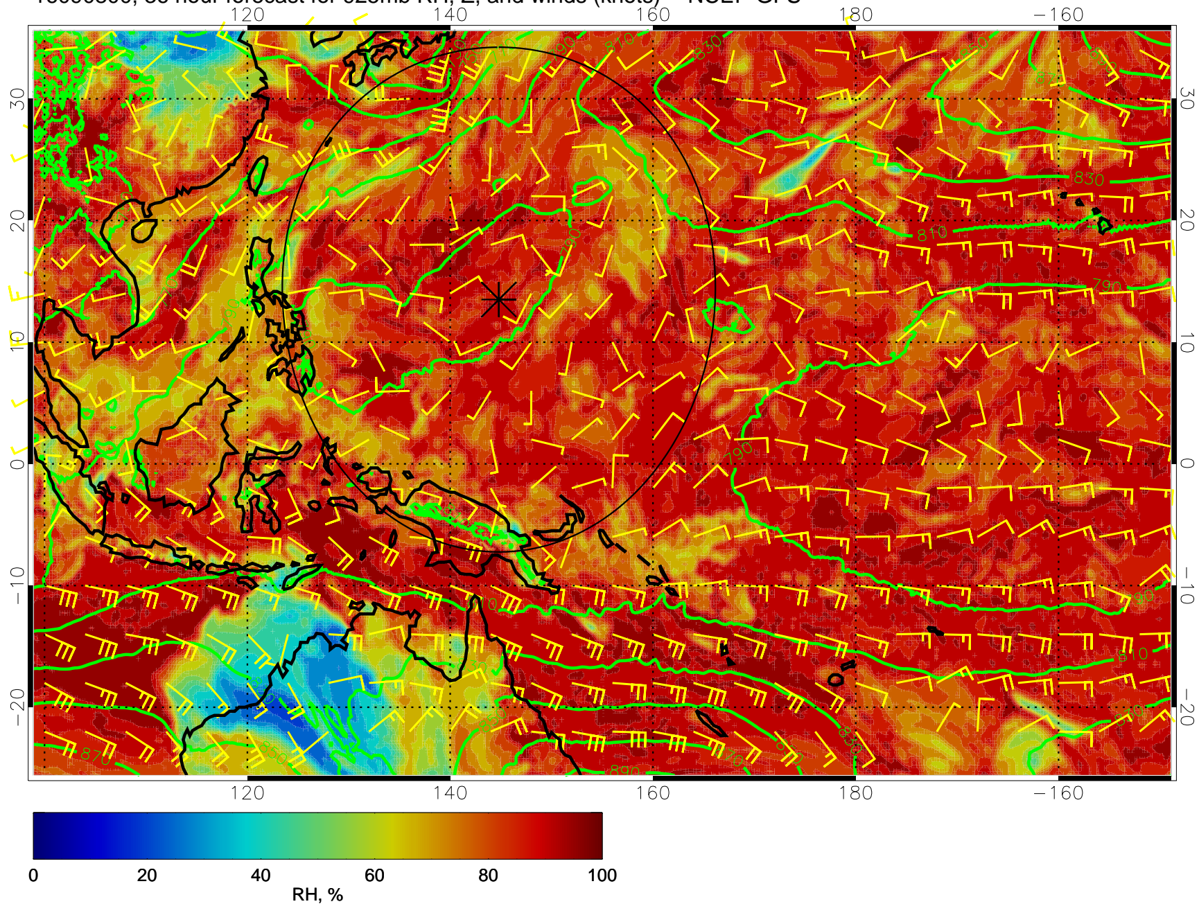
16090800, 36 hour forecast for 925mb RH, Z, and winds (knots) -- NCEP GFS
