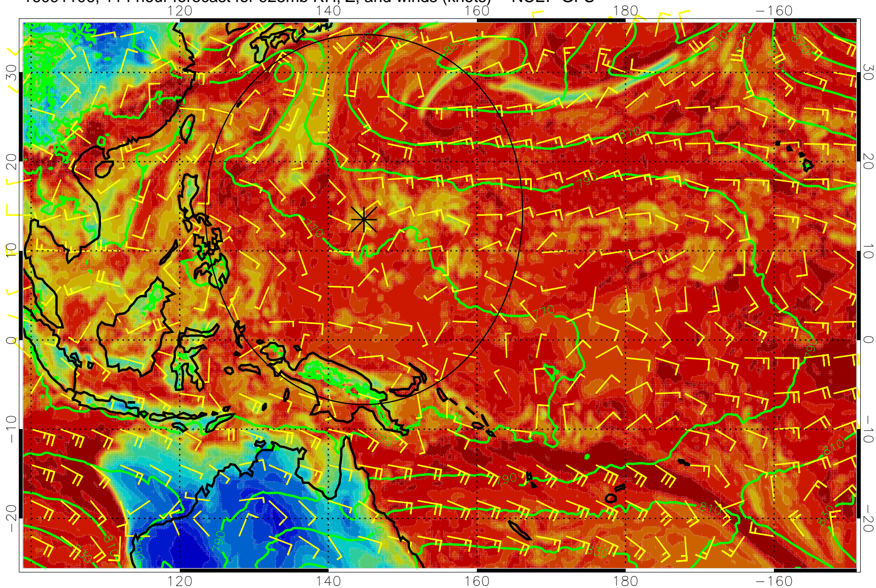
16091106, 114 hour forecast for 925mb RH, Z, and winds (knots) -- NCEP GFS
