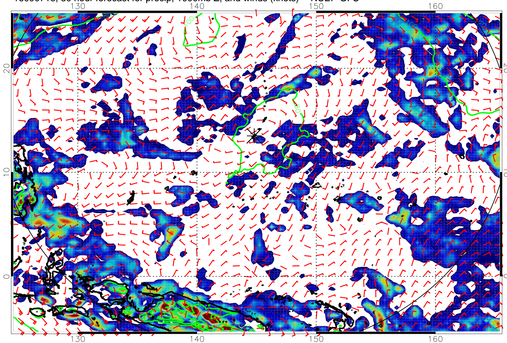
16090718, 30 hour forecast for precip, 1000mb Z, and winds (knots) -- NCEP GFS
