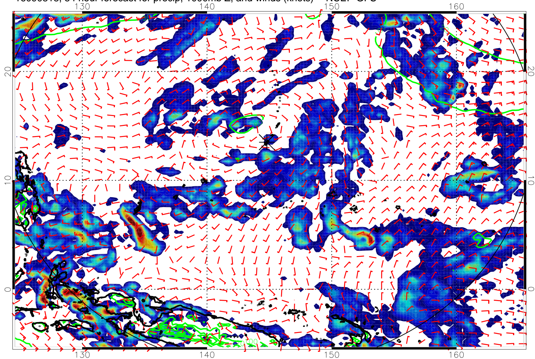
16090818, 54 hour forecast for precip, 1000mb Z, and winds (knots) -- NCEP GFS
