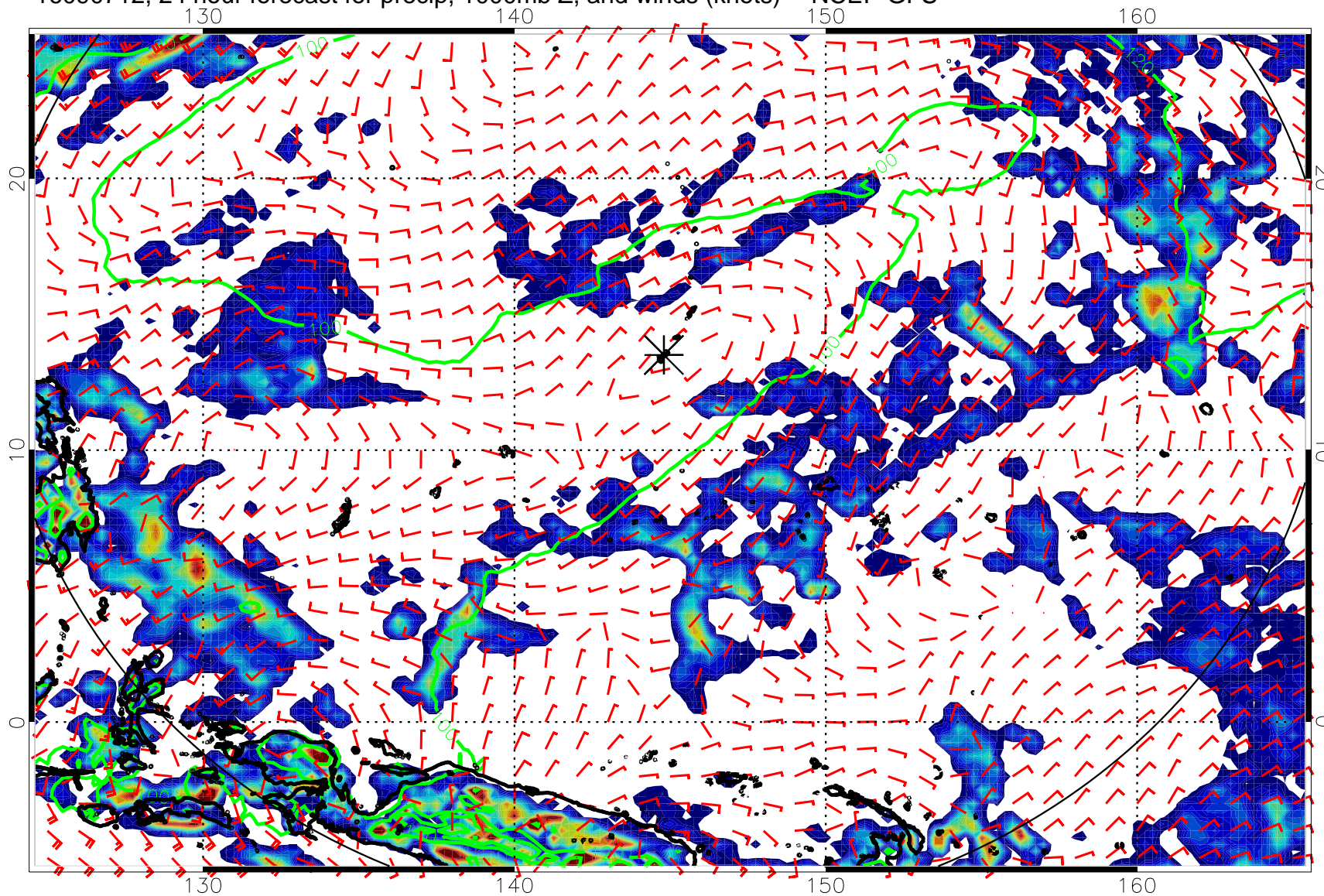
16090712, 24 hour forecast for precip, 1000mb Z, and winds (knots) -- NCEP GFS
