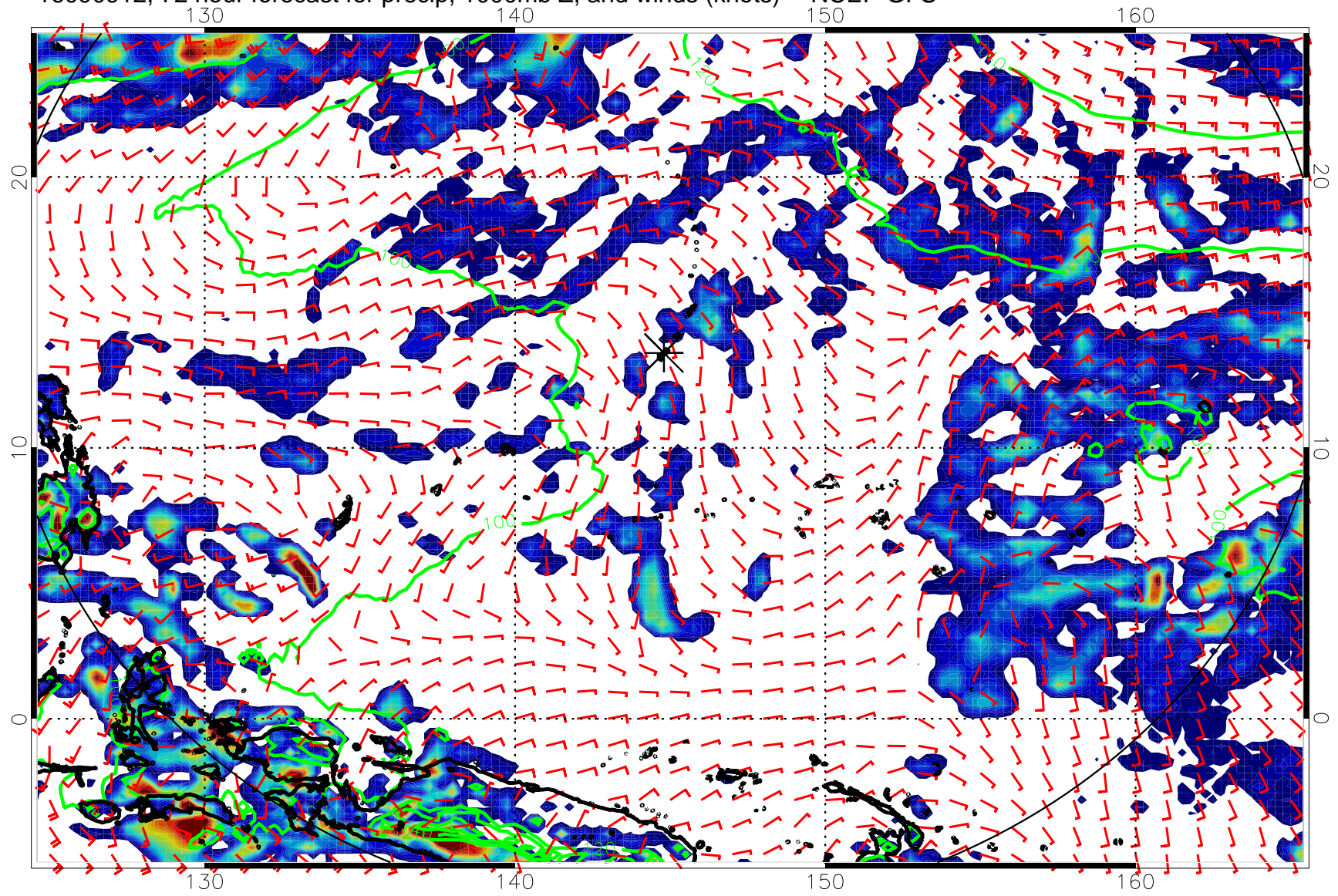
16090912, 72 hour forecast for precip, 1000mb Z, and winds (knots) -- NCEP GFS
