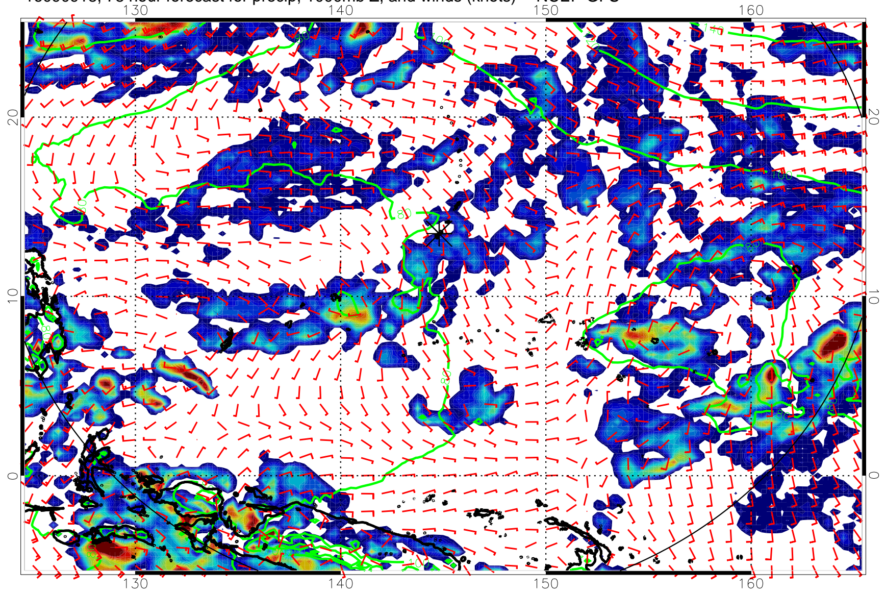
16090918, 78 hour forecast for precip, 1000mb Z, and winds (knots) -- NCEP GFS
