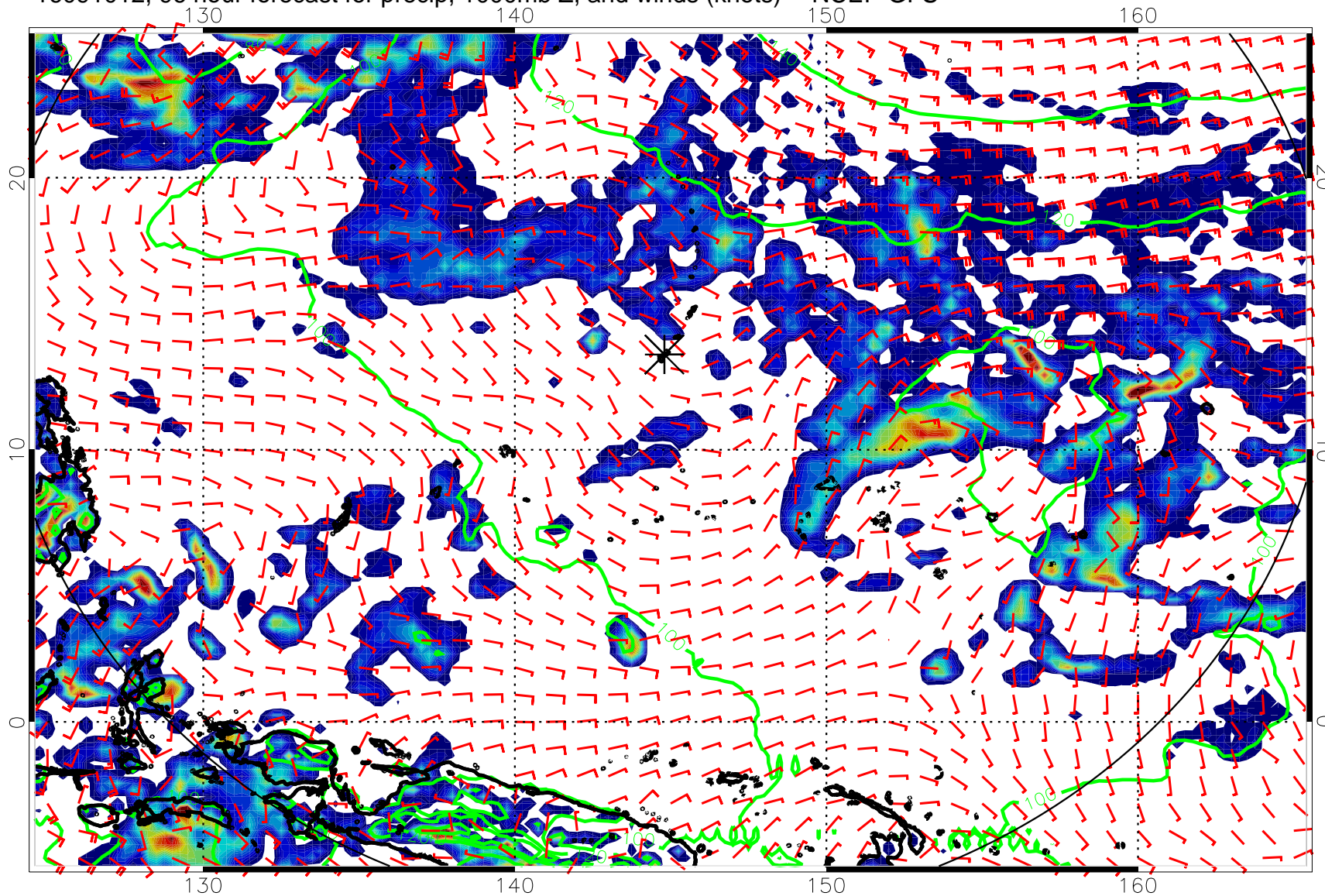
16091012, 96 hour forecast for precip, 1000mb Z, and winds (knots) -- NCEP GFS
