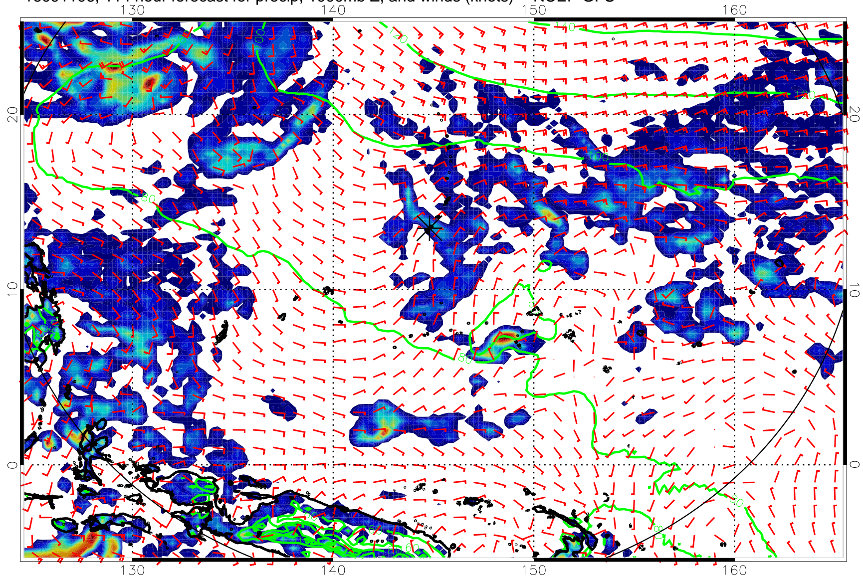
16091106, 114 hour forecast for precip, 1000mb Z, and winds (knots) -- NCEP GFS
