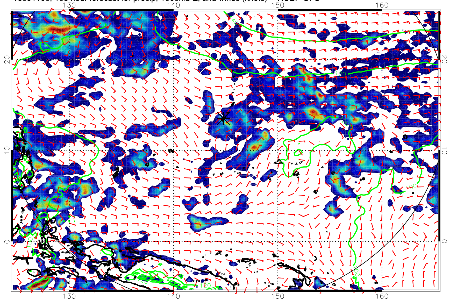
16091100, 108 hour forecast for precip, 1000mb Z, and winds (knots) -- NCEP GFS
