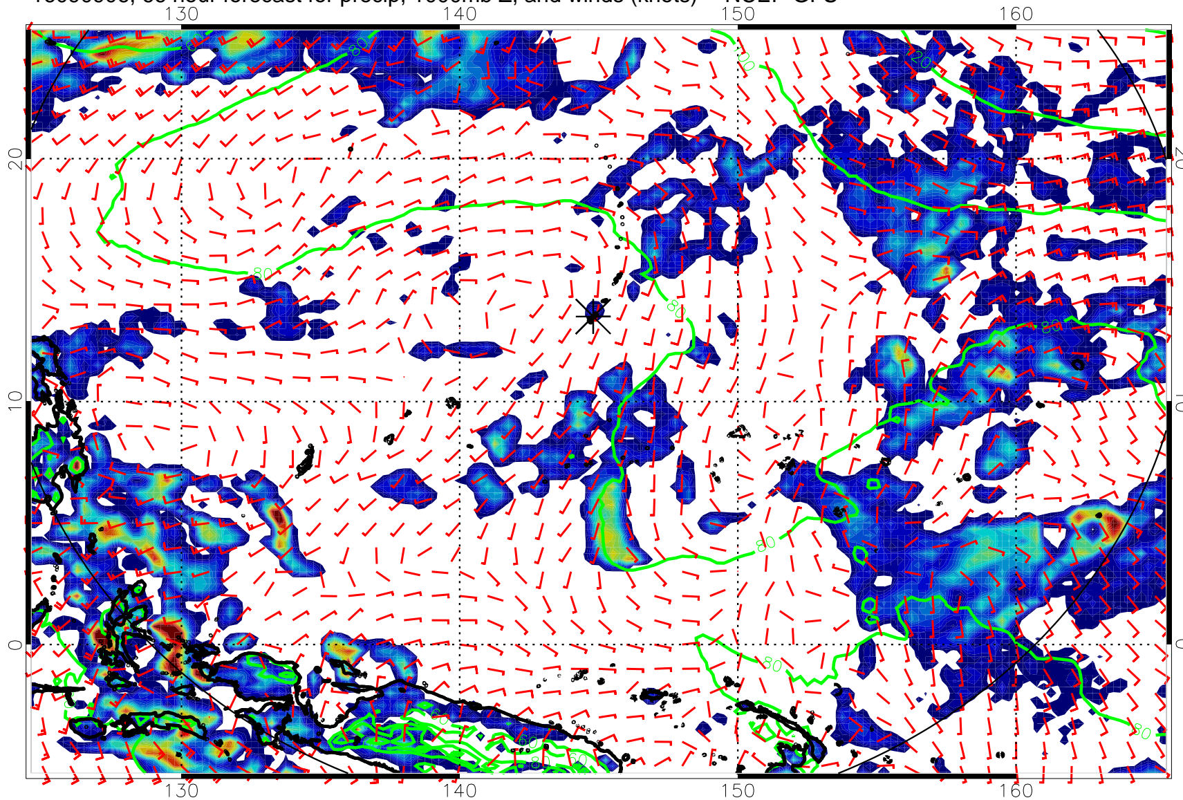
16090906, 66 hour forecast for precip, 1000mb Z, and winds (knots) -- NCEP GFS
