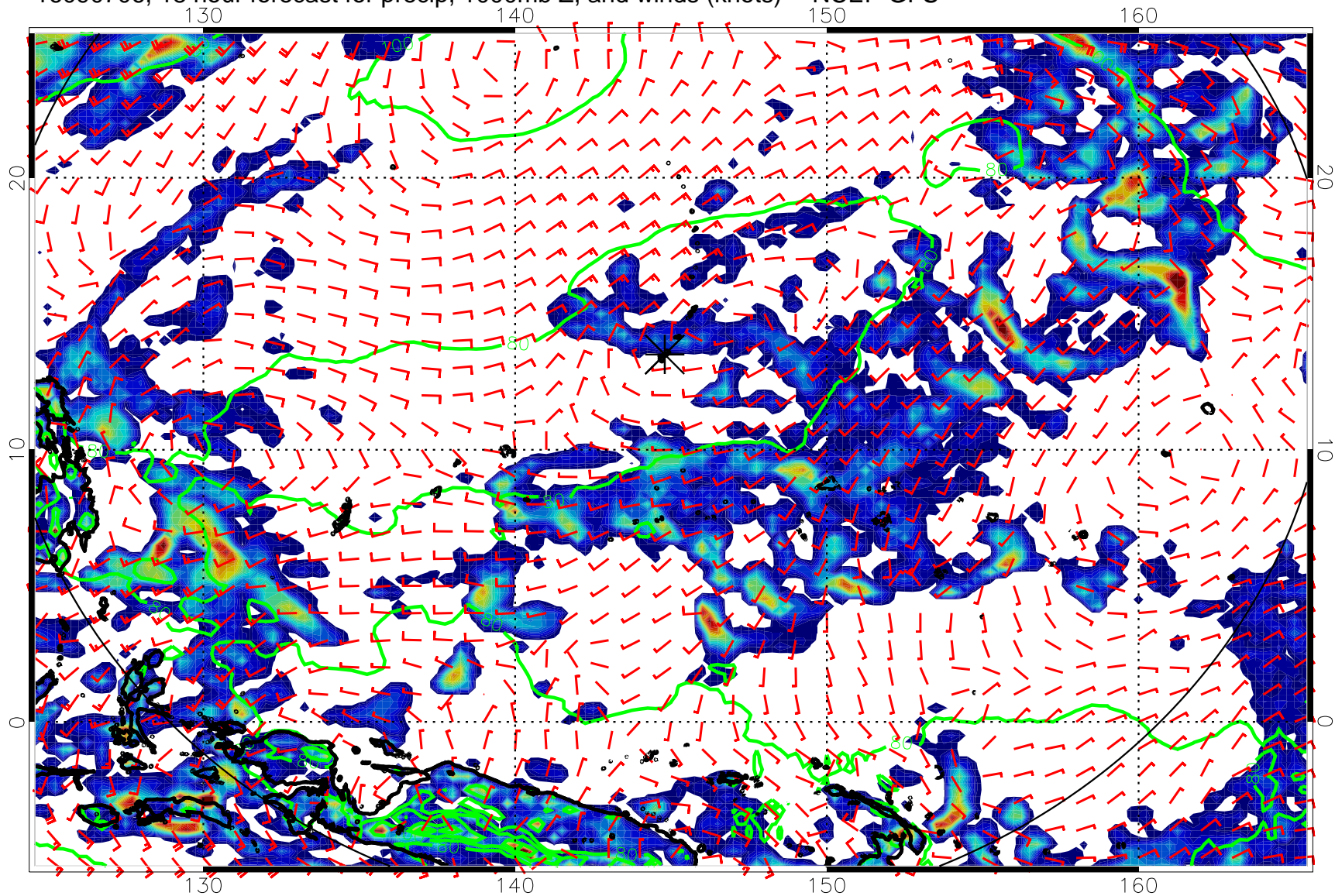
16090706, 18 hour forecast for precip, 1000mb Z, and winds (knots) -- NCEP GFS
