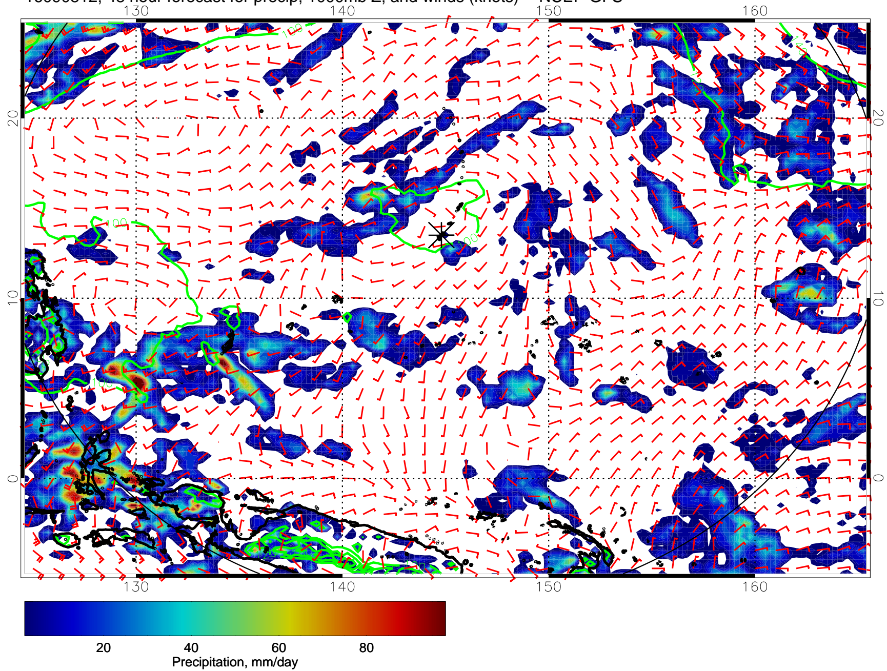
16090812, 48 hour forecast for precip, 1000mb Z, and winds (knots) -- NCEP GFS
