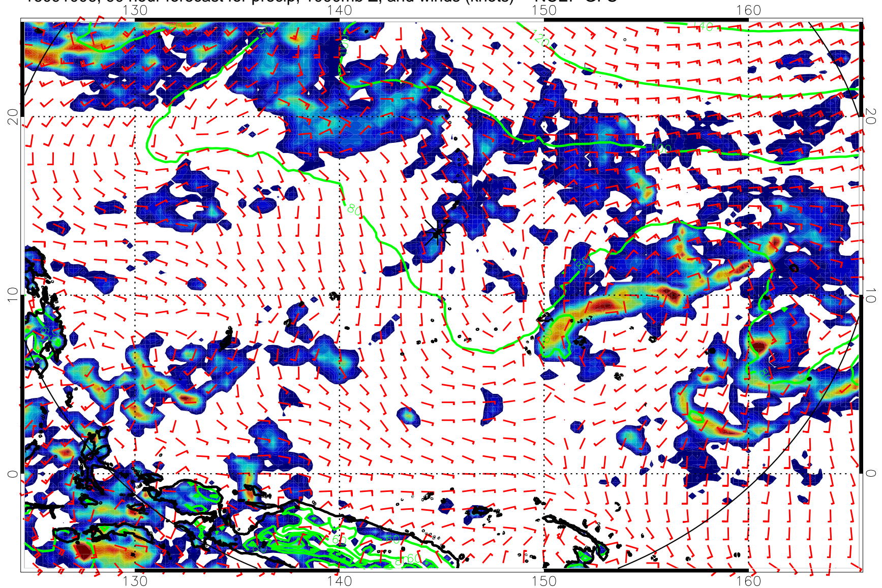
16091006, 90 hour forecast for precip, 1000mb Z, and winds (knots) -- NCEP GFS
