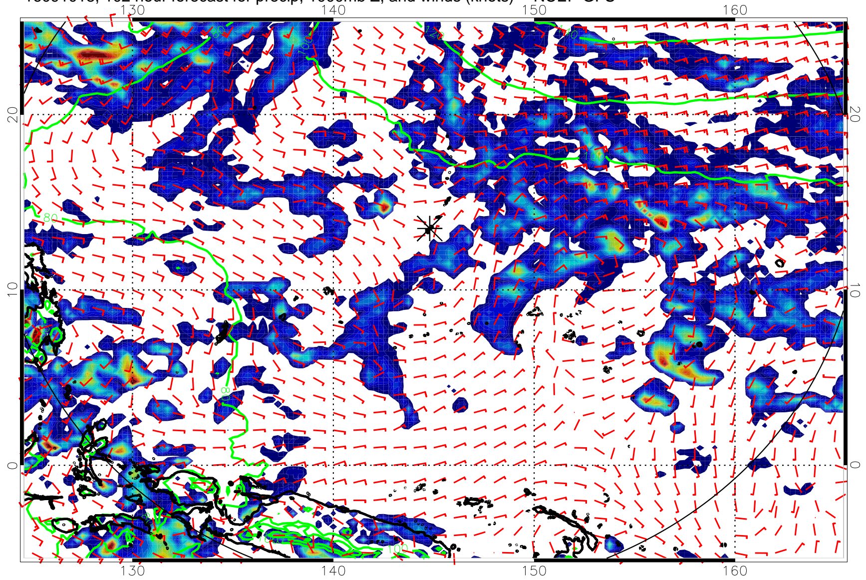
16091018, 102 hour forecast for precip, 1000mb Z, and winds (knots) -- NCEP GFS
