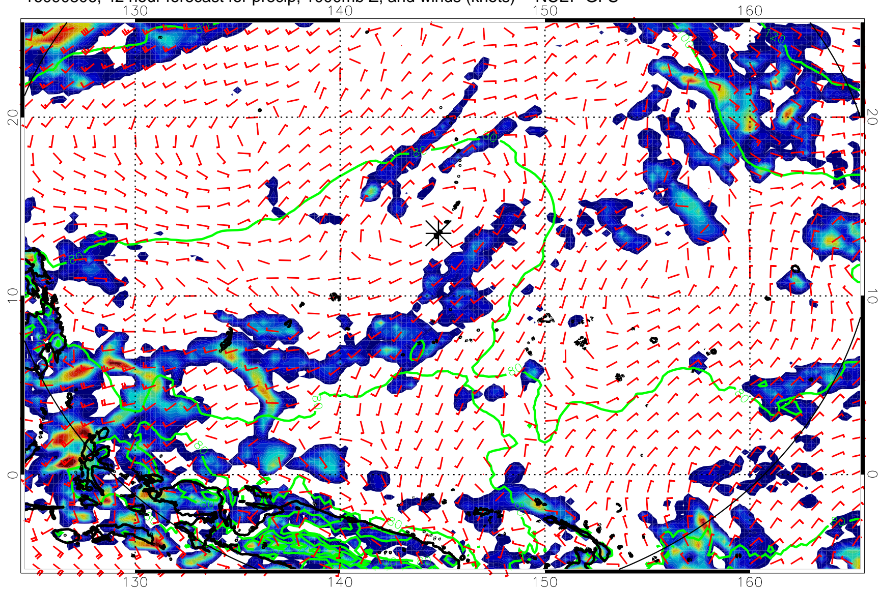
16090806, 42 hour forecast for precip, 1000mb Z, and winds (knots) -- NCEP GFS
