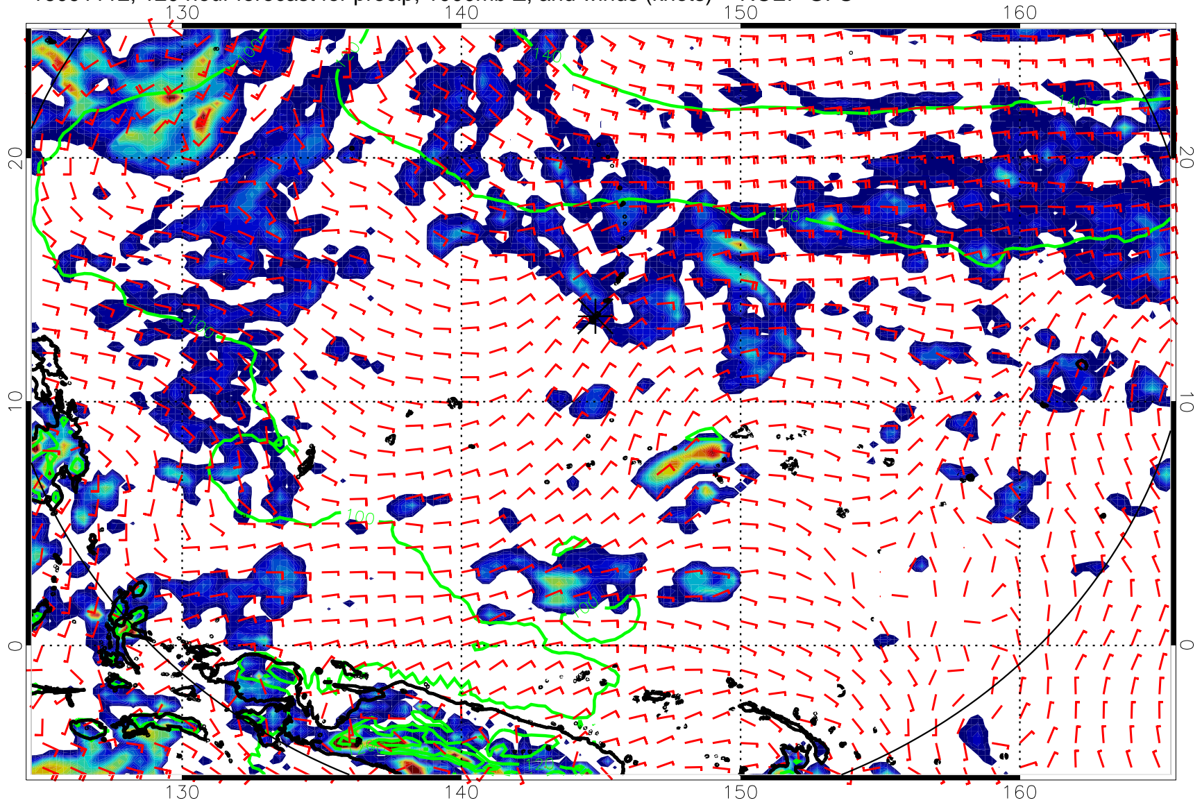
16091112, 120 hour forecast for precip, 1000mb Z, and winds (knots) -- NCEP GFS
