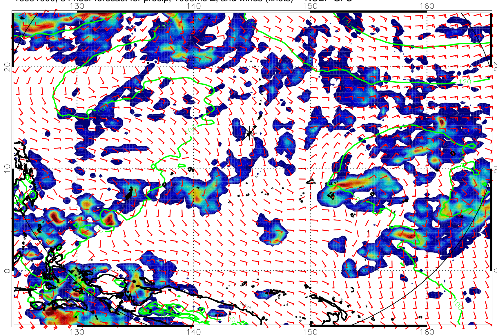
16091000, 84 hour forecast for precip, 1000mb Z, and winds (knots) -- NCEP GFS
