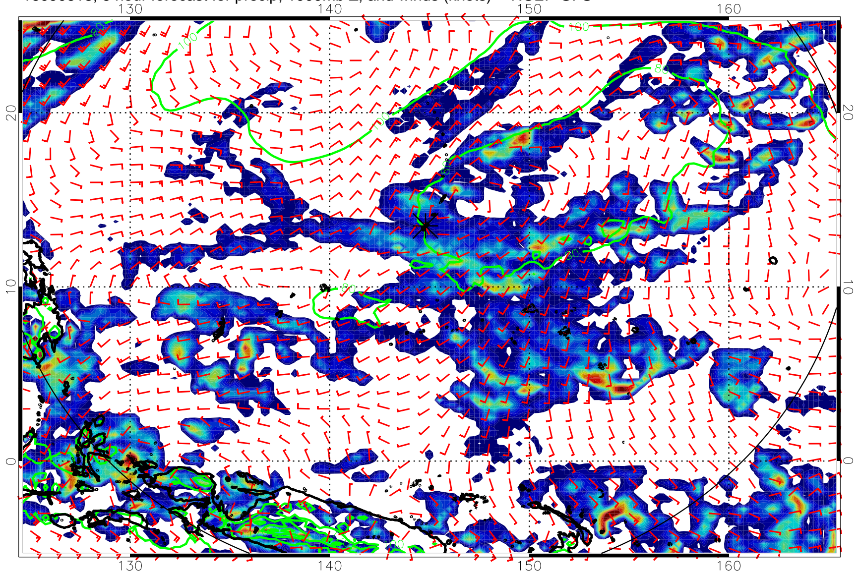
16090618, 6 hour forecast for precip, 1000mb Z, and winds (knots) -- NCEP GFS
