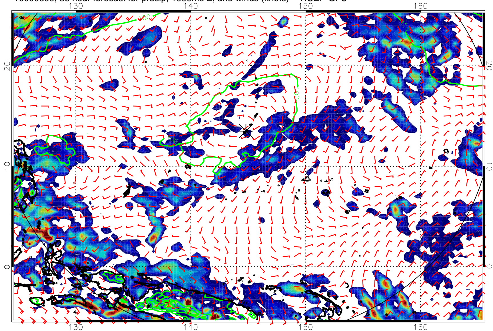
16090800, 36 hour forecast for precip, 1000mb Z, and winds (knots) -- NCEP GFS
