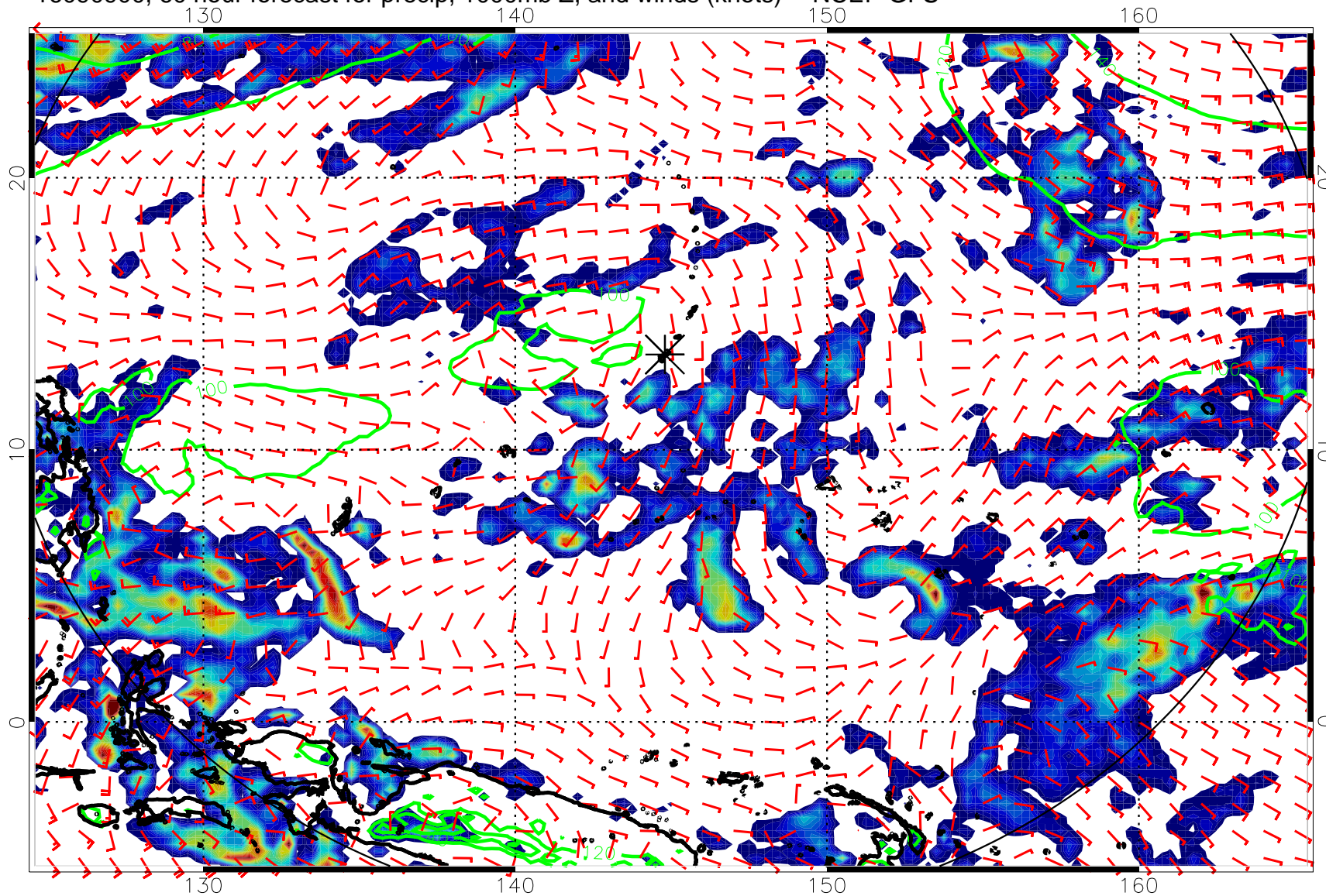
16090900, 60 hour forecast for precip, 1000mb Z, and winds (knots) -- NCEP GFS
