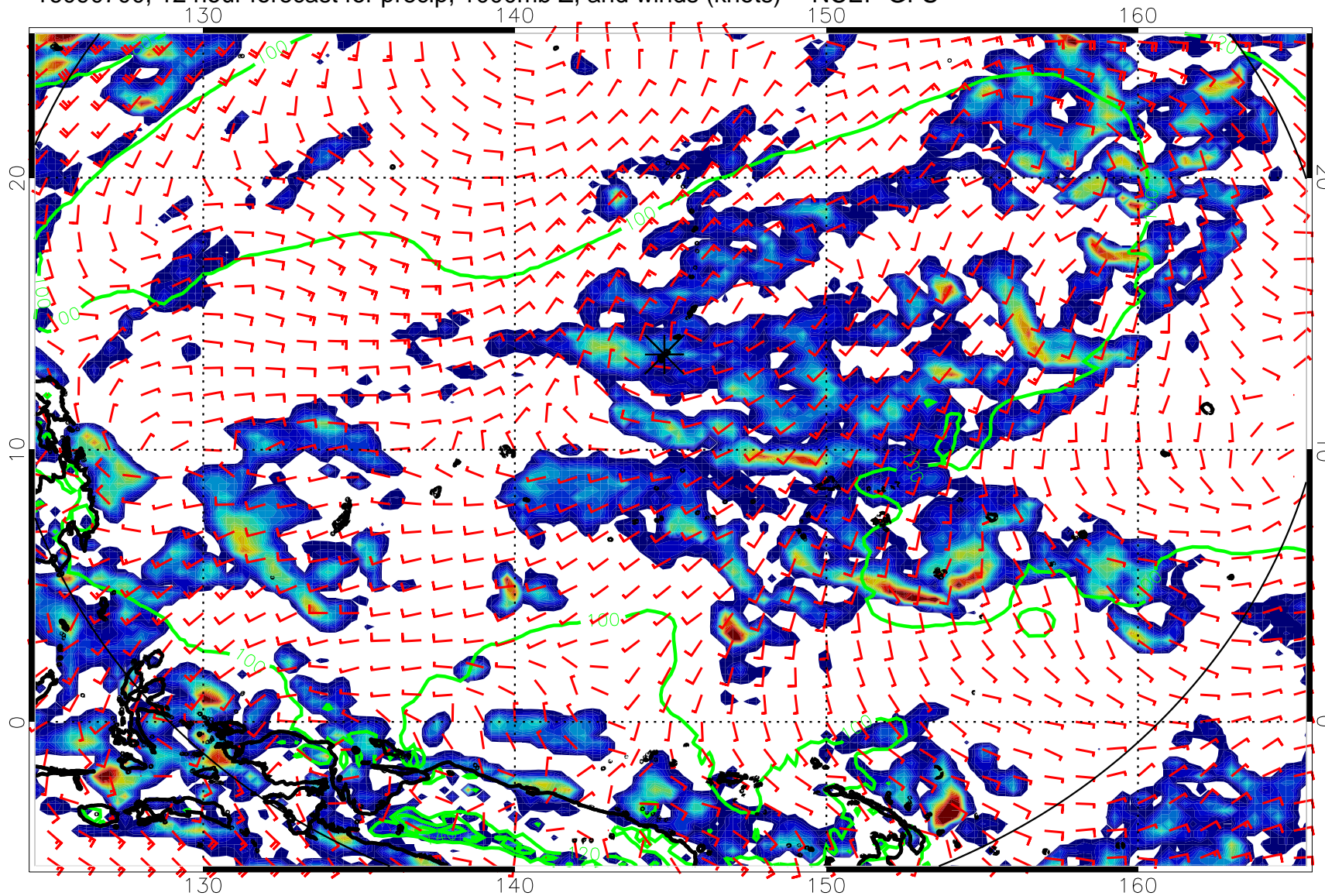
16090700, 12 hour forecast for precip, 1000mb Z, and winds (knots) -- NCEP GFS
