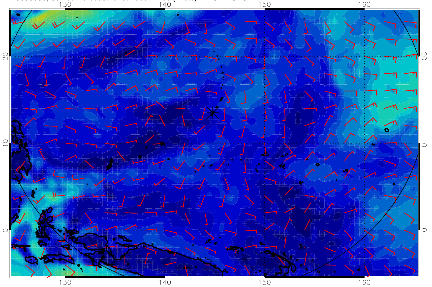
16090900, 60 hour forecast for surface winds (knots) -- NCEP GFS
