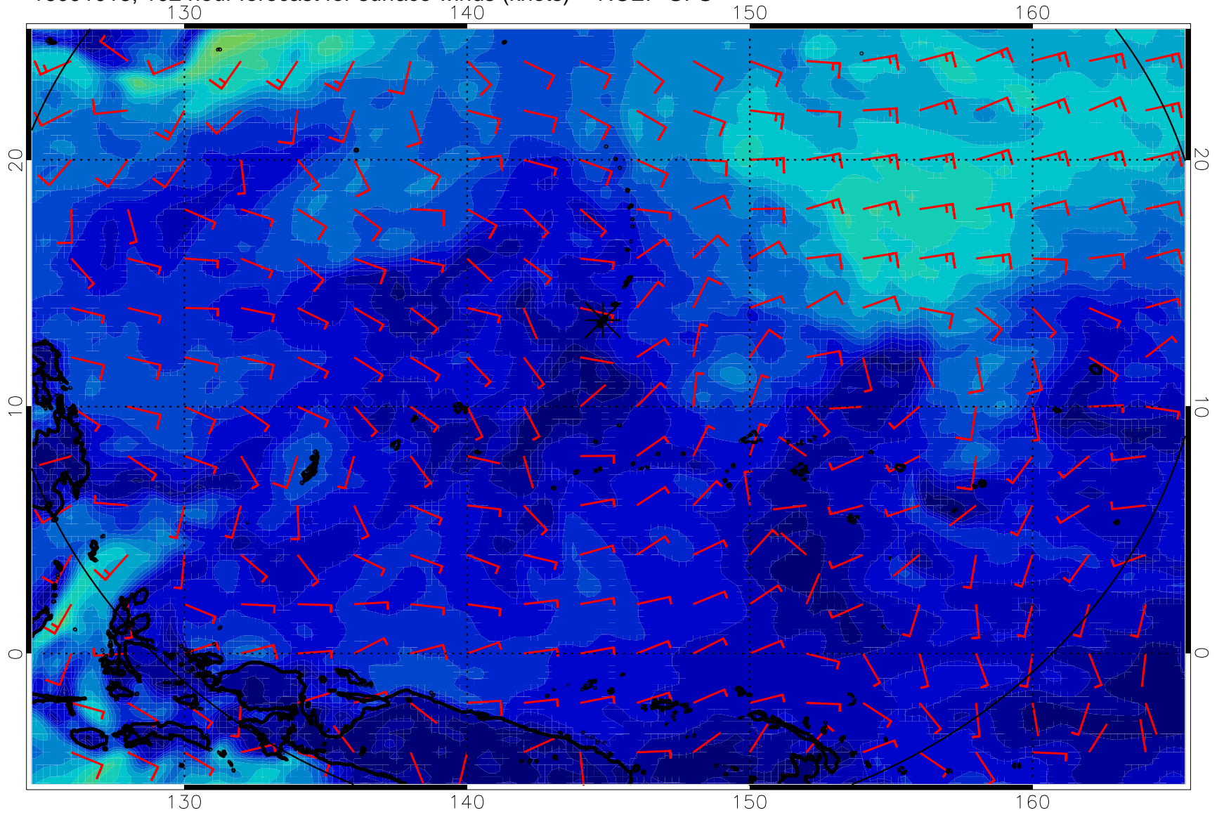
16091018, 102 hour forecast for surface winds (knots) -- NCEP GFS
