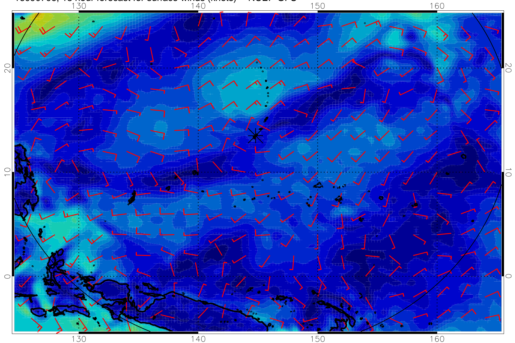
16090706, 18 hour forecast for surface winds (knots) -- NCEP GFS
