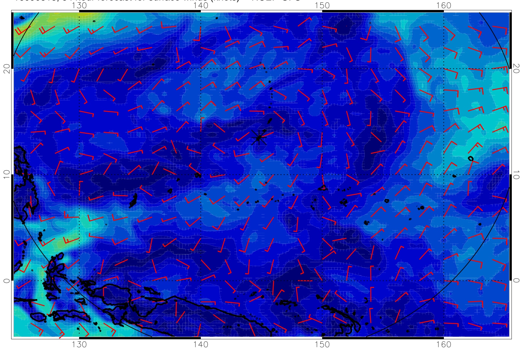
16090818, 54 hour forecast for surface winds (knots) -- NCEP GFS
