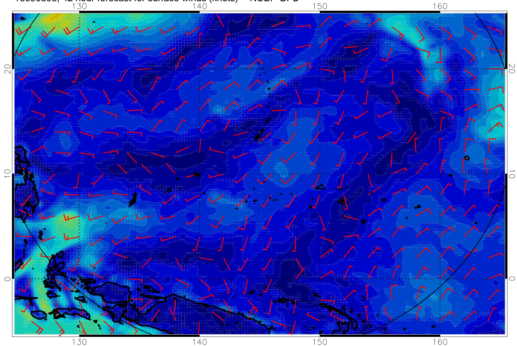
16090806, 42 hour forecast for surface winds (knots) -- NCEP GFS
