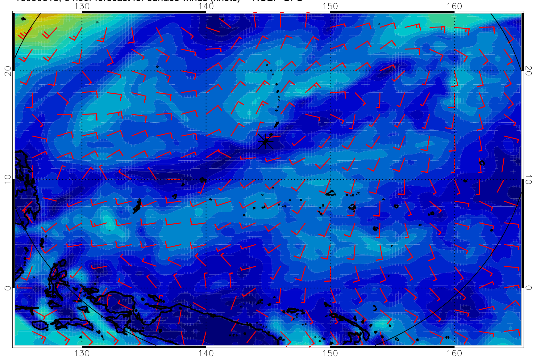
16090618, 6 hour forecast for surface winds (knots) -- NCEP GFS
