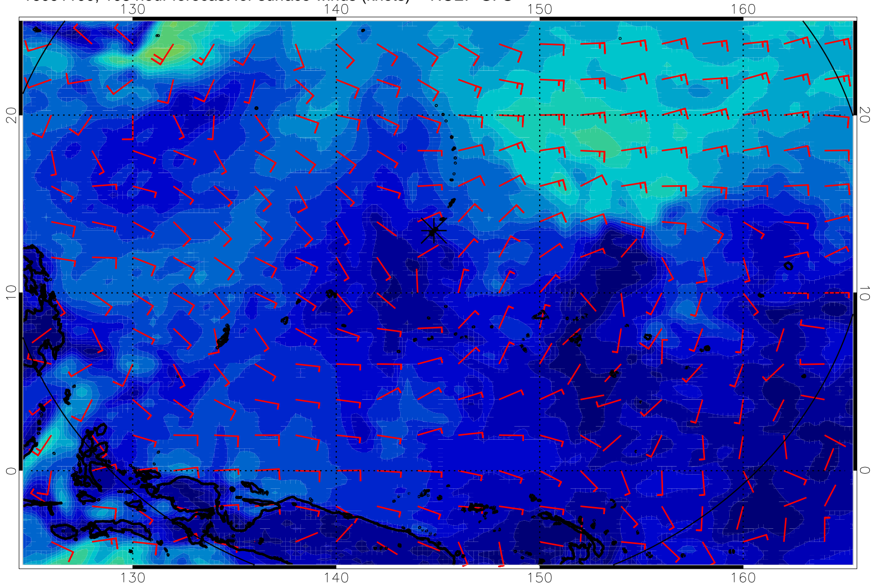
16091100, 108 hour forecast for surface winds (knots) -- NCEP GFS
