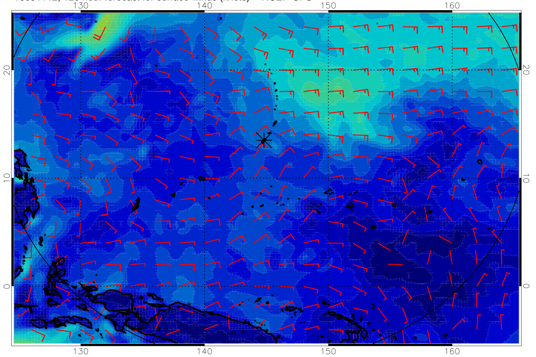
16091112, 120 hour forecast for surface winds (knots) -- NCEP GFS
