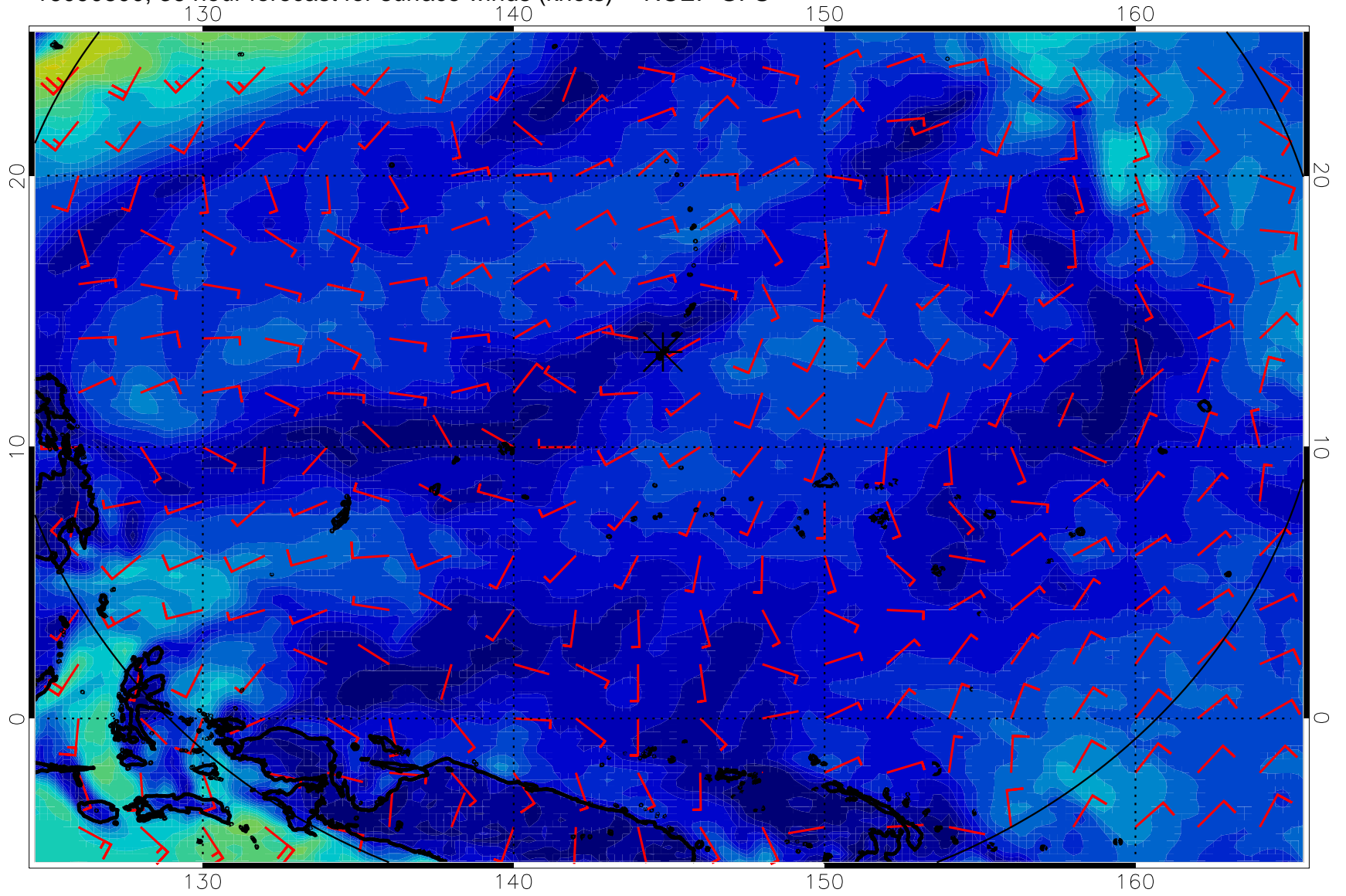
16090800, 36 hour forecast for surface winds (knots) -- NCEP GFS
