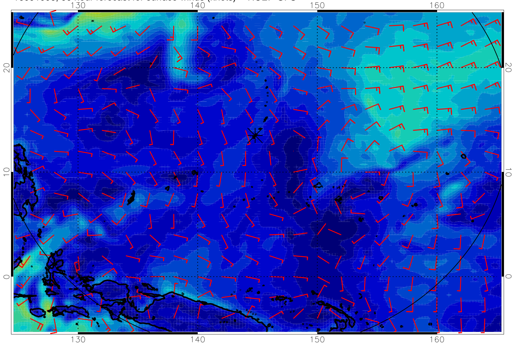
16091006, 90 hour forecast for surface winds (knots) -- NCEP GFS
