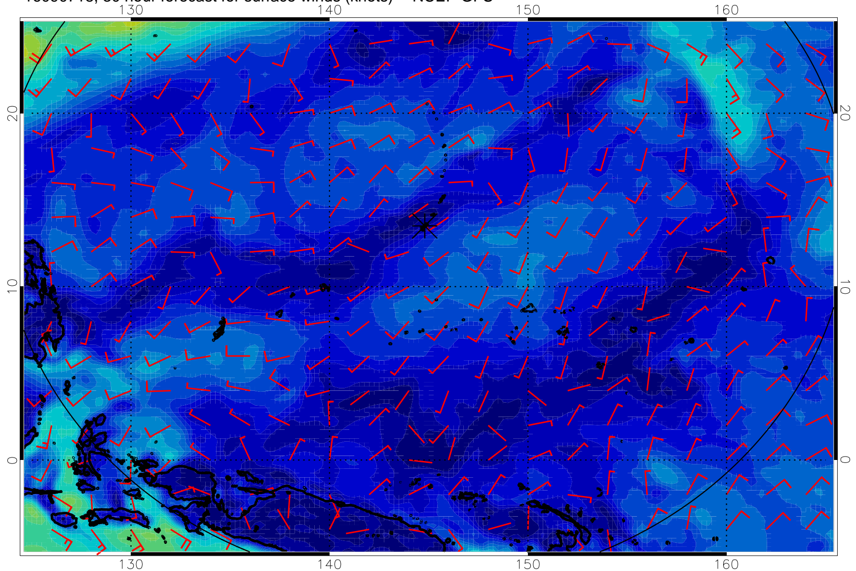
16090718, 30 hour forecast for surface winds (knots) -- NCEP GFS
