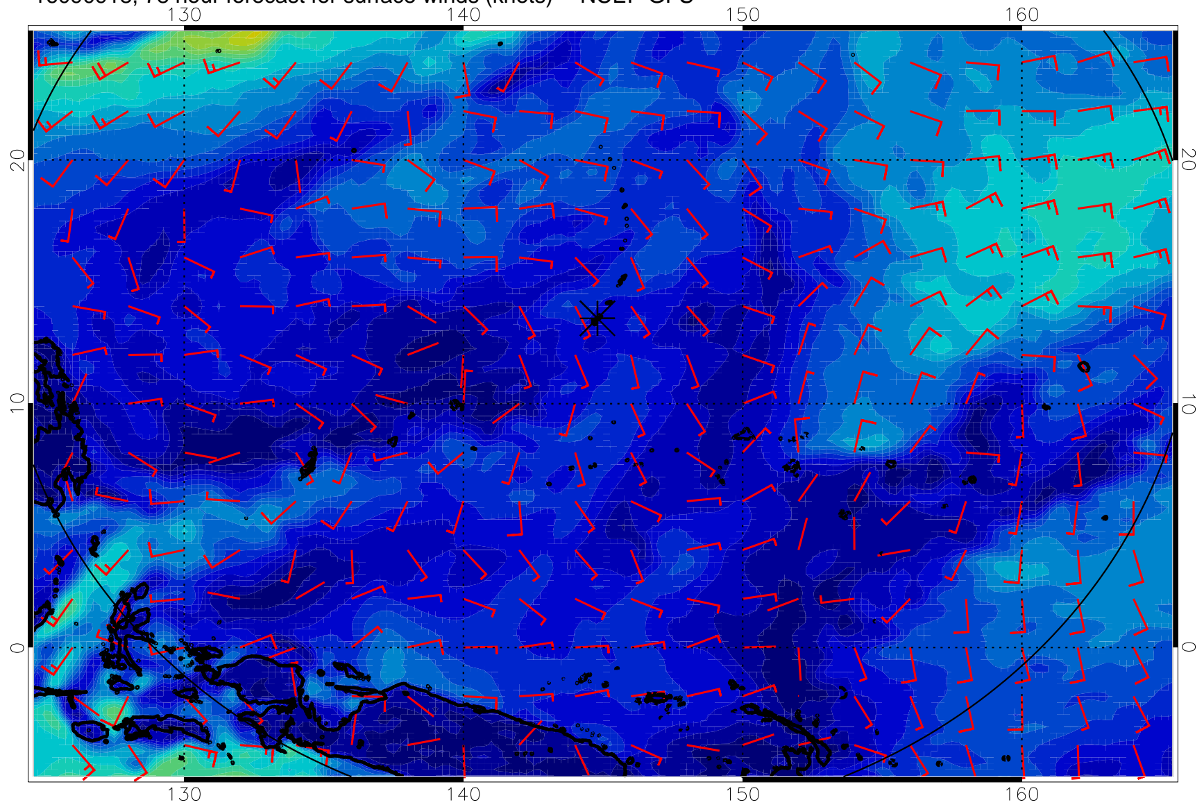
16090918, 78 hour forecast for surface winds (knots) -- NCEP GFS
