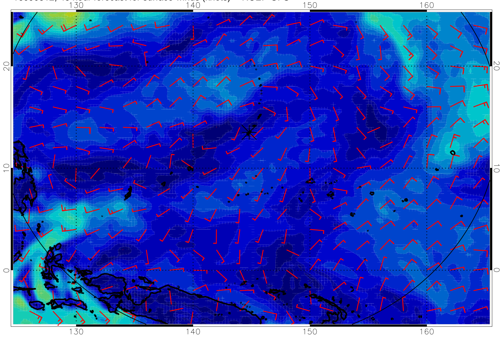
16090812, 48 hour forecast for surface winds (knots) -- NCEP GFS
