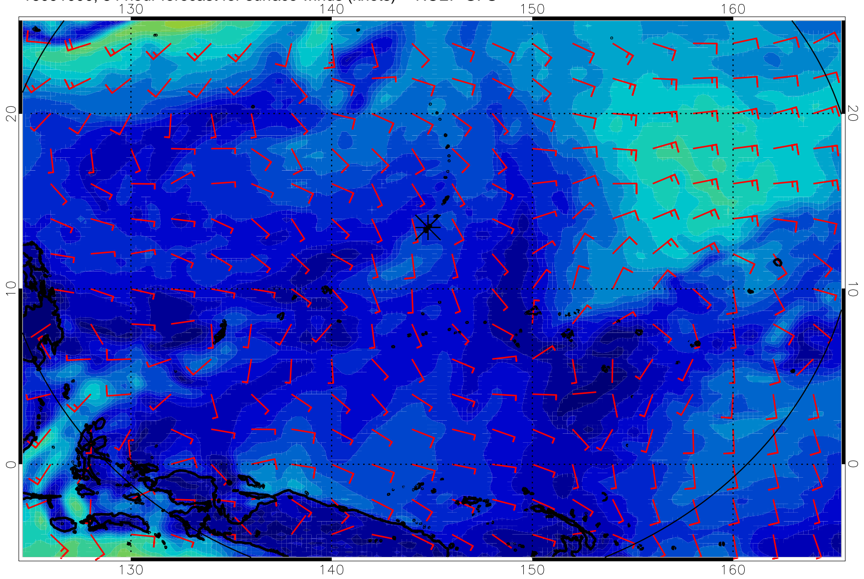
16091000, 84 hour forecast for surface winds (knots) -- NCEP GFS
