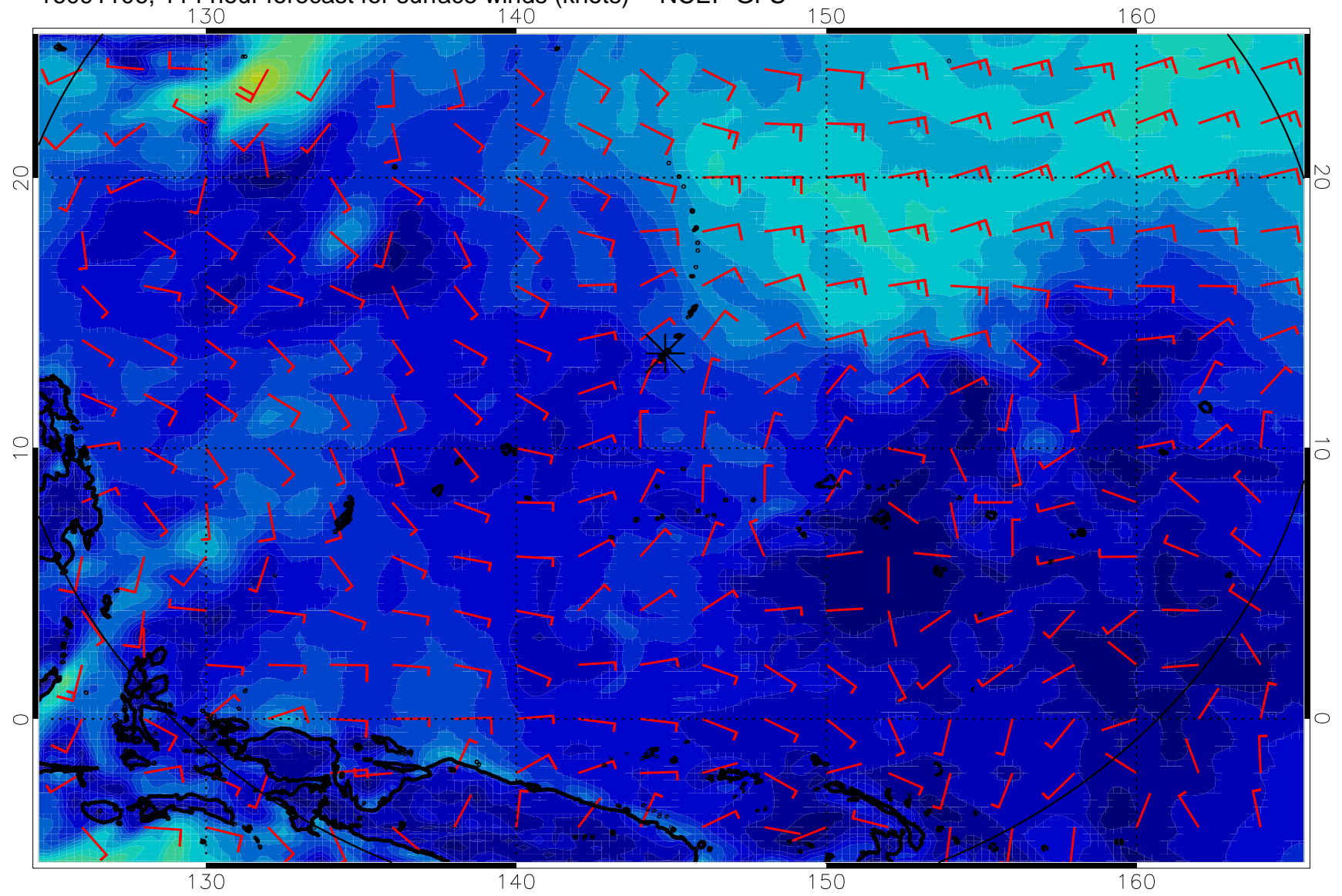
16091106, 114 hour forecast for surface winds (knots) -- NCEP GFS
