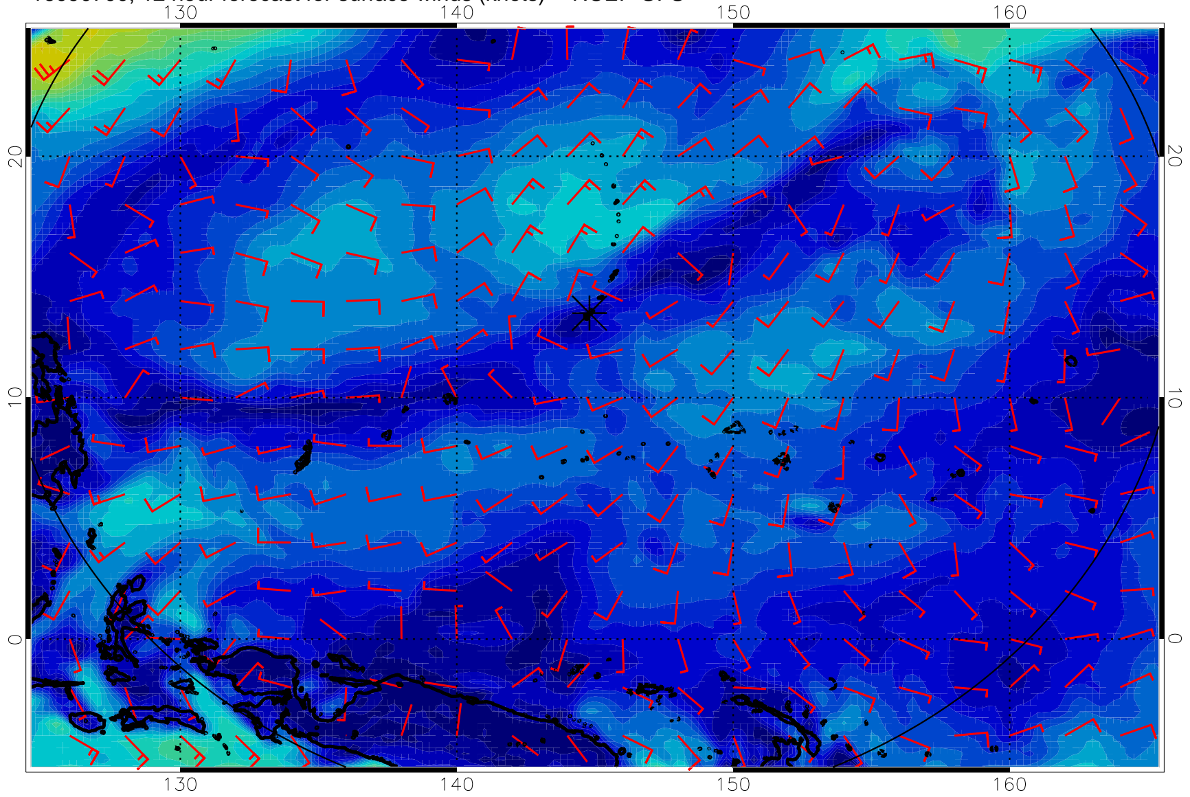
16090700, 12 hour forecast for surface winds (knots) -- NCEP GFS
