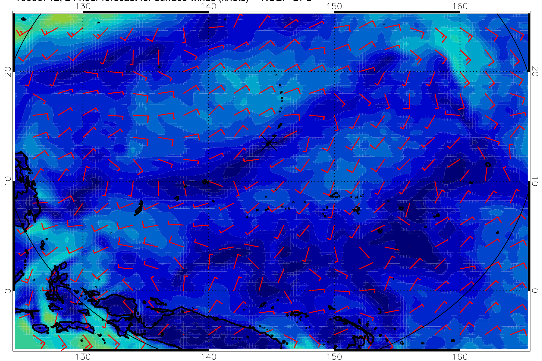
16090712, 24 hour forecast for surface winds (knots) -- NCEP GFS
