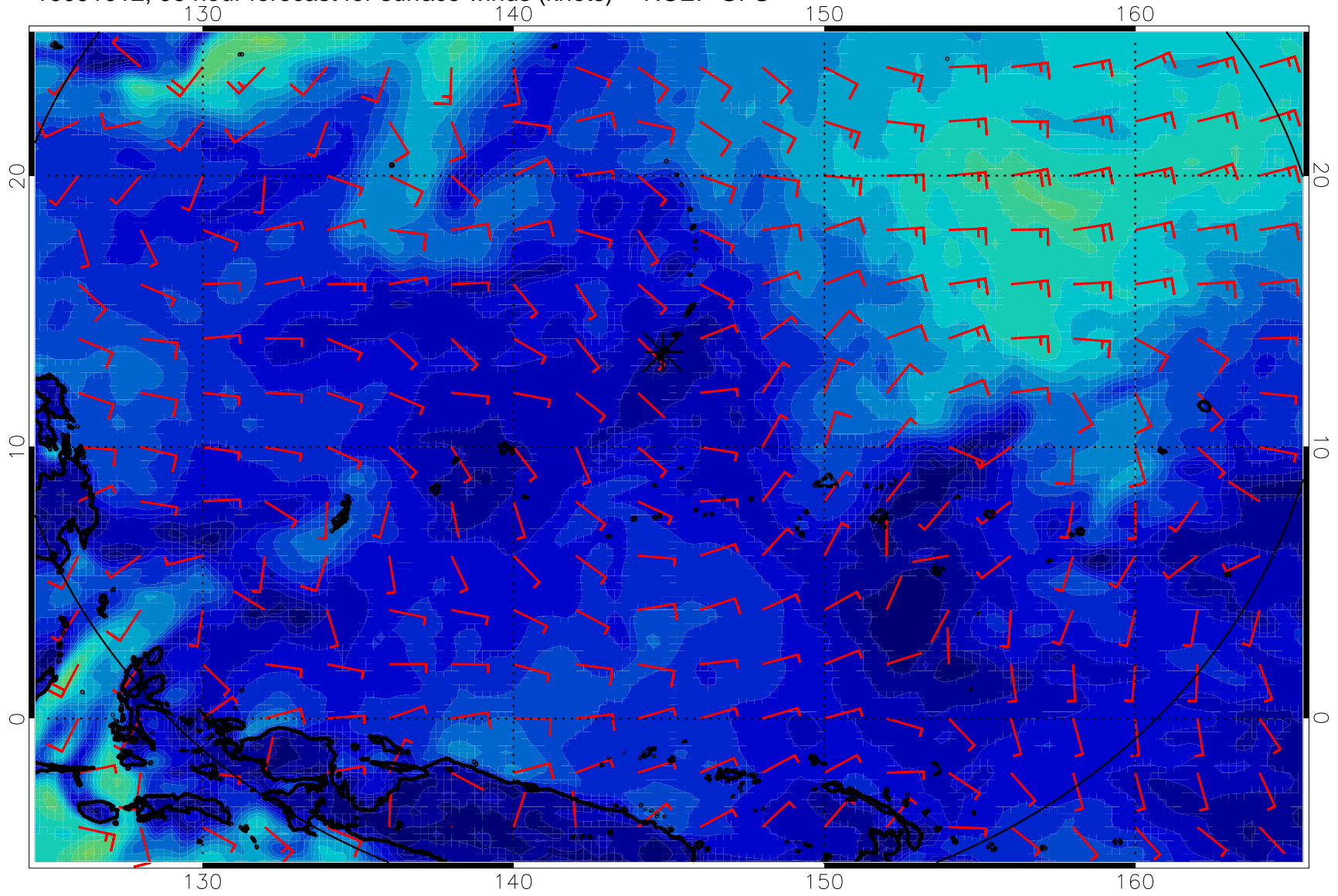
16091012, 96 hour forecast for surface winds (knots) -- NCEP GFS
