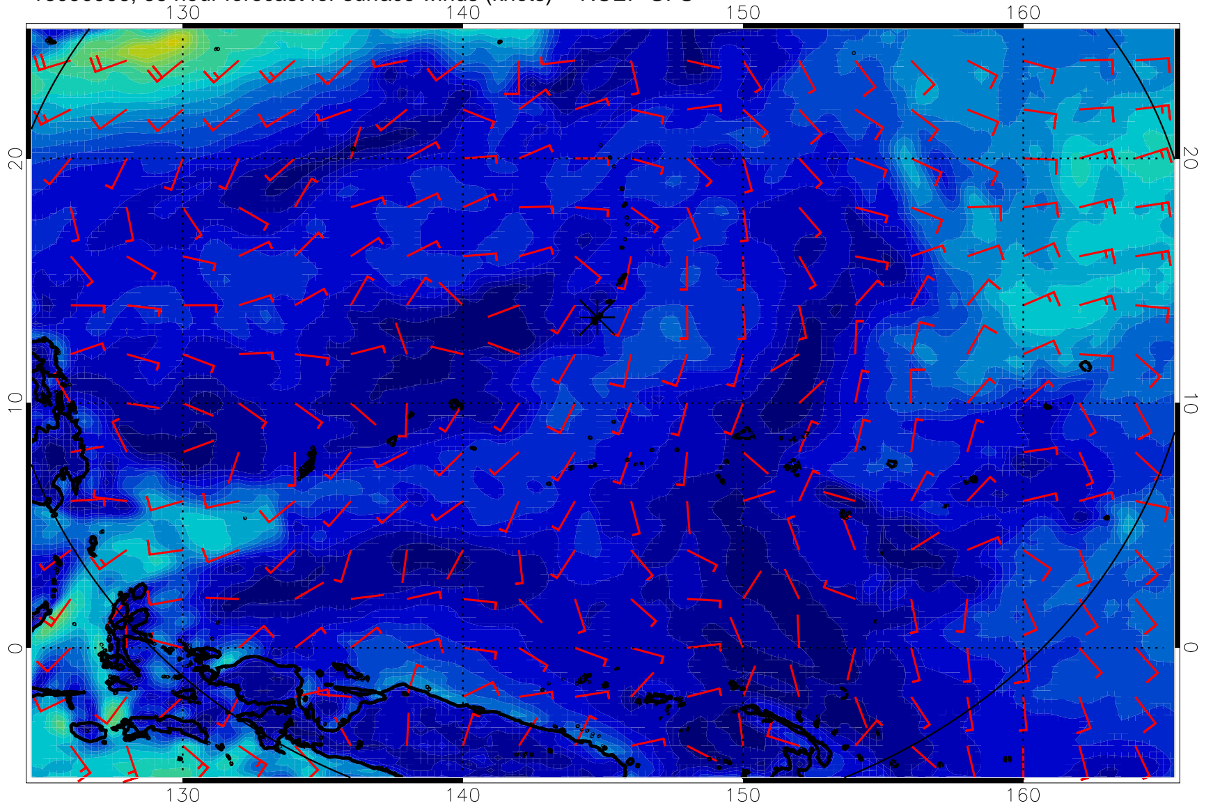
16090906, 66 hour forecast for surface winds (knots) -- NCEP GFS
