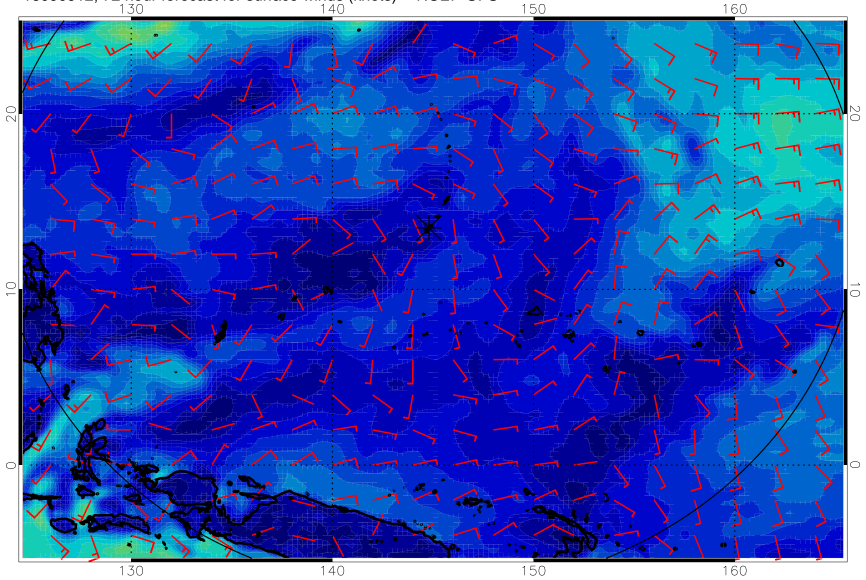
16090912, 72 hour forecast for surface winds (knots) -- NCEP GFS
