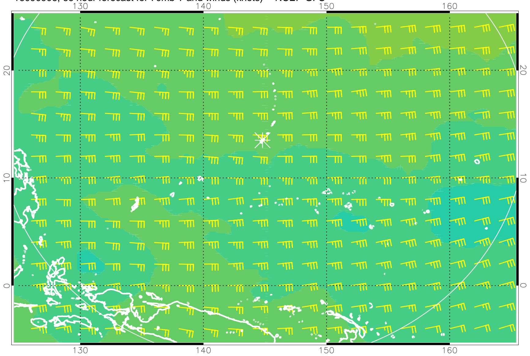
16090906, 66 hour forecast for 70mb T and winds (knots) -- NCEP GFS
