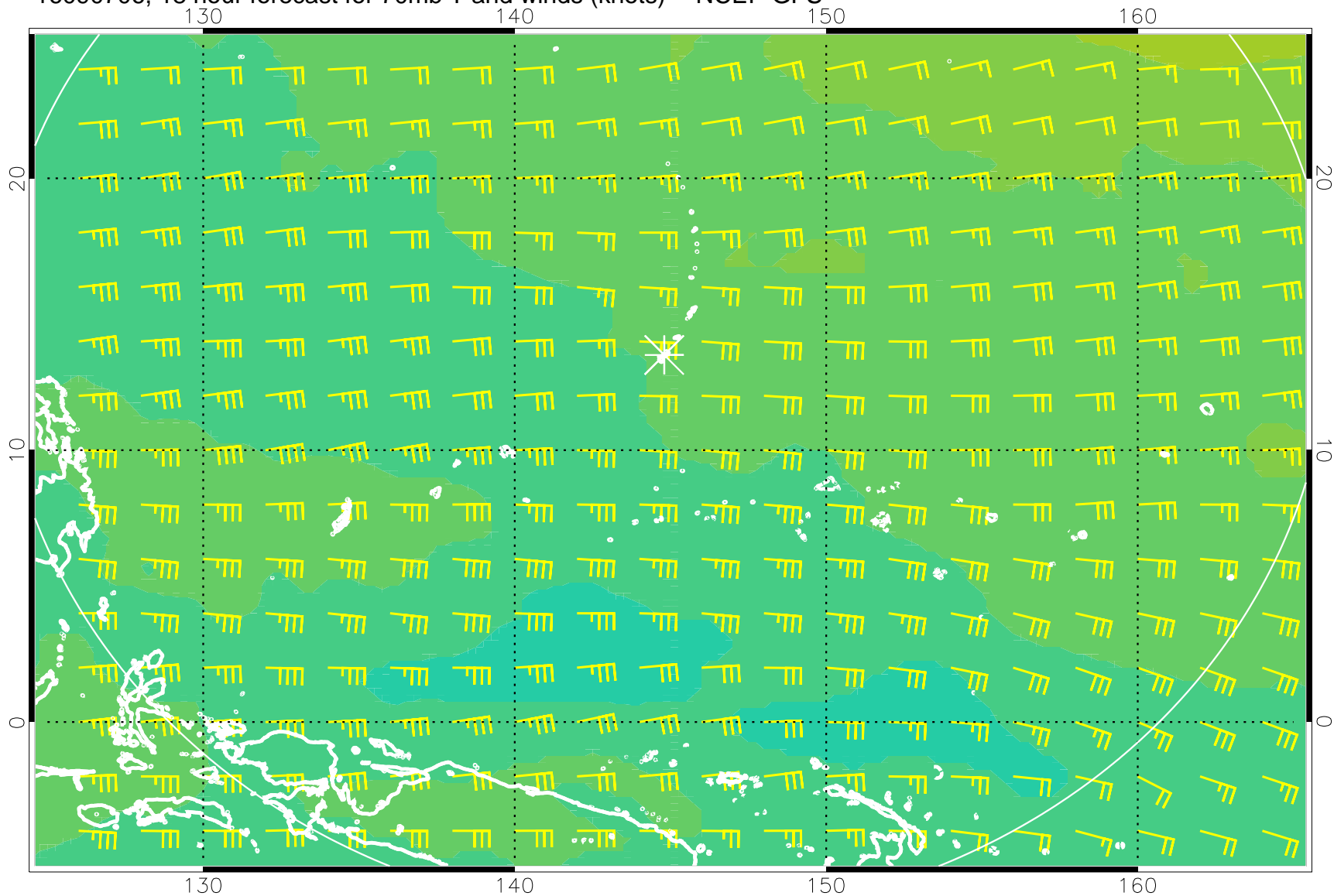
16090706, 18 hour forecast for 70mb T and winds (knots) -- NCEP GFS
