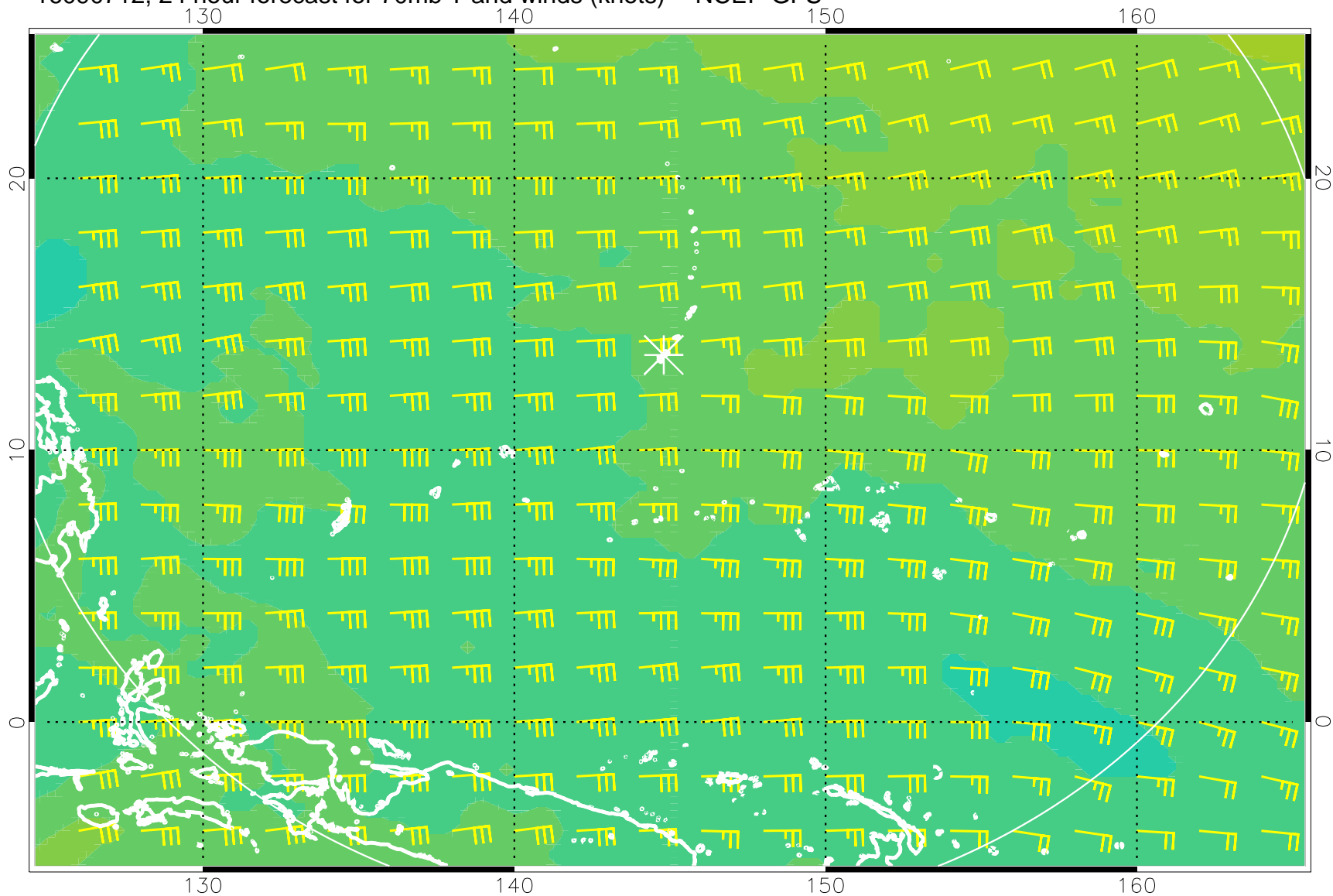
16090712, 24 hour forecast for 70mb T and winds (knots) -- NCEP GFS
