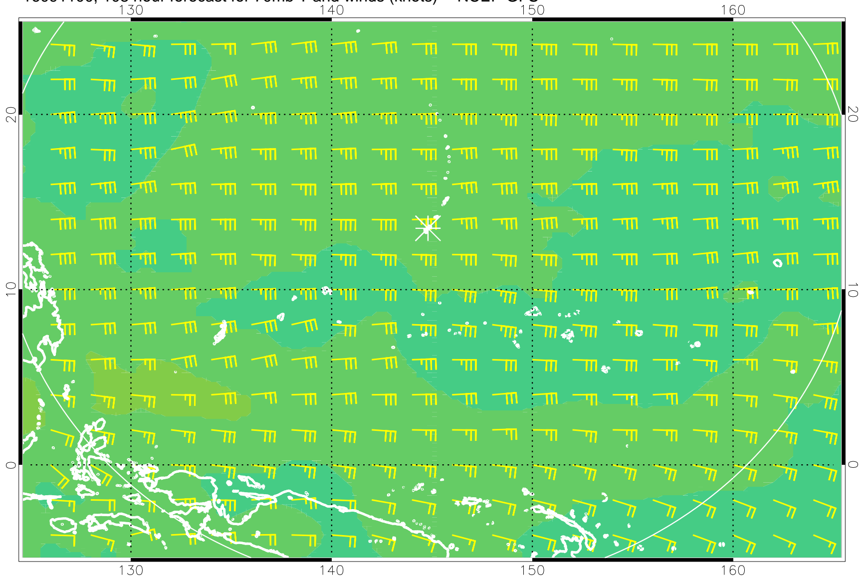
16091100, 108 hour forecast for 70mb T and winds (knots) -- NCEP GFS
