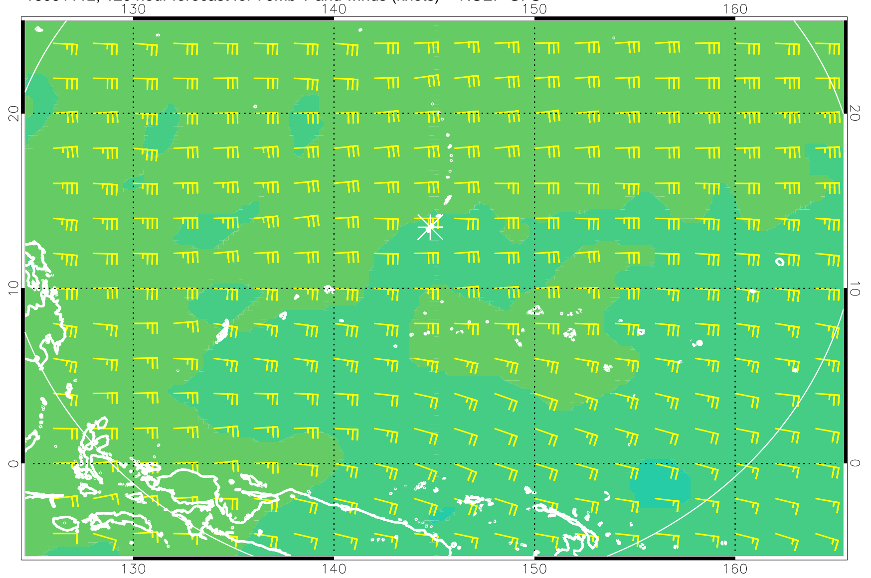
16091112, 120 hour forecast for 70mb T and winds (knots) -- NCEP GFS
