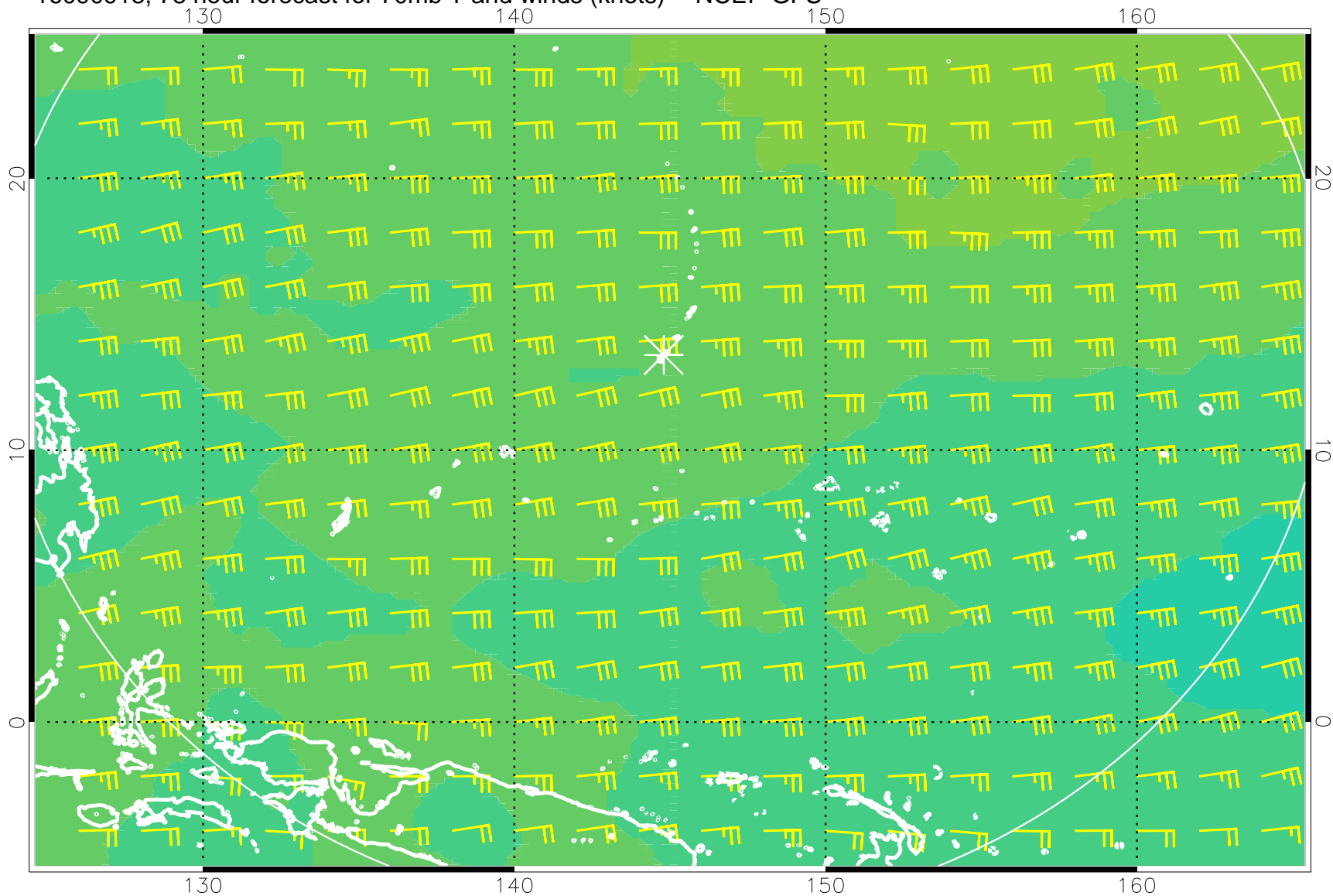
16090918, 78 hour forecast for 70mb T and winds (knots) -- NCEP GFS
