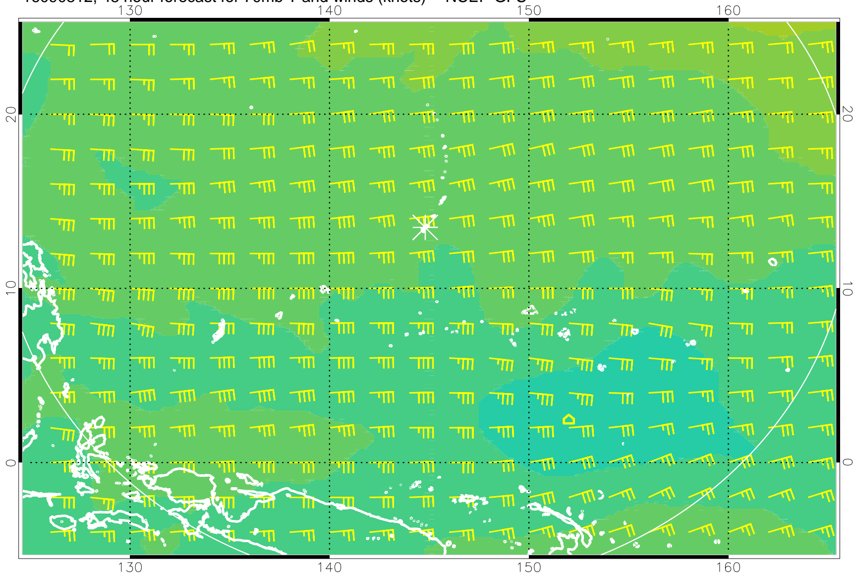
16090812, 48 hour forecast for 70mb T and winds (knots) -- NCEP GFS
