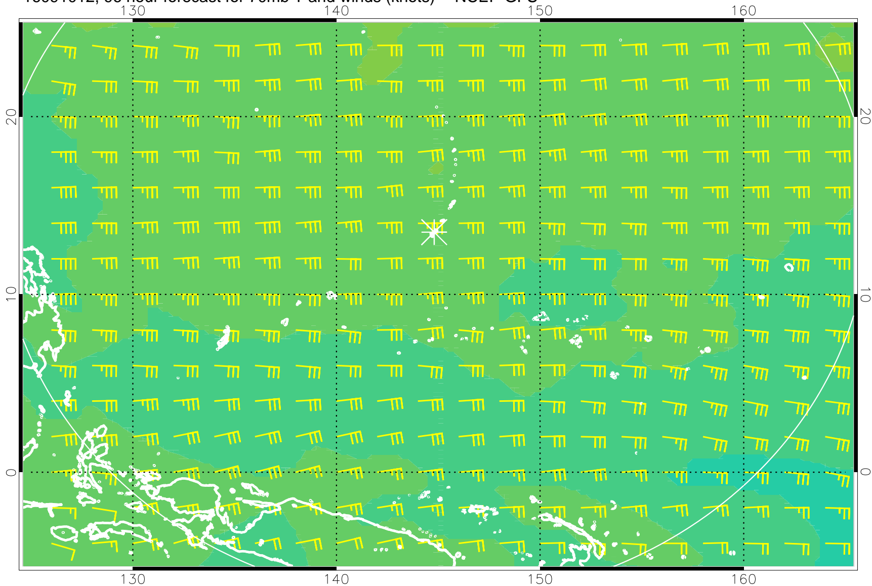
16091012, 96 hour forecast for 70mb T and winds (knots) -- NCEP GFS
