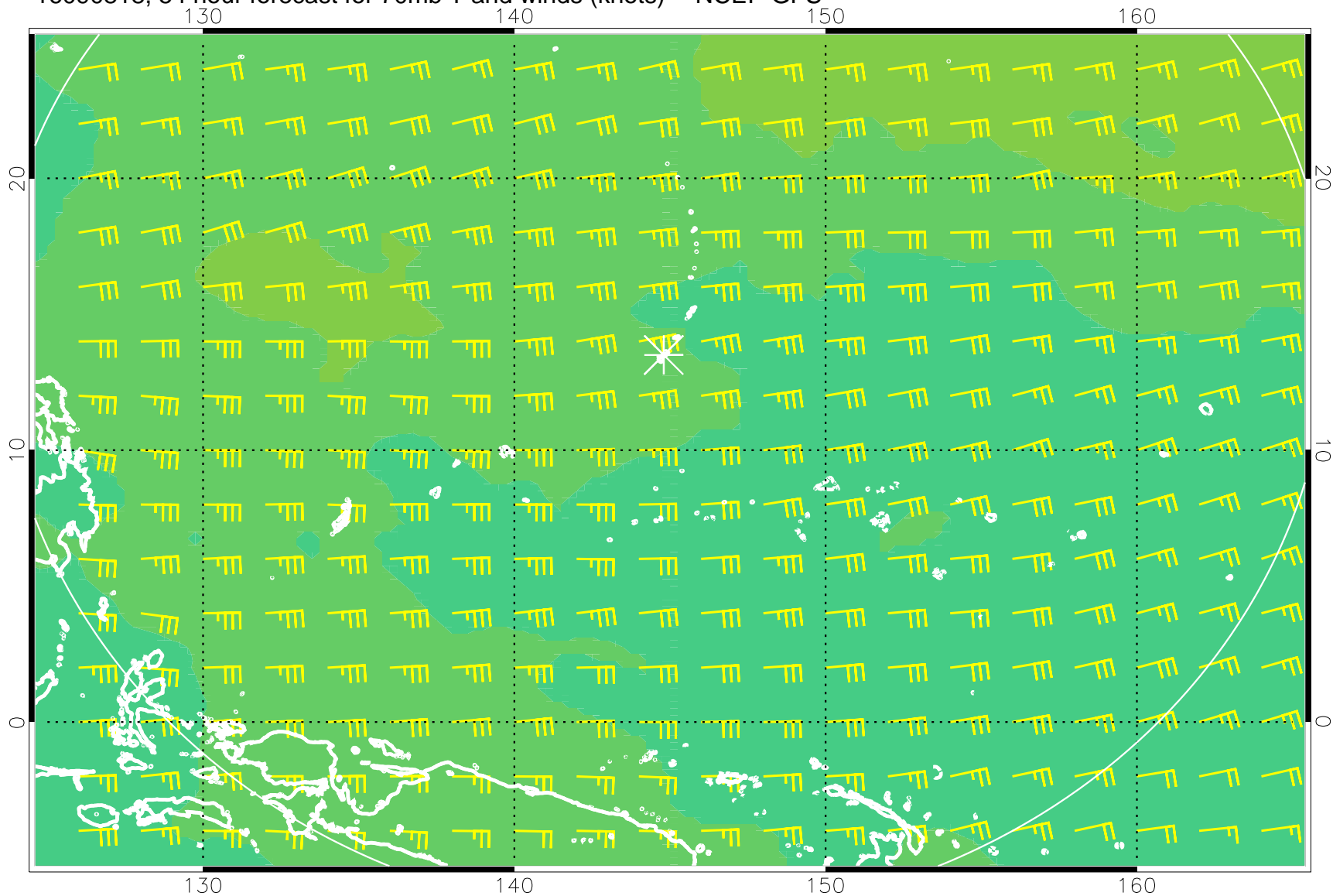
16090818, 54 hour forecast for 70mb T and winds (knots) -- NCEP GFS
