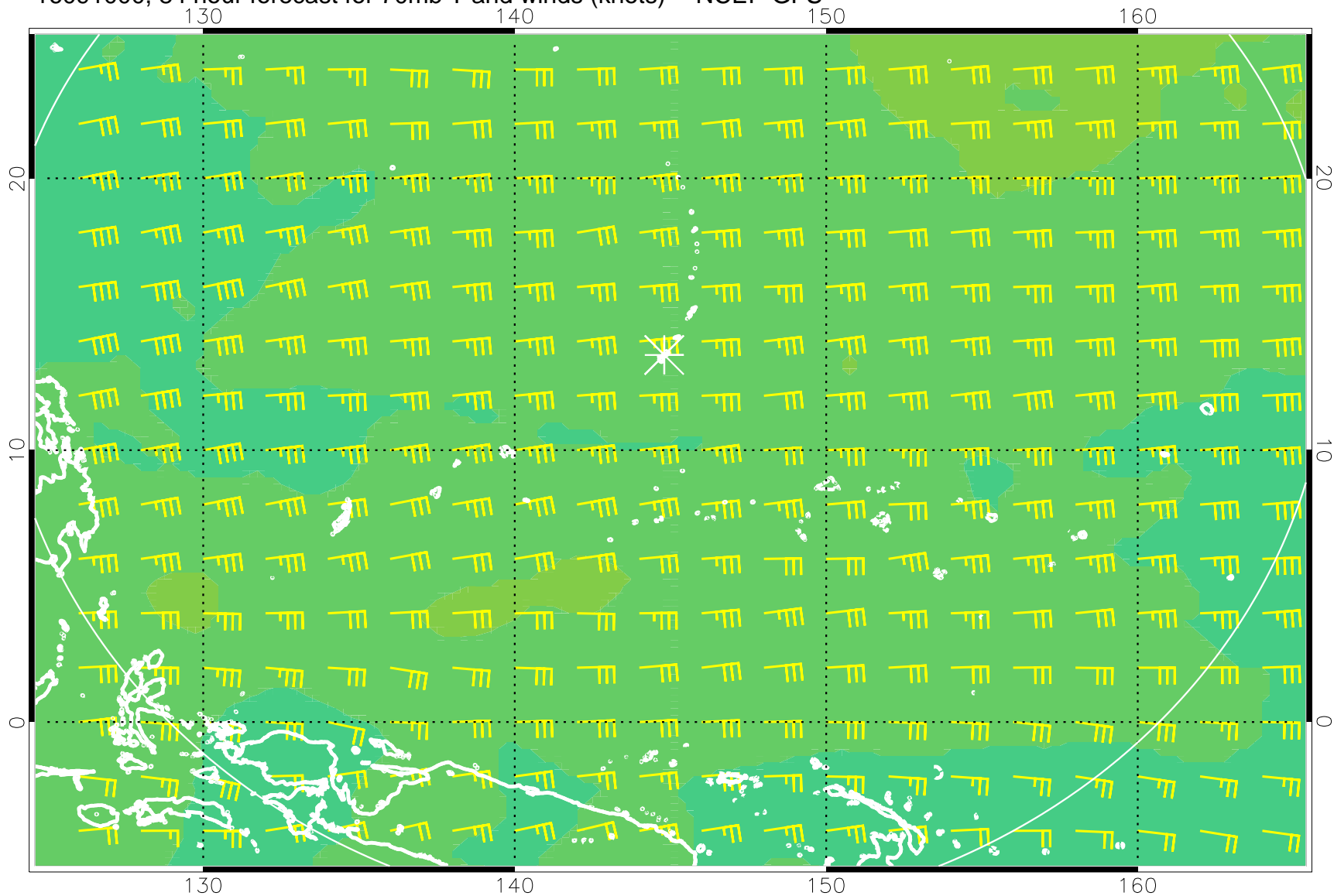
16091000, 84 hour forecast for 70mb T and winds (knots) -- NCEP GFS
