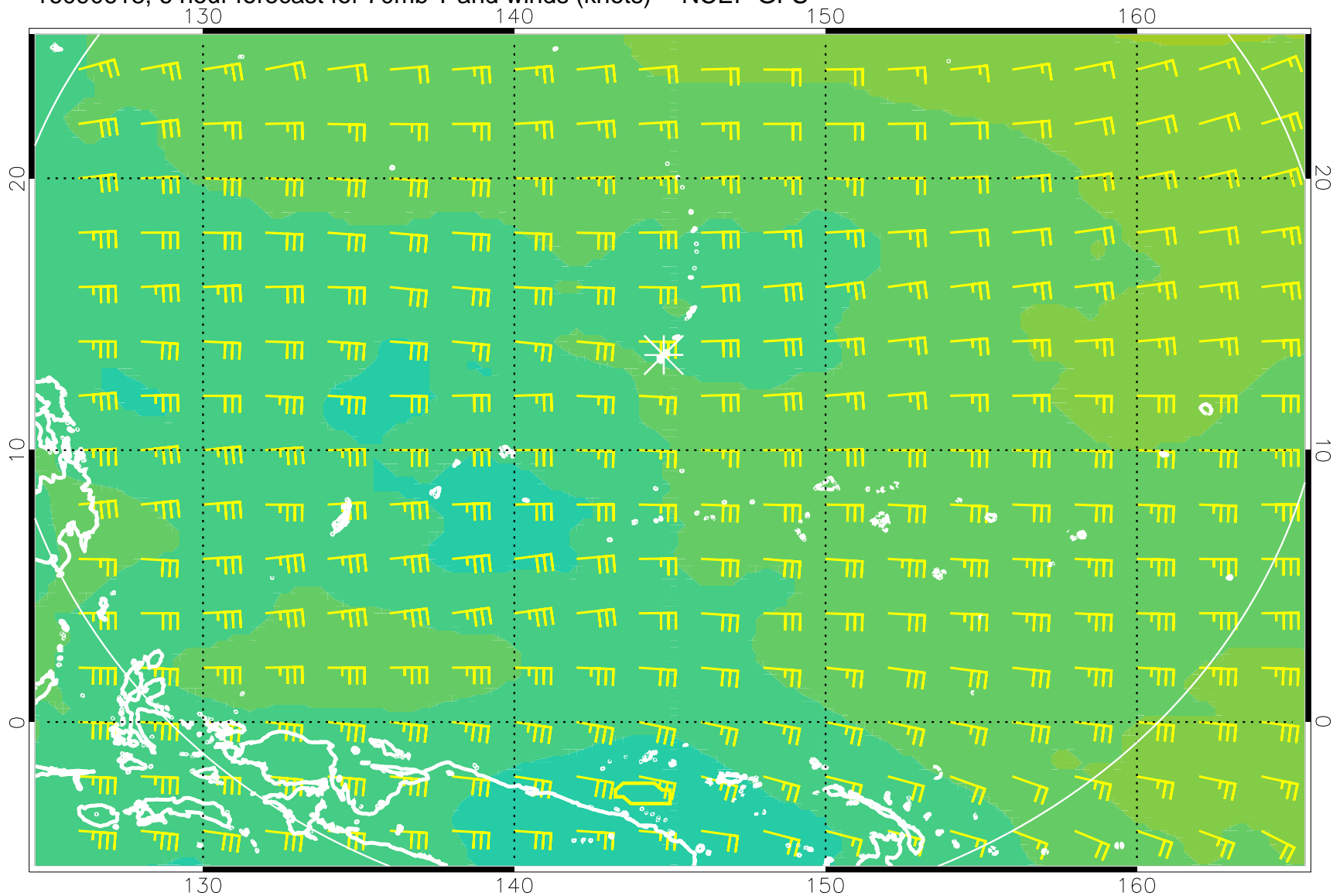
16090618, 6 hour forecast for 70mb T and winds (knots) -- NCEP GFS
