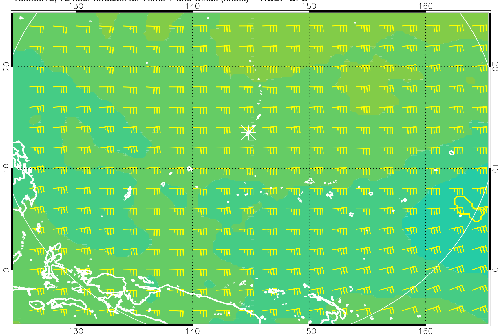
16090912, 72 hour forecast for 70mb T and winds (knots) -- NCEP GFS
