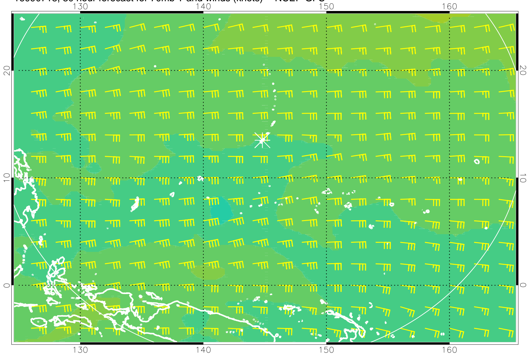
16090718, 30 hour forecast for 70mb T and winds (knots) -- NCEP GFS
