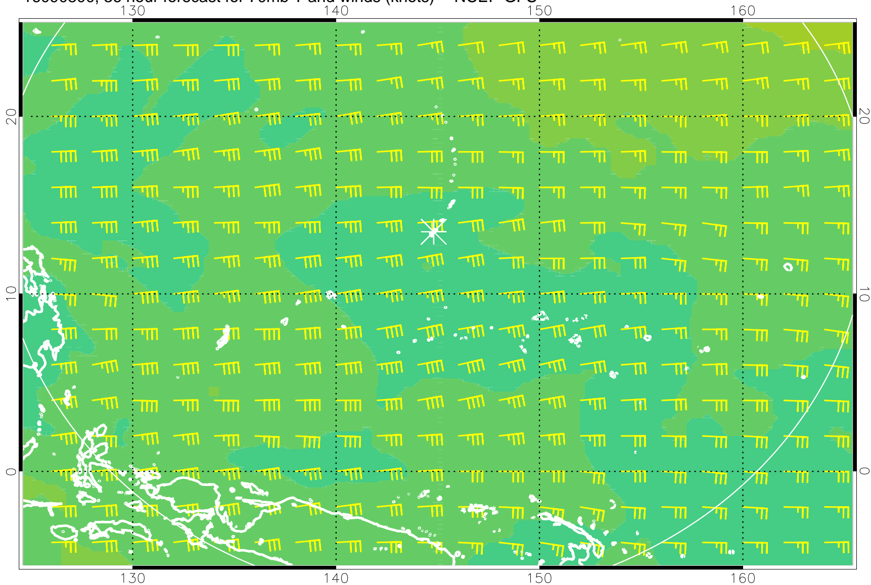
16090800, 36 hour forecast for 70mb T and winds (knots) -- NCEP GFS
