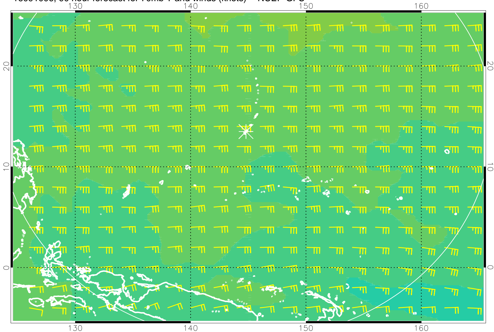
16091006, 90 hour forecast for 70mb T and winds (knots) -- NCEP GFS
