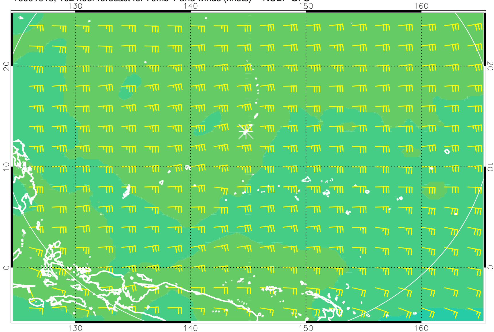
16091018, 102 hour forecast for 70mb T and winds (knots) -- NCEP GFS
