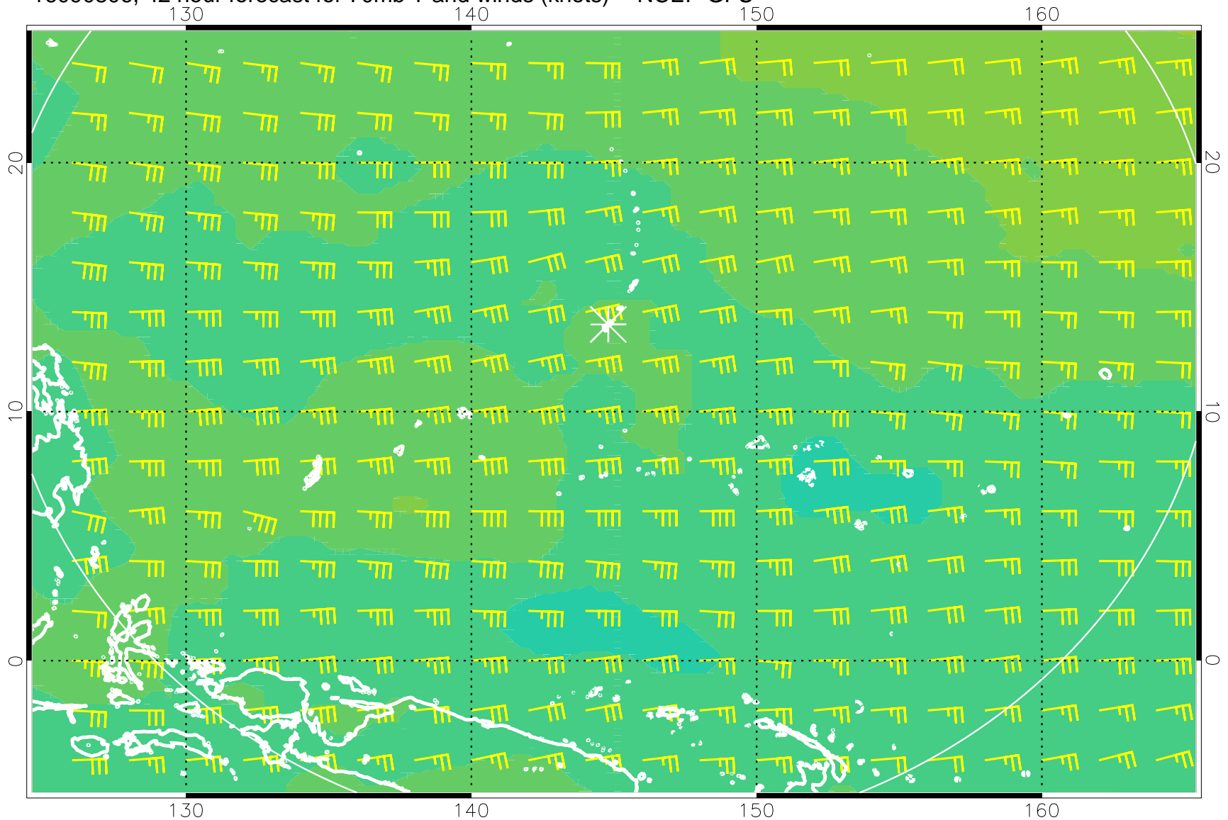
16090806, 42 hour forecast for 70mb T and winds (knots) -- NCEP GFS
