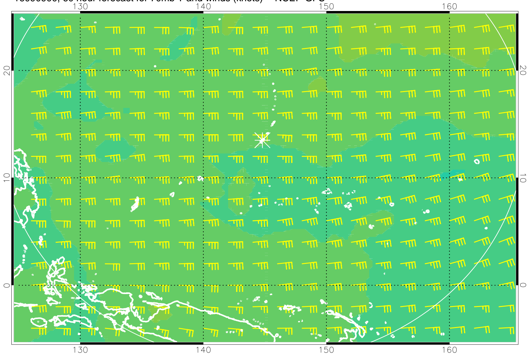
16090900, 60 hour forecast for 70mb T and winds (knots) -- NCEP GFS
