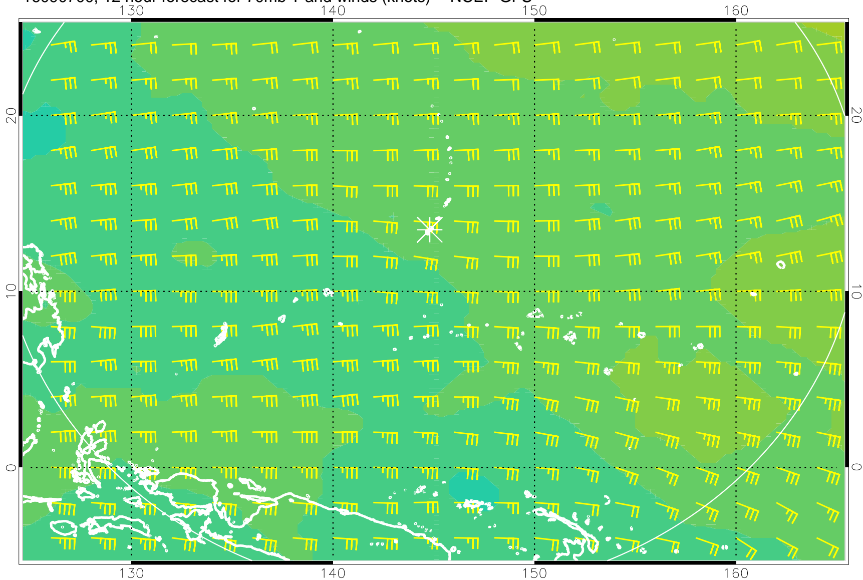
16090700, 12 hour forecast for 70mb T and winds (knots) -- NCEP GFS
